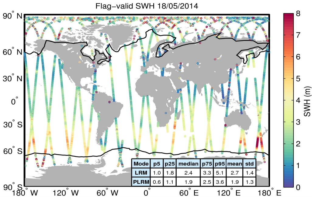
Figure 15. Geographical distribution of flag-valid SWH data over oceans and lakes for 18/05/2014. The statistical values shown in the table refer to the SWH in m and are calculated separately for LRM and PLRM regions. Measurements taken over polar regions have been excluded from the computation of the statistical values. The black lines mark the outer limit of the Arctic and Antarctic polar regions.
