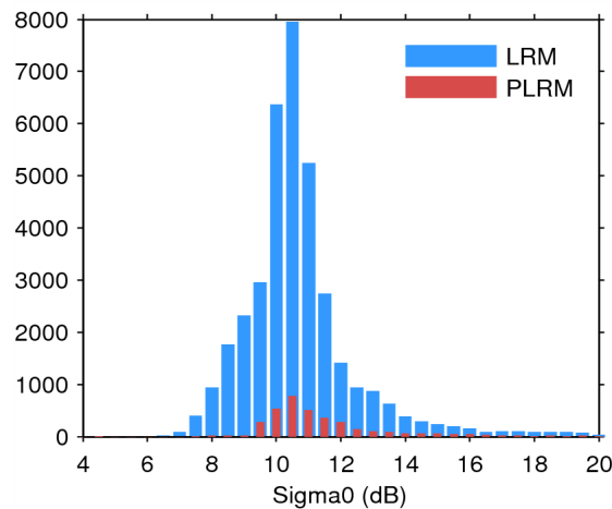
Figure 25. Histogram of flag-valid sigma0 over oceans and lakes for LRM (blue) and PLRM (red) for 18/05/2014.
