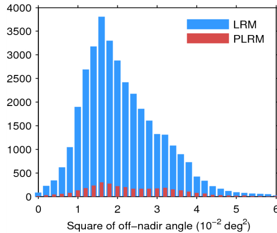
Figure 39. Histogram of flag-valid mispointing over oceans and lakes for LRM (blue) and PLRM (red) for 18/05/2014. Only positive values have been considered.
