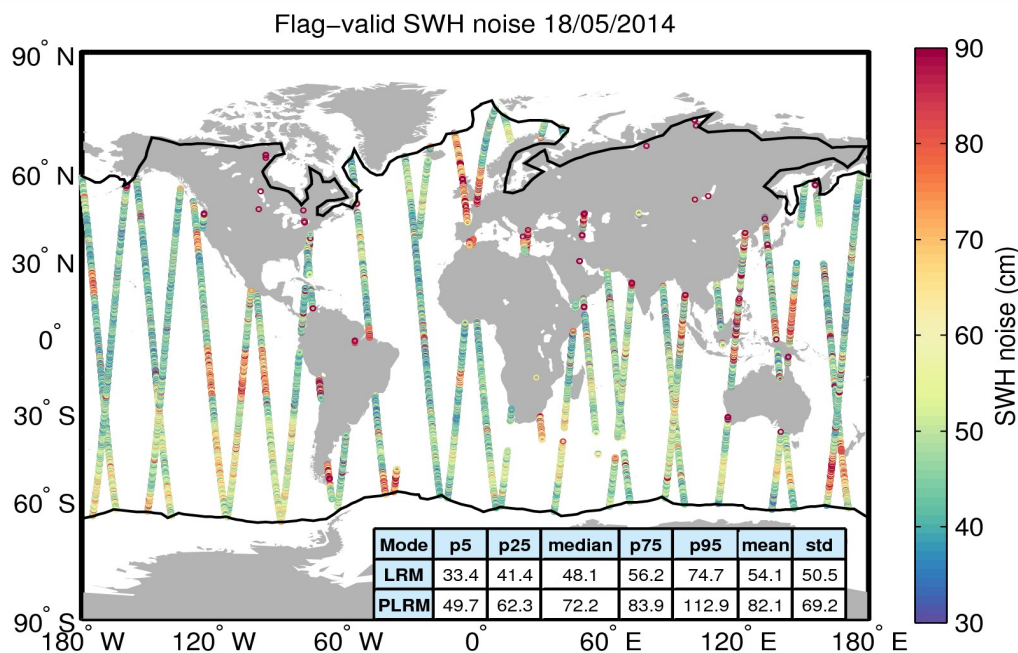
Figure 18. Geographical distribution of flag-valid 20-Hz SWH measurement noise over oceans and lakes for 18/05/2014. The statistical values shown in the table refer to the
