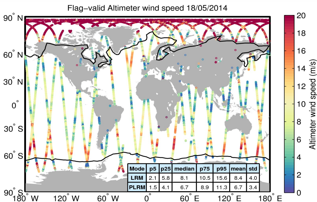
Figure 31. Geographical distribution of flag-valid wind data over oceans and lakes for 18/05/2014. The statistical values shown in the table refer to the wind in m/s and are calculated separately for LRM and PLRM regions. Measurements taken over polar regions have been excluded from the computation of the statistical values. The black lines mark the outer limit of the Arctic and Antarctic polar regions.
