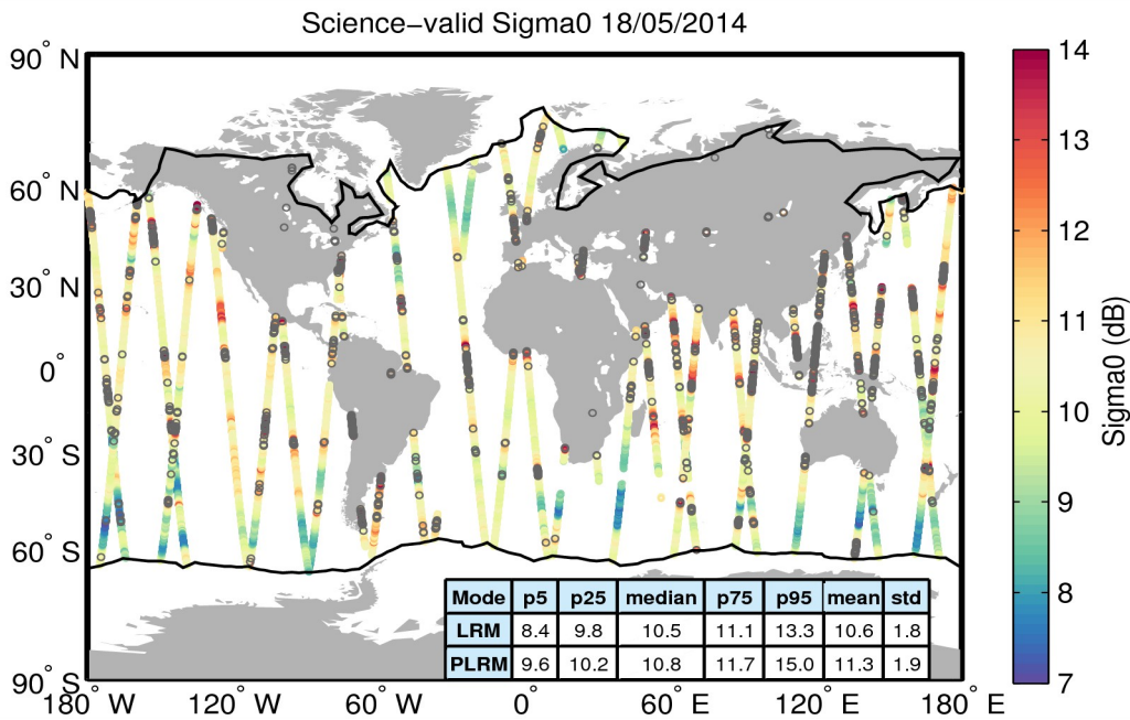
Figure 27. Geographical distribution of science-valid sigma0 data over oceans and lakes for 18/05/2014. The statistical values shown in the table refer to the sigma0 in dB and are calculated separately for LRM and PLRM regions. The black lines mark the outer limit of the Arctic and Antarctic polar regions. Gray circles denote records that have been rejected based on the editing criteria described in Table 4.
