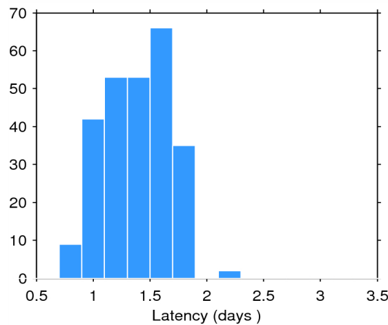
Figure 2. Histogram of the data latency for 18/05/2014.
