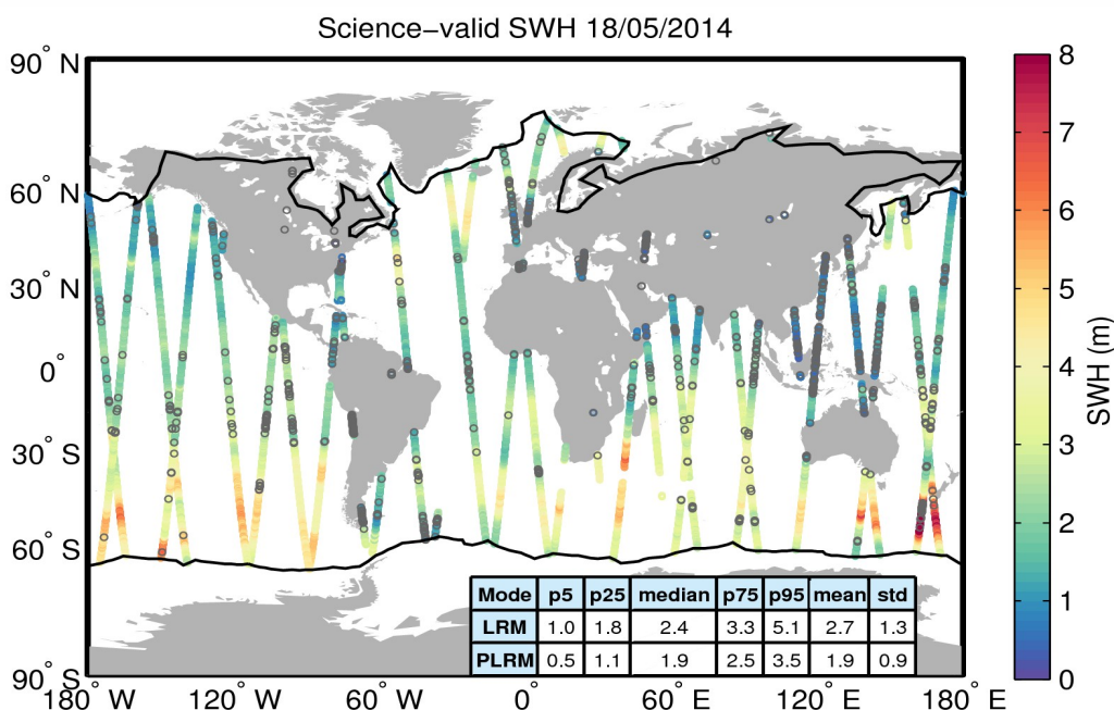
Figure 19. Geographical distribution of science-valid SWH data over oceans and lakes for 18/05/2014. The statistical values shown in the table refer to the SWH in m and are calculated separately for LRM and PLRM regions. The black lines mark the outer limit of the Arctic and Antarctic polar regions. Gray circles denote records that have been rejected based on the editing criteria described in Table 3.
