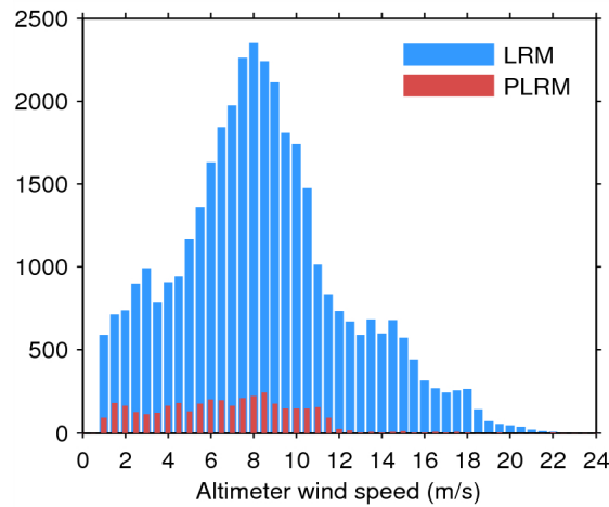
Figure 33. Histogram of flag-valid wind over oceans and lakes for LRM (blue) and PLRM (red) for 18/05/2014.
