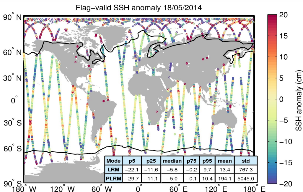
Figure 5. Geographical distribution of flag-valid SSH anomaly data over oceans and lakes for 18/05/2014. The statistical values shown in the table refer to the SSH anomaly in cm and are calculated separately for LRM and PLRM regions. Measurements taken over polar regions have been excluded from the computation of the statistical values. The black lines mark the outer limit of the Arctic and Antarctic polar regions.
