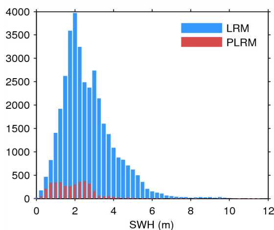
Figure 17. Histogram of flag-valid SWH over oceans and lakes for LRM (blue) and PLRM (red) for 18/05/2014.
