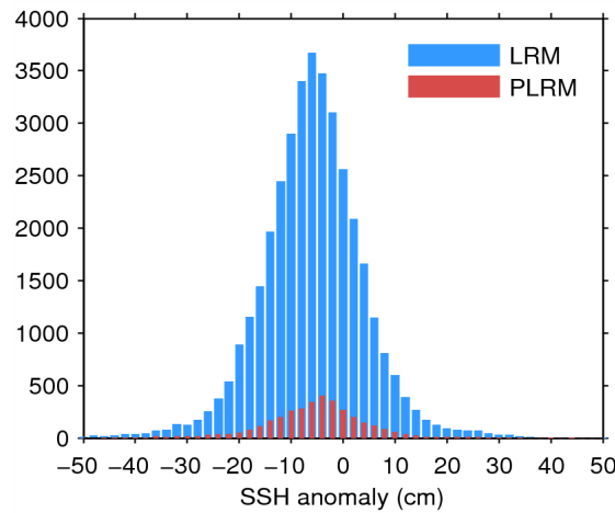
Figure 7. Histogram of flag-valid SSH anomaly over oceans and lakes for LRM (blue) and PLRM (red) for 18/05/2014.
