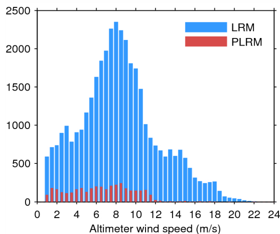
Figure 35. Histogram of science-valid wind over oceans and lakes for LRM (blue) and PLRM (red) for 18/05/2014.
