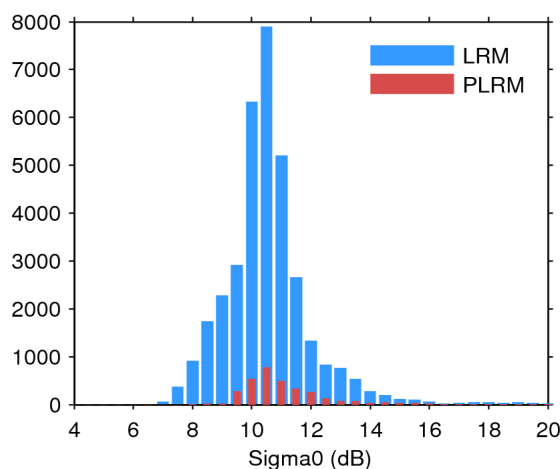
Figure 28. Histogram of science-valid sigma0 over oceans and lakes for LRM (blue) and PLRM (red) for 18/05/2014.
