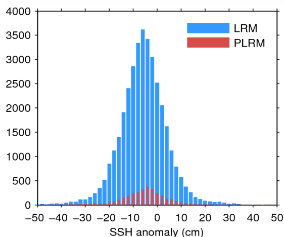
Figure 11. Histogram of science-valid SSH anomaly over oceans and lakes for LRM (blue) and PLRM (red) for 18/05/2014.
