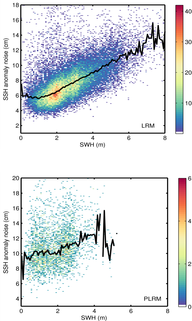
Figure 9. 2D histogram showing flag-valid SSH anomaly noise as a function of SWH for LRM (top) and PLRM (bottom) for 18/05/2014. The black line denotes the median SSH anomaly as a function of SWH.
