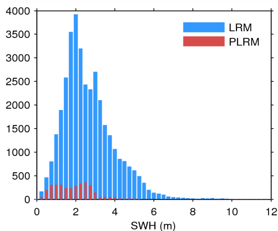
Figure 20. Histogram of science-valid SWH over oceans and lakes for LRM (blue) and PLRM (red) for 18/05/2014.
