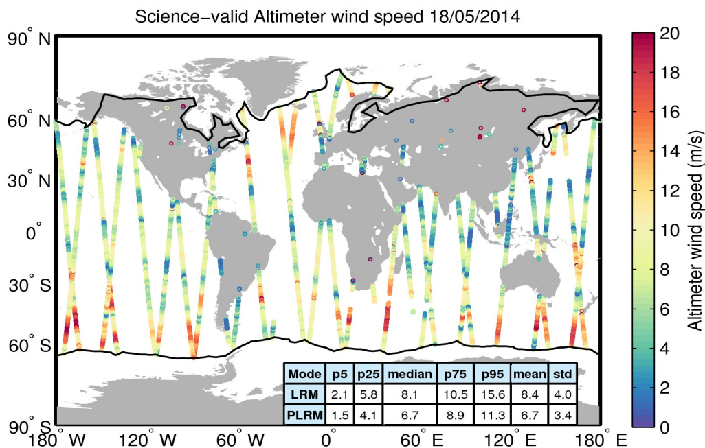
Figure 34. Geographical distribution of science-valid wind data over oceans and lakes for 18/05/2014. The statistical values shown in the table refer to the wind in m/s and are calculated separately for LRM and PLRM regions. The black lines mark the outer limit of the Arctic and Antarctic polar regions. Gray circles denote records that have been rejected based on the editing criteria described in Table 5.
