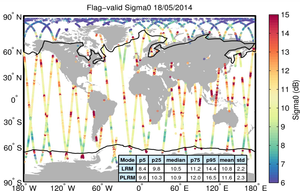
Figure 23. Geographical distribution of flag-valid sigma0 data over oceans and lakes for 18/05/2014. The statistical values shown in the table refer to the sigma0 in dB and are calculated separately for LRM and PLRM regions. Measurements taken over polar regions have been excluded from the computation of the statistical values. The black lines mark the outer limit of the Arctic and Antarctic polar regions.
