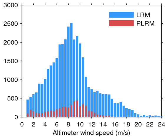
Figure 33. Histogram of flag-valid wind over oceans and lakes for LRM (blue) and PLRM (red) for 17/05/2014.
