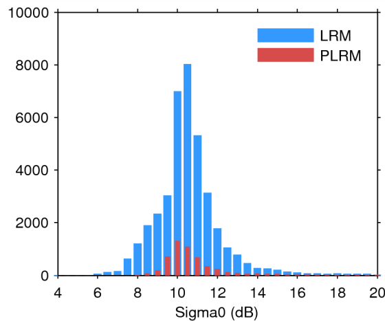
Figure 25. Histogram of flag-valid sigma0 over oceans and lakes for LRM (blue) and PLRM (red) for 17/05/2014.
