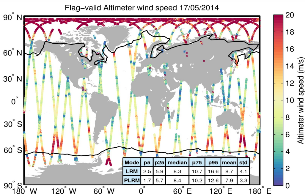
Figure 31. Geographical distribution of flag-valid wind data over oceans and lakes for 17/05/2014. The statistical values shown in the table refer to the wind in m/s and are calculated separately for LRM and PLRM regions. Measurements taken over polar regions have been excluded from the computation of the statistical values. The black lines mark the outer limit of the Arctic and Antarctic polar regions.
