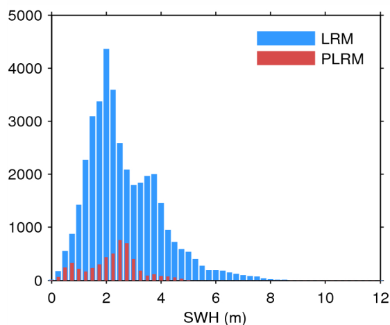
Figure 20. Histogram of science-valid SWH over oceans and lakes for LRM (blue) and PLRM (red) for 17/05/2014.
