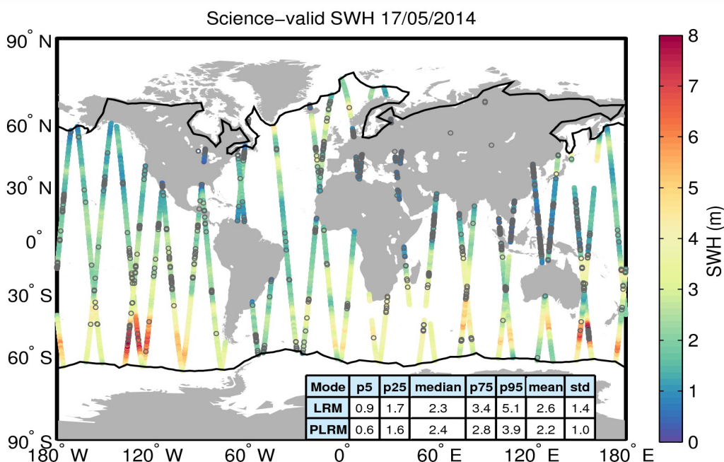
Figure 19. Geographical distribution of science-valid SWH data over oceans and lakes for 17/05/2014. The statistical values shown in the table refer to the SWH in m and are calculated separately for LRM and PLRM regions. The black lines mark the outer limit of the Arctic and Antarctic polar regions. Gray circles denote records that have been rejected based on the editing criteria described in Table 3.
