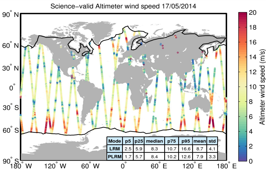
Figure 34. Geographical distribution of science-valid wind data over oceans and lakes for 17/05/2014. The statistical values shown in the table refer to the wind in m/s and are calculated separately for LRM and PLRM regions. The black lines mark the outer limit of the Arctic and Antarctic polar regions. Gray circles denote records that have been rejected based on the editing criteria described in Table 5.
