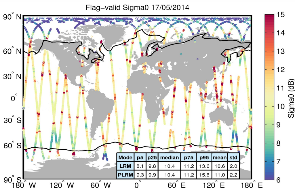
Figure 23. Geographical distribution of flag-valid sigma0 data over oceans and lakes for 17/05/2014. The statistical values shown in the table refer to the sigma0 in dB and are calculated separately for LRM and PLRM regions. Measurements taken over polar regions have been excluded from the computation of the statistical values. The black lines mark the outer limit of the Arctic and Antarctic polar regions.
