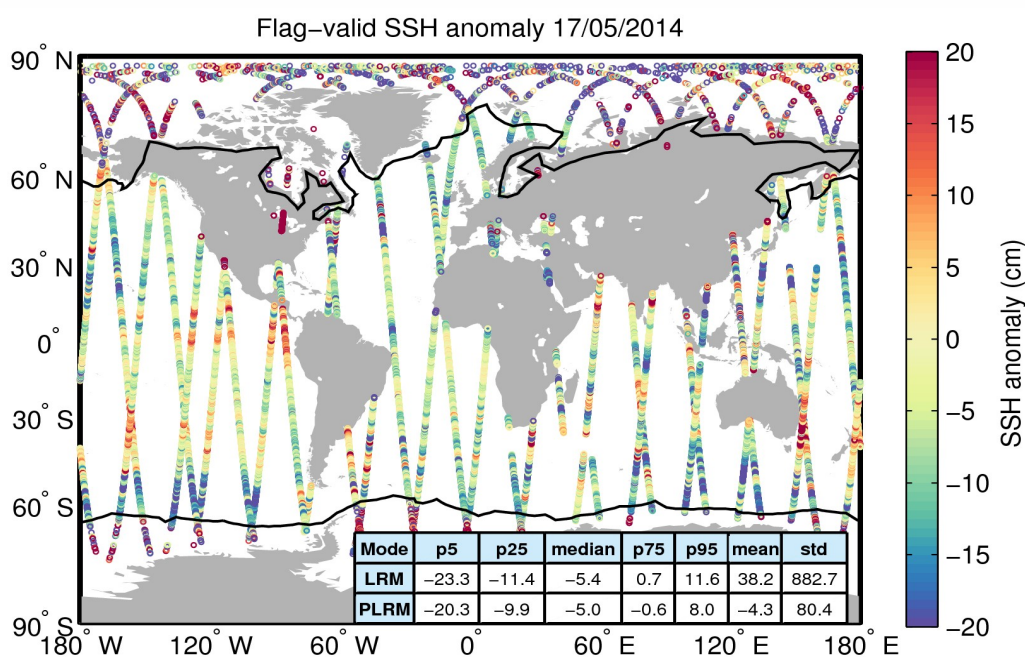
Figure 5. Geographical distribution of flag-valid SSH anomaly data over oceans and lakes for 17/05/2014. The statistical values shown in the table refer to the SSH anomaly in cm and are calculated separately for LRM and PLRM regions. Measurements taken over polar regions have been excluded from the computation of the statistical values. The black lines mark the outer limit of the Arctic and Antarctic polar regions.
