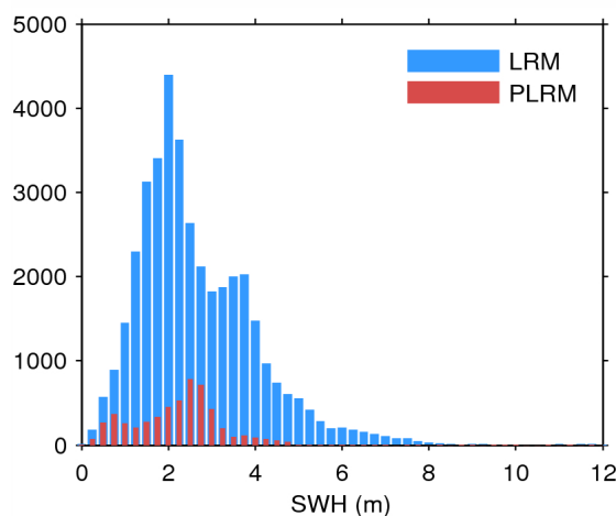
Figure 17. Histogram of flag-valid SWH over oceans and lakes for LRM (blue) and PLRM (red) for 17/05/2014.
