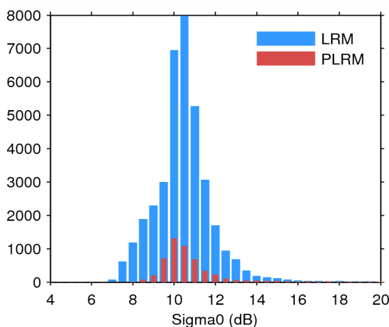
Figure 28. Histogram of science-valid sigma0 over oceans and lakes for LRM (blue) and PLRM (red) for 17/05/2014.
