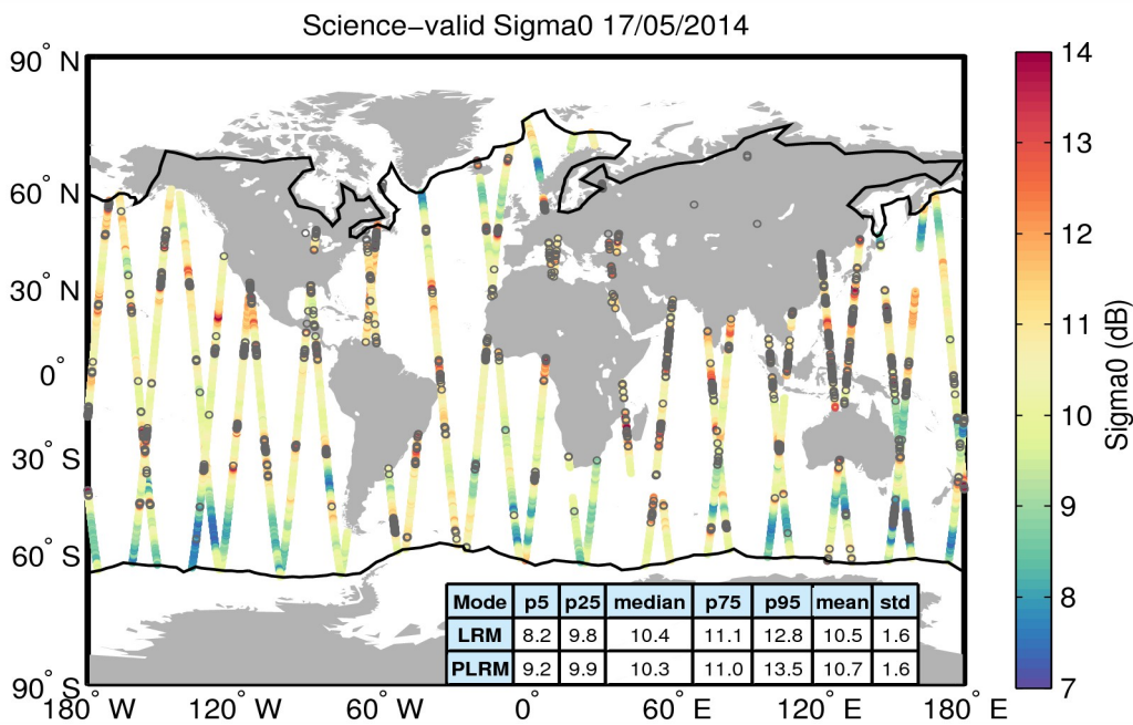
Figure 27. Geographical distribution of science-valid sigma0 data over oceans and lakes for 17/05/2014. The statistical values shown in the table refer to the sigma0 in dB and are calculated separately for LRM and PLRM regions. The black lines mark the outer limit of the Arctic and Antarctic polar regions. Gray circles denote records that have been rejected based on the editing criteria described in Table 4.
