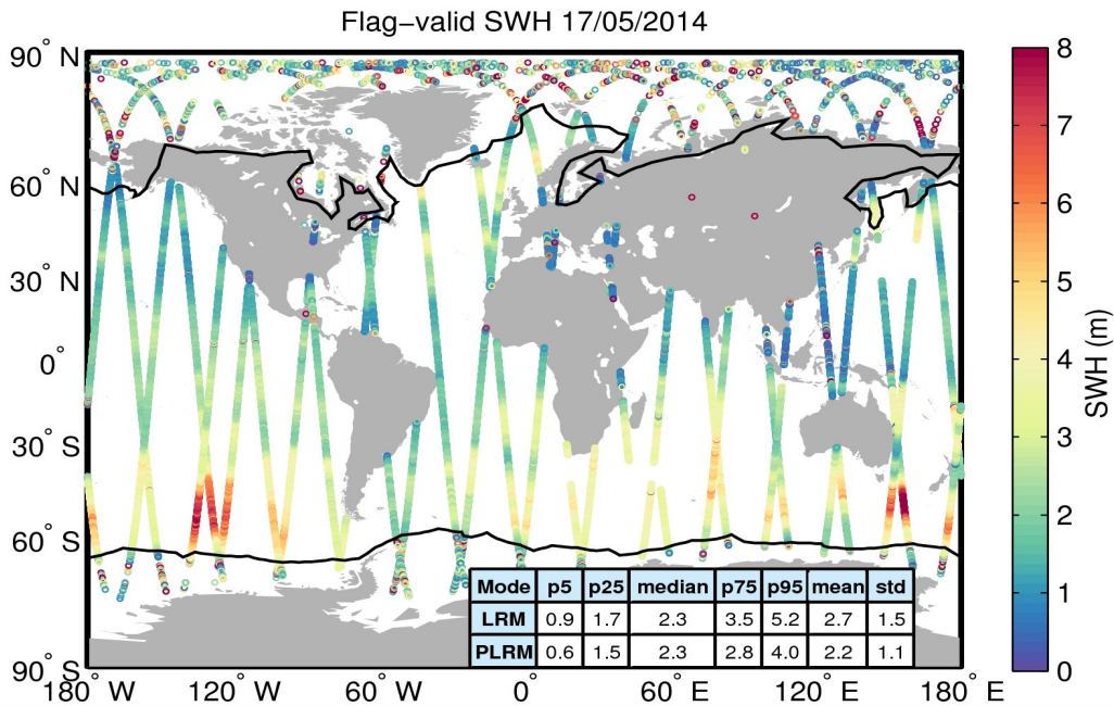
Figure 15. Geographical distribution of flag-valid SWH data over oceans and lakes for 17/05/2014. The statistical values shown in the table refer to the SWH in m and are calculated separately for LRM and PLRM regions. Measurements taken over polar regions have been excluded from the computation of the statistical values. The black lines mark the outer limit of the Arctic and Antarctic polar regions.
