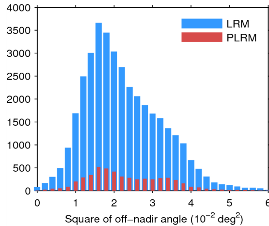
Figure 39. Histogram of flag-valid mispointing over oceans and lakes for LRM (blue) and PLRM (red) for 17/05/2014. Only positive values have been considered.
