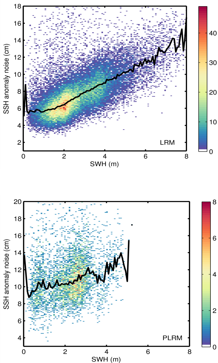
Figure 9. 2D histogram showing flag-valid SSH anomaly noise as a function of SWH for LRM (top) and PLRM (bottom) for 17/05/2014. The black line denotes the median SSH anomaly as a function of SWH.
