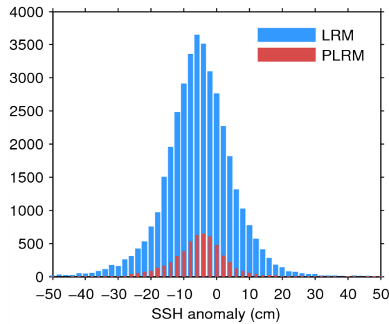
Figure 7. Histogram of flag-valid SSH anomaly over oceans and lakes for LRM (blue) and PLRM (red) for 17/05/2014.
