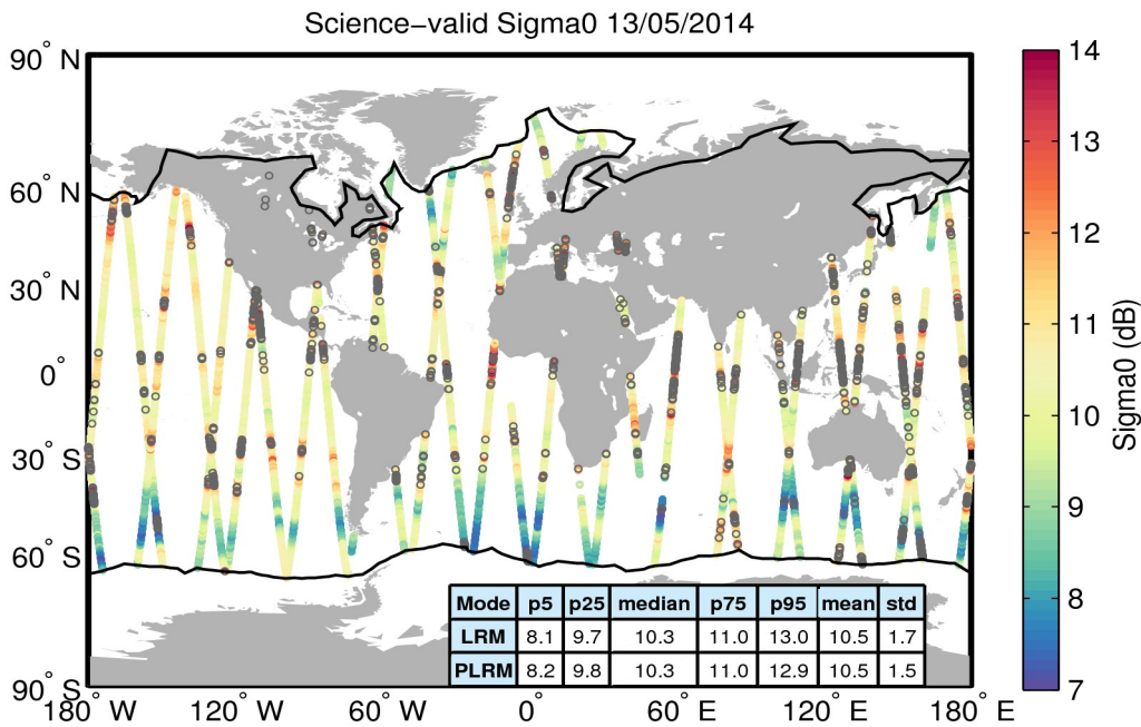
Figure 27. Geographical distribution of science-valid sigma0 data over oceans and lakes for 13/05/2014. The statistical values shown in the table refer to the sigma0 in dB and are calculated separately for LRM and PLRM regions. The black lines mark the outer limit of the Arctic and Antarctic polar regions. Gray circles denote records that have been rejected based on the editing criteria described in Table 4.
