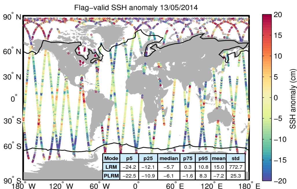
Figure 5. Geographical distribution of flag-valid SSH anomaly data over oceans and lakes for 13/05/2014. The statistical values shown in the table refer to the SSH anomaly in cm and are calculated separately for LRM and PLRM regions. Measurements taken over polar regions have been excluded from the computation of the statistical values. The black lines mark the outer limit of the Arctic and Antarctic polar regions.
