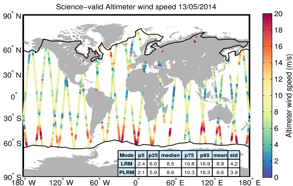
Figure 34. Geographical distribution of science-valid wind data over oceans and lakes for 13/05/2014. The statistical values shown in the table refer to the wind in m/s and are calculated separately for LRM and PLRM regions. The black lines mark the outer limit of the Arctic and Antarctic polar regions. Gray circles denote records that have been rejected based on the editing criteria described in Table 5.
