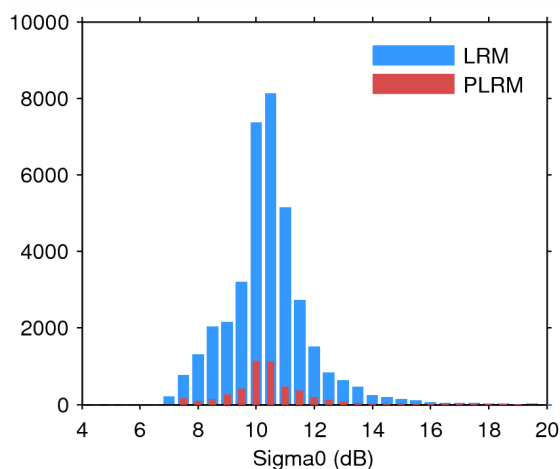
Figure 28. Histogram of science-valid sigma0 over oceans and lakes for LRM (blue) and PLRM (red) for 13/05/2014.
