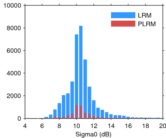
Figure 25. Histogram of flag-valid sigma0 over oceans and lakes for LRM (blue) and PLRM (red) for 13/05/2014.
