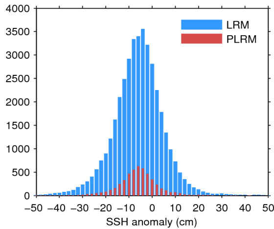
Figure 7. Histogram of flag-valid SSH anomaly over oceans and lakes for LRM (blue) and PLRM (red) for 13/05/2014.
