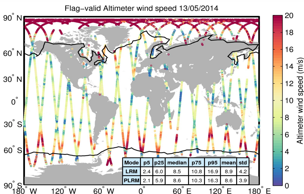
Figure 31. Geographical distribution of flag-valid wind data over oceans and lakes for 13/05/2014. The statistical values shown in the table refer to the wind in m/s and are calculated separately for LRM and PLRM regions. Measurements taken over polar regions have been excluded from the computation of the statistical values. The black lines mark the outer limit of the Arctic and Antarctic polar regions.
