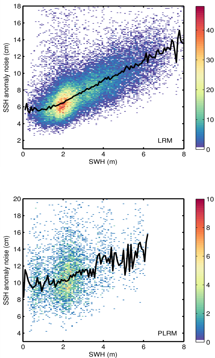
Figure 9. 2D histogram showing flag-valid SSH anomaly noise as a function of SWH for LRM (top) and PLRM (bottom) for 13/05/2014. The black line denotes the median SSH anomaly as a function of SWH.
