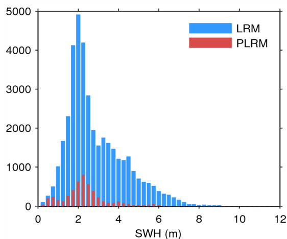
Figure 20. Histogram of science-valid SWH over oceans and lakes for LRM (blue) and PLRM (red) for 13/05/2014.
