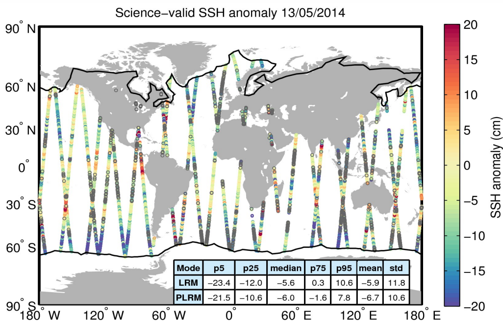
Figure 10. Geographical distribution of science-valid SSH anomaly data over oceans and lakes for 13/05/2014. The statistical values shown in the table refer to the SSH anomaly in cm and are calculated separately for LRM and PLRM regions. The black lines mark the outer limit of the Arctic and Antarctic polar regions. Gray circles denote records that have been rejected based on the editing criteria described in Table 2.
