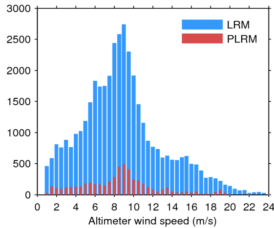
Figure 33. Histogram of flag-valid wind over oceans and lakes for LRM (blue) and PLRM (red) for 13/05/2014.
