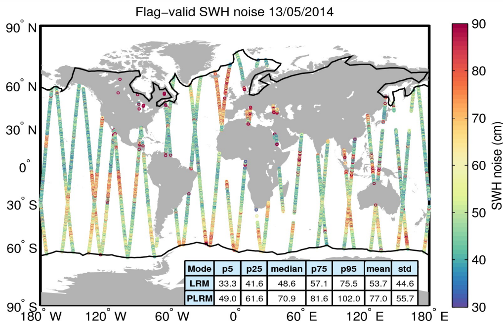
Figure 18. Geographical distribution of flag-valid 20-Hz SWH measurement noise over oceans and lakes for 13/05/2014. The statistical values shown in the table refer to the
