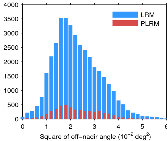
Figure 39. Histogram of flag-valid mispointing over oceans and lakes for LRM (blue) and PLRM (red) for 13/05/2014. Only positive values have been considered.
