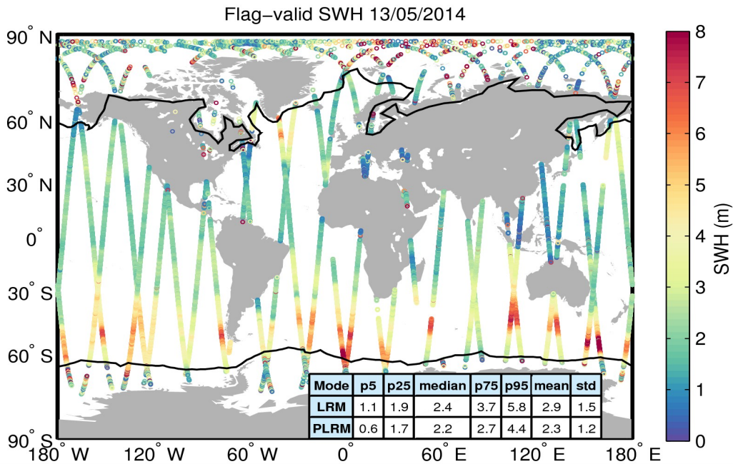
Figure 15. Geographical distribution of flag-valid SWH data over oceans and lakes for 13/05/2014. The statistical values shown in the table refer to the SWH in m and are calculated separately for LRM and PLRM regions. Measurements taken over polar regions have been excluded from the computation of the statistical values. The black lines mark the outer limit of the Arctic and Antarctic polar regions.
