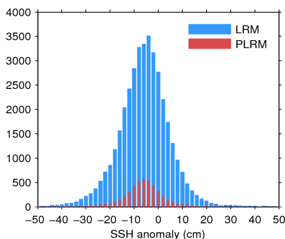
Figure 11. Histogram of science-valid SSH anomaly over oceans and lakes for LRM (blue) and PLRM (red) for 13/05/2014.
