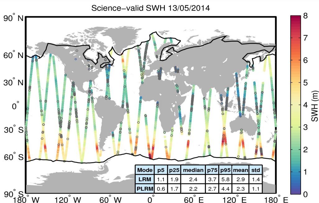
Figure 19. Geographical distribution of science-valid SWH data over oceans and lakes for 13/05/2014. The statistical values shown in the table refer to the SWH in m and are calculated separately for LRM and PLRM regions. The black lines mark the outer limit of the Arctic and Antarctic polar regions. Gray circles denote records that have been rejected based on the editing criteria described in Table 3.
