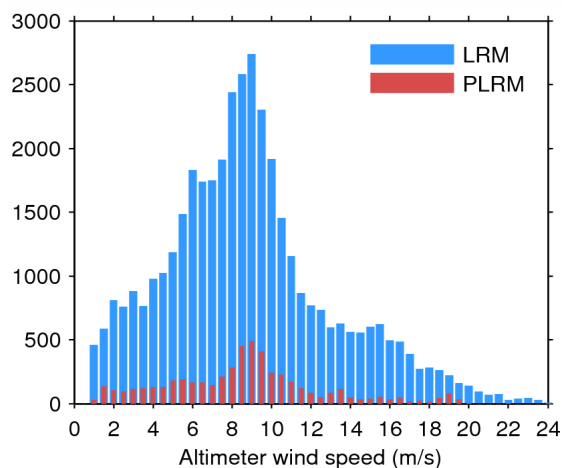
Figure 35. Histogram of science-valid wind over oceans and lakes for LRM (blue) and PLRM (red) for 13/05/2014.
