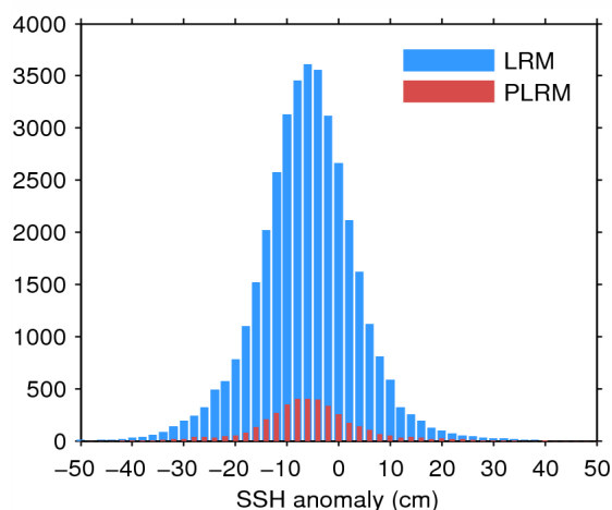
Figure 11. Histogram of science-valid SSH anomaly over oceans and lakes for LRM (blue) and PLRM (red) for 12/05/2014.
