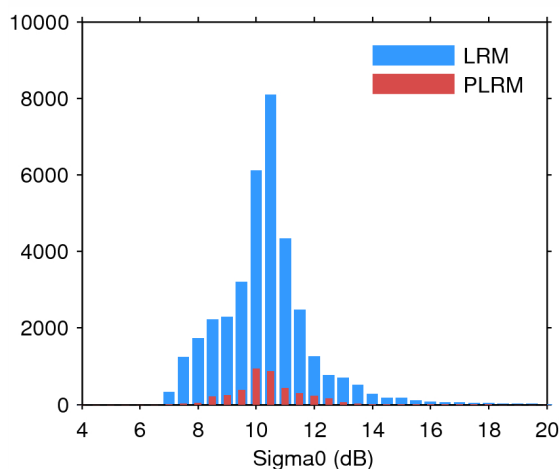
Figure 28. Histogram of science-valid sigma0 over oceans and lakes for LRM (blue) and PLRM (red) for 12/05/2014.
