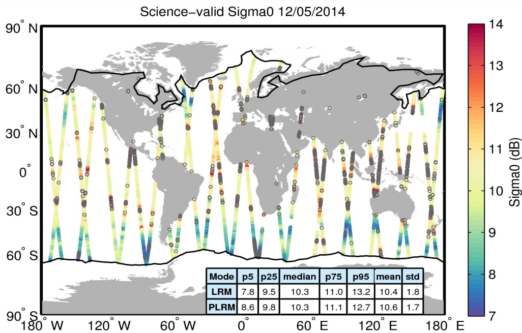
Figure 27. Geographical distribution of science-valid sigma0 data over oceans and lakes for 12/05/2014. The statistical values shown in the table refer to the sigma0 in dB and are calculated separately for LRM and PLRM regions. The black lines mark the outer limit of the Arctic and Antarctic polar regions. Gray circles denote records that have been rejected based on the editing criteria described in Table 4.
