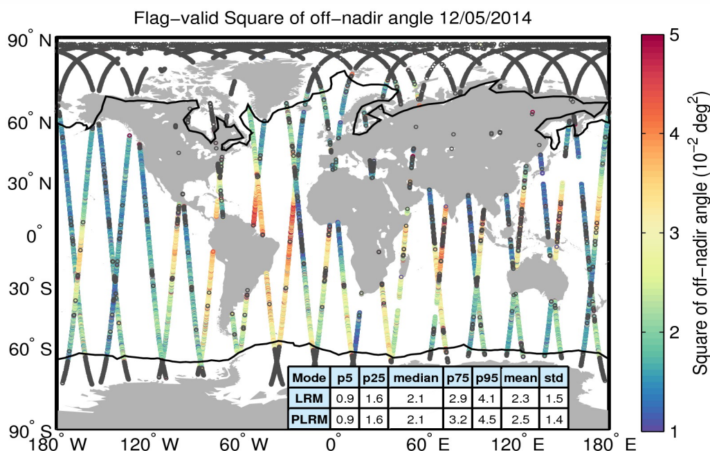
Figure 37. Geographical distribution of flag-valid mispointing data over oceans and lakes for 12/05/2014. The statistical values shown in the table refer to the mispointing in 10^{-2} \text{ deg}^2 and are calculated separately for LRM and PLRM regions. Measurements taken over polar regions have been excluded from the computation of the statistical values. The black lines mark the outer limit of the Arctic and Antarctic polar regions.
