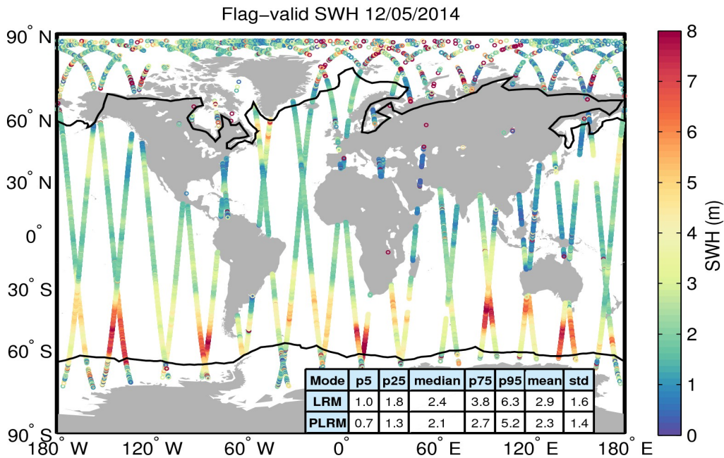
Figure 15. Geographical distribution of flag-valid SWH data over oceans and lakes for 12/05/2014. The statistical values shown in the table refer to the SWH in m and are calculated separately for LRM and PLRM regions. Measurements taken over polar regions have been excluded from the computation of the statistical values. The black lines mark the outer limit of the Arctic and Antarctic polar regions.
