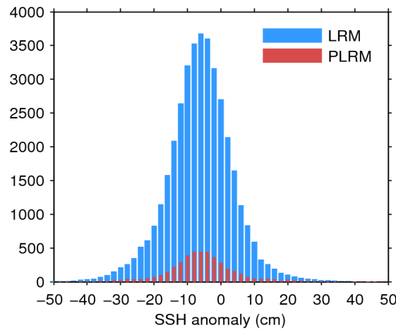
Figure 7. Histogram of flag-valid SSH anomaly over oceans and lakes for LRM (blue) and PLRM (red) for 12/05/2014.
