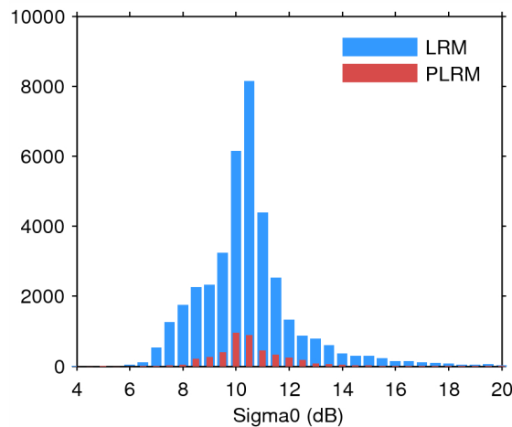
Figure 25. Histogram of flag-valid sigma0 over oceans and lakes for LRM (blue) and PLRM (red) for 12/05/2014.
