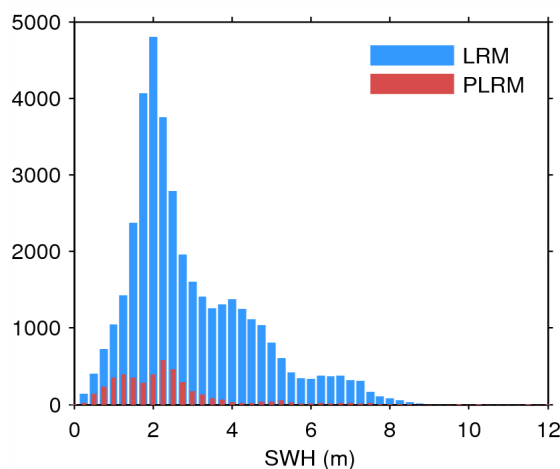
Figure 17. Histogram of flag-valid SWH over oceans and lakes for LRM (blue) and PLRM (red) for 12/05/2014.
