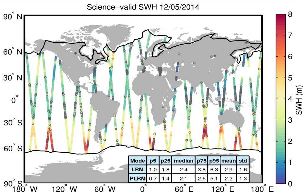
Figure 19. Geographical distribution of science-valid SWH data over oceans and lakes for 12/05/2014. The statistical values shown in the table refer to the SWH in m and are calculated separately for LRM and PLRM regions. The black lines mark the outer limit of the Arctic and Antarctic polar regions. Gray circles denote records that have been rejected based on the editing criteria described in Table 3.
