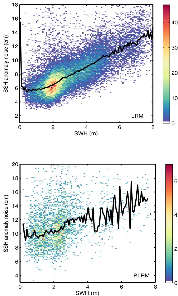
Figure 9. 2D histogram showing flag-valid SSH anomaly noise as a function of SWH for LRM (top) and PLRM (bottom) for 12/05/2014. The black line denotes the median SSH anomaly as a function of SWH.
