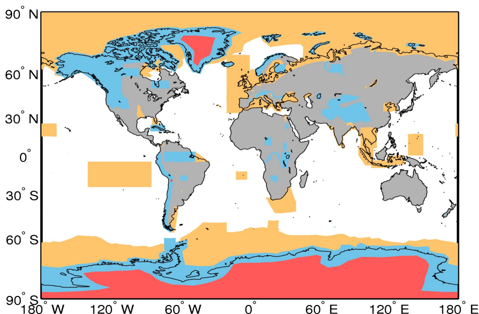
Figure A1. Extent of the regions defining the geographical mode mask for 12/05/2014. The regions where SAR, and SARIn are operated are denoted by the orange and blue polygons, respectively. LRM is operated over areas of the continental ice sheets (red polygons) and over oceans and land not covered by other modes.
