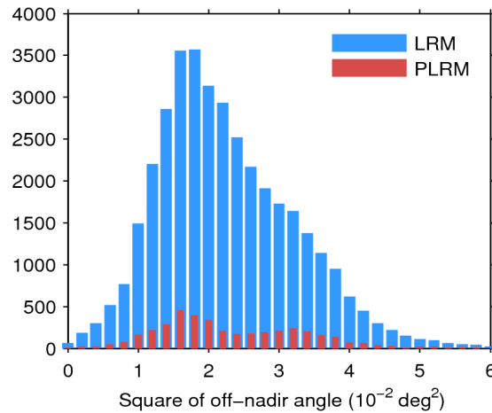
Figure 39. Histogram of flag-valid mispointing over oceans and lakes for LRM (blue) and PLRM (red) for 12/05/2014. Only positive values have been considered.
