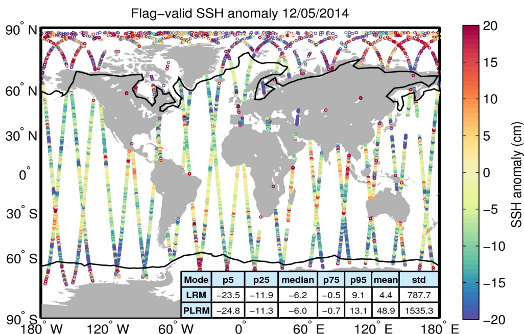
Figure 5. Geographical distribution of flag-valid SSH anomaly data over oceans and lakes for 12/05/2014. The statistical values shown in the table refer to the SSH anomaly in cm and are calculated separately for LRM and PLRM regions. Measurements taken over polar regions have been excluded from the computation of the statistical values. The black lines mark the outer limit of the Arctic and Antarctic polar regions.
