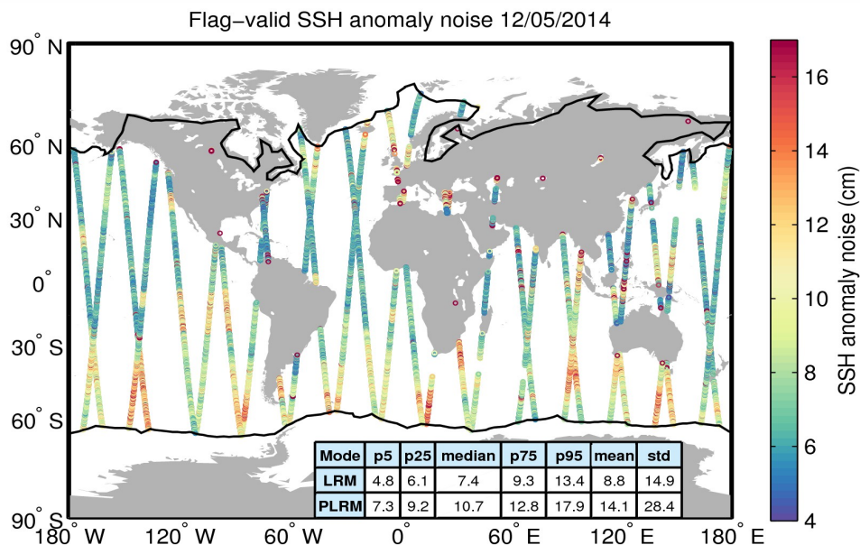
Figure 8. Geographical distribution of flag-valid 20-Hz SSH anomaly measurement noise over oceans and lakes for 12/05/2014. The statistical values shown in the table refer to the SSH anomaly noise and are calculated separately for LRM and PLRM regions. Measurements taken over polar regions have been excluded from the computation of the
