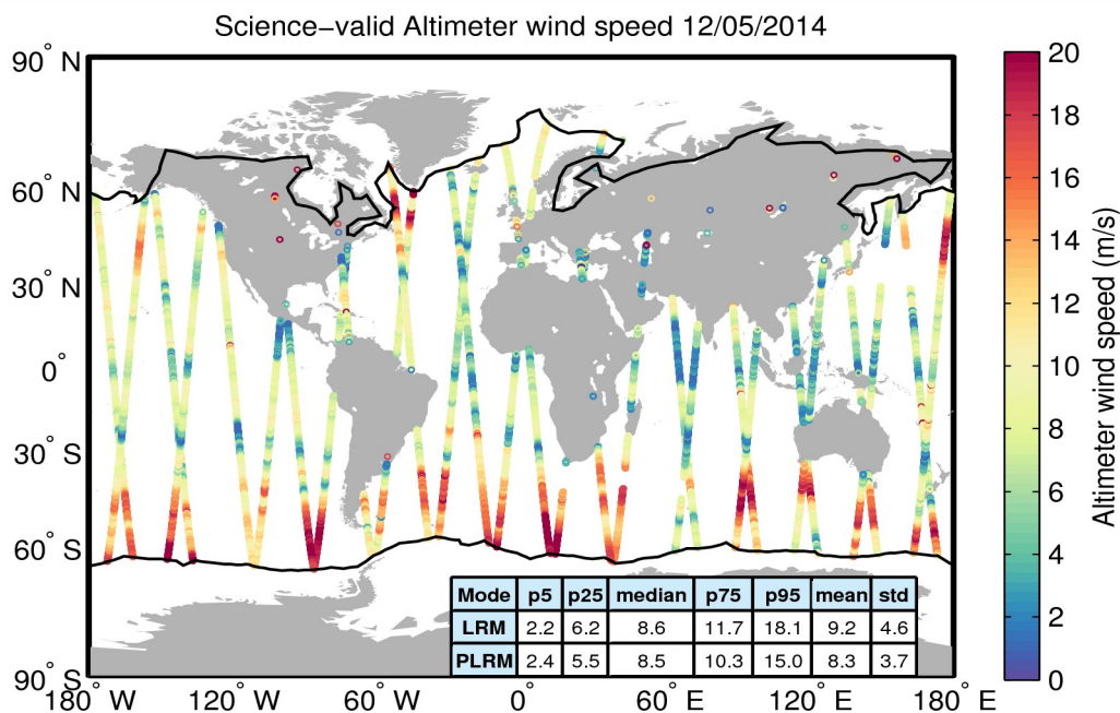
Figure 34. Geographical distribution of science-valid wind data over oceans and lakes for 12/05/2014. The statistical values shown in the table refer to the wind in m/s and are calculated separately for LRM and PLRM regions. The black lines mark the outer limit of the Arctic and Antarctic polar regions. Gray circles denote records that have been rejected based on the editing criteria described in Table 5.
