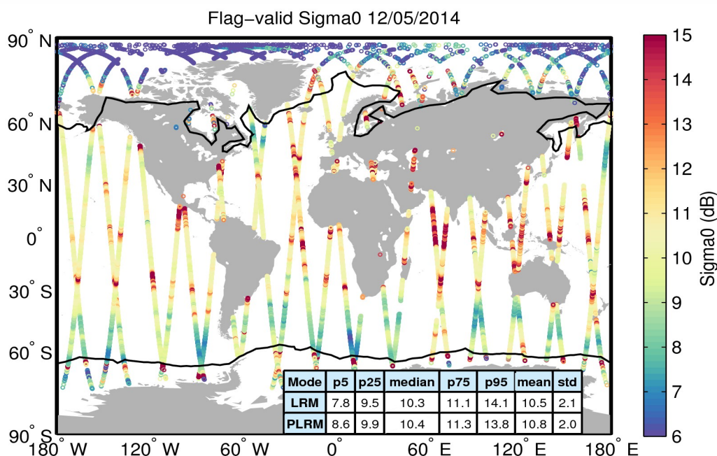
Figure 23. Geographical distribution of flag-valid sigma0 data over oceans and lakes for 12/05/2014. The statistical values shown in the table refer to the sigma0 in dB and are calculated separately for LRM and PLRM regions. Measurements taken over polar regions have been excluded from the computation of the statistical values. The black lines mark the outer limit of the Arctic and Antarctic polar regions.
