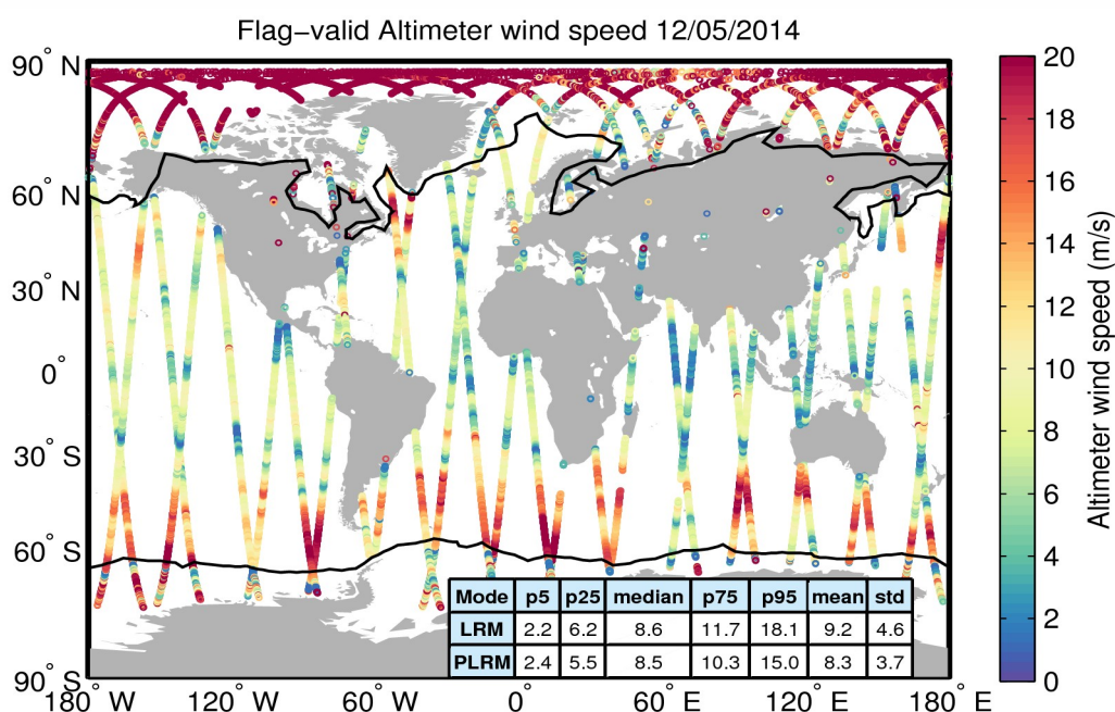
Figure 31. Geographical distribution of flag-valid wind data over oceans and lakes for 12/05/2014. The statistical values shown in the table refer to the wind in m/s and are calculated separately for LRM and PLRM regions. Measurements taken over polar regions have been excluded from the computation of the statistical values. The black lines mark the outer limit of the Arctic and Antarctic polar regions.
