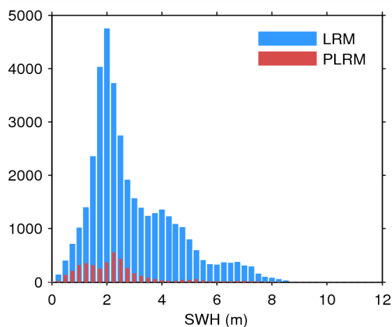
Figure 20. Histogram of science-valid SWH over oceans and lakes for LRM (blue) and PLRM (red) for 12/05/2014.
