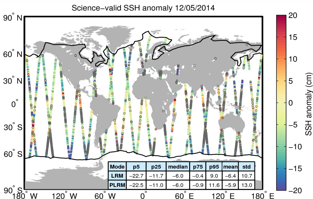
Figure 10. Geographical distribution of science-valid SSH anomaly data over oceans and lakes for 12/05/2014. The statistical values shown in the table refer to the SSH anomaly in cm and are calculated separately for LRM and PLRM regions. The black lines mark the outer limit of the Arctic and Antarctic polar regions. Gray circles denote records that have been rejected based on the editing criteria described in Table 2.
