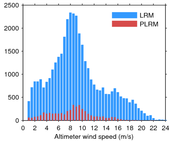
Figure 33. Histogram of flag-valid wind over oceans and lakes for LRM (blue) and PLRM (red) for 12/05/2014.
