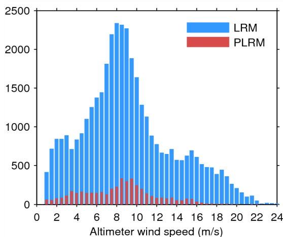
Figure 35. Histogram of science-valid wind over oceans and lakes for LRM (blue) and PLRM (red) for 12/05/2014.
