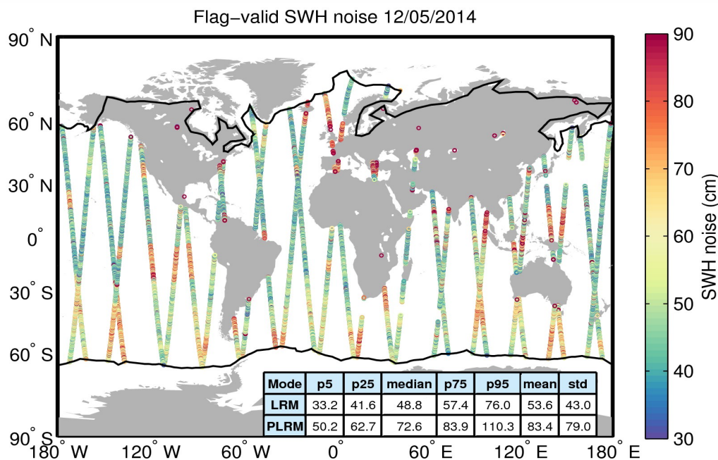
Figure 18. Geographical distribution of flag-valid 20-Hz SWH measurement noise over oceans and lakes for 12/05/2014. The statistical values shown in the table refer to the
