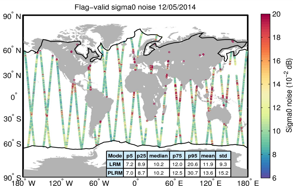
Figure 26. Geographical distribution of flag-valid 20-Hz sigma0 measurement noise over oceans and lakes for 12/05/2014. The statistical values shown in the table refer to the sigma0 noise and are calculated separately for LRM and PLRM regions. Measurements taken over polar regions have been excluded from the computation of the statistical values. The black lines mark the outer limit of the Arctic and Antarctic polar regions.
