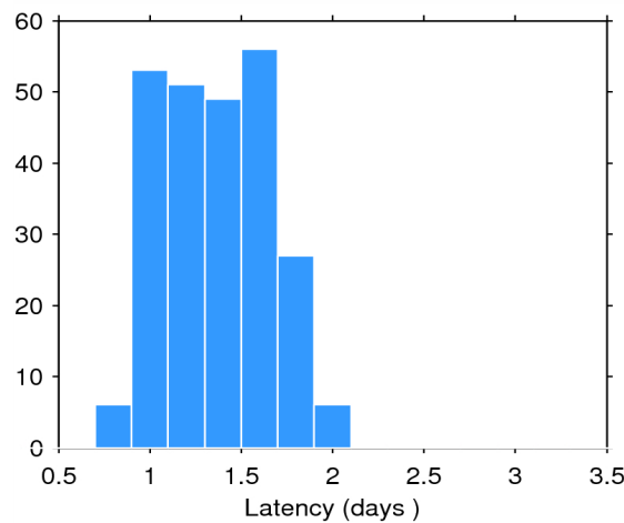
Figure 2. Histogram of the data latency for 12/05/2014.
