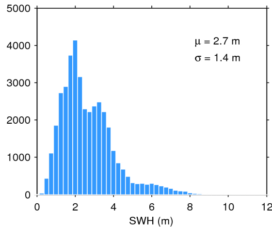
Figure 20. Histogram of science-valid SWH over oceans and lakes for 18/08/2020. The mean ( \mu ) and standard deviation ( \sigma ) are also shown. Note that values larger than 12 m are excluded from the histogram for the sake of readability but not from the computation of \mu and \sigma .
