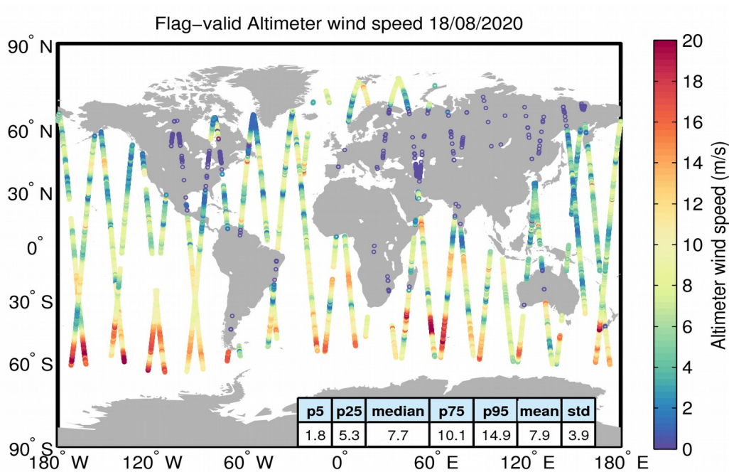
Figure 31. Geographical distribution of flag-valid wind data over oceans and lakes for 18/08/2020. The statistical values shown in the table refer to the wind in m/s and are calculated over all measurements shown in the figure.
