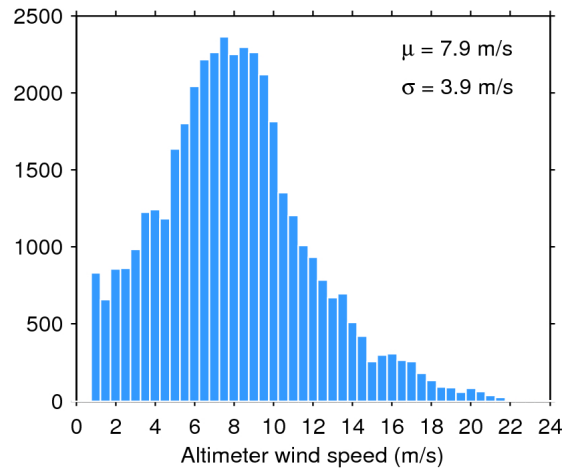
Figure 33. Histogram of flag-valid wind over oceans and lakes for 18/08/2020. The mean ( \mu ) and standard deviation ( \sigma ) are also shown. Note that values larger than 24 m/s are excluded from the histogram for the sake of readability but not from the computation of \mu and \sigma .
