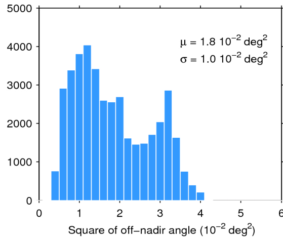
Figure 39. Histogram of flag-valid mispointing over oceans and lakes for 18/08/2020. The mean ( \mu ) and standard deviation ( \sigma ) are also shown. Note that values larger than 6 \cdot 10^{-2} \text{ deg}^2 are excluded from the histogram for the sake of readability but not from the computation of \mu and \sigma .
