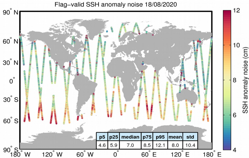
Figure 8. Geographical distribution of flag-valid 20-Hz SSH anomaly measurement noise over oceans and lakes for 18/08/2020. The statistical values shown in the table refer to the SSH anomaly noise and are calculated over all measurements shown in the figure.
