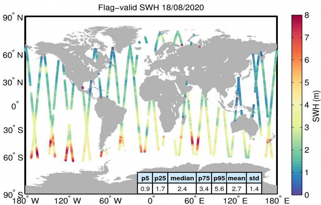
Figure 15. Geographical distribution of flag-valid SWH data over oceans and lakes for 18/08/2020. The statistical values shown in the table refer to the SWH in m and are calculated over all measurements shown in the figure.
