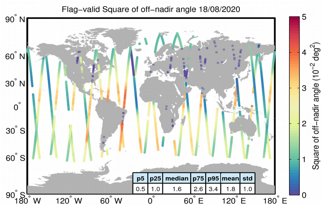
Figure 37. Geographical distribution of flag-valid mispointing data over oceans and lakes for 18/08/2020. The statistical values shown in the table refer to the mispointing in 10^{-2} \text{ deg}^2 and are calculated over all measurements shown in the figure.
