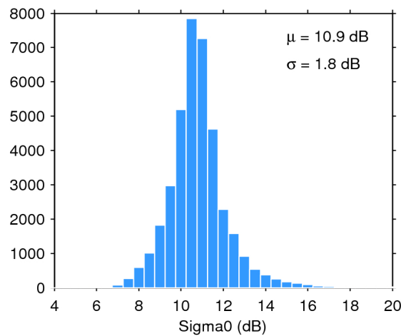
Figure 28. Histogram of science-valid sigma0 over oceans and lakes for 18/08/2020. The mean ( \mu ) and standard deviation ( \sigma ) are also shown. Note that values outside [4 20] dB are excluded from the histogram for the sake of readability but not from the computation of \mu and \sigma .
