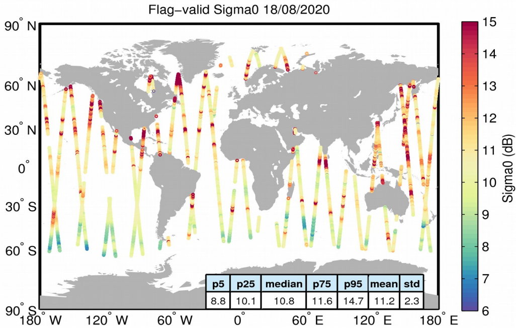
Figure 23. Geographical distribution of flag-valid sigma0 data over oceans and lakes for 18/08/2020. The statistical values shown in the table refer to the sigma0 in dB and are calculated over all measurements shown in the figure.
