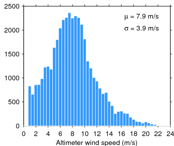
Figure 35. Histogram of science-valid wind over oceans and lakes for 18/08/2020. The mean ( \mu ) and standard deviation ( \sigma ) are also shown. Note that values larger than 24 m/s are excluded from the histogram for the sake of readability but not from the computation of \mu and \sigma .
