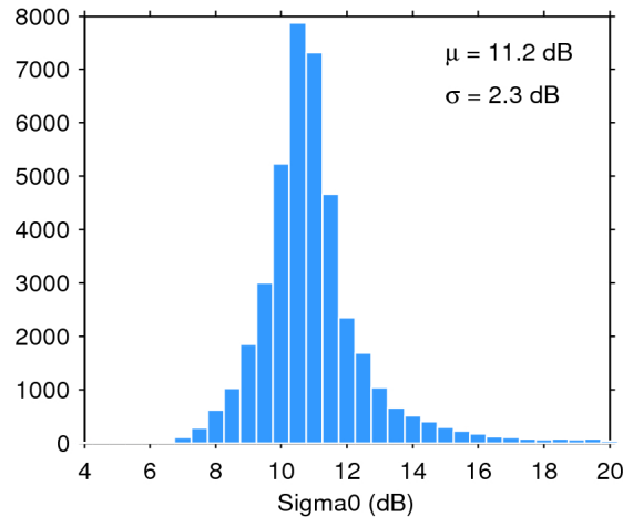
Figure 25. Histogram of flag-valid sigma0 over oceans and lakes for 18/08/2020. The mean ( \mu ) and standard deviation ( \sigma ) are also shown. Note that values outside [4 20] dB are excluded from the histogram for the sake of readability but not from the computation of \mu and \sigma .
