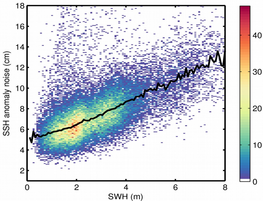
Figure 9. 2D histogram showing flag-valid SSH anomaly noise as a function of SWH for 18/08/2020. The black line denotes the median SSH anomaly noise as a function of SWH.
