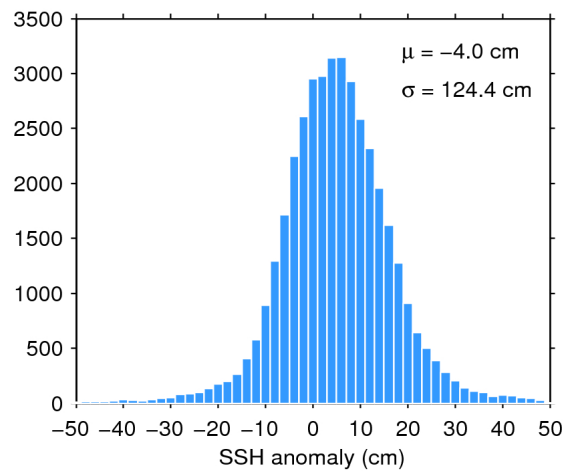
Figure 7. Histogram of flag-valid SSH anomaly over oceans and lakes for 18/08/2020. The mean ( \mu ) and standard deviation ( \sigma ) are also shown. Note that values outside [-50 50] cm are excluded from the histogram for the sake of readability but not from the computation of \mu and \sigma .
