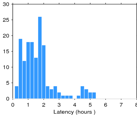
Figure 2. Histogram of the data latency for 18/08/2020. The y-axis denotes the number of files that are made available with a delay of x-hours with respect to the mean time of the records stored in the file.
