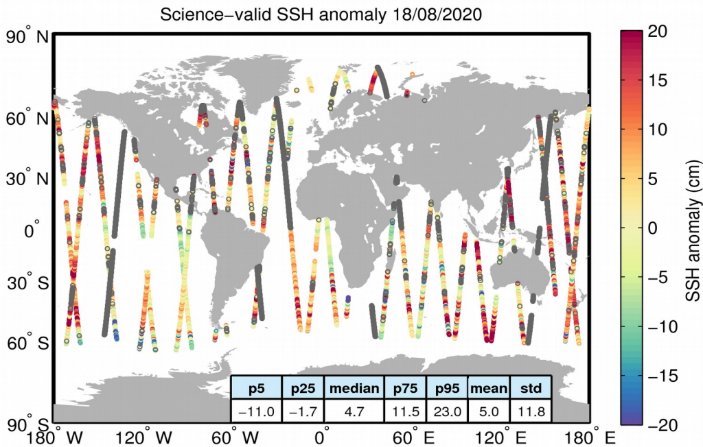
Figure 10. Geographical distribution of science-valid SSH anomaly data over oceans and lakes for 18/08/2020. The statistical values shown in the table refer to the SSH anomaly in cm and are calculated over all measurements shown in the figure. Gray circles denote records that have been rejected based on the editing criteria described in Table 2.
