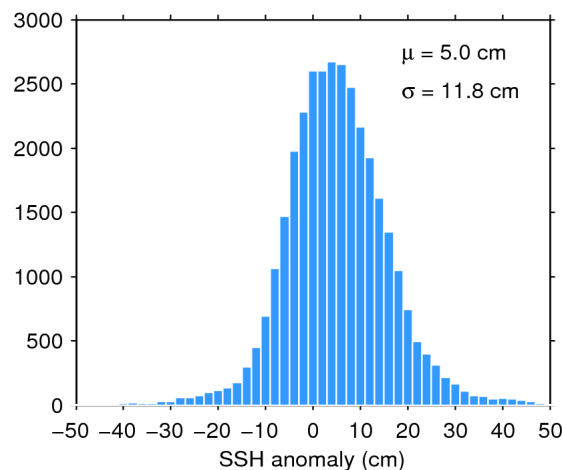
Figure 11. Histogram of science-valid SSH anomaly over oceans and lakes for 18/08/2020. The mean ( \mu ) and standard deviation ( \sigma ) are also shown. Note that values outside [-50 50] cm are excluded from the histogram for the sake of readability but not from the computation of \mu and \sigma .
