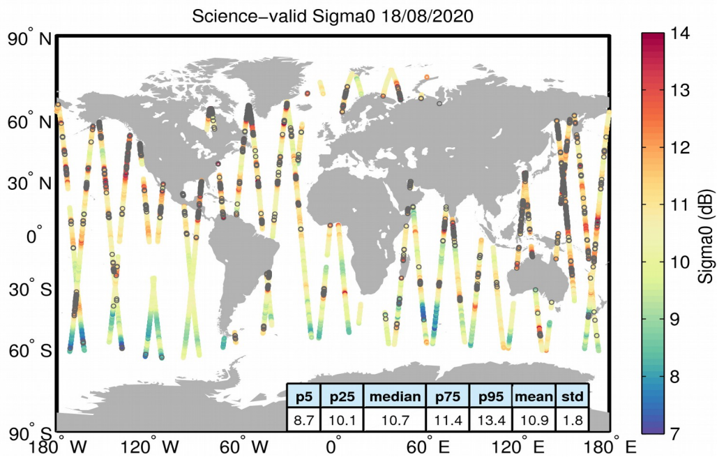
Figure 27. Geographical distribution of science-valid sigma0 data over oceans and lakes for 18/08/2020. The statistical values shown in the table refer to the sigma0 in dB and are calculated over all measurements shown in the figure. Gray circles denote records that have been rejected based on the editing criteria described in Table 4.
