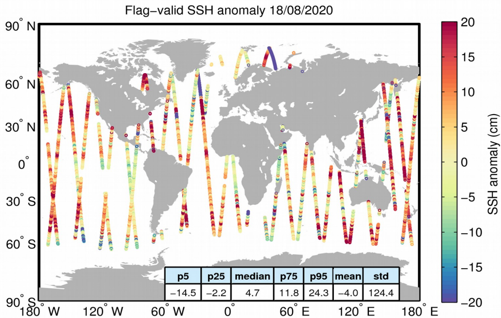
Figure 5. Geographical distribution of flag-valid 1-Hz SSH anomaly data over oceans and lakes for 18/08/2020. The statistical values shown in the table refer to the SSH anomaly in cm and are calculated over all measurements shown in the figure.
