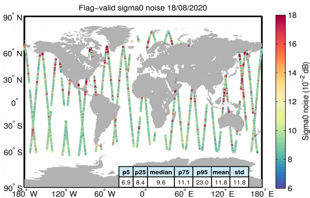
Figure 26. Geographical distribution of flag-valid 20-Hz sigma0 measurement noise over oceans and lakes for 18/08/2020. The statistical values shown in the table refer to the sigma0 noise and are calculated over all measurements shown in the figure.
