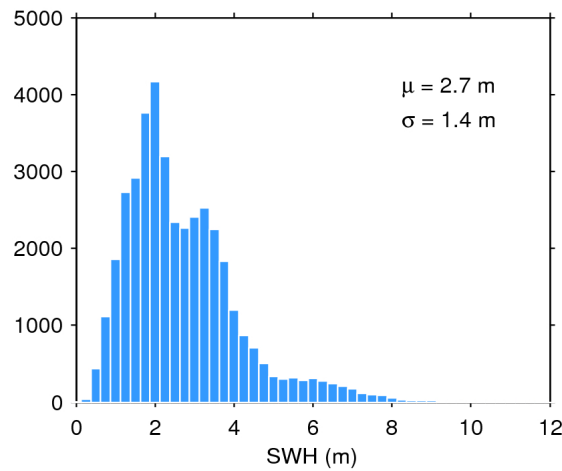
Figure 17. Histogram of flag-valid SWH over oceans and lakes for 18/08/2020. The mean ( \mu ) and standard deviation ( \sigma ) are also shown. Note that values larger than 12 m are excluded from the histogram for the sake of readability but not from the computation of \mu and \sigma .
