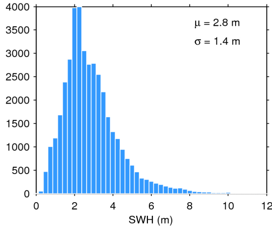
Figure 20. Histogram of science-valid SWH over oceans and lakes for 17/08/2020. The mean ( \mu ) and standard deviation ( \sigma ) are also shown. Note that values larger than 12 m are excluded from the histogram for the sake of readability but not from the computation of \mu and \sigma .
