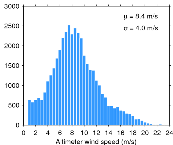
Figure 35. Histogram of science-valid wind over oceans and lakes for 17/08/2020. The mean ( \mu ) and standard deviation ( \sigma ) are also shown. Note that values larger than 24 m/s are excluded from the histogram for the sake of readability but not from the computation of \mu and \sigma .
