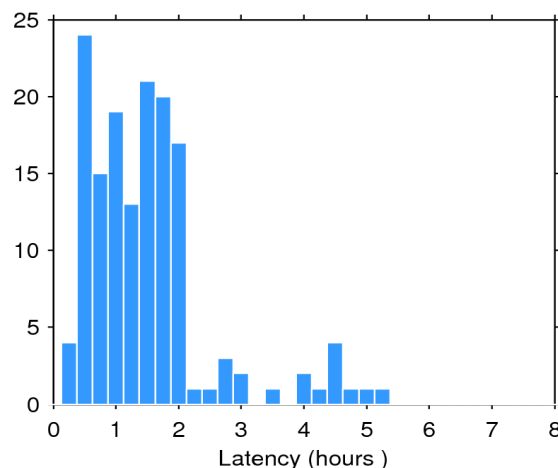
Figure 2. Histogram of the data latency for 17/08/2020. The y-axis denotes the number of files that are made available with a delay of x-hours with respect to the mean time of the records stored in the file.
