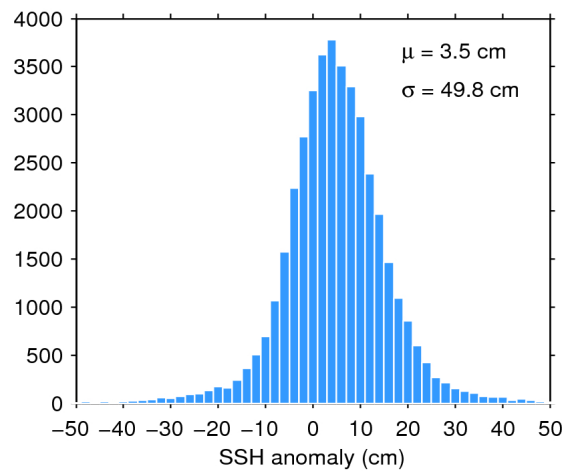
Figure 7. Histogram of flag-valid SSH anomaly over oceans and lakes for 17/08/2020. The mean ( \mu ) and standard deviation ( \sigma ) are also shown. Note that values outside [-50\ 50] cm are excluded from the histogram for the sake of readability but not from the computation of \mu and \sigma .
