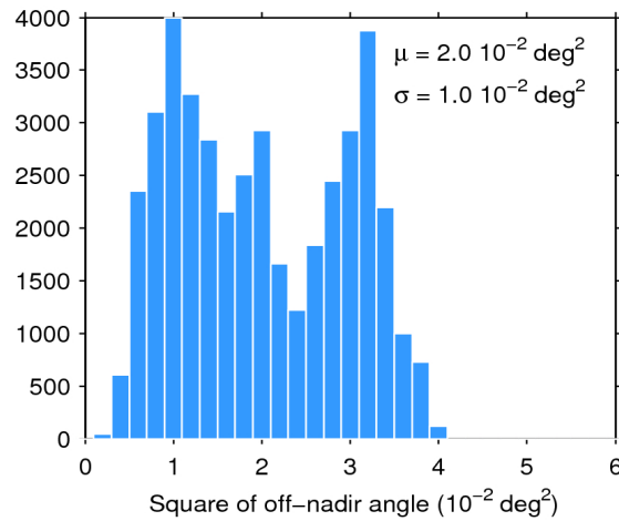
Figure 39. Histogram of flag-valid mispointing over oceans and lakes for 17/08/2020. The mean ( \mu ) and standard deviation ( \sigma ) are also shown. Note that values larger than 6 \cdot 10^{-2} \text{ deg}^2 are excluded from the histogram for the sake of readability but not from the computation of \mu and \sigma .
