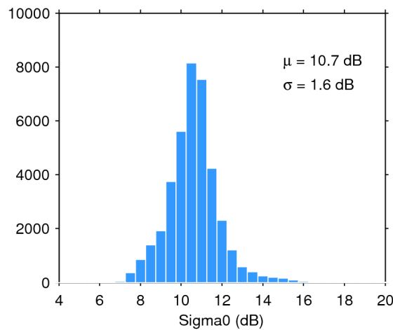
Figure 28. Histogram of science-valid sigma0 over oceans and lakes for 17/08/2020. The mean ( \mu ) and standard deviation ( \sigma ) are also shown. Note that values outside [4 20] dB are excluded from the histogram for the sake of readability but not from the computation of \mu and \sigma .
