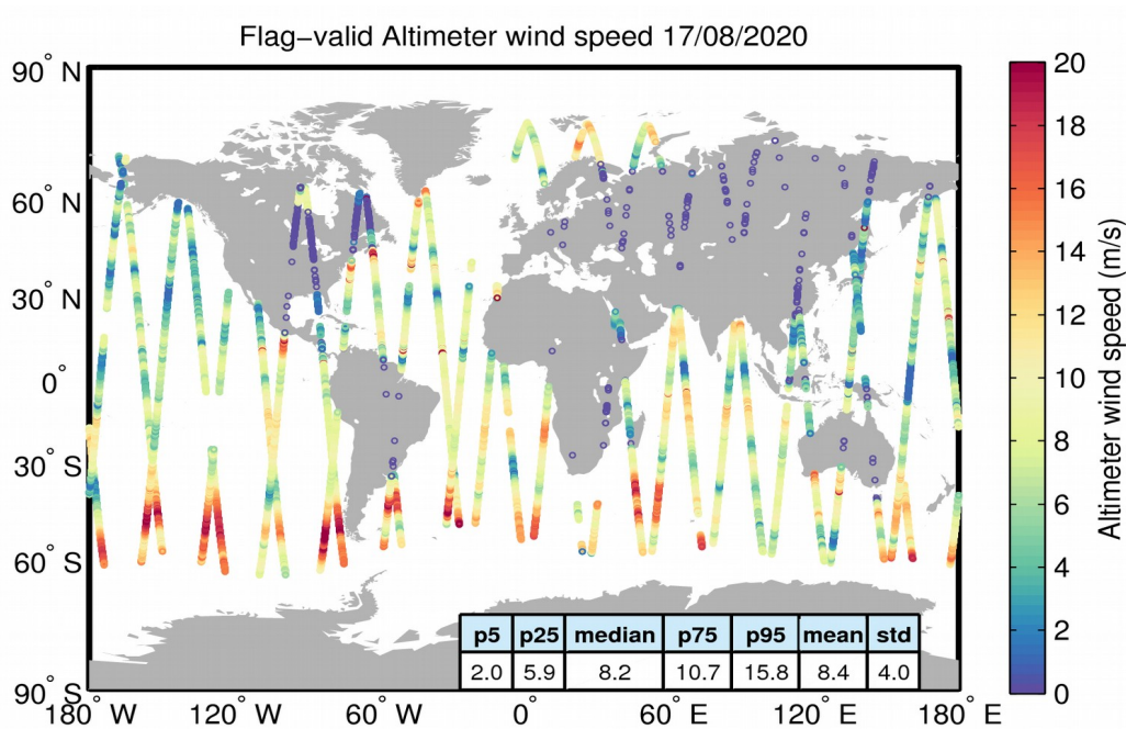
Figure 31. Geographical distribution of flag-valid wind data over oceans and lakes for 17/08/2020. The statistical values shown in the table refer to the wind in m/s and are calculated over all measurements shown in the figure.
