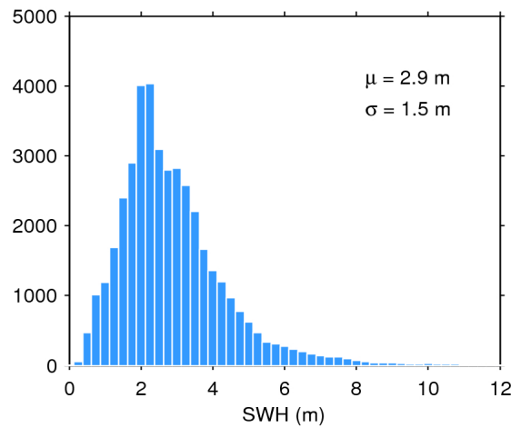
Figure 17. Histogram of flag-valid SWH over oceans and lakes for 17/08/2020. The mean ( \mu ) and standard deviation ( \sigma ) are also shown. Note that values larger than 12 m are excluded from the histogram for the sake of readability but not from the computation of \mu and \sigma .
