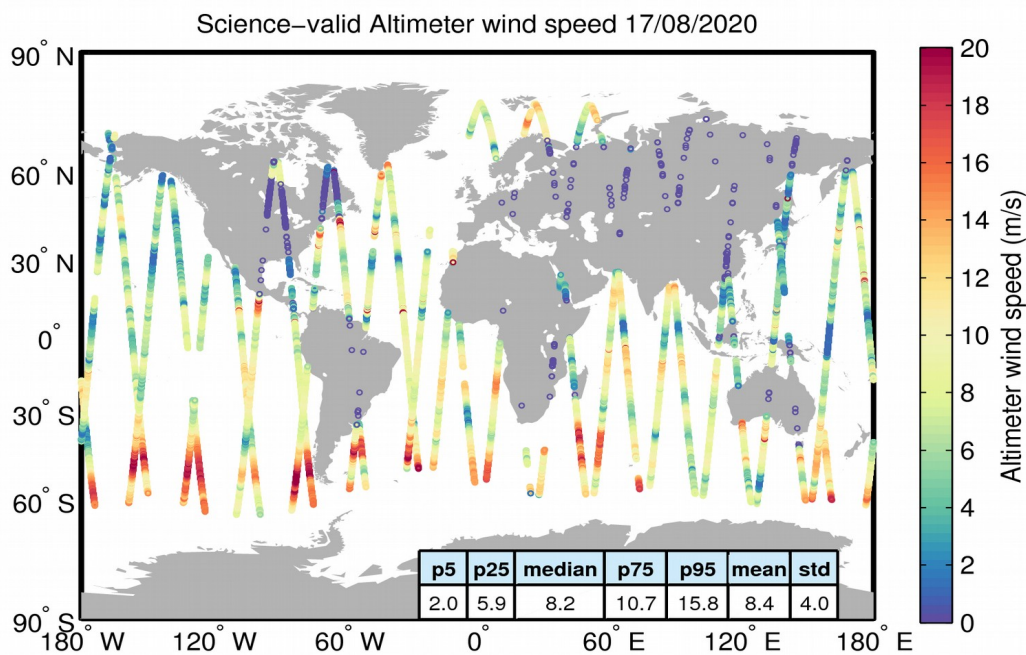
Figure 34. Geographical distribution of science-valid wind data over oceans and lakes for 17/08/2020. The statistical values shown in the table refer to the wind in m/s and are calculated over all measurements shown in the figure. Gray circles denote records that have been rejected based on the editing criteria described in Table 5.
