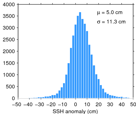
Figure 11. Histogram of science-valid SSH anomaly over oceans and lakes for 17/08/2020. The mean ( \mu ) and standard deviation ( \sigma ) are also shown. Note that values outside [-50 50] cm are excluded from the histogram for the sake of readability but not from the computation of \mu and \sigma .
