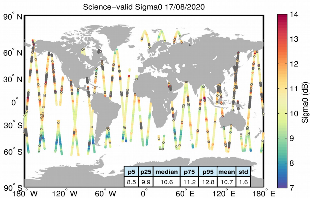
Figure 27. Geographical distribution of science-valid sigma0 data over oceans and lakes for 17/08/2020. The statistical values shown in the table refer to the sigma0 in dB and are calculated over all measurements shown in the figure. Gray circles denote records that have been rejected based on the editing criteria described in Table 4.
