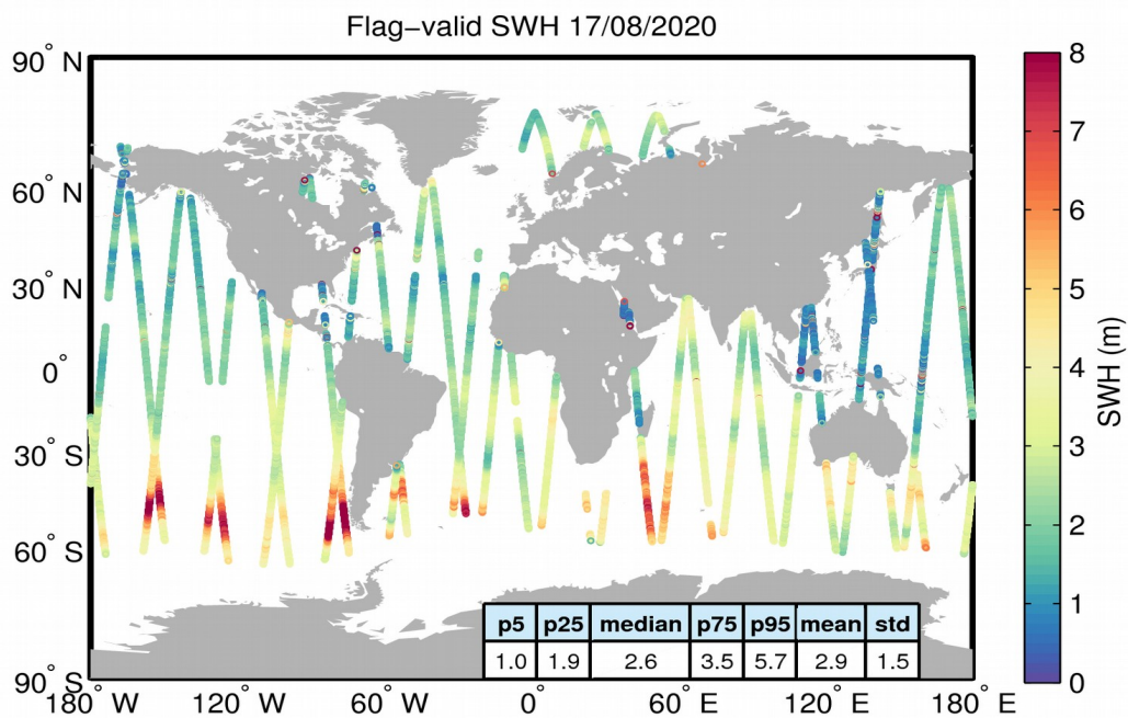
Figure 15. Geographical distribution of flag-valid SWH data over oceans and lakes for 17/08/2020. The statistical values shown in the table refer to the SWH in m and are calculated over all measurements shown in the figure.
