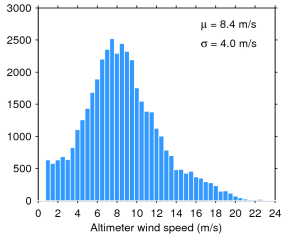
Figure 33. Histogram of flag-valid wind over oceans and lakes for 17/08/2020. The mean ( \mu ) and standard deviation ( \sigma ) are also shown. Note that values larger than 24 m/s are excluded from the histogram for the sake of readability but not from the computation of \mu and \sigma .
