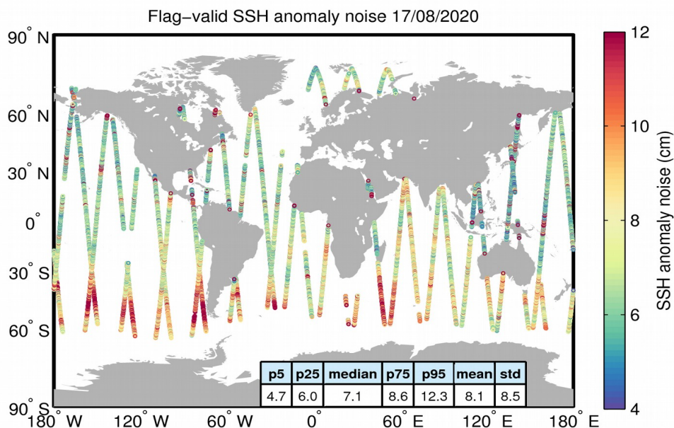
Figure 8. Geographical distribution of flag-valid 20-Hz SSH anomaly measurement noise over oceans and lakes for 17/08/2020. The statistical values shown in the table refer to the SSH anomaly noise and are calculated over all measurements shown in the figure.
