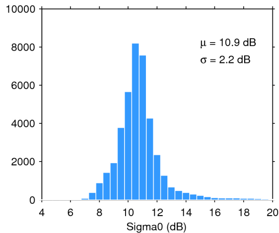
Figure 25. Histogram of flag-valid sigma0 over oceans and lakes for 17/08/2020. The mean ( \mu ) and standard deviation ( \sigma ) are also shown. Note that values outside [4 20] dB are excluded from the histogram for the sake of readability but not from the computation of \mu and \sigma .
