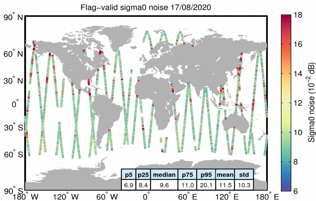
Figure 26. Geographical distribution of flag-valid 20-Hz sigma0 measurement noise over oceans and lakes for 17/08/2020. The statistical values shown in the table refer to the sigma0 noise and are calculated over all measurements shown in the figure.
