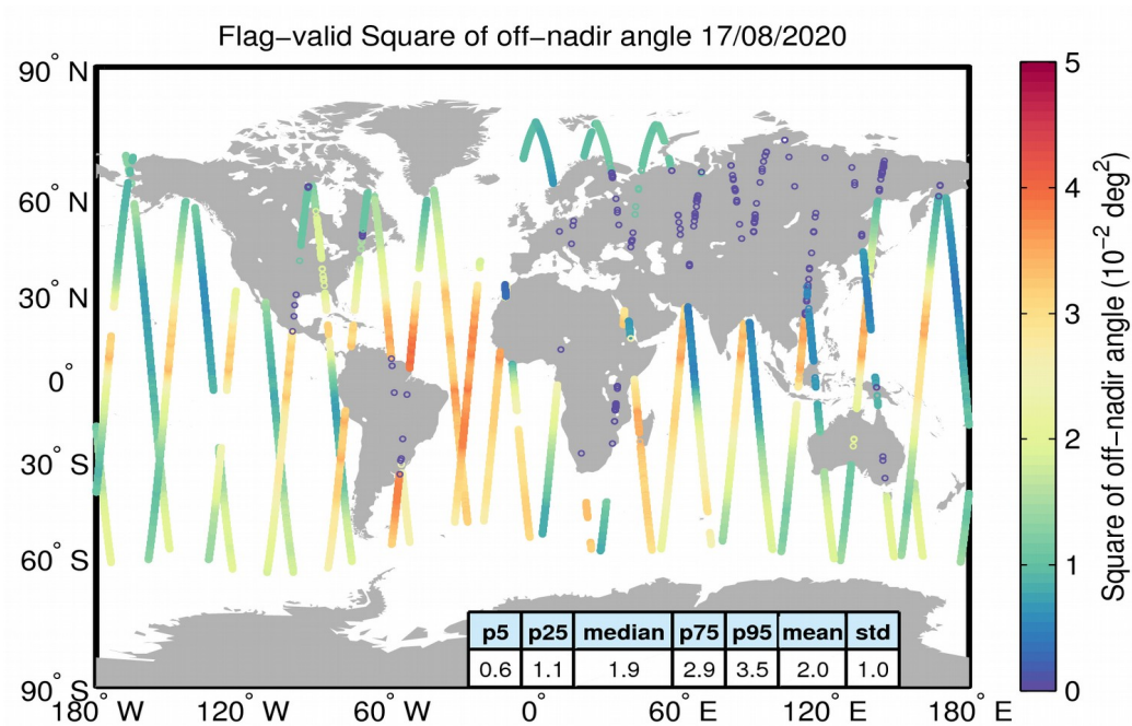
Figure 37. Geographical distribution of flag-valid mispointing data over oceans and lakes for 17/08/2020. The statistical values shown in the table refer to the mispointing in 10^{-2} deg 2 and are calculated over all measurements shown in the figure.
