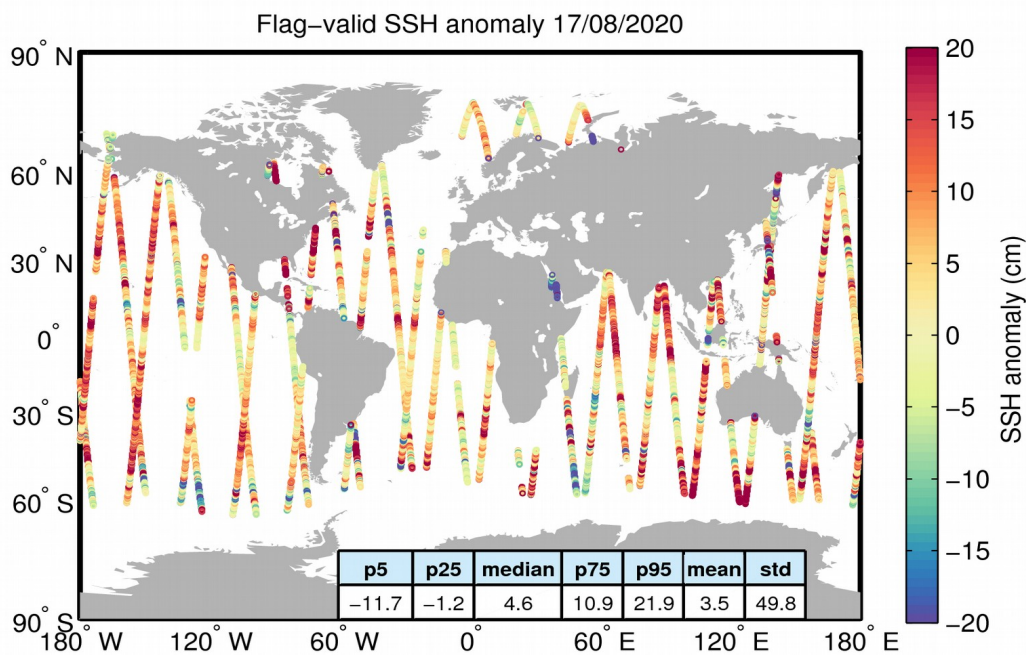
Figure 5. Geographical distribution of flag-valid 1-Hz SSH anomaly data over oceans and lakes for 17/08/2020. The statistical values shown in the table refer to the SSH anomaly in cm and are calculated over all measurements shown in the figure.
