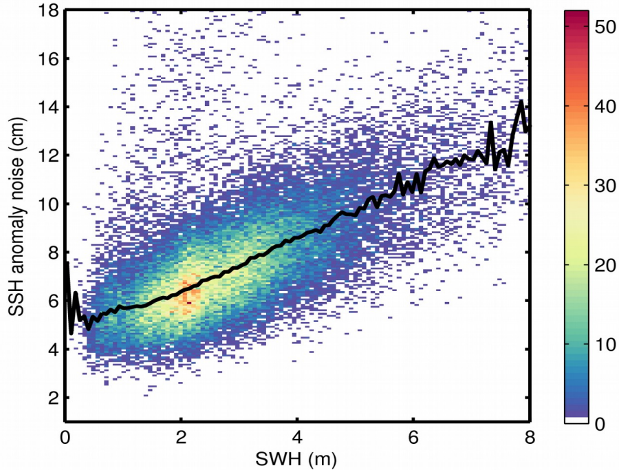
Figure 9. 2D histogram showing flag-valid SSH anomaly noise as a function of SWH for 17/08/2020. The black line denotes the median SSH anomaly noise as a function of SWH.
