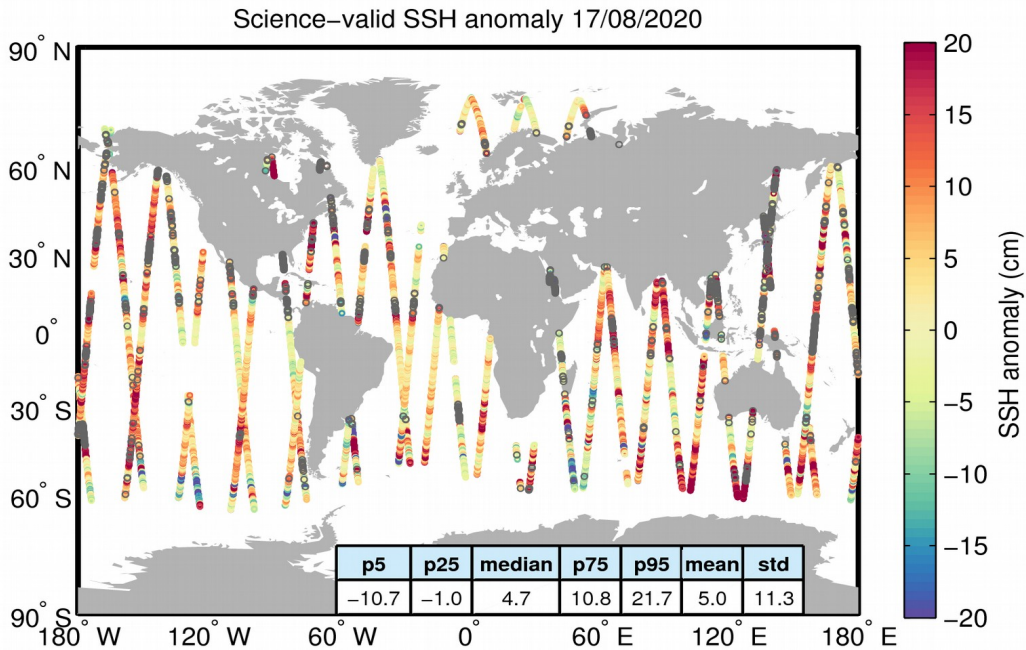
Figure 10. Geographical distribution of science-valid SSH anomaly data over oceans and lakes for 17/08/2020. The statistical values shown in the table refer to the SSH anomaly in cm and are calculated over all measurements shown in the figure. Gray circles denote records that have been rejected based on the editing criteria described in Table 2.
