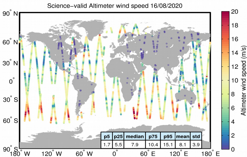
Figure 34. Geographical distribution of science-valid wind data over oceans and lakes for 16/08/2020. The statistical values shown in the table refer to the wind in m/s and are calculated over all measurements shown in the figure. Gray circles denote records that have been rejected based on the editing criteria described in Table 5.
