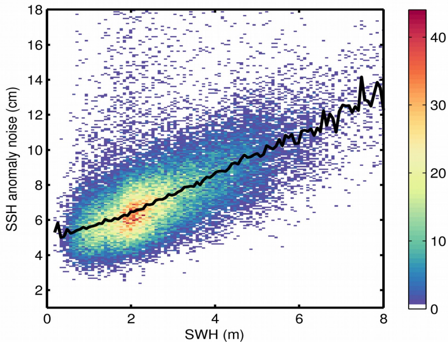
Figure 9. 2D histogram showing flag-valid SSH anomaly noise as a function of SWH for 16/08/2020. The black line denotes the median SSH anomaly noise as a function of SWH.
