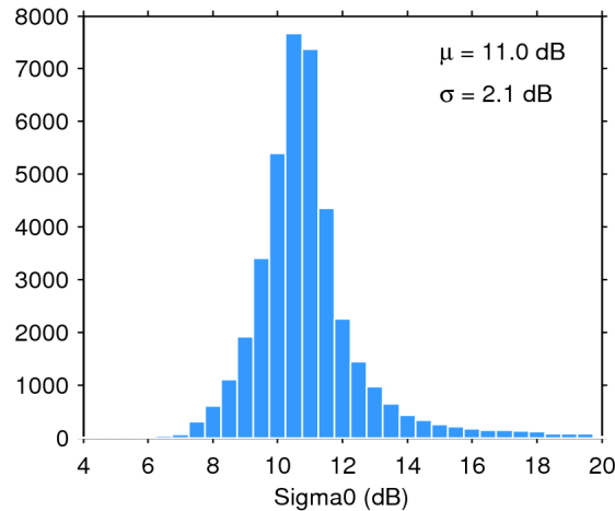
Figure 25. Histogram of flag-valid sigma0 over oceans and lakes for 16/08/2020. The mean ( \mu ) and standard deviation ( \sigma ) are also shown. Note that values outside [4 20] dB are excluded from the histogram for the sake of readability but not from the computation of \mu and \sigma .
