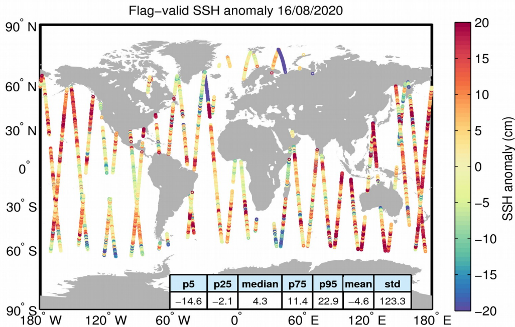
Figure 5. Geographical distribution of flag-valid 1-Hz SSH anomaly data over oceans and lakes for 16/08/2020. The statistical values shown in the table refer to the SSH anomaly in cm and are calculated over all measurements shown in the figure.
