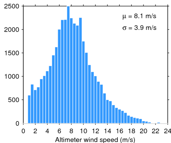
Figure 35. Histogram of science-valid wind over oceans and lakes for 16/08/2020. The mean ( \mu ) and standard deviation ( \sigma ) are also shown. Note that values larger than 24 m/s are excluded from the histogram for the sake of readability but not from the computation of \mu and \sigma .
