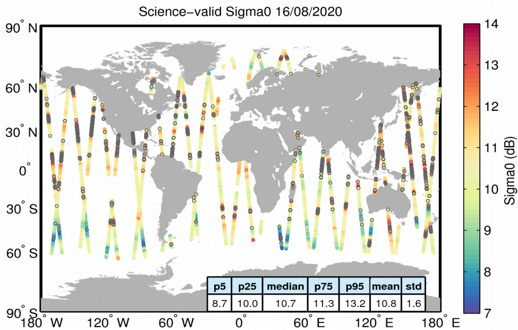
Figure 27. Geographical distribution of science-valid sigma0 data over oceans and lakes for 16/08/2020. The statistical values shown in the table refer to the sigma0 in dB and are calculated over all measurements shown in the figure. Gray circles denote records that have been rejected based on the editing criteria described in Table 4.
