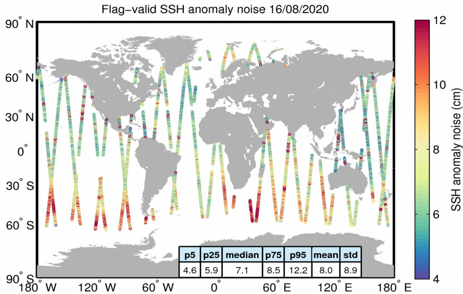
Figure 8. Geographical distribution of flag-valid 20-Hz SSH anomaly measurement noise over oceans and lakes for 16/08/2020. The statistical values shown in the table refer to the SSH anomaly noise and are calculated over all measurements shown in the figure.
