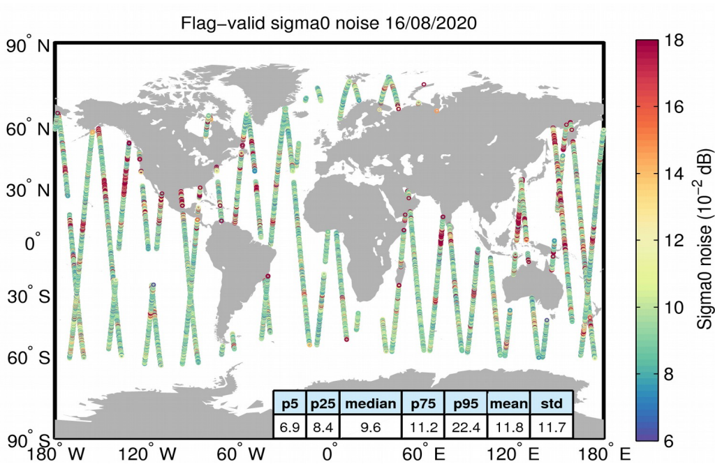
Figure 26. Geographical distribution of flag-valid 20-Hz sigma0 measurement noise over oceans and lakes for 16/08/2020. The statistical values shown in the table refer to the sigma0 noise and are calculated over all measurements shown in the figure.
