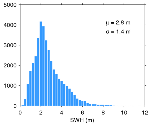
Figure 17. Histogram of flag-valid SWH over oceans and lakes for 16/08/2020. The mean ( \mu ) and standard deviation ( \sigma ) are also shown. Note that values larger than 12 m are excluded from the histogram for the sake of readability but not from the computation of \mu and \sigma .
