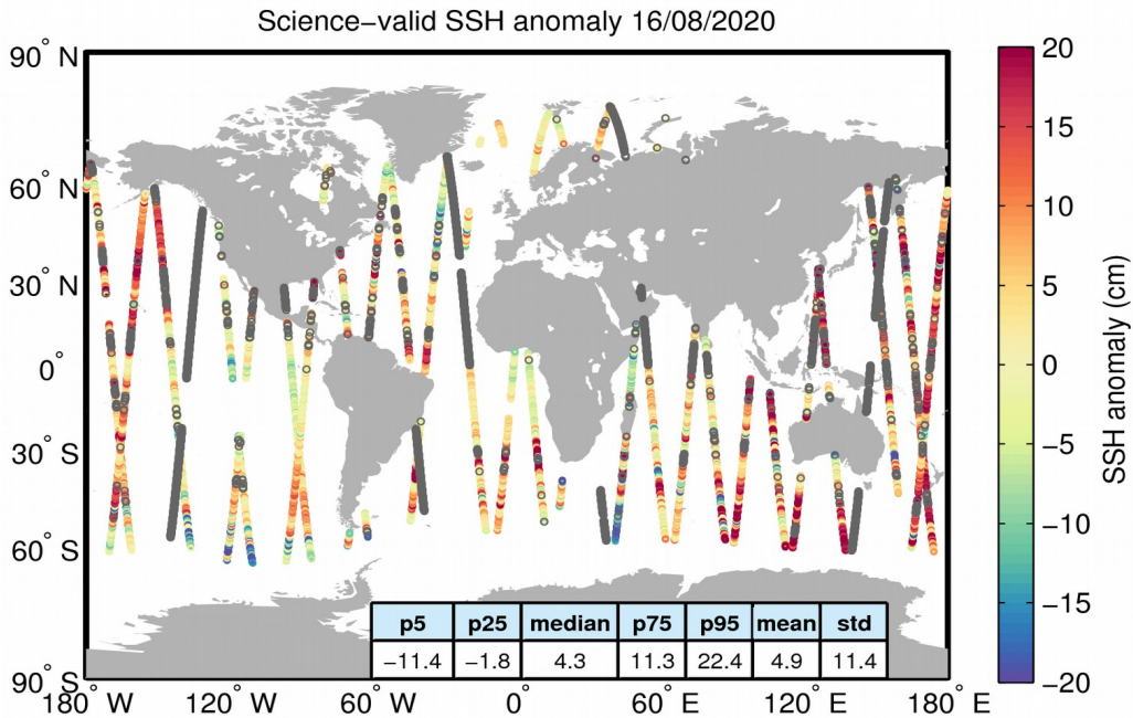
Figure 10. Geographical distribution of science-valid SSH anomaly data over oceans and lakes for 16/08/2020. The statistical values shown in the table refer to the SSH anomaly in cm and are calculated over all measurements shown in the figure. Gray circles denote records that have been rejected based on the editing criteria described in Table 2.
