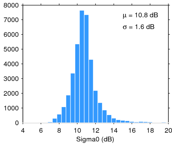
Figure 28. Histogram of science-valid sigma0 over oceans and lakes for 16/08/2020. The mean ( \mu ) and standard deviation ( \sigma ) are also shown. Note that values outside [4 20] dB are excluded from the histogram for the sake of readability but not from the computation of \mu and \sigma .
