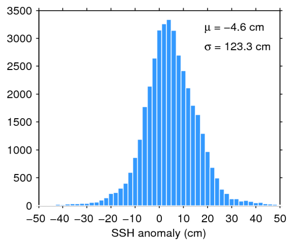
Figure 7. Histogram of flag-valid SSH anomaly over oceans and lakes for 16/08/2020. The mean ( \mu ) and standard deviation ( \sigma ) are also shown. Note that values outside [-50 50] cm are excluded from the histogram for the sake of readability but not from the computation of \mu and \sigma .
