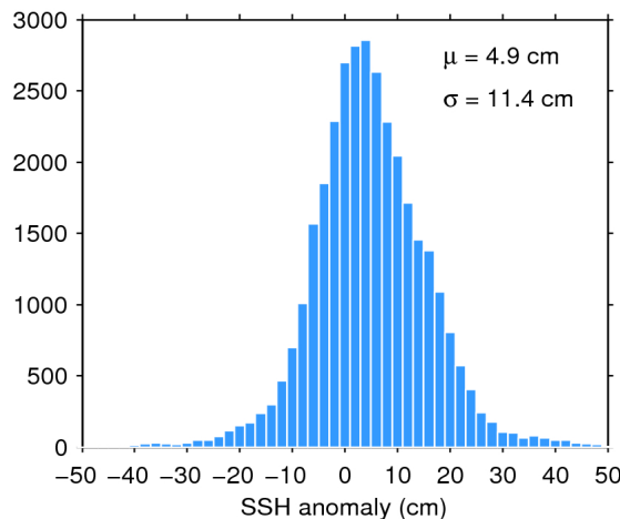
Figure 11. Histogram of science-valid SSH anomaly over oceans and lakes for 16/08/2020. The mean ( \mu ) and standard deviation ( \sigma ) are also shown. Note that values outside [-50 50] cm are excluded from the histogram for the sake of readability but not from the computation of \mu and \sigma .
