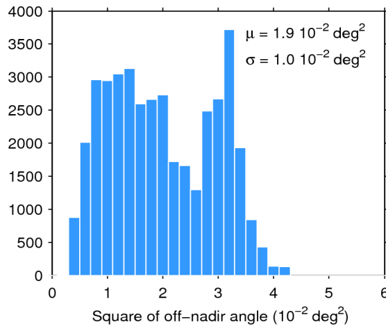
Figure 39. Histogram of flag-valid mispointing over oceans and lakes for 16/08/2020. The mean ( \mu ) and standard deviation ( \sigma ) are also shown. Note that values larger than 6 \cdot 10^{-2} \text{ deg}^2 are excluded from the histogram for the sake of readability but not from the computation of \mu and \sigma .
