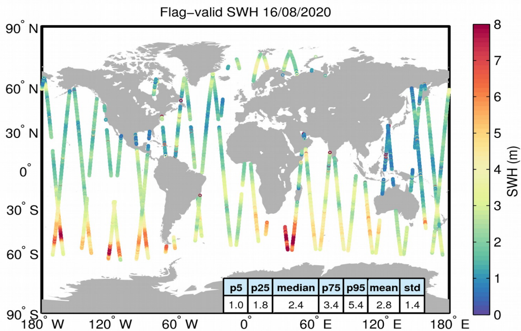
Figure 15. Geographical distribution of flag-valid SWH data over oceans and lakes for 16/08/2020. The statistical values shown in the table refer to the SWH in m and are calculated over all measurements shown in the figure.
