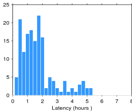
Figure 2. Histogram of the data latency for 16/08/2020. The y-axis denotes the number of files that are made available with a delay of x-hours with respect to the mean time of the records stored in the file.
