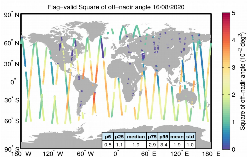
Figure 37. Geographical distribution of flag-valid mispointing data over oceans and lakes for 16/08/2020. The statistical values shown in the table refer to the mispointing in 10^{-2} \text{ deg}^2 and are calculated over all measurements shown in the figure.
