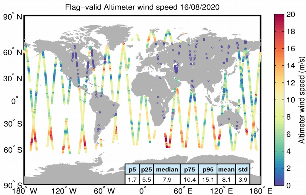
Figure 31. Geographical distribution of flag-valid wind data over oceans and lakes for 16/08/2020. The statistical values shown in the table refer to the wind in m/s and are calculated over all measurements shown in the figure.
