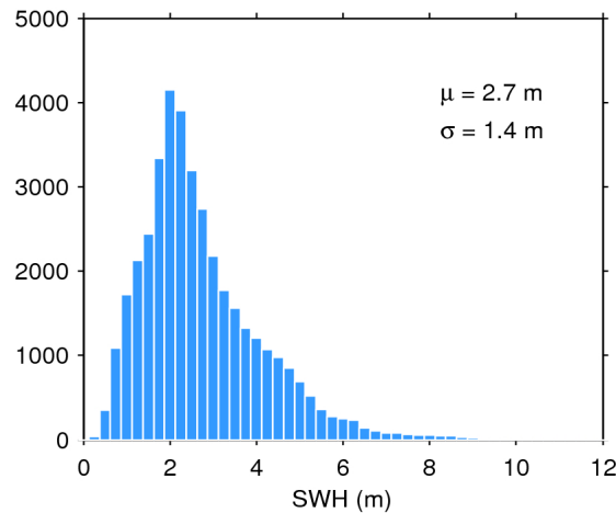
Figure 20. Histogram of science-valid SWH over oceans and lakes for 16/08/2020. The mean ( \mu ) and standard deviation ( \sigma ) are also shown. Note that values larger than 12 m are excluded from the histogram for the sake of readability but not from the computation of \mu and \sigma .
