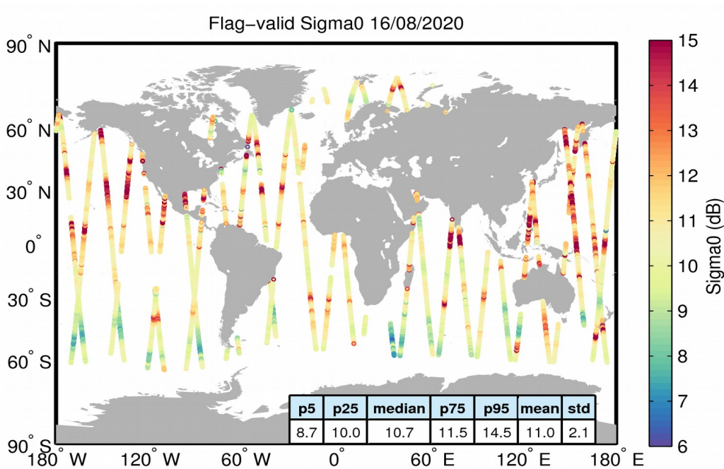
Figure 23. Geographical distribution of flag-valid sigma0 data over oceans and lakes for 16/08/2020. The statistical values shown in the table refer to the sigma0 in dB and are calculated over all measurements shown in the figure.
