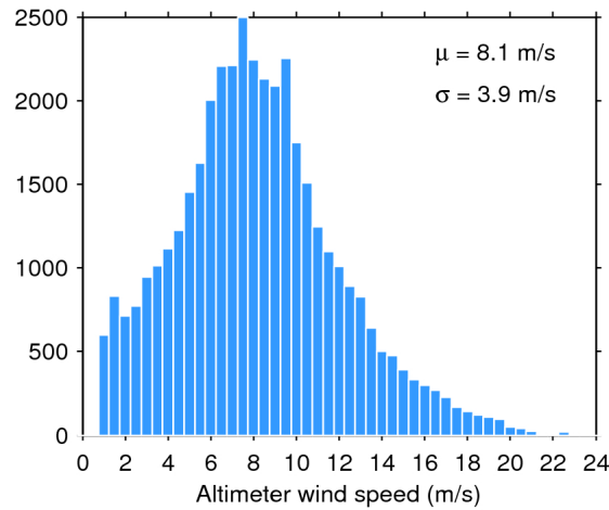
Figure 33. Histogram of flag-valid wind over oceans and lakes for 16/08/2020. The mean ( \mu ) and standard deviation ( \sigma ) are also shown. Note that values larger than 24 m/s are excluded from the histogram for the sake of readability but not from the computation of \mu and \sigma .
