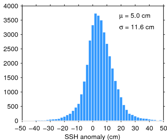
Figure 11. Histogram of science-valid SSH anomaly over oceans and lakes for 15/08/2020. The mean ( \mu ) and standard deviation ( \sigma ) are also shown. Note that values outside [-50 50] cm are excluded from the histogram for the sake of readability but not from the computation of \mu and \sigma .
