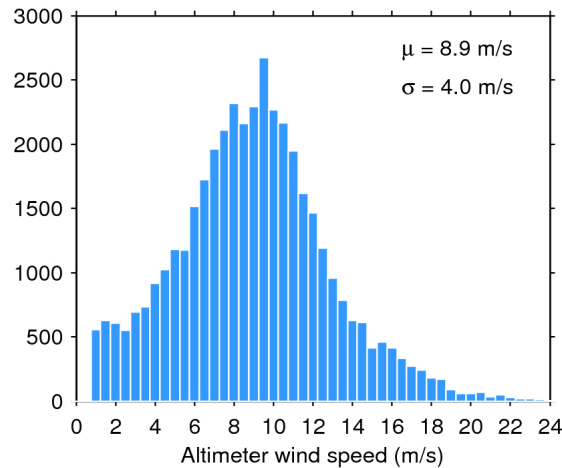
Figure 33. Histogram of flag-valid wind over oceans and lakes for 15/08/2020. The mean ( \mu ) and standard deviation ( \sigma ) are also shown. Note that values larger than 24 m/s are excluded from the histogram for the sake of readability but not from the computation of \mu and \sigma .
