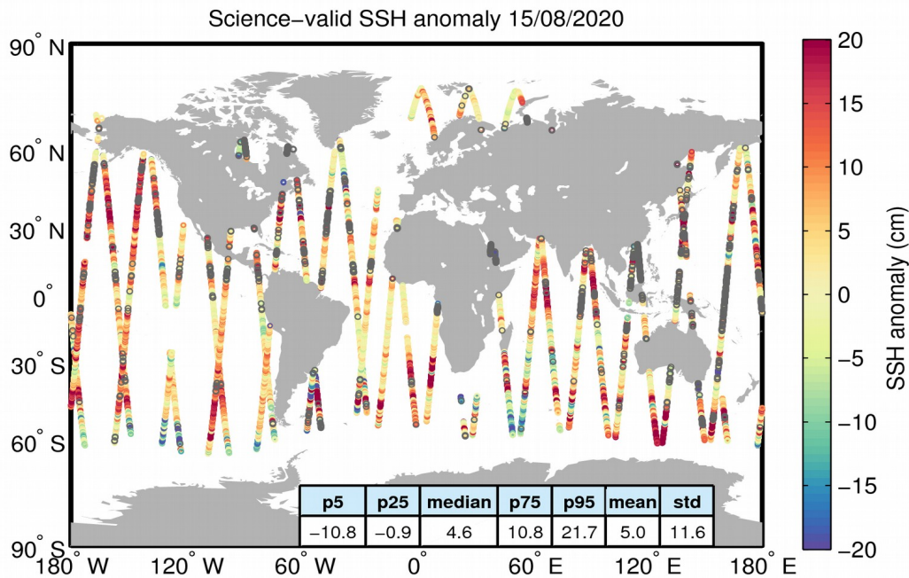
Figure 10. Geographical distribution of science-valid SSH anomaly data over oceans and lakes for 15/08/2020. The statistical values shown in the table refer to the SSH anomaly in cm and are calculated over all measurements shown in the figure. Gray circles denote records that have been rejected based on the editing criteria described in Table 2.
