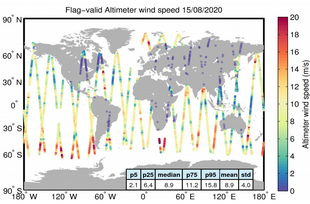
Figure 31. Geographical distribution of flag-valid wind data over oceans and lakes for 15/08/2020. The statistical values shown in the table refer to the wind in m/s and are calculated over all measurements shown in the figure.
