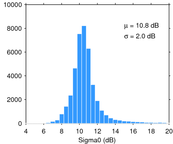
Figure 25. Histogram of flag-valid sigma0 over oceans and lakes for 15/08/2020. The mean ( \mu ) and standard deviation ( \sigma ) are also shown. Note that values outside [4 20] dB are excluded from the histogram for the sake of readability but not from the computation of \mu and \sigma .
