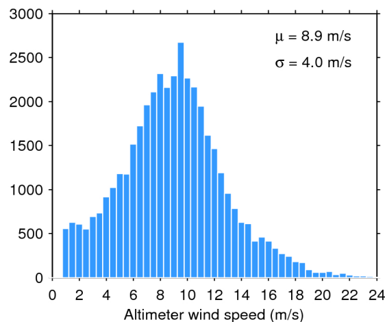
Figure 35. Histogram of science-valid wind over oceans and lakes for 15/08/2020. The mean ( \mu ) and standard deviation ( \sigma ) are also shown. Note that values larger than 24 m/s are excluded from the histogram for the sake of readability but not from the computation of \mu and \sigma .
