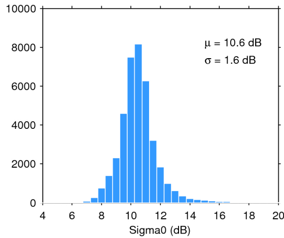
Figure 28. Histogram of science-valid sigma0 over oceans and lakes for 15/08/2020. The mean ( \mu ) and standard deviation ( \sigma ) are also shown. Note that values outside [4 20] dB are excluded from the histogram for the sake of readability but not from the computation of \mu and \sigma .
