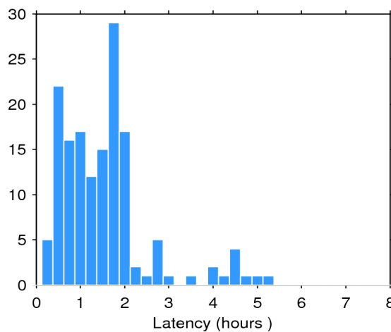
Figure 2. Histogram of the data latency for 15/08/2020. The y-axis denotes the number of files that are made available with a delay of x-hours with respect to the mean time of the records stored in the file.
