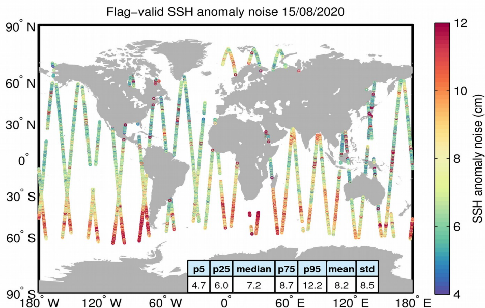
Figure 8. Geographical distribution of flag-valid 20-Hz SSH anomaly measurement noise over oceans and lakes for 15/08/2020. The statistical values shown in the table refer to the SSH anomaly noise and are calculated over all measurements shown in the figure.
