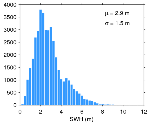
Figure 17. Histogram of flag-valid SWH over oceans and lakes for 15/08/2020. The mean ( \mu ) and standard deviation ( \sigma ) are also shown. Note that values larger than 12 m are excluded from the histogram for the sake of readability but not from the computation of \mu and \sigma .
