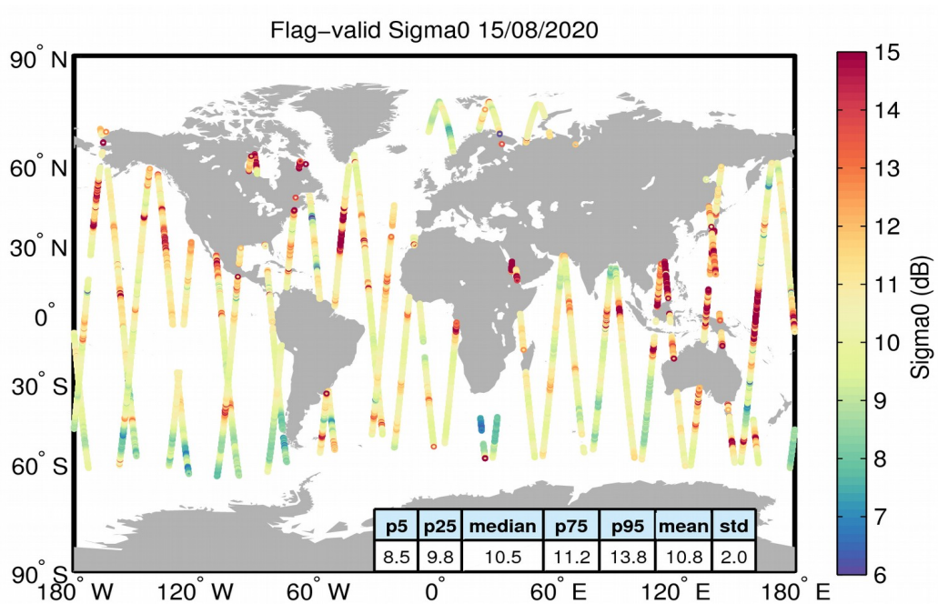
Figure 23. Geographical distribution of flag-valid sigma0 data over oceans and lakes for 15/08/2020. The statistical values shown in the table refer to the sigma0 in dB and are calculated over all measurements shown in the figure.
