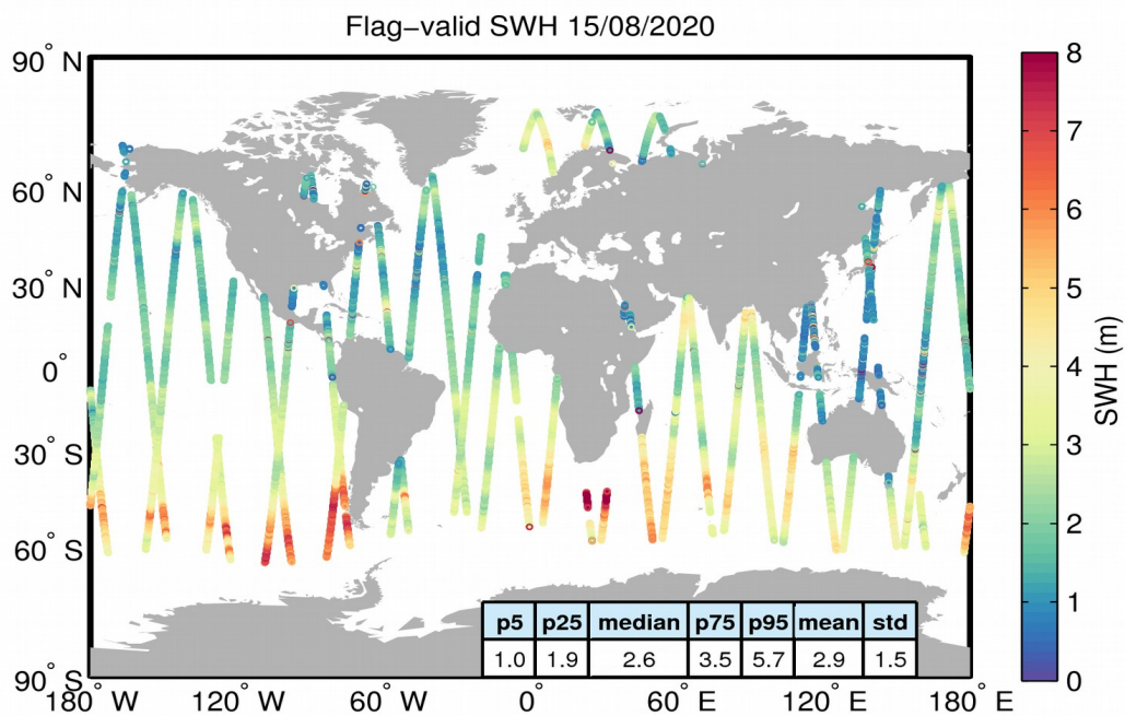
Figure 15. Geographical distribution of flag-valid SWH data over oceans and lakes for 15/08/2020. The statistical values shown in the table refer to the SWH in m and are calculated over all measurements shown in the figure.
