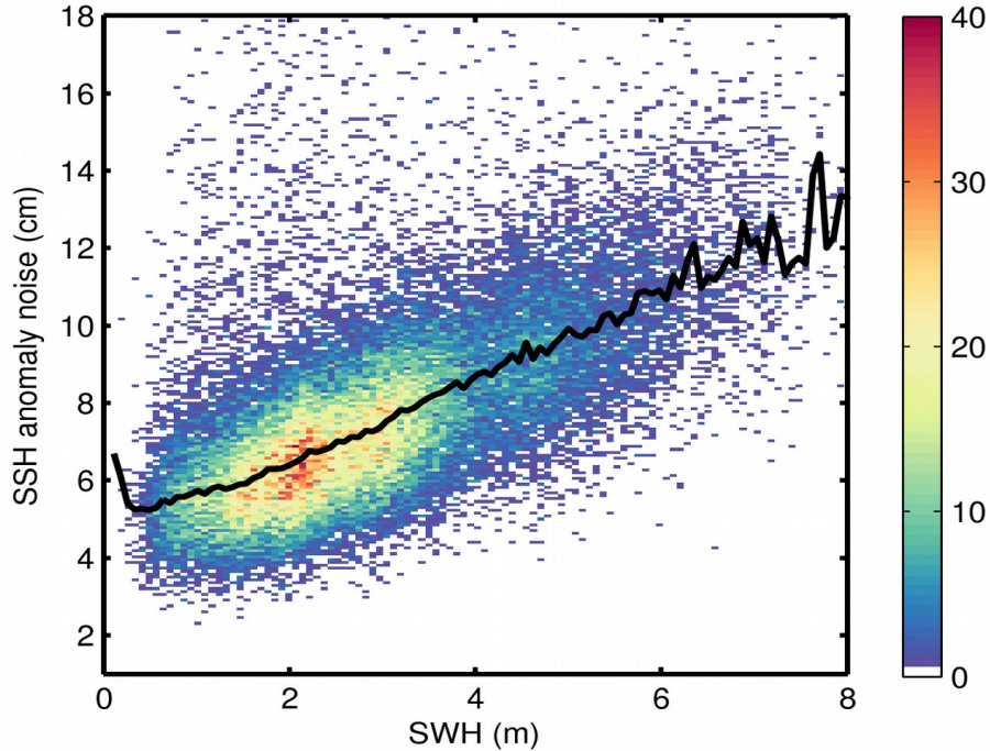
Figure 9. 2D histogram showing flag-valid SSH anomaly noise as a function of SWH for 15/08/2020. The black line denotes the median SSH anomaly noise as a function of SWH.
