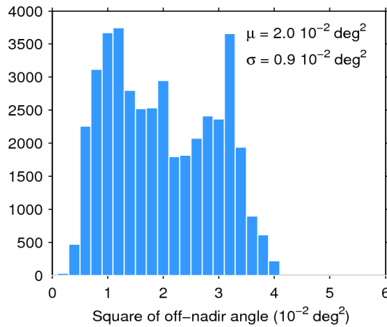
Figure 39. Histogram of flag-valid mispointing over oceans and lakes for 15/08/2020. The mean ( \mu ) and standard deviation ( \sigma ) are also shown. Note that values larger than 6 \cdot 10^{-2} \text{ deg}^2 are excluded from the histogram for the sake of readability but not from the computation of \mu and \sigma .
