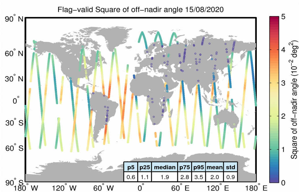
Figure 37. Geographical distribution of flag-valid mispointing data over oceans and lakes for 15/08/2020. The statistical values shown in the table refer to the mispointing in 10^{-2} \text{ deg}^2 and are calculated over all measurements shown in the figure.
