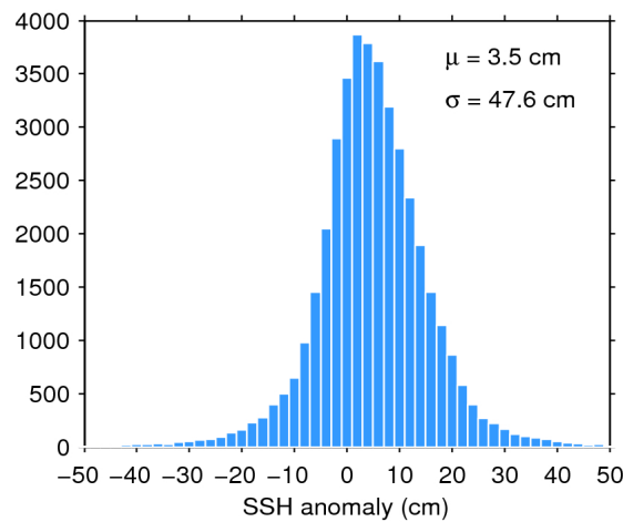
Figure 7. Histogram of flag-valid SSH anomaly over oceans and lakes for 15/08/2020. The mean ( \mu ) and standard deviation ( \sigma ) are also shown. Note that values outside [-50 50] cm are excluded from the histogram for the sake of readability but not from the computation of \mu and \sigma .
