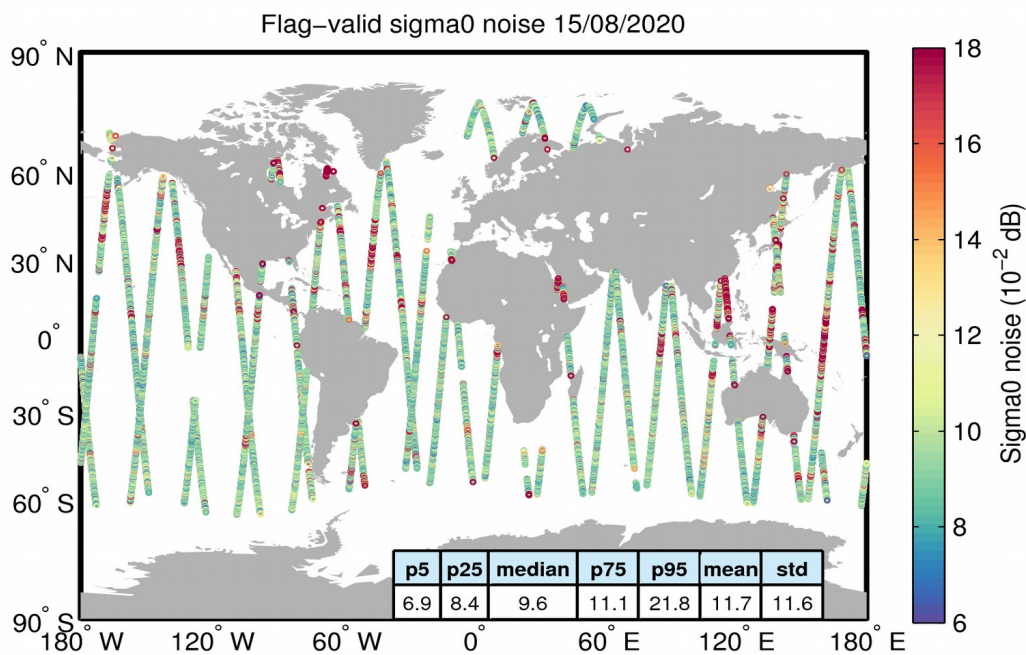
Figure 26. Geographical distribution of flag-valid 20-Hz sigma0 measurement noise over oceans and lakes for 15/08/2020. The statistical values shown in the table refer to the sigma0 noise and are calculated over all measurements shown in the figure.
