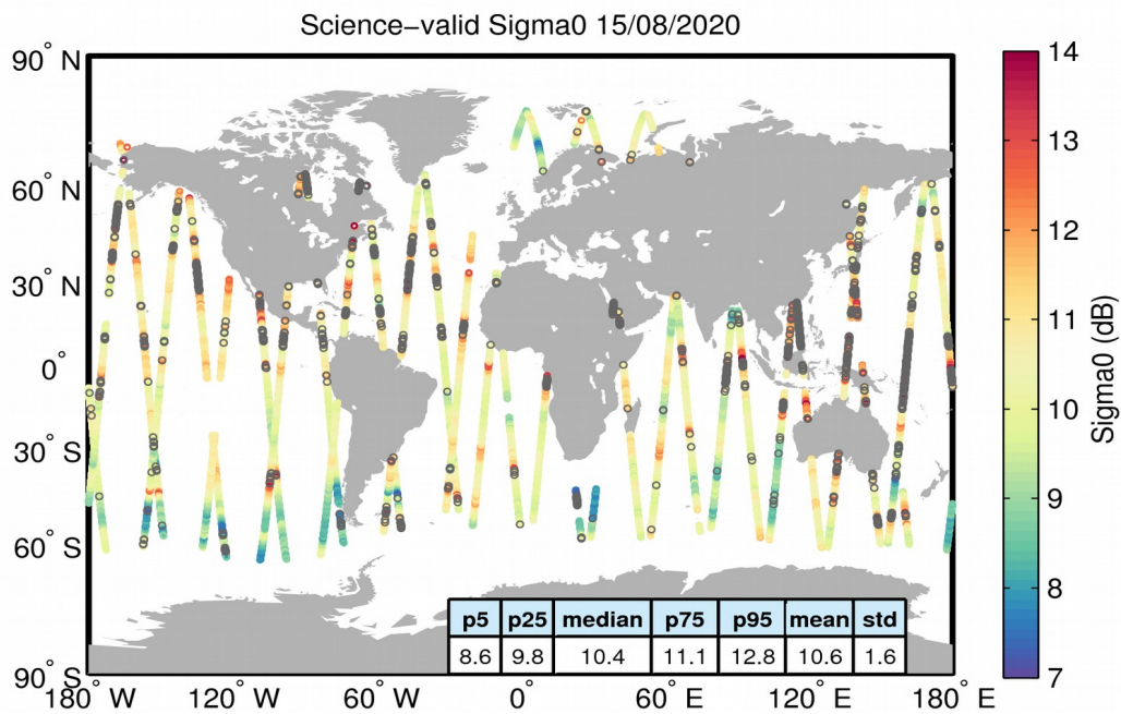
Figure 27. Geographical distribution of science-valid sigma0 data over oceans and lakes for 15/08/2020. The statistical values shown in the table refer to the sigma0 in dB and are calculated over all measurements shown in the figure. Gray circles denote records that have been rejected based on the editing criteria described in Table 4.
