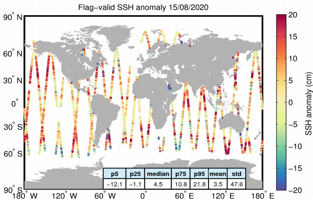
Figure 5. Geographical distribution of flag-valid 1-Hz SSH anomaly data over oceans and lakes for 15/08/2020. The statistical values shown in the table refer to the SSH anomaly in cm and are calculated over all measurements shown in the figure.
