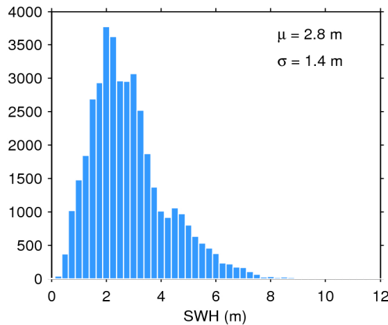
Figure 20. Histogram of science-valid SWH over oceans and lakes for 15/08/2020. The mean ( \mu ) and standard deviation ( \sigma ) are also shown. Note that values larger than 12 m are excluded from the histogram for the sake of readability but not from the computation of \mu and \sigma .
