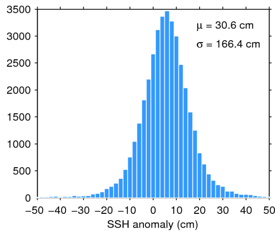
Figure 7. Histogram of flag-valid SSH anomaly over oceans and lakes for 13/08/2020. The mean ( \mu ) and standard deviation ( \sigma ) are also shown. Note that values outside [-50\ 50] cm are excluded from the histogram for the sake of readability but not from the computation of \mu and \sigma .
