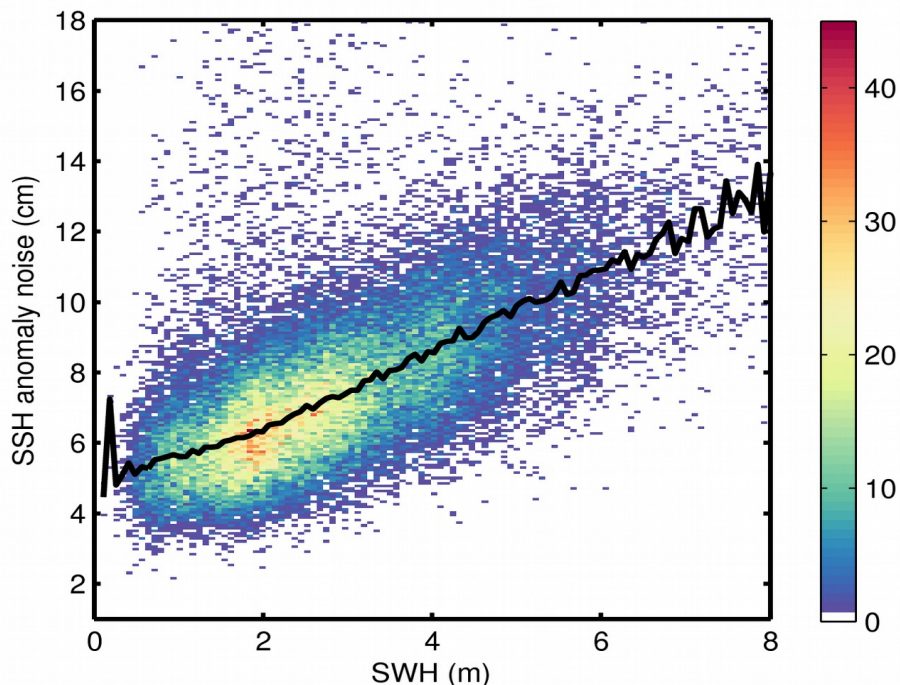
Figure 9. 2D histogram showing flag-valid SSH anomaly noise as a function of SWH for 13/08/2020. The black line denotes the median SSH anomaly noise as a function of SWH.
