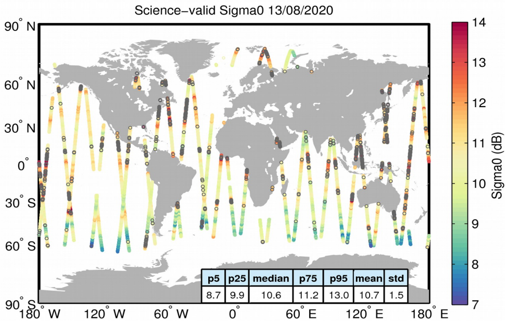
Figure 27. Geographical distribution of science-valid sigma0 data over oceans and lakes for 13/08/2020. The statistical values shown in the table refer to the sigma0 in dB and are calculated over all measurements shown in the figure. Gray circles denote records that have been rejected based on the editing criteria described in Table 4.
