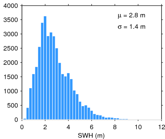
Figure 20. Histogram of science-valid SWH over oceans and lakes for 13/08/2020. The mean ( \mu ) and standard deviation ( \sigma ) are also shown. Note that values larger than 12 m are excluded from the histogram for the sake of readability but not from the computation of \mu and \sigma .
