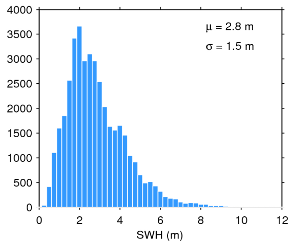
Figure 17. Histogram of flag-valid SWH over oceans and lakes for 13/08/2020. The mean ( \mu ) and standard deviation ( \sigma ) are also shown. Note that values larger than 12 m are excluded from the histogram for the sake of readability but not from the computation of \mu and \sigma .
