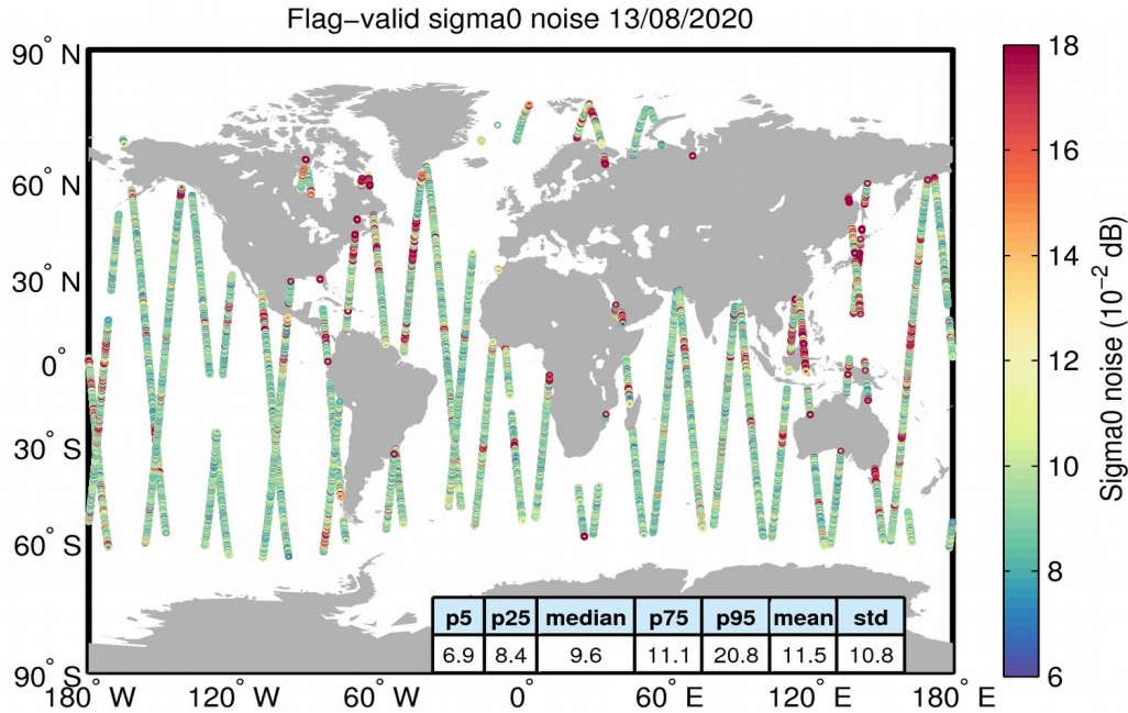
Figure 26. Geographical distribution of flag-valid 20-Hz sigma0 measurement noise over oceans and lakes for 13/08/2020. The statistical values shown in the table refer to the sigma0 noise and are calculated over all measurements shown in the figure.
