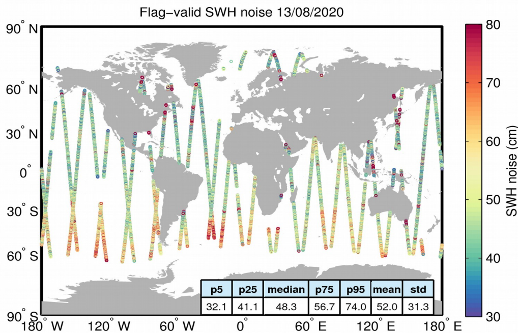
Figure 18. Geographical distribution of flag-valid 20-Hz SWH measurement noise over oceans and lakes for 13/08/2020. The statistical values shown in the figure refer to the SWH noise and are calculated over all measurements shown in the figure.
