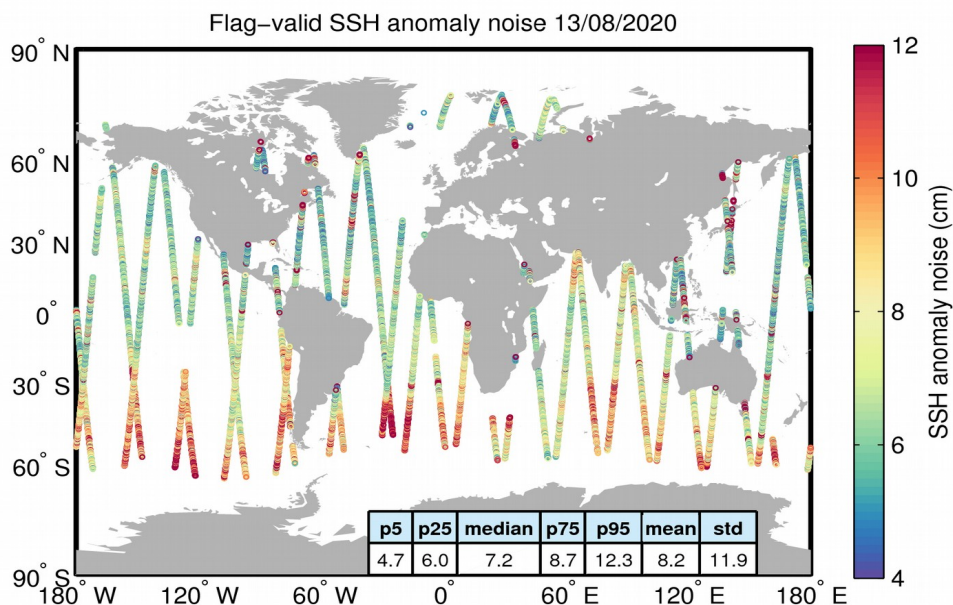
Figure 8. Geographical distribution of flag-valid 20-Hz SSH anomaly measurement noise over oceans and lakes for 13/08/2020. The statistical values shown in the table refer to the SSH anomaly noise and are calculated over all measurements shown in the figure.
