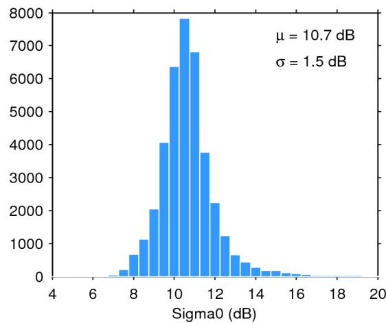
Figure 28. Histogram of science-valid sigma0 over oceans and lakes for 13/08/2020. The mean ( \mu ) and standard deviation ( \sigma ) are also shown. Note that values outside [4 20] dB are excluded from the histogram for the sake of readability but not from the computation of \mu and \sigma .
