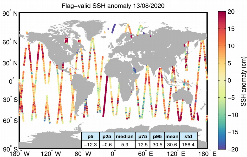
Figure 5. Geographical distribution of flag-valid 1-Hz SSH anomaly data over oceans and lakes for 13/08/2020. The statistical values shown in the table refer to the SSH anomaly in cm and are calculated over all measurements shown in the figure.
