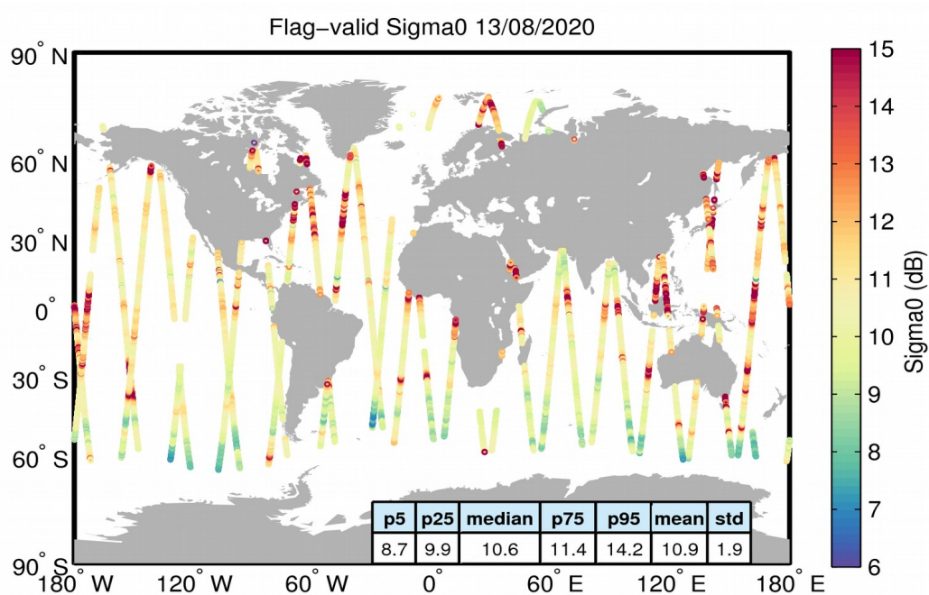
Figure 23. Geographical distribution of flag-valid sigma0 data over oceans and lakes for 13/08/2020. The statistical values shown in the table refer to the sigma0 in dB and are calculated over all measurements shown in the figure.
