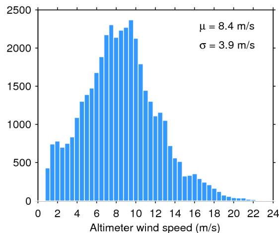
Figure 35. Histogram of science-valid wind over oceans and lakes for 13/08/2020. The mean ( \mu ) and standard deviation ( \sigma ) are also shown. Note that values larger than 24 m/s are excluded from the histogram for the sake of readability but not from the computation of \mu and \sigma .
