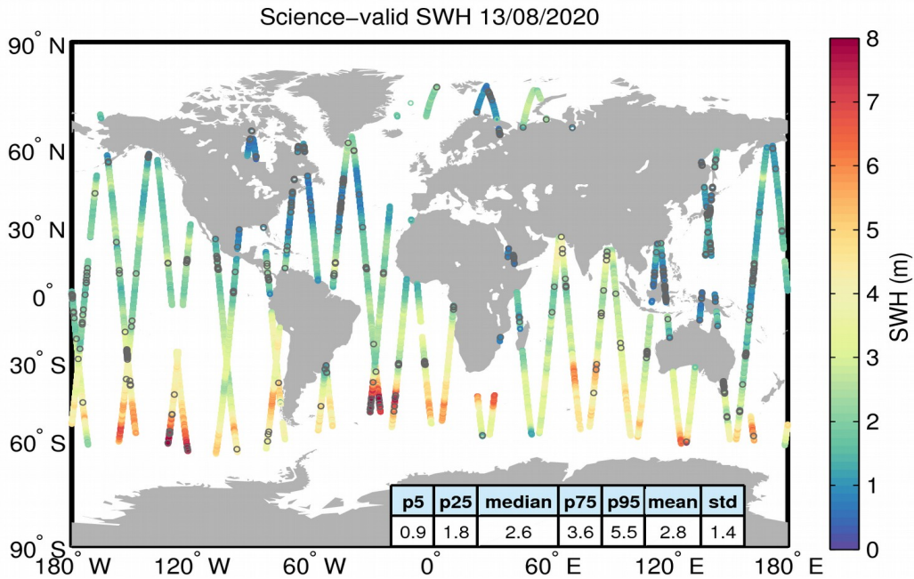
Figure 19. Geographical distribution of science-valid SWH data over oceans and lakes for 13/08/2020. The statistical values shown in the table refer to the SWH in m and are calculated over all measurements shown in the figure. Gray circles denote records that have been rejected based on the editing criteria described in Table 3.
