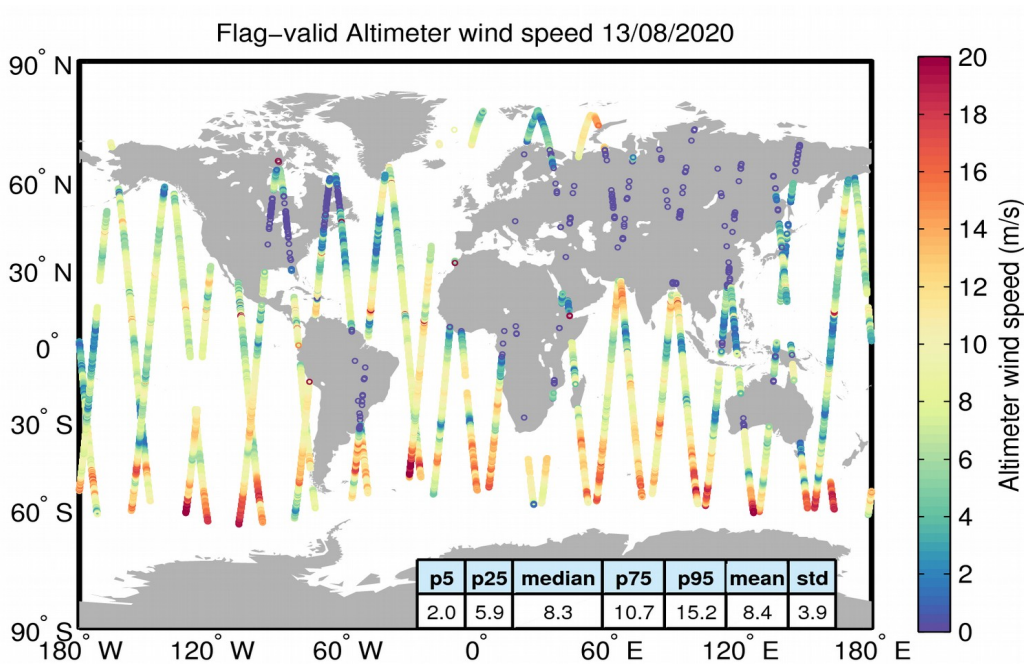
Figure 31. Geographical distribution of flag-valid wind data over oceans and lakes for 13/08/2020. The statistical values shown in the table refer to the wind in m/s and are calculated over all measurements shown in the figure.
