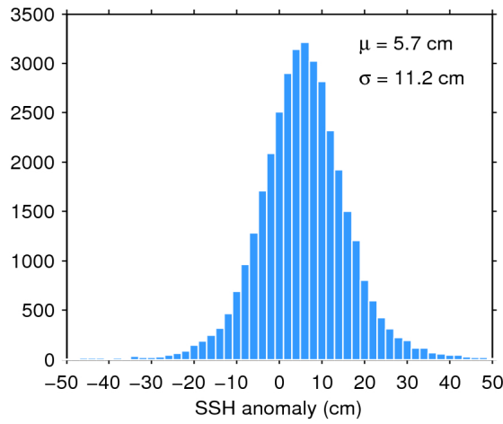
Figure 11. Histogram of science-valid SSH anomaly over oceans and lakes for 13/08/2020. The mean ( \mu ) and standard deviation ( \sigma ) are also shown. Note that values outside [-50 50] cm are excluded from the histogram for the sake of readability but not from the computation of \mu and \sigma .
