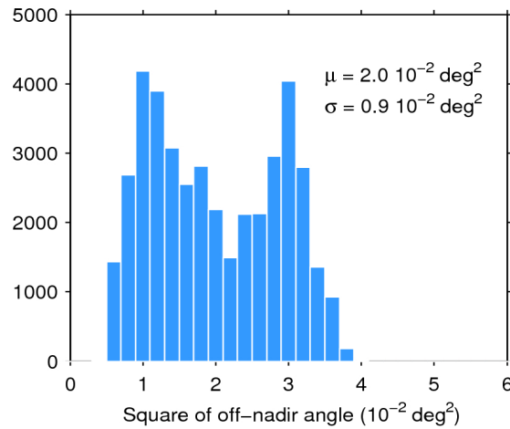
Figure 39. Histogram of flag-valid mispointing over oceans and lakes for 13/08/2020. The mean ( \mu ) and standard deviation ( \sigma ) are also shown. Note that values larger than 6 \cdot 10^{-2} \text{ deg}^2 are excluded from the histogram for the sake of readability but not from the computation of \mu and \sigma .
