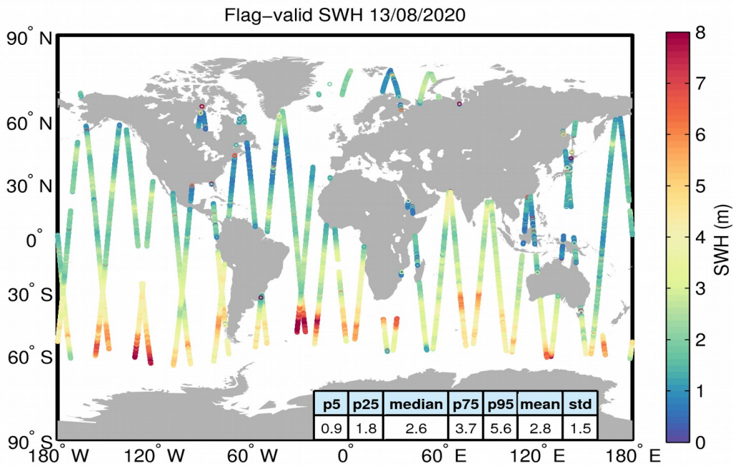
Figure 15. Geographical distribution of flag-valid SWH data over oceans and lakes for 13/08/2020. The statistical values shown in the table refer to the SWH in m and are calculated over all measurements shown in the figure.
