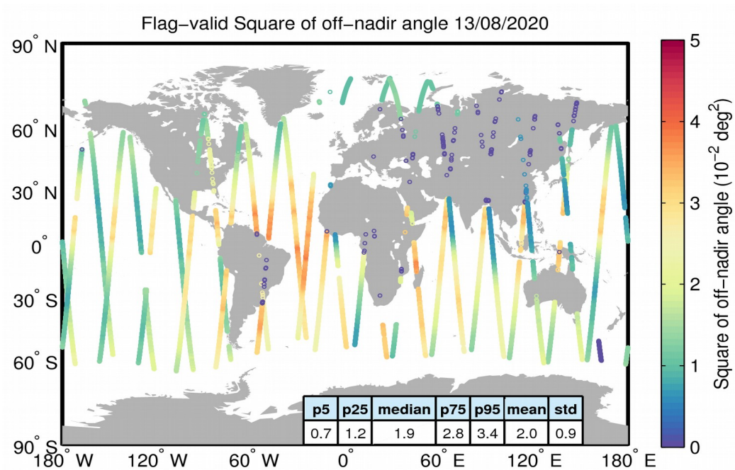
Figure 37. Geographical distribution of flag-valid mispointing data over oceans and lakes for 13/08/2020. The statistical values shown in the table refer to the mispointing in 10^{-2} \text{ deg}^2 and are calculated over all measurements shown in the figure.
