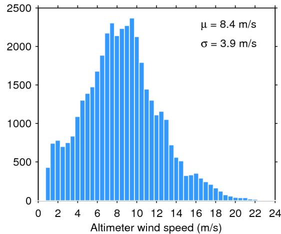
Figure 33. Histogram of flag-valid wind over oceans and lakes for 13/08/2020. The mean ( \mu ) and standard deviation ( \sigma ) are also shown. Note that values larger than 24 m/s are excluded from the histogram for the sake of readability but not from the computation of \mu and \sigma .
