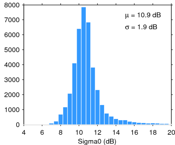
Figure 25. Histogram of flag-valid sigma0 over oceans and lakes for 13/08/2020. The mean ( \mu ) and standard deviation ( \sigma ) are also shown. Note that values outside [4 20] dB are excluded from the histogram for the sake of readability but not from the computation of \mu and \sigma .
