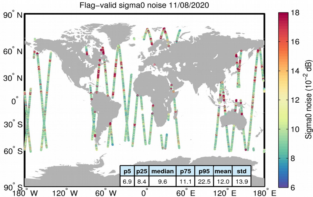
Figure 26. Geographical distribution of flag-valid 20-Hz sigma0 measurement noise over oceans and lakes for 11/08/2020. The statistical values shown in the table refer to the sigma0 noise and are calculated over all measurements shown in the figure.
