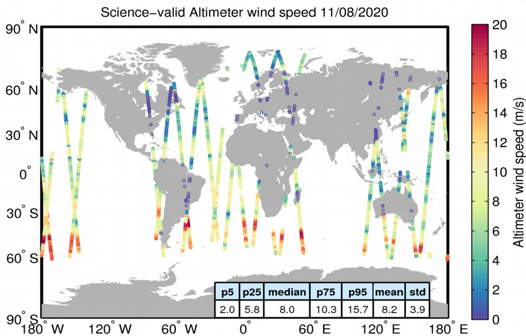
Figure 34. Geographical distribution of science-valid wind data over oceans and lakes for 11/08/2020. The statistical values shown in the table refer to the wind in m/s and are calculated over all measurements shown in the figure. Gray circles denote records that have been rejected based on the editing criteria described in Table 5.
