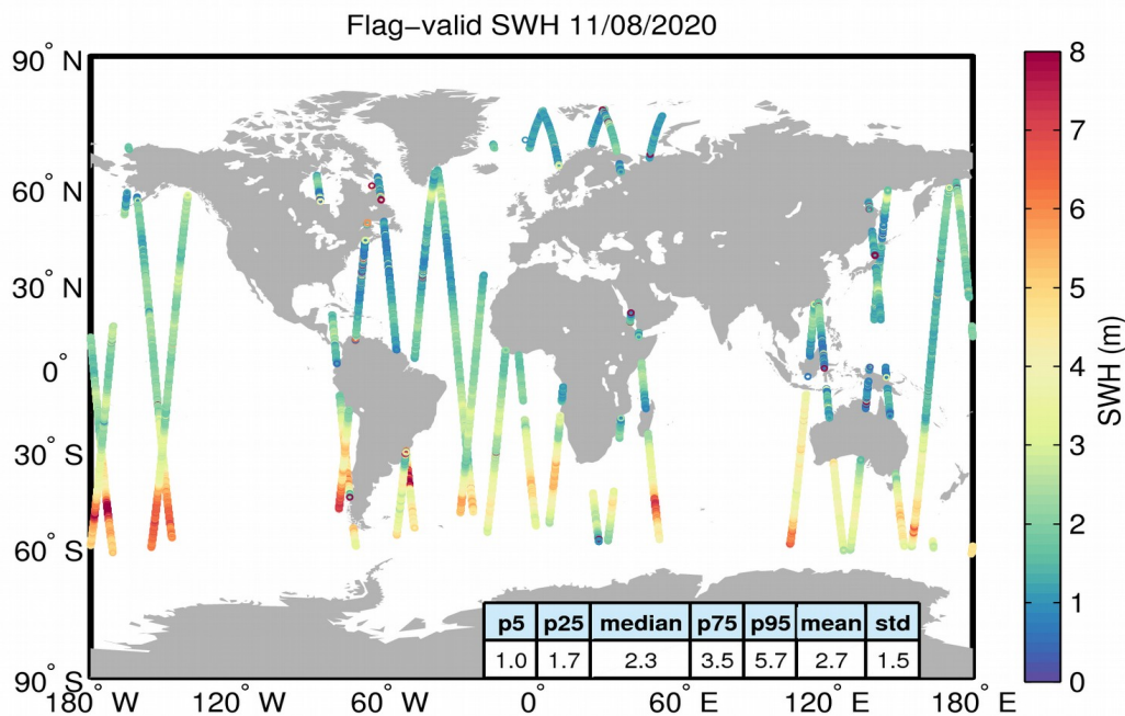
Figure 15. Geographical distribution of flag-valid SWH data over oceans and lakes for 11/08/2020. The statistical values shown in the table refer to the SWH in m and are calculated over all measurements shown in the figure.
