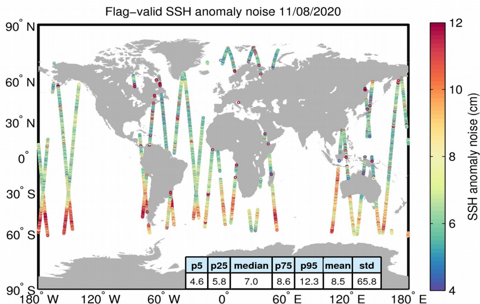
Figure 8. Geographical distribution of flag-valid 20-Hz SSH anomaly measurement noise over oceans and lakes for 11/08/2020. The statistical values shown in the table refer to the SSH anomaly noise and are calculated over all measurements shown in the figure.
