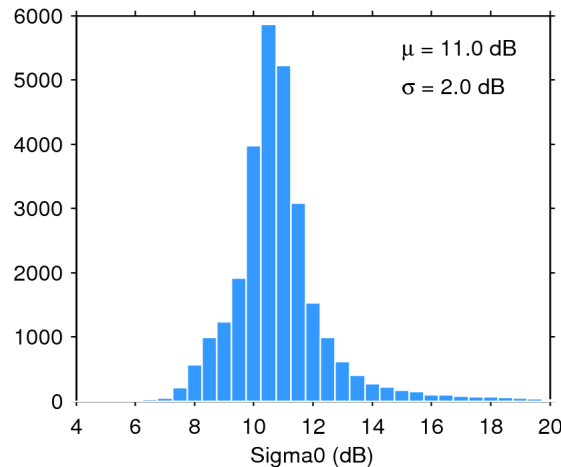
Figure 25. Histogram of flag-valid sigma0 over oceans and lakes for 11/08/2020. The mean ( \mu ) and standard deviation ( \sigma ) are also shown. Note that values outside [4 20] dB are excluded from the histogram for the sake of readability but not from the computation of \mu and \sigma .
