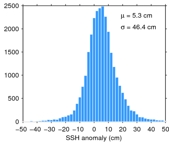
Figure 7. Histogram of flag-valid SSH anomaly over oceans and lakes for 11/08/2020. The mean ( \mu ) and standard deviation ( \sigma ) are also shown. Note that values outside [-50 50] cm are excluded from the histogram for the sake of readability but not from the computation of \mu and \sigma .
