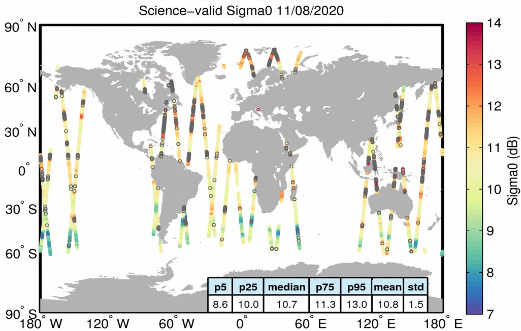
Figure 27. Geographical distribution of science-valid sigma0 data over oceans and lakes for 11/08/2020. The statistical values shown in the table refer to the sigma0 in dB and are calculated over all measurements shown in the figure. Gray circles denote records that have been rejected based on the editing criteria described in Table 4.
