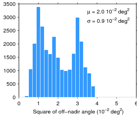
Figure 39. Histogram of flag-valid mispointing over oceans and lakes for 11/08/2020. The mean ( \mu ) and standard deviation ( \sigma ) are also shown. Note that values larger than 6 \cdot 10^{-2} \text{ deg}^2 are excluded from the histogram for the sake of readability but not from the computation of \mu and \sigma .
