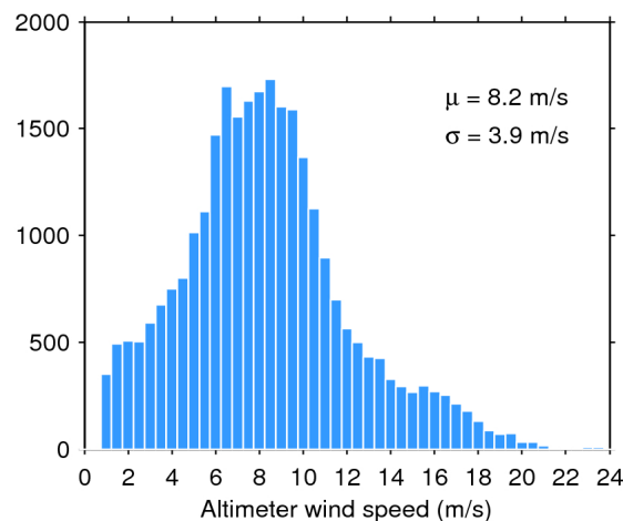
Figure 35. Histogram of science-valid wind over oceans and lakes for 11/08/2020. The mean ( \mu ) and standard deviation ( \sigma ) are also shown. Note that values larger than 24 m/s are excluded from the histogram for the sake of readability but not from the computation of \mu and \sigma .
