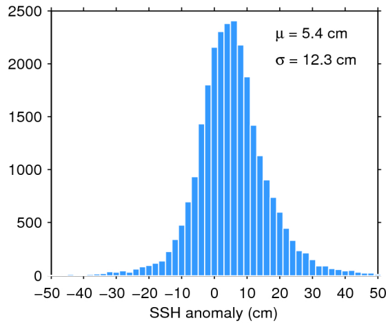
Figure 11. Histogram of science-valid SSH anomaly over oceans and lakes for 11/08/2020. The mean ( \mu ) and standard deviation ( \sigma ) are also shown. Note that values outside [-50 50] cm are excluded from the histogram for the sake of readability but not from the computation of \mu and \sigma .
