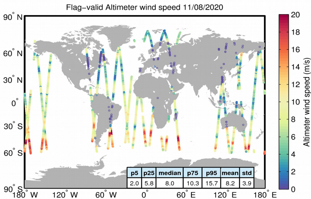
Figure 31. Geographical distribution of flag-valid wind data over oceans and lakes for 11/08/2020. The statistical values shown in the table refer to the wind in m/s and are calculated over all measurements shown in the figure.
