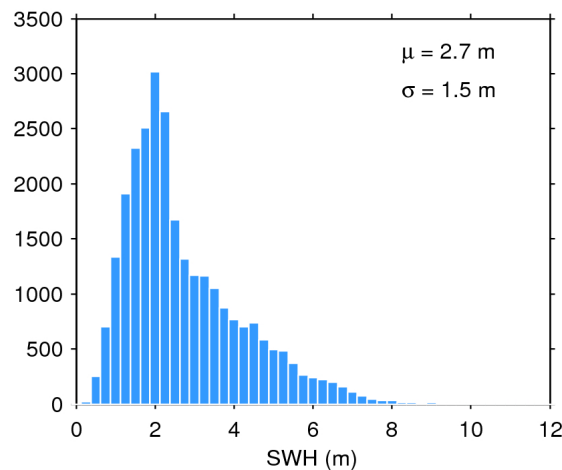
Figure 20. Histogram of science-valid SWH over oceans and lakes for 11/08/2020. The mean ( \mu ) and standard deviation ( \sigma ) are also shown. Note that values larger than 12 m are excluded from the histogram for the sake of readability but not from the computation of \mu and \sigma .
