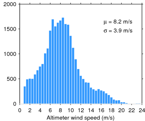
Figure 33. Histogram of flag-valid wind over oceans and lakes for 11/08/2020. The mean ( \mu ) and standard deviation ( \sigma ) are also shown. Note that values larger than 24 m/s are excluded from the histogram for the sake of readability but not from the computation of \mu and \sigma .
