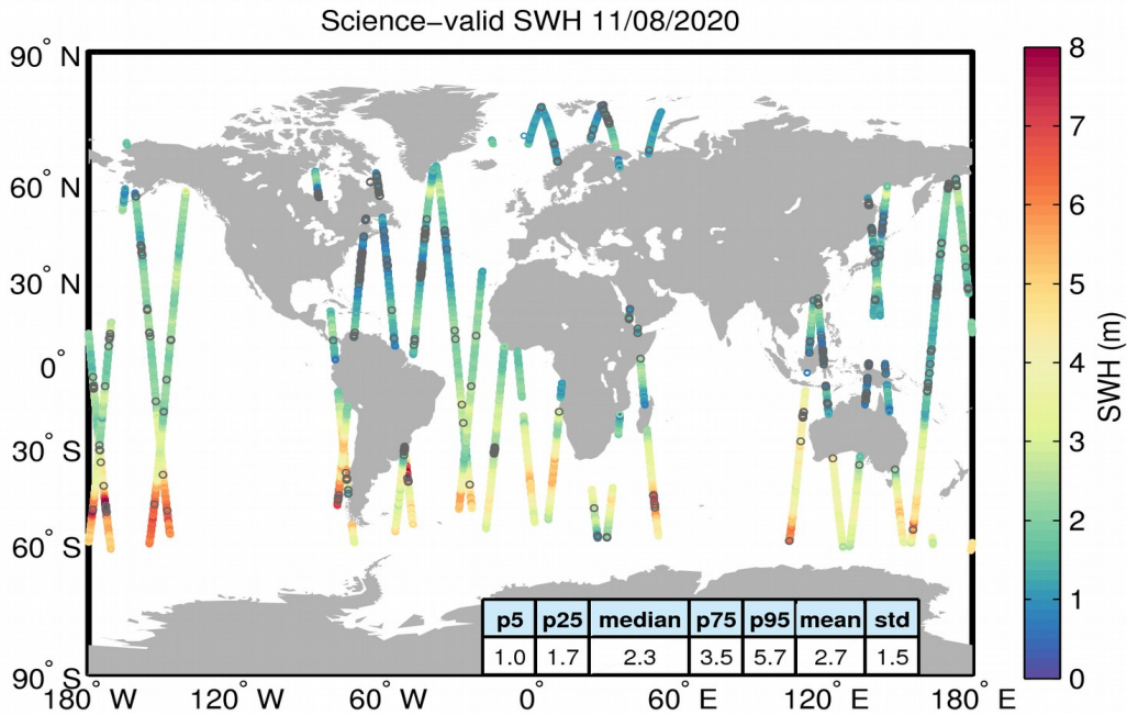
Figure 19. Geographical distribution of science-valid SWH data over oceans and lakes for 11/08/2020. The statistical values shown in the table refer to the SWH in m and are calculated over all measurements shown in the figure. Gray circles denote records that have been rejected based on the editing criteria described in Table 3.
