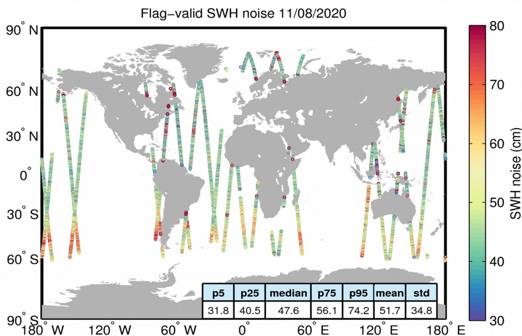
Figure 18. Geographical distribution of flag-valid 20-Hz SWH measurement noise over oceans and lakes for 11/08/2020. The statistical values shown in the figure refer to the SWH noise and are calculated over all measurements shown in the figure.
