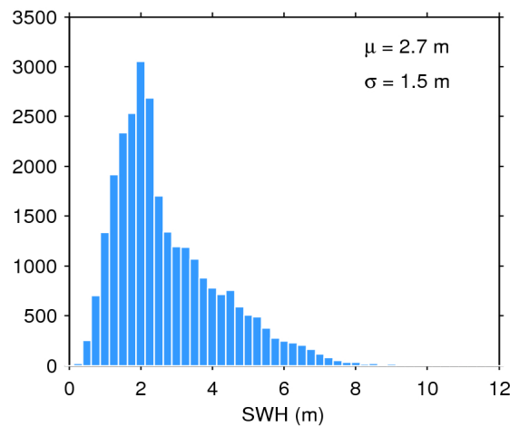
Figure 17. Histogram of flag-valid SWH over oceans and lakes for 11/08/2020. The mean ( \mu ) and standard deviation ( \sigma ) are also shown. Note that values larger than 12 m are excluded from the histogram for the sake of readability but not from the computation of \mu and \sigma .
