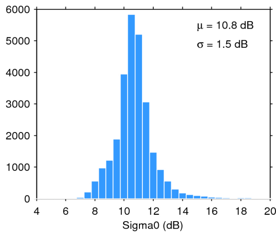
Figure 28. Histogram of science-valid sigma0 over oceans and lakes for 11/08/2020. The mean ( \mu ) and standard deviation ( \sigma ) are also shown. Note that values outside [4 20] dB are excluded from the histogram for the sake of readability but not from the computation of \mu and \sigma .
