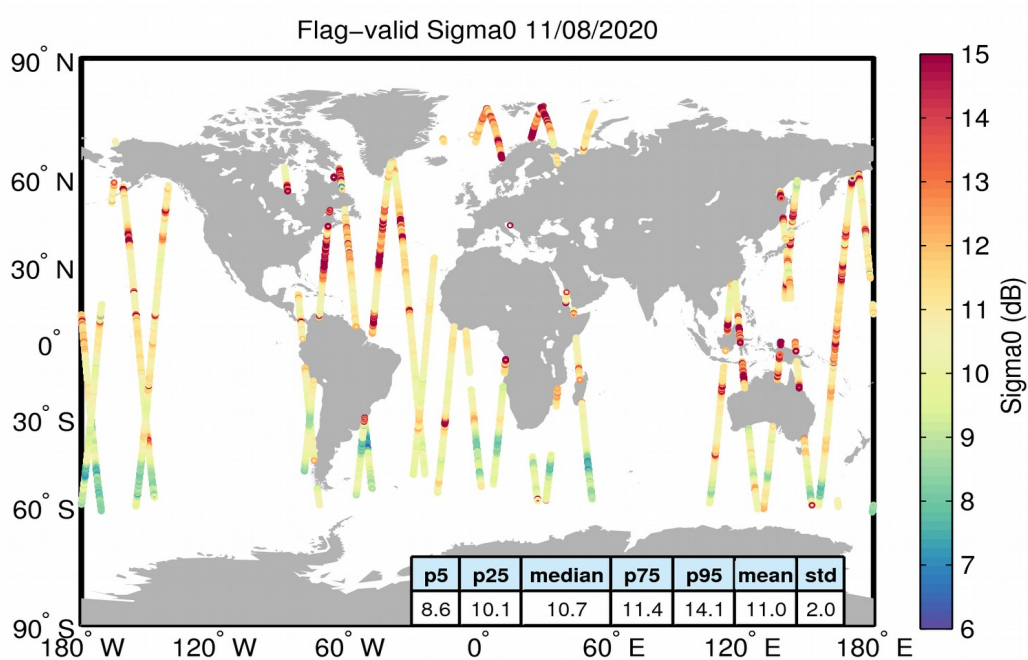
Figure 23. Geographical distribution of flag-valid sigma0 data over oceans and lakes for 11/08/2020. The statistical values shown in the table refer to the sigma0 in dB and are calculated over all measurements shown in the figure.
