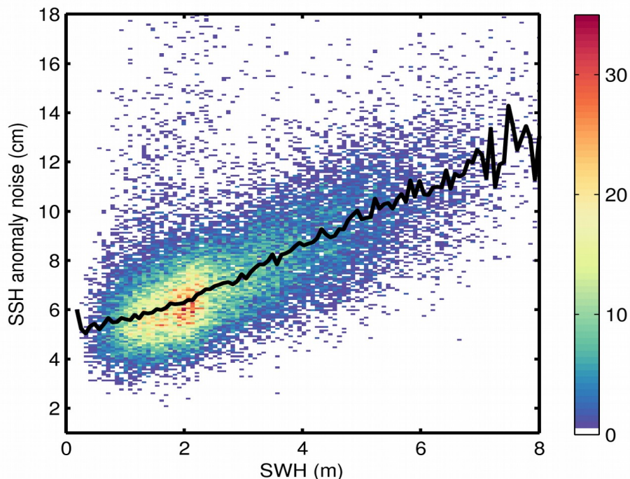
Figure 9. 2D histogram showing flag-valid SSH anomaly noise as a function of SWH for 11/08/2020. The black line denotes the median SSH anomaly noise as a function of SWH.
