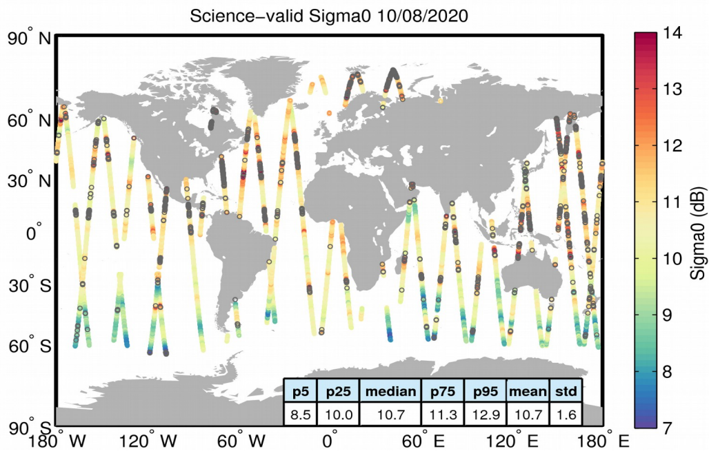
Figure 27. Geographical distribution of science-valid sigma0 data over oceans and lakes for 10/08/2020. The statistical values shown in the table refer to the sigma0 in dB and are calculated over all measurements shown in the figure. Gray circles denote records that have been rejected based on the editing criteria described in Table 4.
