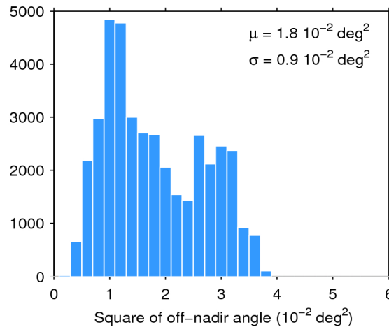
Figure 39. Histogram of flag-valid mispointing over oceans and lakes for 10/08/2020. The mean ( \mu ) and standard deviation ( \sigma ) are also shown. Note that values larger than 6 \cdot 10^{-2} \text{ deg}^2 are excluded from the histogram for the sake of readability but not from the computation of \mu and \sigma .
