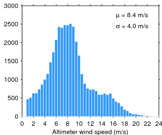
Figure 35. Histogram of science-valid wind over oceans and lakes for 10/08/2020. The mean ( \mu ) and standard deviation ( \sigma ) are also shown. Note that values larger than 24 m/s are excluded from the histogram for the sake of readability but not from the computation of \mu and \sigma .
