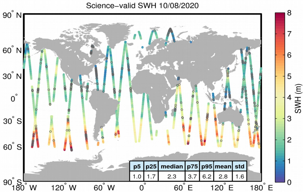
Figure 19. Geographical distribution of science-valid SWH data over oceans and lakes for 10/08/2020. The statistical values shown in the table refer to the SWH in m and are calculated over all measurements shown in the figure. Gray circles denote records that have been rejected based on the editing criteria described in Table 3.
