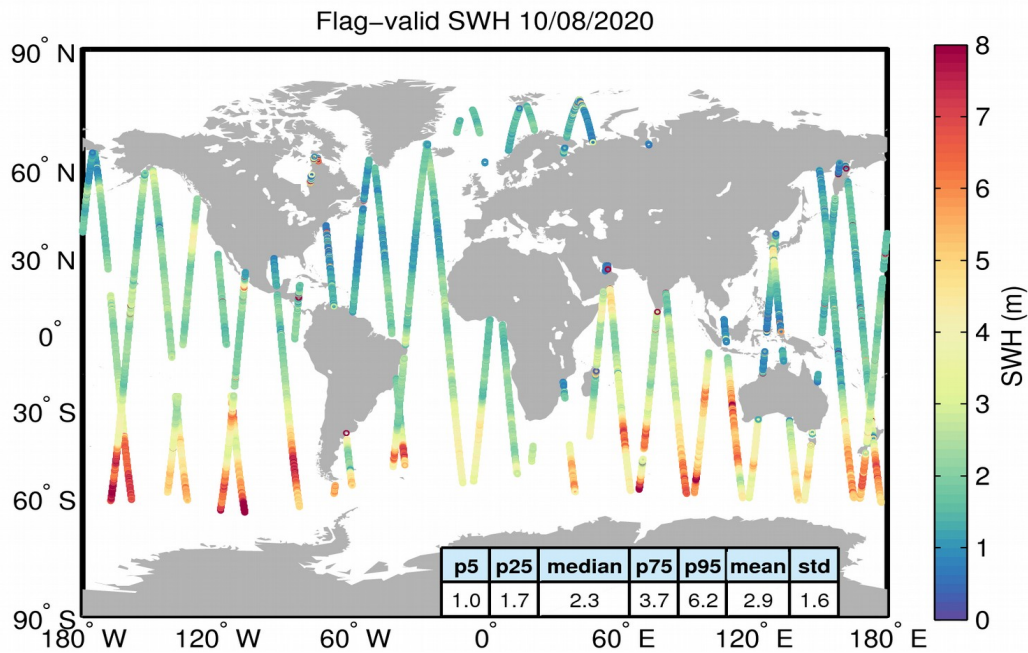
Figure 15. Geographical distribution of flag-valid SWH data over oceans and lakes for 10/08/2020. The statistical values shown in the table refer to the SWH in m and are calculated over all measurements shown in the figure.
