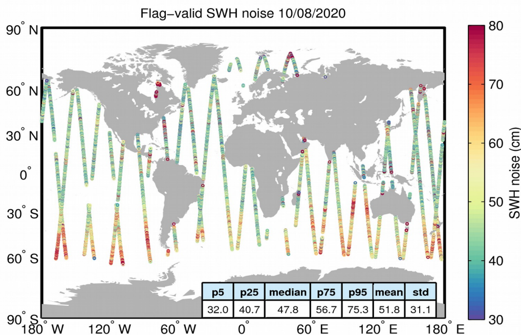
Figure 18. Geographical distribution of flag-valid 20-Hz SWH measurement noise over oceans and lakes for 10/08/2020. The statistical values shown in the table refer to the SWH noise and are calculated over all measurements shown in the figure.
