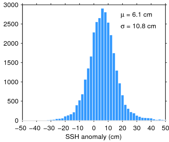
Figure 11. Histogram of science-valid SSH anomaly over oceans and lakes for 10/08/2020. The mean ( \mu ) and standard deviation ( \sigma ) are also shown. Note that values outside [-50 50] cm are excluded from the histogram for the sake of readability but not from the computation of \mu and \sigma .
