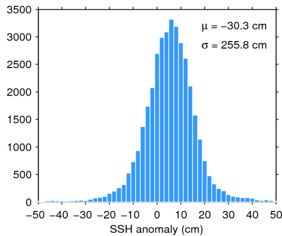
Figure 7. Histogram of flag-valid SSH anomaly over oceans and lakes for 10/08/2020. The mean ( \mu ) and standard deviation ( \sigma ) are also shown. Note that values outside [-50\ 50] cm are excluded from the histogram for the sake of readability but not from the computation of \mu and \sigma .
