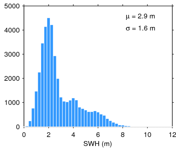
Figure 17. Histogram of flag-valid SWH over oceans and lakes for 10/08/2020. The mean ( \mu ) and standard deviation ( \sigma ) are also shown. Note that values larger than 12 m are excluded from the histogram for the sake of readability but not from the computation of \mu and \sigma .
