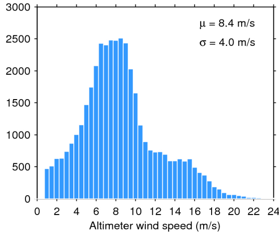
Figure 33. Histogram of flag-valid wind over oceans and lakes for 10/08/2020. The mean ( \mu ) and standard deviation ( \sigma ) are also shown. Note that values larger than 24 m/s are excluded from the histogram for the sake of readability but not from the computation of \mu and \sigma .
