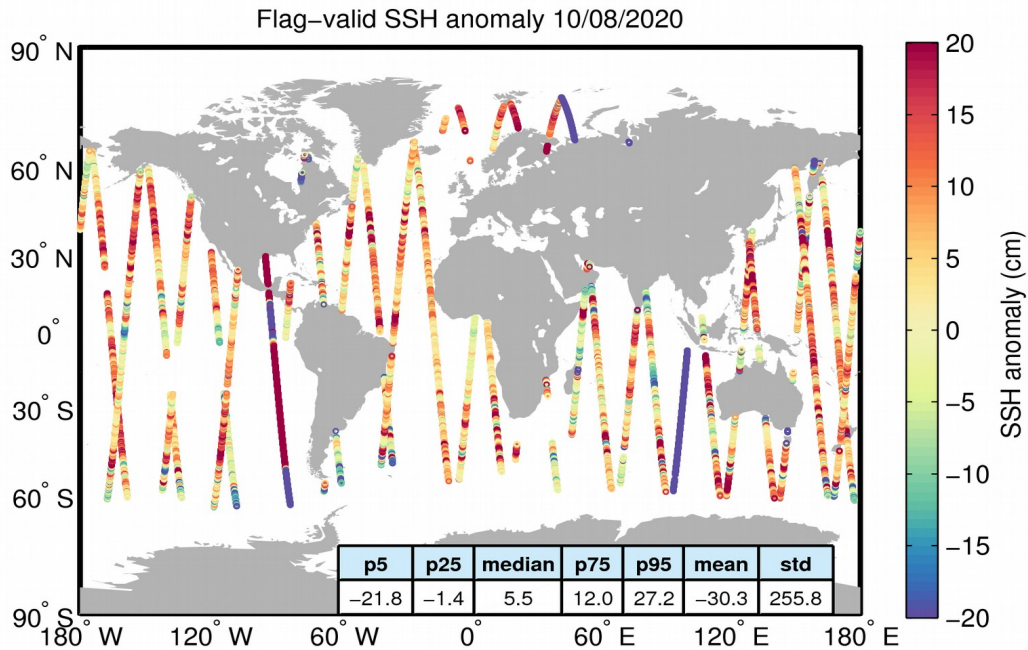
Figure 5. Geographical distribution of flag-valid 1-Hz SSH anomaly data over oceans and lakes for 10/08/2020. The statistical values shown in the table refer to the SSH anomaly in cm and are calculated over all measurements shown in the figure.
