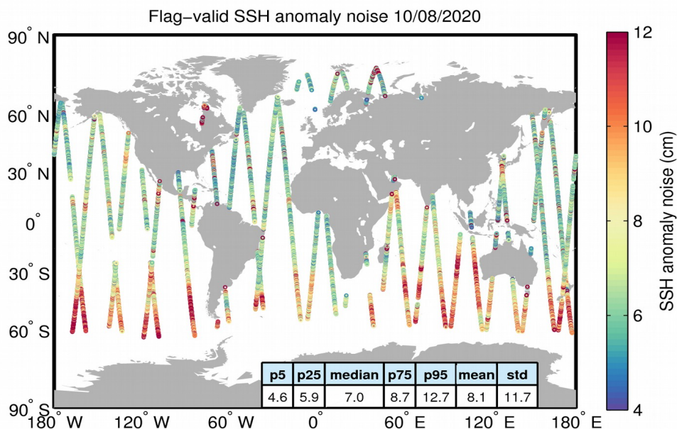
Figure 8. Geographical distribution of flag-valid 20-Hz SSH anomaly measurement noise over oceans and lakes for 10/08/2020. The statistical values shown in the table refer to the SSH anomaly noise and are calculated over all measurements shown in the figure.
