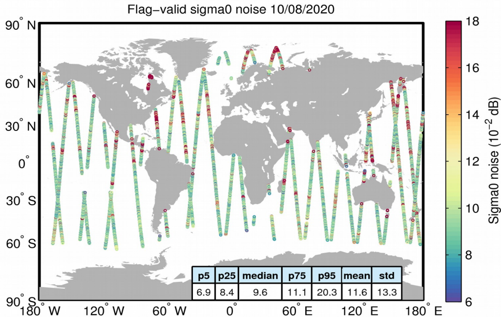
Figure 26. Geographical distribution of flag-valid 20-Hz sigma0 measurement noise over oceans and lakes for 10/08/2020. The statistical values shown in the table refer to the sigma0 noise and are calculated over all measurements shown in the figure.
