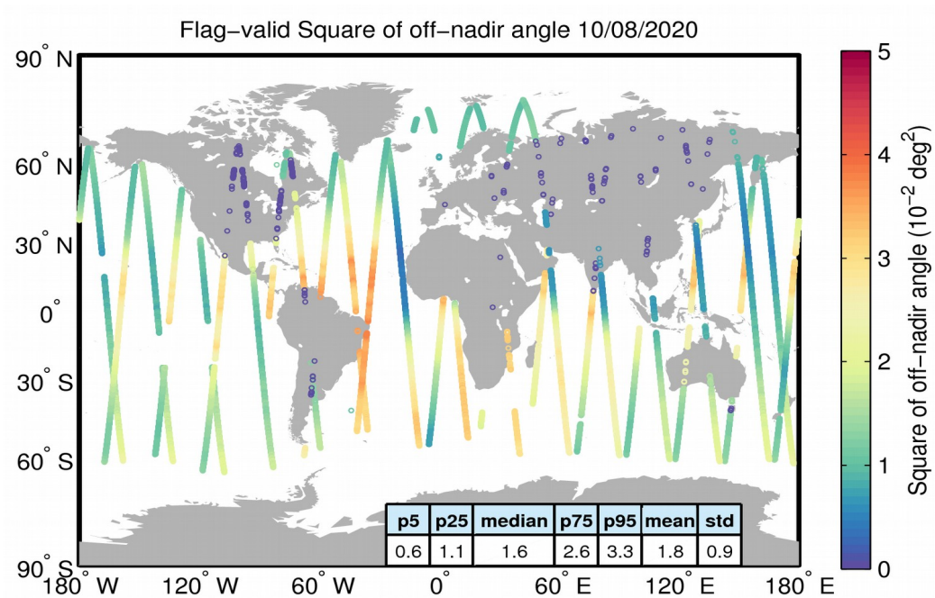
Figure 37. Geographical distribution of flag-valid mispointing data over oceans and lakes for 10/08/2020. The statistical values shown in the table refer to the mispointing in 10^{-2} deg 2 and are calculated over all measurements shown in the figure.
