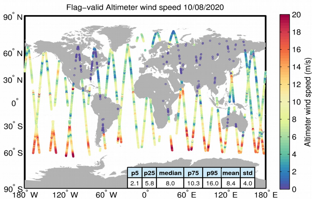
Figure 31. Geographical distribution of flag-valid wind data over oceans and lakes for 10/08/2020. The statistical values shown in the table refer to the wind in m/s and are calculated over all measurements shown in the figure.
