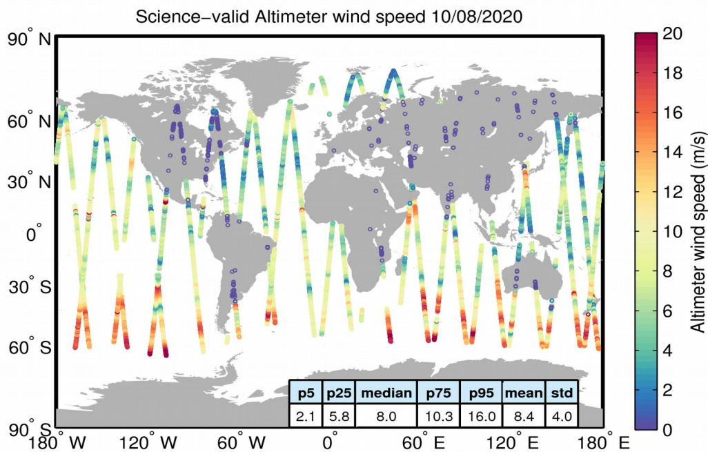
Figure 34. Geographical distribution of science-valid wind data over oceans and lakes for 10/08/2020. The statistical values shown in the table refer to the wind in m/s and are calculated over all measurements shown in the figure. Gray circles denote records that have been rejected based on the editing criteria described in Table 5.
