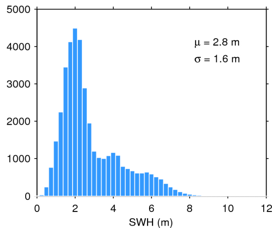
Figure 20. Histogram of science-valid SWH over oceans and lakes for 10/08/2020. The mean ( \mu ) and standard deviation ( \sigma ) are also shown. Note that values larger than 12 m are excluded from the histogram for the sake of readability but not from the computation of \mu and \sigma .
