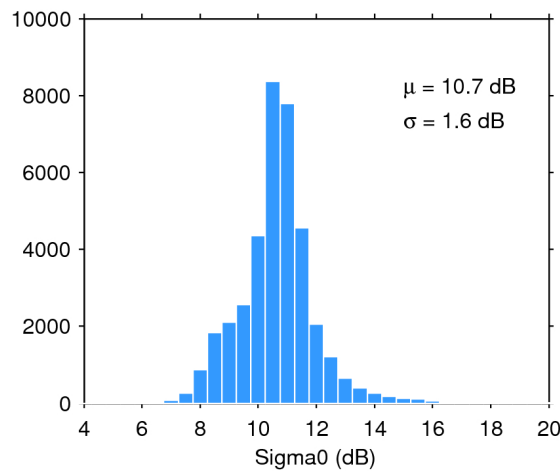
Figure 28. Histogram of science-valid sigma0 over oceans and lakes for 10/08/2020. The mean ( \mu ) and standard deviation ( \sigma ) are also shown. Note that values outside [4 20] dB are excluded from the histogram for the sake of readability but not from the computation of \mu and \sigma .
