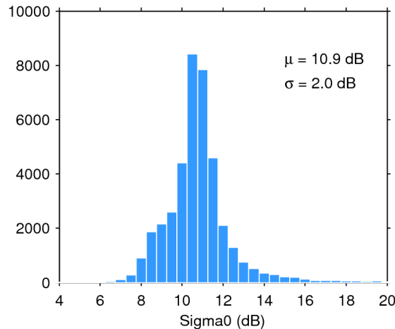
Figure 25. Histogram of flag-valid sigma0 over oceans and lakes for 10/08/2020. The mean ( \mu ) and standard deviation ( \sigma ) are also shown. Note that values outside [4 20] dB are excluded from the histogram for the sake of readability but not from the computation of \mu and \sigma .
