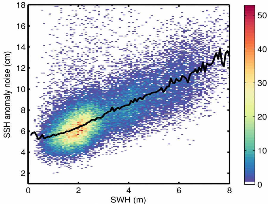
Figure 9. 2D histogram showing flag-valid SSH anomaly noise as a function of SWH for 10/08/2020. The black line denotes the median SSH anomaly noise as a function of SWH.
