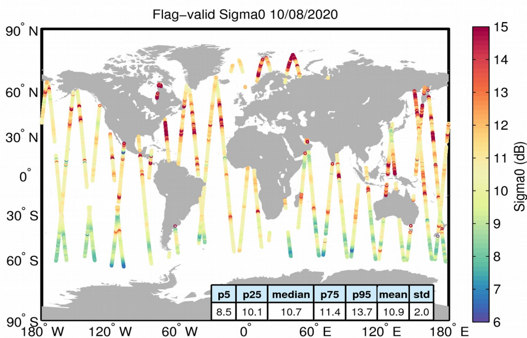
Figure 23. Geographical distribution of flag-valid sigma0 data over oceans and lakes for 10/08/2020. The statistical values shown in the table refer to the sigma0 in dB and are calculated over all measurements shown in the figure.
