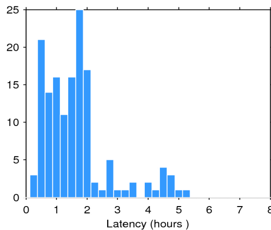
Figure 2. Histogram of the data latency for 09/08/2020. The y-axis denotes the number of files that are made available with a delay of x-hours with respect to the mean time of the records stored in the file.
