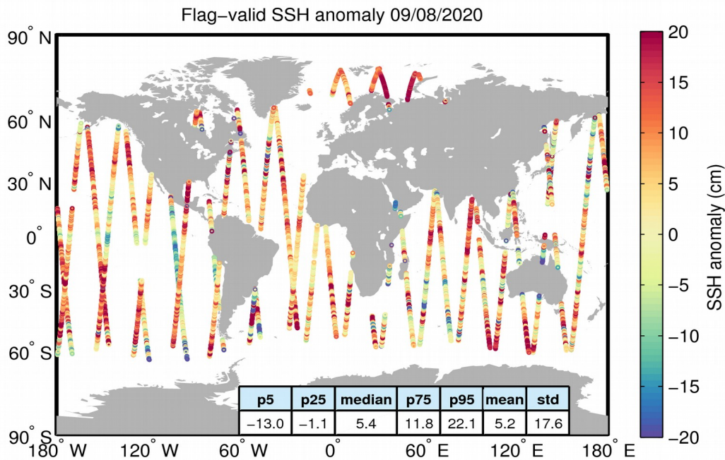
Figure 5. Geographical distribution of flag-valid 1-Hz SSH anomaly data over oceans and lakes for 09/08/2020. The statistical values shown in the table refer to the SSH anomaly in cm and are calculated over all measurements shown in the figure.
