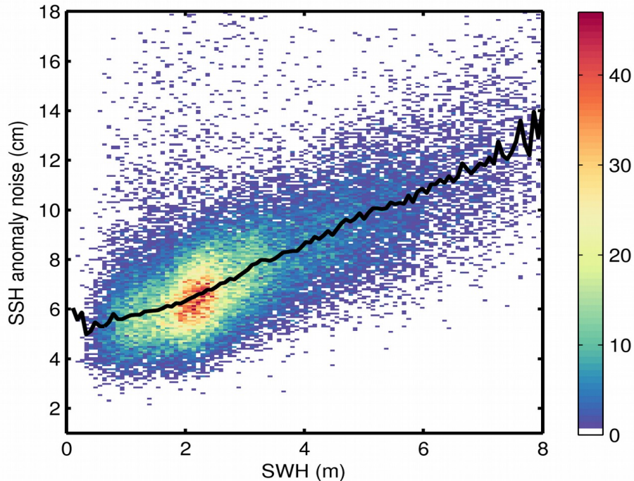
Figure 9. 2D histogram showing flag-valid SSH anomaly noise as a function of SWH for 09/08/2020. The black line denotes the median SSH anomaly noise as a function of SWH.
