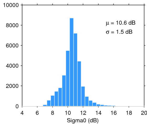
Figure 28. Histogram of science-valid sigma0 over oceans and lakes for 09/08/2020. The mean ( \mu ) and standard deviation ( \sigma ) are also shown. Note that values outside [4 20] dB are excluded from the histogram for the sake of readability but not from the computation of \mu and \sigma .
