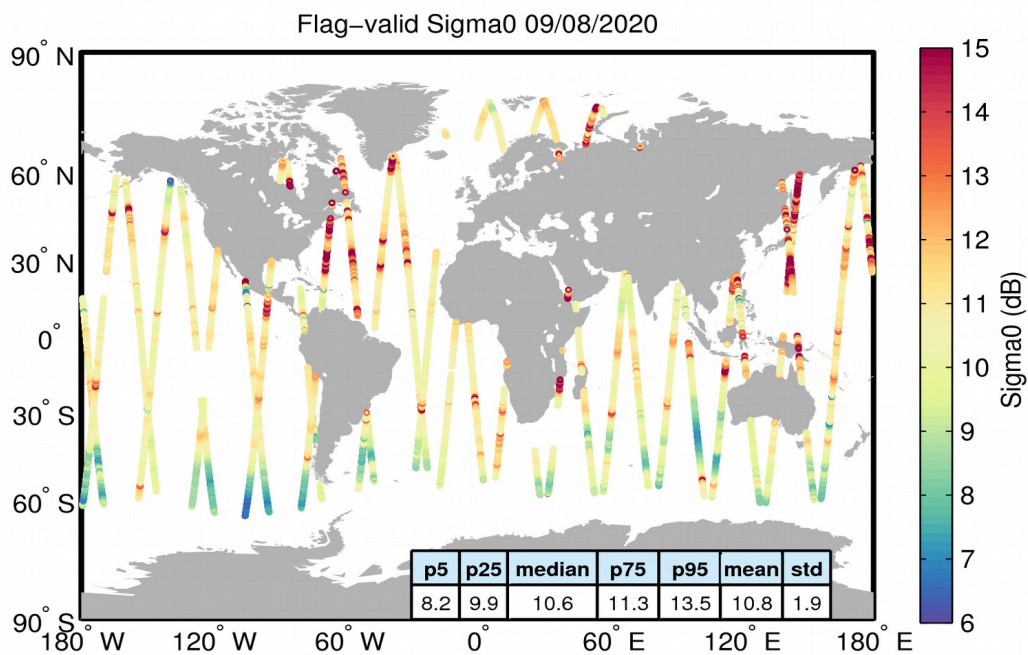
Figure 23. Geographical distribution of flag-valid sigma0 data over oceans and lakes for 09/08/2020. The statistical values shown in the table refer to the sigma0 in dB and are calculated over all measurements shown in the figure.
