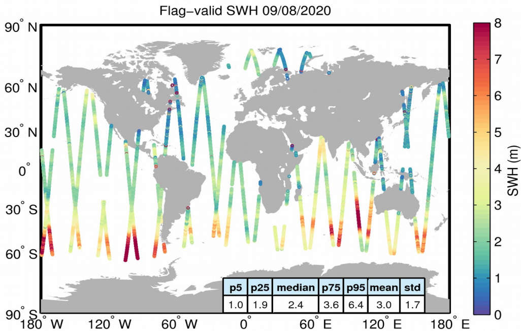
Figure 15. Geographical distribution of flag-valid SWH data over oceans and lakes for 09/08/2020. The statistical values shown in the table refer to the SWH in m and are calculated over all measurements shown in the figure.
