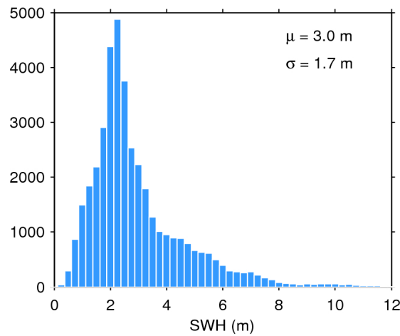
Figure 17. Histogram of flag-valid SWH over oceans and lakes for 09/08/2020. The mean ( \mu ) and standard deviation ( \sigma ) are also shown. Note that values larger than 12 m are excluded from the histogram for the sake of readability but not from the computation of \mu and \sigma .
