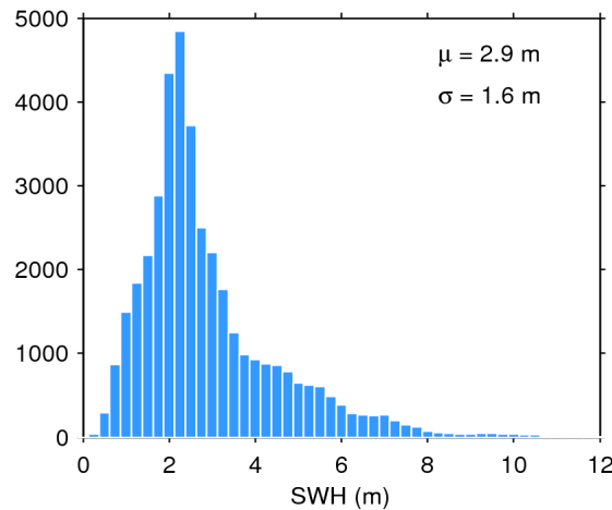
Figure 20. Histogram of science-valid SWH over oceans and lakes for 09/08/2020. The mean ( \mu ) and standard deviation ( \sigma ) are also shown. Note that values larger than 12 m are excluded from the histogram for the sake of readability but not from the computation of \mu and \sigma .
