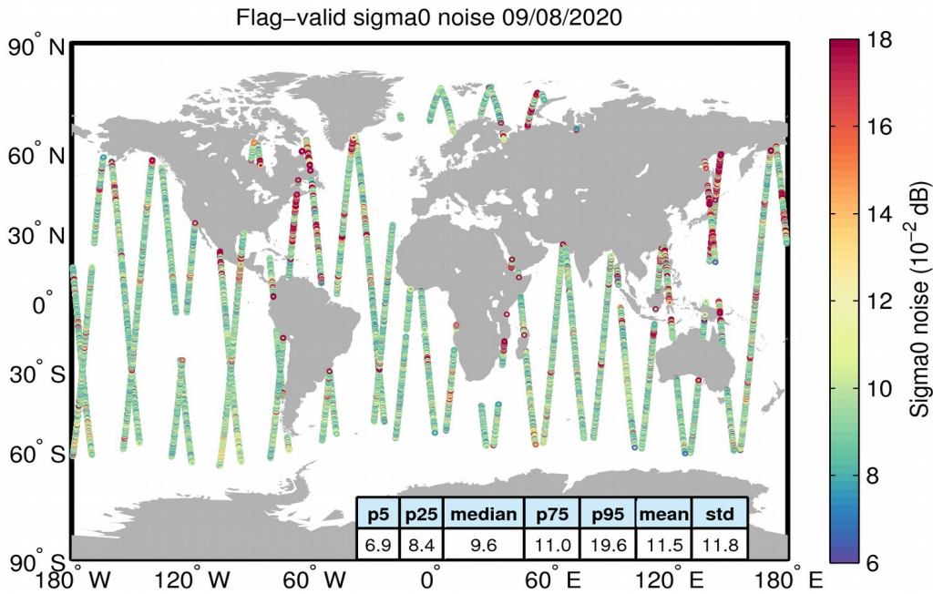
Figure 26. Geographical distribution of flag-valid 20-Hz sigma0 measurement noise over oceans and lakes for 09/08/2020. The statistical values shown in the table refer to the sigma0 noise and are calculated over all measurements shown in the figure.
