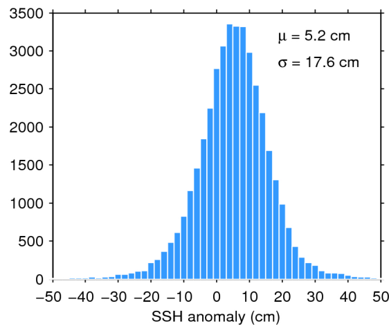
Figure 7. Histogram of flag-valid SSH anomaly over oceans and lakes for 09/08/2020. The mean ( \mu ) and standard deviation ( \sigma ) are also shown. Note that values outside [-50\ 50] cm are excluded from the histogram for the sake of readability but not from the computation of \mu and \sigma .
