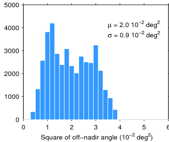
Figure 39. Histogram of flag-valid mispointing over oceans and lakes for 09/08/2020. The mean ( \mu ) and standard deviation ( \sigma ) are also shown. Note that values larger than 6 \cdot 10^{-2} \text{ deg}^2 are excluded from the histogram for the sake of readability but not from the computation of \mu and \sigma .
