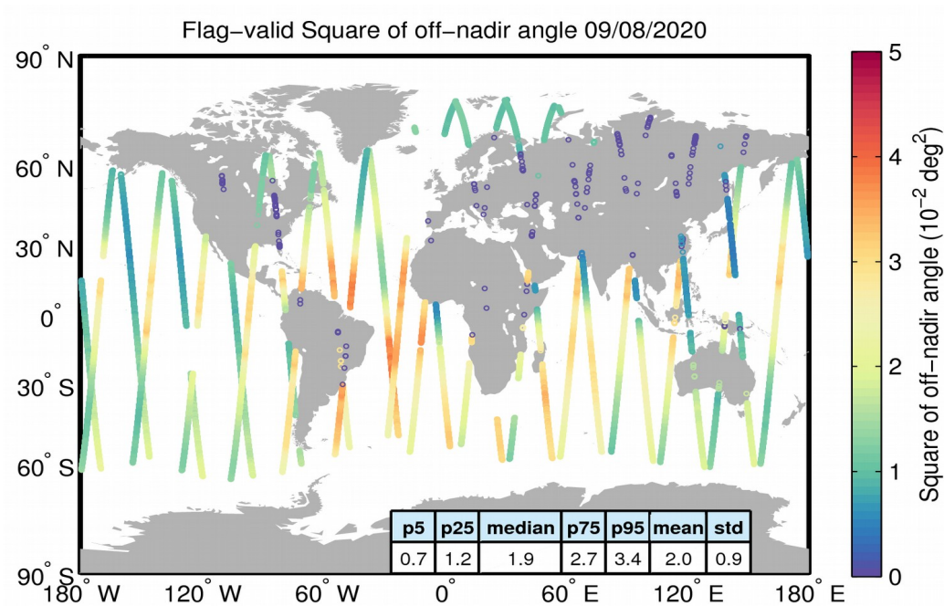
Figure 37. Geographical distribution of flag-valid mispointing data over oceans and lakes for 09/08/2020. The statistical values shown in the table refer to the mispointing in 10^{-2} \text{ deg}^2 and are calculated over all measurements shown in the figure.
