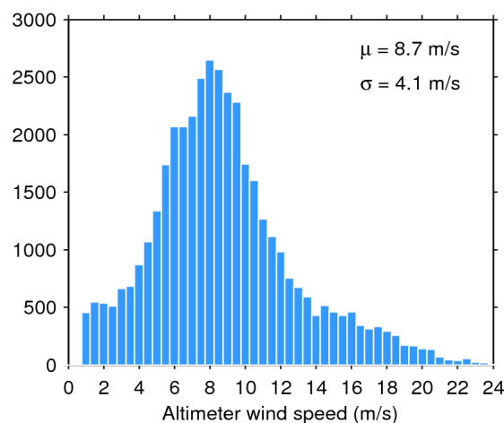
Figure 35. Histogram of science-valid wind over oceans and lakes for 09/08/2020. The mean ( \mu ) and standard deviation ( \sigma ) are also shown. Note that values larger than 24 m/s are excluded from the histogram for the sake of readability but not from the computation of \mu and \sigma .
