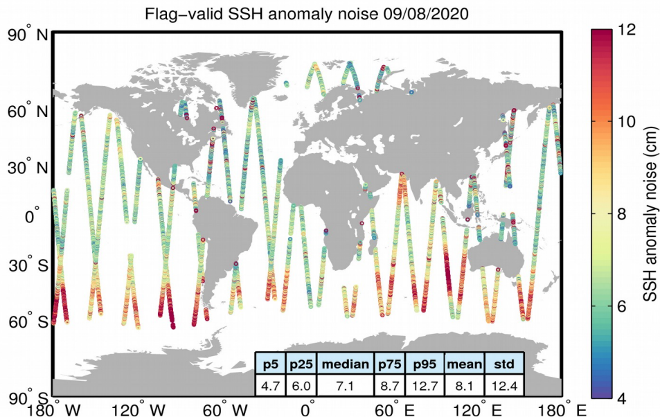
Figure 8. Geographical distribution of flag-valid 20-Hz SSH anomaly measurement noise over oceans and lakes for 09/08/2020. The statistical values shown in the table refer to the SSH anomaly noise and are calculated over all measurements shown in the figure.
