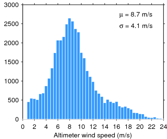
Figure 33. Histogram of flag-valid wind over oceans and lakes for 09/08/2020. The mean ( \mu ) and standard deviation ( \sigma ) are also shown. Note that values larger than 24 m/s are excluded from the histogram for the sake of readability but not from the computation of \mu and \sigma .
