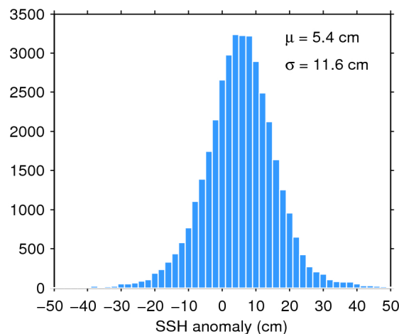
Figure 11. Histogram of science-valid SSH anomaly over oceans and lakes for 09/08/2020. The mean ( \mu ) and standard deviation ( \sigma ) are also shown. Note that values outside [-50 50] cm are excluded from the histogram for the sake of readability but not from the computation of \mu and \sigma .
