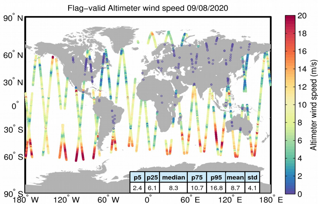
Figure 31. Geographical distribution of flag-valid wind data over oceans and lakes for 09/08/2020. The statistical values shown in the table refer to the wind in m/s and are calculated over all measurements shown in the figure.
