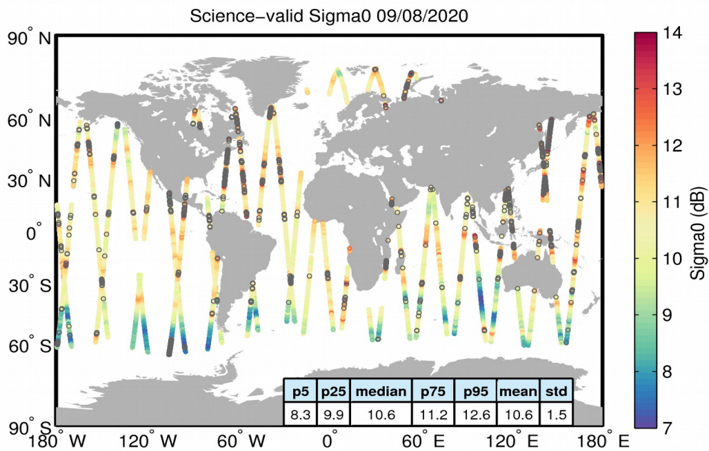
Figure 27. Geographical distribution of science-valid sigma0 data over oceans and lakes for 09/08/2020. The statistical values shown in the table refer to the sigma0 in dB and are calculated over all measurements shown in the figure. Gray circles denote records that have been rejected based on the editing criteria described in Table 4.
