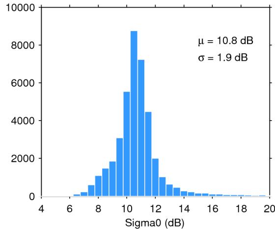
Figure 25. Histogram of flag-valid sigma0 over oceans and lakes for 09/08/2020. The mean ( \mu ) and standard deviation ( \sigma ) are also shown. Note that values outside [4 20] dB are excluded from the histogram for the sake of readability but not from the computation of \mu and \sigma .
