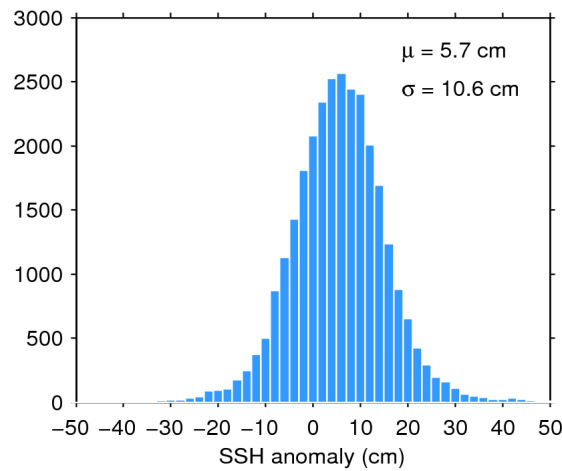
Figure 11. Histogram of science-valid SSH anomaly over oceans and lakes for 08/08/2020. The mean ( \mu ) and standard deviation ( \sigma ) are also shown. Note that values outside [-50 50] cm are excluded from the histogram for the sake of readability but not from the computation of \mu and \sigma .
