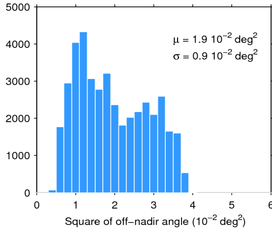
Figure 39. Histogram of flag-valid mispointing over oceans and lakes for 08/08/2020. The mean ( \mu ) and standard deviation ( \sigma ) are also shown. Note that values larger than 6 \cdot 10^{-2} \text{ deg}^2 are excluded from the histogram for the sake of readability but not from the computation of \mu and \sigma .
