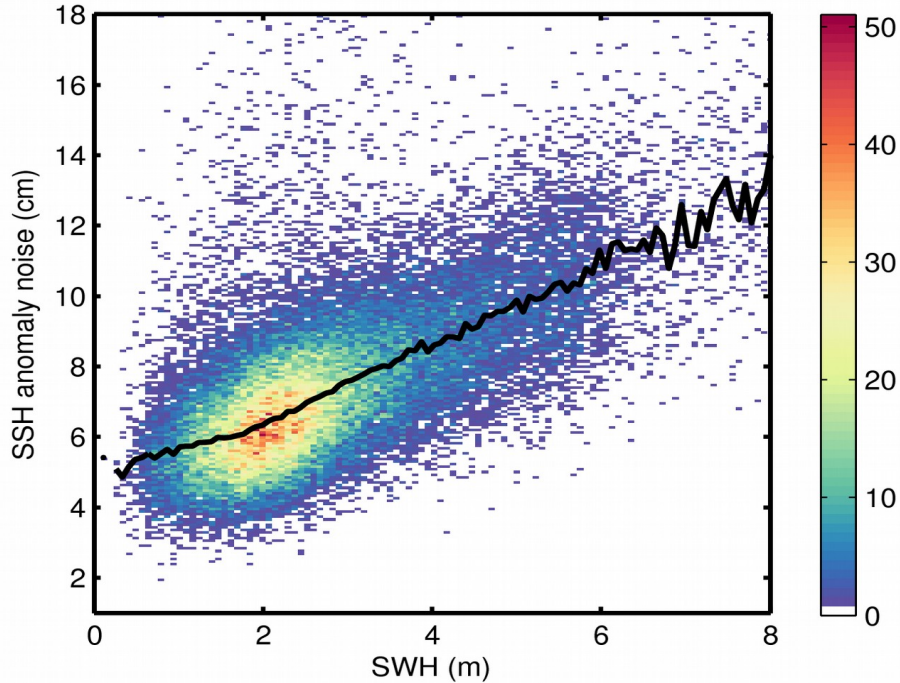
Figure 9. 2D histogram showing flag-valid SSH anomaly noise as a function of SWH for 08/08/2020. The black line denotes the median SSH anomaly noise as a function of SWH.
