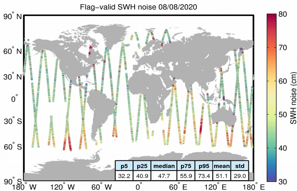
Figure 18. Geographical distribution of flag-valid 20-Hz SWH measurement noise over oceans and lakes for 08/08/2020. The statistical values shown in the table refer to the SWH noise and are calculated over all measurements shown in the figure.
