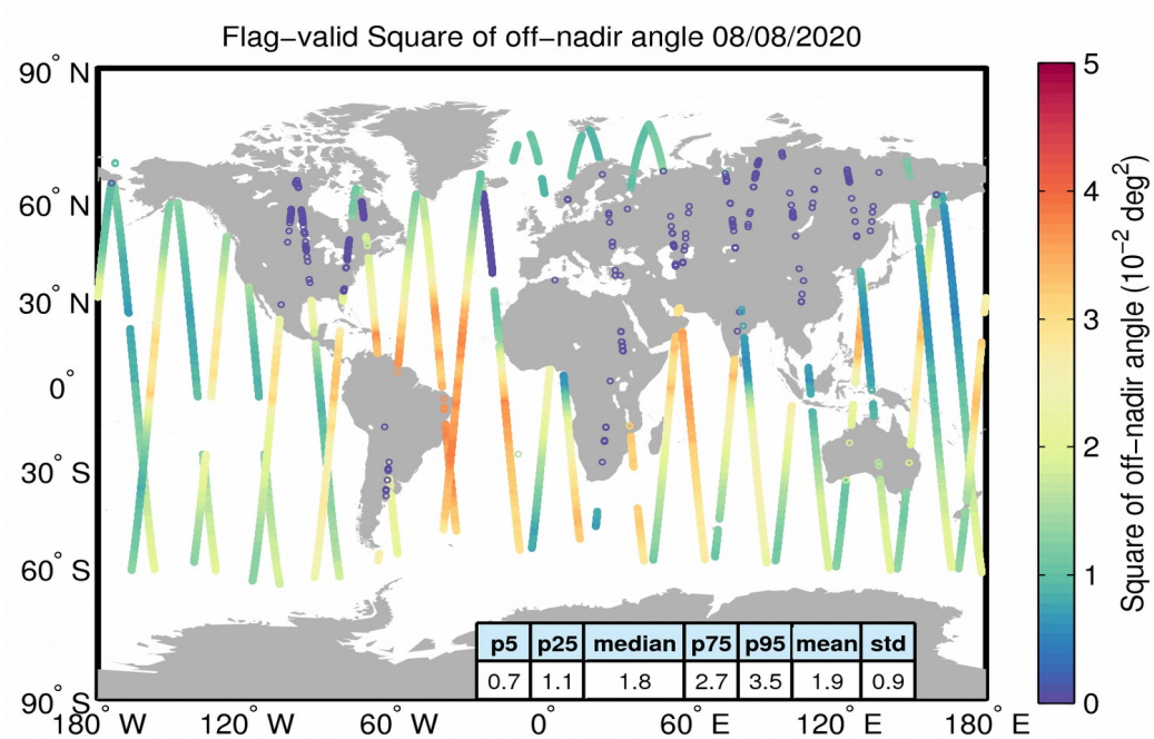
Figure 37. Geographical distribution of flag-valid mispointing data over oceans and lakes for 08/08/2020. The statistical values shown in the table refer to the mispointing in 10^{-2} \text{deg}^2 and are calculated over all measurements shown in the figure.
