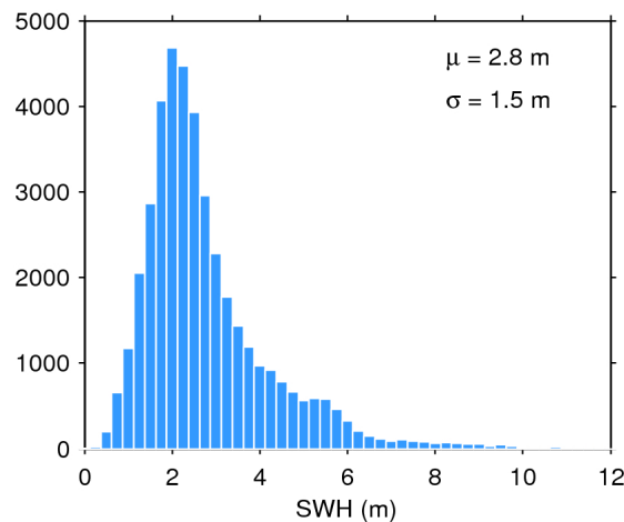
Figure 20. Histogram of science-valid SWH over oceans and lakes for 08/08/2020. The mean ( \mu ) and standard deviation ( \sigma ) are also shown. Note that values larger than 12 m are excluded from the histogram for the sake of readability but not from the computation of \mu and \sigma .
