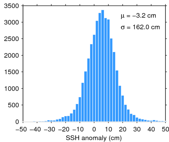
Figure 7. Histogram of flag-valid SSH anomaly over oceans and lakes for 08/08/2020. The mean ( \mu ) and standard deviation ( \sigma ) are also shown. Note that values outside [-50\ 50] cm are excluded from the histogram for the sake of readability but not from the computation of \mu and \sigma .
