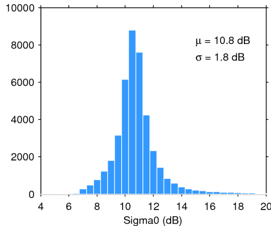
Figure 25. Histogram of flag-valid sigma0 over oceans and lakes for 08/08/2020. The mean ( \mu ) and standard deviation ( \sigma ) are also shown. Note that values outside [4 20] dB are excluded from the histogram for the sake of readability but not from the computation of \mu and \sigma .
