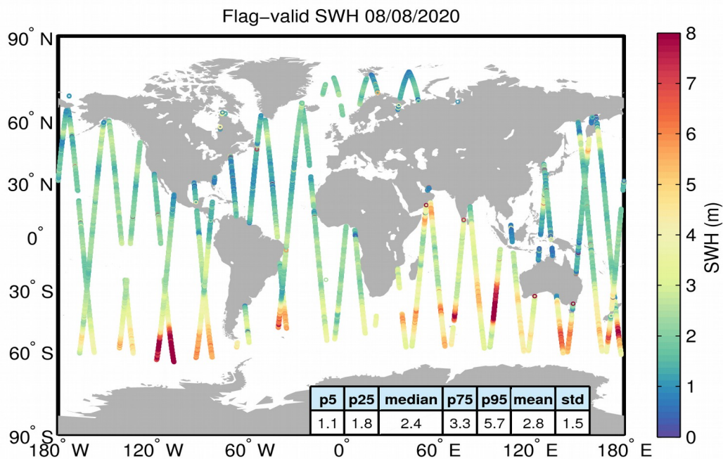
Figure 15. Geographical distribution of flag-valid SWH data over oceans and lakes for 08/08/2020. The statistical values shown in the table refer to the SWH in m and are calculated over all measurements shown in the figure.
