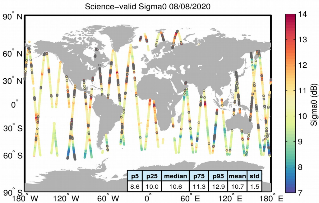
Figure 27. Geographical distribution of science-valid sigma0 data over oceans and lakes for 08/08/2020. The statistical values shown in the table refer to the sigma0 in dB and are calculated over all measurements shown in the figure. Gray circles denote records that have been rejected based on the editing criteria described in Table 4.
