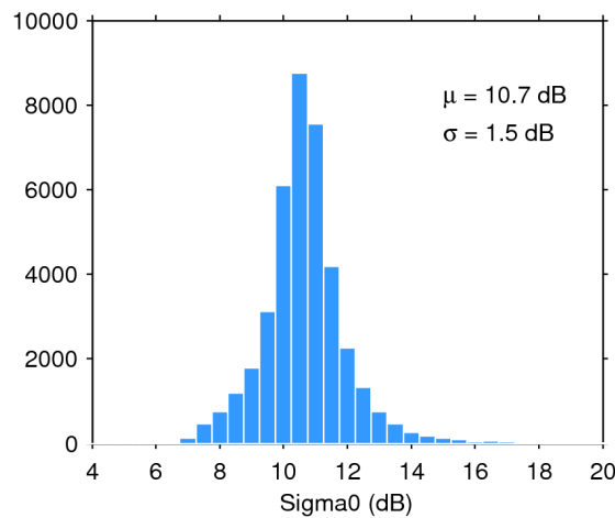
Figure 28. Histogram of science-valid sigma0 over oceans and lakes for 08/08/2020. The mean ( \mu ) and standard deviation ( \sigma ) are also shown. Note that values outside [4 20] dB are excluded from the histogram for the sake of readability but not from the computation of \mu and \sigma .
