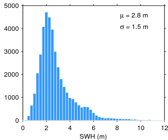
Figure 17. Histogram of flag-valid SWH over oceans and lakes for 08/08/2020. The mean ( \mu ) and standard deviation ( \sigma ) are also shown. Note that values larger than 12 m are excluded from the histogram for the sake of readability but not from the computation of \mu and \sigma .
