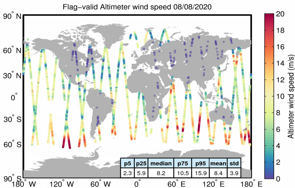
Figure 31. Geographical distribution of flag-valid wind data over oceans and lakes for 08/08/2020. The statistical values shown in the table refer to the wind in m/s and are calculated over all measurements shown in the figure.
