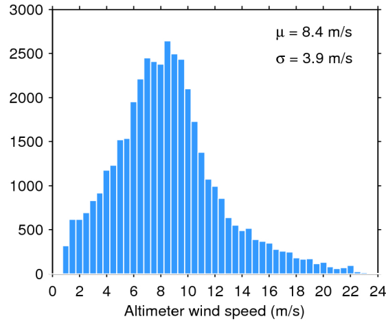
Figure 33. Histogram of flag-valid wind over oceans and lakes for 08/08/2020. The mean ( \mu ) and standard deviation ( \sigma ) are also shown. Note that values larger than 24 m/s are excluded from the histogram for the sake of readability but not from the computation of \mu and \sigma .
