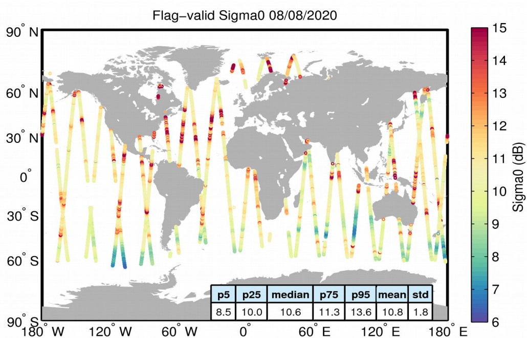
Figure 23. Geographical distribution of flag-valid sigma0 data over oceans and lakes for 08/08/2020. The statistical values shown in the table refer to the sigma0 in dB and are calculated over all measurements shown in the figure.
