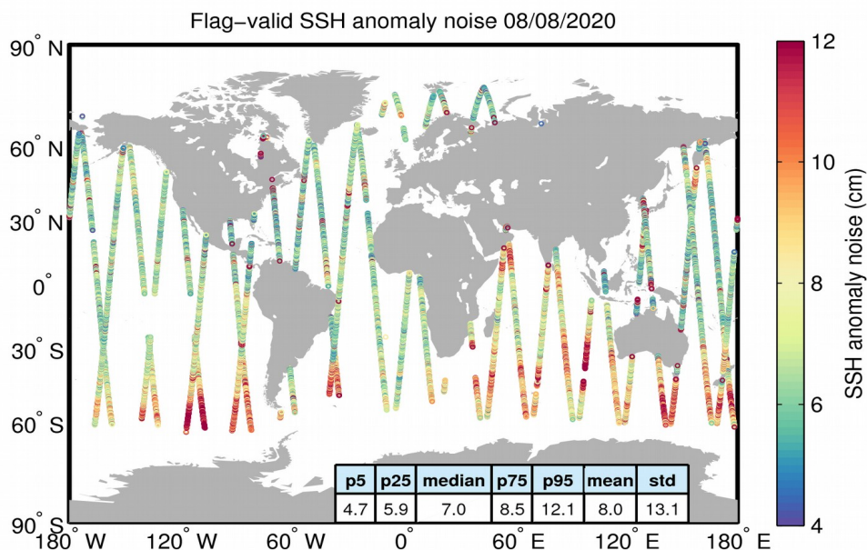
Figure 8. Geographical distribution of flag-valid 20-Hz SSH anomaly measurement noise over oceans and lakes for 08/08/2020. The statistical values shown in the table refer to the SSH anomaly noise and are calculated over all measurements shown in the figure.
