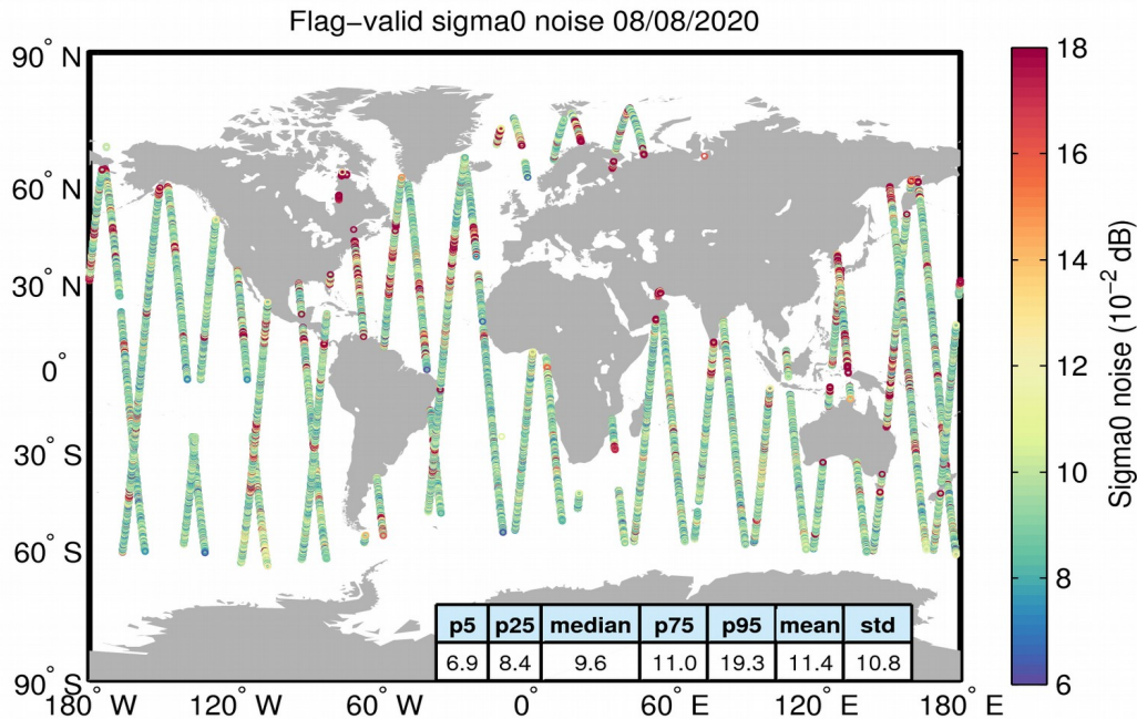
Figure 26. Geographical distribution of flag-valid 20-Hz sigma0 measurement noise over oceans and lakes for 08/08/2020. The statistical values shown in the table refer to the sigma0 noise and are calculated over all measurements shown in the figure.
