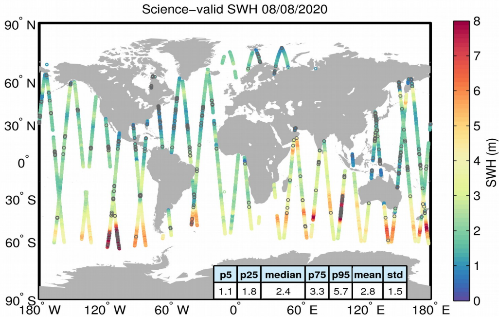
Figure 19. Geographical distribution of science-valid SWH data over oceans and lakes for 08/08/2020. The statistical values shown in the table refer to the SWH in m and are calculated over all measurements shown in the figure. Gray circles denote records that have been rejected based on the editing criteria described in Table 3.
