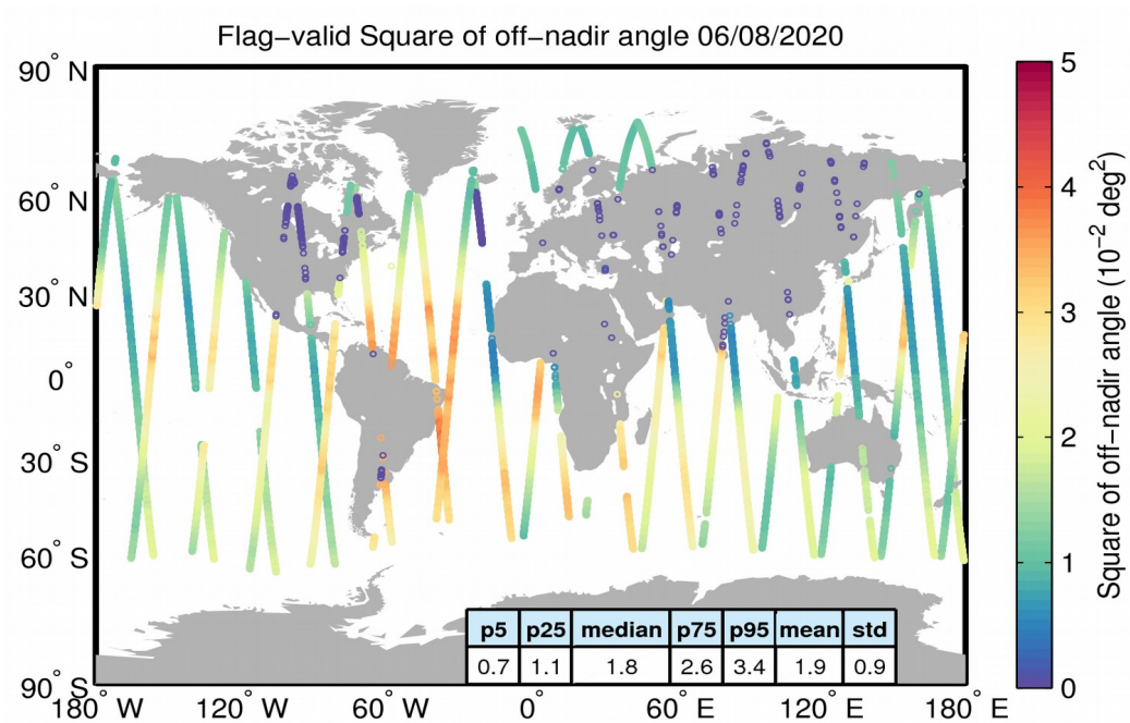
Figure 37. Geographical distribution of flag-valid mispointing data over oceans and lakes for 06/08/2020. The statistical values shown in the table refer to the mispointing in 10^{-2} deg 2 and are calculated over all measurements shown in the figure.
