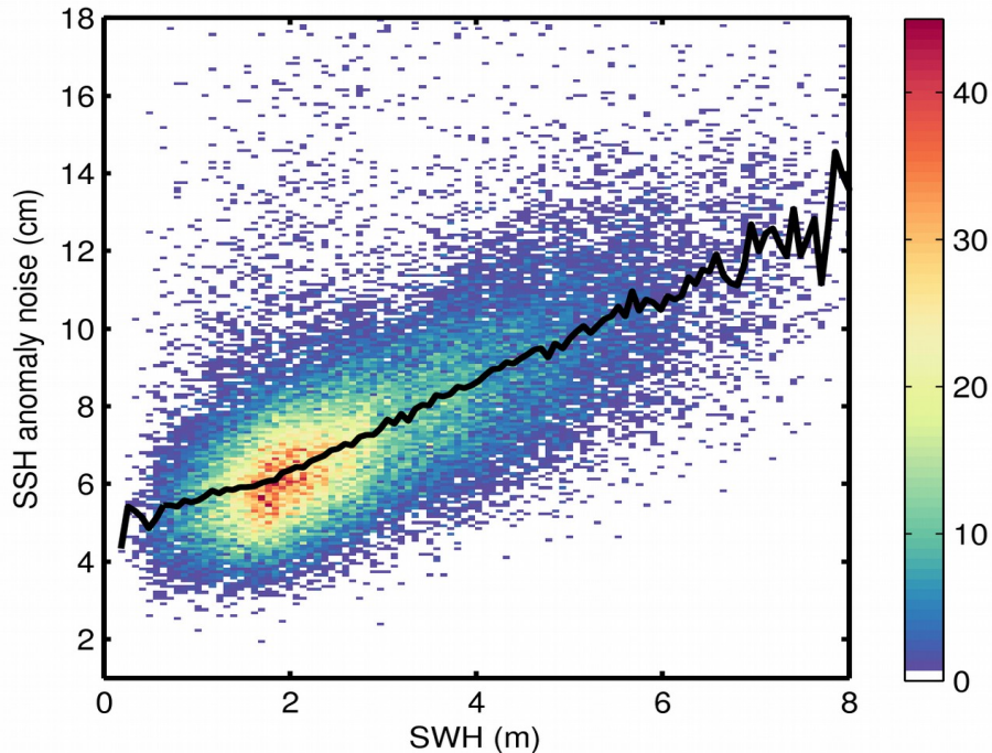
Figure 9. 2D histogram showing flag-valid SSH anomaly noise as a function of SWH for 06/08/2020. The black line denotes the median SSH anomaly noise as a function of SWH.
