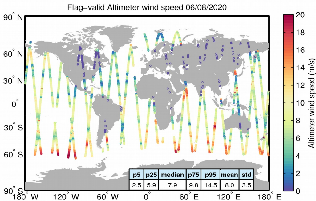
Figure 31. Geographical distribution of flag-valid wind data over oceans and lakes for 06/08/2020. The statistical values shown in the table refer to the wind in m/s and are calculated over all measurements shown in the figure.
