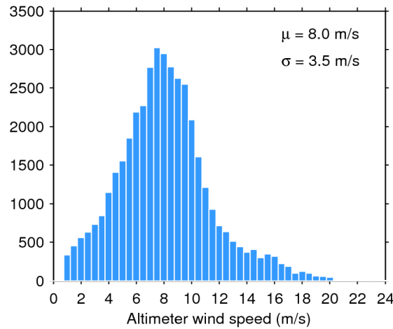
Figure 33. Histogram of flag-valid wind over oceans and lakes for 06/08/2020. The mean ( \mu ) and standard deviation ( \sigma ) are also shown. Note that values larger than 24 m/s are excluded from the histogram for the sake of readability but not from the computation of \mu and \sigma .
