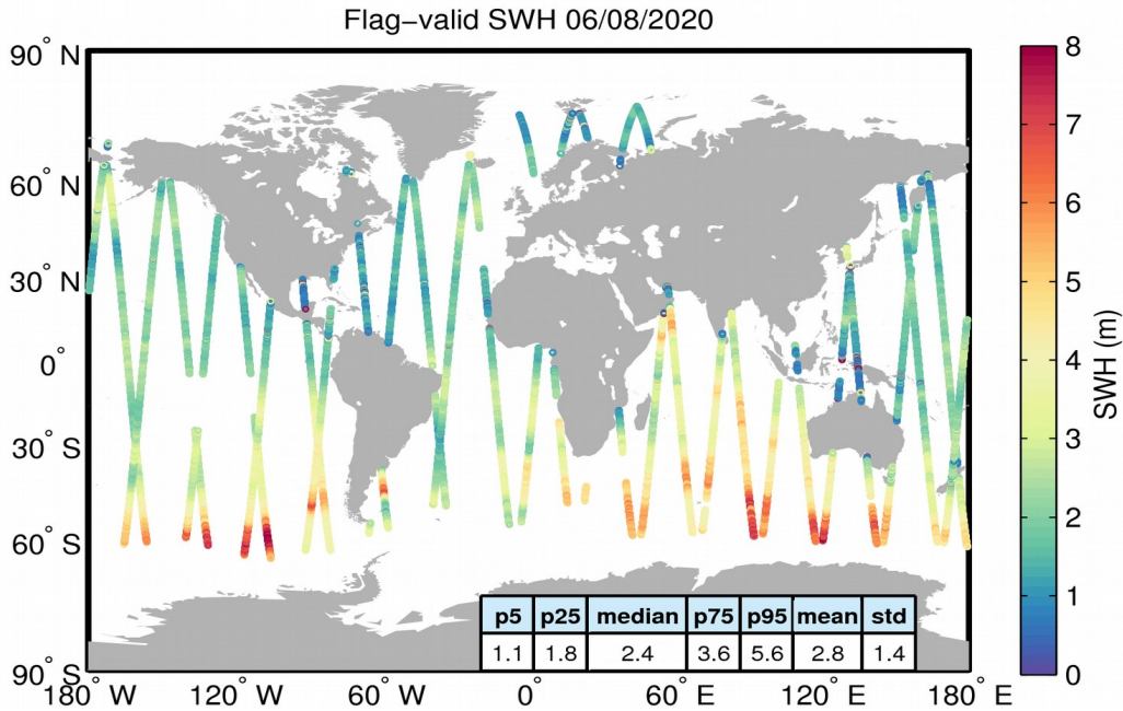
Figure 15. Geographical distribution of flag-valid SWH data over oceans and lakes for 06/08/2020. The statistical values shown in the table refer to the SWH in m and are calculated over all measurements shown in the figure.
