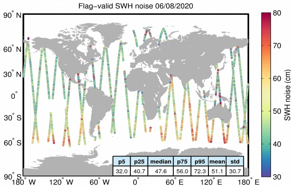
Figure 18. Geographical distribution of flag-valid 20-Hz SWH measurement noise over oceans and lakes for 06/08/2020. The statistical values shown in the figure refer to the SWH noise and are calculated over all measurements shown in the figure.
