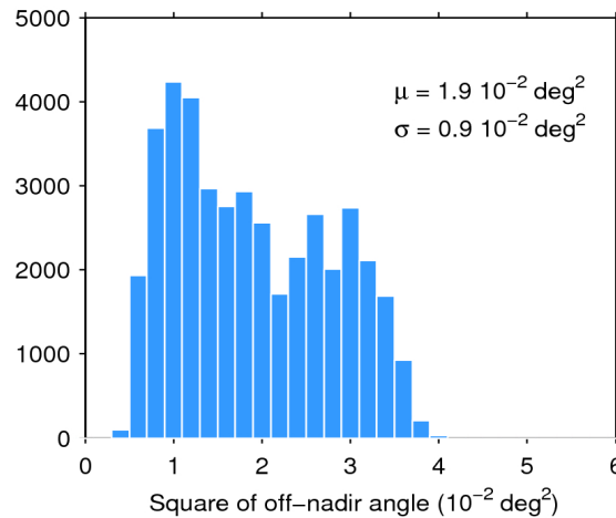
Figure 39. Histogram of flag-valid mispointing over oceans and lakes for 06/08/2020. The mean ( \mu ) and standard deviation ( \sigma ) are also shown. Note that values larger than 6 \cdot 10^{-2} \text{ deg}^2 are excluded from the histogram for the sake of readability but not from the computation of \mu and \sigma .
