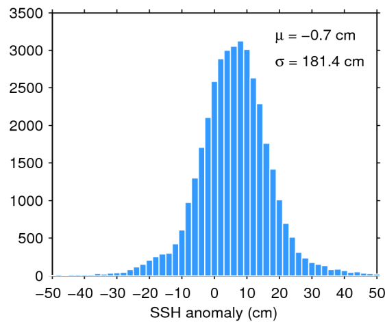
Figure 7. Histogram of flag-valid SSH anomaly over oceans and lakes for 06/08/2020. The mean ( \mu ) and standard deviation ( \sigma ) are also shown. Note that values outside [-50\ 50] cm are excluded from the histogram for the sake of readability but not from the computation of \mu and \sigma .
