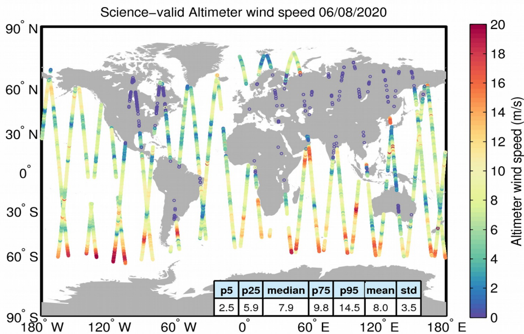
Figure 34. Geographical distribution of science-valid wind data over oceans and lakes for 06/08/2020. The statistical values shown in the table refer to the wind in m/s and are calculated over all measurements shown in the figure. Gray circles denote records that have been rejected based on the editing criteria described in Table 5.
