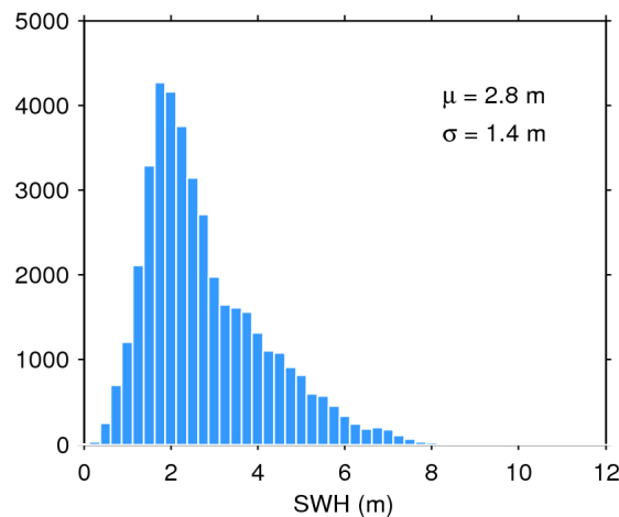
Figure 20. Histogram of science-valid SWH over oceans and lakes for 06/08/2020. The mean ( \mu ) and standard deviation ( \sigma ) are also shown. Note that values larger than 12 m are excluded from the histogram for the sake of readability but not from the computation of \mu and \sigma .
