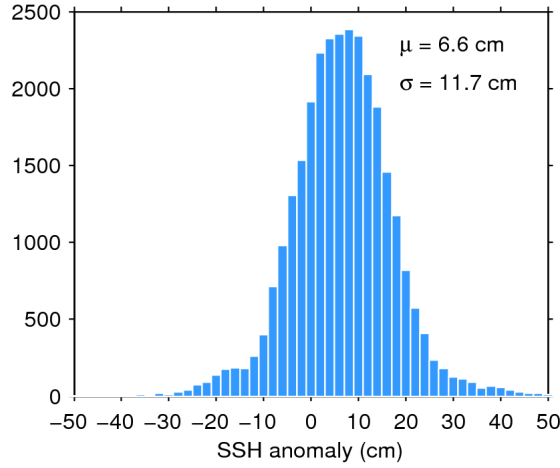
Figure 11. Histogram of science-valid SSH anomaly over oceans and lakes for 06/08/2020. The mean ( \mu ) and standard deviation ( \sigma ) are also shown. Note that values outside [-50 50] cm are excluded from the histogram for the sake of readability but not from the computation of \mu and \sigma .
