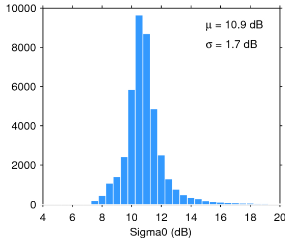
Figure 25. Histogram of flag-valid sigma0 over oceans and lakes for 06/08/2020. The mean ( \mu ) and standard deviation ( \sigma ) are also shown. Note that values outside [4 20] dB are excluded from the histogram for the sake of readability but not from the computation of \mu and \sigma .
