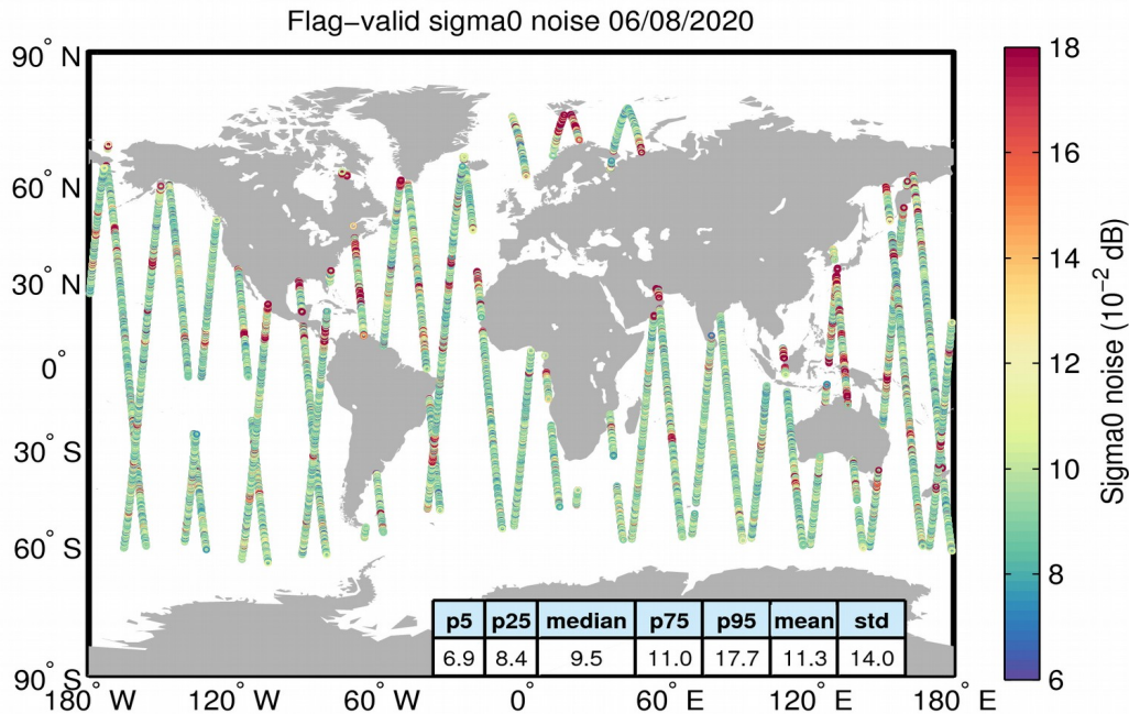
Figure 26. Geographical distribution of flag-valid 20-Hz sigma0 measurement noise over oceans and lakes for 06/08/2020. The statistical values shown in the table refer to the sigma0 noise and are calculated over all measurements shown in the figure.
