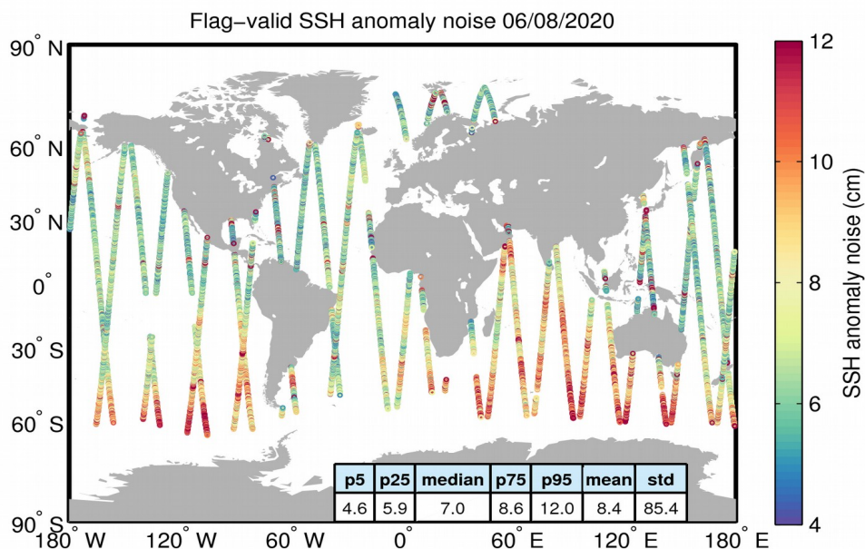
Figure 8. Geographical distribution of flag-valid 20-Hz SSH anomaly measurement noise over oceans and lakes for 06/08/2020. The statistical values shown in the table refer to the SSH anomaly noise and are calculated over all measurements shown in the figure.
