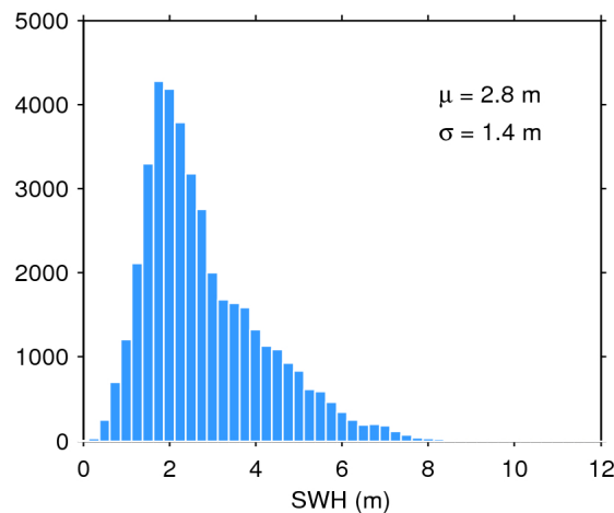
Figure 17. Histogram of flag-valid SWH over oceans and lakes for 06/08/2020. The mean ( \mu ) and standard deviation ( \sigma ) are also shown. Note that values larger than 12 m are excluded from the histogram for the sake of readability but not from the computation of \mu and \sigma .
