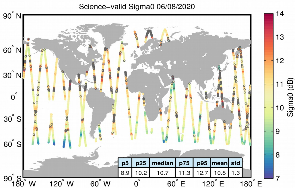
Figure 27. Geographical distribution of science-valid sigma0 data over oceans and lakes for 06/08/2020. The statistical values shown in the table refer to the sigma0 in dB and are calculated over all measurements shown in the figure. Gray circles denote records that have been rejected based on the editing criteria described in Table 4.
