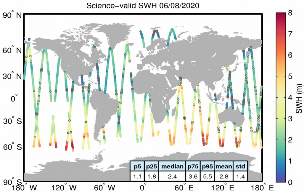
Figure 19. Geographical distribution of science-valid SWH data over oceans and lakes for 06/08/2020. The statistical values shown in the table refer to the SWH in m and are calculated over all measurements shown in the figure. Gray circles denote records that have been rejected based on the editing criteria described in Table 3.
