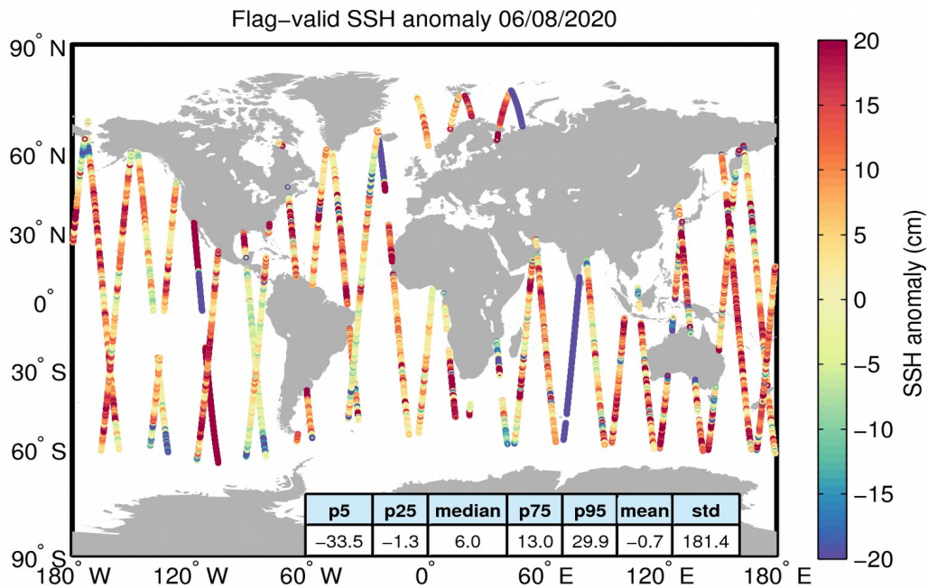
Figure 5. Geographical distribution of flag-valid 1-Hz SSH anomaly data over oceans and lakes for 06/08/2020. The statistical values shown in the table refer to the SSH anomaly in cm and are calculated over all measurements shown in the figure.
