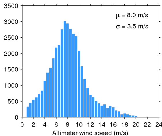
Figure 35. Histogram of science-valid wind over oceans and lakes for 06/08/2020. The mean ( \mu ) and standard deviation ( \sigma ) are also shown. Note that values larger than 24 m/s are excluded from the histogram for the sake of readability but not from the computation of \mu and \sigma .
