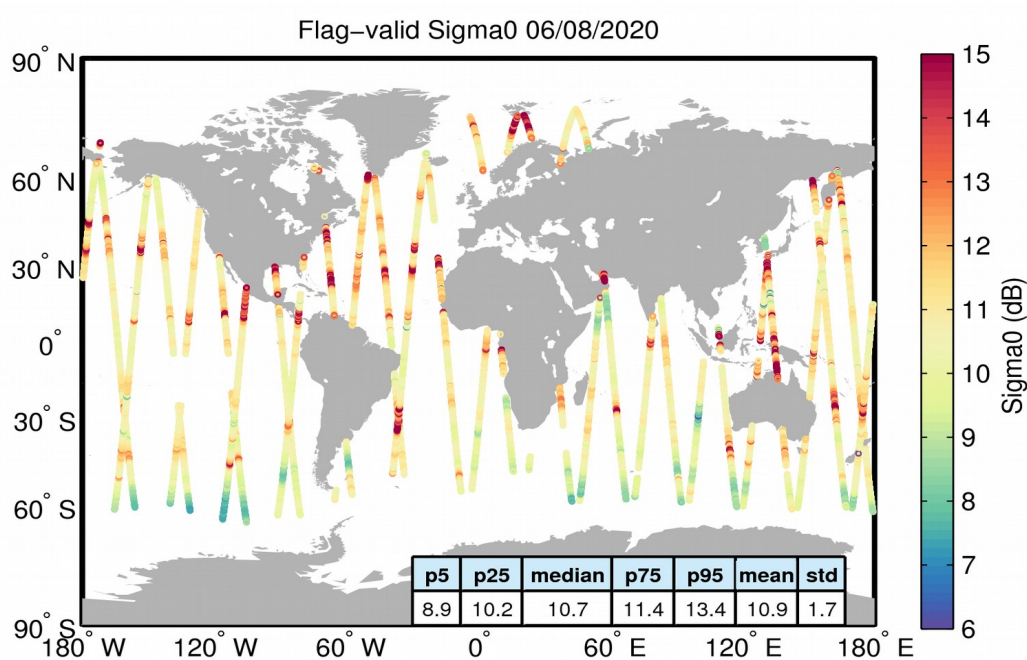
Figure 23. Geographical distribution of flag-valid sigma0 data over oceans and lakes for 06/08/2020. The statistical values shown in the table refer to the sigma0 in dB and are calculated over all measurements shown in the figure.
