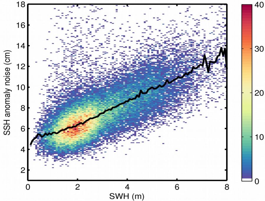
Figure 9. 2D histogram showing flag-valid SSH anomaly noise as a function of SWH for 05/08/2020. The black line denotes the median SSH anomaly noise as a function of SWH.
