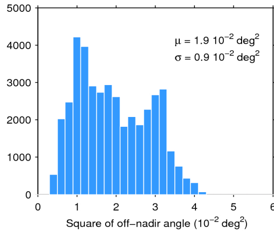
Figure 39. Histogram of flag-valid mispointing over oceans and lakes for 05/08/2020. The mean ( \mu ) and standard deviation ( \sigma ) are also shown. Note that values larger than 6 \cdot 10^{-2} \text{ deg}^2 are excluded from the histogram for the sake of readability but not from the computation of \mu and \sigma .
