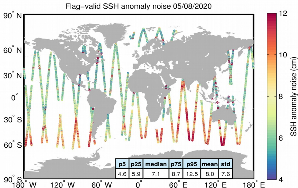
Figure 8. Geographical distribution of flag-valid 20-Hz SSH anomaly measurement noise over oceans and lakes for 05/08/2020. The statistical values shown in the table refer to the SSH anomaly noise and are calculated over all measurements shown in the figure.
