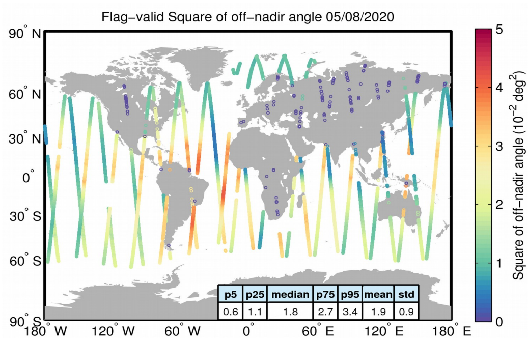
Figure 37. Geographical distribution of flag-valid mispointing data over oceans and lakes for 05/08/2020. The statistical values shown in the table refer to the mispointing in 10^{-2} \text{ deg}^2 and are calculated over all measurements shown in the figure.
