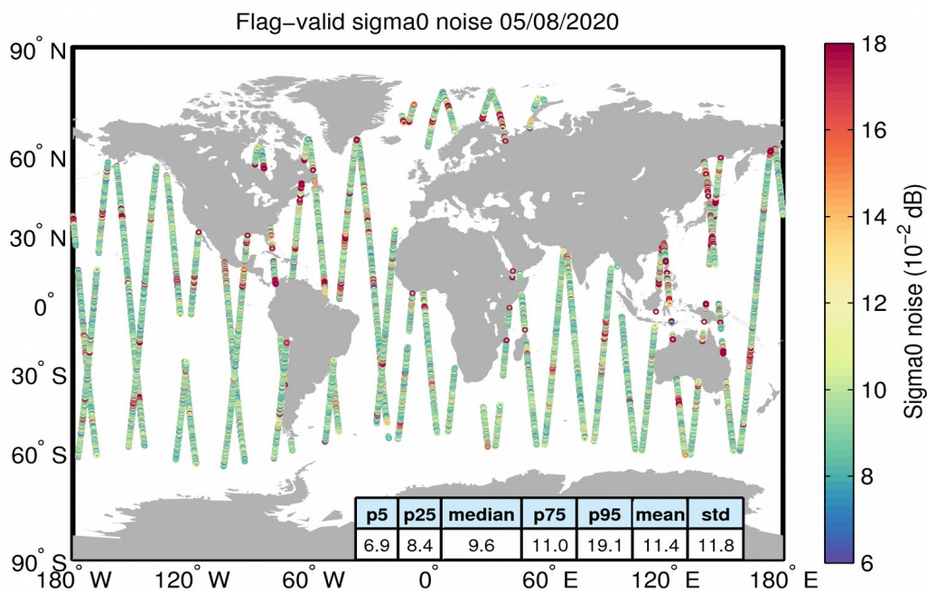
Figure 26. Geographical distribution of flag-valid 20-Hz sigma0 measurement noise over oceans and lakes for 05/08/2020. The statistical values shown in the table refer to the sigma0 noise and are calculated over all measurements shown in the figure.
