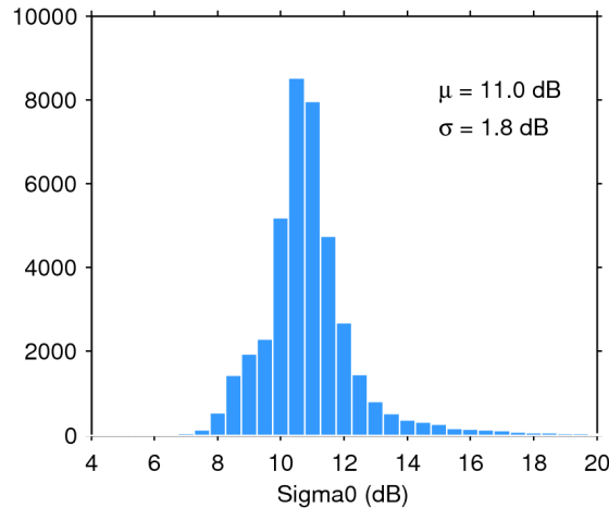
Figure 25. Histogram of flag-valid sigma0 over oceans and lakes for 05/08/2020. The mean ( \mu ) and standard deviation ( \sigma ) are also shown. Note that values outside [4 20] dB are excluded from the histogram for the sake of readability but not from the computation of \mu and \sigma .
