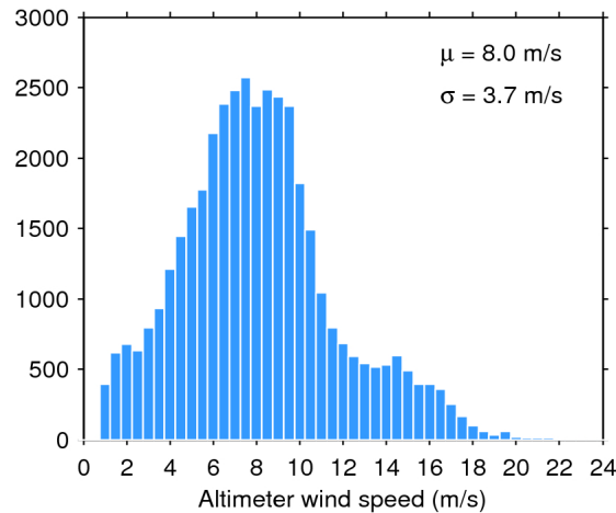
Figure 33. Histogram of flag-valid wind over oceans and lakes for 05/08/2020. The mean ( \mu ) and standard deviation ( \sigma ) are also shown. Note that values larger than 24 m/s are excluded from the histogram for the sake of readability but not from the computation of \mu and \sigma .
