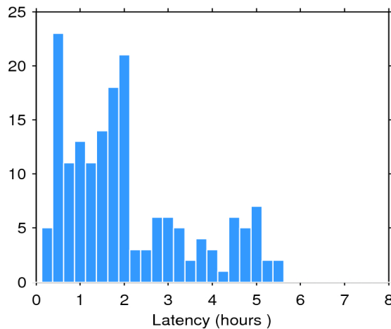
Figure 2. Histogram of the data latency for 05/08/2020. The y-axis denotes the number of files that are made available with a delay of x-hours with respect to the mean time of the records stored in the file.
