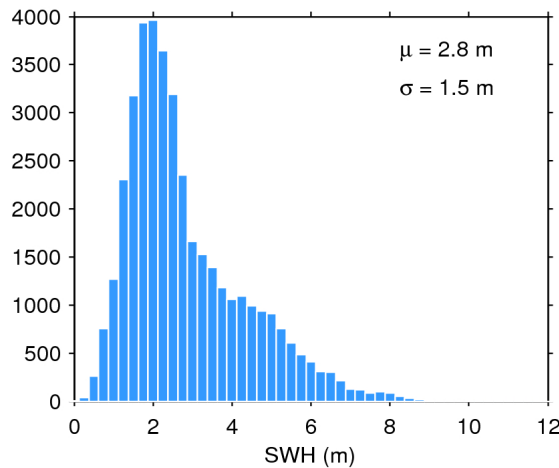
Figure 20. Histogram of science-valid SWH over oceans and lakes for 05/08/2020. The mean ( \mu ) and standard deviation ( \sigma ) are also shown. Note that values larger than 12 m are excluded from the histogram for the sake of readability but not from the computation of \mu and \sigma .
