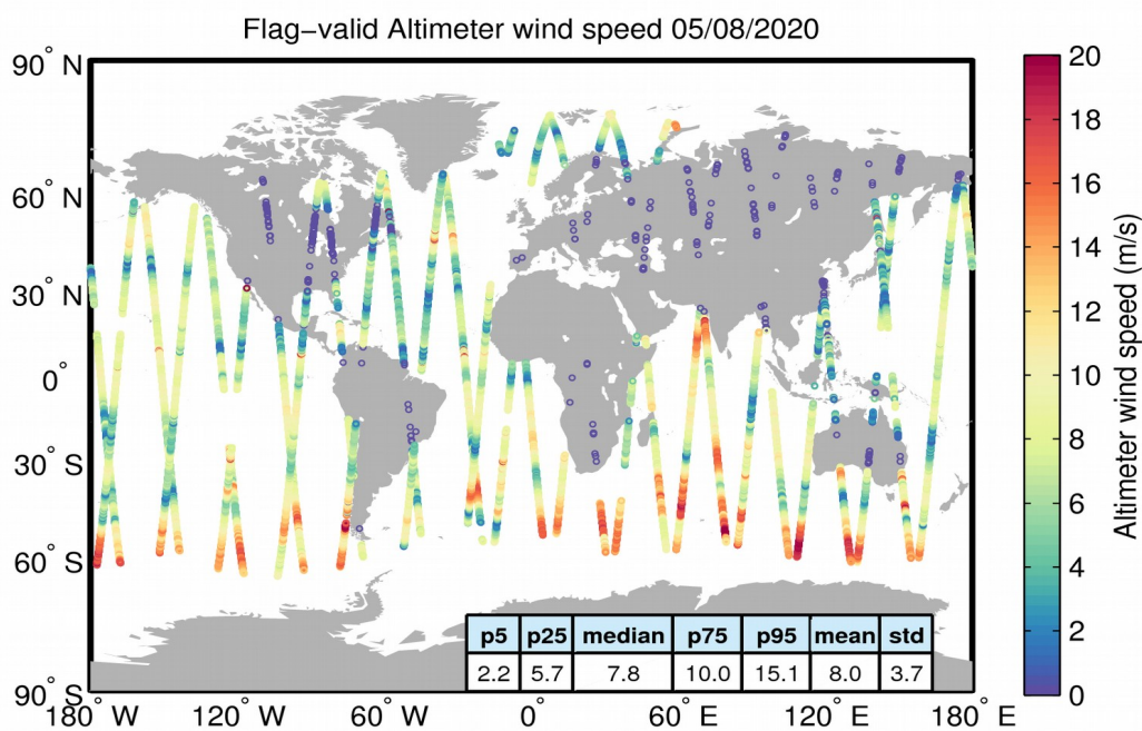
Figure 31. Geographical distribution of flag-valid wind data over oceans and lakes for 05/08/2020. The statistical values shown in the table refer to the wind in m/s and are calculated over all measurements shown in the figure.
