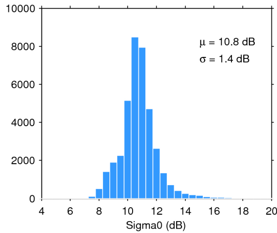
Figure 28. Histogram of science-valid sigma0 over oceans and lakes for 05/08/2020. The mean ( \mu ) and standard deviation ( \sigma ) are also shown. Note that values outside [4 20] dB are excluded from the histogram for the sake of readability but not from the computation of \mu and \sigma .
