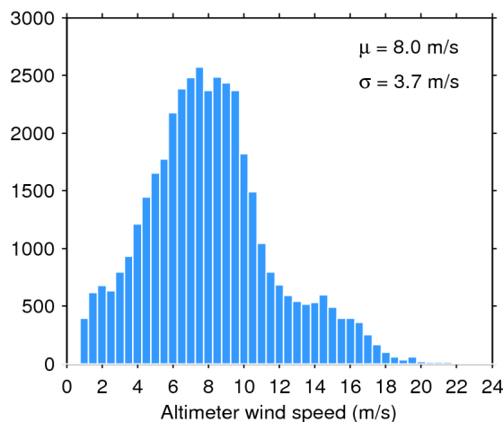
Figure 35. Histogram of science-valid wind over oceans and lakes for 05/08/2020. The mean ( \mu ) and standard deviation ( \sigma ) are also shown. Note that values larger than 24 m/s are excluded from the histogram for the sake of readability but not from the computation of \mu and \sigma .
