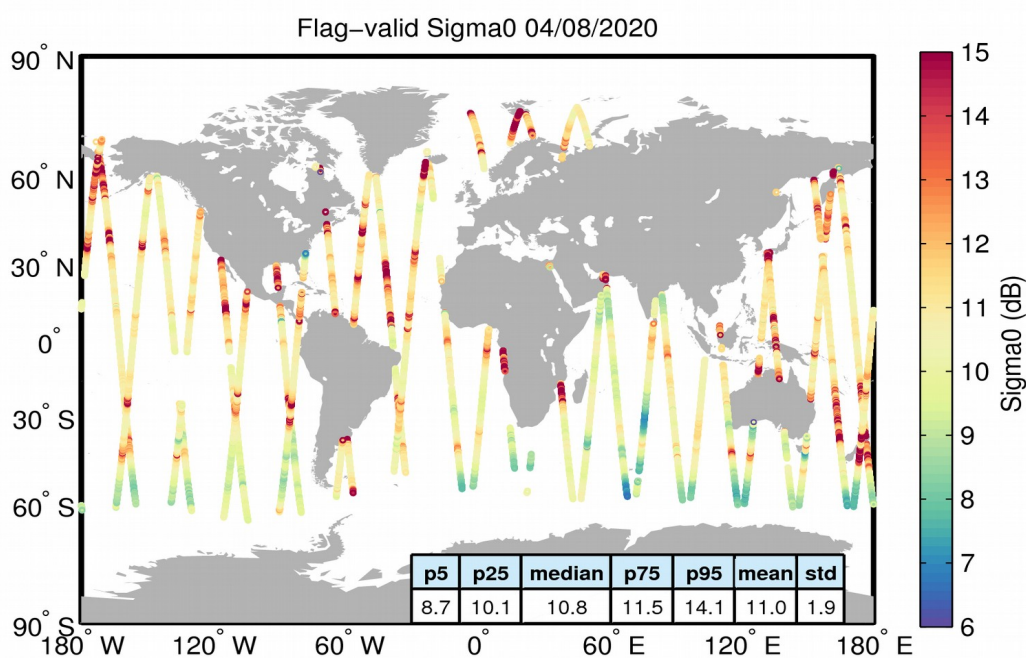
Figure 23. Geographical distribution of flag-valid sigma0 data over oceans and lakes for 04/08/2020. The statistical values shown in the table refer to the sigma0 in dB and are calculated over all measurements shown in the figure.
