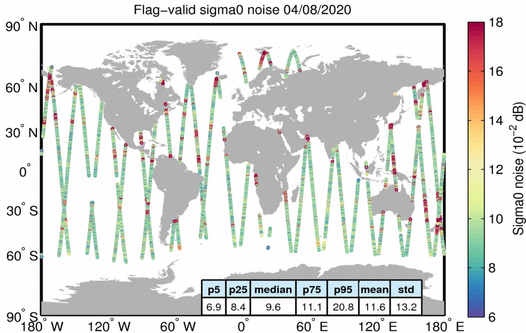
Figure 26. Geographical distribution of flag-valid 20-Hz sigma0 measurement noise over oceans and lakes for 04/08/2020. The statistical values shown in the table refer to the sigma0 noise and are calculated over all measurements shown in the figure.
