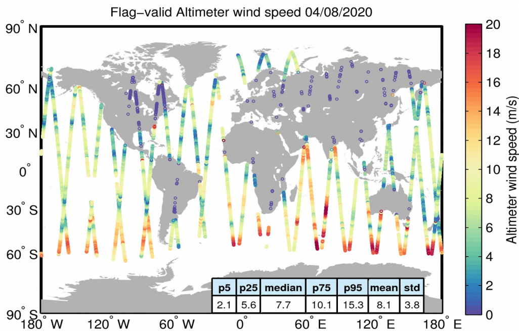
Figure 31. Geographical distribution of flag-valid wind data over oceans and lakes for 04/08/2020. The statistical values shown in the table refer to the wind in m/s and are calculated over all measurements shown in the figure.
