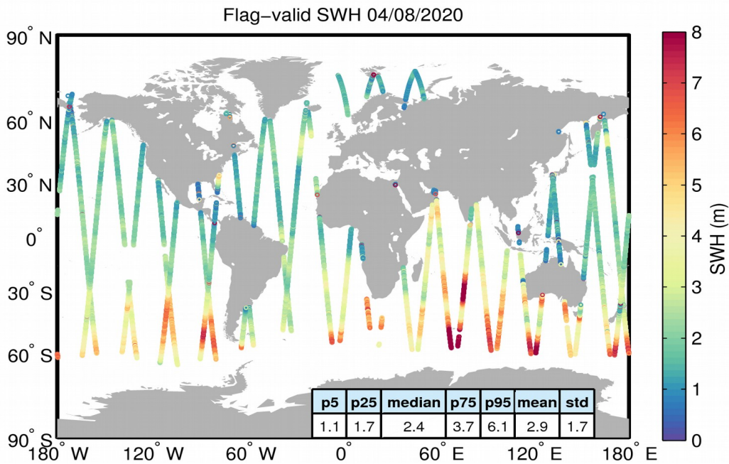
Figure 15. Geographical distribution of flag-valid SWH data over oceans and lakes for 04/08/2020. The statistical values shown in the table refer to the SWH in m and are calculated over all measurements shown in the figure.
