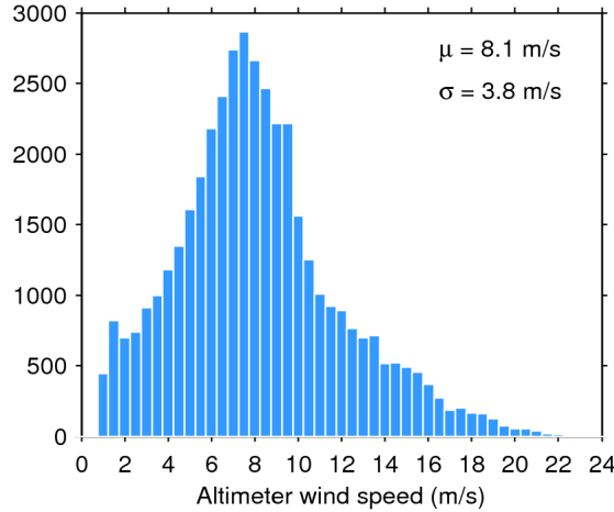
Figure 33. Histogram of flag-valid wind over oceans and lakes for 04/08/2020. The mean ( \mu ) and standard deviation ( \sigma ) are also shown. Note that values larger than 24 m/s are excluded from the histogram for the sake of readability but not from the computation of \mu and \sigma .
