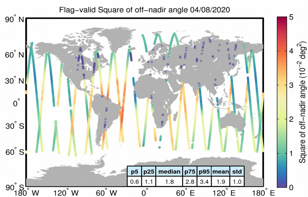
Figure 37. Geographical distribution of flag-valid mispointing data over oceans and lakes for 04/08/2020. The statistical values shown in the table refer to the mispointing in 10^{-2} deg 2 and are calculated over all measurements shown in the figure.
