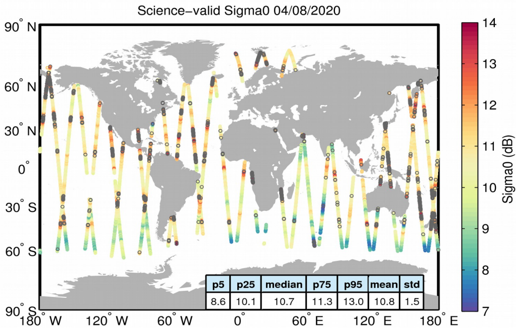
Figure 27. Geographical distribution of science-valid sigma0 data over oceans and lakes for 04/08/2020. The statistical values shown in the table refer to the sigma0 in dB and are calculated over all measurements shown in the figure. Gray circles denote records that have been rejected based on the editing criteria described in Table 4.
