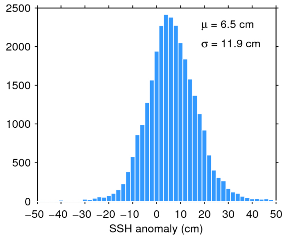
Figure 11. Histogram of science-valid SSH anomaly over oceans and lakes for 04/08/2020. The mean ( \mu ) and standard deviation ( \sigma ) are also shown. Note that values outside [-50 50] cm are excluded from the histogram for the sake of readability but not from the computation of \mu and \sigma .
