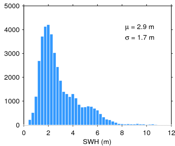
Figure 17. Histogram of flag-valid SWH over oceans and lakes for 04/08/2020. The mean ( \mu ) and standard deviation ( \sigma ) are also shown. Note that values larger than 12 m are excluded from the histogram for the sake of readability but not from the computation of \mu and \sigma .
