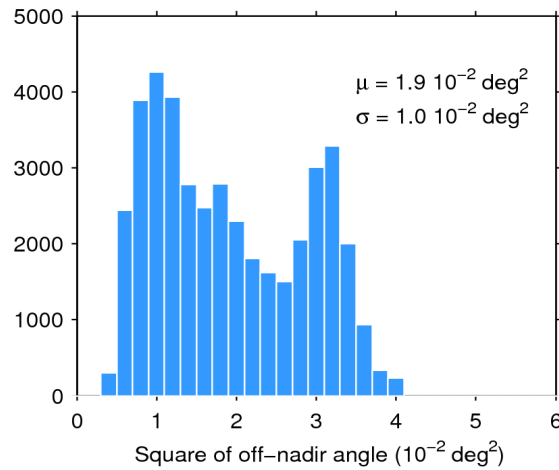
Figure 39. Histogram of flag-valid mispointing over oceans and lakes for 04/08/2020. The mean ( \mu ) and standard deviation ( \sigma ) are also shown. Note that values larger than 6 \cdot 10^{-2} \text{ deg}^2 are excluded from the histogram for the sake of readability but not from the computation of \mu and \sigma .
