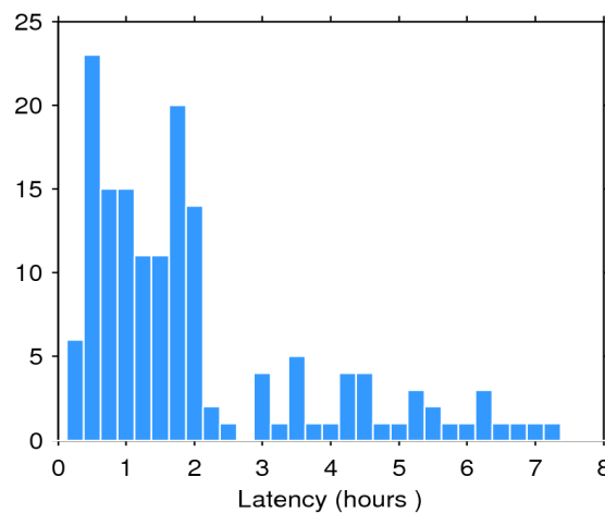
Figure 2. Histogram of the data latency for 04/08/2020. The y-axis denotes the number of files that are made available with a delay of x-hours with respect to the mean time of the records stored in the file.
