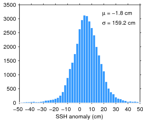
Figure 7. Histogram of flag-valid SSH anomaly over oceans and lakes for 04/08/2020. The mean ( \mu ) and standard deviation ( \sigma ) are also shown. Note that values outside [-50\ 50] cm are excluded from the histogram for the sake of readability but not from the computation of \mu and \sigma .
