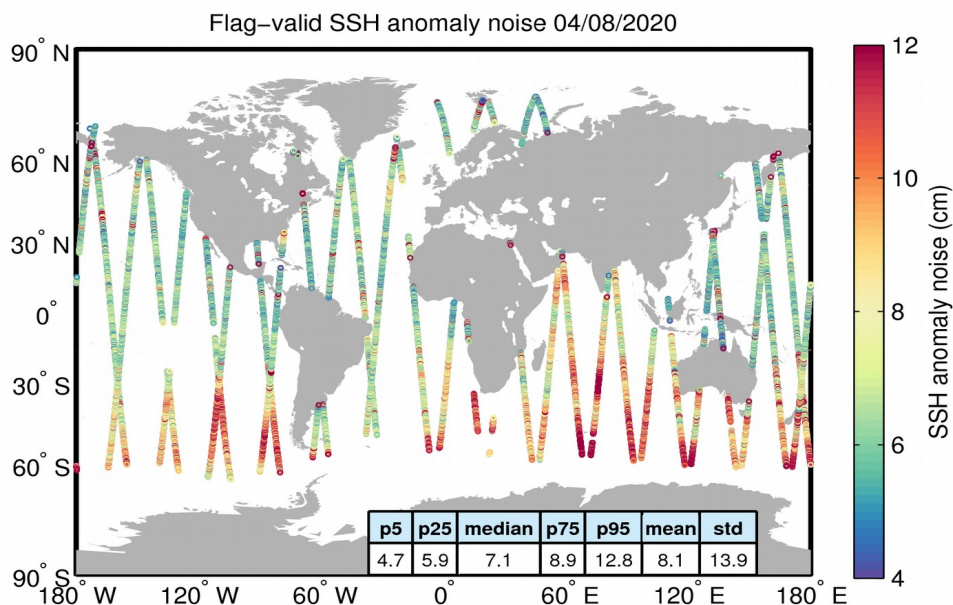
Figure 8. Geographical distribution of flag-valid 20-Hz SSH anomaly measurement noise over oceans and lakes for 04/08/2020. The statistical values shown in the table refer to the SSH anomaly noise and are calculated over all measurements shown in the figure.
