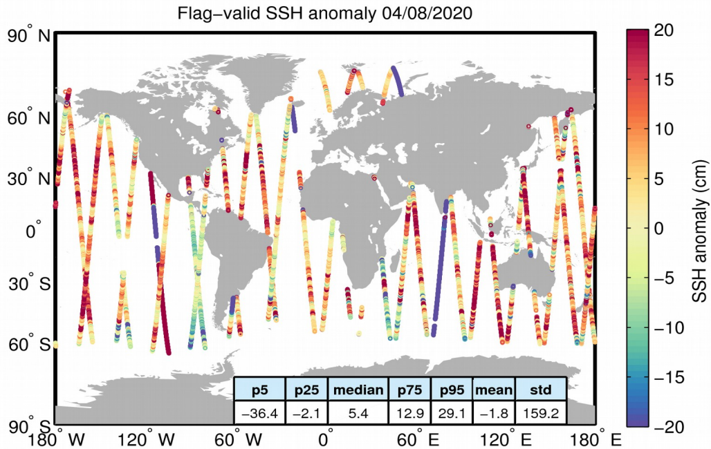
Figure 5. Geographical distribution of flag-valid 1-Hz SSH anomaly data over oceans and lakes for 04/08/2020. The statistical values shown in the table refer to the SSH anomaly in cm and are calculated over all measurements shown in the figure.
