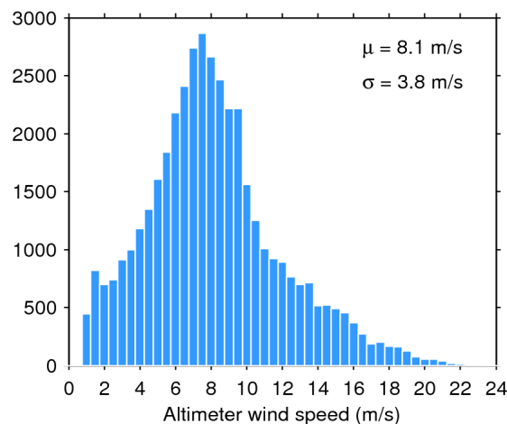
Figure 35. Histogram of science-valid wind over oceans and lakes for 04/08/2020. The mean ( \mu ) and standard deviation ( \sigma ) are also shown. Note that values larger than 24 m/s are excluded from the histogram for the sake of readability but not from the computation of \mu and \sigma .
