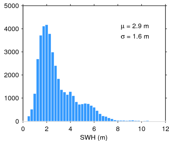
Figure 20. Histogram of science-valid SWH over oceans and lakes for 04/08/2020. The mean ( \mu ) and standard deviation ( \sigma ) are also shown. Note that values larger than 12 m are excluded from the histogram for the sake of readability but not from the computation of \mu and \sigma .
