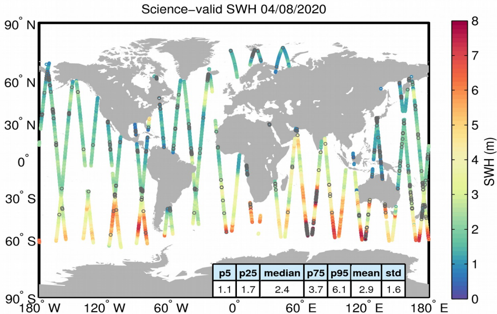
Figure 19. Geographical distribution of science-valid SWH data over oceans and lakes for 04/08/2020. The statistical values shown in the table refer to the SWH in m and are calculated over all measurements shown in the figure. Gray circles denote records that have been rejected based on the editing criteria described in Table 3.
