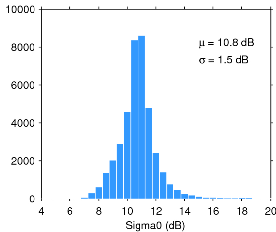
Figure 28. Histogram of science-valid sigma0 over oceans and lakes for 04/08/2020. The mean ( \mu ) and standard deviation ( \sigma ) are also shown. Note that values outside [4 20] dB are excluded from the histogram for the sake of readability but not from the computation of \mu and \sigma .
