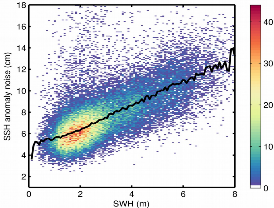
Figure 9. 2D histogram showing flag-valid SSH anomaly noise as a function of SWH for 04/08/2020. The black line denotes the median SSH anomaly noise as a function of SWH.
