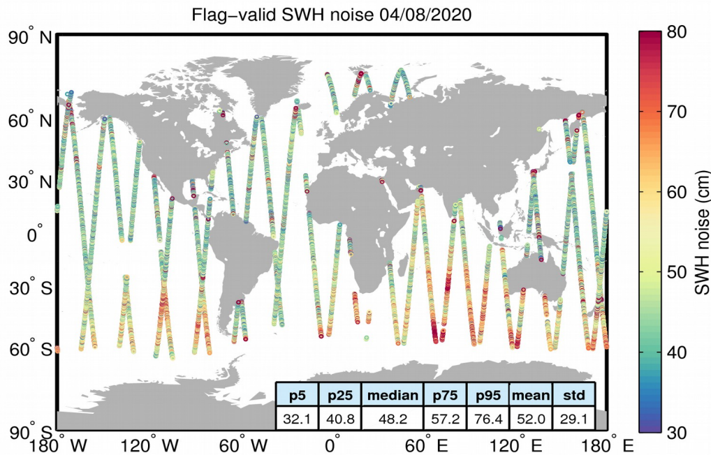
Figure 18. Geographical distribution of flag-valid 20-Hz SWH measurement noise over oceans and lakes for 04/08/2020. The statistical values shown in the figure refer to the SWH noise and are calculated over all measurements shown in the figure.
