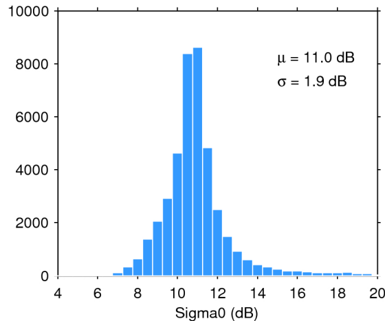
Figure 25. Histogram of flag-valid sigma0 over oceans and lakes for 04/08/2020. The mean ( \mu ) and standard deviation ( \sigma ) are also shown. Note that values outside [4 20] dB are excluded from the histogram for the sake of readability but not from the computation of \mu and \sigma .
