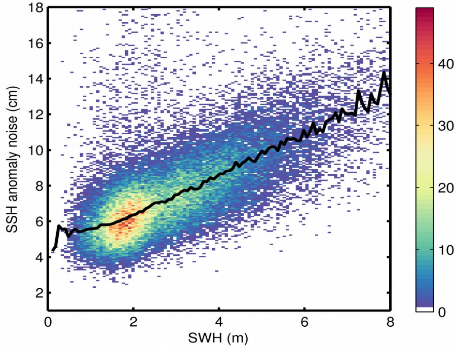
Figure 9. 2D histogram showing flag-valid SSH anomaly noise as a function of SWH for 02/08/2020. The black line denotes the median SSH anomaly noise as a function of SWH.
