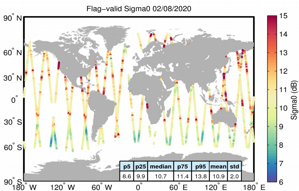
Figure 23. Geographical distribution of flag-valid sigma0 data over oceans and lakes for 02/08/2020. The statistical values shown in the table refer to the sigma0 in dB and are calculated over all measurements shown in the figure.
