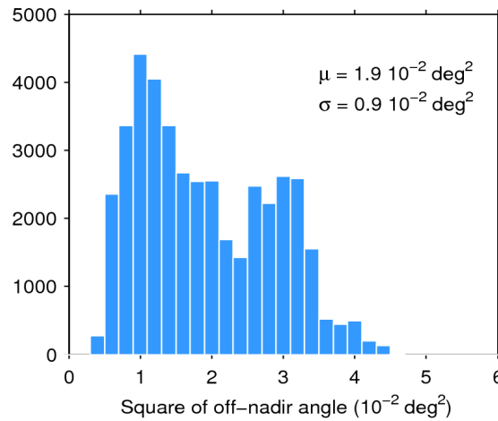
Figure 39. Histogram of flag-valid mispointing over oceans and lakes for 02/08/2020. The mean ( \mu ) and standard deviation ( \sigma ) are also shown. Note that values larger than 6 \cdot 10^{-2} \text{ deg}^2 are excluded from the histogram for the sake of readability but not from the computation of \mu and \sigma .
