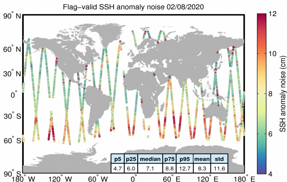
Figure 8. Geographical distribution of flag-valid 20-Hz SSH anomaly measurement noise over oceans and lakes for 02/08/2020. The statistical values shown in the table refer to the SSH anomaly noise and are calculated over all measurements shown in the figure.
