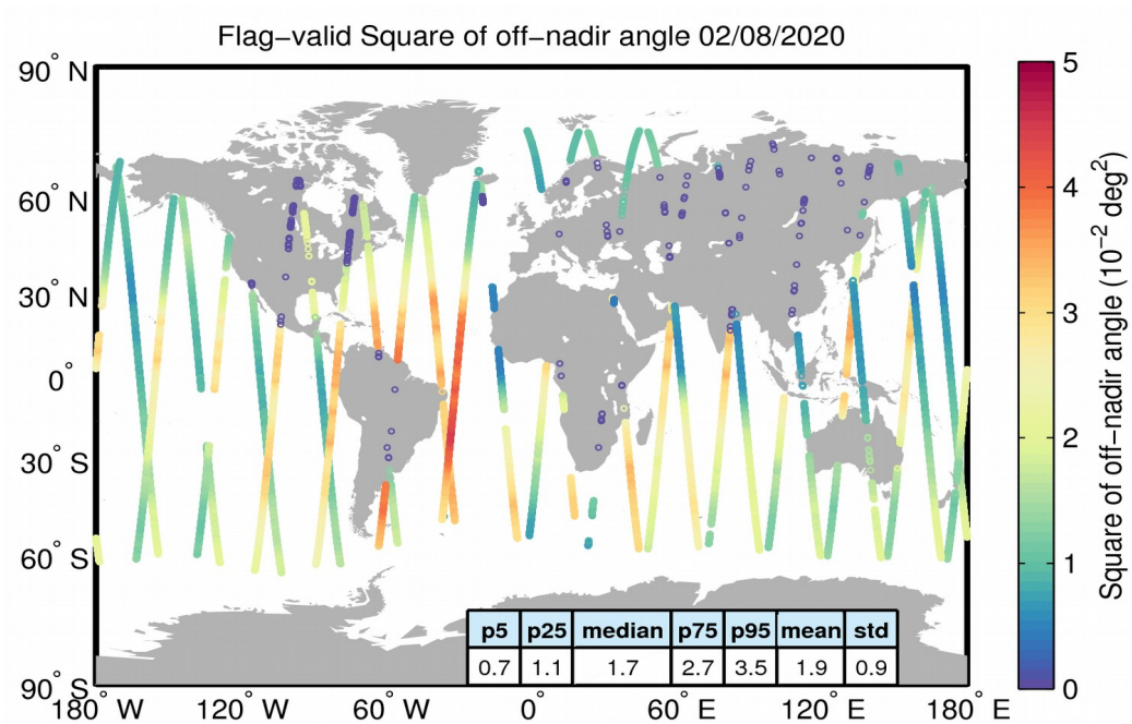
Figure 37. Geographical distribution of flag-valid mispointing data over oceans and lakes for 02/08/2020. The statistical values shown in the table refer to the mispointing in 10^{-2} \text{deg}^2 and are calculated over all measurements shown in the figure.
