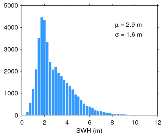
Figure 17. Histogram of flag-valid SWH over oceans and lakes for 02/08/2020. The mean ( \mu ) and standard deviation ( \sigma ) are also shown. Note that values larger than 12 m are excluded from the histogram for the sake of readability but not from the computation of \mu and \sigma .
