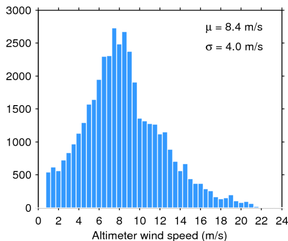
Figure 35. Histogram of science-valid wind over oceans and lakes for 02/08/2020. The mean ( \mu ) and standard deviation ( \sigma ) are also shown. Note that values larger than 24 m/s are excluded from the histogram for the sake of readability but not from the computation of \mu and \sigma .
