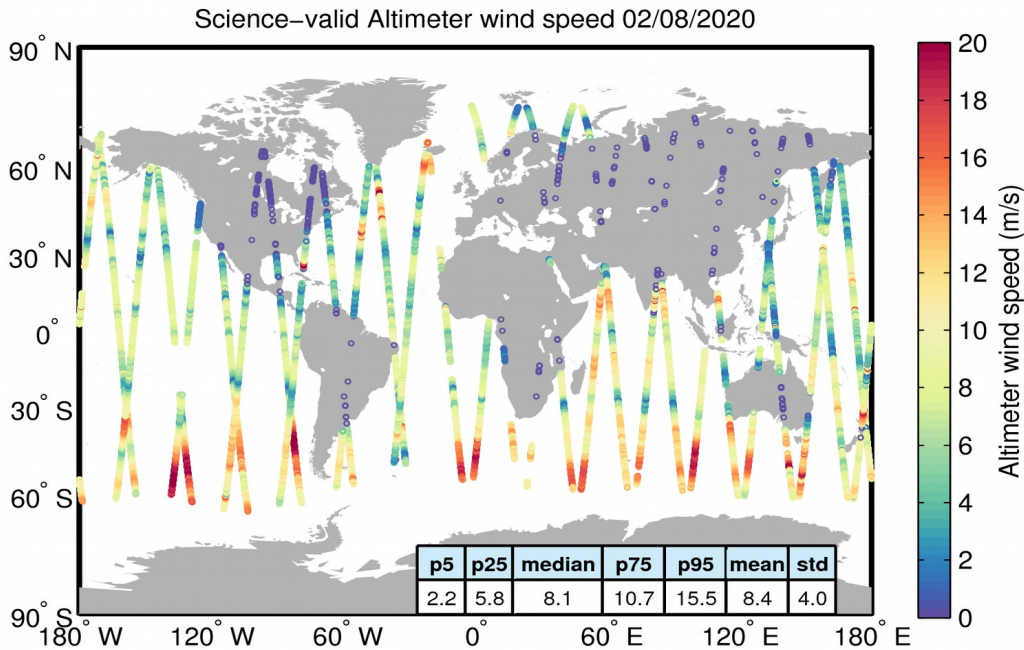
Figure 34. Geographical distribution of science-valid wind data over oceans and lakes for 02/08/2020. The statistical values shown in the table refer to the wind in m/s and are calculated over all measurements shown in the figure. Gray circles denote records that have been rejected based on the editing criteria described in Table 5.
