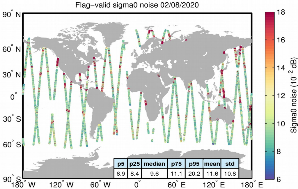
Figure 26. Geographical distribution of flag-valid 20-Hz sigma0 measurement noise over oceans and lakes for 02/08/2020. The statistical values shown in the table refer to the sigma0 noise and are calculated over all measurements shown in the figure.
