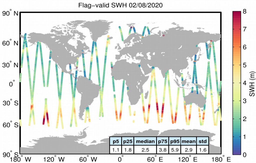
Figure 15. Geographical distribution of flag-valid SWH data over oceans and lakes for 02/08/2020. The statistical values shown in the table refer to the SWH in m and are calculated over all measurements shown in the figure.
