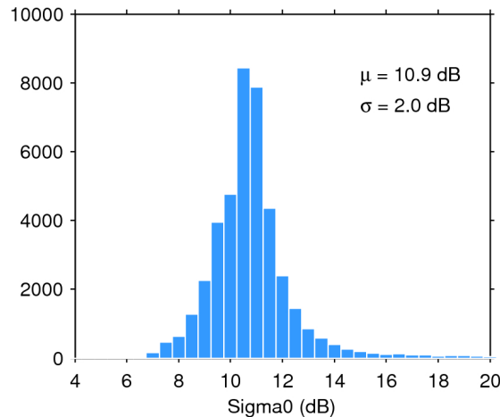
Figure 25. Histogram of flag-valid sigma0 over oceans and lakes for 02/08/2020. The mean ( \mu ) and standard deviation ( \sigma ) are also shown. Note that values outside [4 20] dB are excluded from the histogram for the sake of readability but not from the computation of \mu and \sigma .
