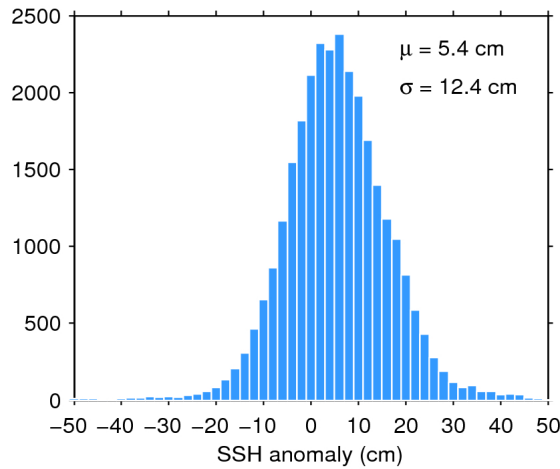
Figure 11. Histogram of science-valid SSH anomaly over oceans and lakes for 02/08/2020. The mean ( \mu ) and standard deviation ( \sigma ) are also shown. Note that values outside [-50 50] cm are excluded from the histogram for the sake of readability but not from the computation of \mu and \sigma .
