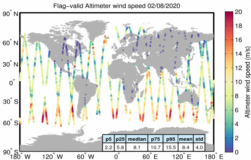
Figure 31. Geographical distribution of flag-valid wind data over oceans and lakes for 02/08/2020. The statistical values shown in the table refer to the wind in m/s and are calculated over all measurements shown in the figure.
