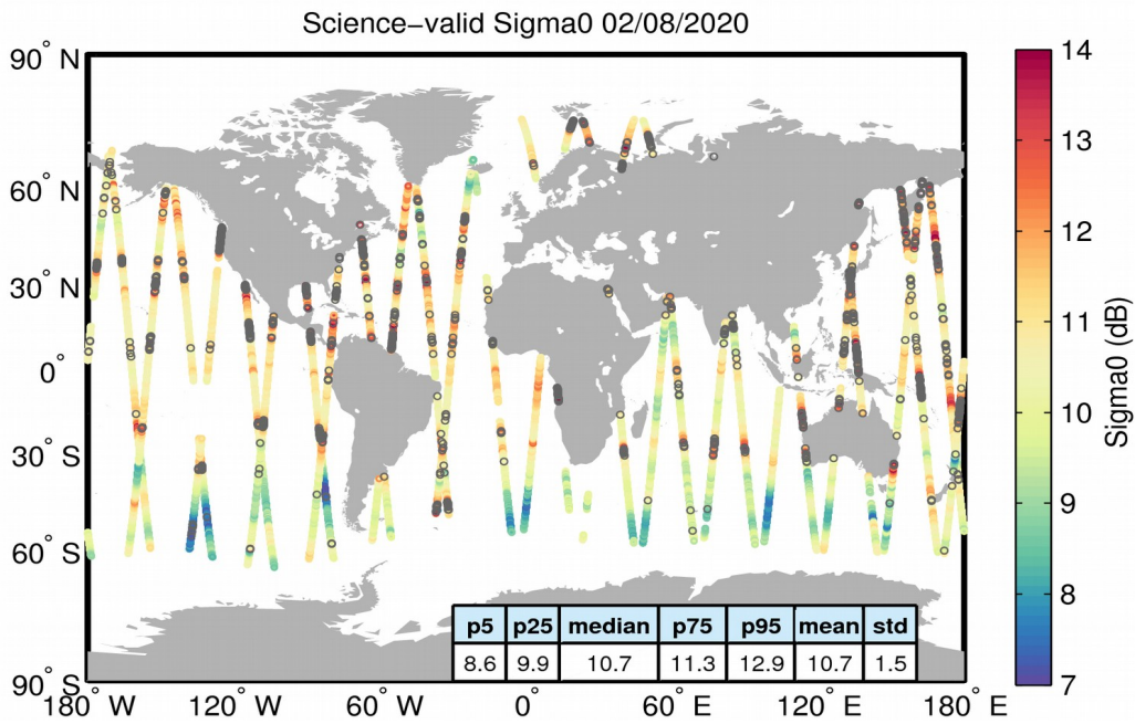
Figure 27. Geographical distribution of science-valid sigma0 data over oceans and lakes for 02/08/2020. The statistical values shown in the table refer to the sigma0 in dB and are calculated over all measurements shown in the figure. Gray circles denote records that have been rejected based on the editing criteria described in Table 4.
