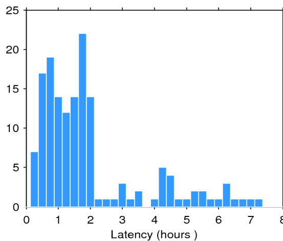
Figure 2. Histogram of the data latency for 02/08/2020. The y-axis denotes the number of files that are made available with a delay of x-hours with respect to the mean time of the records stored in the file.
