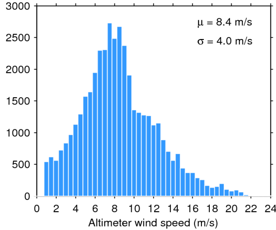
Figure 33. Histogram of flag-valid wind over oceans and lakes for 02/08/2020. The mean ( \mu ) and standard deviation ( \sigma ) are also shown. Note that values larger than 24 m/s are excluded from the histogram for the sake of readability but not from the computation of \mu and \sigma .
