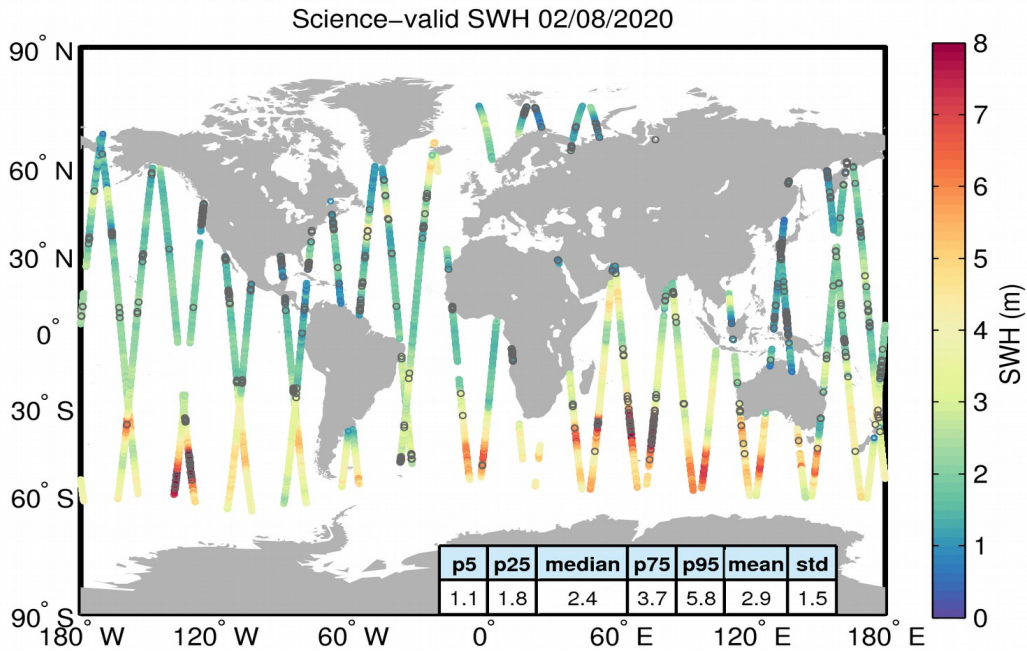
Figure 19. Geographical distribution of science-valid SWH data over oceans and lakes for 02/08/2020. The statistical values shown in the table refer to the SWH in m and are calculated over all measurements shown in the figure. Gray circles denote records that have been rejected based on the editing criteria described in Table 3.
