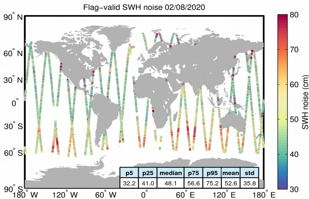
Figure 18. Geographical distribution of flag-valid 20-Hz SWH measurement noise over oceans and lakes for 02/08/2020. The statistical values shown in the figure refer to the SWH noise and are calculated over all measurements shown in the figure.
