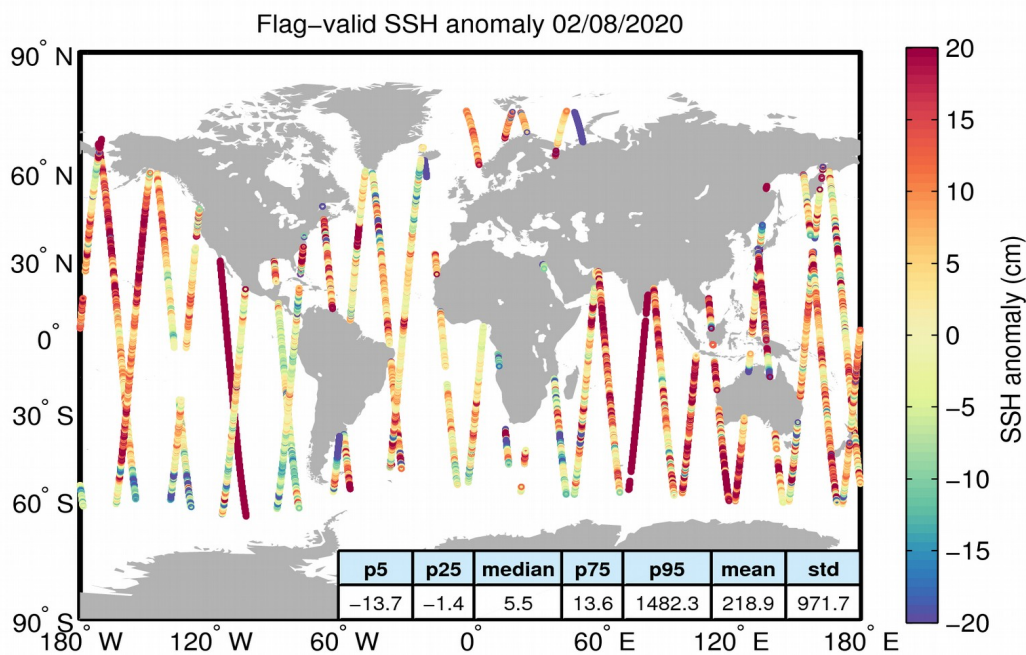
Figure 5. Geographical distribution of flag-valid 1-Hz SSH anomaly data over oceans and lakes for 02/08/2020. The statistical values shown in the table refer to the SSH anomaly in cm and are calculated over all measurements shown in the figure.
