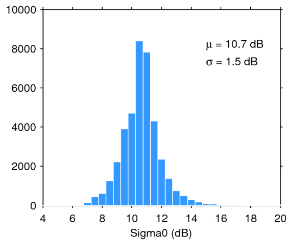
Figure 28. Histogram of science-valid sigma0 over oceans and lakes for 02/08/2020. The mean ( \mu ) and standard deviation ( \sigma ) are also shown. Note that values outside [4 20] dB are excluded from the histogram for the sake of readability but not from the computation of \mu and \sigma .
