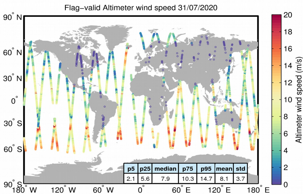
Figure 31. Geographical distribution of flag-valid wind data over oceans and lakes for 31/07/2020. The statistical values shown in the table refer to the wind in m/s and are calculated over all measurements shown in the figure.
