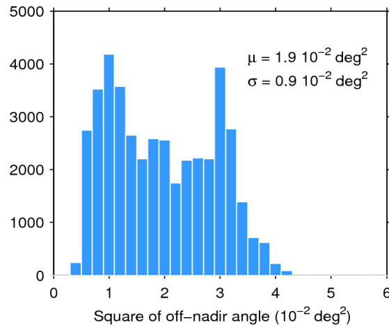
Figure 39. Histogram of flag-valid mispointing over oceans and lakes for 31/07/2020. The mean ( \mu ) and standard deviation ( \sigma ) are also shown. Note that values larger than 6 \cdot 10^{-2} \text{ deg}^2 are excluded from the histogram for the sake of readability but not from the computation of \mu and \sigma .
