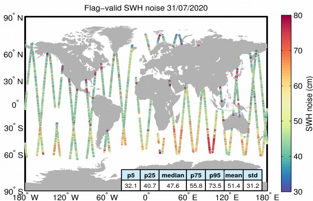
Figure 18. Geographical distribution of flag-valid 20-Hz SWH measurement noise over oceans and lakes for 31/07/2020. The statistical values shown in the figure refer to the SWH noise and are calculated over all measurements shown in the figure.
