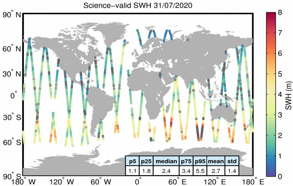
Figure 19. Geographical distribution of science-valid SWH data over oceans and lakes for 31/07/2020. The statistical values shown in the table refer to the SWH in m and are calculated over all measurements shown in the figure. Gray circles denote records that have been rejected based on the editing criteria described in Table 3.
