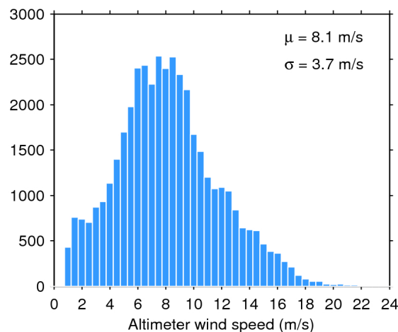
Figure 35. Histogram of science-valid wind over oceans and lakes for 31/07/2020. The mean ( \mu ) and standard deviation ( \sigma ) are also shown. Note that values larger than 24 m/s are excluded from the histogram for the sake of readability but not from the computation of \mu and \sigma .
