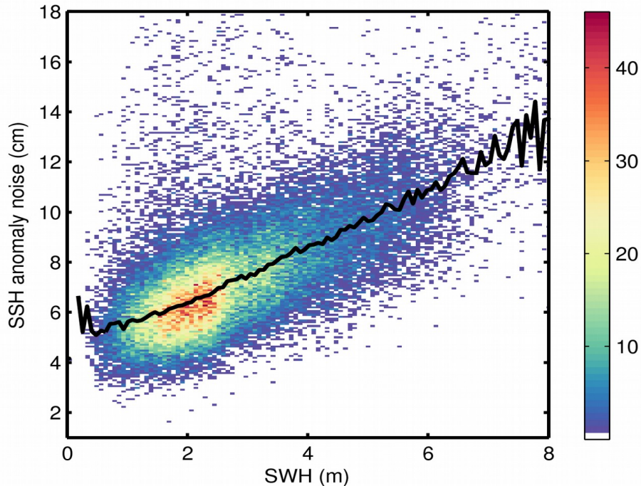
Figure 9. 2D histogram showing flag-valid SSH anomaly noise as a function of SWH for 31/07/2020. The black line denotes the median SSH anomaly noise as a function of SWH.
