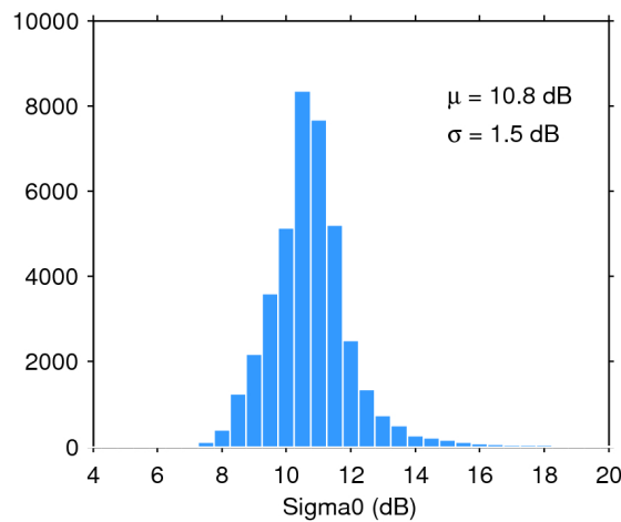
Figure 28. Histogram of science-valid sigma0 over oceans and lakes for 31/07/2020. The mean ( \mu ) and standard deviation ( \sigma ) are also shown. Note that values outside [4 20] dB are excluded from the histogram for the sake of readability but not from the computation of \mu and \sigma .
