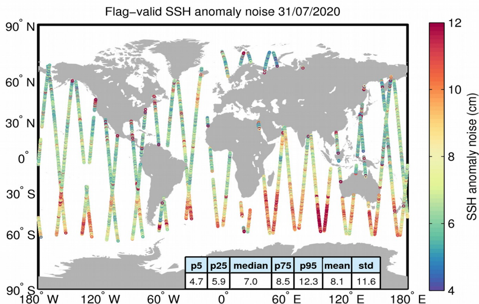
Figure 8. Geographical distribution of flag-valid 20-Hz SSH anomaly measurement noise over oceans and lakes for 31/07/2020. The statistical values shown in the table refer to the SSH anomaly noise and are calculated over all measurements shown in the figure.
