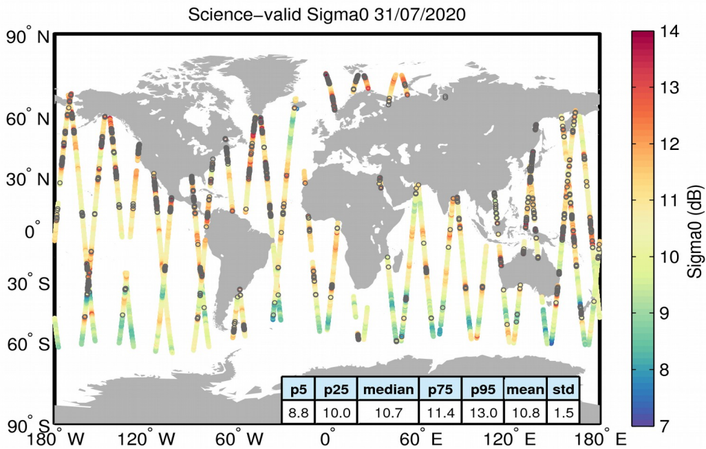
Figure 27. Geographical distribution of science-valid sigma0 data over oceans and lakes for 31/07/2020. The statistical values shown in the table refer to the sigma0 in dB and are calculated over all measurements shown in the figure. Gray circles denote records that have been rejected based on the editing criteria described in Table 4.
