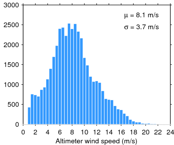
Figure 33. Histogram of flag-valid wind over oceans and lakes for 31/07/2020. The mean ( \mu ) and standard deviation ( \sigma ) are also shown. Note that values larger than 24 m/s are excluded from the histogram for the sake of readability but not from the computation of \mu and \sigma .
