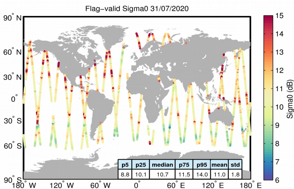
Figure 23. Geographical distribution of flag-valid sigma0 data over oceans and lakes for 31/07/2020. The statistical values shown in the table refer to the sigma0 in dB and are calculated over all measurements shown in the figure.
