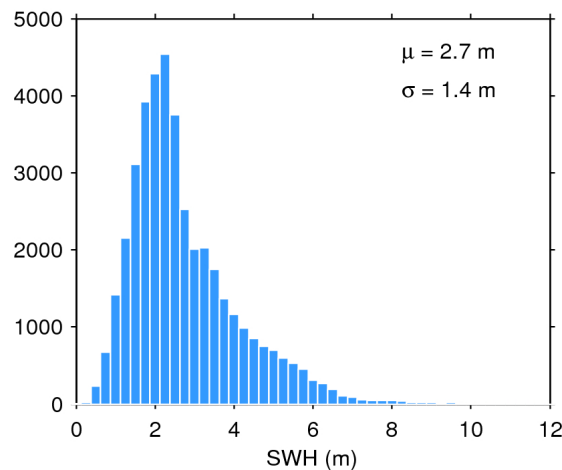
Figure 20. Histogram of science-valid SWH over oceans and lakes for 31/07/2020. The mean ( \mu ) and standard deviation ( \sigma ) are also shown. Note that values larger than 12 m are excluded from the histogram for the sake of readability but not from the computation of \mu and \sigma .
