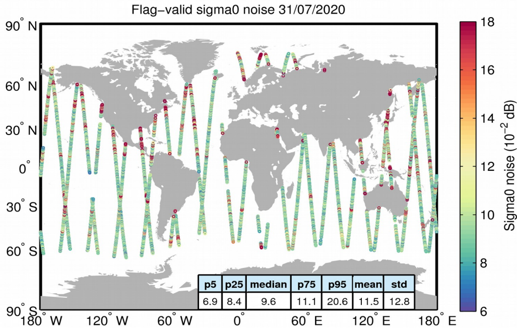
Figure 26. Geographical distribution of flag-valid 20-Hz sigma0 measurement noise over oceans and lakes for 31/07/2020. The statistical values shown in the table refer to the sigma0 noise and are calculated over all measurements shown in the figure.
