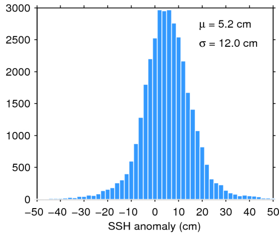
Figure 11. Histogram of science-valid SSH anomaly over oceans and lakes for 31/07/2020. The mean ( \mu ) and standard deviation ( \sigma ) are also shown. Note that values outside [-50 50] cm are excluded from the histogram for the sake of readability but not from the computation of \mu and \sigma .
