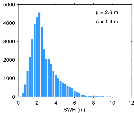
Figure 17. Histogram of flag-valid SWH over oceans and lakes for 31/07/2020. The mean ( \mu ) and standard deviation ( \sigma ) are also shown. Note that values larger than 12 m are excluded from the histogram for the sake of readability but not from the computation of \mu and \sigma .
