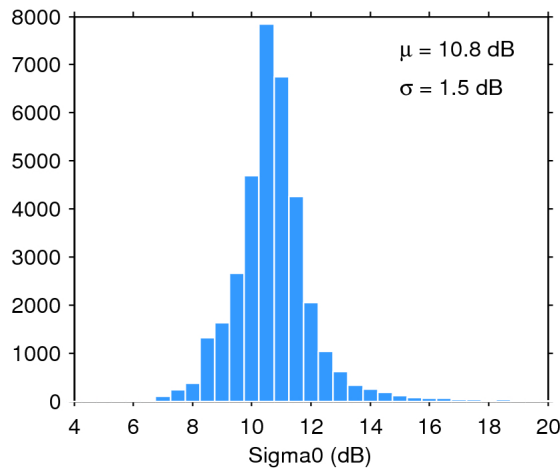
Figure 28. Histogram of science-valid sigma0 over oceans and lakes for 30/07/2020. The mean ( \mu ) and standard deviation ( \sigma ) are also shown. Note that values outside [4 20] dB are excluded from the histogram for the sake of readability but not from the computation of \mu and \sigma .
