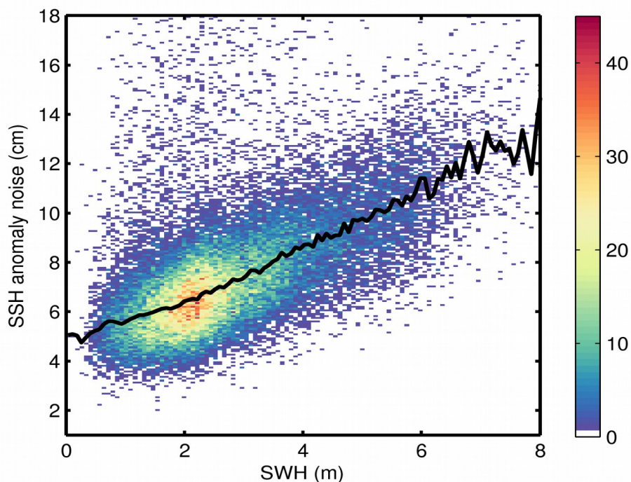
Figure 9. 2D histogram showing flag-valid SSH anomaly noise as a function of SWH for 30/07/2020. The black line denotes the median SSH anomaly noise as a function of SWH.
