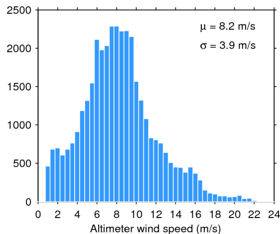
Figure 35. Histogram of science-valid wind over oceans and lakes for 30/07/2020. The mean ( \mu ) and standard deviation ( \sigma ) are also shown. Note that values larger than 24 m/s are excluded from the histogram for the sake of readability but not from the computation of \mu and \sigma .
