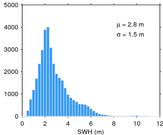
Figure 20. Histogram of science-valid SWH over oceans and lakes for 30/07/2020. The mean ( \mu ) and standard deviation ( \sigma ) are also shown. Note that values larger than 12 m are excluded from the histogram for the sake of readability but not from the computation of \mu and \sigma .
