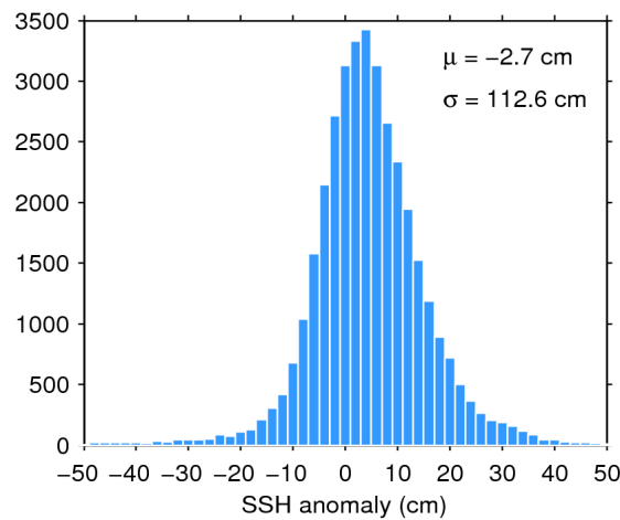
Figure 7. Histogram of flag-valid SSH anomaly over oceans and lakes for 30/07/2020. The mean ( \mu ) and standard deviation ( \sigma ) are also shown. Note that values outside [-50 50] cm are excluded from the histogram for the sake of readability but not from the computation of \mu and \sigma .
