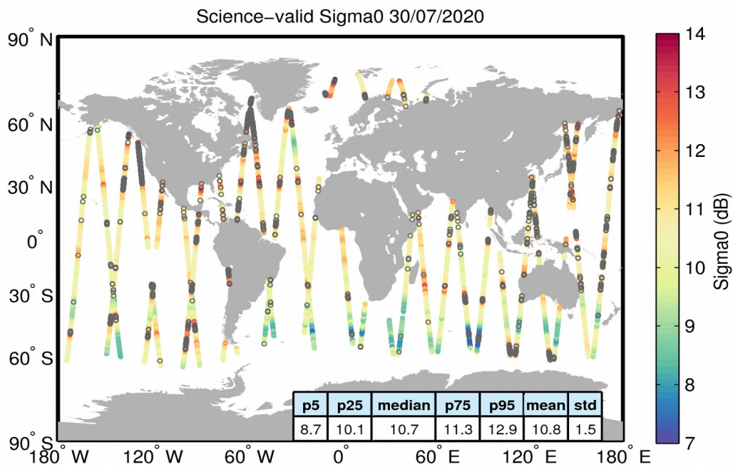
Figure 27. Geographical distribution of science-valid sigma0 data over oceans and lakes for 30/07/2020. The statistical values shown in the table refer to the sigma0 in dB and are calculated over all measurements shown in the figure. Gray circles denote records that have been rejected based on the editing criteria described in Table 4.
