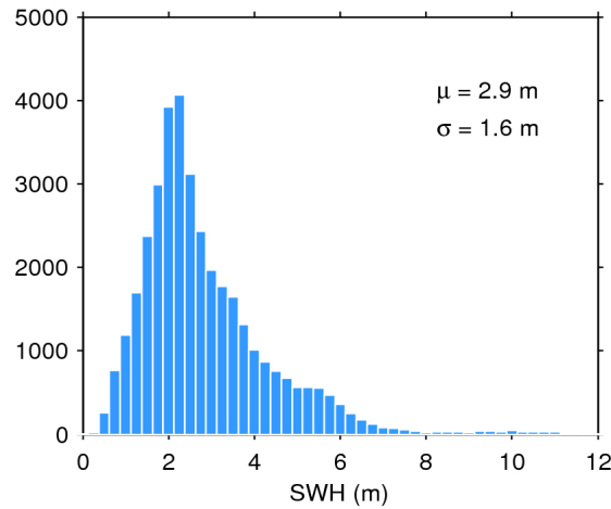
Figure 17. Histogram of flag-valid SWH over oceans and lakes for 30/07/2020. The mean ( \mu ) and standard deviation ( \sigma ) are also shown. Note that values larger than 12 m are excluded from the histogram for the sake of readability but not from the computation of \mu and \sigma .
