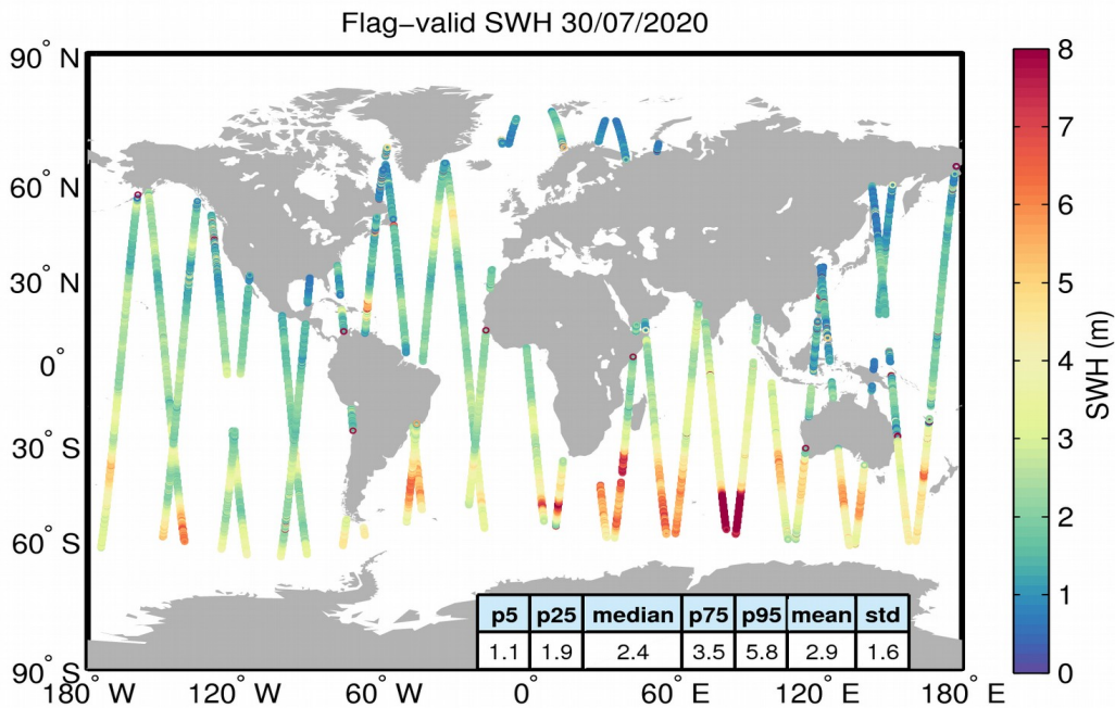
Figure 15. Geographical distribution of flag-valid SWH data over oceans and lakes for 30/07/2020. The statistical values shown in the table refer to the SWH in m and are calculated over all measurements shown in the figure.
