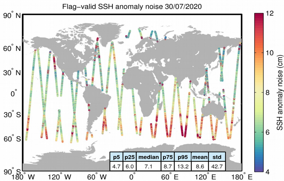
Figure 8. Geographical distribution of flag-valid 20-Hz SSH anomaly measurement noise over oceans and lakes for 30/07/2020. The statistical values shown in the table refer to the SSH anomaly noise and are calculated over all measurements shown in the figure.
