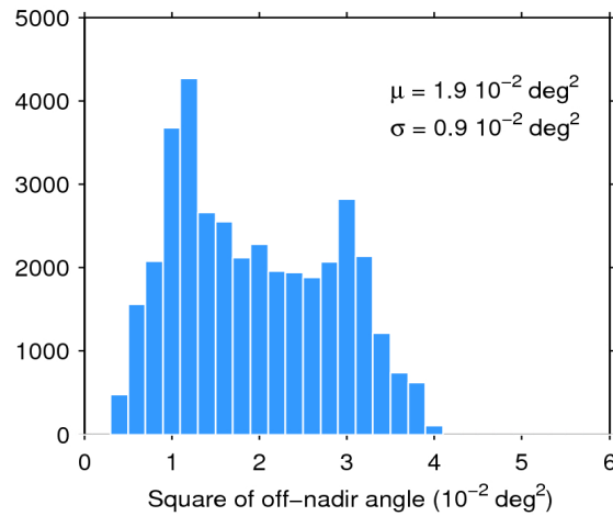
Figure 39. Histogram of flag-valid mispointing over oceans and lakes for 30/07/2020. The mean ( \mu ) and standard deviation ( \sigma ) are also shown. Note that values larger than 6 \cdot 10^{-2} \text{ deg}^2 are excluded from the histogram for the sake of readability but not from the computation of \mu and \sigma .
