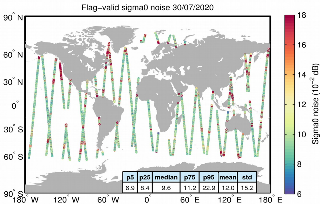
Figure 26. Geographical distribution of flag-valid 20-Hz sigma0 measurement noise over oceans and lakes for 30/07/2020. The statistical values shown in the table refer to the sigma0 noise and are calculated over all measurements shown in the figure.
