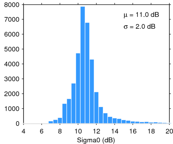
Figure 25. Histogram of flag-valid sigma0 over oceans and lakes for 30/07/2020. The mean ( \mu ) and standard deviation ( \sigma ) are also shown. Note that values outside [4 20] dB are excluded from the histogram for the sake of readability but not from the computation of \mu and \sigma .
