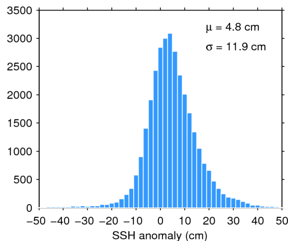
Figure 11. Histogram of science-valid SSH anomaly over oceans and lakes for 30/07/2020. The mean ( \mu ) and standard deviation ( \sigma ) are also shown. Note that values outside [-50 50] cm are excluded from the histogram for the sake of readability but not from the computation of \mu and \sigma .
