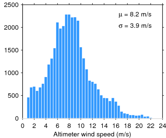
Figure 33. Histogram of flag-valid wind over oceans and lakes for 30/07/2020. The mean ( \mu ) and standard deviation ( \sigma ) are also shown. Note that values larger than 24 m/s are excluded from the histogram for the sake of readability but not from the computation of \mu and \sigma .
