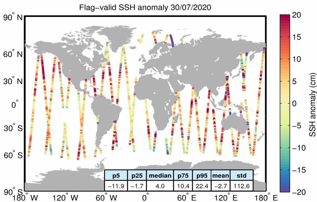
Figure 5. Geographical distribution of flag-valid 1-Hz SSH anomaly data over oceans and lakes for 30/07/2020. The statistical values shown in the table refer to the SSH anomaly in cm and are calculated over all measurements shown in the figure.
