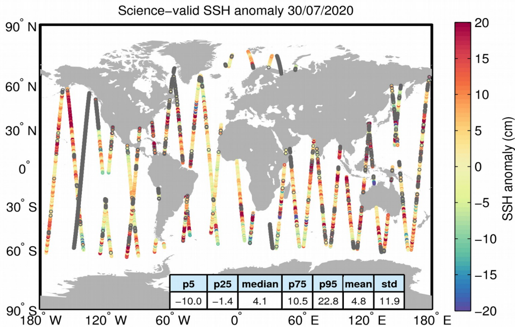
Figure 10. Geographical distribution of science-valid SSH anomaly data over oceans and lakes for 30/07/2020. The statistical values shown in the table refer to the SSH anomaly in cm and are calculated over all measurements shown in the figure. Gray circles denote records that have been rejected based on the editing criteria described in Table 2.
