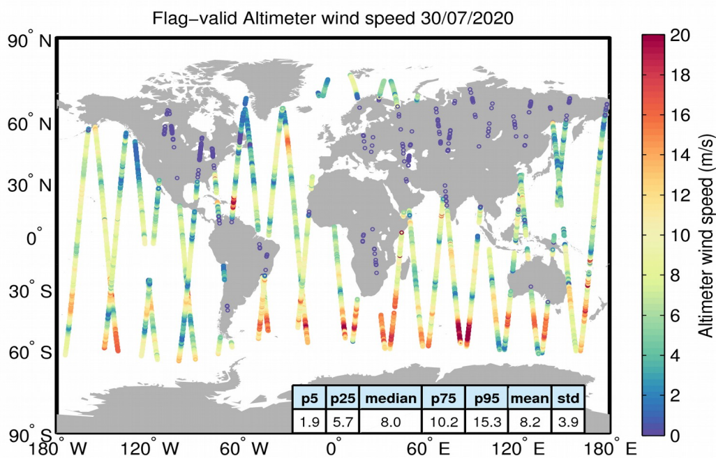
Figure 31. Geographical distribution of flag-valid wind data over oceans and lakes for 30/07/2020. The statistical values shown in the figure refer to the wind in m/s and are calculated over all measurements shown in the figure.
