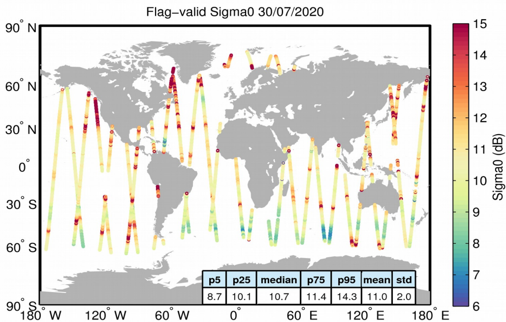
Figure 23. Geographical distribution of flag-valid sigma0 data over oceans and lakes for 30/07/2020. The statistical values shown in the table refer to the sigma0 in dB and are calculated over all measurements shown in the figure.
