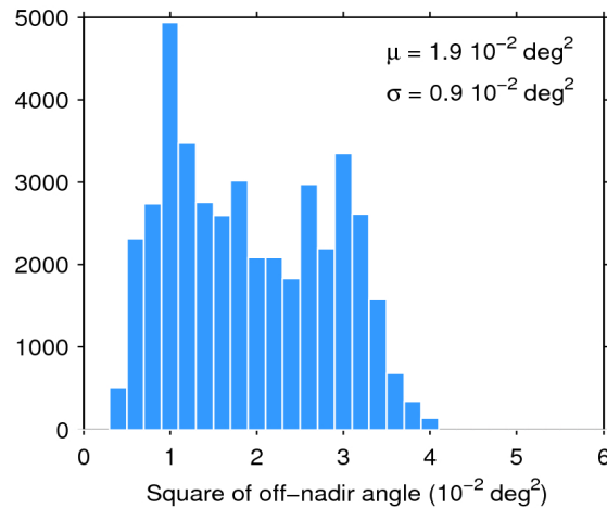
Figure 39. Histogram of flag-valid mispointing over oceans and lakes for 29/07/2020. The mean ( \mu ) and standard deviation ( \sigma ) are also shown. Note that values larger than 6 \cdot 10^{-2} \text{ deg}^2 are excluded from the histogram for the sake of readability but not from the computation of \mu and \sigma .
