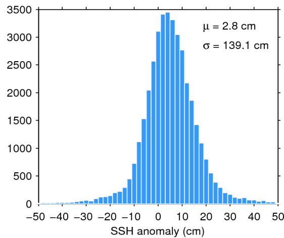
Figure 7. Histogram of flag-valid SSH anomaly over oceans and lakes for 29/07/2020. The mean ( \mu ) and standard deviation ( \sigma ) are also shown. Note that values outside [-50 50] cm are excluded from the histogram for the sake of readability but not from the computation of \mu and \sigma .
