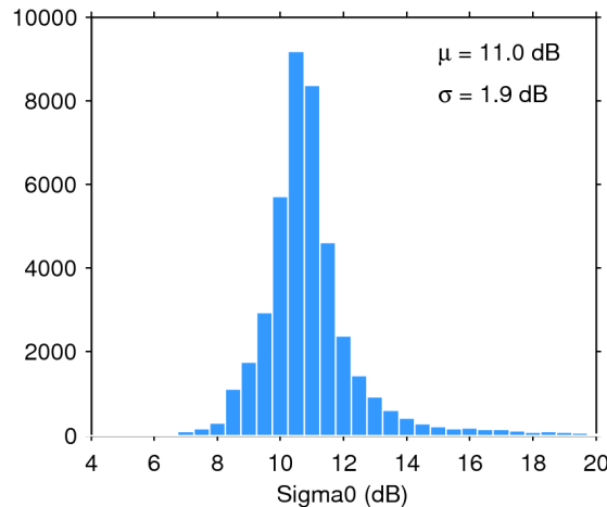
Figure 25. Histogram of flag-valid sigma0 over oceans and lakes for 29/07/2020. The mean ( \mu ) and standard deviation ( \sigma ) are also shown. Note that values outside [4 20] dB are excluded from the histogram for the sake of readability but not from the computation of \mu and \sigma .
