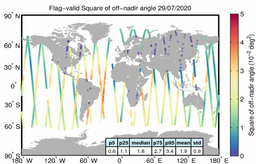
Figure 37. Geographical distribution of flag-valid mispointing data over oceans and lakes for 29/07/2020. The statistical values shown in the table refer to the mispointing in 10^{-2} deg 2 and are calculated over all measurements shown in the figure.
