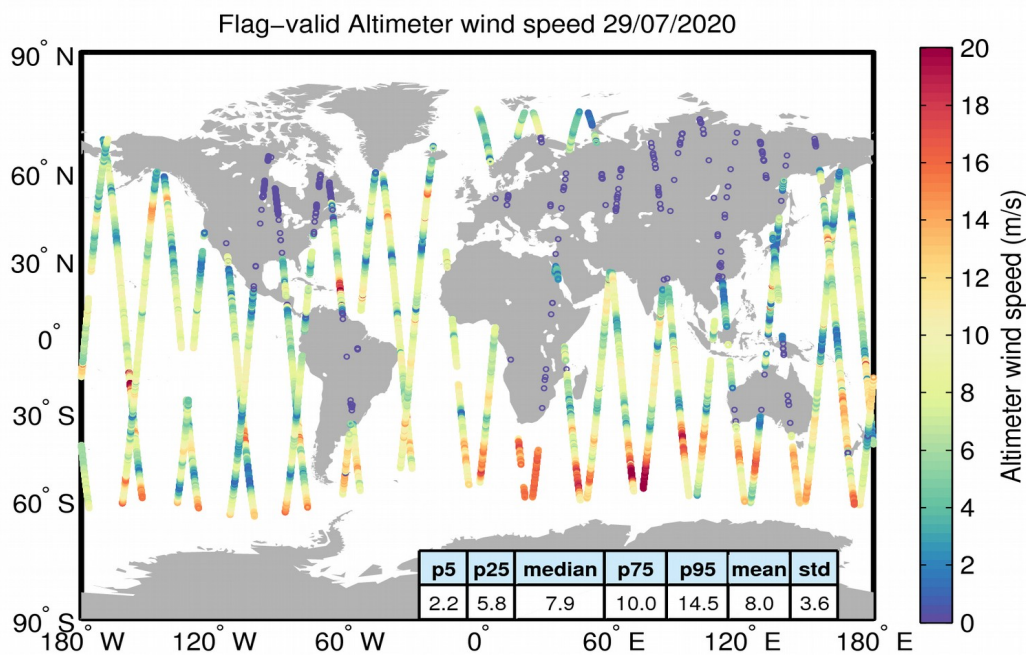
Figure 31. Geographical distribution of flag-valid wind data over oceans and lakes for 29/07/2020. The statistical values shown in the table refer to the wind in m/s and are calculated over all measurements shown in the figure.
