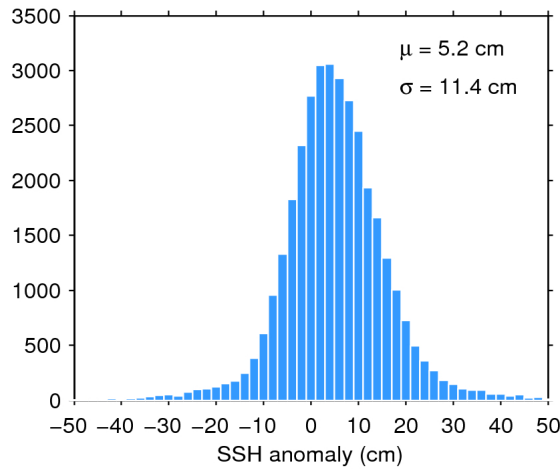
Figure 11. Histogram of science-valid SSH anomaly over oceans and lakes for 29/07/2020. The mean ( \mu ) and standard deviation ( \sigma ) are also shown. Note that values outside [-50 50] cm are excluded from the histogram for the sake of readability but not from the computation of \mu and \sigma .
