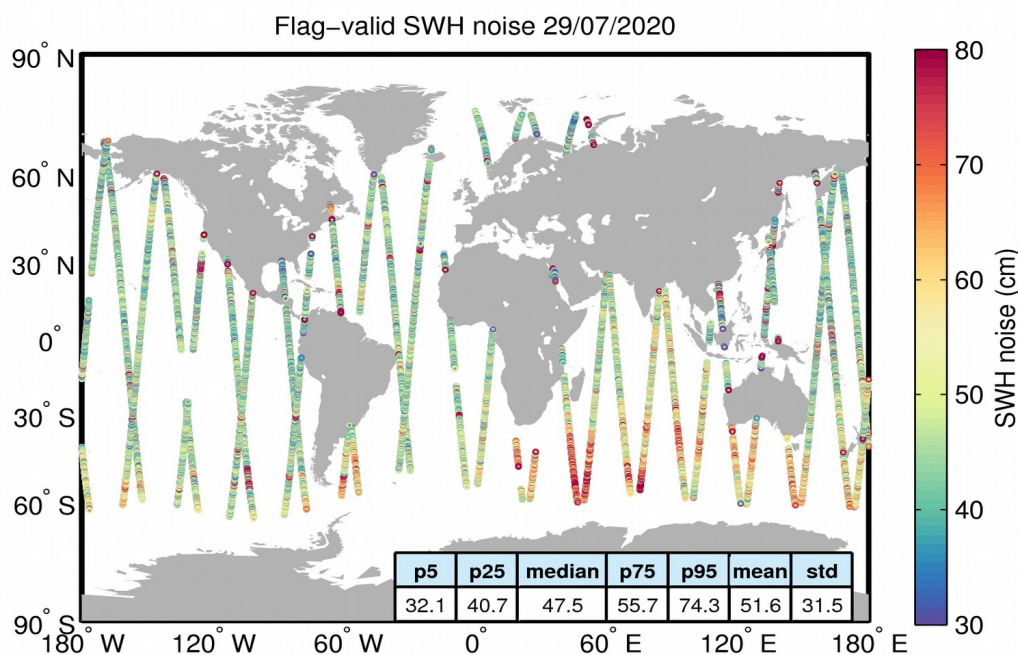
Figure 18. Geographical distribution of flag-valid 20-Hz SWH measurement noise over oceans and lakes for 29/07/2020. The statistical values shown in the figure refer to the SWH noise and are calculated over all measurements shown in the figure.
