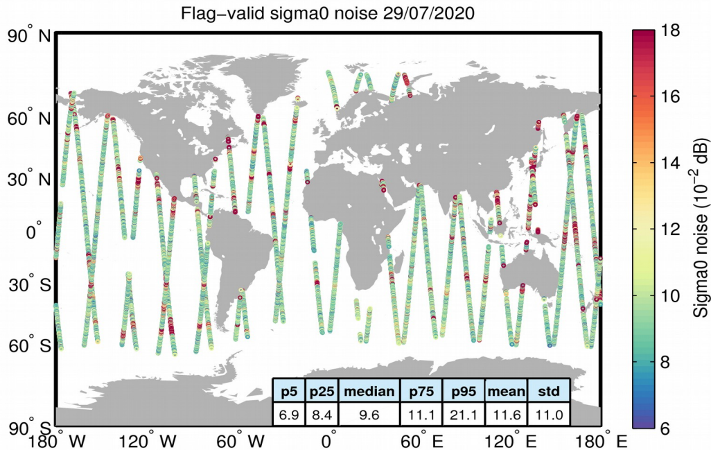
Figure 26. Geographical distribution of flag-valid 20-Hz sigma0 measurement noise over oceans and lakes for 29/07/2020. The statistical values shown in the table refer to the sigma0 noise and are calculated over all measurements shown in the figure.
