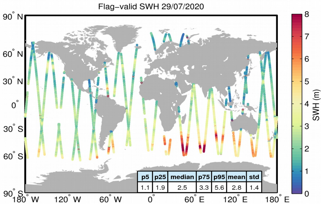
Figure 15. Geographical distribution of flag-valid SWH data over oceans and lakes for 29/07/2020. The statistical values shown in the table refer to the SWH in m and are calculated over all measurements shown in the figure.
