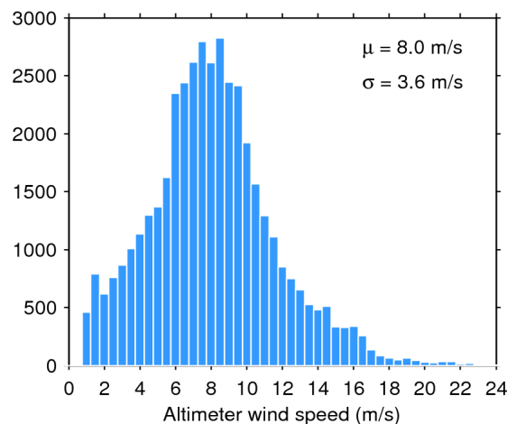
Figure 35. Histogram of science-valid wind over oceans and lakes for 29/07/2020. The mean ( \mu ) and standard deviation ( \sigma ) are also shown. Note that values larger than 24 m/s are excluded from the histogram for the sake of readability but not from the computation of \mu and \sigma .
