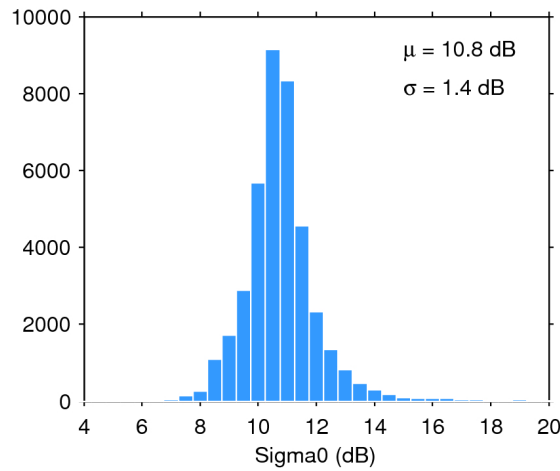
Figure 28. Histogram of science-valid sigma0 over oceans and lakes for 29/07/2020. The mean ( \mu ) and standard deviation ( \sigma ) are also shown. Note that values outside [4 20] dB are excluded from the histogram for the sake of readability but not from the computation of \mu and \sigma .
