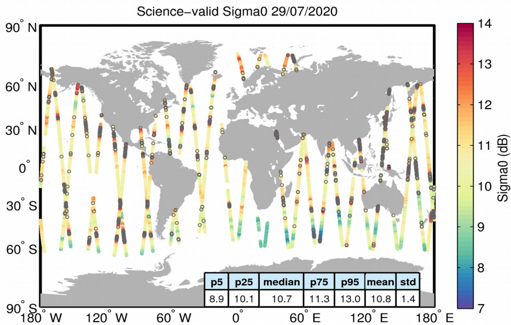
Figure 27. Geographical distribution of science-valid sigma0 data over oceans and lakes for 29/07/2020. The statistical values shown in the table refer to the sigma0 in dB and are calculated over all measurements shown in the figure. Gray circles denote records that have been rejected based on the editing criteria described in Table 4.
