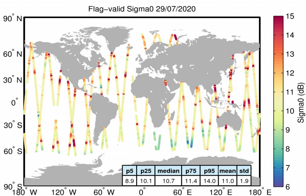
Figure 23. Geographical distribution of flag-valid sigma0 data over oceans and lakes for 29/07/2020. The statistical values shown in the table refer to the sigma0 in dB and are calculated over all measurements shown in the figure.
