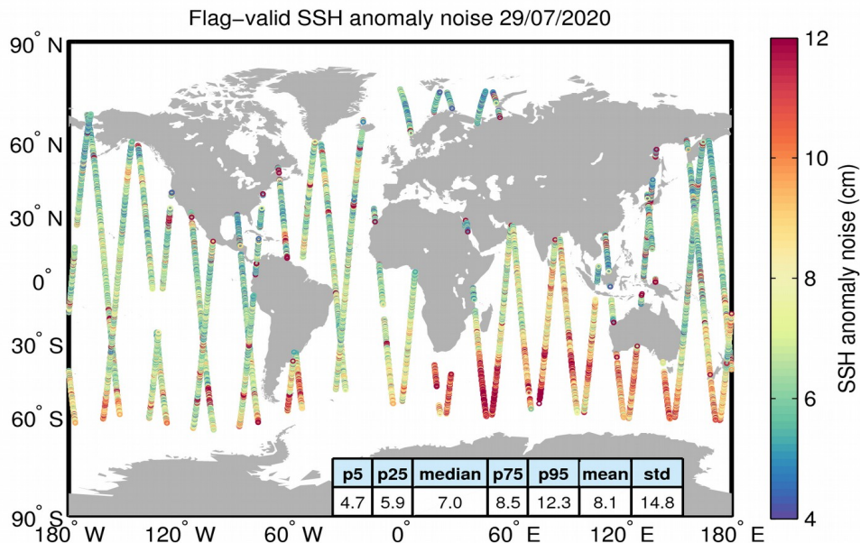
Figure 8. Geographical distribution of flag-valid 20-Hz SSH anomaly measurement noise over oceans and lakes for 29/07/2020. The statistical values shown in the table refer to the SSH anomaly noise and are calculated over all measurements shown in the figure.
