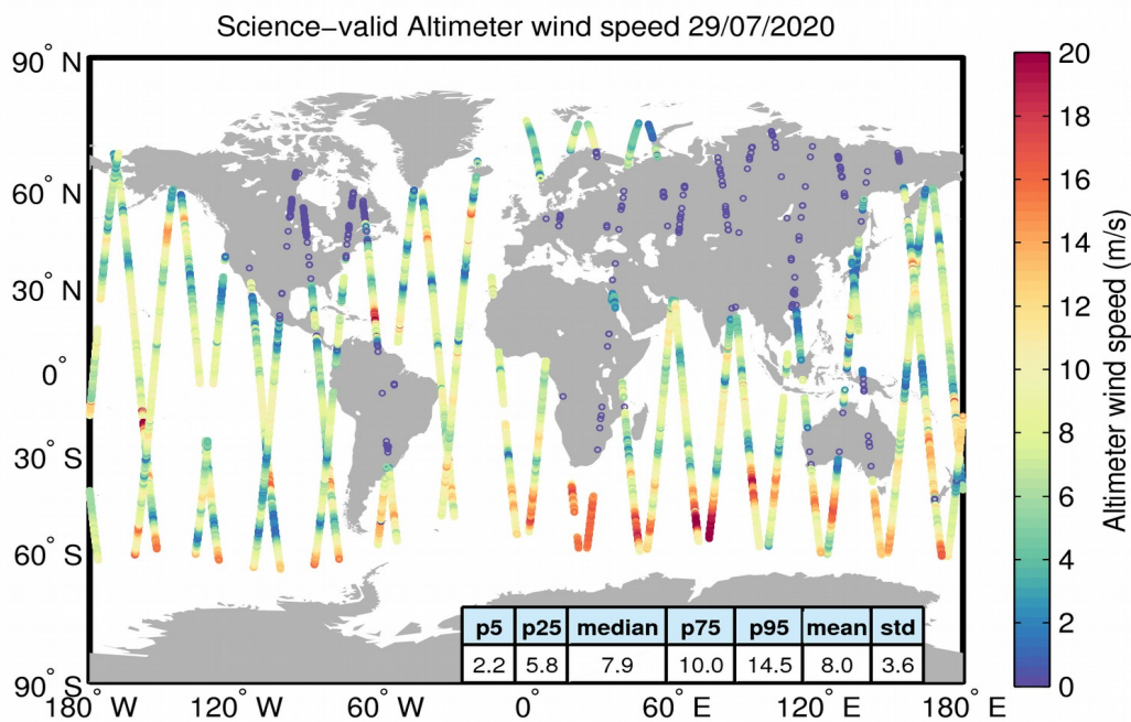
Figure 34. Geographical distribution of science-valid wind data over oceans and lakes for 29/07/2020. The statistical values shown in the table refer to the wind in m/s and are calculated over all measurements shown in the figure. Gray circles denote records that have been rejected based on the editing criteria described in Table 5.
