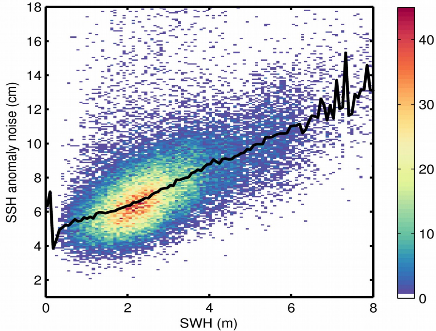
Figure 9. 2D histogram showing flag-valid SSH anomaly noise as a function of SWH for 29/07/2020. The black line denotes the median SSH anomaly noise as a function of SWH.
