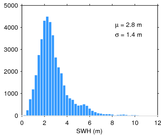
Figure 17. Histogram of flag-valid SWH over oceans and lakes for 29/07/2020. The mean ( \mu ) and standard deviation ( \sigma ) are also shown. Note that values larger than 12 m are excluded from the histogram for the sake of readability but not from the computation of \mu and \sigma .
