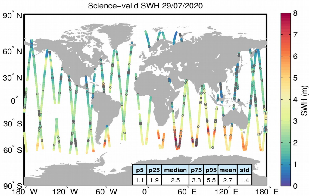
Figure 19. Geographical distribution of science-valid SWH data over oceans and lakes for 29/07/2020. The statistical values shown in the table refer to the SWH in m and are calculated over all measurements shown in the figure. Gray circles denote records that have been rejected based on the editing criteria described in Table 3.
