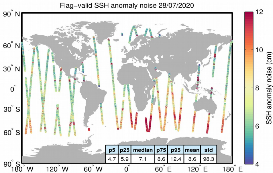
Figure 8. Geographical distribution of flag-valid 20-Hz SSH anomaly measurement noise over oceans and lakes for 28/07/2020. The statistical values shown in the table refer to the SSH anomaly noise and are calculated over all measurements shown in the figure.
