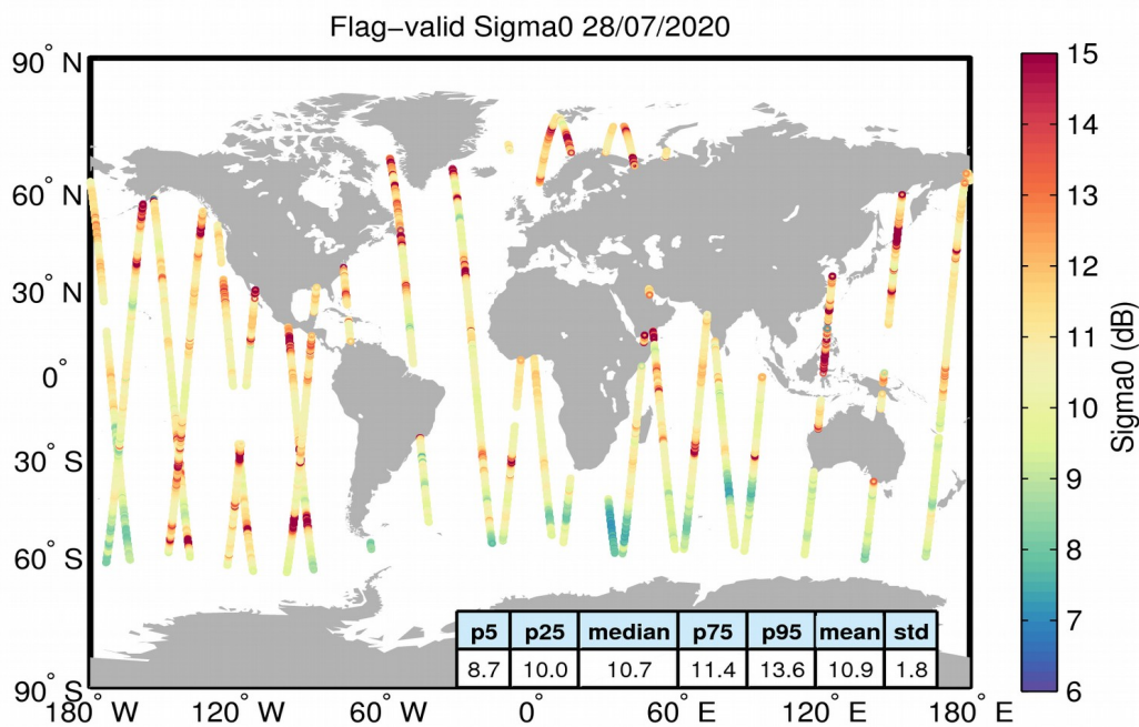
Figure 23. Geographical distribution of flag-valid sigma0 data over oceans and lakes for 28/07/2020. The statistical values shown in the table refer to the sigma0 in dB and are calculated over all measurements shown in the figure.
