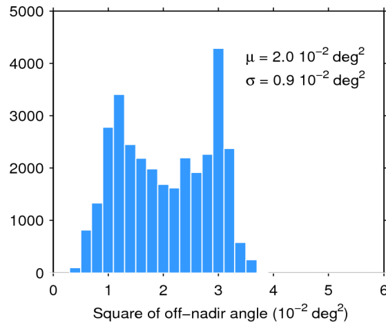
Figure 39. Histogram of flag-valid mispointing over oceans and lakes for 28/07/2020. The mean ( \mu ) and standard deviation ( \sigma ) are also shown. Note that values larger than 6 \cdot 10^{-2} \text{ deg}^2 are excluded from the histogram for the sake of readability but not from the computation of \mu and \sigma .
