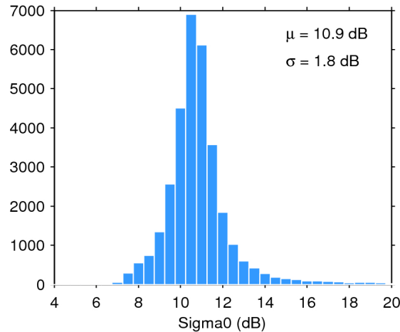
Figure 25. Histogram of flag-valid sigma0 over oceans and lakes for 28/07/2020. The mean ( \mu ) and standard deviation ( \sigma ) are also shown. Note that values outside [4 20] dB are excluded from the histogram for the sake of readability but not from the computation of \mu and \sigma .
