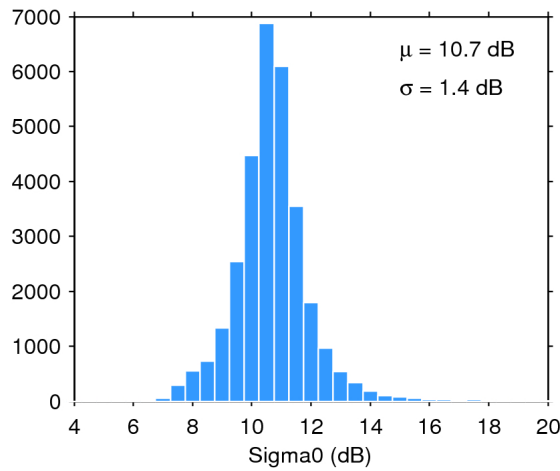
Figure 28. Histogram of science-valid sigma0 over oceans and lakes for 28/07/2020. The mean ( \mu ) and standard deviation ( \sigma ) are also shown. Note that values outside [4 20] dB are excluded from the histogram for the sake of readability but not from the computation of \mu and \sigma .
