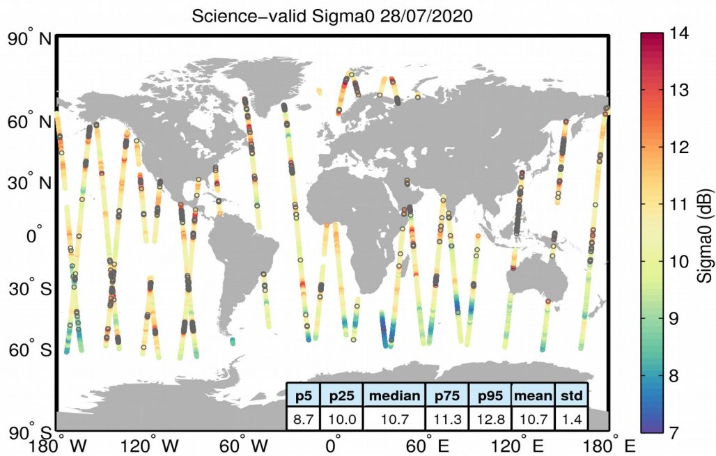
Figure 27. Geographical distribution of science-valid sigma0 data over oceans and lakes for 28/07/2020. The statistical values shown in the table refer to the sigma0 in dB and are calculated over all measurements shown in the figure. Gray circles denote records that have been rejected based on the editing criteria described in Table 4.
