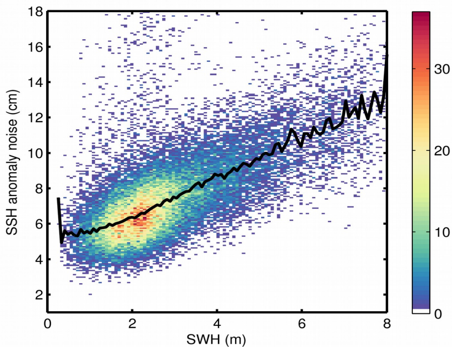
Figure 9. 2D histogram showing flag-valid SSH anomaly noise as a function of SWH for 28/07/2020. The black line denotes the median SSH anomaly noise as a function of SWH.
