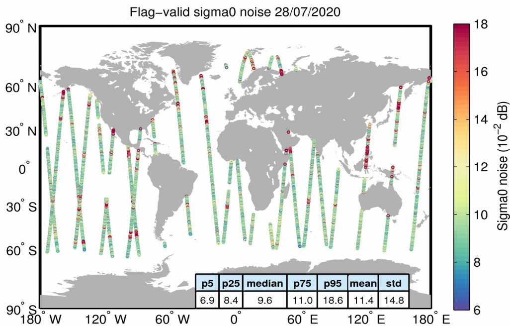
Figure 26. Geographical distribution of flag-valid 20-Hz sigma0 measurement noise over oceans and lakes for 28/07/2020. The statistical values shown in the table refer to the sigma0 noise and are calculated over all measurements shown in the figure.
