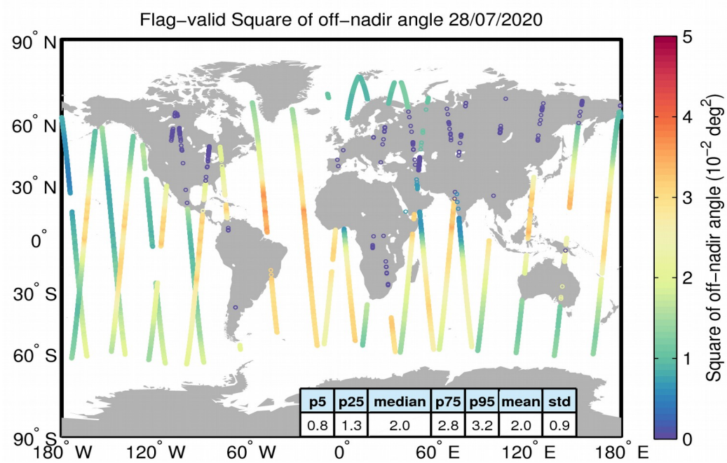
Figure 37. Geographical distribution of flag-valid mispointing data over oceans and lakes for 28/07/2020. The statistical values shown in the table refer to the mispointing in 10^{-2} \text{ deg}^2 and are calculated over all measurements shown in the figure.
