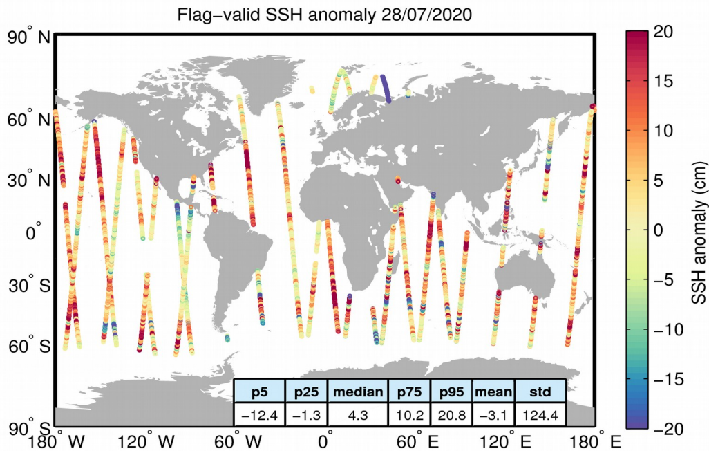
Figure 5. Geographical distribution of flag-valid 1-Hz SSH anomaly data over oceans and lakes for 28/07/2020. The statistical values shown in the table refer to the SSH anomaly in cm and are calculated over all measurements shown in the figure.
