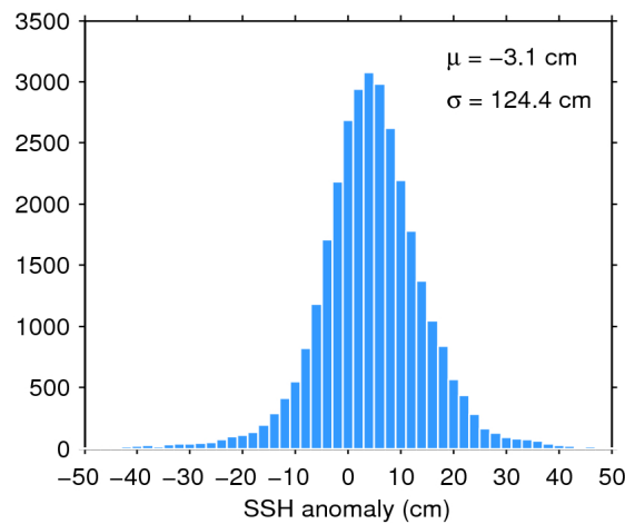
Figure 7. Histogram of flag-valid SSH anomaly over oceans and lakes for 28/07/2020. The mean ( \mu ) and standard deviation ( \sigma ) are also shown. Note that values outside [-50 50] cm are excluded from the histogram for the sake of readability but not from the computation of \mu and \sigma .
