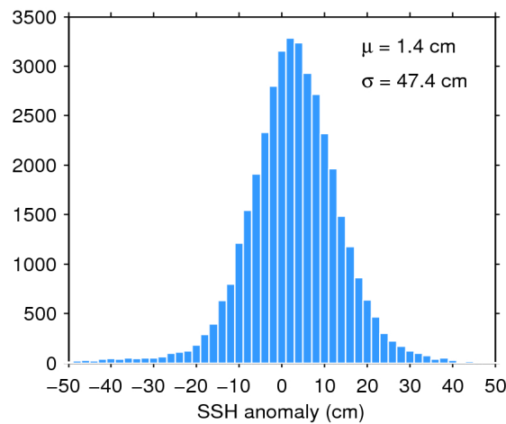
Figure 7. Histogram of flag-valid SSH anomaly over oceans and lakes for 27/07/2020. The mean ( \mu ) and standard deviation ( \sigma ) are also shown. Note that values outside [-50\ 50] cm are excluded from the histogram for the sake of readability but not from the computation of \mu and \sigma .
