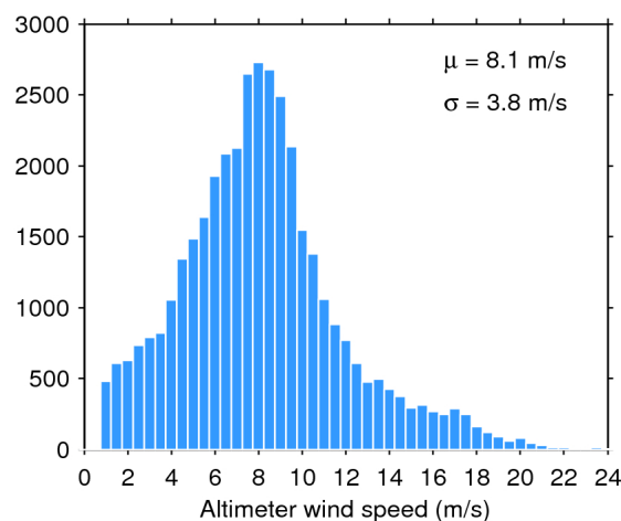
Figure 35. Histogram of science-valid wind over oceans and lakes for 27/07/2020. The mean ( \mu ) and standard deviation ( \sigma ) are also shown. Note that values larger than 24 m/s are excluded from the histogram for the sake of readability but not from the computation of \mu and \sigma .
