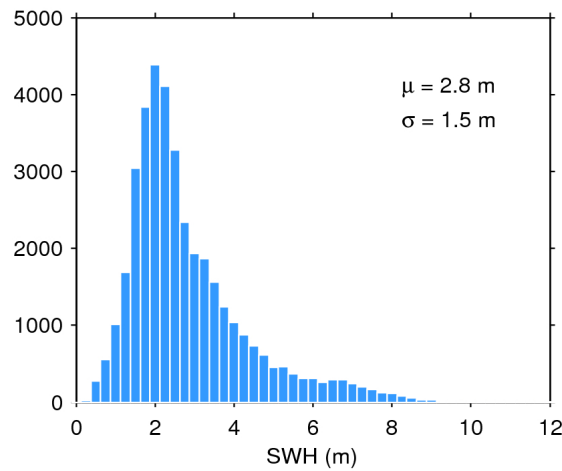
Figure 17. Histogram of flag-valid SWH over oceans and lakes for 27/07/2020. The mean ( \mu ) and standard deviation ( \sigma ) are also shown. Note that values larger than 12 m are excluded from the histogram for the sake of readability but not from the computation of \mu and \sigma .
