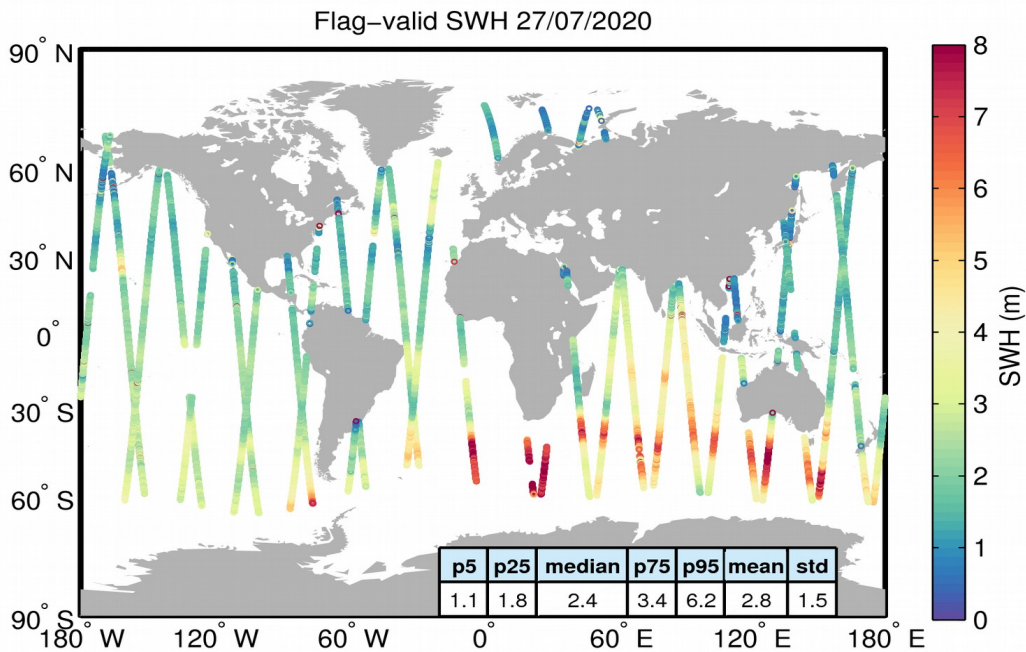
Figure 15. Geographical distribution of flag-valid SWH data over oceans and lakes for 27/07/2020. The statistical values shown in the table refer to the SWH in m and are calculated over all measurements shown in the figure.
