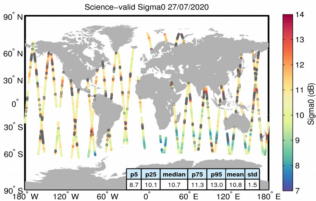
Figure 27. Geographical distribution of science-valid sigma0 data over oceans and lakes for 27/07/2020. The statistical values shown in the table refer to the sigma0 in dB and are calculated over all measurements shown in the figure. Gray circles denote records that have been rejected based on the editing criteria described in Table 4.
