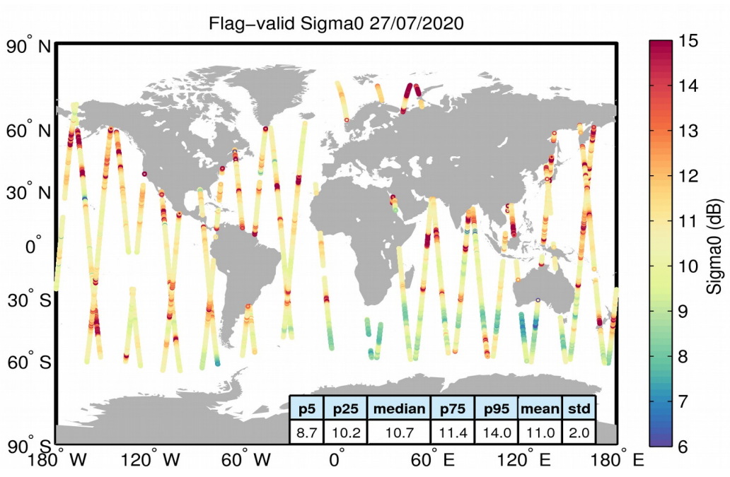
Figure 23. Geographical distribution of flag-valid sigma0 data over oceans and lakes for 27/07/2020. The statistical values shown in the table refer to the sigma0 in dB and are calculated over all measurements shown in the figure.
