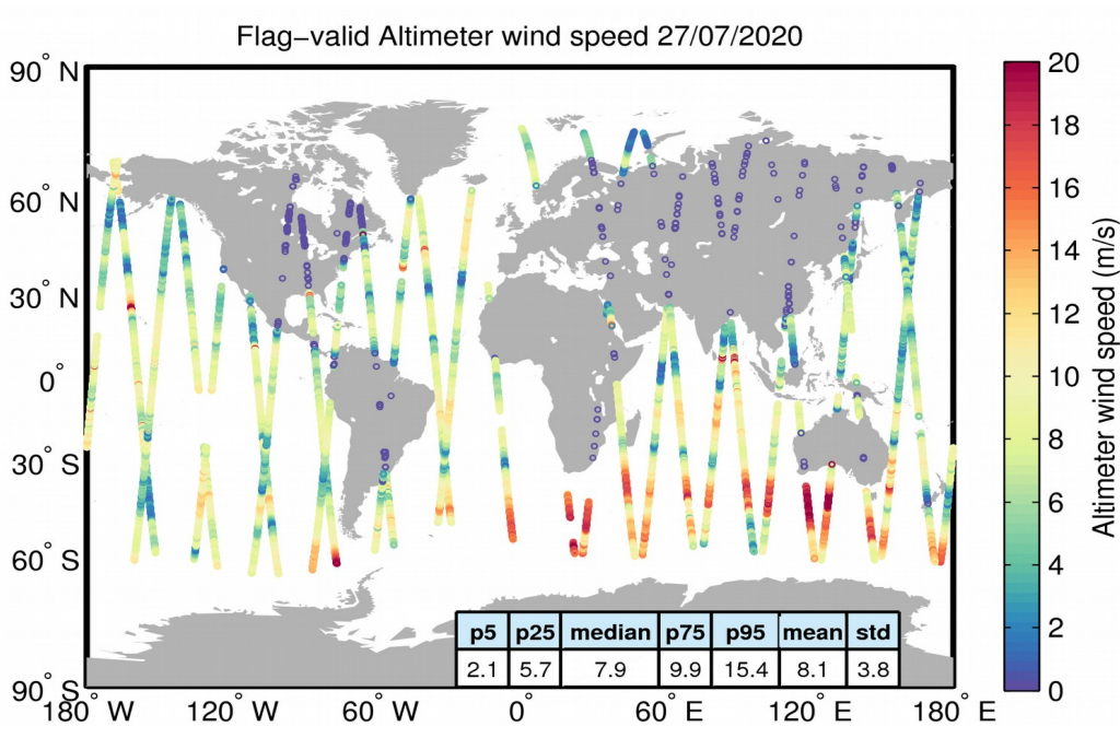
Figure 31. Geographical distribution of flag-valid wind data over oceans and lakes for 27/07/2020. The statistical values shown in the table refer to the wind in m/s and are calculated over all measurements shown in the figure.
