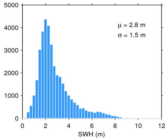
Figure 20. Histogram of science-valid SWH over oceans and lakes for 27/07/2020. The mean ( \mu ) and standard deviation ( \sigma ) are also shown. Note that values larger than 12 m are excluded from the histogram for the sake of readability but not from the computation of \mu and \sigma .
