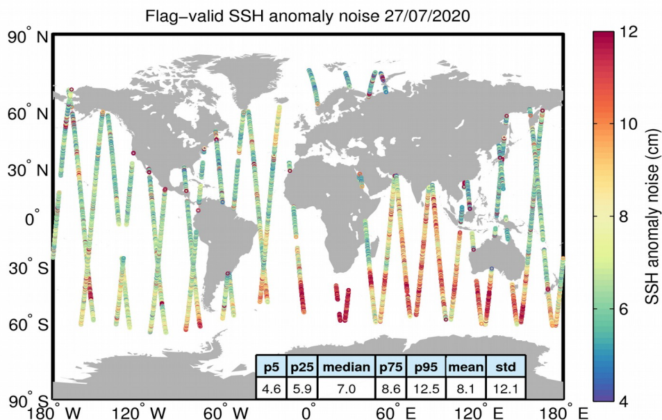
Figure 8. Geographical distribution of flag-valid 20-Hz SSH anomaly measurement noise over oceans and lakes for 27/07/2020. The statistical values shown in the table refer to the SSH anomaly noise and are calculated over all measurements shown in the figure.
