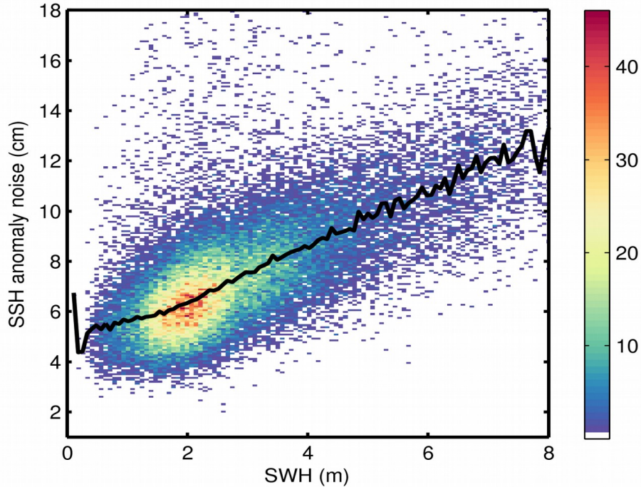
Figure 9. 2D histogram showing flag-valid SSH anomaly noise as a function of SWH for 27/07/2020. The black line denotes the median SSH anomaly noise as a function of SWH.
