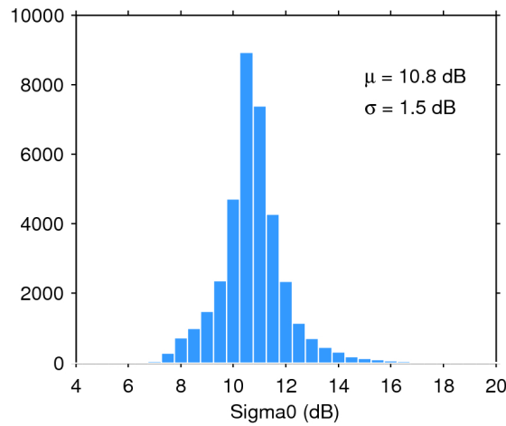
Figure 28. Histogram of science-valid sigma0 over oceans and lakes for 27/07/2020. The mean ( \mu ) and standard deviation ( \sigma ) are also shown. Note that values outside [4 20] dB are excluded from the histogram for the sake of readability but not from the computation of \mu and \sigma .
