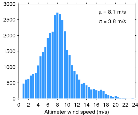
Figure 33. Histogram of flag-valid wind over oceans and lakes for 27/07/2020. The mean ( \mu ) and standard deviation ( \sigma ) are also shown. Note that values larger than 24 m/s are excluded from the histogram for the sake of readability but not from the computation of \mu and \sigma .
