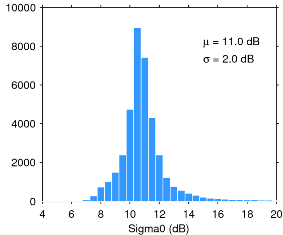
Figure 25. Histogram of flag-valid sigma0 over oceans and lakes for 27/07/2020. The mean ( \mu ) and standard deviation ( \sigma ) are also shown. Note that values outside [4 20] dB are excluded from the histogram for the sake of readability but not from the computation of \mu and \sigma .
