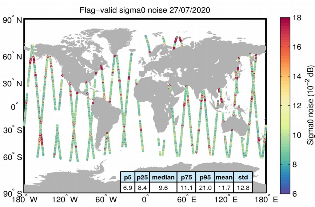
Figure 26. Geographical distribution of flag-valid 20-Hz sigma0 measurement noise over oceans and lakes for 27/07/2020. The statistical values shown in the table refer to the sigma0 noise and are calculated over all measurements shown in the figure.
