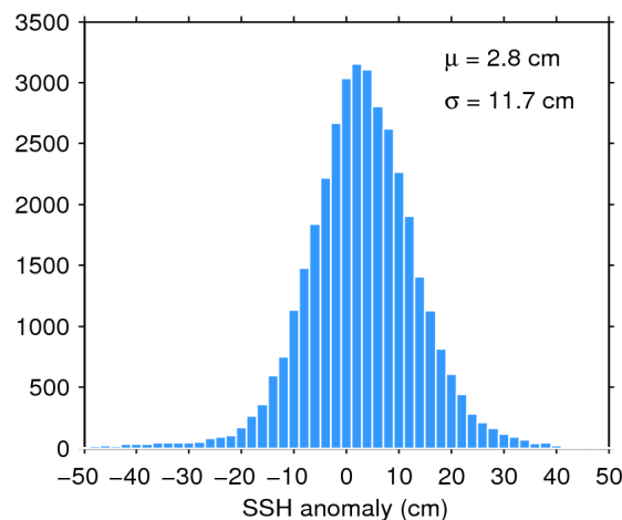
Figure 11. Histogram of science-valid SSH anomaly over oceans and lakes for 27/07/2020. The mean ( \mu ) and standard deviation ( \sigma ) are also shown. Note that values outside [-50 50] cm are excluded from the histogram for the sake of readability but not from the computation of \mu and \sigma .
