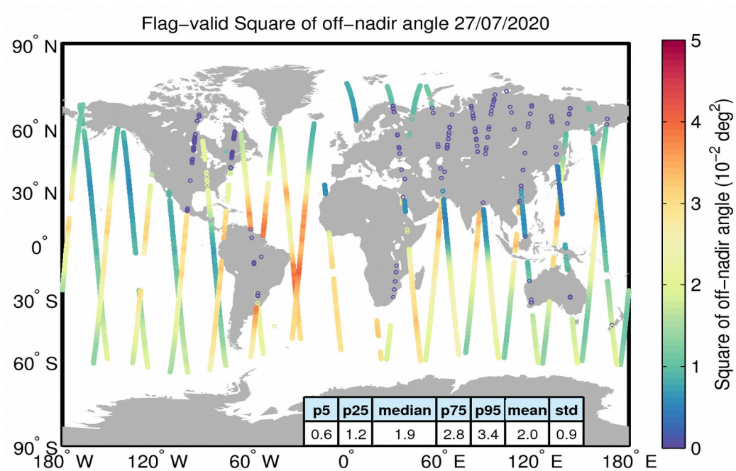
Figure 37. Geographical distribution of flag-valid mispointing data over oceans and lakes for 27/07/2020. The statistical values shown in the table refer to the mispointing in 10^{-2} deg 2 and are calculated over all measurements shown in the figure.
