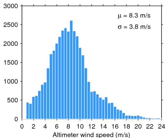
Figure 35. Histogram of science-valid wind over oceans and lakes for 26/07/2020. The mean ( \mu ) and standard deviation ( \sigma ) are also shown. Note that values larger than 24 m/s are excluded from the histogram for the sake of readability but not from the computation of \mu and \sigma .
