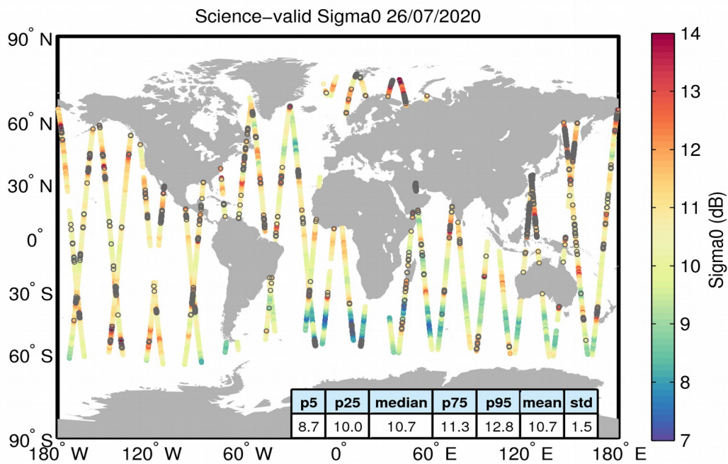
Figure 27. Geographical distribution of science-valid sigma0 data over oceans and lakes for 26/07/2020. The statistical values shown in the table refer to the sigma0 in dB and are calculated over all measurements shown in the figure. Gray circles denote records that have been rejected based on the editing criteria described in Table 4.
