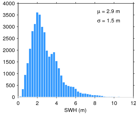
Figure 20. Histogram of science-valid SWH over oceans and lakes for 26/07/2020. The mean ( \mu ) and standard deviation ( \sigma ) are also shown. Note that values larger than 12 m are excluded from the histogram for the sake of readability but not from the computation of \mu and \sigma .
