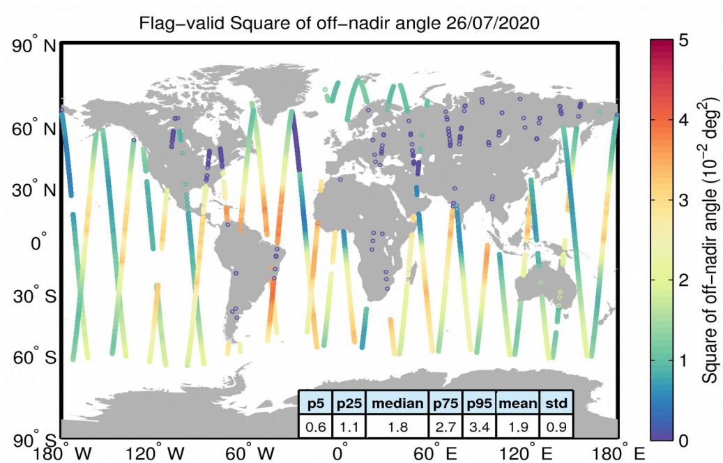
Figure 37. Geographical distribution of flag-valid mispointing data over oceans and lakes for 26/07/2020. The statistical values shown in the table refer to the mispointing in 10^{-2} deg 2 and are calculated over all measurements shown in the figure.
