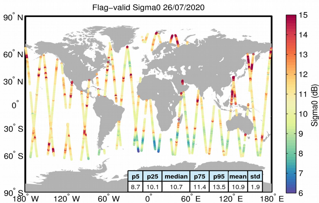
Figure 23. Geographical distribution of flag-valid sigma0 data over oceans and lakes for 26/07/2020. The statistical values shown in the table refer to the sigma0 in dB and are calculated over all measurements shown in the figure.
