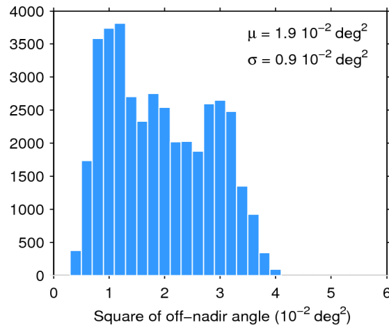
Figure 39. Histogram of flag-valid mispointing over oceans and lakes for 26/07/2020. The mean ( \mu ) and standard deviation ( \sigma ) are also shown. Note that values larger than 6 \cdot 10^{-2} \text{ deg}^2 are excluded from the histogram for the sake of readability but not from the computation of \mu and \sigma .
