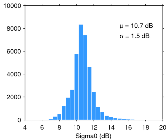
Figure 28. Histogram of science-valid sigma0 over oceans and lakes for 26/07/2020. The mean ( \mu ) and standard deviation ( \sigma ) are also shown. Note that values outside [4 20] dB are excluded from the histogram for the sake of readability but not from the computation of \mu and \sigma .
