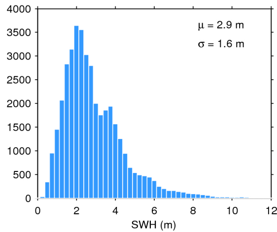
Figure 17. Histogram of flag-valid SWH over oceans and lakes for 26/07/2020. The mean ( \mu ) and standard deviation ( \sigma ) are also shown. Note that values larger than 12 m are excluded from the histogram for the sake of readability but not from the computation of \mu and \sigma .
