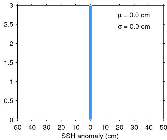
Figure 11. Histogram of science-valid SSH anomaly over oceans and lakes for 26/07/2020. The mean ( \mu ) and standard deviation ( \sigma ) are also shown. Note that values outside [-50 50] cm are excluded from the histogram for the sake of readability but not from the computation of \mu and \sigma .
