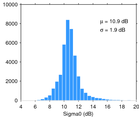
Figure 25. Histogram of flag-valid sigma0 over oceans and lakes for 26/07/2020. The mean ( \mu ) and standard deviation ( \sigma ) are also shown. Note that values outside [4 20] dB are excluded from the histogram for the sake of readability but not from the computation of \mu and \sigma .
