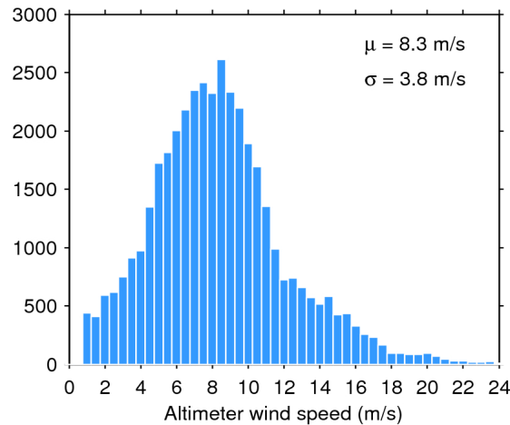
Figure 33. Histogram of flag-valid wind over oceans and lakes for 26/07/2020. The mean ( \mu ) and standard deviation ( \sigma ) are also shown. Note that values larger than 24 m/s are excluded from the histogram for the sake of readability but not from the computation of \mu and \sigma .
