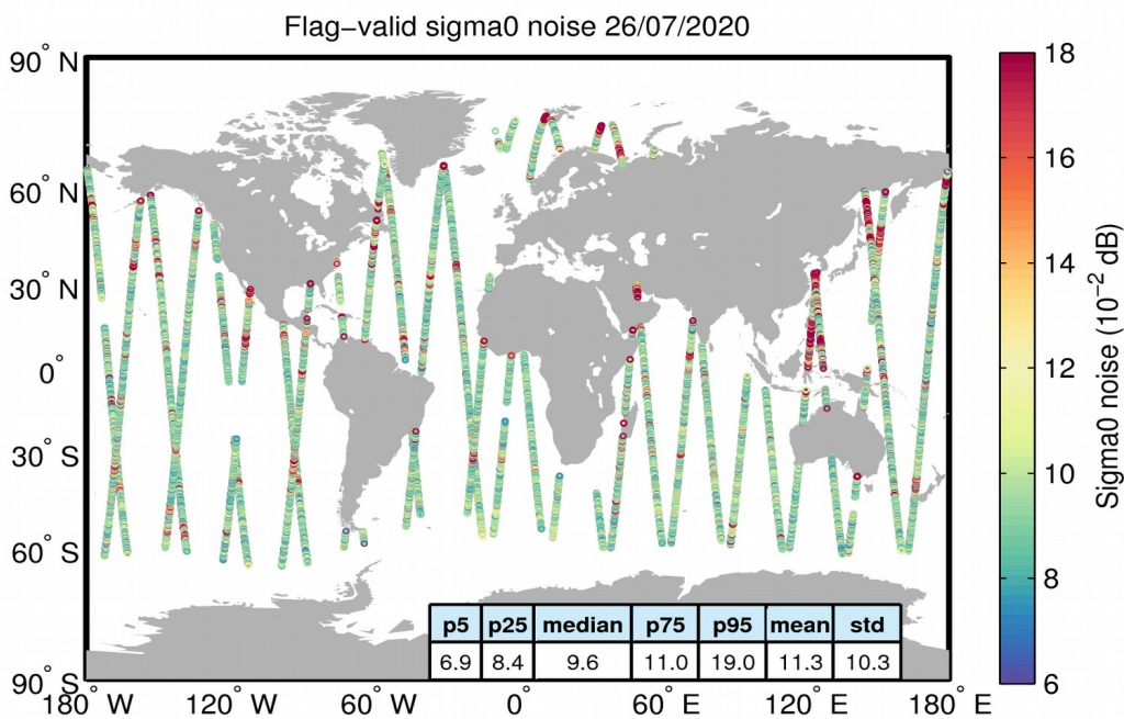
Figure 26. Geographical distribution of flag-valid 20-Hz sigma0 measurement noise over oceans and lakes for 26/07/2020. The statistical values shown in the figure refer to the sigma0 noise and are calculated over all measurements shown in the figure.
