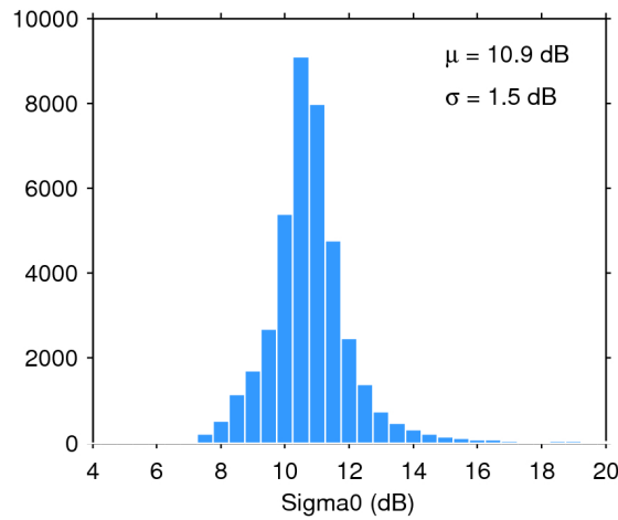
Figure 28. Histogram of science-valid sigma0 over oceans and lakes for 25/07/2020. The mean ( \mu ) and standard deviation ( \sigma ) are also shown. Note that values outside [4 20] dB are excluded from the histogram for the sake of readability but not from the computation of \mu and \sigma .
