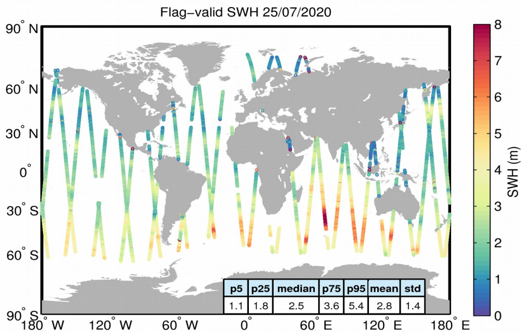
Figure 15. Geographical distribution of flag-valid SWH data over oceans and lakes for 25/07/2020. The statistical values shown in the table refer to the SWH in m and are calculated over all measurements shown in the figure.
