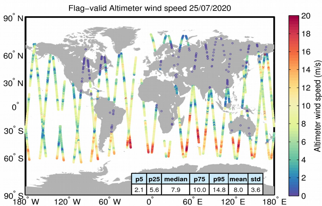
Figure 31. Geographical distribution of flag-valid wind data over oceans and lakes for 25/07/2020. The statistical values shown in the table refer to the wind in m/s and are calculated over all measurements shown in the figure.
