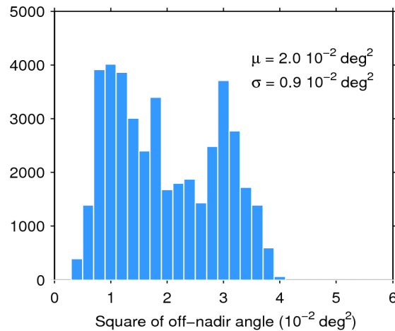
Figure 39. Histogram of flag-valid mispointing over oceans and lakes for 25/07/2020. The mean ( \mu ) and standard deviation ( \sigma ) are also shown. Note that values larger than 6 \cdot 10^{-2} \text{ deg}^2 are excluded from the histogram for the sake of readability but not from the computation of \mu and \sigma .
