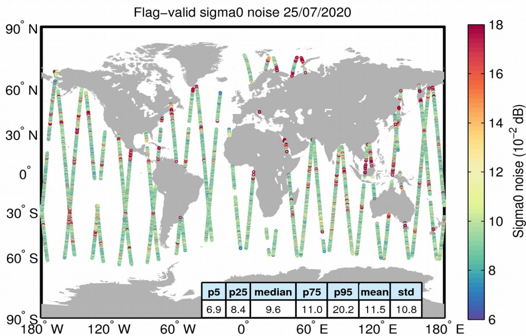
Figure 26. Geographical distribution of flag-valid 20-Hz sigma0 measurement noise over oceans and lakes for 25/07/2020. The statistical values shown in the table refer to the sigma0 noise and are calculated over all measurements shown in the figure.
