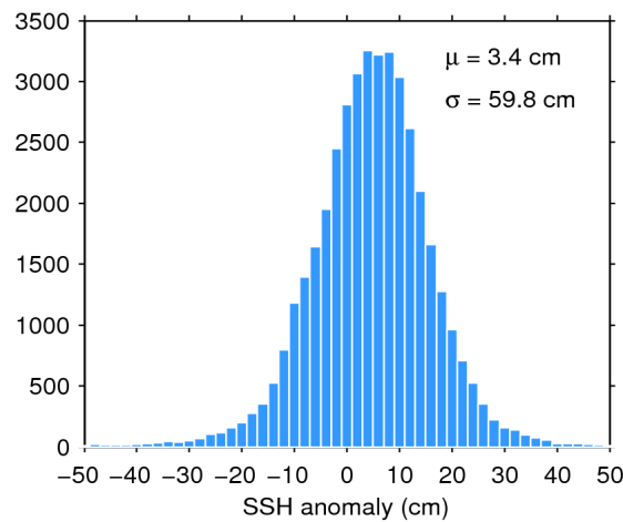
Figure 7. Histogram of flag-valid SSH anomaly over oceans and lakes for 25/07/2020. The mean ( \mu ) and standard deviation ( \sigma ) are also shown. Note that values outside [-50 50] cm are excluded from the histogram for the sake of readability but not from the computation of \mu and \sigma .
