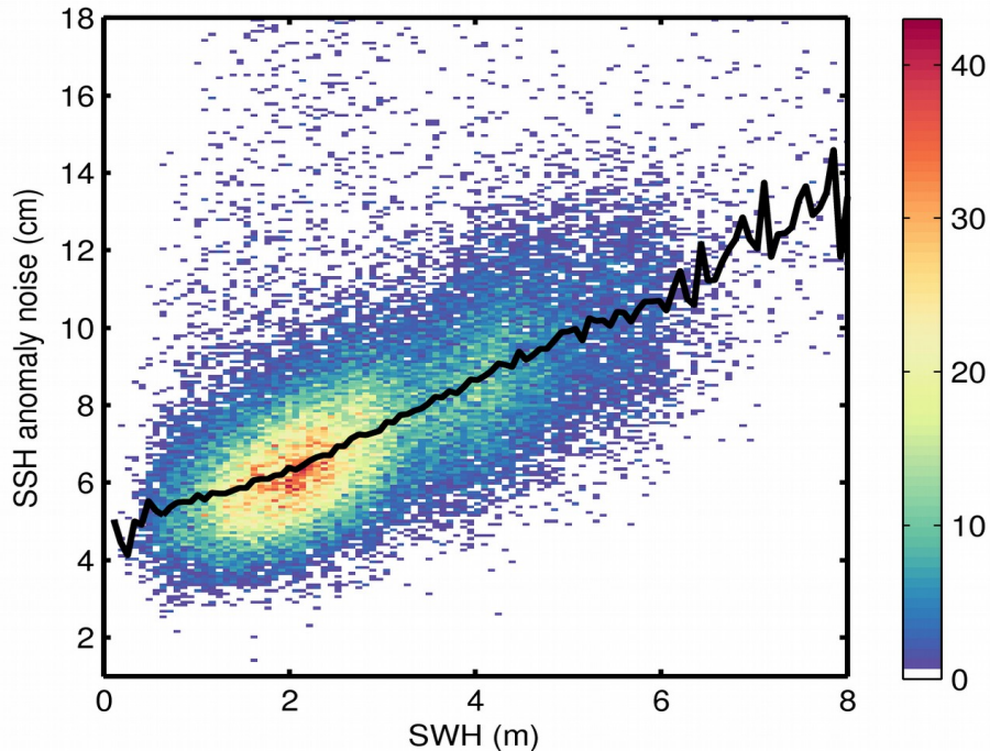
Figure 9. 2D histogram showing flag-valid SSH anomaly noise as a function of SWH for 25/07/2020. The black line denotes the median SSH anomaly noise as a function of SWH.
