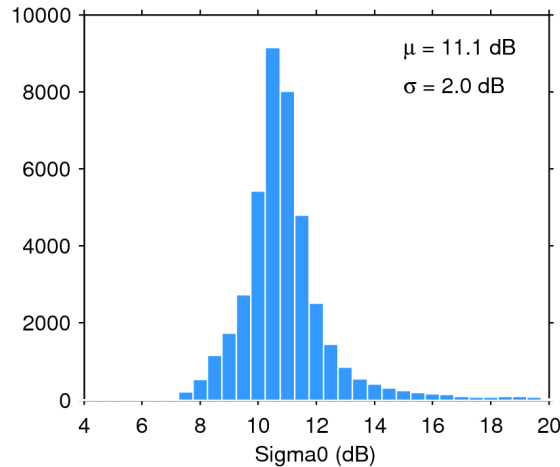
Figure 25. Histogram of flag-valid sigma0 over oceans and lakes for 25/07/2020. The mean ( \mu ) and standard deviation ( \sigma ) are also shown. Note that values outside [4 20] dB are excluded from the histogram for the sake of readability but not from the computation of \mu and \sigma .
