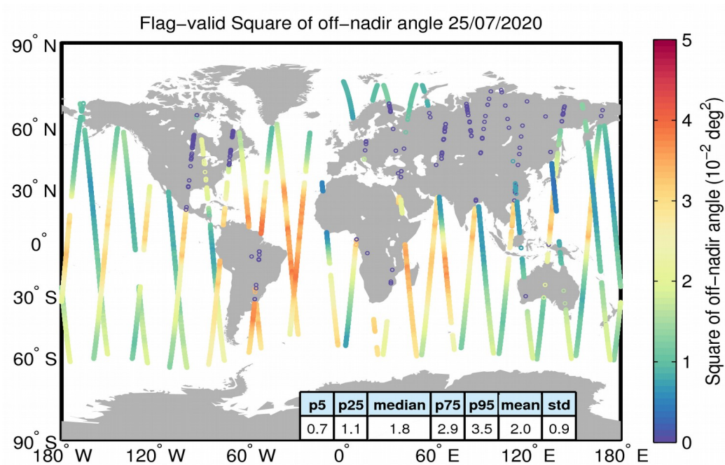
Figure 37. Geographical distribution of flag-valid mispointing data over oceans and lakes for 25/07/2020. The statistical values shown in the table refer to the mispointing in 10^{-2} \text{ deg}^2 and are calculated over all measurements shown in the figure.
