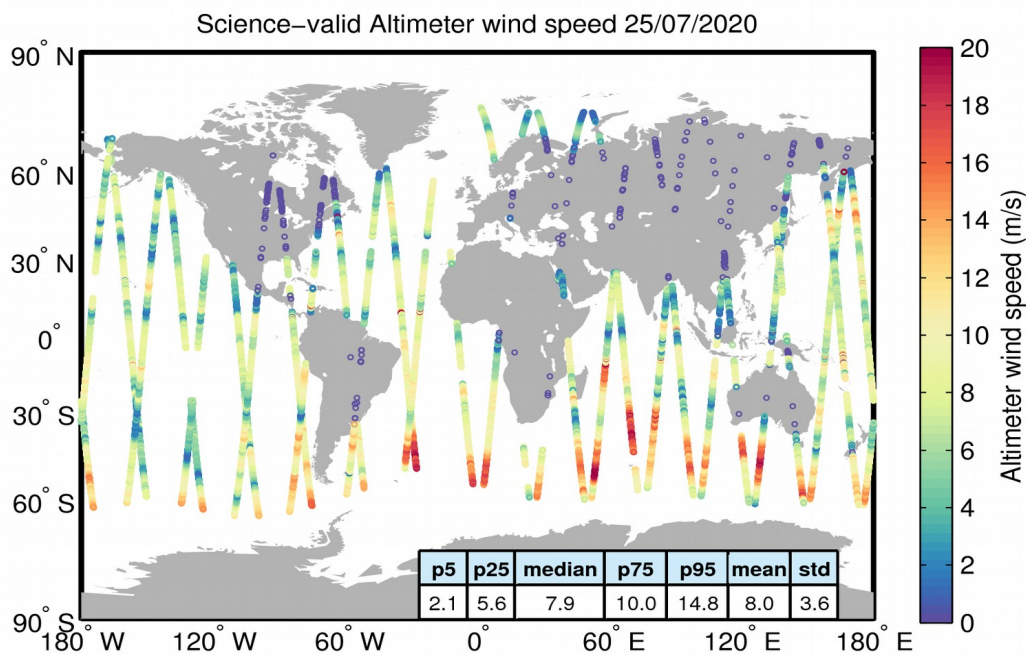
Figure 34. Geographical distribution of science-valid wind data over oceans and lakes for 25/07/2020. The statistical values shown in the table refer to the wind in m/s and are calculated over all measurements shown in the figure. Gray circles denote records that have been rejected based on the editing criteria described in Table 5.
