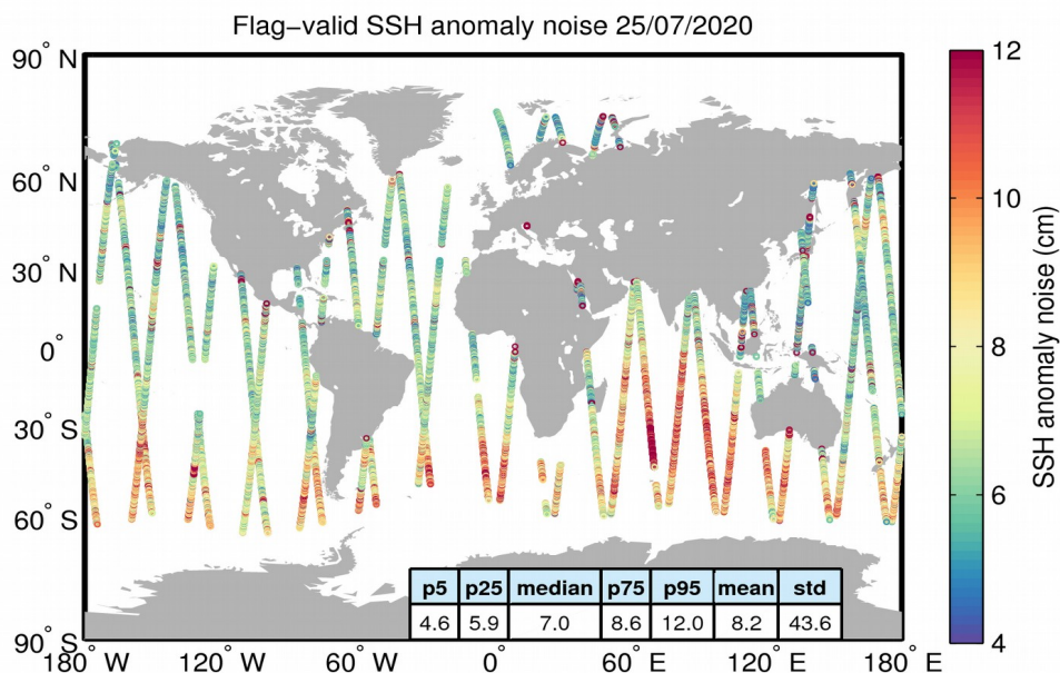
Figure 8. Geographical distribution of flag-valid 20-Hz SSH anomaly measurement noise over oceans and lakes for 25/07/2020. The statistical values shown in the table refer to the SSH anomaly noise and are calculated over all measurements shown in the figure.
