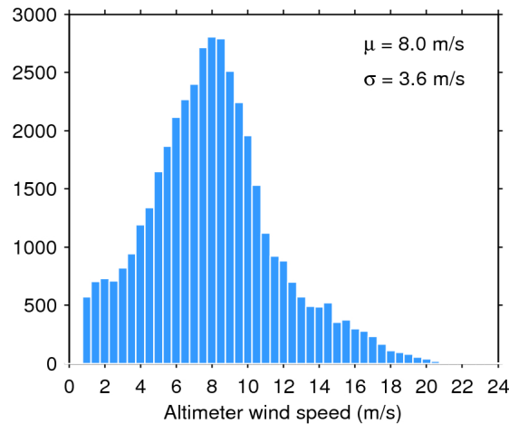
Figure 33. Histogram of flag-valid wind over oceans and lakes for 25/07/2020. The mean ( \mu ) and standard deviation ( \sigma ) are also shown. Note that values larger than 24 m/s are excluded from the histogram for the sake of readability but not from the computation of \mu and \sigma .
