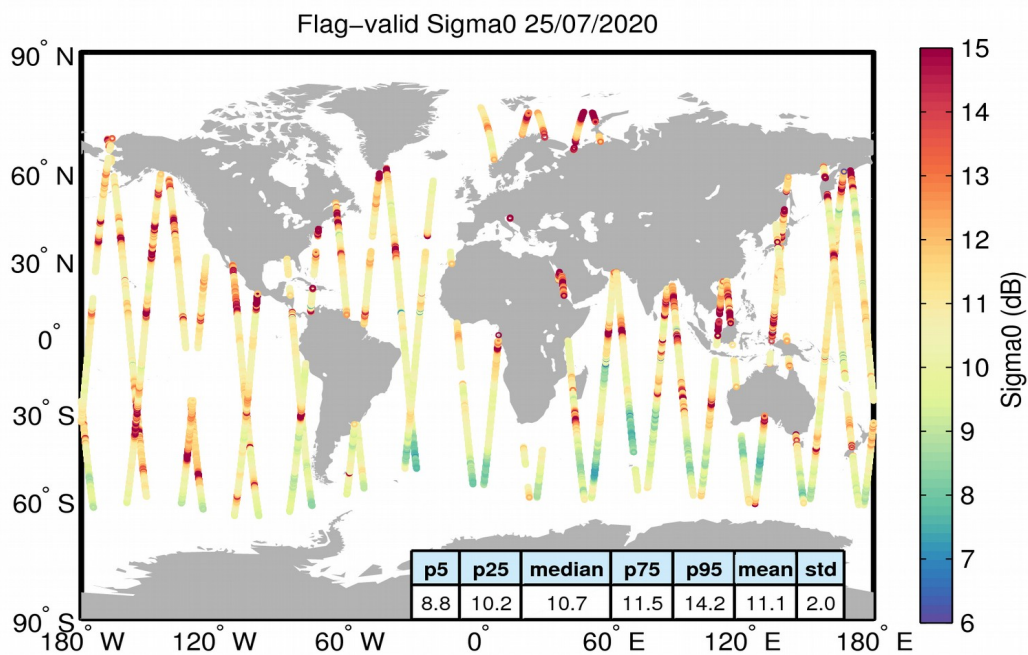
Figure 23. Geographical distribution of flag-valid sigma0 data over oceans and lakes for 25/07/2020. The statistical values shown in the table refer to the sigma0 in dB and are calculated over all measurements shown in the figure.
