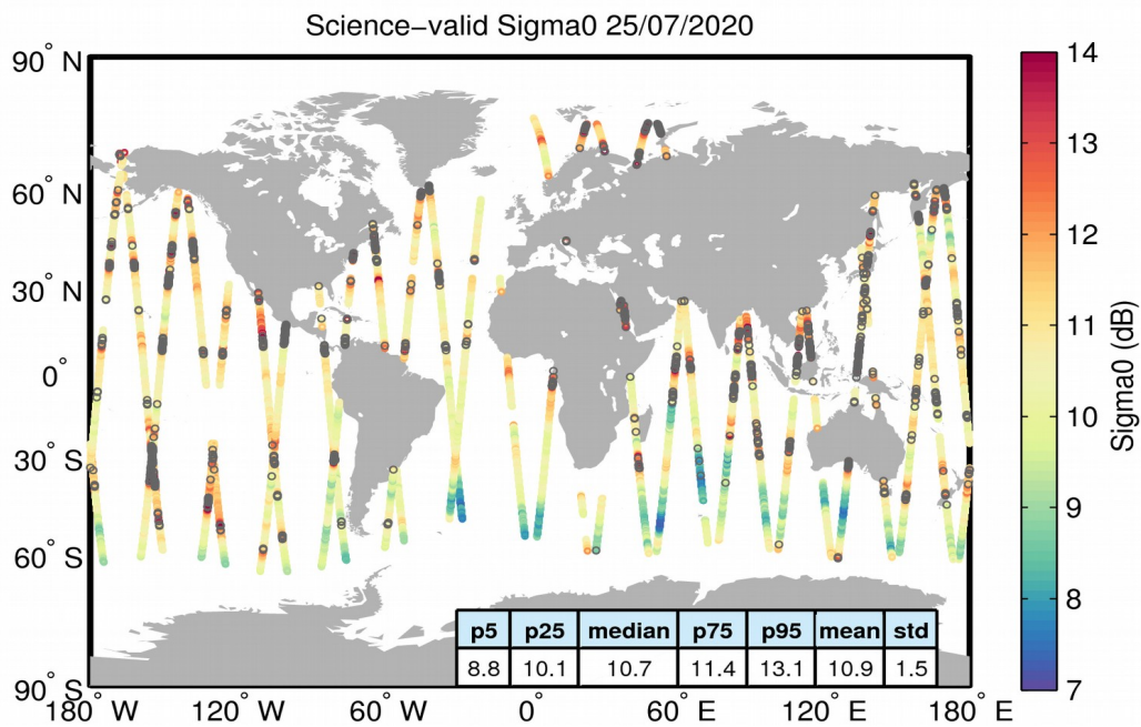
Figure 27. Geographical distribution of science-valid sigma0 data over oceans and lakes for 25/07/2020. The statistical values shown in the table refer to the sigma0 in dB and are calculated over all measurements shown in the figure. Gray circles denote records that have been rejected based on the editing criteria described in Table 4.
