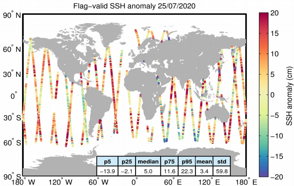
Figure 5. Geographical distribution of flag-valid 1-Hz SSH anomaly data over oceans and lakes for 25/07/2020. The statistical values shown in the table refer to the SSH anomaly in cm and are calculated over all measurements shown in the figure.
