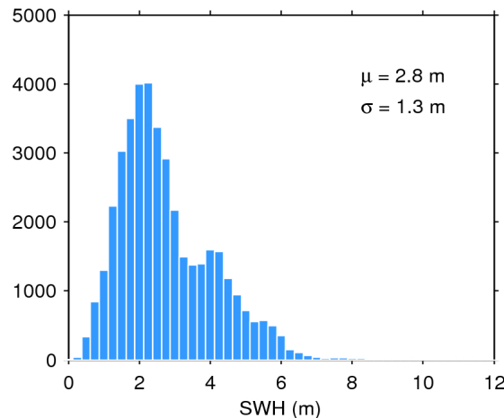
Figure 20. Histogram of science-valid SWH over oceans and lakes for 25/07/2020. The mean ( \mu ) and standard deviation ( \sigma ) are also shown. Note that values larger than 12 m are excluded from the histogram for the sake of readability but not from the computation of \mu and \sigma .
