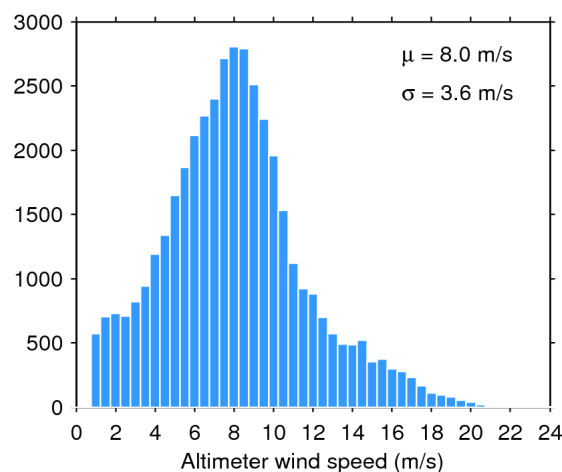
Figure 35. Histogram of science-valid wind over oceans and lakes for 25/07/2020. The mean ( \mu ) and standard deviation ( \sigma ) are also shown. Note that values larger than 24 m/s are excluded from the histogram for the sake of readability but not from the computation of \mu and \sigma .
