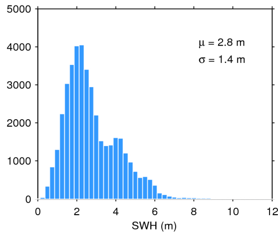
Figure 17. Histogram of flag-valid SWH over oceans and lakes for 25/07/2020. The mean ( \mu ) and standard deviation ( \sigma ) are also shown. Note that values larger than 12 m are excluded from the histogram for the sake of readability but not from the computation of \mu and \sigma .
