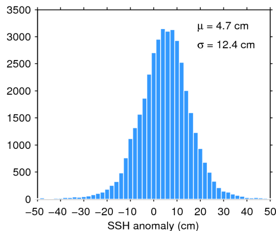
Figure 11. Histogram of science-valid SSH anomaly over oceans and lakes for 25/07/2020. The mean ( \mu ) and standard deviation ( \sigma ) are also shown. Note that values outside [-50 50] cm are excluded from the histogram for the sake of readability but not from the computation of \mu and \sigma .
