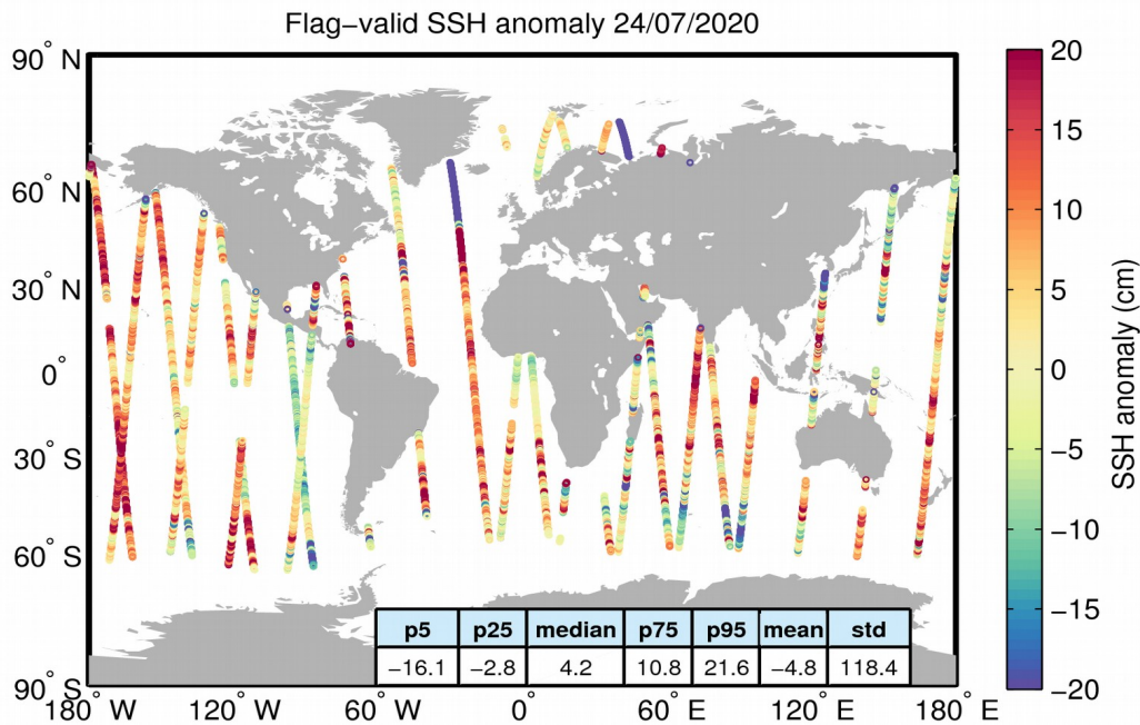
Figure 5. Geographical distribution of flag-valid 1-Hz SSH anomaly data over oceans and lakes for 24/07/2020. The statistical values shown in the table refer to the SSH anomaly in cm and are calculated over all measurements shown in the figure.
