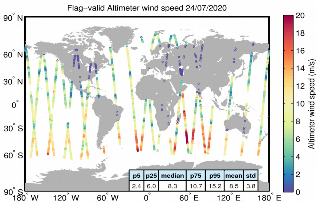
Figure 31. Geographical distribution of flag-valid wind data over oceans and lakes for 24/07/2020. The statistical values shown in the table refer to the wind in m/s and are calculated over all measurements shown in the figure.
