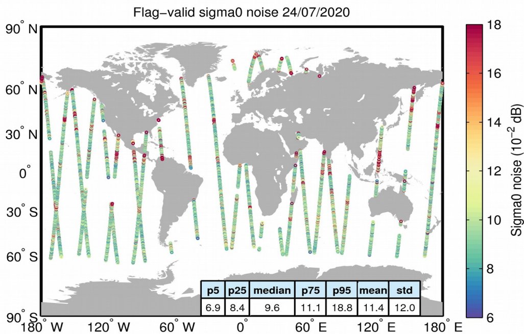
Figure 26. Geographical distribution of flag-valid 20-Hz sigma0 measurement noise over oceans and lakes for 24/07/2020. The statistical values shown in the table refer to the sigma0 noise and are calculated over all measurements shown in the figure.
