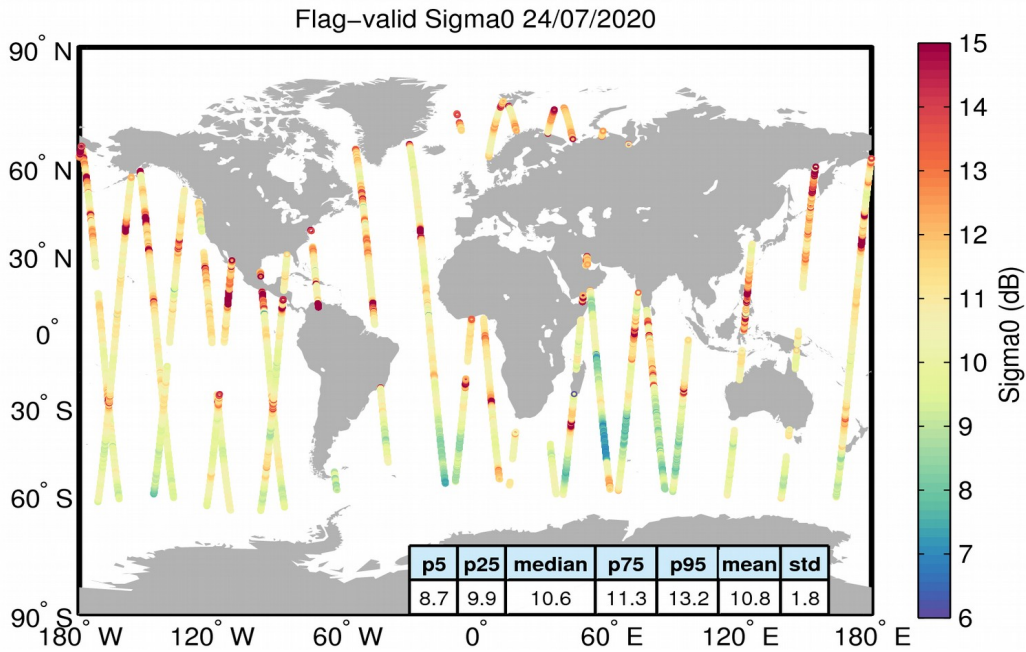
Figure 23. Geographical distribution of flag-valid sigma0 data over oceans and lakes for 24/07/2020. The statistical values shown in the table refer to the sigma0 in dB and are calculated over all measurements shown in the figure.
