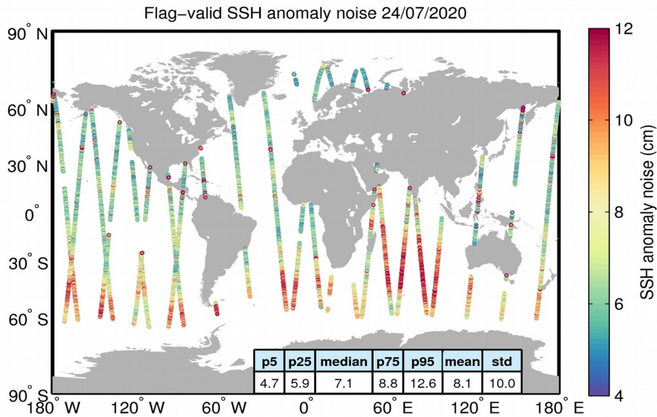
Figure 8. Geographical distribution of flag-valid 20-Hz SSH anomaly measurement noise over oceans and lakes for 24/07/2020. The statistical values shown in the table refer to the SSH anomaly noise and are calculated over all measurements shown in the figure.
