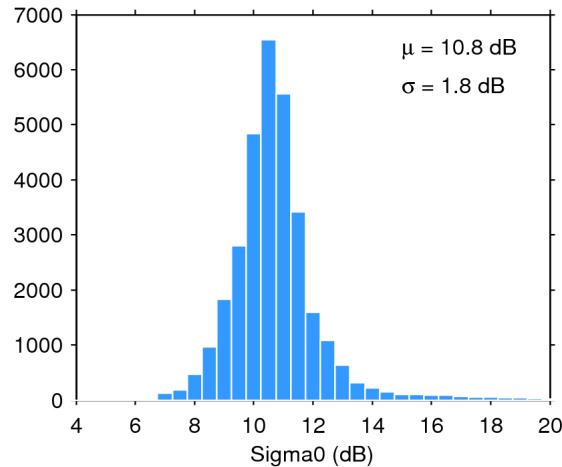
Figure 25. Histogram of flag-valid sigma0 over oceans and lakes for 24/07/2020. The mean ( \mu ) and standard deviation ( \sigma ) are also shown. Note that values outside [4 20] dB are excluded from the histogram for the sake of readability but not from the computation of \mu and \sigma .
