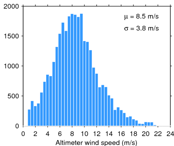
Figure 35. Histogram of science-valid wind over oceans and lakes for 24/07/2020. The mean ( \mu ) and standard deviation ( \sigma ) are also shown. Note that values larger than 24 m/s are excluded from the histogram for the sake of readability but not from the computation of \mu and \sigma .
