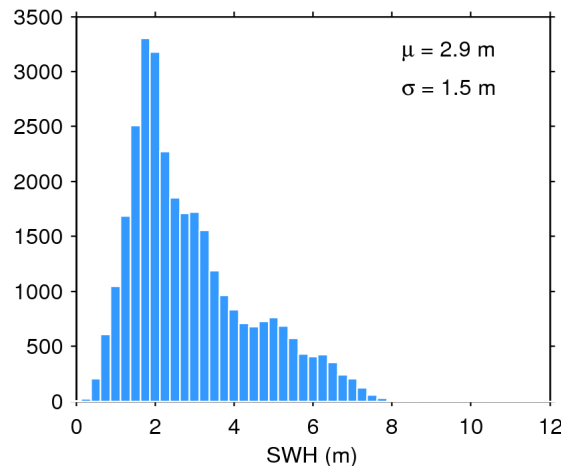
Figure 20. Histogram of science-valid SWH over oceans and lakes for 24/07/2020. The mean ( \mu ) and standard deviation ( \sigma ) are also shown. Note that values larger than 12 m are excluded from the histogram for the sake of readability but not from the computation of \mu and \sigma .
