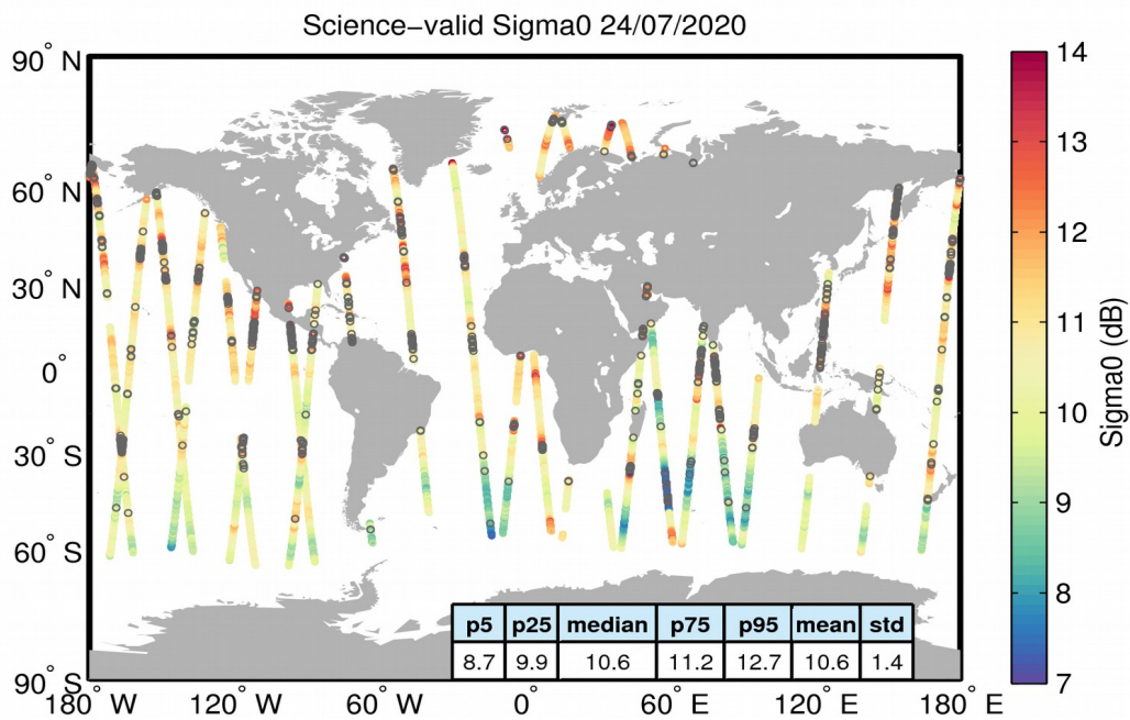
Figure 27. Geographical distribution of science-valid sigma0 data over oceans and lakes for 24/07/2020. The statistical values shown in the table refer to the sigma0 in dB and are calculated over all measurements shown in the figure. Gray circles denote records that have been rejected based on the editing criteria described in Table 4.
