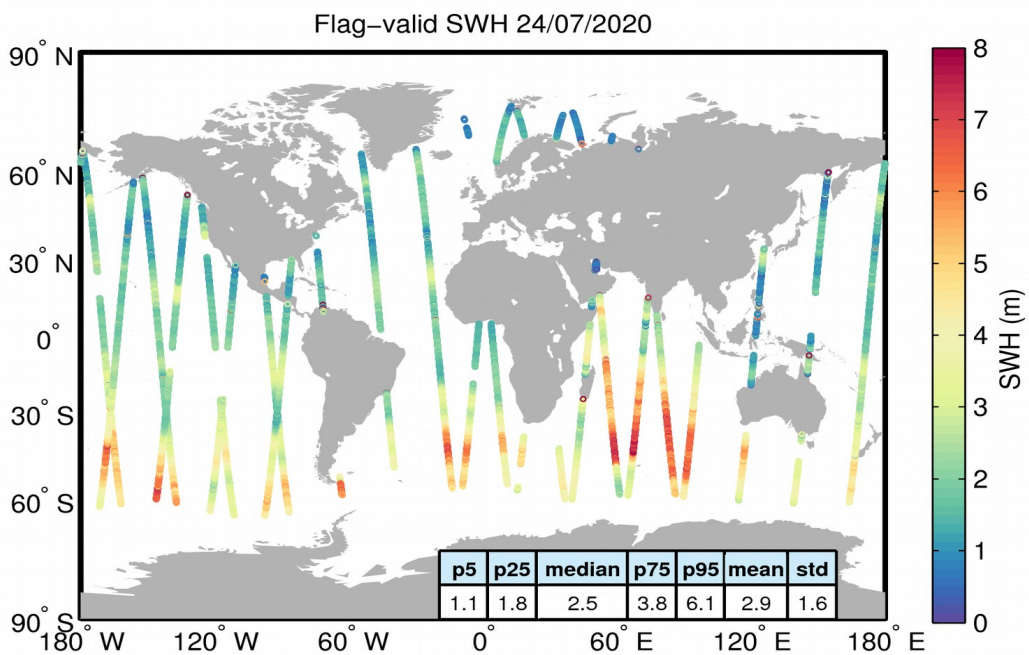
Figure 15. Geographical distribution of flag-valid SWH data over oceans and lakes for 24/07/2020. The statistical values shown in the table refer to the SWH in m and are calculated over all measurements shown in the figure.
