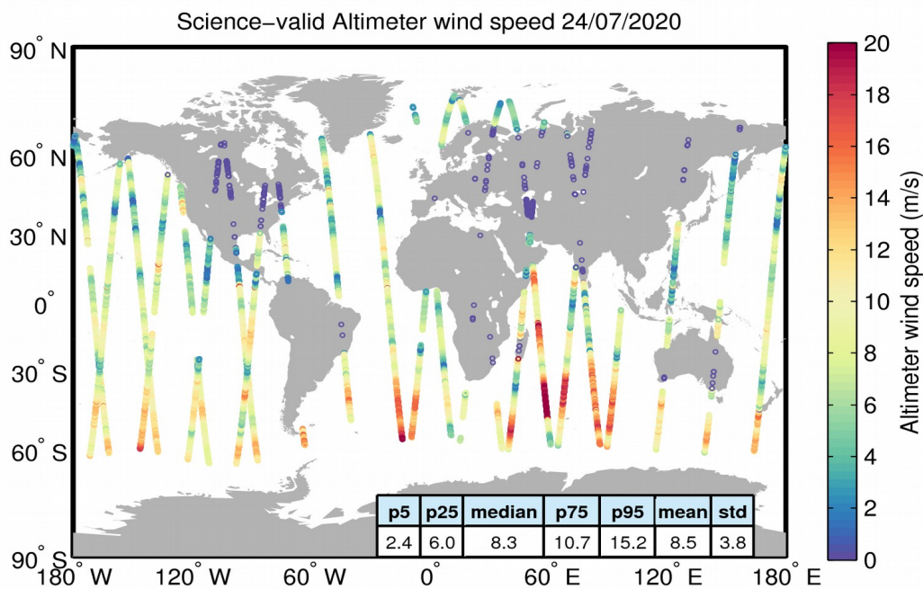
Figure 34. Geographical distribution of science-valid wind data over oceans and lakes for 24/07/2020. The statistical values shown in the table refer to the wind in m/s and are calculated over all measurements shown in the figure. Gray circles denote records that have been rejected based on the editing criteria described in Table 5.
