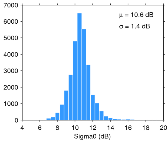
Figure 28. Histogram of science-valid sigma0 over oceans and lakes for 24/07/2020. The mean ( \mu ) and standard deviation ( \sigma ) are also shown. Note that values outside [4 20] dB are excluded from the histogram for the sake of readability but not from the computation of \mu and \sigma .
