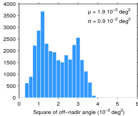
Figure 39. Histogram of flag-valid mispointing over oceans and lakes for 24/07/2020. The mean ( \mu ) and standard deviation ( \sigma ) are also shown. Note that values larger than 6 \cdot 10^{-2} \text{ deg}^2 are excluded from the histogram for the sake of readability but not from the computation of \mu and \sigma .
