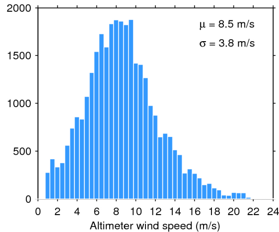
Figure 33. Histogram of flag-valid wind over oceans and lakes for 24/07/2020. The mean ( \mu ) and standard deviation ( \sigma ) are also shown. Note that values larger than 24 m/s are excluded from the histogram for the sake of readability but not from the computation of \mu and \sigma .
