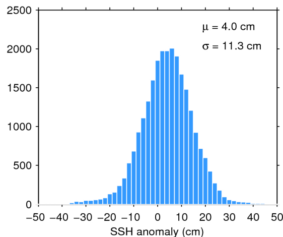
Figure 11. Histogram of science-valid SSH anomaly over oceans and lakes for 24/07/2020. The mean ( \mu ) and standard deviation ( \sigma ) are also shown. Note that values outside [-50 50] cm are excluded from the histogram for the sake of readability but not from the computation of \mu and \sigma .
