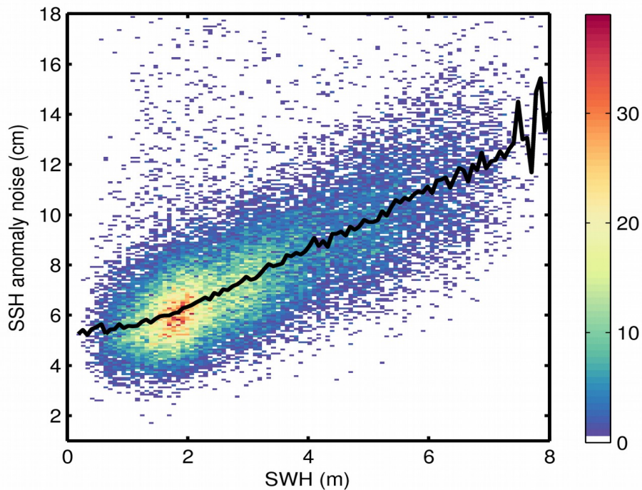
Figure 9. 2D histogram showing flag-valid SSH anomaly noise as a function of SWH for 24/07/2020. The black line denotes the median SSH anomaly noise as a function of SWH.
