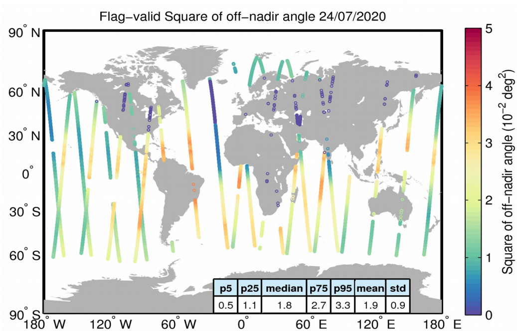
Figure 37. Geographical distribution of flag-valid mispointing data over oceans and lakes for 24/07/2020. The statistical values shown in the table refer to the mispointing in 10^{-2} \text{ deg}^2 and are calculated over all measurements shown in the figure.
