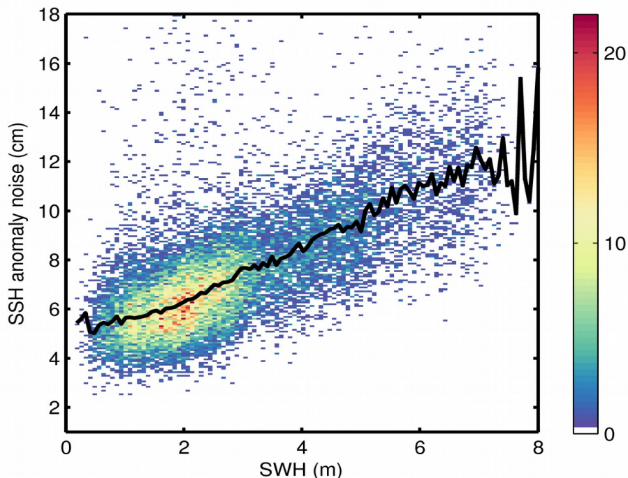
Figure 9. 2D histogram showing flag-valid SSH anomaly noise as a function of SWH for 23/07/2020. The black line denotes the median SSH anomaly noise as a function of SWH.
