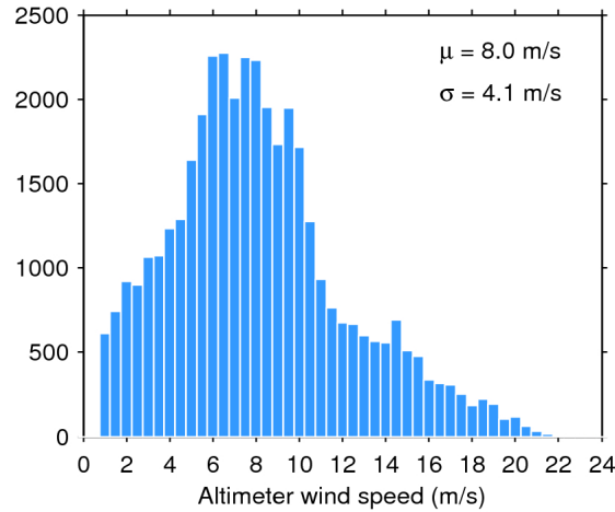
Figure 33. Histogram of flag-valid wind over oceans and lakes for 22/07/2020. The mean ( \mu ) and standard deviation ( \sigma ) are also shown. Note that values larger than 24 m/s are excluded from the histogram for the sake of readability but not from the computation of \mu and \sigma .
