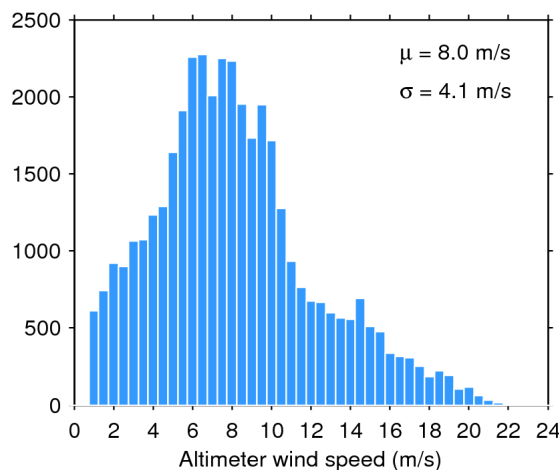
Figure 35. Histogram of science-valid wind over oceans and lakes for 22/07/2020. The mean ( \mu ) and standard deviation ( \sigma ) are also shown. Note that values larger than 24 m/s are excluded from the histogram for the sake of readability but not from the computation of \mu and \sigma .
