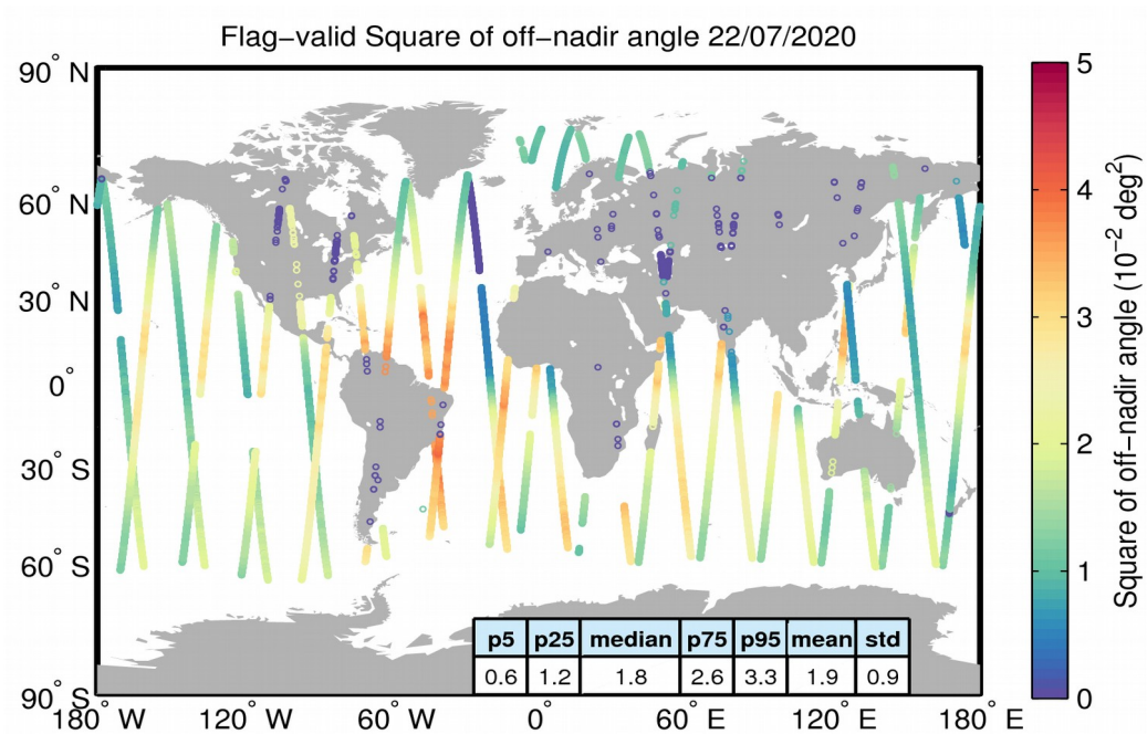
Figure 37. Geographical distribution of flag-valid mispointing data over oceans and lakes for 22/07/2020. The statistical values shown in the table refer to the mispointing in 10^{-2} deg 2 and are calculated over all measurements shown in the figure.
