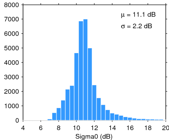
Figure 25. Histogram of flag-valid sigma0 over oceans and lakes for 22/07/2020. The mean ( \mu ) and standard deviation ( \sigma ) are also shown. Note that values outside [4 20] dB are excluded from the histogram for the sake of readability but not from the computation of \mu and \sigma .
