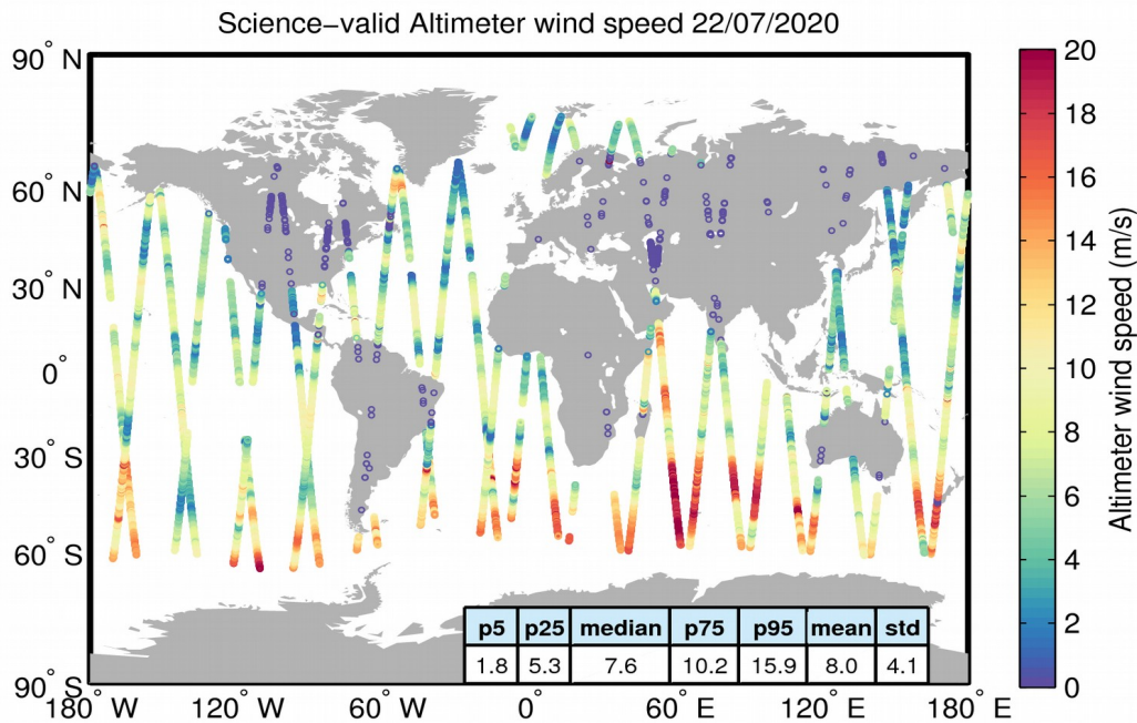
Figure 34. Geographical distribution of science-valid wind data over oceans and lakes for 22/07/2020. The statistical values shown in the table refer to the wind in m/s and are calculated over all measurements shown in the figure. Gray circles denote records that have been rejected based on the editing criteria described in Table 5.
