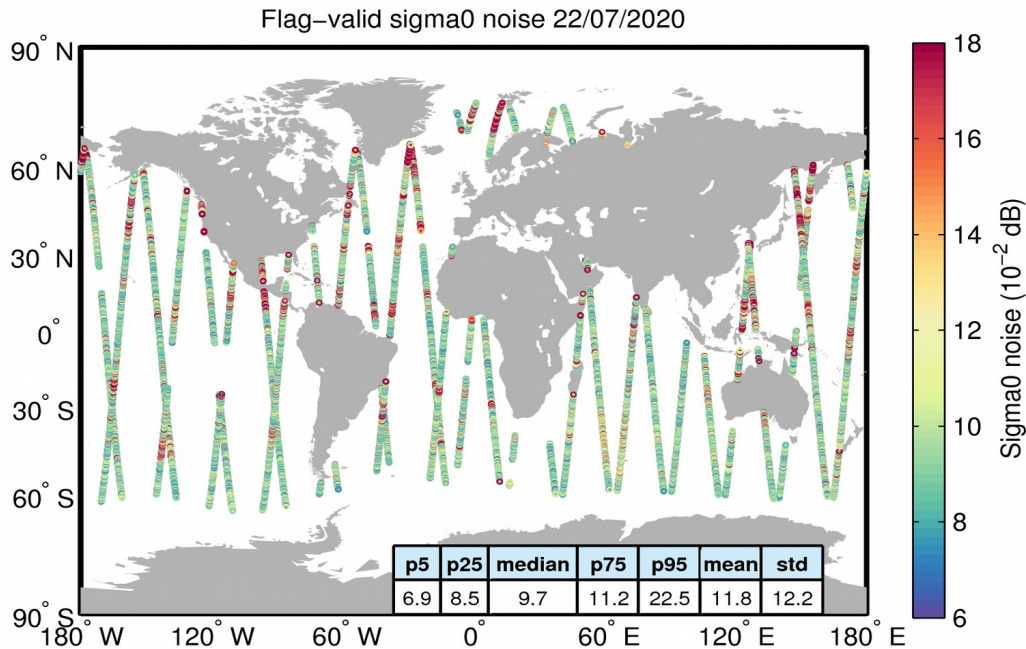
Figure 26. Geographical distribution of flag-valid 20-Hz sigma0 measurement noise over oceans and lakes for 22/07/2020. The statistical values shown in the table refer to the sigma0 noise and are calculated over all measurements shown in the figure.
