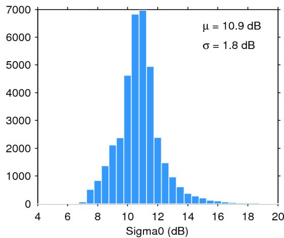
Figure 28. Histogram of science-valid sigma0 over oceans and lakes for 22/07/2020. The mean ( \mu ) and standard deviation ( \sigma ) are also shown. Note that values outside [4 20] dB are excluded from the histogram for the sake of readability but not from the computation of \mu and \sigma .
