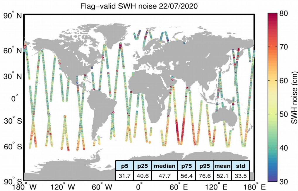
Figure 18. Geographical distribution of flag-valid 20-Hz SWH measurement noise over oceans and lakes for 22/07/2020. The statistical values shown in the figure refer to the SWH noise and are calculated over all measurements shown in the figure.
