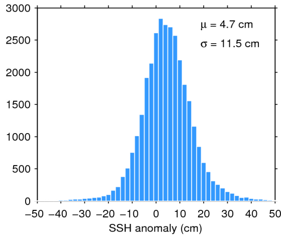
Figure 11. Histogram of science-valid SSH anomaly over oceans and lakes for 22/07/2020. The mean ( \mu ) and standard deviation ( \sigma ) are also shown. Note that values outside [-50 50] cm are excluded from the histogram for the sake of readability but not from the computation of \mu and \sigma .
