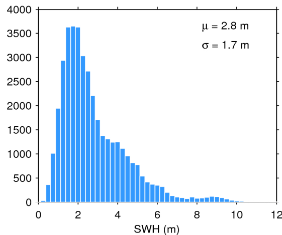
Figure 17. Histogram of flag-valid SWH over oceans and lakes for 22/07/2020. The mean ( \mu ) and standard deviation ( \sigma ) are also shown. Note that values larger than 12 m are excluded from the histogram for the sake of readability but not from the computation of \mu and \sigma .
