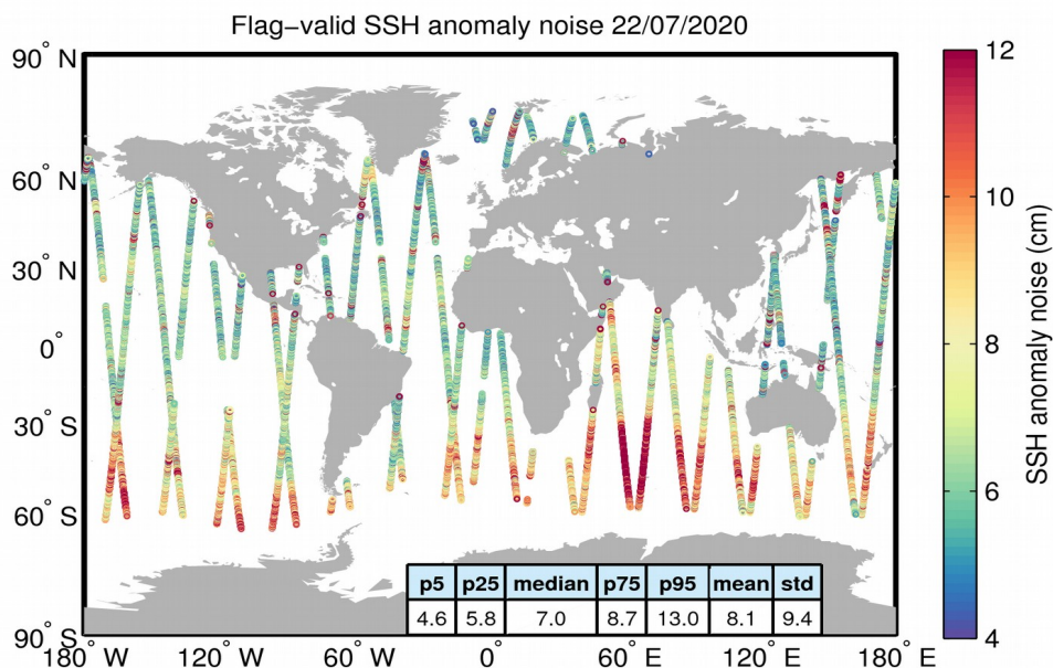
Figure 8. Geographical distribution of flag-valid 20-Hz SSH anomaly measurement noise over oceans and lakes for 22/07/2020. The statistical values shown in the table refer to the SSH anomaly noise and are calculated over all measurements shown in the figure.
