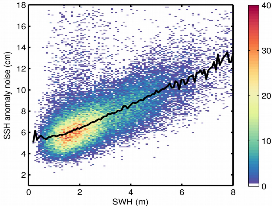
Figure 9. 2D histogram showing flag-valid SSH anomaly noise as a function of SWH for 22/07/2020. The black line denotes the median SSH anomaly noise as a function of SWH.
