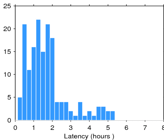
Figure 2. Histogram of the data latency for 22/07/2020. The y-axis denotes the number of files that are made available with a delay of x-hours with respect to the mean time of the records stored in the file.
