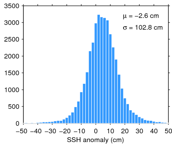
Figure 7. Histogram of flag-valid SSH anomaly over oceans and lakes for 22/07/2020. The mean ( \mu ) and standard deviation ( \sigma ) are also shown. Note that values outside [-50 50] cm are excluded from the histogram for the sake of readability but not from the computation of \mu and \sigma .
