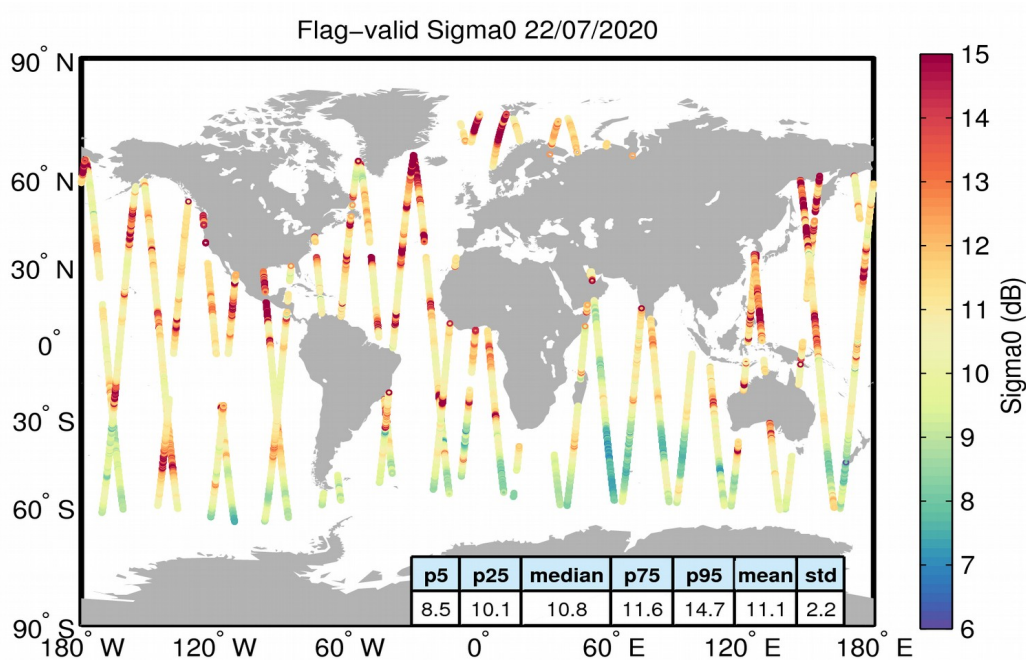
Figure 23. Geographical distribution of flag-valid sigma0 data over oceans and lakes for 22/07/2020. The statistical values shown in the table refer to the sigma0 in dB and are calculated over all measurements shown in the figure.
