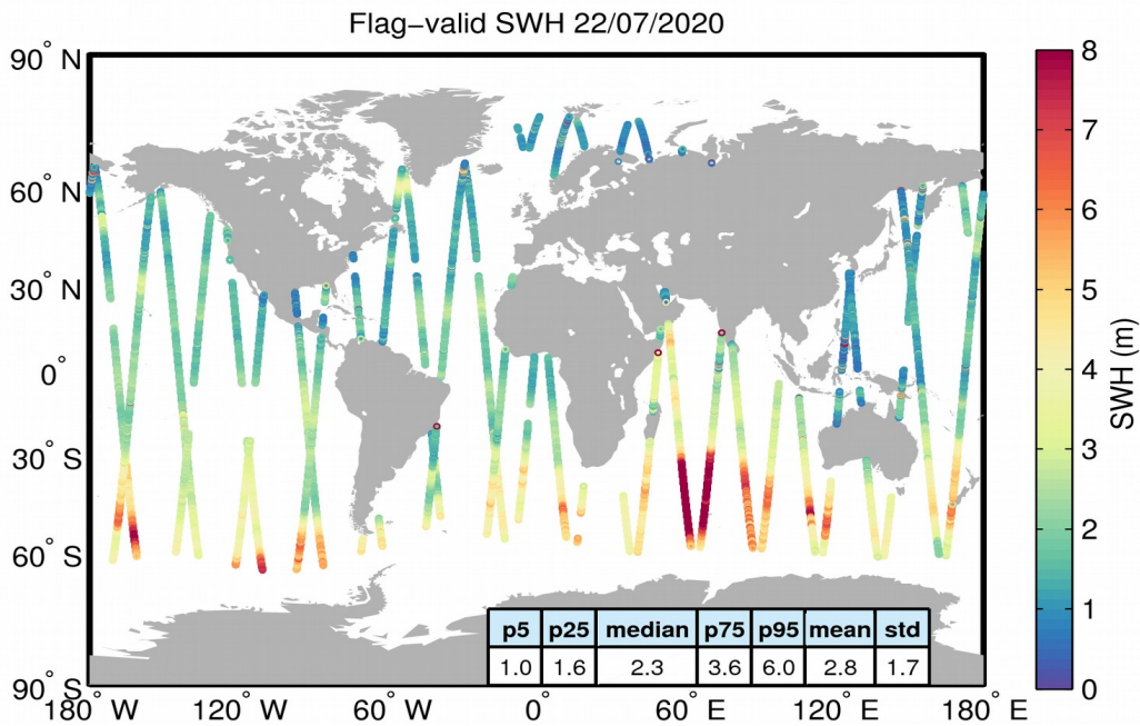
Figure 15. Geographical distribution of flag-valid SWH data over oceans and lakes for 22/07/2020. The statistical values shown in the table refer to the SWH in m and are calculated over all measurements shown in the figure.
