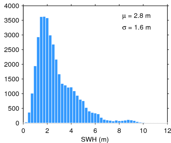
Figure 20. Histogram of science-valid SWH over oceans and lakes for 22/07/2020. The mean ( \mu ) and standard deviation ( \sigma ) are also shown. Note that values larger than 12 m are excluded from the histogram for the sake of readability but not from the computation of \mu and \sigma .
