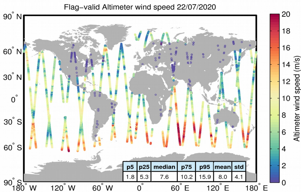
Figure 31. Geographical distribution of flag-valid wind data over oceans and lakes for 22/07/2020. The statistical values shown in the table refer to the wind in m/s and are calculated over all measurements shown in the figure.
