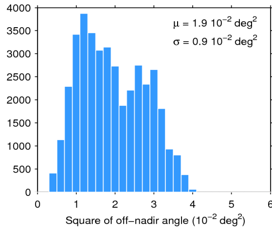
Figure 39. Histogram of flag-valid mispointing over oceans and lakes for 22/07/2020. The mean ( \mu ) and standard deviation ( \sigma ) are also shown. Note that values larger than 6 \cdot 10^{-2} \text{ deg}^2 are excluded from the histogram for the sake of readability but not from the computation of \mu and \sigma .
