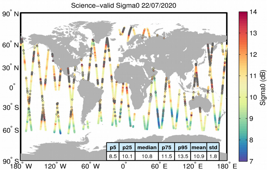
Figure 27. Geographical distribution of science-valid sigma0 data over oceans and lakes for 22/07/2020. The statistical values shown in the table refer to the sigma0 in dB and are calculated over all measurements shown in the figure. Gray circles denote records that have been rejected based on the editing criteria described in Table 4.
