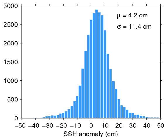
Figure 11. Histogram of science-valid SSH anomaly over oceans and lakes for 21/07/2020. The mean ( \mu ) and standard deviation ( \sigma ) are also shown. Note that values outside [-50 50] cm are excluded from the histogram for the sake of readability but not from the computation of \mu and \sigma .
