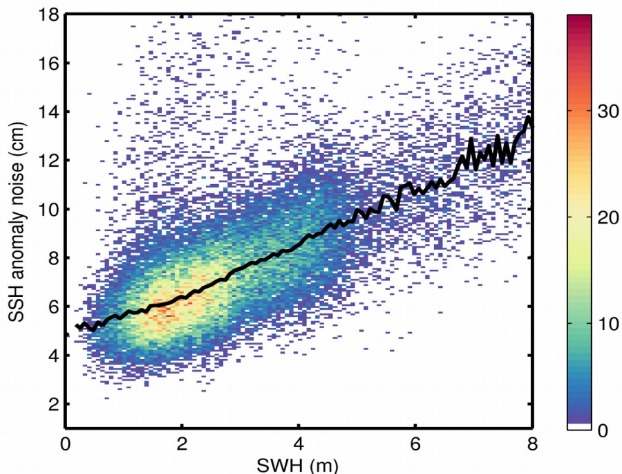
Figure 9. 2D histogram showing flag-valid SSH anomaly noise as a function of SWH for 21/07/2020. The black line denotes the median SSH anomaly noise as a function of SWH.
