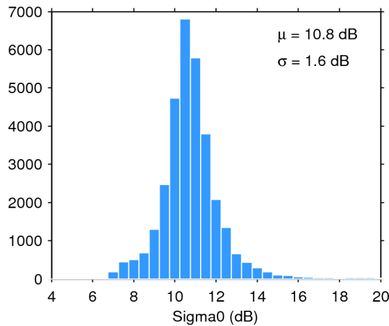
Figure 28. Histogram of science-valid sigma0 over oceans and lakes for 21/07/2020. The mean ( \mu ) and standard deviation ( \sigma ) are also shown. Note that values outside [4 20] dB are excluded from the histogram for the sake of readability but not from the computation of \mu and \sigma .
