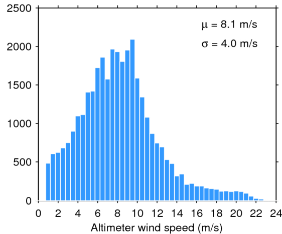
Figure 33. Histogram of flag-valid wind over oceans and lakes for 21/07/2020. The mean ( \mu ) and standard deviation ( \sigma ) are also shown. Note that values larger than 24 m/s are excluded from the histogram for the sake of readability but not from the computation of \mu and \sigma .
