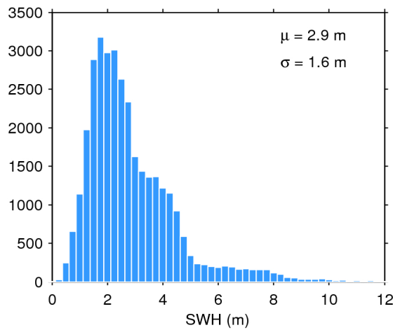
Figure 17. Histogram of flag-valid SWH over oceans and lakes for 21/07/2020. The mean ( \mu ) and standard deviation ( \sigma ) are also shown. Note that values larger than 12 m are excluded from the histogram for the sake of readability but not from the computation of \mu and \sigma .
