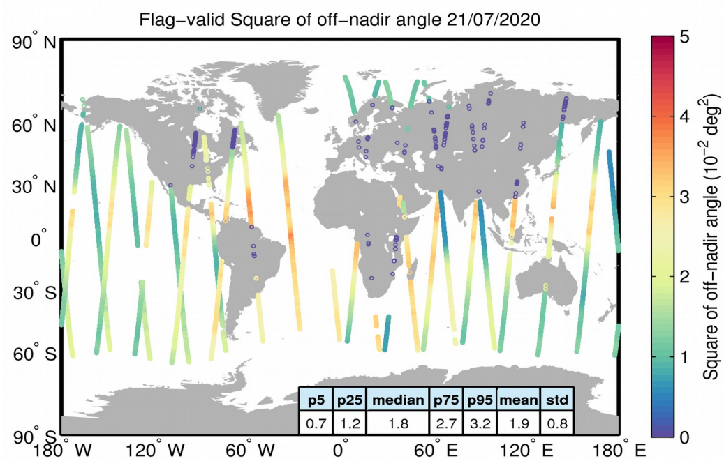
Figure 37. Geographical distribution of flag-valid mispointing data over oceans and lakes for 21/07/2020. The statistical values shown in the table refer to the mispointing in 10^{-2} \text{ deg}^2 and are calculated over all measurements shown in the figure.
