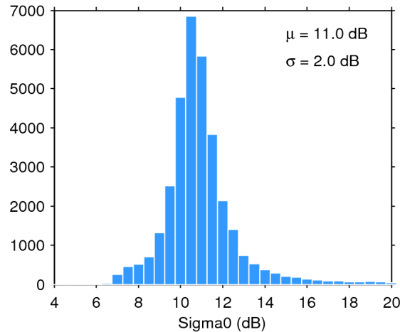
Figure 25. Histogram of flag-valid sigma0 over oceans and lakes for 21/07/2020. The mean ( \mu ) and standard deviation ( \sigma ) are also shown. Note that values outside [4 20] dB are excluded from the histogram for the sake of readability but not from the computation of \mu and \sigma .
