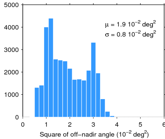
Figure 39. Histogram of flag-valid mispointing over oceans and lakes for 21/07/2020. The mean ( \mu ) and standard deviation ( \sigma ) are also shown. Note that values larger than 6 \cdot 10^{-2} \text{ deg}^2 are excluded from the histogram for the sake of readability but not from the computation of \mu and \sigma .
