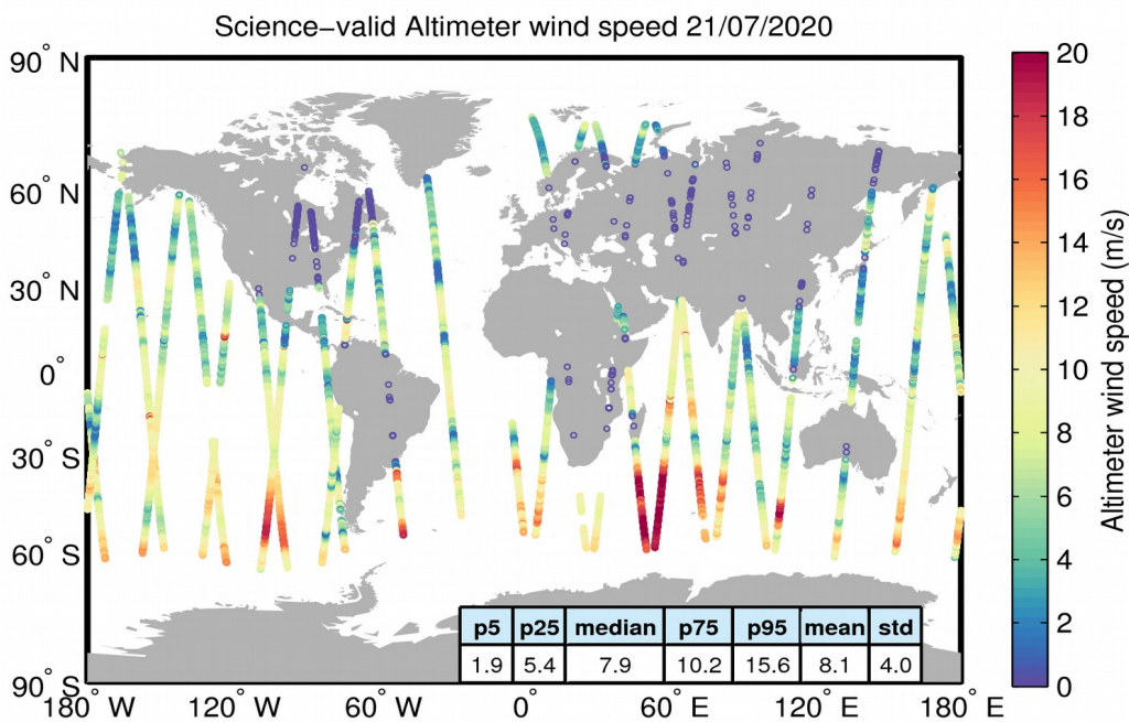
Figure 34. Geographical distribution of science-valid wind data over oceans and lakes for 21/07/2020. The statistical values shown in the table refer to the wind in m/s and are calculated over all measurements shown in the figure. Gray circles denote records that have been rejected based on the editing criteria described in Table 5.
