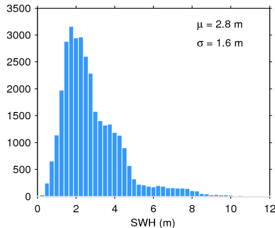
Figure 20. Histogram of science-valid SWH over oceans and lakes for 21/07/2020. The mean ( \mu ) and standard deviation ( \sigma ) are also shown. Note that values larger than 12 m are excluded from the histogram for the sake of readability but not from the computation of \mu and \sigma .
