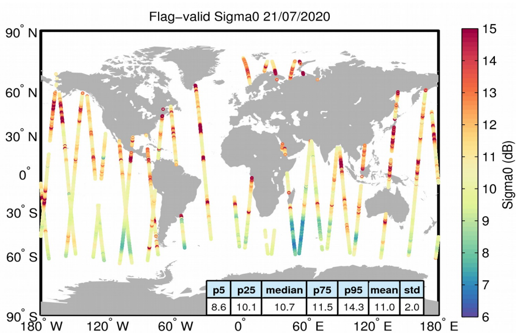
Figure 23. Geographical distribution of flag-valid sigma0 data over oceans and lakes for 21/07/2020. The statistical values shown in the table refer to the sigma0 in dB and are calculated over all measurements shown in the figure.
