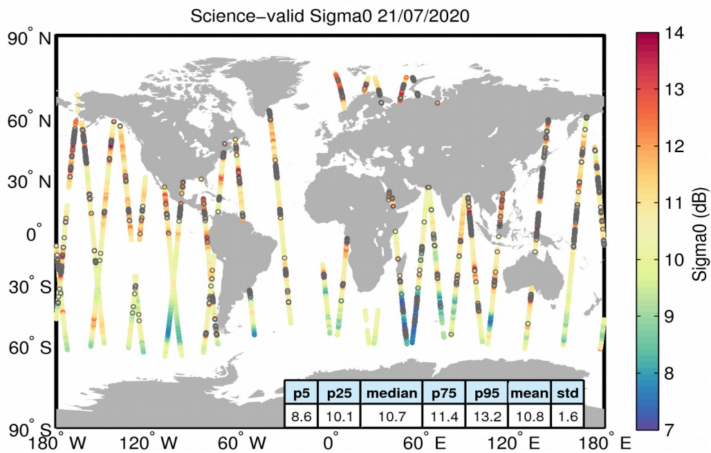
Figure 27. Geographical distribution of science-valid sigma0 data over oceans and lakes for 21/07/2020. The statistical values shown in the table refer to the sigma0 in dB and are calculated over all measurements shown in the figure. Gray circles denote records that have been rejected based on the editing criteria described in Table 4.
