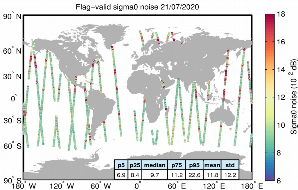
Figure 26. Geographical distribution of flag-valid 20-Hz sigma0 measurement noise over oceans and lakes for 21/07/2020. The statistical values shown in the table refer to the sigma0 noise and are calculated over all measurements shown in the figure.
