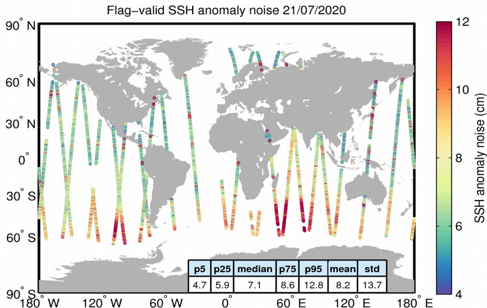
Figure 8. Geographical distribution of flag-valid 20-Hz SSH anomaly measurement noise over oceans and lakes for 21/07/2020. The statistical values shown in the table refer to the SSH anomaly noise and are calculated over all measurements shown in the figure.
