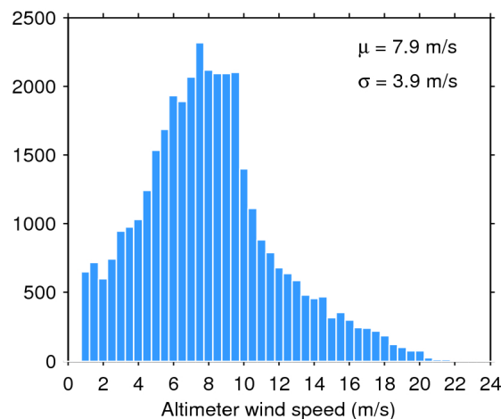
Figure 35. Histogram of science-valid wind over oceans and lakes for 20/07/2020. The mean ( \mu ) and standard deviation ( \sigma ) are also shown. Note that values larger than 24 m/s are excluded from the histogram for the sake of readability but not from the computation of \mu and \sigma .
