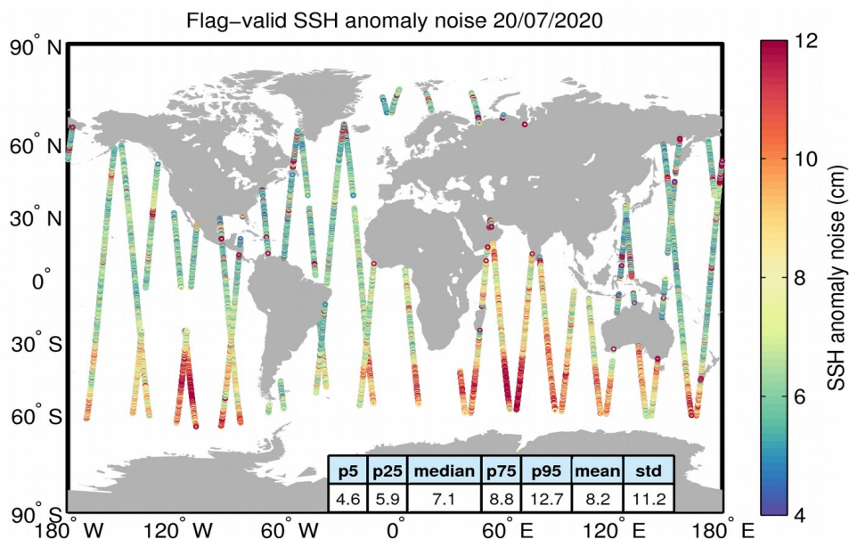
Figure 8. Geographical distribution of flag-valid 20-Hz SSH anomaly measurement noise over oceans and lakes for 20/07/2020. The statistical values shown in the table refer to the SSH anomaly noise and are calculated over all measurements shown in the figure.
