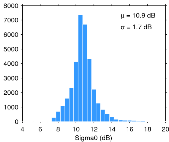
Figure 28. Histogram of science-valid sigma0 over oceans and lakes for 20/07/2020. The mean ( \mu ) and standard deviation ( \sigma ) are also shown. Note that values outside [4 20] dB are excluded from the histogram for the sake of readability but not from the computation of \mu and \sigma .
