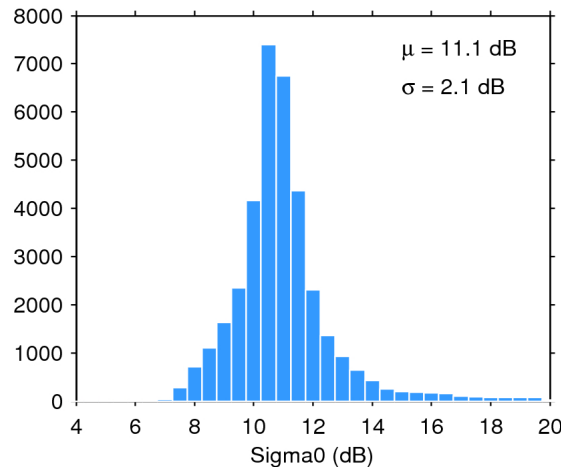
Figure 25. Histogram of flag-valid sigma0 over oceans and lakes for 20/07/2020. The mean ( \mu ) and standard deviation ( \sigma ) are also shown. Note that values outside [4 20] dB are excluded from the histogram for the sake of readability but not from the computation of \mu and \sigma .
