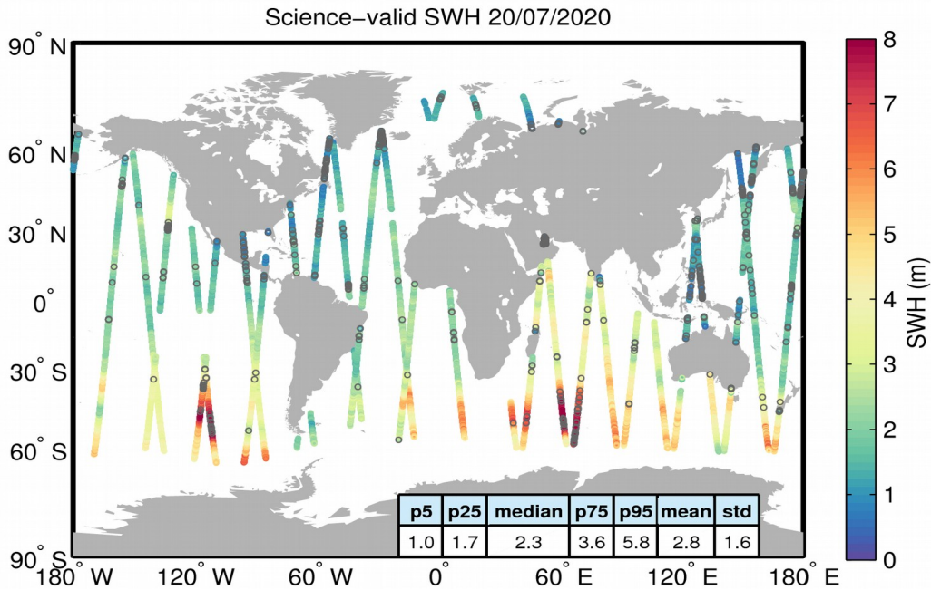
Figure 19. Geographical distribution of science-valid SWH data over oceans and lakes for 20/07/2020. The statistical values shown in the table refer to the SWH in m and are calculated over all measurements shown in the figure. Gray circles denote records that have been rejected based on the editing criteria described in Table 3.
