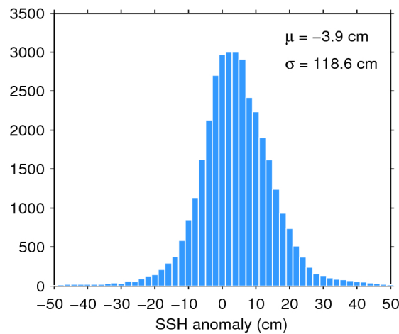
Figure 7. Histogram of flag-valid SSH anomaly over oceans and lakes for 20/07/2020. The mean ( \mu ) and standard deviation ( \sigma ) are also shown. Note that values outside [-50\ 50] cm are excluded from the histogram for the sake of readability but not from the computation of \mu and \sigma .
