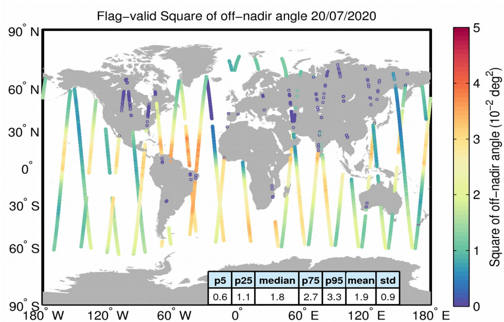
Figure 37. Geographical distribution of flag-valid mispointing data over oceans and lakes for 20/07/2020. The statistical values shown in the table refer to the mispointing in 10^{-2} \text{ deg}^2 and are calculated over all measurements shown in the figure.
