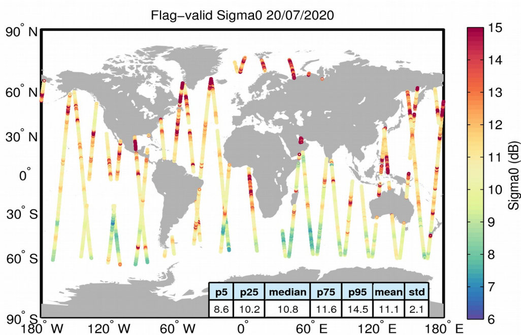
Figure 23. Geographical distribution of flag-valid sigma0 data over oceans and lakes for 20/07/2020. The statistical values shown in the table refer to the sigma0 in dB and are calculated over all measurements shown in the figure.
