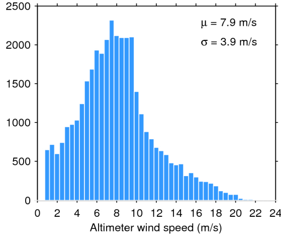
Figure 33. Histogram of flag-valid wind over oceans and lakes for 20/07/2020. The mean ( \mu ) and standard deviation ( \sigma ) are also shown. Note that values larger than 24 m/s are excluded from the histogram for the sake of readability but not from the computation of \mu and \sigma .
