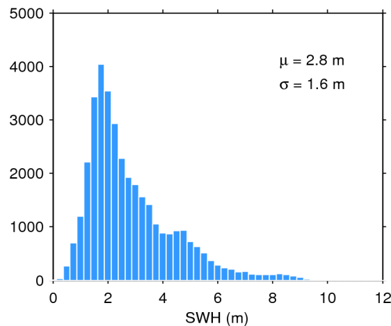
Figure 17. Histogram of flag-valid SWH over oceans and lakes for 20/07/2020. The mean ( \mu ) and standard deviation ( \sigma ) are also shown. Note that values larger than 12 m are excluded from the histogram for the sake of readability but not from the computation of \mu and \sigma .
