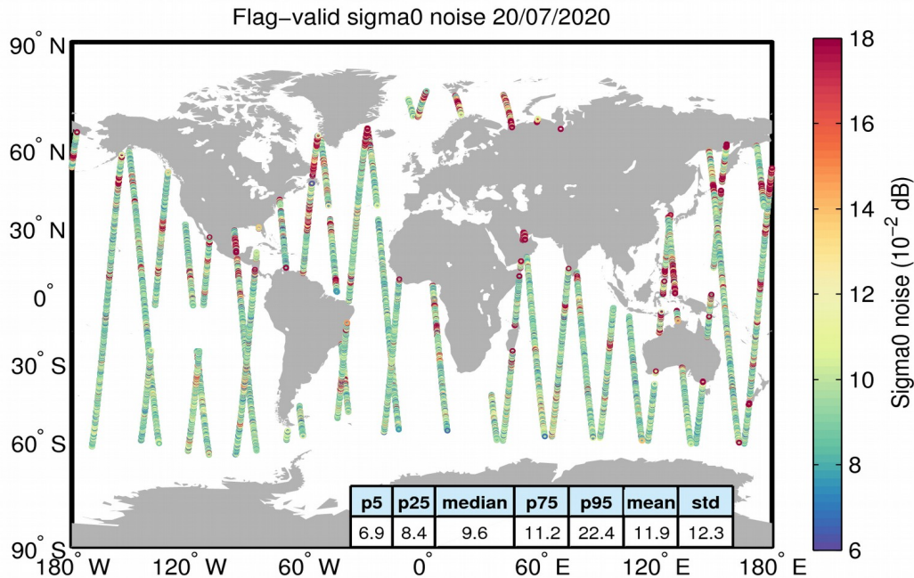
Figure 26. Geographical distribution of flag-valid 20-Hz sigma0 measurement noise over oceans and lakes for 20/07/2020. The statistical values shown in the table refer to the sigma0 noise and are calculated over all measurements shown in the figure.
