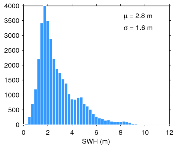
Figure 20. Histogram of science-valid SWH over oceans and lakes for 20/07/2020. The mean ( \mu ) and standard deviation ( \sigma ) are also shown. Note that values larger than 12 m are excluded from the histogram for the sake of readability but not from the computation of \mu and \sigma .
