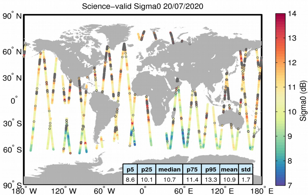
Figure 27. Geographical distribution of science-valid sigma0 data over oceans and lakes for 20/07/2020. The statistical values shown in the table refer to the sigma0 in dB and are calculated over all measurements shown in the figure. Gray circles denote records that have been rejected based on the editing criteria described in Table 4.
