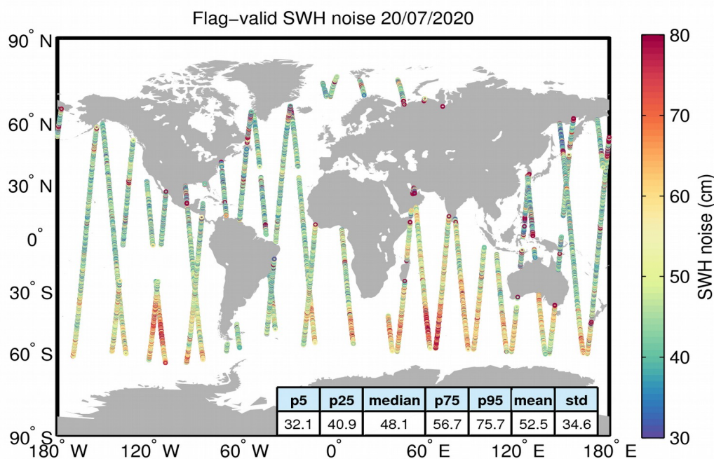
Figure 18. Geographical distribution of flag-valid 20-Hz SWH measurement noise over oceans and lakes for 20/07/2020. The statistical values shown in the figure refer to the SWH noise and are calculated over all measurements shown in the figure.
