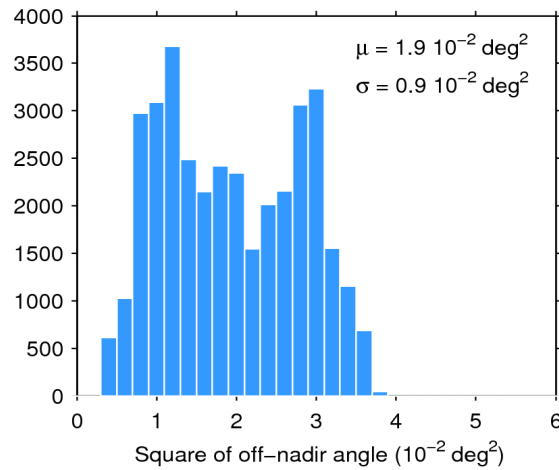
Figure 39. Histogram of flag-valid mispointing over oceans and lakes for 20/07/2020. The mean ( \mu ) and standard deviation ( \sigma ) are also shown. Note that values larger than 6 \cdot 10^{-2} \text{ deg}^2 are excluded from the histogram for the sake of readability but not from the computation of \mu and \sigma .
