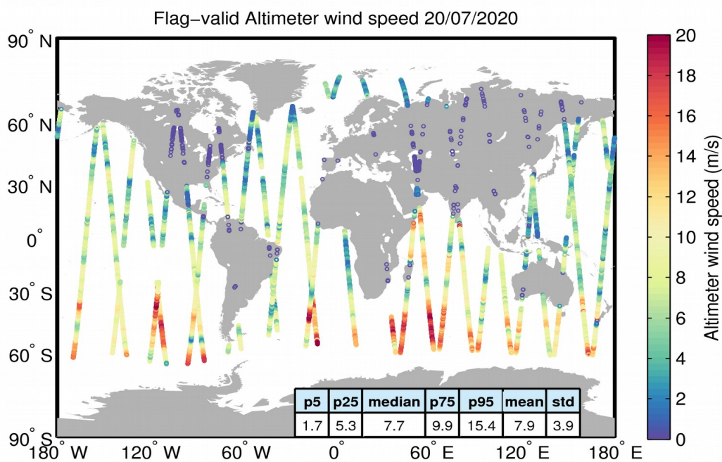
Figure 31. Geographical distribution of flag-valid wind data over oceans and lakes for 20/07/2020. The statistical values shown in the table refer to the wind in m/s and are calculated over all measurements shown in the figure.
