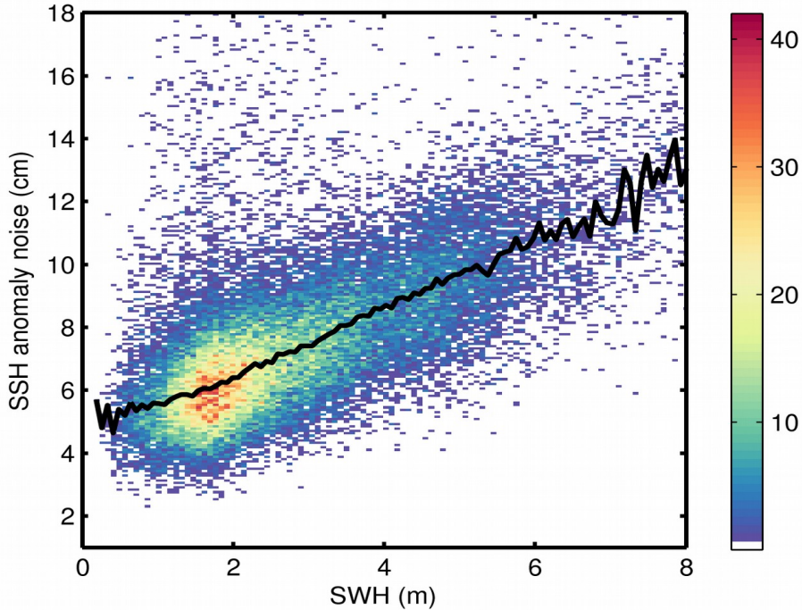
Figure 9. 2D histogram showing flag-valid SSH anomaly noise as a function of SWH for 20/07/2020. The black line denotes the median SSH anomaly noise as a function of SWH.
