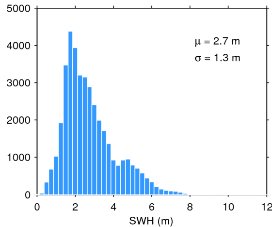
Figure 20. Histogram of science-valid SWH over oceans and lakes for 19/07/2020. The mean ( \mu ) and standard deviation ( \sigma ) are also shown. Note that values larger than 12 m are excluded from the histogram for the sake of readability but not from the computation of \mu and \sigma .
