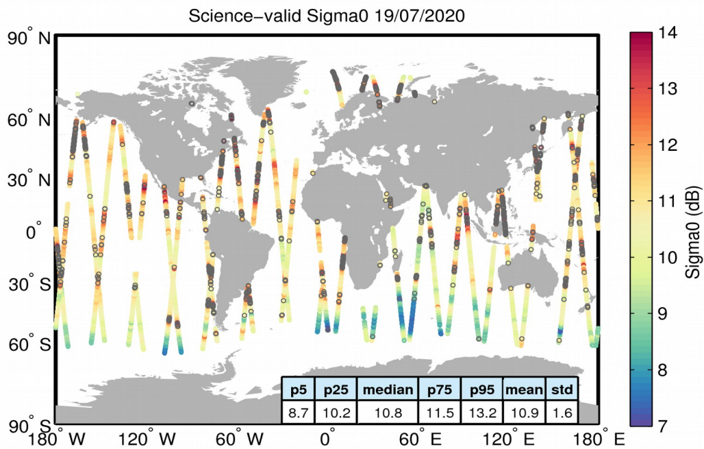
Figure 27. Geographical distribution of science-valid sigma0 data over oceans and lakes for 19/07/2020. The statistical values shown in the table refer to the sigma0 in dB and are calculated over all measurements shown in the figure. Gray circles denote records that have been rejected based on the editing criteria described in Table 4.
