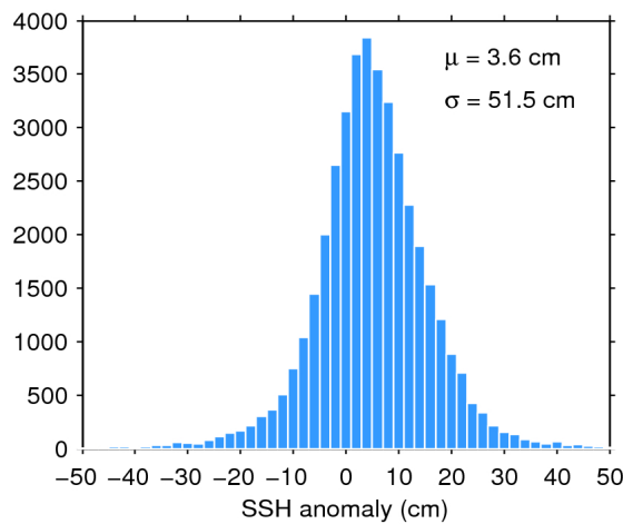
Figure 7. Histogram of flag-valid SSH anomaly over oceans and lakes for 19/07/2020. The mean ( \mu ) and standard deviation ( \sigma ) are also shown. Note that values outside [-50 50] cm are excluded from the histogram for the sake of readability but not from the computation of \mu and \sigma .
