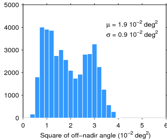
Figure 39. Histogram of flag-valid mispointing over oceans and lakes for 19/07/2020. The mean ( \mu ) and standard deviation ( \sigma ) are also shown. Note that values larger than 6 \cdot 10^{-2} \text{ deg}^2 are excluded from the histogram for the sake of readability but not from the computation of \mu and \sigma .
