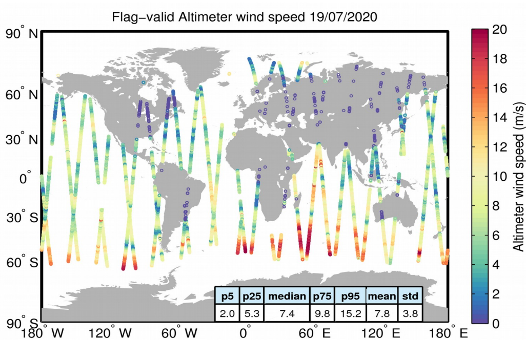
Figure 31. Geographical distribution of flag-valid wind data over oceans and lakes for 19/07/2020. The statistical values shown in the table refer to the wind in m/s and are calculated over all measurements shown in the figure.
