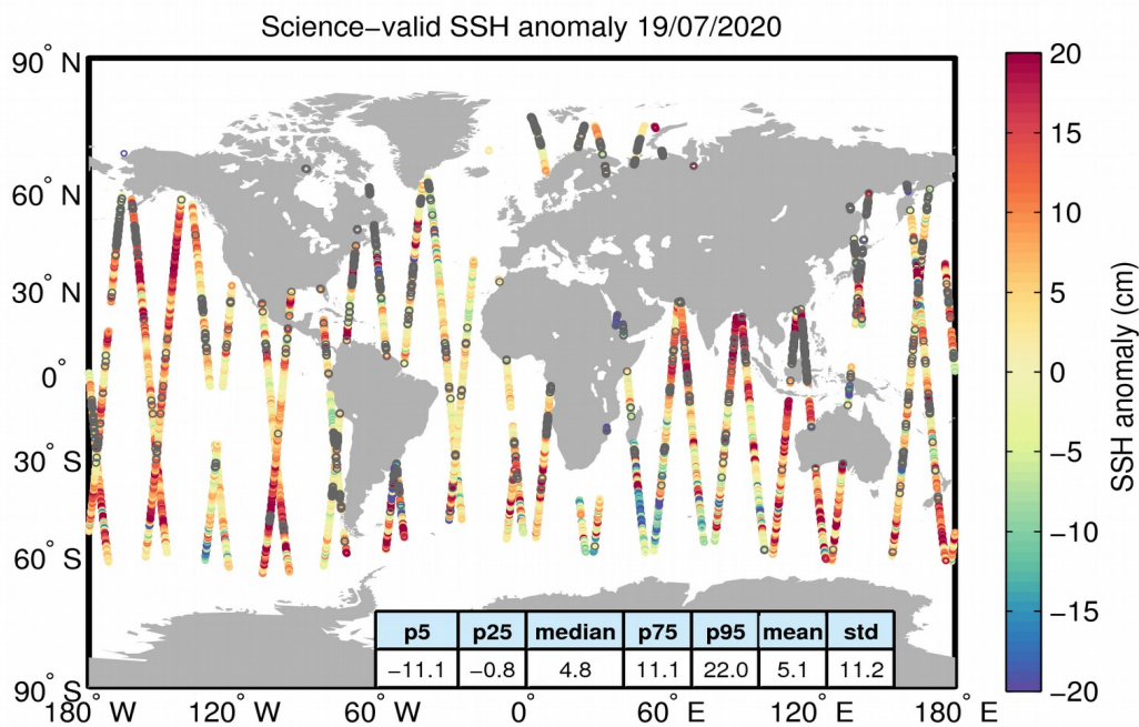
Figure 10. Geographical distribution of science-valid SSH anomaly data over oceans and lakes for 19/07/2020. The statistical values shown in the table refer to the SSH anomaly in cm and are calculated over all measurements shown in the figure. Gray circles denote records that have been rejected based on the editing criteria described in Table 2.
