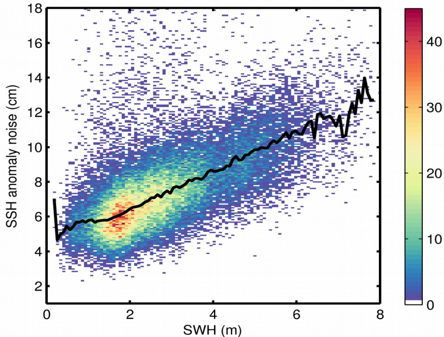
Figure 9. 2D histogram showing flag-valid SSH anomaly noise as a function of SWH for 19/07/2020. The black line denotes the median SSH anomaly noise as a function of SWH.
