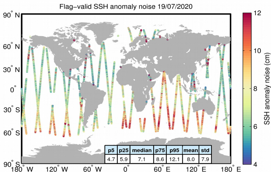
Figure 8. Geographical distribution of flag-valid 20-Hz SSH anomaly measurement noise over oceans and lakes for 19/07/2020. The statistical values shown in the table refer to the SSH anomaly noise and are calculated over all measurements shown in the figure.
