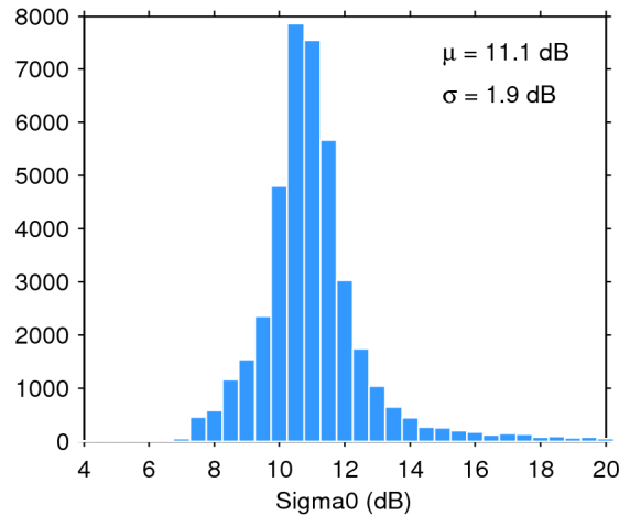
Figure 25. Histogram of flag-valid sigma0 over oceans and lakes for 19/07/2020. The mean ( \mu ) and standard deviation ( \sigma ) are also shown. Note that values outside [4 20] dB are excluded from the histogram for the sake of readability but not from the computation of \mu and \sigma .
