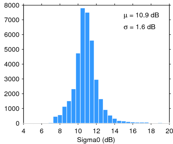
Figure 28. Histogram of science-valid sigma0 over oceans and lakes for 19/07/2020. The mean ( \mu ) and standard deviation ( \sigma ) are also shown. Note that values outside [4 20] dB are excluded from the histogram for the sake of readability but not from the computation of \mu and \sigma .
