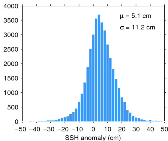
Figure 11. Histogram of science-valid SSH anomaly over oceans and lakes for 19/07/2020. The mean ( \mu ) and standard deviation ( \sigma ) are also shown. Note that values outside [-50 50] cm are excluded from the histogram for the sake of readability but not from the computation of \mu and \sigma .
