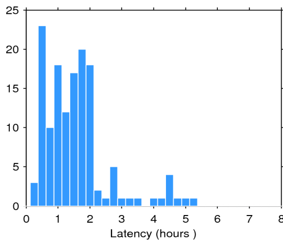
Figure 2. Histogram of the data latency for 19/07/2020. The y-axis denotes the number of files that are made available with a delay of x-hours with respect to the mean time of the records stored in the file.
