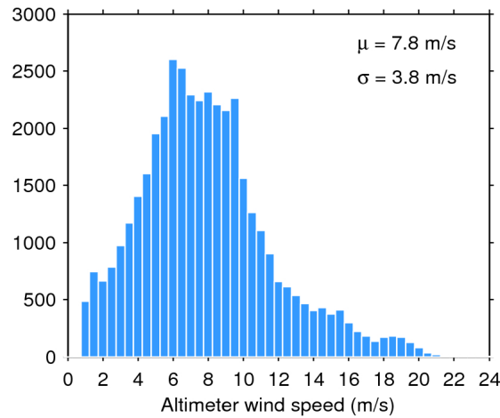
Figure 33. Histogram of flag-valid wind over oceans and lakes for 19/07/2020. The mean ( \mu ) and standard deviation ( \sigma ) are also shown. Note that values larger than 24 m/s are excluded from the histogram for the sake of readability but not from the computation of \mu and \sigma .
