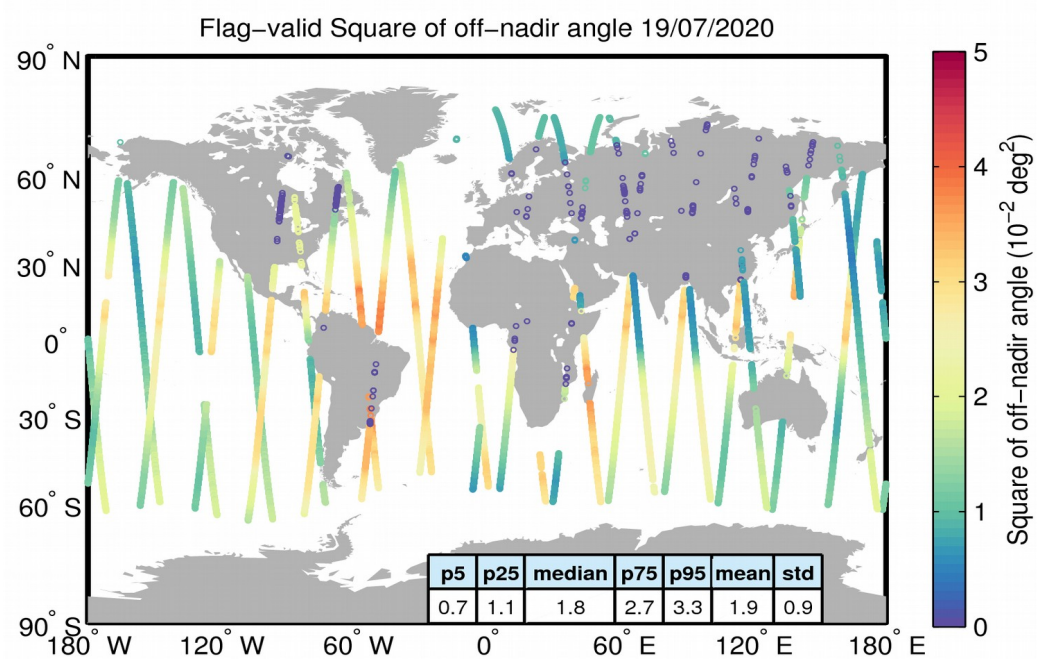
Figure 37. Geographical distribution of flag-valid mispointing data over oceans and lakes for 19/07/2020. The statistical values shown in the table refer to the mispointing in 10^{-2} deg 2 and are calculated over all measurements shown in the figure.
