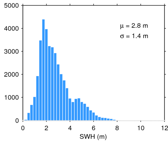
Figure 17. Histogram of flag-valid SWH over oceans and lakes for 19/07/2020. The mean ( \mu ) and standard deviation ( \sigma ) are also shown. Note that values larger than 12 m are excluded from the histogram for the sake of readability but not from the computation of \mu and \sigma .
