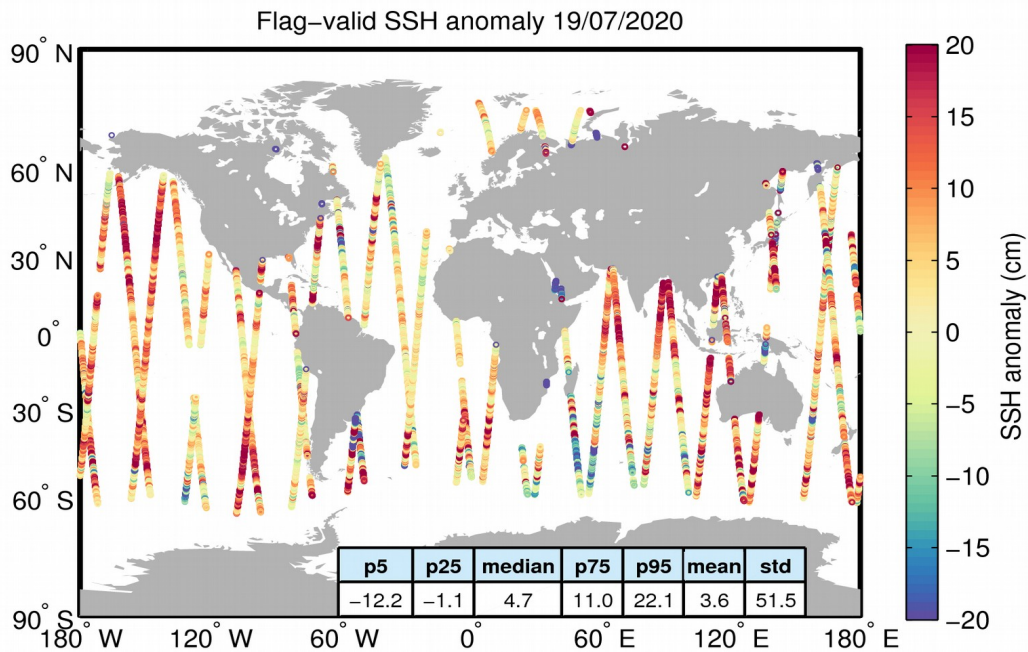
Figure 5. Geographical distribution of flag-valid 1-Hz SSH anomaly data over oceans and lakes for 19/07/2020. The statistical values shown in the table refer to the SSH anomaly in cm and are calculated over all measurements shown in the figure.
