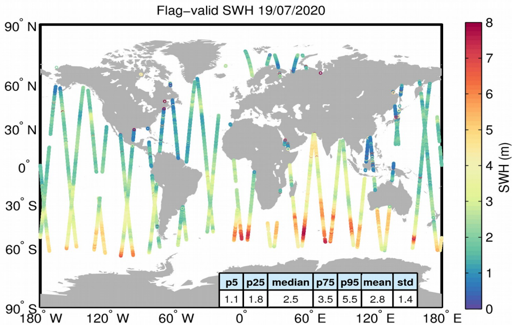
Figure 15. Geographical distribution of flag-valid SWH data over oceans and lakes for 19/07/2020. The statistical values shown in the table refer to the SWH in m and are calculated over all measurements shown in the figure.
