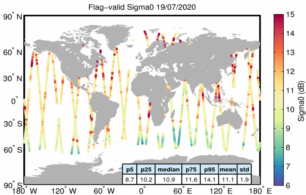
Figure 23. Geographical distribution of flag-valid sigma0 data over oceans and lakes for 19/07/2020. The statistical values shown in the table refer to the sigma0 in dB and are calculated over all measurements shown in the figure.
