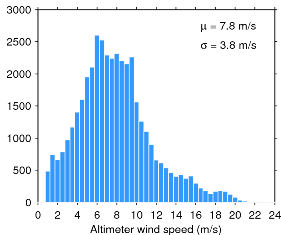
Figure 35. Histogram of science-valid wind over oceans and lakes for 19/07/2020. The mean ( \mu ) and standard deviation ( \sigma ) are also shown. Note that values larger than 24 m/s are excluded from the histogram for the sake of readability but not from the computation of \mu and \sigma .
