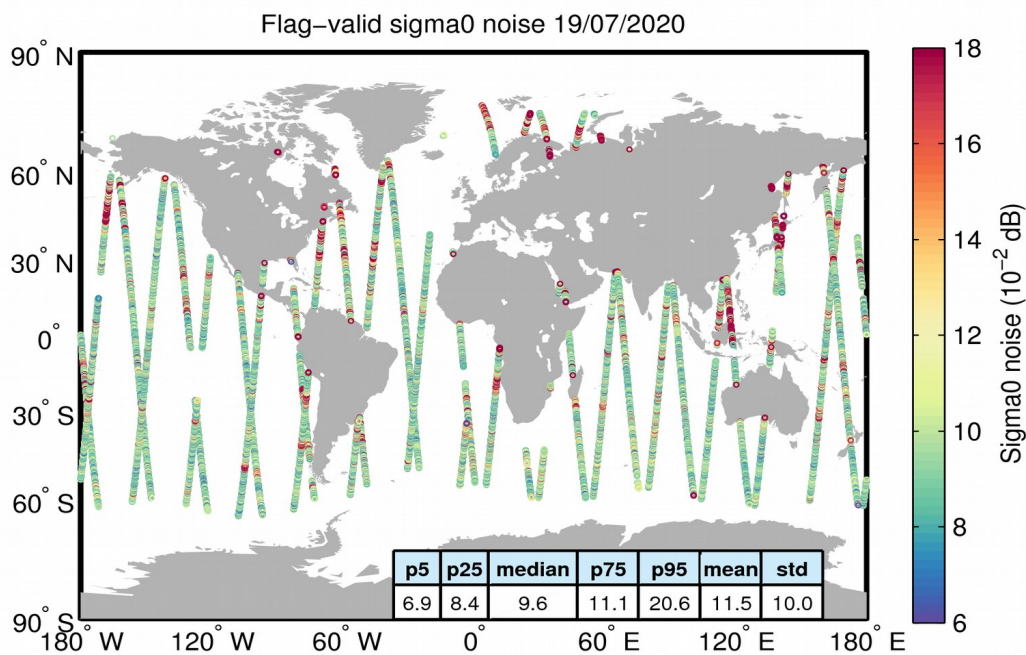
Figure 26. Geographical distribution of flag-valid 20-Hz sigma0 measurement noise over oceans and lakes for 19/07/2020. The statistical values shown in the table refer to the sigma0 noise and are calculated over all measurements shown in the figure.
