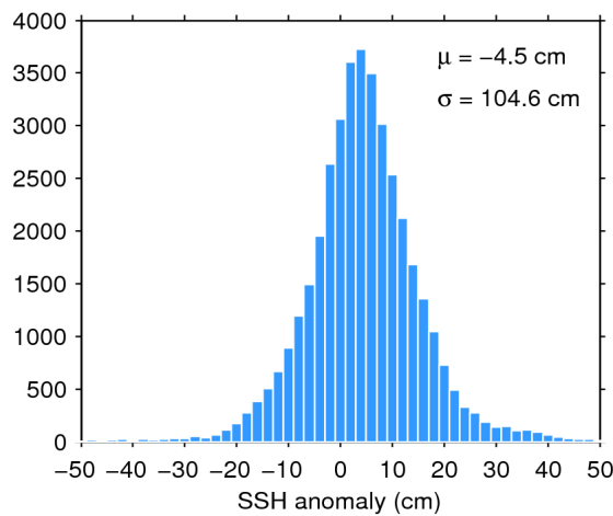
Figure 7. Histogram of flag-valid SSH anomaly over oceans and lakes for 18/07/2020. The mean ( \mu ) and standard deviation ( \sigma ) are also shown. Note that values outside [-50 50] cm are excluded from the histogram for the sake of readability but not from the computation of \mu and \sigma .
