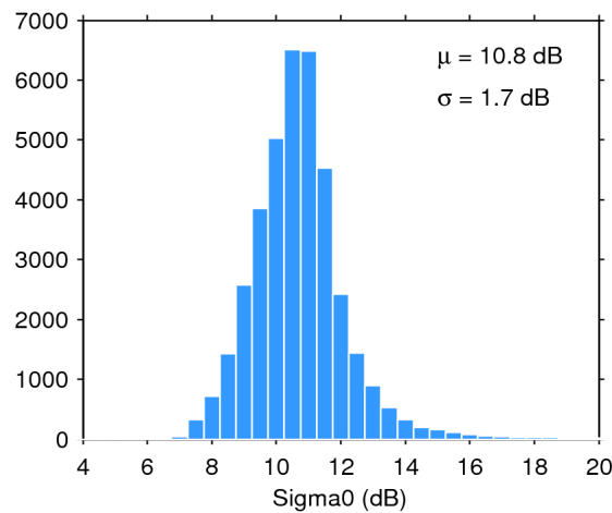
Figure 28. Histogram of science-valid sigma0 over oceans and lakes for 18/07/2020. The mean ( \mu ) and standard deviation ( \sigma ) are also shown. Note that values outside [4 20] dB are excluded from the histogram for the sake of readability but not from the computation of \mu and \sigma .
