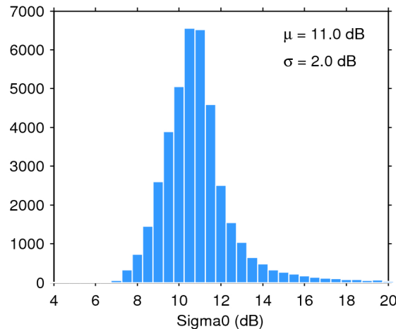
Figure 25. Histogram of flag-valid sigma0 over oceans and lakes for 18/07/2020. The mean ( \mu ) and standard deviation ( \sigma ) are also shown. Note that values outside [4 20] dB are excluded from the histogram for the sake of readability but not from the computation of \mu and \sigma .
