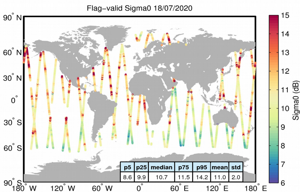
Figure 23. Geographical distribution of flag-valid sigma0 data over oceans and lakes for 18/07/2020. The statistical values shown in the table refer to the sigma0 in dB and are calculated over all measurements shown in the figure.
