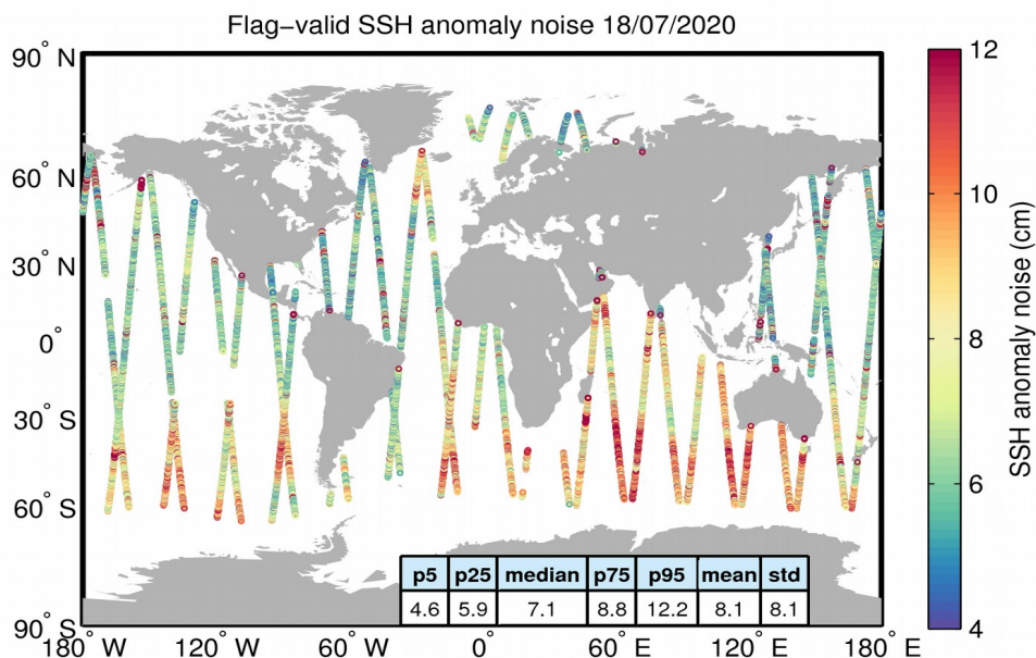
Figure 8. Geographical distribution of flag-valid 20-Hz SSH anomaly measurement noise over oceans and lakes for 18/07/2020. The statistical values shown in the table refer to the SSH anomaly noise and are calculated over all measurements shown in the figure.
