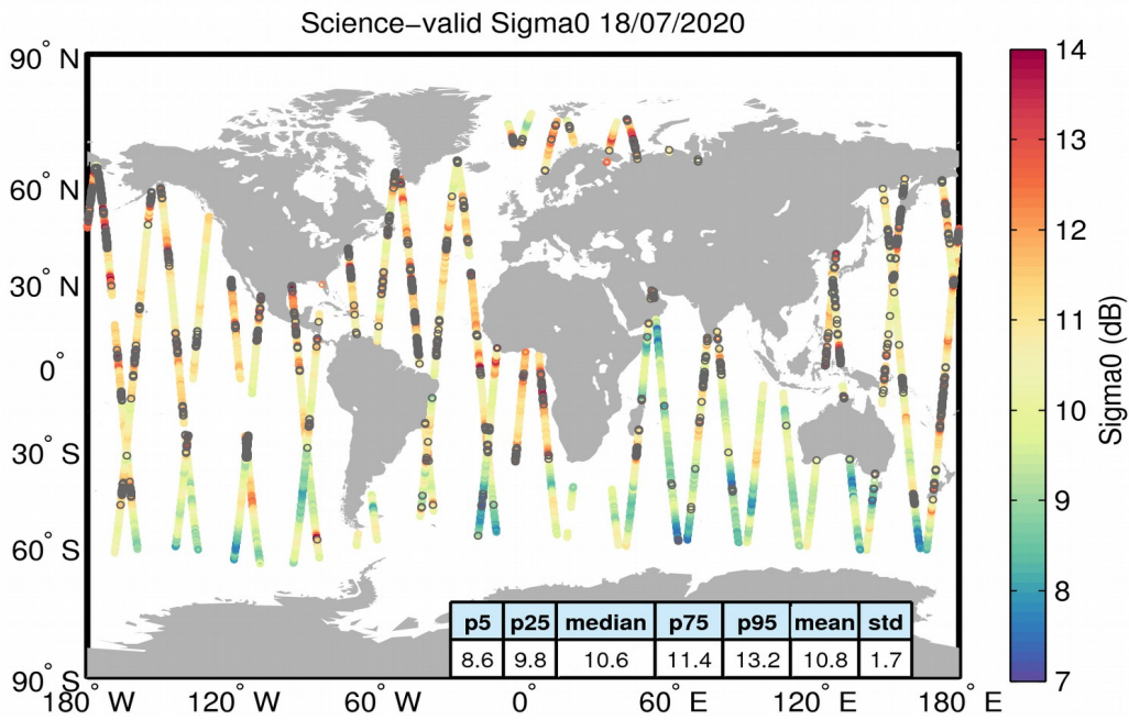
Figure 27. Geographical distribution of science-valid sigma0 data over oceans and lakes for 18/07/2020. The statistical values shown in the table refer to the sigma0 in dB and are calculated over all measurements shown in the figure. Gray circles denote records that have been rejected based on the editing criteria described in Table 4.
