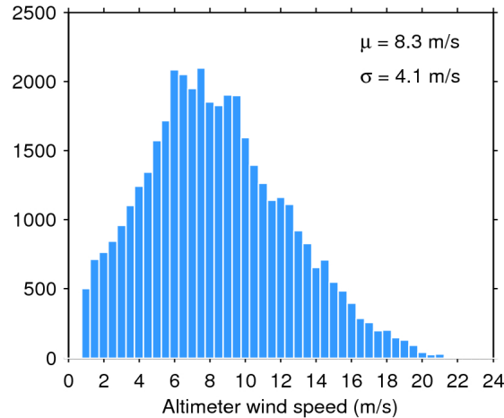
Figure 33. Histogram of flag-valid wind over oceans and lakes for 18/07/2020. The mean ( \mu ) and standard deviation ( \sigma ) are also shown. Note that values larger than 24 m/s are excluded from the histogram for the sake of readability but not from the computation of \mu and \sigma .
