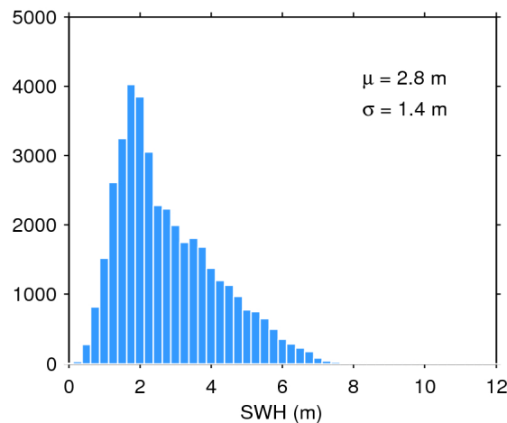
Figure 17. Histogram of flag-valid SWH over oceans and lakes for 18/07/2020. The mean ( \mu ) and standard deviation ( \sigma ) are also shown. Note that values larger than 12 m are excluded from the histogram for the sake of readability but not from the computation of \mu and \sigma .
