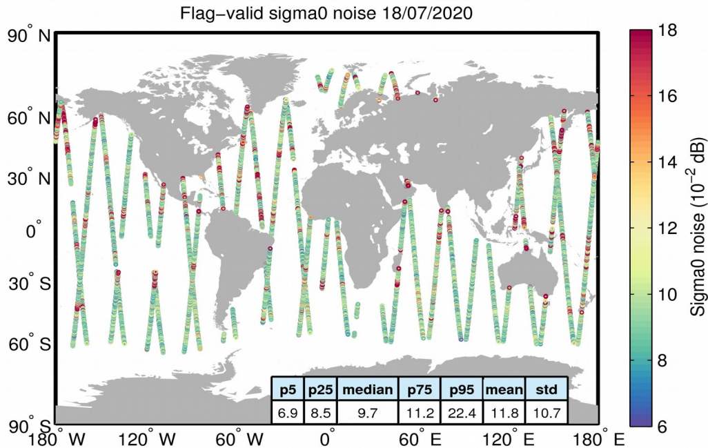
Figure 26. Geographical distribution of flag-valid 20-Hz sigma0 measurement noise over oceans and lakes for 18/07/2020. The statistical values shown in the table refer to the sigma0 noise and are calculated over all measurements shown in the figure.
