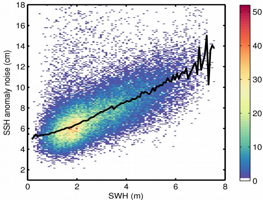
Figure 9. 2D histogram showing flag-valid SSH anomaly noise as a function of SWH for 18/07/2020. The black line denotes the median SSH anomaly noise as a function of SWH.
