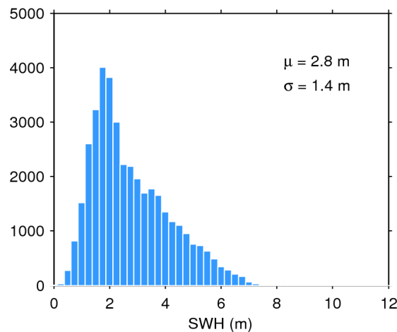
Figure 20. Histogram of science-valid SWH over oceans and lakes for 18/07/2020. The mean ( \mu ) and standard deviation ( \sigma ) are also shown. Note that values larger than 12 m are excluded from the histogram for the sake of readability but not from the computation of \mu and \sigma .
