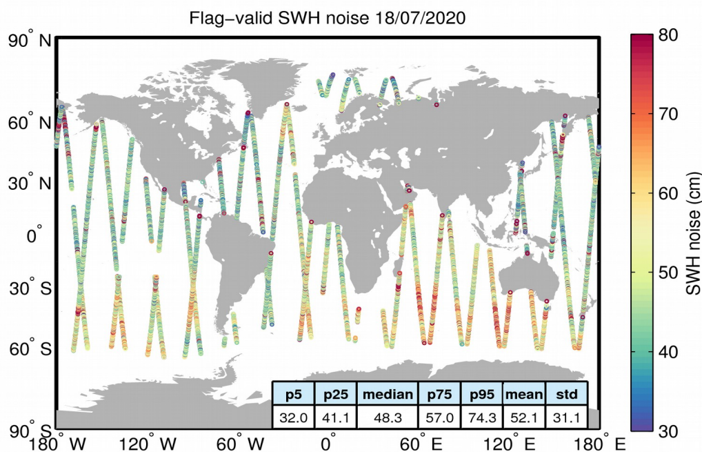
Figure 18. Geographical distribution of flag-valid 20-Hz SWH measurement noise over oceans and lakes for 18/07/2020. The statistical values shown in the table refer to the SWH noise and are calculated over all measurements shown in the figure.
