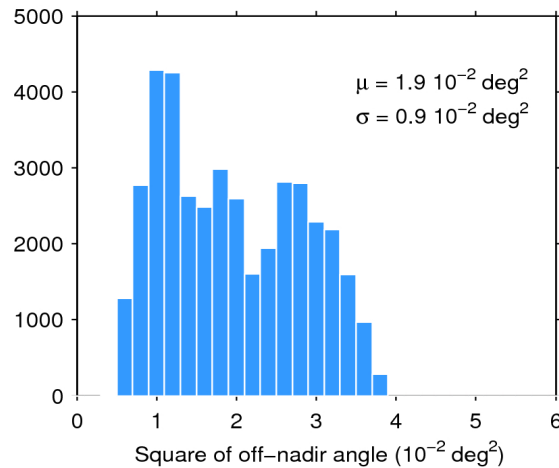
Figure 39. Histogram of flag-valid mispointing over oceans and lakes for 18/07/2020. The mean ( \mu ) and standard deviation ( \sigma ) are also shown. Note that values larger than 6 \cdot 10^{-2} \text{ deg}^2 are excluded from the histogram for the sake of readability but not from the computation of \mu and \sigma .
