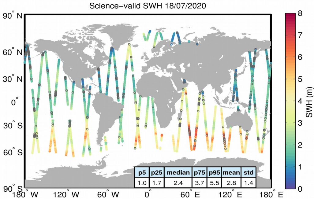
Figure 19. Geographical distribution of science-valid SWH data over oceans and lakes for 18/07/2020. The statistical values shown in the table refer to the SWH in m and are calculated over all measurements shown in the figure. Gray circles denote records that have been rejected based on the editing criteria described in Table 3.
