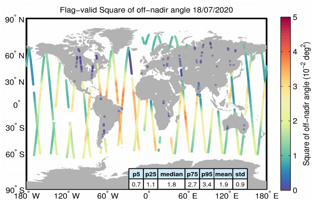
Figure 37. Geographical distribution of flag-valid mispointing data over oceans and lakes for 18/07/2020. The statistical values shown in the table refer to the mispointing in 10^{-2} deg 2 and are calculated over all measurements shown in the figure.
