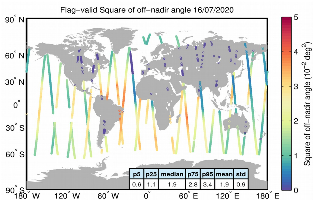
Figure 37. Geographical distribution of flag-valid mispointing data over oceans and lakes for 16/07/2020. The statistical values shown in the table refer to the mispointing in 10^{-2} \text{ deg}^2 and are calculated over all measurements shown in the figure.
