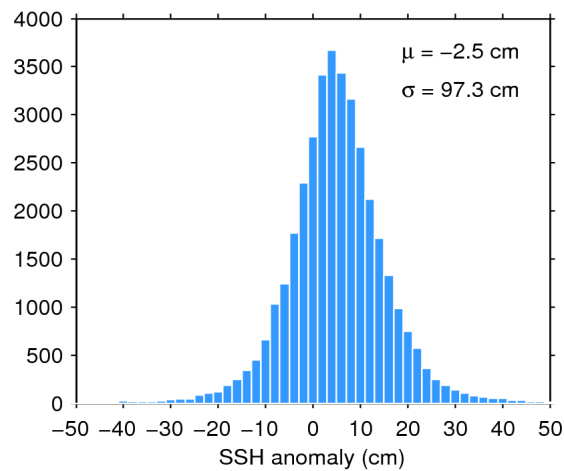
Figure 7. Histogram of flag-valid SSH anomaly over oceans and lakes for 16/07/2020. The mean ( \mu ) and standard deviation ( \sigma ) are also shown. Note that values outside [-50 50] cm are excluded from the histogram for the sake of readability but not from the computation of \mu and \sigma .
