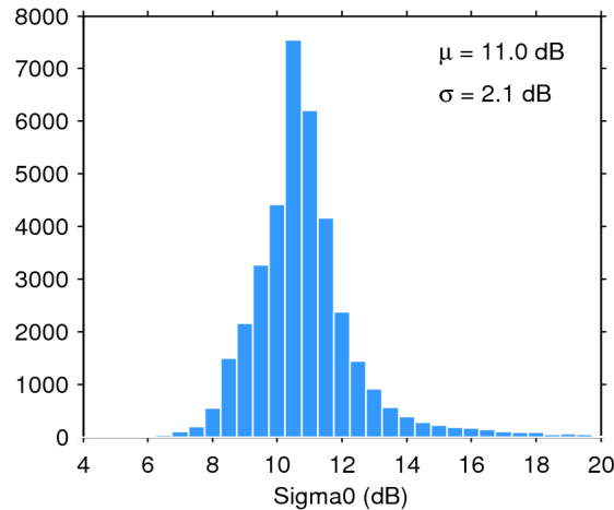
Figure 25. Histogram of flag-valid sigma0 over oceans and lakes for 16/07/2020. The mean ( \mu ) and standard deviation ( \sigma ) are also shown. Note that values outside [4 20] dB are excluded from the histogram for the sake of readability but not from the computation of \mu and \sigma .
