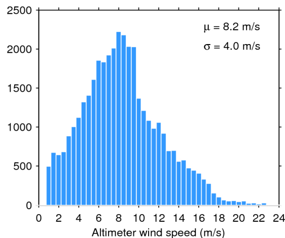
Figure 35. Histogram of science-valid wind over oceans and lakes for 16/07/2020. The mean ( \mu ) and standard deviation ( \sigma ) are also shown. Note that values larger than 24 m/s are excluded from the histogram for the sake of readability but not from the computation of \mu and \sigma .
