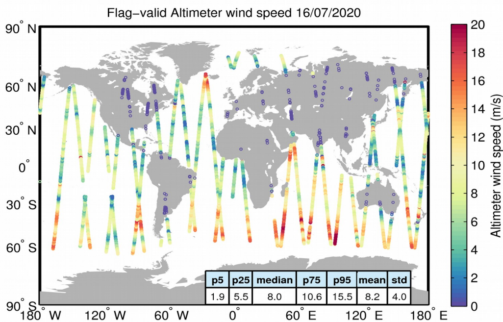
Figure 31. Geographical distribution of flag-valid wind data over oceans and lakes for 16/07/2020. The statistical values shown in the table refer to the wind in m/s and are calculated over all measurements shown in the figure.
