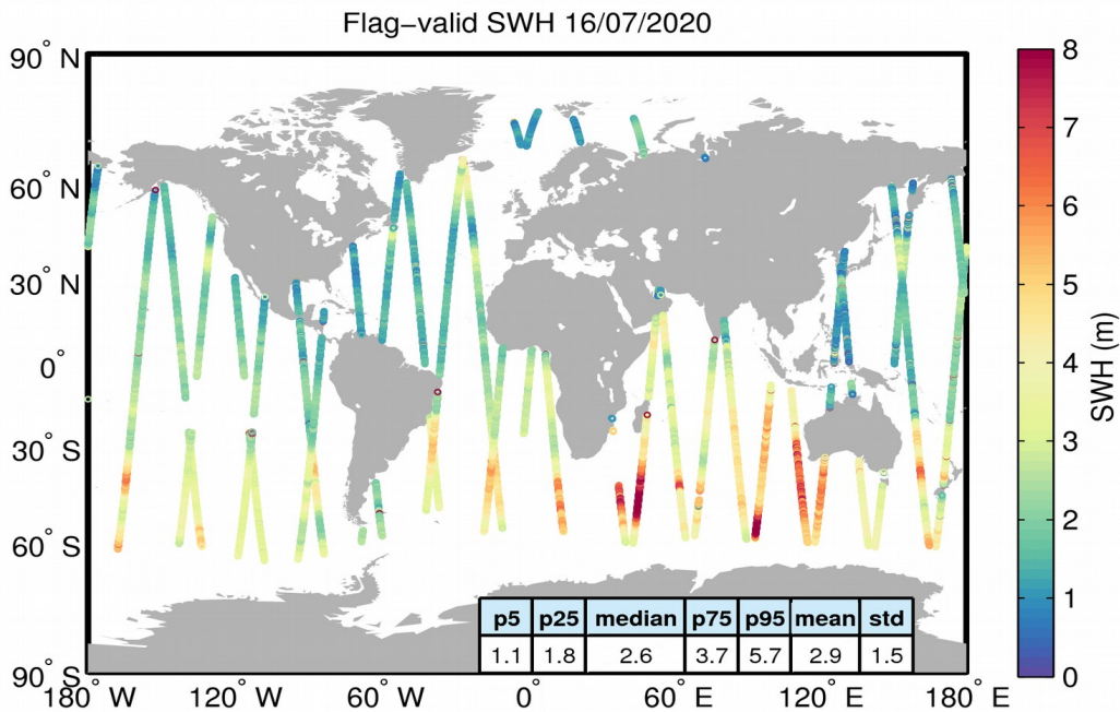
Figure 15. Geographical distribution of flag-valid SWH data over oceans and lakes for 16/07/2020. The statistical values shown in the table refer to the SWH in m and are calculated over all measurements shown in the figure.
