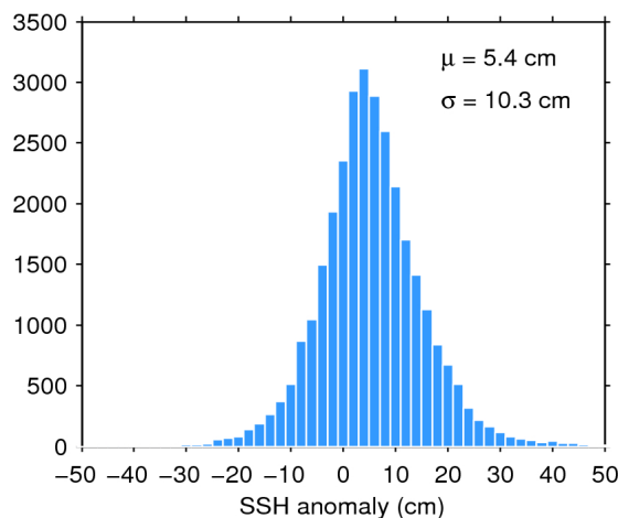
Figure 11. Histogram of science-valid SSH anomaly over oceans and lakes for 16/07/2020. The mean ( \mu ) and standard deviation ( \sigma ) are also shown. Note that values outside [-50 50] cm are excluded from the histogram for the sake of readability but not from the computation of \mu and \sigma .
