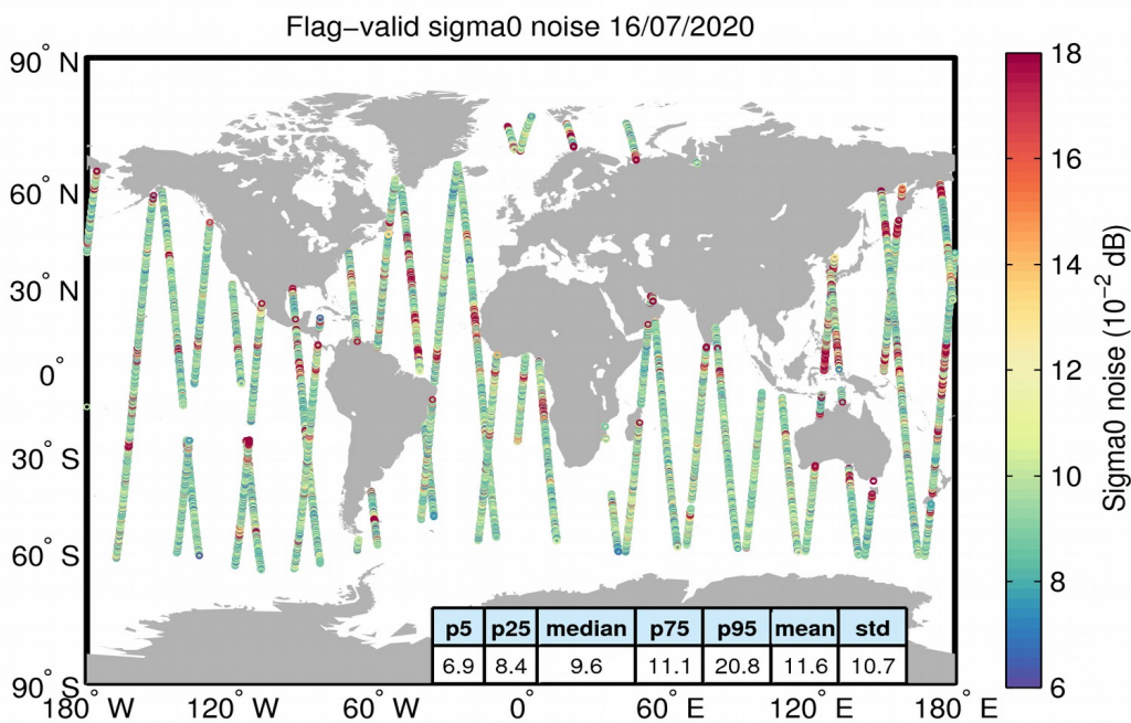
Figure 26. Geographical distribution of flag-valid 20-Hz sigma0 measurement noise over oceans and lakes for 16/07/2020. The statistical values shown in the table refer to the sigma0 noise and are calculated over all measurements shown in the figure.
