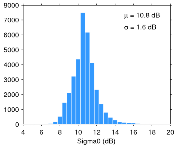
Figure 28. Histogram of science-valid sigma0 over oceans and lakes for 16/07/2020. The mean ( \mu ) and standard deviation ( \sigma ) are also shown. Note that values outside [4 20] dB are excluded from the histogram for the sake of readability but not from the computation of \mu and \sigma .
