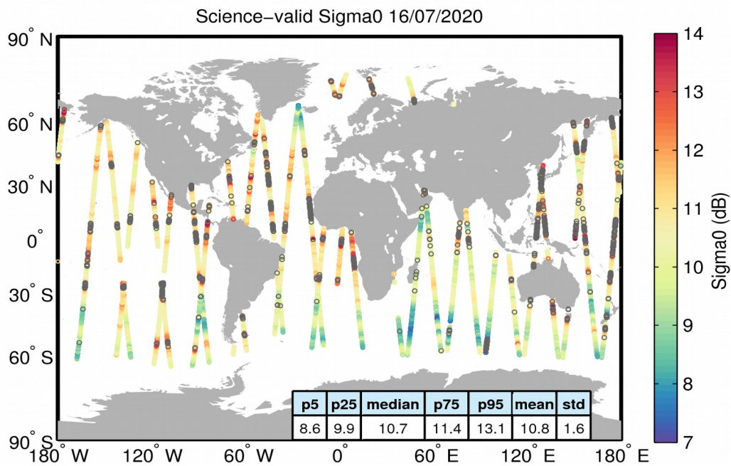
Figure 27. Geographical distribution of science-valid sigma0 data over oceans and lakes for 16/07/2020. The statistical values shown in the table refer to the sigma0 in dB and are calculated over all measurements shown in the figure. Gray circles denote records that have been rejected based on the editing criteria described in Table 4.
