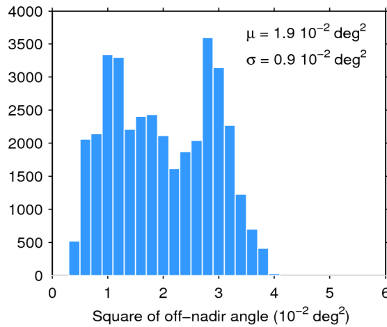
Figure 39. Histogram of flag-valid mispointing over oceans and lakes for 16/07/2020. The mean ( \mu ) and standard deviation ( \sigma ) are also shown. Note that values larger than 6 \cdot 10^{-2} \text{ deg}^2 are excluded from the histogram for the sake of readability but not from the computation of \mu and \sigma .
