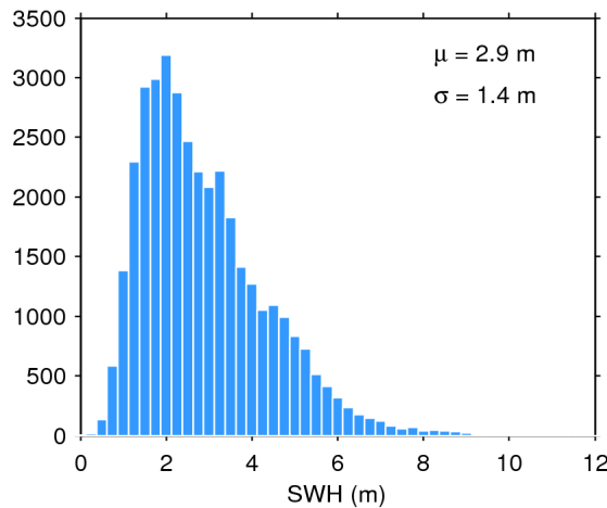
Figure 20. Histogram of science-valid SWH over oceans and lakes for 16/07/2020. The mean ( \mu ) and standard deviation ( \sigma ) are also shown. Note that values larger than 12 m are excluded from the histogram for the sake of readability but not from the computation of \mu and \sigma .
