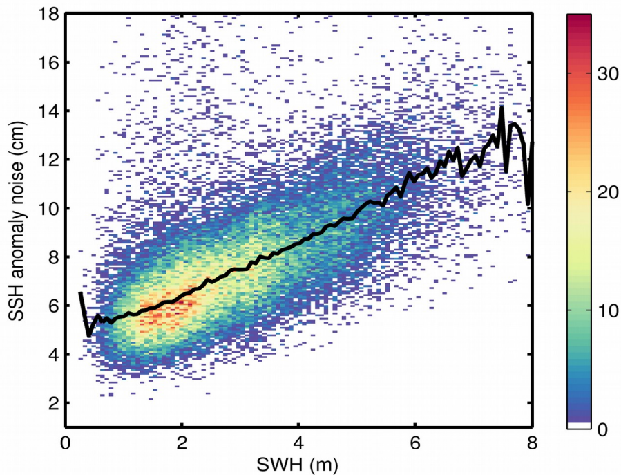
Figure 9. 2D histogram showing flag-valid SSH anomaly noise as a function of SWH for 16/07/2020. The black line denotes the median SSH anomaly noise as a function of SWH.
