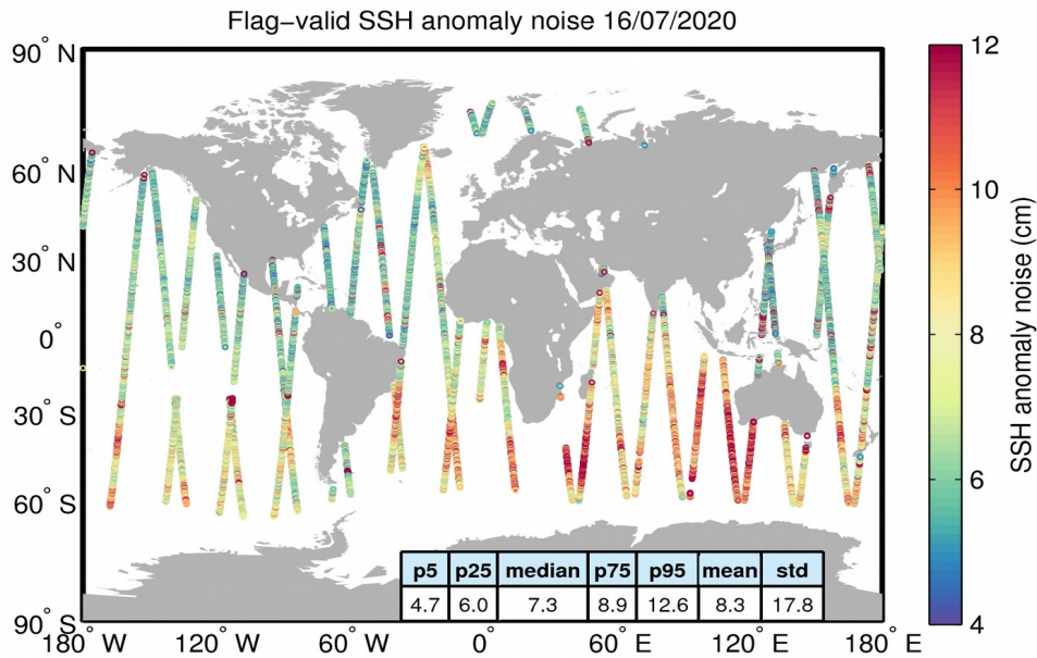
Figure 8. Geographical distribution of flag-valid 20-Hz SSH anomaly measurement noise over oceans and lakes for 16/07/2020. The statistical values shown in the table refer to the SSH anomaly noise and are calculated over all measurements shown in the figure.
