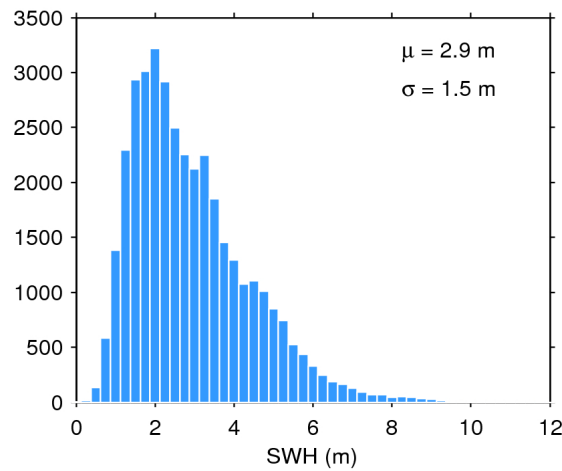
Figure 17. Histogram of flag-valid SWH over oceans and lakes for 16/07/2020. The mean ( \mu ) and standard deviation ( \sigma ) are also shown. Note that values larger than 12 m are excluded from the histogram for the sake of readability but not from the computation of \mu and \sigma .
