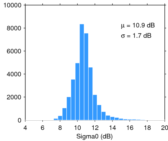
Figure 28. Histogram of science-valid sigma0 over oceans and lakes for 15/07/2020. The mean ( \mu ) and standard deviation ( \sigma ) are also shown. Note that values outside [4 20] dB are excluded from the histogram for the sake of readability but not from the computation of \mu and \sigma .
