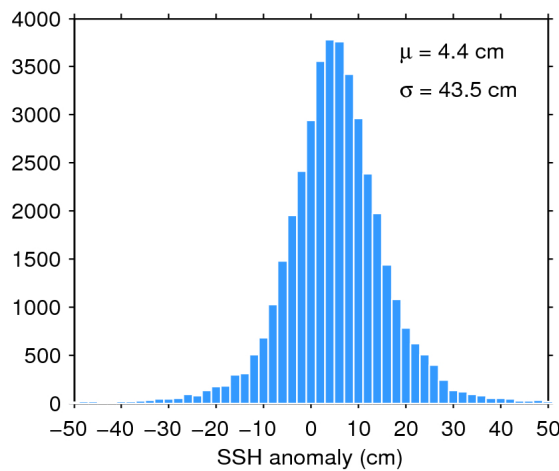
Figure 7. Histogram of flag-valid SSH anomaly over oceans and lakes for 15/07/2020. The mean ( \mu ) and standard deviation ( \sigma ) are also shown. Note that values outside [-50 50] cm are excluded from the histogram for the sake of readability but not from the computation of \mu and \sigma .
