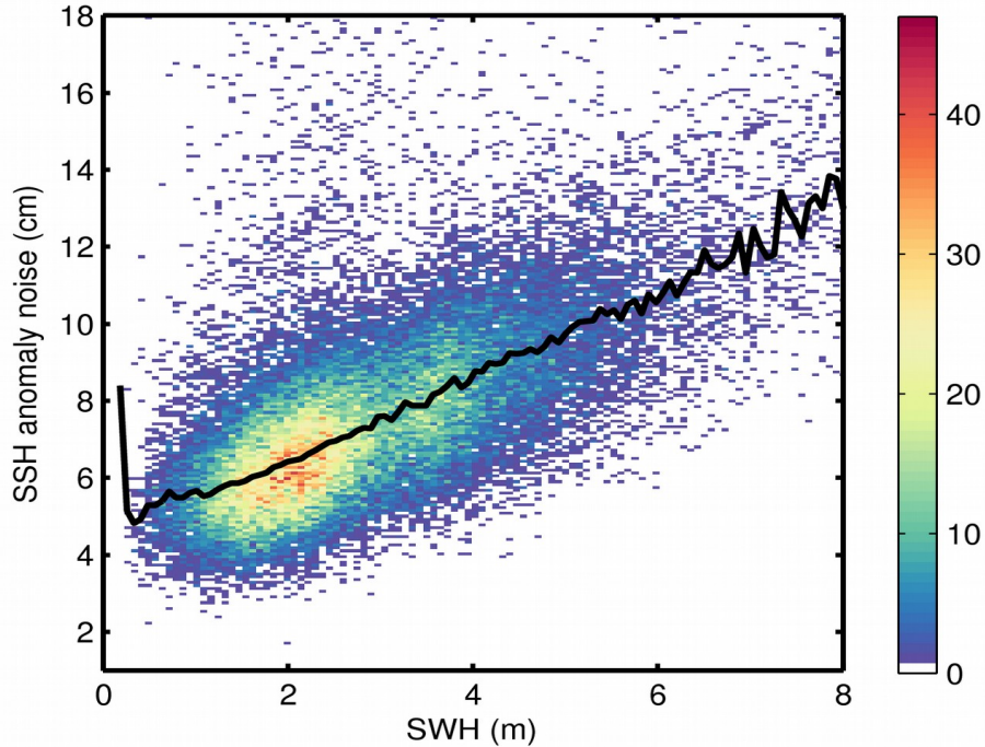
Figure 9. 2D histogram showing flag-valid SSH anomaly noise as a function of SWH for 15/07/2020. The black line denotes the median SSH anomaly noise as a function of SWH.
