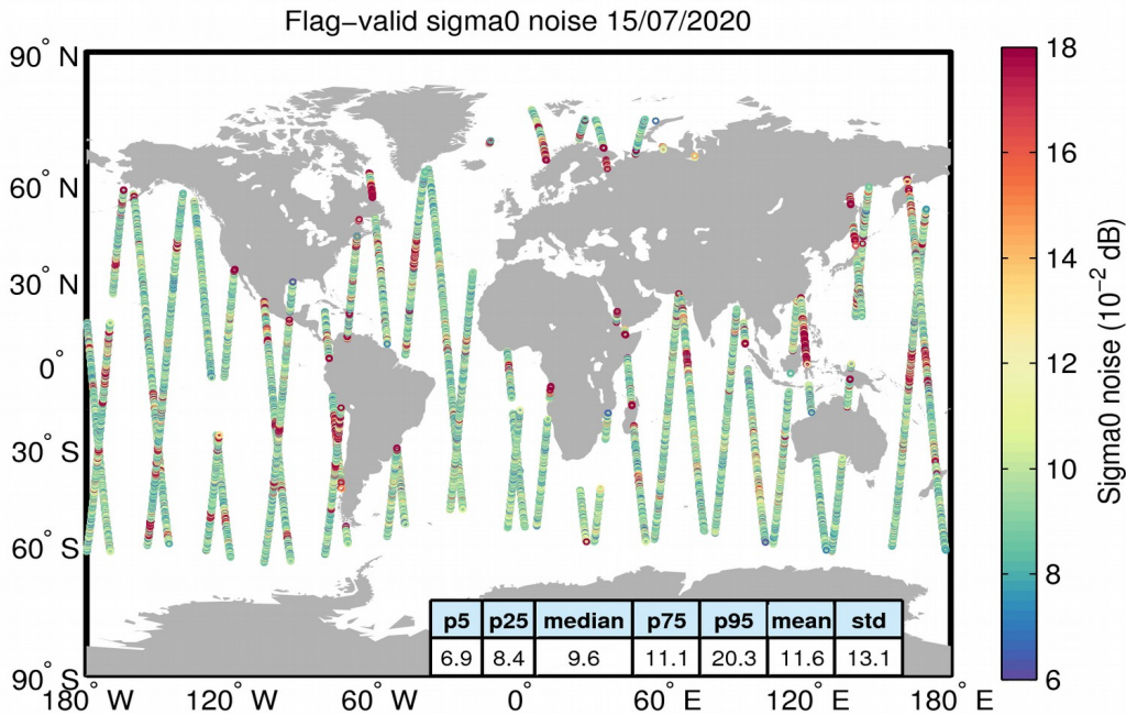
Figure 26. Geographical distribution of flag-valid 20-Hz sigma0 measurement noise over oceans and lakes for 15/07/2020. The statistical values shown in the table refer to the sigma0 noise and are calculated over all measurements shown in the figure.
