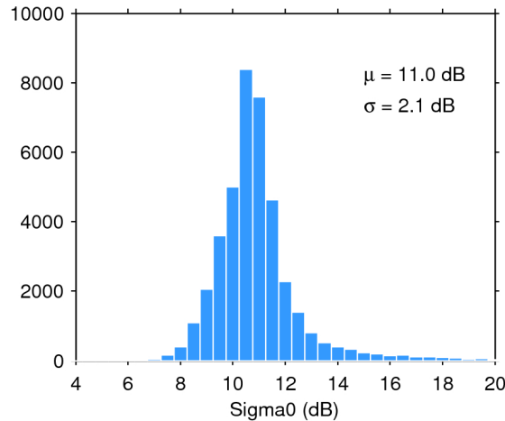
Figure 25. Histogram of flag-valid sigma0 over oceans and lakes for 15/07/2020. The mean ( \mu ) and standard deviation ( \sigma ) are also shown. Note that values outside [4 20] dB are excluded from the histogram for the sake of readability but not from the computation of \mu and \sigma .
