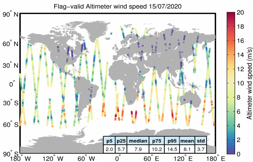
Figure 31. Geographical distribution of flag-valid wind data over oceans and lakes for 15/07/2020. The statistical values shown in the table refer to the wind in m/s and are calculated over all measurements shown in the figure.
