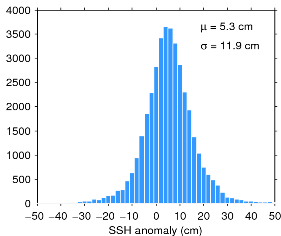
Figure 11. Histogram of science-valid SSH anomaly over oceans and lakes for 15/07/2020. The mean ( \mu ) and standard deviation ( \sigma ) are also shown. Note that values outside [-50 50] cm are excluded from the histogram for the sake of readability but not from the computation of \mu and \sigma .
