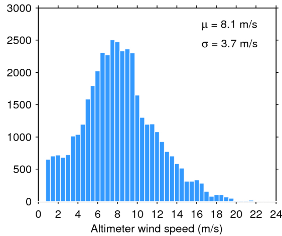
Figure 33. Histogram of flag-valid wind over oceans and lakes for 15/07/2020. The mean ( \mu ) and standard deviation ( \sigma ) are also shown. Note that values larger than 24 m/s are excluded from the histogram for the sake of readability but not from the computation of \mu and \sigma .
