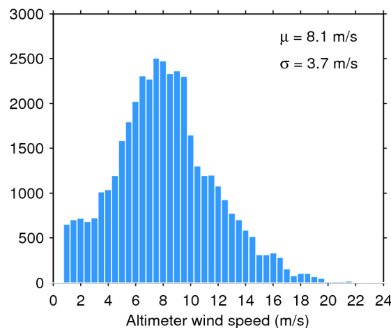
Figure 35. Histogram of science-valid wind over oceans and lakes for 15/07/2020. The mean ( \mu ) and standard deviation ( \sigma ) are also shown. Note that values larger than 24 m/s are excluded from the histogram for the sake of readability but not from the computation of \mu and \sigma .
