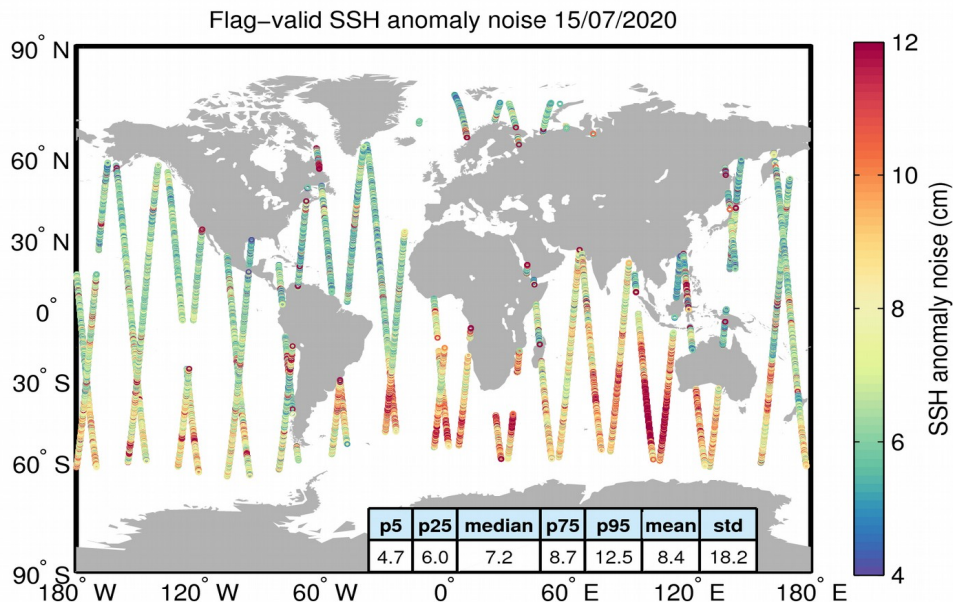
Figure 8. Geographical distribution of flag-valid 20-Hz SSH anomaly measurement noise over oceans and lakes for 15/07/2020. The statistical values shown in the table refer to the SSH anomaly noise and are calculated over all measurements shown in the figure.
