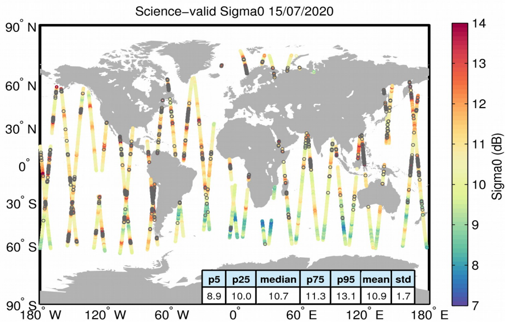
Figure 27. Geographical distribution of science-valid sigma0 data over oceans and lakes for 15/07/2020. The statistical values shown in the table refer to the sigma0 in dB and are calculated over all measurements shown in the figure. Gray circles denote records that have been rejected based on the editing criteria described in Table 4.
