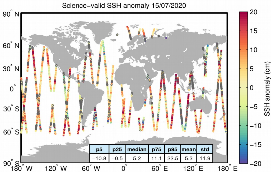
Figure 10. Geographical distribution of science-valid SSH anomaly data over oceans and lakes for 15/07/2020. The statistical values shown in the table refer to the SSH anomaly in cm and are calculated over all measurements shown in the figure. Gray circles denote records that have been rejected based on the editing criteria described in Table 2.
