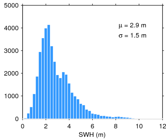
Figure 17. Histogram of flag-valid SWH over oceans and lakes for 15/07/2020. The mean ( \mu ) and standard deviation ( \sigma ) are also shown. Note that values larger than 12 m are excluded from the histogram for the sake of readability but not from the computation of \mu and \sigma .
