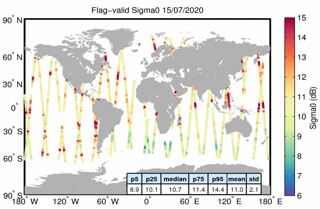
Figure 23. Geographical distribution of flag-valid sigma0 data over oceans and lakes for 15/07/2020. The statistical values shown in the table refer to the sigma0 in dB and are calculated over all measurements shown in the figure.
