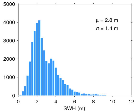
Figure 20. Histogram of science-valid SWH over oceans and lakes for 15/07/2020. The mean ( \mu ) and standard deviation ( \sigma ) are also shown. Note that values larger than 12 m are excluded from the histogram for the sake of readability but not from the computation of \mu and \sigma .
