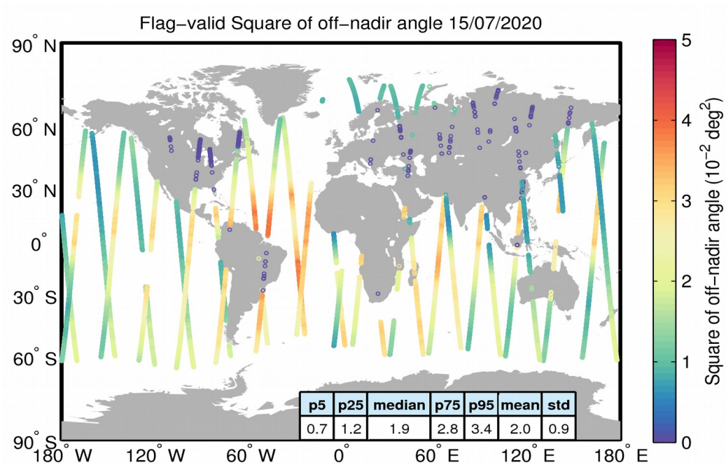
Figure 37. Geographical distribution of flag-valid mispointing data over oceans and lakes for 15/07/2020. The statistical values shown in the table refer to the mispointing in 10^{-2} \text{ deg}^2 and are calculated over all measurements shown in the figure.
