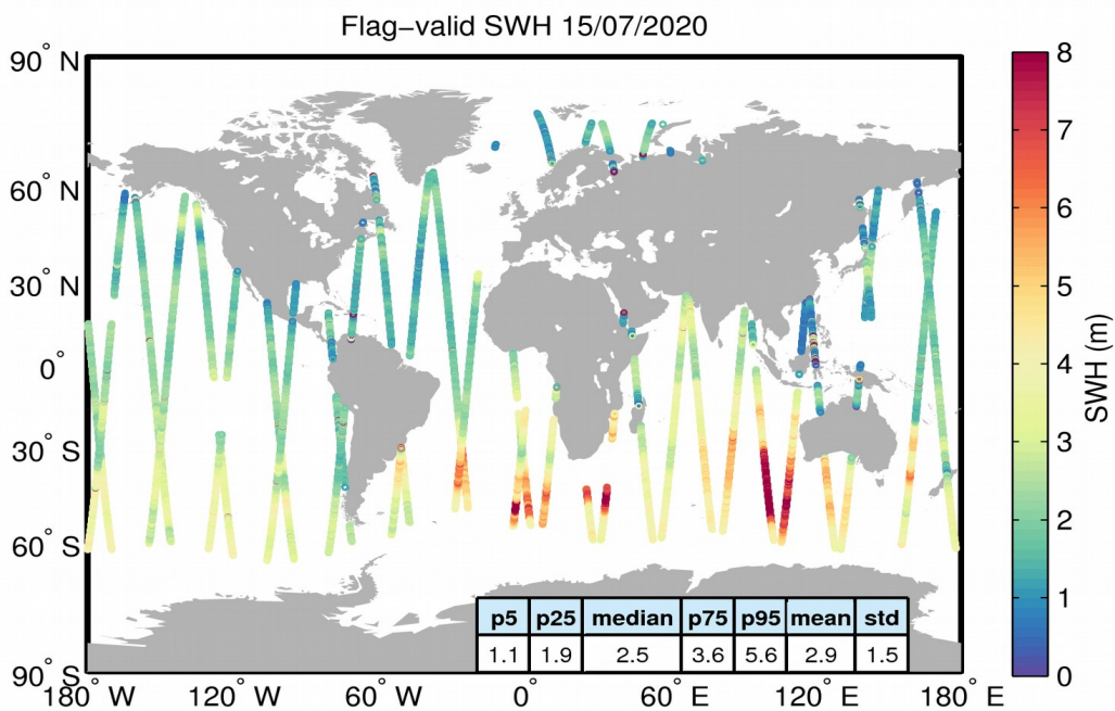
Figure 15. Geographical distribution of flag-valid SWH data over oceans and lakes for 15/07/2020. The statistical values shown in the table refer to the SWH in m and are calculated over all measurements shown in the figure.
