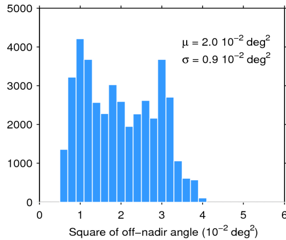
Figure 39. Histogram of flag-valid mispointing over oceans and lakes for 15/07/2020. The mean ( \mu ) and standard deviation ( \sigma ) are also shown. Note that values larger than 6 \cdot 10^{-2} \text{ deg}^2 are excluded from the histogram for the sake of readability but not from the computation of \mu and \sigma .
