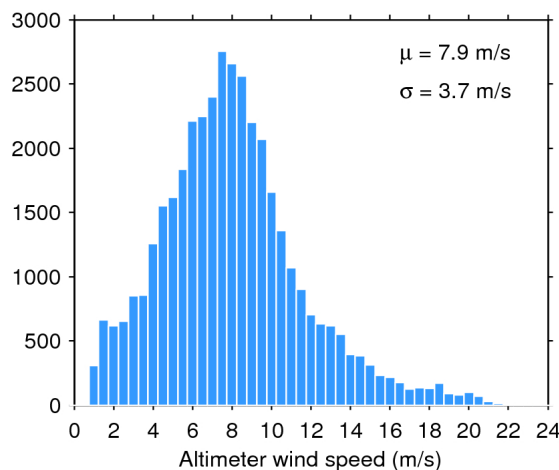
Figure 35. Histogram of science-valid wind over oceans and lakes for 14/07/2020. The mean ( \mu ) and standard deviation ( \sigma ) are also shown. Note that values larger than 24 m/s are excluded from the histogram for the sake of readability but not from the computation of \mu and \sigma .
