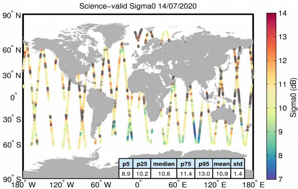
Figure 27. Geographical distribution of science-valid sigma0 data over oceans and lakes for 14/07/2020. The statistical values shown in the table refer to the sigma0 in dB and are calculated over all measurements shown in the figure. Gray circles denote records that have been rejected based on the editing criteria described in Table 4.
