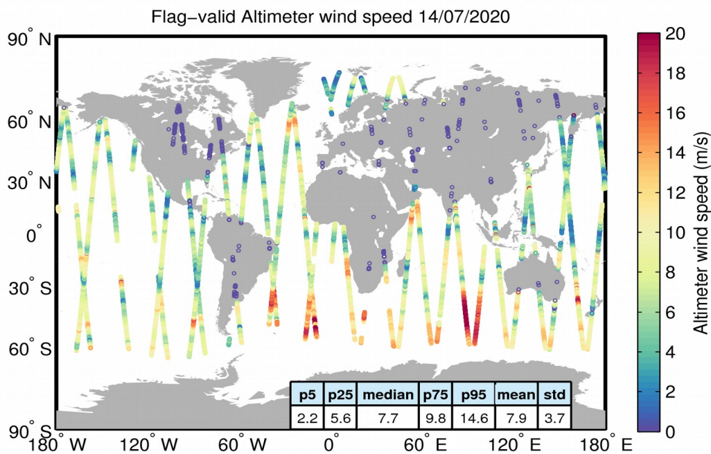
Figure 31. Geographical distribution of flag-valid wind data over oceans and lakes for 14/07/2020. The statistical values shown in the table refer to the wind in m/s and are calculated over all measurements shown in the figure.
