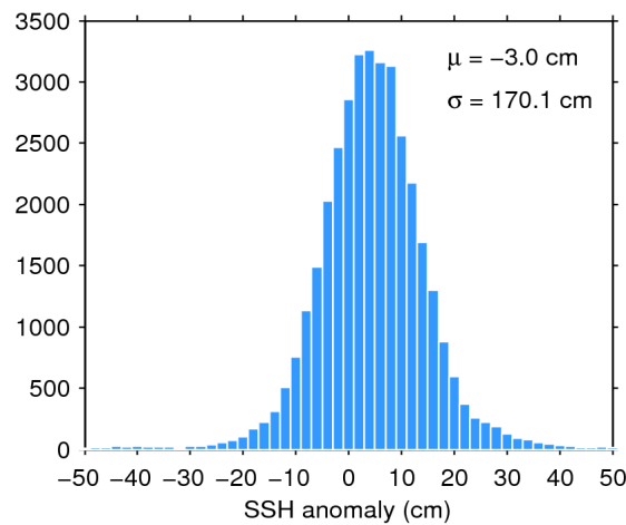
Figure 7. Histogram of flag-valid SSH anomaly over oceans and lakes for 14/07/2020. The mean ( \mu ) and standard deviation ( \sigma ) are also shown. Note that values outside [-50\ 50] cm are excluded from the histogram for the sake of readability but not from the computation of \mu and \sigma .
