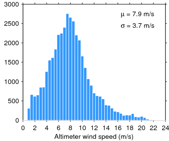
Figure 33. Histogram of flag-valid wind over oceans and lakes for 14/07/2020. The mean ( \mu ) and standard deviation ( \sigma ) are also shown. Note that values larger than 24 m/s are excluded from the histogram for the sake of readability but not from the computation of \mu and \sigma .
