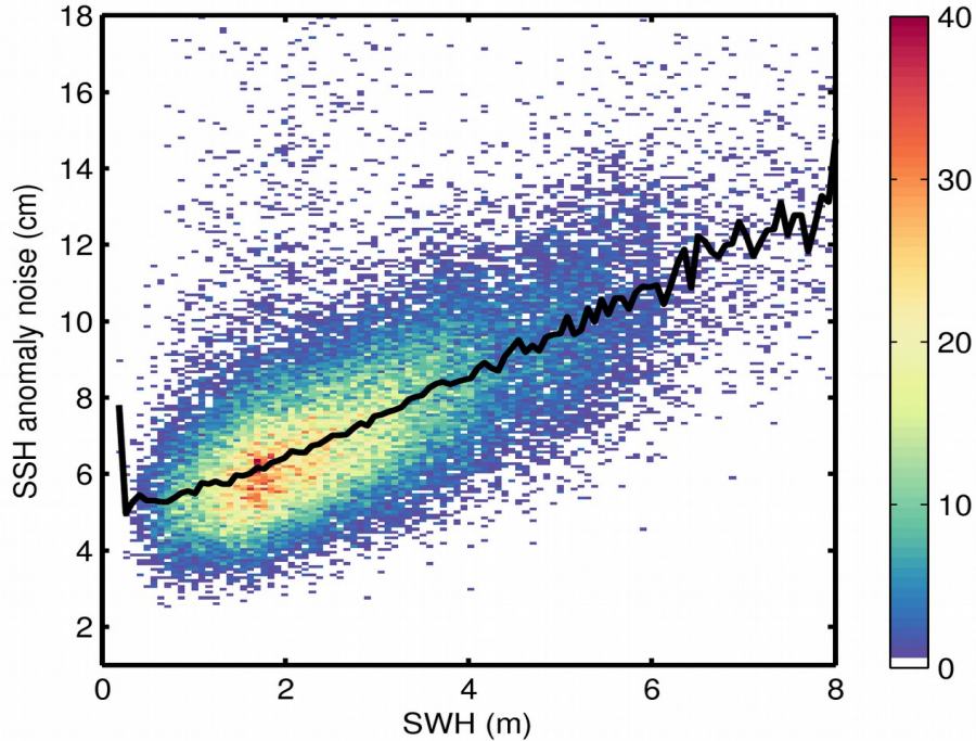
Figure 9. 2D histogram showing flag-valid SSH anomaly noise as a function of SWH for 14/07/2020. The black line denotes the median SSH anomaly noise as a function of SWH.
