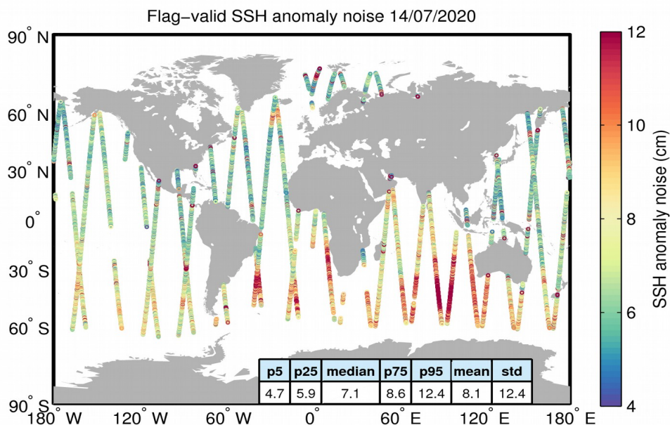
Figure 8. Geographical distribution of flag-valid 20-Hz SSH anomaly measurement noise over oceans and lakes for 14/07/2020. The statistical values shown in the table refer to the SSH anomaly noise and are calculated over all measurements shown in the figure.
