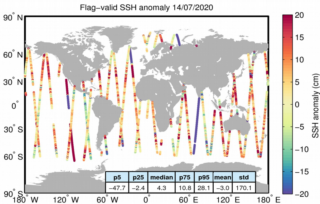
Figure 5. Geographical distribution of flag-valid 1-Hz SSH anomaly data over oceans and lakes for 14/07/2020. The statistical values shown in the table refer to the SSH anomaly in cm and are calculated over all measurements shown in the figure.
