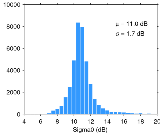
Figure 25. Histogram of flag-valid sigma0 over oceans and lakes for 14/07/2020. The mean ( \mu ) and standard deviation ( \sigma ) are also shown. Note that values outside [4 20] dB are excluded from the histogram for the sake of readability but not from the computation of \mu and \sigma .
