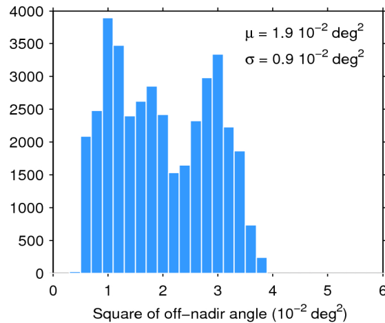
Figure 39. Histogram of flag-valid mispointing over oceans and lakes for 14/07/2020. The mean ( \mu ) and standard deviation ( \sigma ) are also shown. Note that values larger than 6 \cdot 10^{-2} \text{ deg}^2 are excluded from the histogram for the sake of readability but not from the computation of \mu and \sigma .
