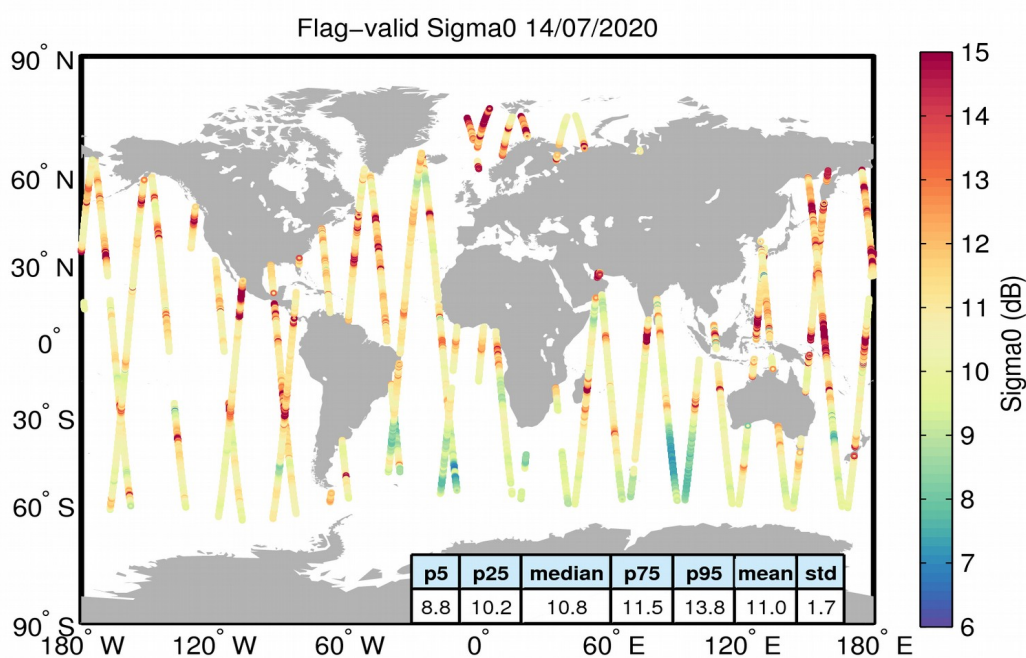
Figure 23. Geographical distribution of flag-valid sigma0 data over oceans and lakes for 14/07/2020. The statistical values shown in the table refer to the sigma0 in dB and are calculated over all measurements shown in the figure.
