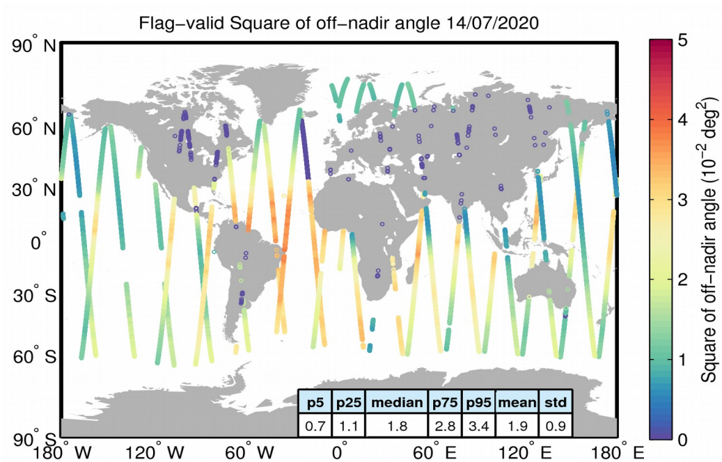
Figure 37. Geographical distribution of flag-valid mispointing data over oceans and lakes for 14/07/2020. The statistical values shown in the table refer to the mispointing in 10^{-2} deg 2 and are calculated over all measurements shown in the figure.
