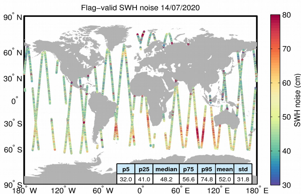
Figure 18. Geographical distribution of flag-valid 20-Hz SWH measurement noise over oceans and lakes for 14/07/2020. The statistical values shown in the table refer to the SWH noise and are calculated over all measurements shown in the figure.
