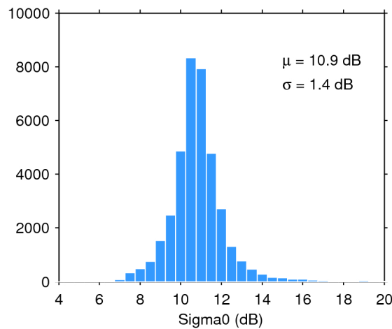
Figure 28. Histogram of science-valid sigma0 over oceans and lakes for 14/07/2020. The mean ( \mu ) and standard deviation ( \sigma ) are also shown. Note that values outside [4 20] dB are excluded from the histogram for the sake of readability but not from the computation of \mu and \sigma .
