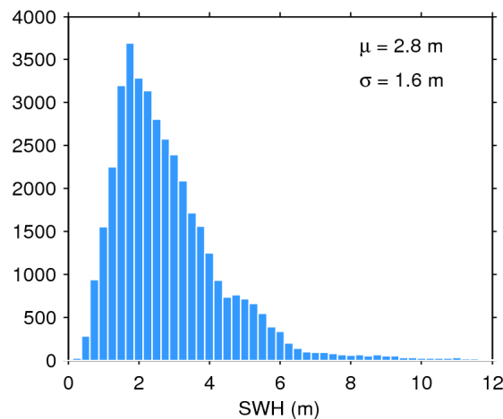
Figure 17. Histogram of flag-valid SWH over oceans and lakes for 14/07/2020. The mean ( \mu ) and standard deviation ( \sigma ) are also shown. Note that values larger than 12 m are excluded from the histogram for the sake of readability but not from the computation of \mu and \sigma .
