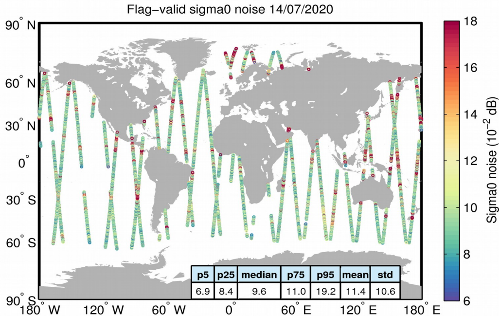
Figure 26. Geographical distribution of flag-valid 20-Hz sigma0 measurement noise over oceans and lakes for 14/07/2020. The statistical values shown in the table refer to the sigma0 noise and are calculated over all measurements shown in the figure.
