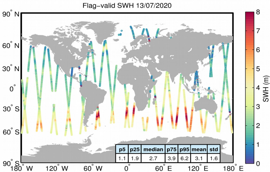
Figure 15. Geographical distribution of flag-valid SWH data over oceans and lakes for 13/07/2020. The statistical values shown in the table refer to the SWH in m and are calculated over all measurements shown in the figure.
