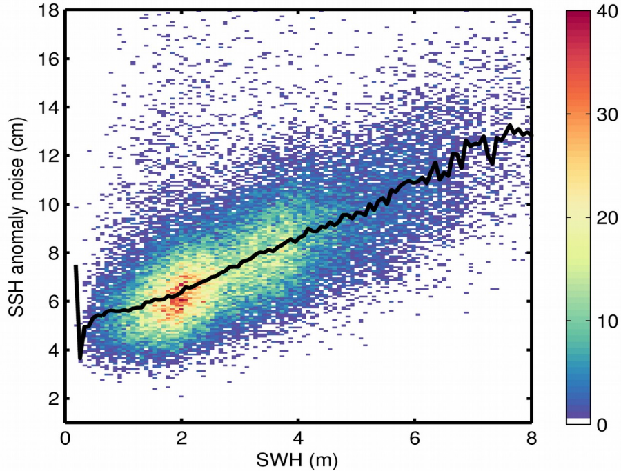
Figure 9. 2D histogram showing flag-valid SSH anomaly noise as a function of SWH for 13/07/2020. The black line denotes the median SSH anomaly noise as a function of SWH.
