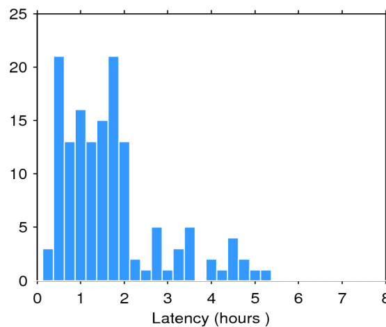
Figure 2. Histogram of the data latency for 13/07/2020. The y-axis denotes the number of files that are made available with a delay of x-hours with respect to the mean time of the records stored in the file.
