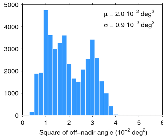
Figure 39. Histogram of flag-valid mispointing over oceans and lakes for 13/07/2020. The mean ( \mu ) and standard deviation ( \sigma ) are also shown. Note that values larger than 6 \cdot 10^{-2} \text{ deg}^2 are excluded from the histogram for the sake of readability but not from the computation of \mu and \sigma .
