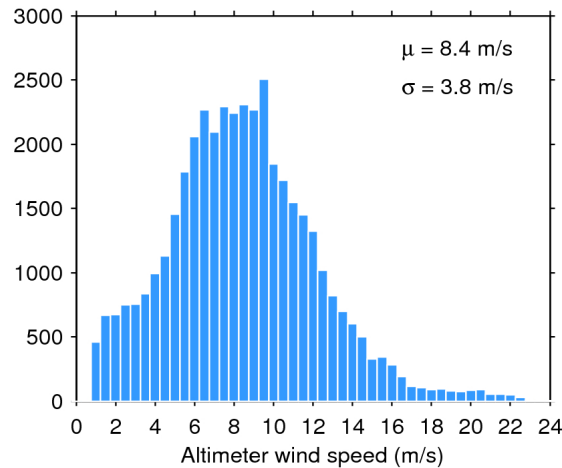
Figure 33. Histogram of flag-valid wind over oceans and lakes for 13/07/2020. The mean ( \mu ) and standard deviation ( \sigma ) are also shown. Note that values larger than 24 m/s are excluded from the histogram for the sake of readability but not from the computation of \mu and \sigma .
