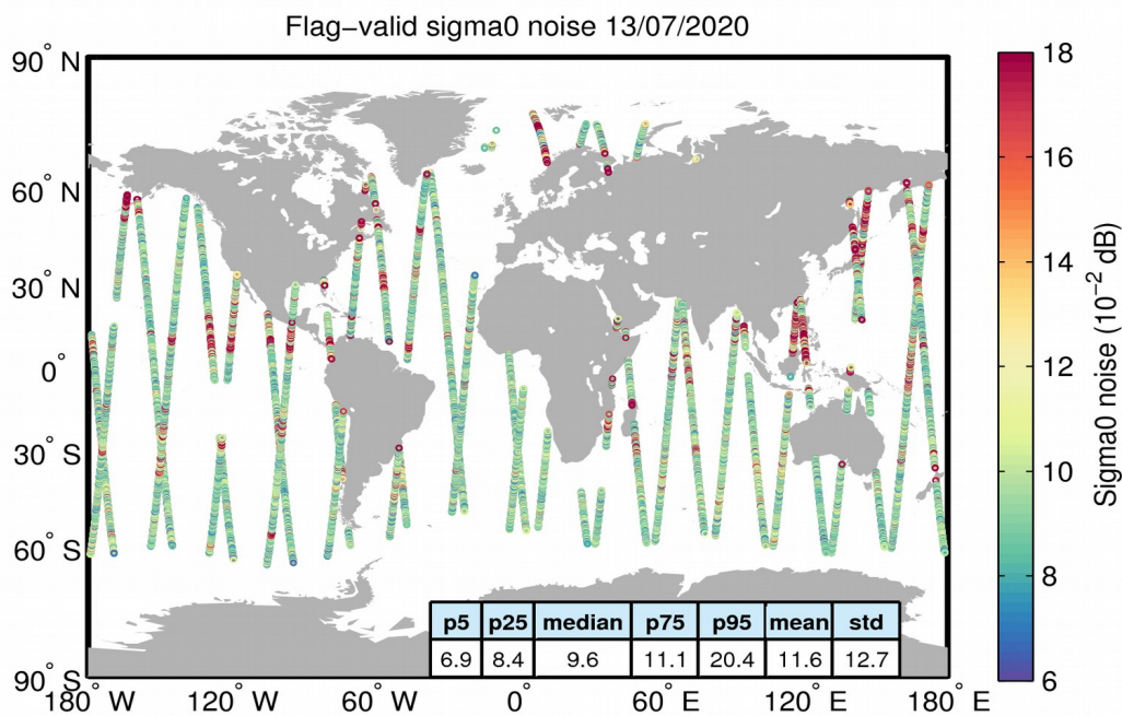
Figure 26. Geographical distribution of flag-valid 20-Hz sigma0 measurement noise over oceans and lakes for 13/07/2020. The statistical values shown in the table refer to the sigma0 noise and are calculated over all measurements shown in the figure.
