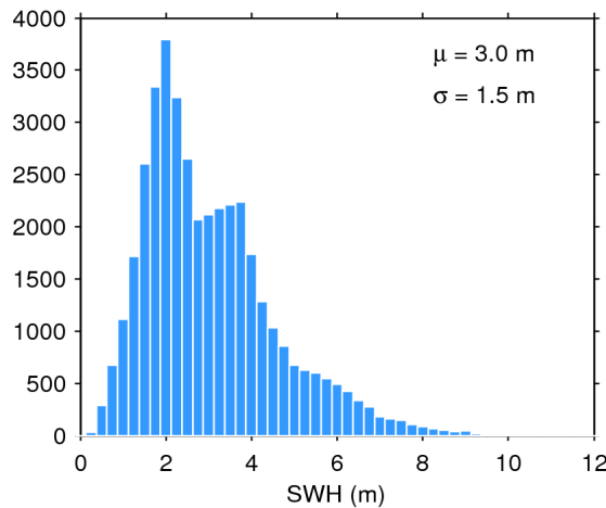
Figure 20. Histogram of science-valid SWH over oceans and lakes for 13/07/2020. The mean ( \mu ) and standard deviation ( \sigma ) are also shown. Note that values larger than 12 m are excluded from the histogram for the sake of readability but not from the computation of \mu and \sigma .
