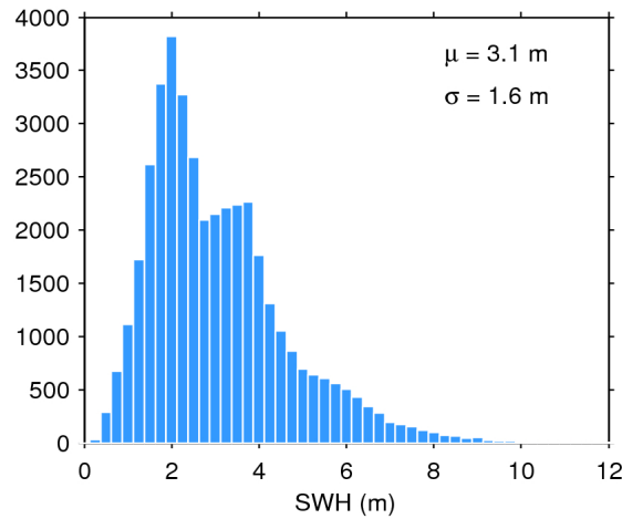
Figure 17. Histogram of flag-valid SWH over oceans and lakes for 13/07/2020. The mean ( \mu ) and standard deviation ( \sigma ) are also shown. Note that values larger than 12 m are excluded from the histogram for the sake of readability but not from the computation of \mu and \sigma .
