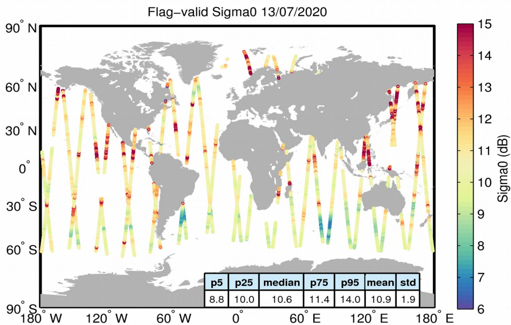
Figure 23. Geographical distribution of flag-valid sigma0 data over oceans and lakes for 13/07/2020. The statistical values shown in the table refer to the sigma0 in dB and are calculated over all measurements shown in the figure.
