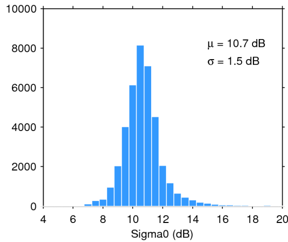
Figure 28. Histogram of science-valid sigma0 over oceans and lakes for 13/07/2020. The mean ( \mu ) and standard deviation ( \sigma ) are also shown. Note that values outside [4 20] dB are excluded from the histogram for the sake of readability but not from the computation of \mu and \sigma .
