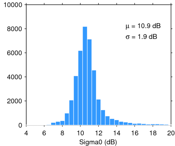
Figure 25. Histogram of flag-valid sigma0 over oceans and lakes for 13/07/2020. The mean ( \mu ) and standard deviation ( \sigma ) are also shown. Note that values outside [4 20] dB are excluded from the histogram for the sake of readability but not from the computation of \mu and \sigma .
