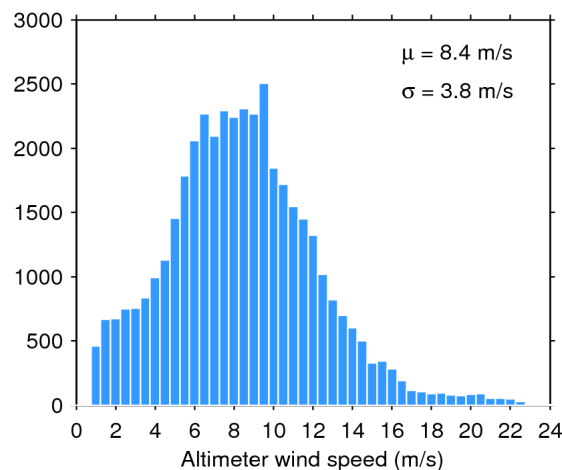
Figure 35. Histogram of science-valid wind over oceans and lakes for 13/07/2020. The mean ( \mu ) and standard deviation ( \sigma ) are also shown. Note that values larger than 24 m/s are excluded from the histogram for the sake of readability but not from the computation of \mu and \sigma .
