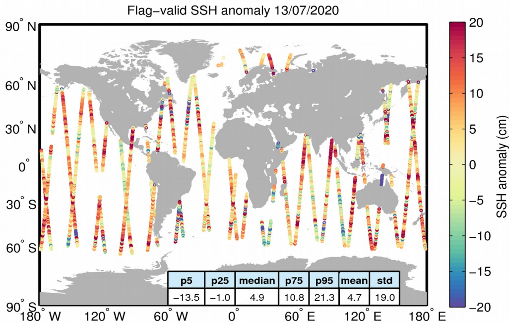
Figure 5. Geographical distribution of flag-valid 1-Hz SSH anomaly data over oceans and lakes for 13/07/2020. The statistical values shown in the table refer to the SSH anomaly in cm and are calculated over all measurements shown in the figure.
