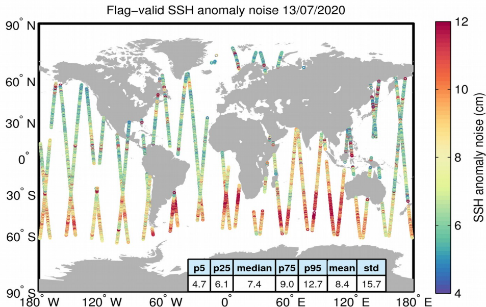
Figure 8. Geographical distribution of flag-valid 20-Hz SSH anomaly measurement noise over oceans and lakes for 13/07/2020. The statistical values shown in the table refer to the SSH anomaly noise and are calculated over all measurements shown in the figure.
