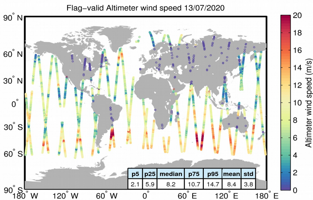
Figure 31. Geographical distribution of flag-valid wind data over oceans and lakes for 13/07/2020. The statistical values shown in the table refer to the wind in m/s and are calculated over all measurements shown in the figure.
