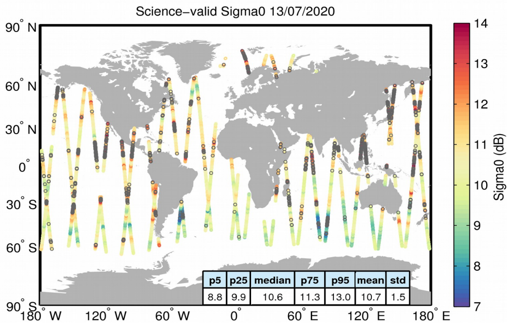
Figure 27. Geographical distribution of science-valid sigma0 data over oceans and lakes for 13/07/2020. The statistical values shown in the table refer to the sigma0 in dB and are calculated over all measurements shown in the figure. Gray circles denote records that have been rejected based on the editing criteria described in Table 4.
