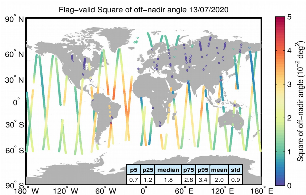
Figure 37. Geographical distribution of flag-valid mispointing data over oceans and lakes for 13/07/2020. The statistical values shown in the table refer to the mispointing in 10^{-2} \text{ deg}^2 and are calculated over all measurements shown in the figure.
