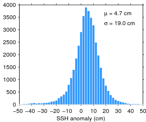
Figure 7. Histogram of flag-valid SSH anomaly over oceans and lakes for 13/07/2020. The mean ( \mu ) and standard deviation ( \sigma ) are also shown. Note that values outside [-50 50] cm are excluded from the histogram for the sake of readability but not from the computation of \mu and \sigma .
