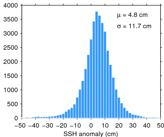
Figure 11. Histogram of science-valid SSH anomaly over oceans and lakes for 13/07/2020. The mean ( \mu ) and standard deviation ( \sigma ) are also shown. Note that values outside [-50 50] cm are excluded from the histogram for the sake of readability but not from the computation of \mu and \sigma .
