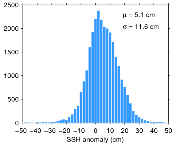
Figure 11. Histogram of science-valid SSH anomaly over oceans and lakes for 08/07/2020. The mean ( \mu ) and standard deviation ( \sigma ) are also shown. Note that values outside [-50 50] cm are excluded from the histogram for the sake of readability but not from the computation of \mu and \sigma .
