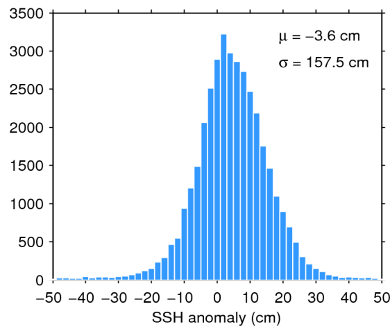
Figure 7. Histogram of flag-valid SSH anomaly over oceans and lakes for 08/07/2020. The mean ( \mu ) and standard deviation ( \sigma ) are also shown. Note that values outside [-50 50] cm are excluded from the histogram for the sake of readability but not from the computation of \mu and \sigma .
