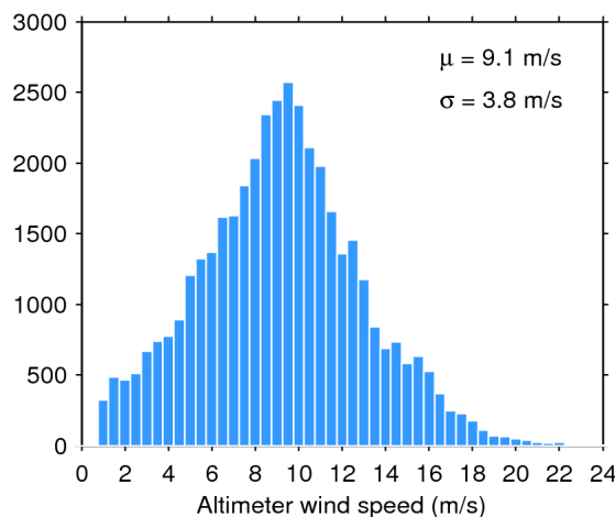
Figure 35. Histogram of science-valid wind over oceans and lakes for 08/07/2020. The mean ( \mu ) and standard deviation ( \sigma ) are also shown. Note that values larger than 24 m/s are excluded from the histogram for the sake of readability but not from the computation of \mu and \sigma .
