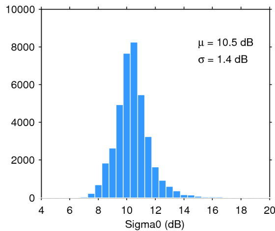
Figure 28. Histogram of science-valid sigma0 over oceans and lakes for 08/07/2020. The mean ( \mu ) and standard deviation ( \sigma ) are also shown. Note that values outside [4 20] dB are excluded from the histogram for the sake of readability but not from the computation of \mu and \sigma .
