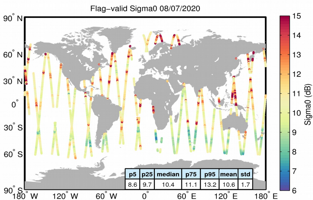
Figure 23. Geographical distribution of flag-valid sigma0 data over oceans and lakes for 08/07/2020. The statistical values shown in the table refer to the sigma0 in dB and are calculated over all measurements shown in the figure.
