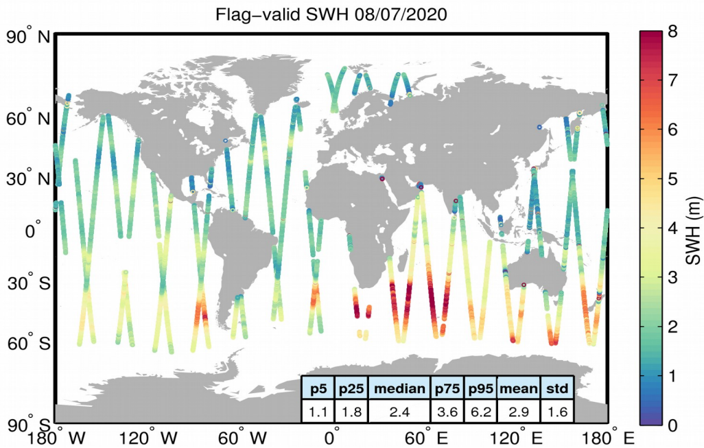
Figure 15. Geographical distribution of flag-valid SWH data over oceans and lakes for 08/07/2020. The statistical values shown in the table refer to the SWH in m and are calculated over all measurements shown in the figure.
