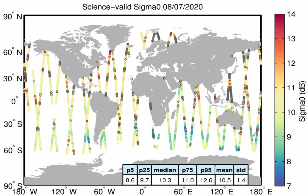
Figure 27. Geographical distribution of science-valid sigma0 data over oceans and lakes for 08/07/2020. The statistical values shown in the table refer to the sigma0 in dB and are calculated over all measurements shown in the figure. Gray circles denote records that have been rejected based on the editing criteria described in Table 4.
