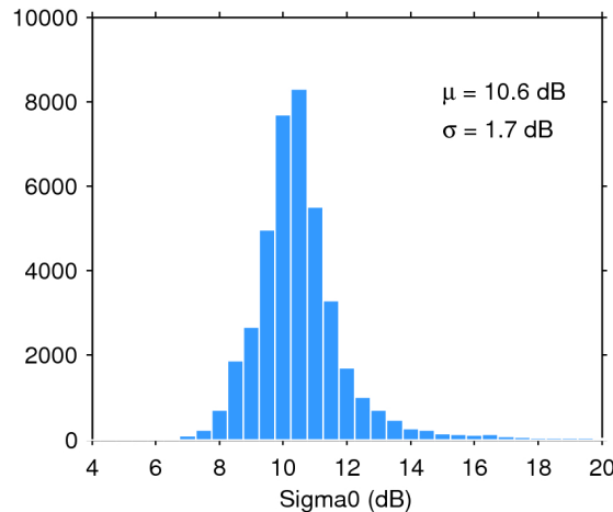
Figure 25. Histogram of flag-valid sigma0 over oceans and lakes for 08/07/2020. The mean ( \mu ) and standard deviation ( \sigma ) are also shown. Note that values outside [4 20] dB are excluded from the histogram for the sake of readability but not from the computation of \mu and \sigma .
