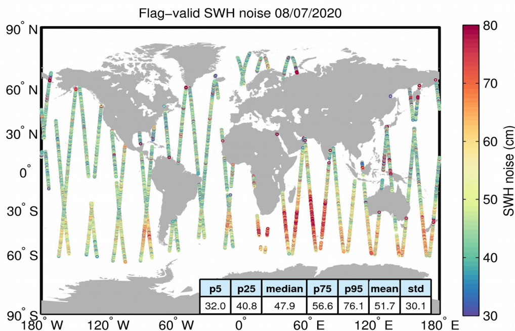
Figure 18. Geographical distribution of flag-valid 20-Hz SWH measurement noise over oceans and lakes for 08/07/2020. The statistical values shown in the figure refer to the SWH noise and are calculated over all measurements shown in the figure.
