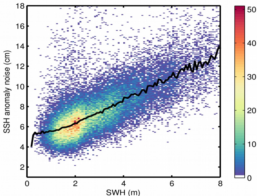
Figure 9. 2D histogram showing flag-valid SSH anomaly noise as a function of SWH for 08/07/2020. The black line denotes the median SSH anomaly noise as a function of SWH.
