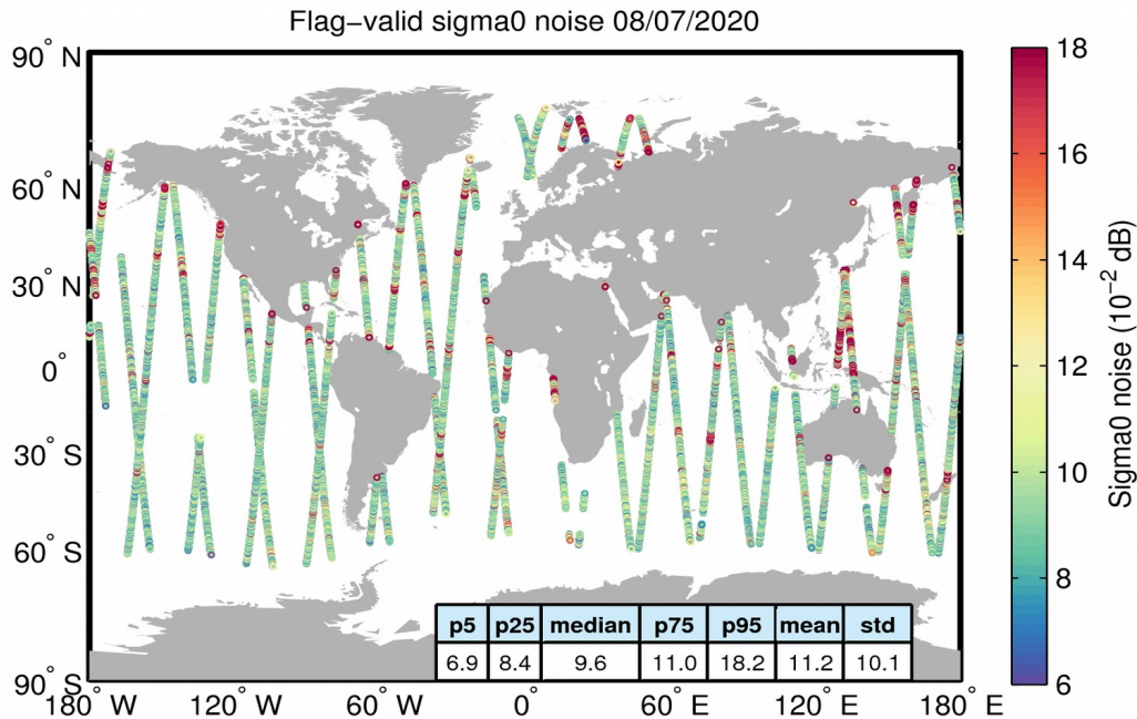
Figure 26. Geographical distribution of flag-valid 20-Hz sigma0 measurement noise over oceans and lakes for 08/07/2020. The statistical values shown in the table refer to the sigma0 noise and are calculated over all measurements shown in the figure.
