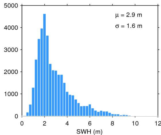
Figure 17. Histogram of flag-valid SWH over oceans and lakes for 08/07/2020. The mean ( \mu ) and standard deviation ( \sigma ) are also shown. Note that values larger than 12 m are excluded from the histogram for the sake of readability but not from the computation of \mu and \sigma .
