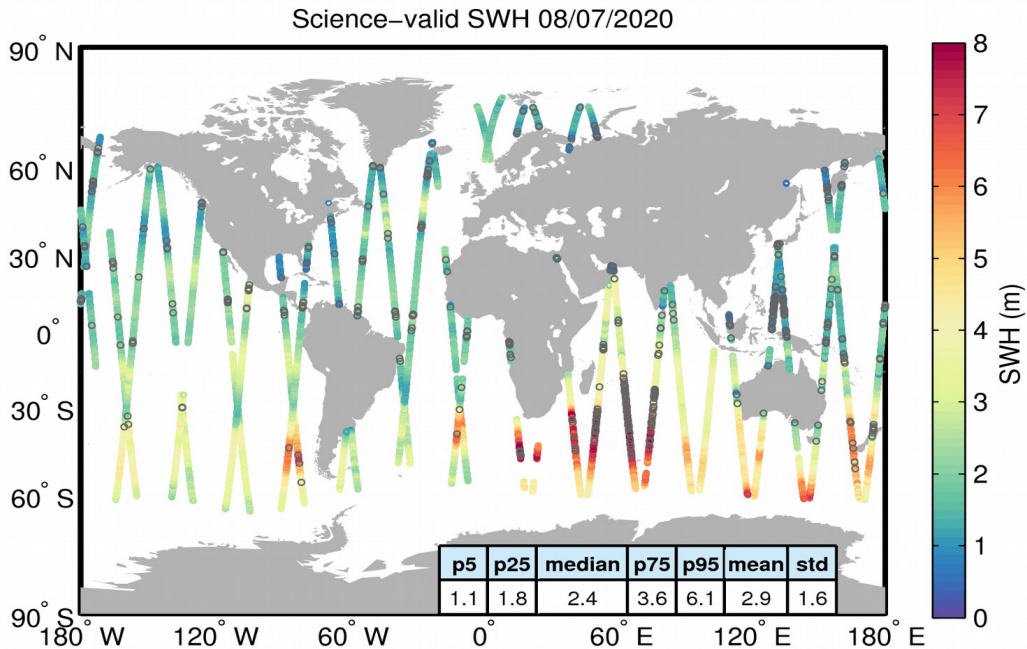
Figure 19. Geographical distribution of science-valid SWH data over oceans and lakes for 08/07/2020. The statistical values shown in the table refer to the SWH in m and are calculated over all measurements shown in the figure. Gray circles denote records that have been rejected based on the editing criteria described in Table 3.
