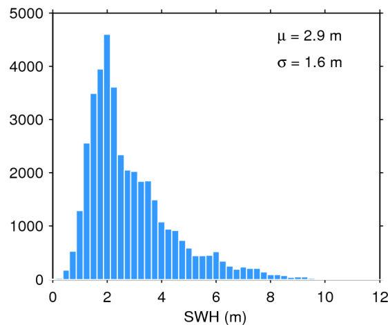
Figure 20. Histogram of science-valid SWH over oceans and lakes for 08/07/2020. The mean ( \mu ) and standard deviation ( \sigma ) are also shown. Note that values larger than 12 m are excluded from the histogram for the sake of readability but not from the computation of \mu and \sigma .
