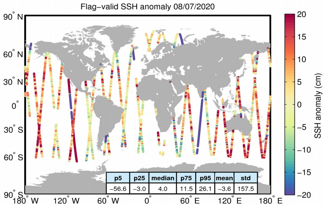
Figure 5. Geographical distribution of flag-valid 1-Hz SSH anomaly data over oceans and lakes for 08/07/2020. The statistical values shown in the table refer to the SSH anomaly in cm and are calculated over all measurements shown in the figure.
