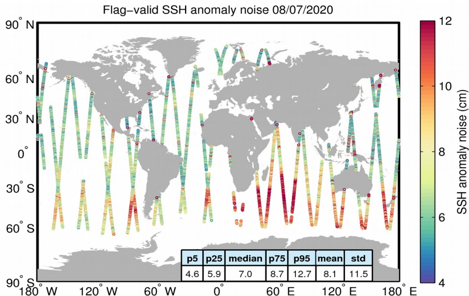
Figure 8. Geographical distribution of flag-valid 20-Hz SSH anomaly measurement noise over oceans and lakes for 08/07/2020. The statistical values shown in the table refer to the SSH anomaly noise and are calculated over all measurements shown in the figure.
