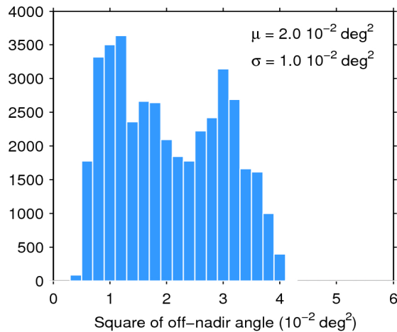
Figure 39. Histogram of flag-valid mispointing over oceans and lakes for 08/07/2020. The mean ( \mu ) and standard deviation ( \sigma ) are also shown. Note that values larger than 6 \cdot 10^{-2} \text{ deg}^2 are excluded from the histogram for the sake of readability but not from the computation of \mu and \sigma .
