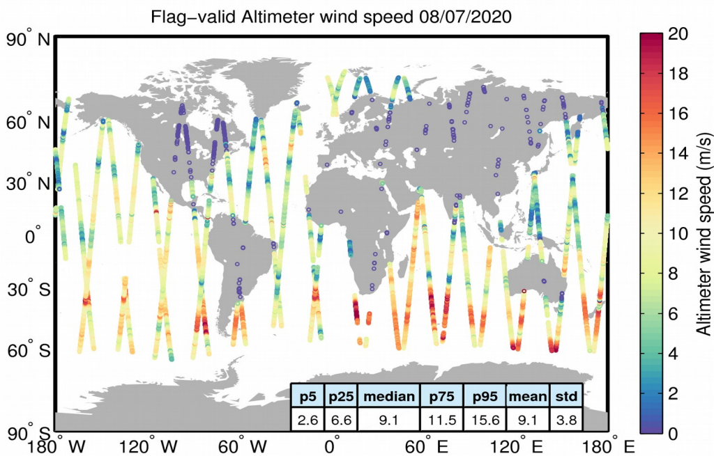
Figure 31. Geographical distribution of flag-valid wind data over oceans and lakes for 08/07/2020. The statistical values shown in the figure refer to the wind in m/s and are calculated over all measurements shown in the figure.
