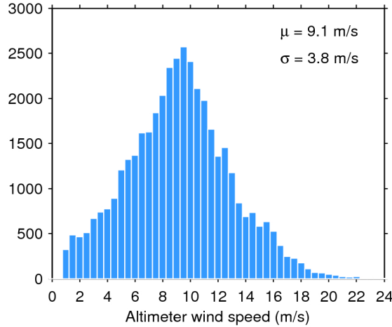
Figure 33. Histogram of flag-valid wind over oceans and lakes for 08/07/2020. The mean ( \mu ) and standard deviation ( \sigma ) are also shown. Note that values larger than 24 m/s are excluded from the histogram for the sake of readability but not from the computation of \mu and \sigma .
