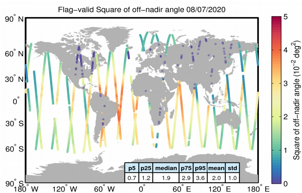
Figure 37. Geographical distribution of flag-valid mispointing data over oceans and lakes for 08/07/2020. The statistical values shown in the table refer to the mispointing in 10^{-2} \text{ deg}^2 and are calculated over all measurements shown in the figure.
