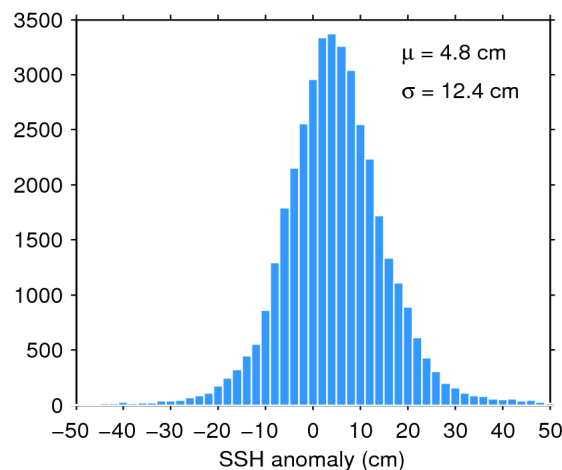
Figure 11. Histogram of science-valid SSH anomaly over oceans and lakes for 07/07/2020. The mean ( \mu ) and standard deviation ( \sigma ) are also shown. Note that values outside [-50 50] cm are excluded from the histogram for the sake of readability but not from the computation of \mu and \sigma .
