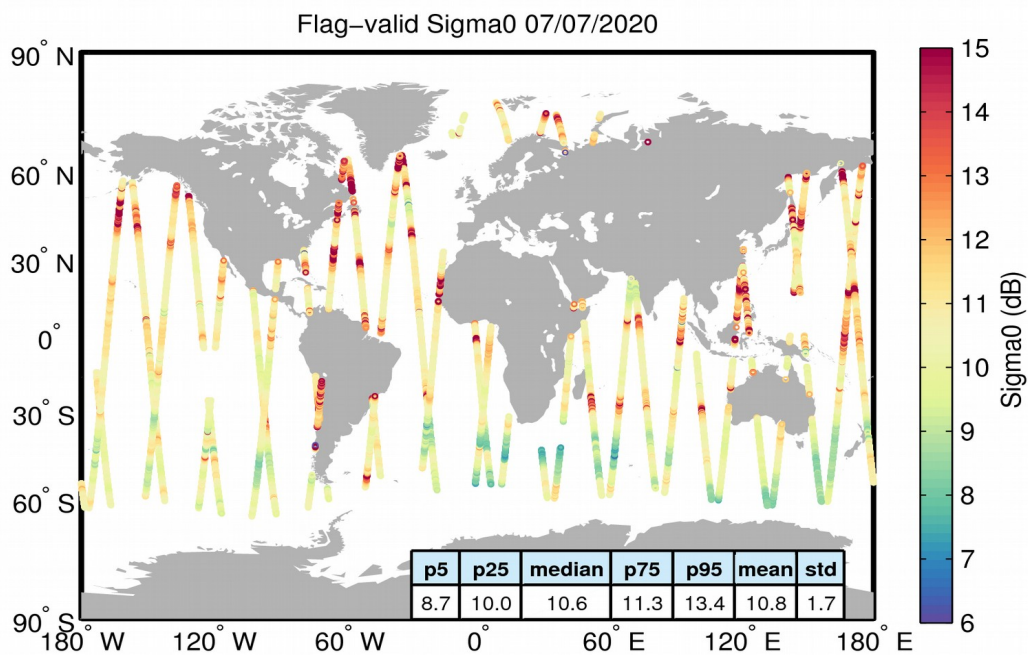
Figure 23. Geographical distribution of flag-valid sigma0 data over oceans and lakes for 07/07/2020. The statistical values shown in the table refer to the sigma0 in dB and are calculated over all measurements shown in the figure.
