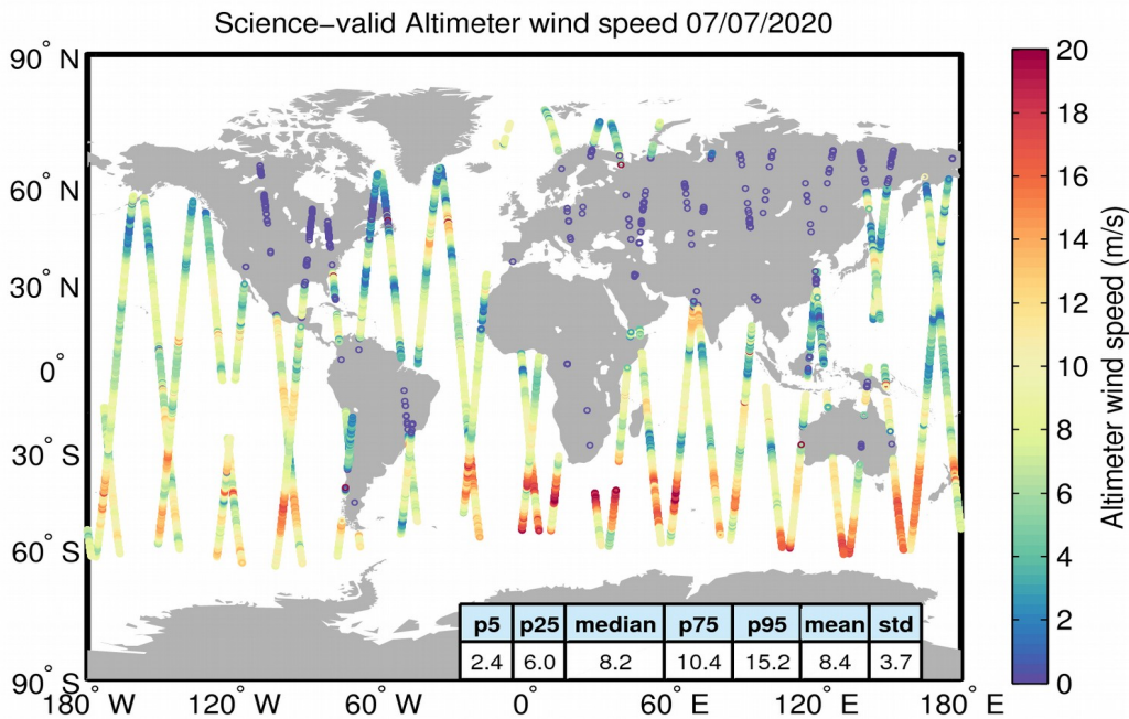
Figure 34. Geographical distribution of science-valid wind data over oceans and lakes for 07/07/2020. The statistical values shown in the table refer to the wind in m/s and are calculated over all measurements shown in the figure. Gray circles denote records that have been rejected based on the editing criteria described in Table 5.
