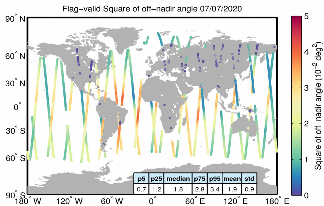
Figure 37. Geographical distribution of flag-valid mispointing data over oceans and lakes for 07/07/2020. The statistical values shown in the table refer to the mispointing in 10^{-2} \text{ deg}^2 and are calculated over all measurements shown in the figure.
