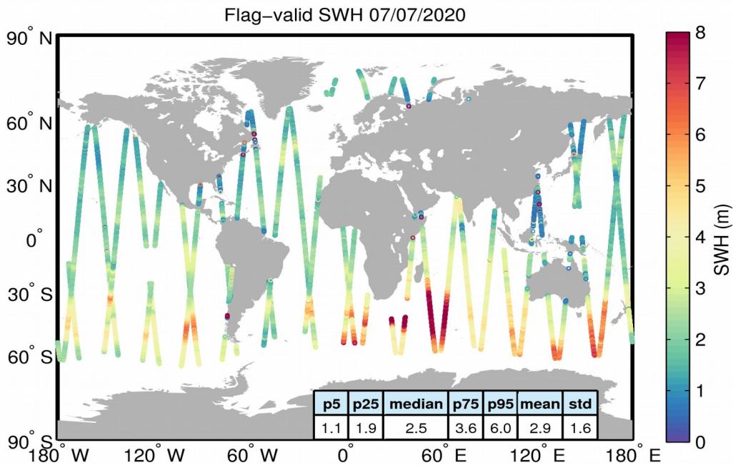
Figure 15. Geographical distribution of flag-valid SWH data over oceans and lakes for 07/07/2020. The statistical values shown in the table refer to the SWH in m and are calculated over all measurements shown in the figure.
