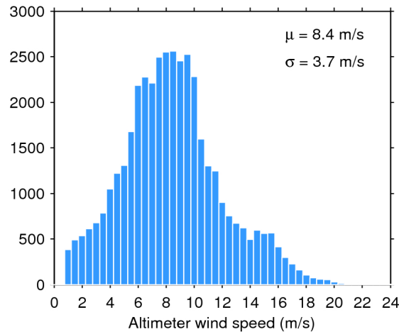
Figure 33. Histogram of flag-valid wind over oceans and lakes for 07/07/2020. The mean ( \mu ) and standard deviation ( \sigma ) are also shown. Note that values larger than 24 m/s are excluded from the histogram for the sake of readability but not from the computation of \mu and \sigma .
