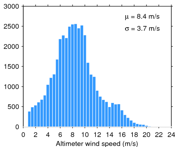
Figure 35. Histogram of science-valid wind over oceans and lakes for 07/07/2020. The mean ( \mu ) and standard deviation ( \sigma ) are also shown. Note that values larger than 24 m/s are excluded from the histogram for the sake of readability but not from the computation of \mu and \sigma .
