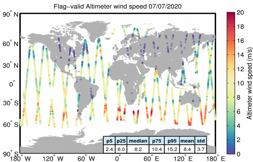
Figure 31. Geographical distribution of flag-valid wind data over oceans and lakes for 07/07/2020. The statistical values shown in the table refer to the wind in m/s and are calculated over all measurements shown in the figure.
