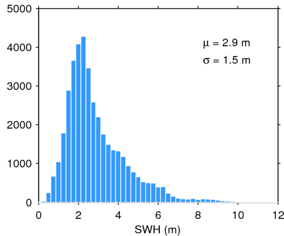
Figure 20. Histogram of science-valid SWH over oceans and lakes for 07/07/2020. The mean ( \mu ) and standard deviation ( \sigma ) are also shown. Note that values larger than 12 m are excluded from the histogram for the sake of readability but not from the computation of \mu and \sigma .
