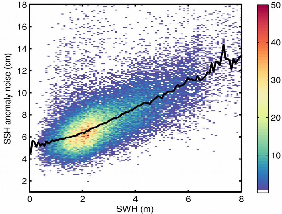
Figure 9. 2D histogram showing flag-valid SSH anomaly noise as a function of SWH for 07/07/2020. The black line denotes the median SSH anomaly noise as a function of SWH.
