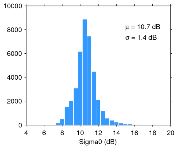
Figure 28. Histogram of science-valid sigma0 over oceans and lakes for 07/07/2020. The mean ( \mu ) and standard deviation ( \sigma ) are also shown. Note that values outside [4 20] dB are excluded from the histogram for the sake of readability but not from the computation of \mu and \sigma .
