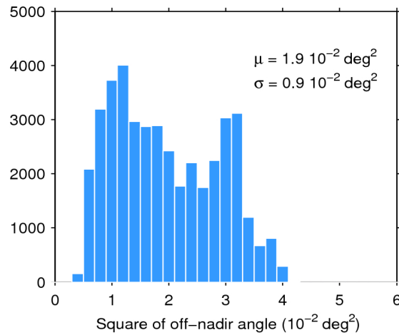
Figure 39. Histogram of flag-valid mispointing over oceans and lakes for 07/07/2020. The mean ( \mu ) and standard deviation ( \sigma ) are also shown. Note that values larger than 6 \cdot 10^{-2} \text{ deg}^2 are excluded from the histogram for the sake of readability but not from the computation of \mu and \sigma .
