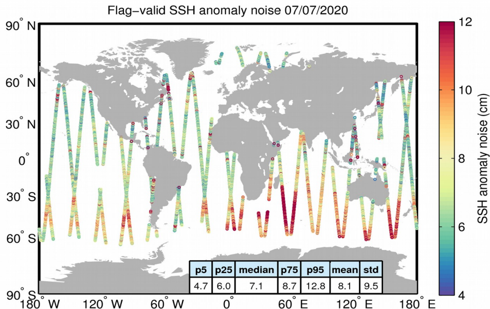
Figure 8. Geographical distribution of flag-valid 20-Hz SSH anomaly measurement noise over oceans and lakes for 07/07/2020. The statistical values shown in the table refer to the SSH anomaly noise and are calculated over all measurements shown in the figure.
