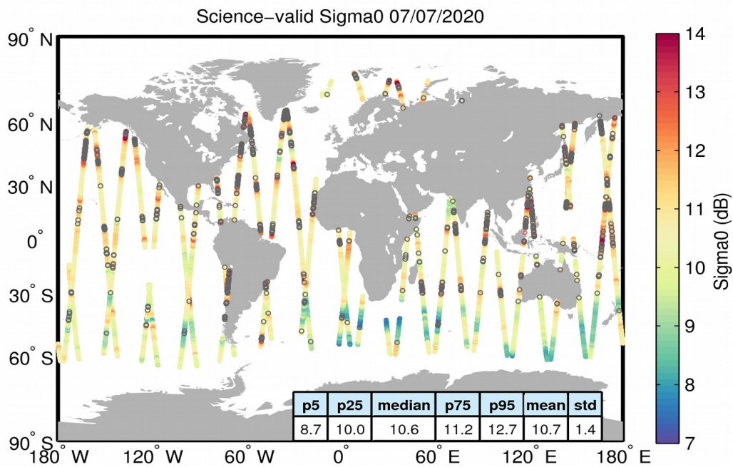
Figure 27. Geographical distribution of science-valid sigma0 data over oceans and lakes for 07/07/2020. The statistical values shown in the table refer to the sigma0 in dB and are calculated over all measurements shown in the figure. Gray circles denote records that have been rejected based on the editing criteria described in Table 4.
