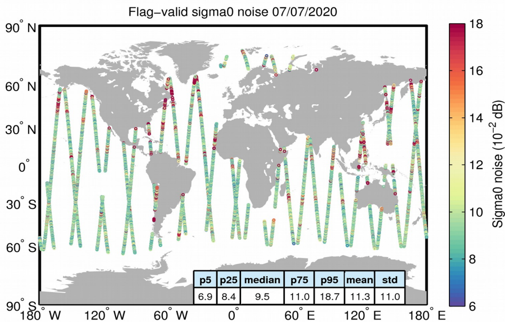
Figure 26. Geographical distribution of flag-valid 20-Hz sigma0 measurement noise over oceans and lakes for 07/07/2020. The statistical values shown in the table refer to the sigma0 noise and are calculated over all measurements shown in the figure.
