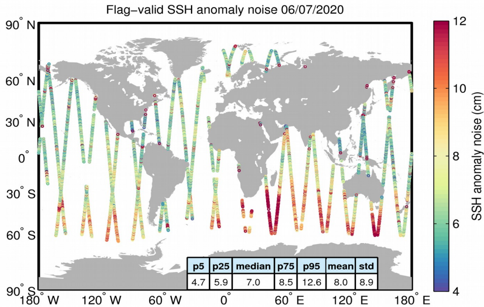
Figure 8. Geographical distribution of flag-valid 20-Hz SSH anomaly measurement noise over oceans and lakes for 06/07/2020. The statistical values shown in the table refer to the SSH anomaly noise and are calculated over all measurements shown in the figure.
