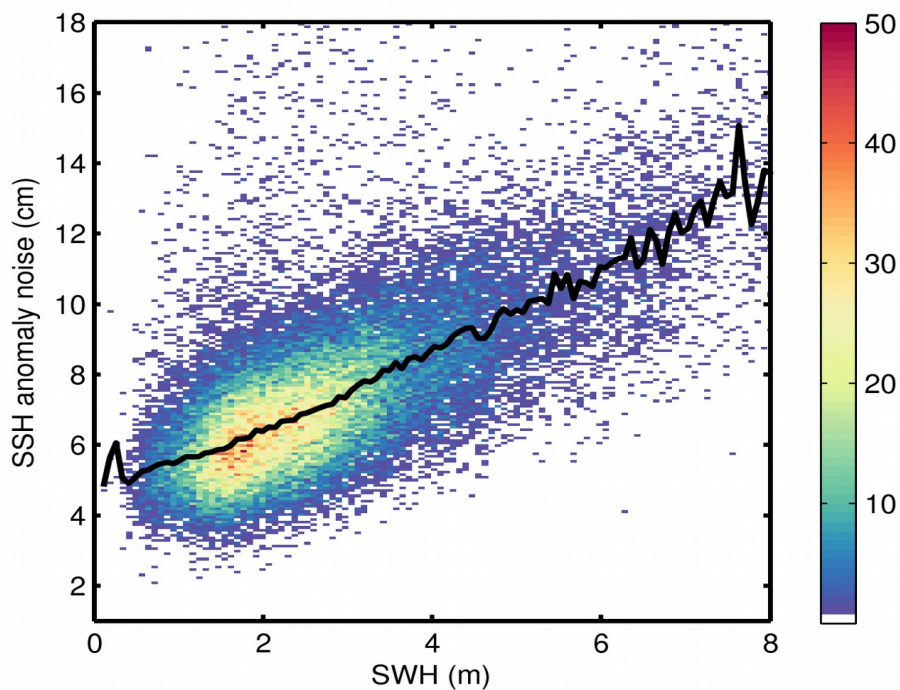
Figure 9. 2D histogram showing flag-valid SSH anomaly noise as a function of SWH for 06/07/2020. The black line denotes the median SSH anomaly noise as a function of SWH.
