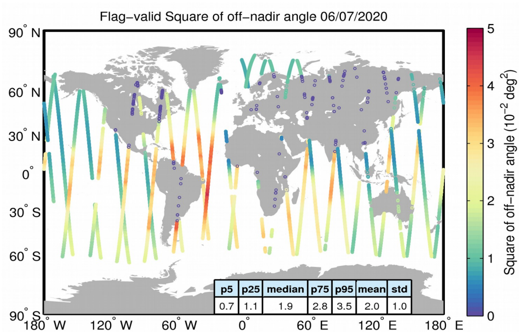
Figure 37. Geographical distribution of flag-valid mispointing data over oceans and lakes for 06/07/2020. The statistical values shown in the table refer to the mispointing in 10^{-2} \text{ deg}^2 and are calculated over all measurements shown in the figure.
