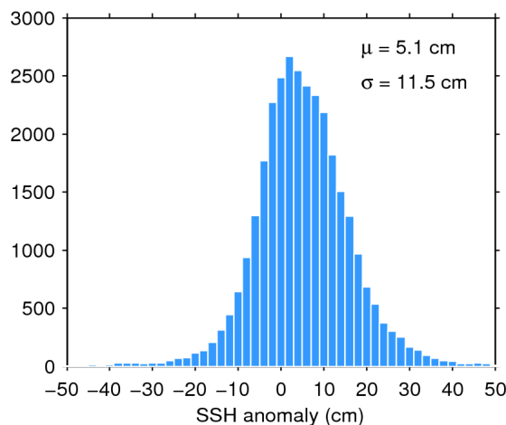
Figure 11. Histogram of science-valid SSH anomaly over oceans and lakes for 06/07/2020. The mean ( \mu ) and standard deviation ( \sigma ) are also shown. Note that values outside [-50 50] cm are excluded from the histogram for the sake of readability but not from the computation of \mu and \sigma .
