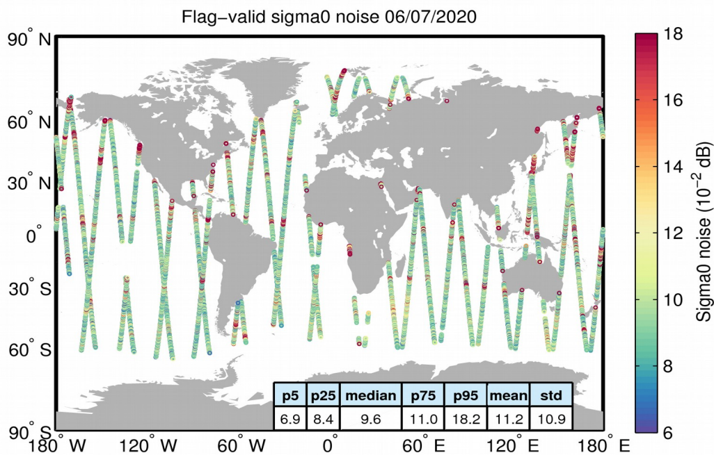
Figure 26. Geographical distribution of flag-valid 20-Hz sigma0 measurement noise over oceans and lakes for 06/07/2020. The statistical values shown in the table refer to the sigma0 noise and are calculated over all measurements shown in the figure.
