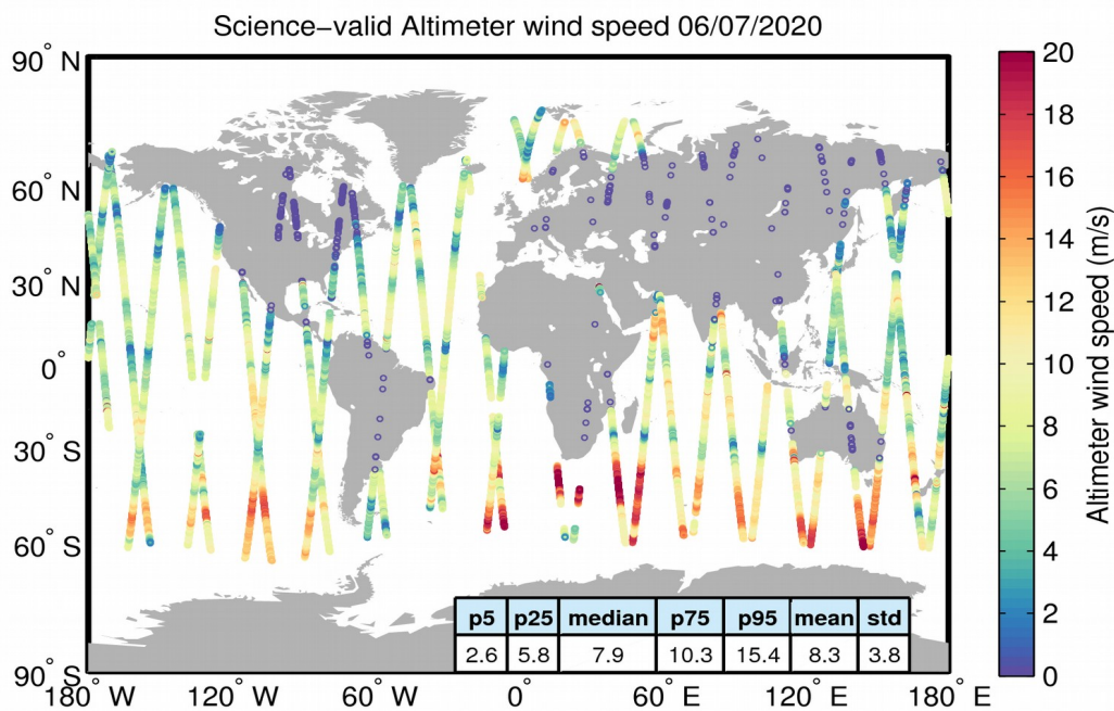
Figure 34. Geographical distribution of science-valid wind data over oceans and lakes for 06/07/2020. The statistical values shown in the table refer to the wind in m/s and are calculated over all measurements shown in the figure. Gray circles denote records that have been rejected based on the editing criteria described in Table 5.
