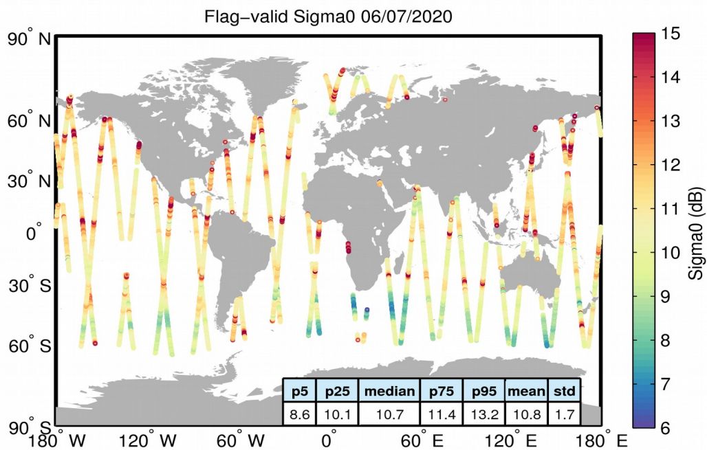
Figure 23. Geographical distribution of flag-valid sigma0 data over oceans and lakes for 06/07/2020. The statistical values shown in the table refer to the sigma0 in dB and are calculated over all measurements shown in the figure.
