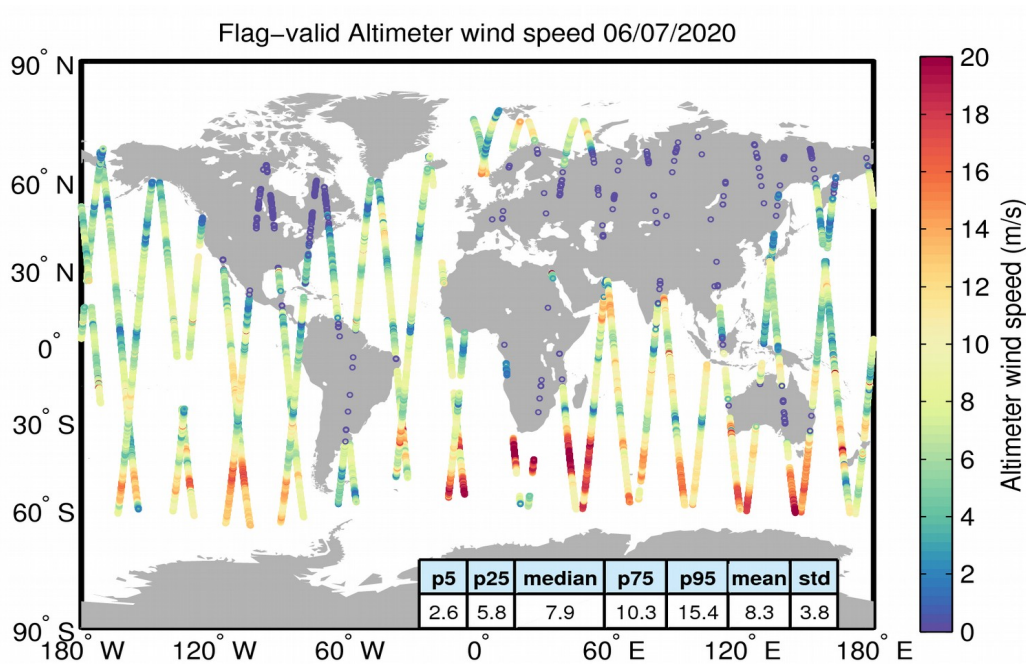
Figure 31. Geographical distribution of flag-valid wind data over oceans and lakes for 06/07/2020. The statistical values shown in the table refer to the wind in m/s and are calculated over all measurements shown in the figure.
