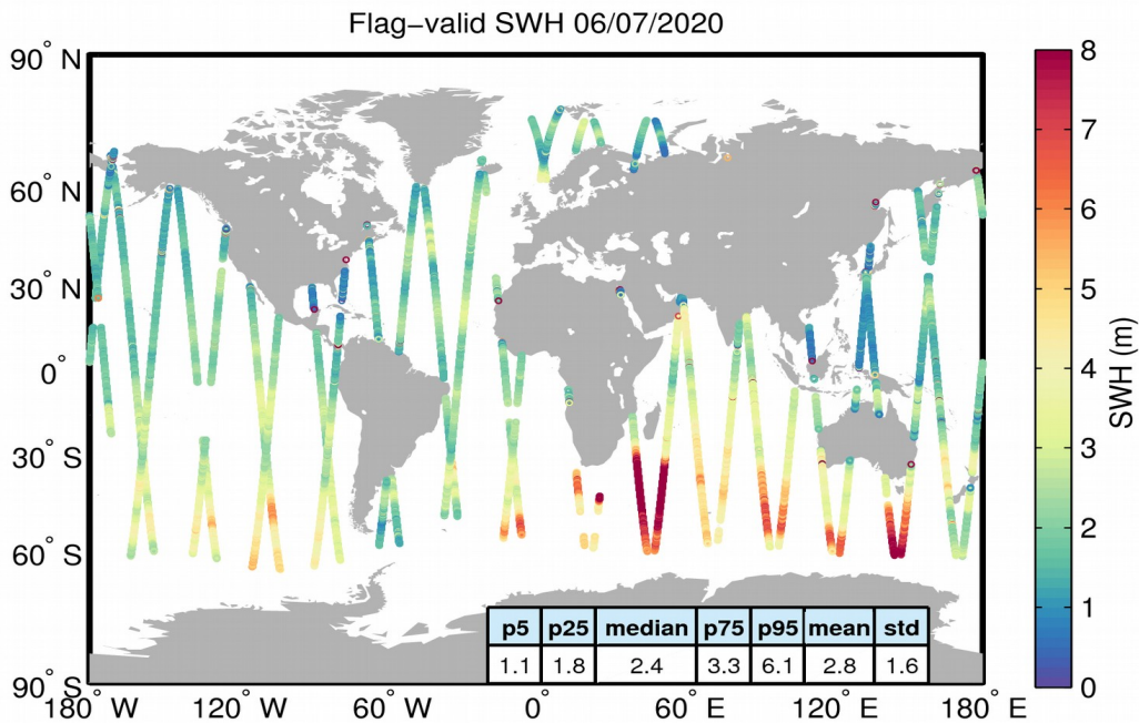
Figure 15. Geographical distribution of flag-valid SWH data over oceans and lakes for 06/07/2020. The statistical values shown in the table refer to the SWH in m and are calculated over all measurements shown in the figure.
