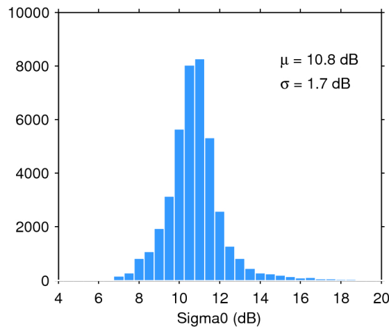
Figure 25. Histogram of flag-valid sigma0 over oceans and lakes for 06/07/2020. The mean ( \mu ) and standard deviation ( \sigma ) are also shown. Note that values outside [4 20] dB are excluded from the histogram for the sake of readability but not from the computation of \mu and \sigma .
