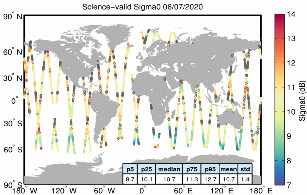
Figure 27. Geographical distribution of science-valid sigma0 data over oceans and lakes for 06/07/2020. The statistical values shown in the table refer to the sigma0 in dB and are calculated over all measurements shown in the figure. Gray circles denote records that have been rejected based on the editing criteria described in Table 4.
