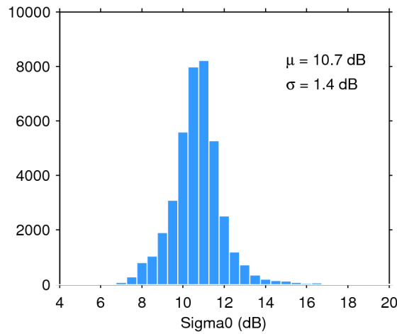
Figure 28. Histogram of science-valid sigma0 over oceans and lakes for 06/07/2020. The mean ( \mu ) and standard deviation ( \sigma ) are also shown. Note that values outside [4 20] dB are excluded from the histogram for the sake of readability but not from the computation of \mu and \sigma .
