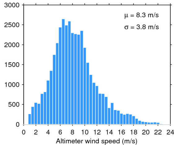
Figure 33. Histogram of flag-valid wind over oceans and lakes for 06/07/2020. The mean ( \mu ) and standard deviation ( \sigma ) are also shown. Note that values larger than 24 m/s are excluded from the histogram for the sake of readability but not from the computation of \mu and \sigma .
