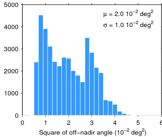
Figure 39. Histogram of flag-valid mispointing over oceans and lakes for 06/07/2020. The mean ( \mu ) and standard deviation ( \sigma ) are also shown. Note that values larger than 6 \cdot 10^{-2} \text{ deg}^2 are excluded from the histogram for the sake of readability but not from the computation of \mu and \sigma .
