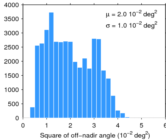
Figure 39. Histogram of flag-valid mispointing over oceans and lakes for 05/07/2020. The mean ( \mu ) and standard deviation ( \sigma ) are also shown. Note that values larger than 6 \cdot 10^{-2} \text{ deg}^2 are excluded from the histogram for the sake of readability but not from the computation of \mu and \sigma .
