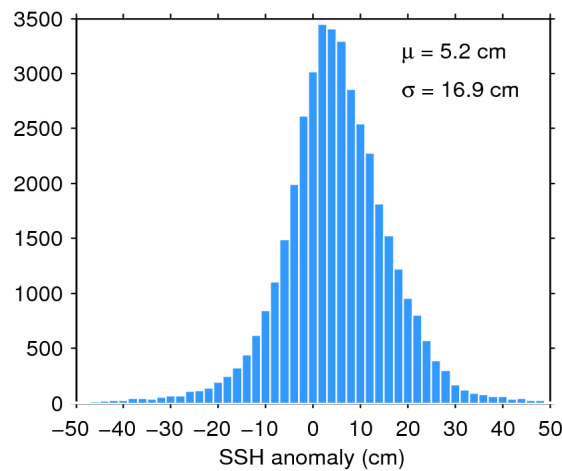
Figure 7. Histogram of flag-valid SSH anomaly over oceans and lakes for 05/07/2020. The mean ( \mu ) and standard deviation ( \sigma ) are also shown. Note that values outside [-50\ 50] cm are excluded from the histogram for the sake of readability but not from the computation of \mu and \sigma .
