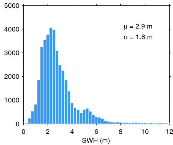
Figure 17. Histogram of flag-valid SWH over oceans and lakes for 05/07/2020. The mean ( \mu ) and standard deviation ( \sigma ) are also shown. Note that values larger than 12 m are excluded from the histogram for the sake of readability but not from the computation of \mu and \sigma .
