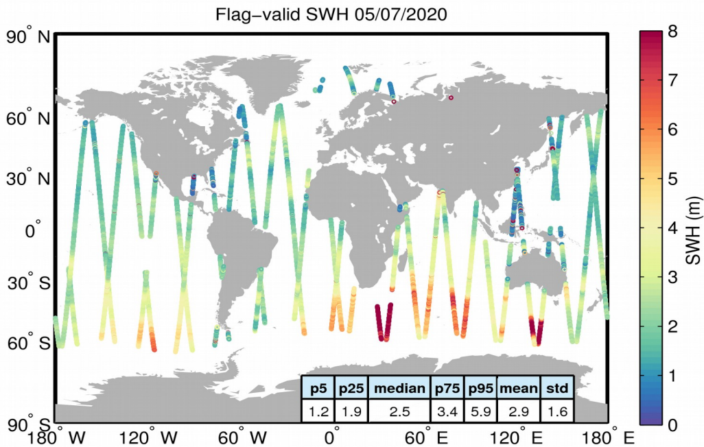
Figure 15. Geographical distribution of flag-valid SWH data over oceans and lakes for 05/07/2020. The statistical values shown in the table refer to the SWH in m and are calculated over all measurements shown in the figure.
