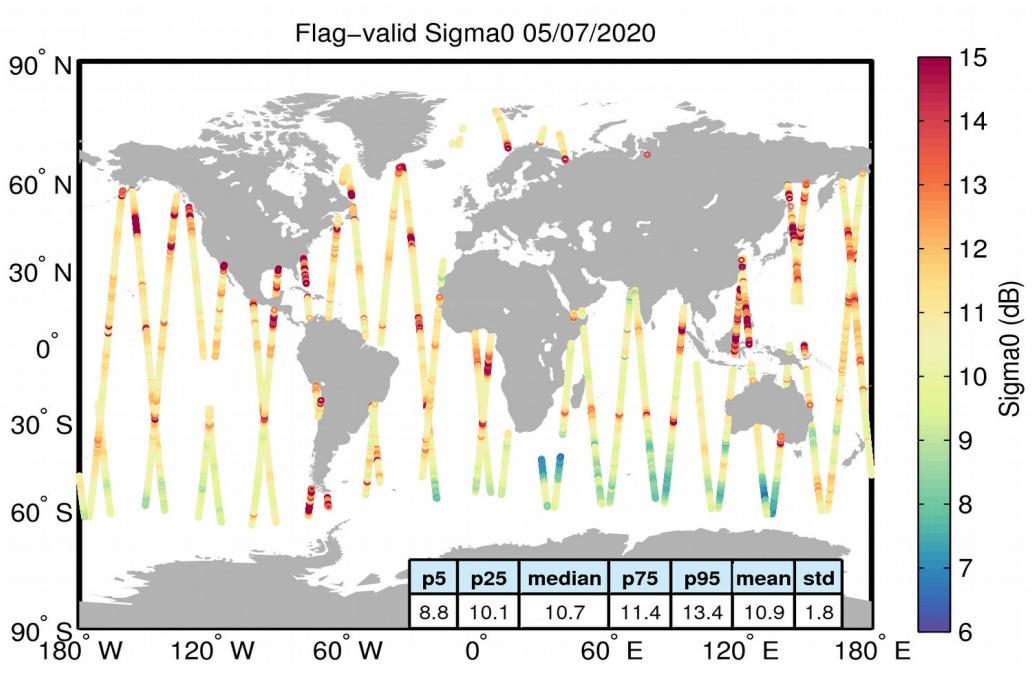
Figure 23. Geographical distribution of flag-valid sigma0 data over oceans and lakes for 05/07/2020. The statistical values shown in the table refer to the sigma0 in dB and are calculated over all measurements shown in the figure.
