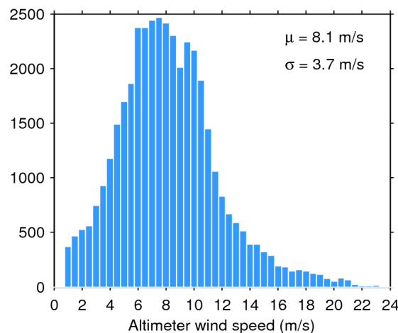
Figure 35. Histogram of science-valid wind over oceans and lakes for 05/07/2020. The mean ( \mu ) and standard deviation ( \sigma ) are also shown. Note that values larger than 24 m/s are excluded from the histogram for the sake of readability but not from the computation of \mu and \sigma .
