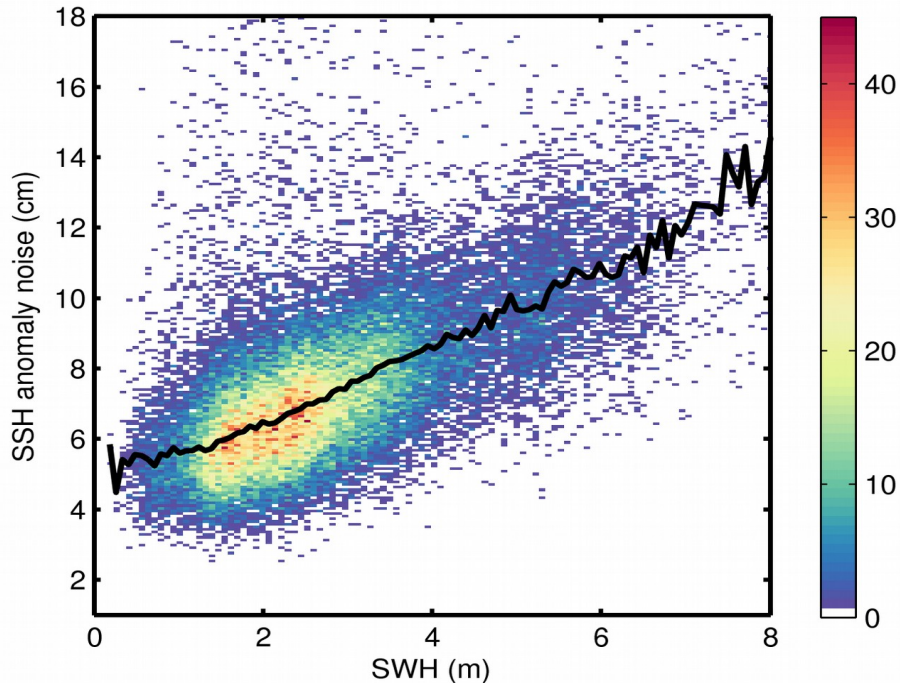
Figure 9. 2D histogram showing flag-valid SSH anomaly noise as a function of SWH for 05/07/2020. The black line denotes the median SSH anomaly noise as a function of SWH.
