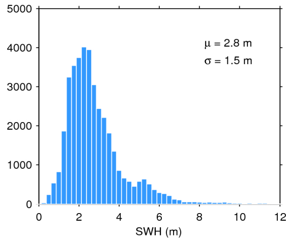
Figure 20. Histogram of science-valid SWH over oceans and lakes for 05/07/2020. The mean ( \mu ) and standard deviation ( \sigma ) are also shown. Note that values larger than 12 m are excluded from the histogram for the sake of readability but not from the computation of \mu and \sigma .
