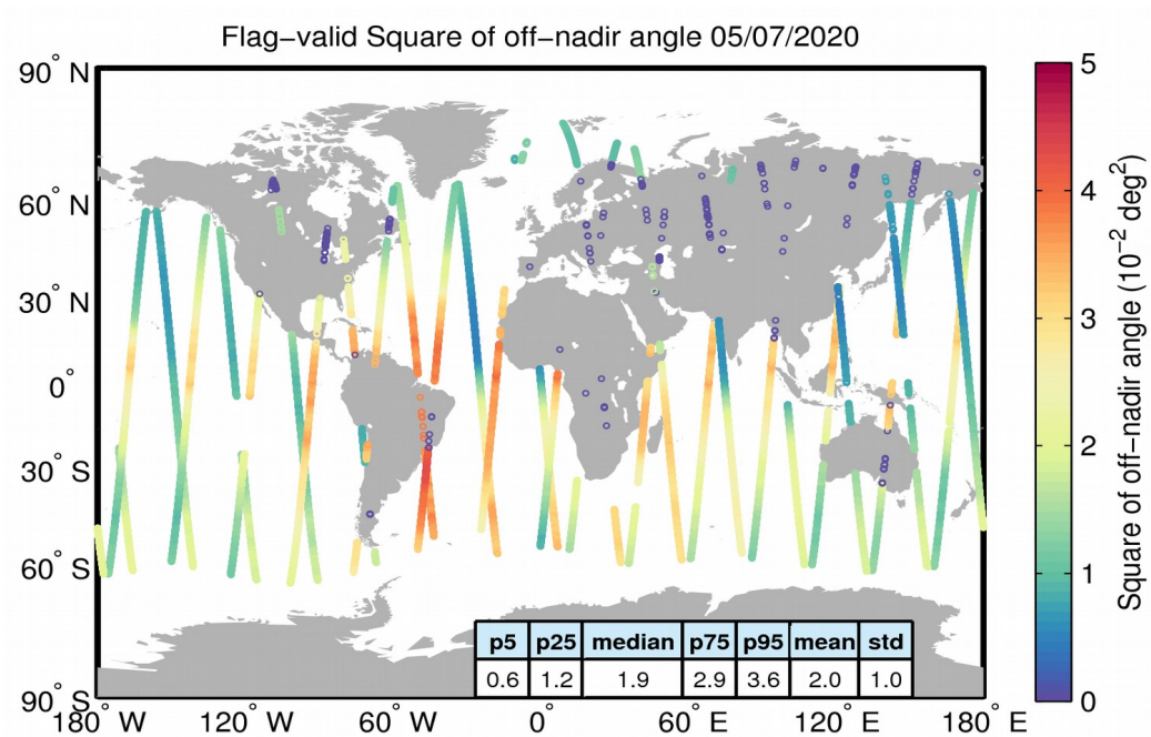
Figure 37. Geographical distribution of flag-valid mispointing data over oceans and lakes for 05/07/2020. The statistical values shown in the table refer to the mispointing in 10^{-2} \text{ deg}^2 and are calculated over all measurements shown in the figure.
