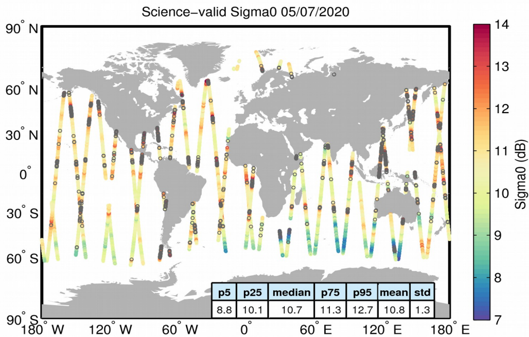
Figure 27. Geographical distribution of science-valid sigma0 data over oceans and lakes for 05/07/2020. The statistical values shown in the table refer to the sigma0 in dB and are calculated over all measurements shown in the figure. Gray circles denote records that have been rejected based on the editing criteria described in Table 4.
