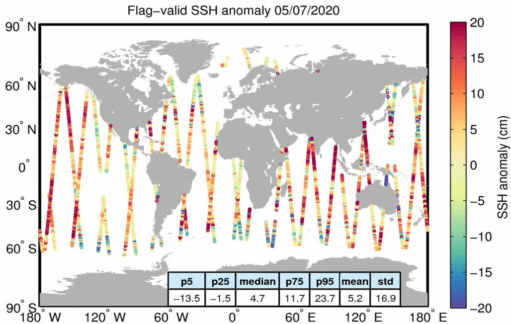
Figure 5. Geographical distribution of flag-valid 1-Hz SSH anomaly data over oceans and lakes for 05/07/2020. The statistical values shown in the table refer to the SSH anomaly in cm and are calculated over all measurements shown in the figure.
