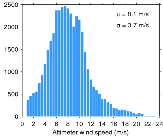
Figure 33. Histogram of flag-valid wind over oceans and lakes for 05/07/2020. The mean ( \mu ) and standard deviation ( \sigma ) are also shown. Note that values larger than 24 m/s are excluded from the histogram for the sake of readability but not from the computation of \mu and \sigma .
