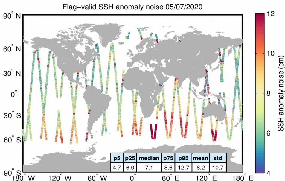
Figure 8. Geographical distribution of flag-valid 20-Hz SSH anomaly measurement noise over oceans and lakes for 05/07/2020. The statistical values shown in the table refer to the SSH anomaly noise and are calculated over all measurements shown in the figure.
