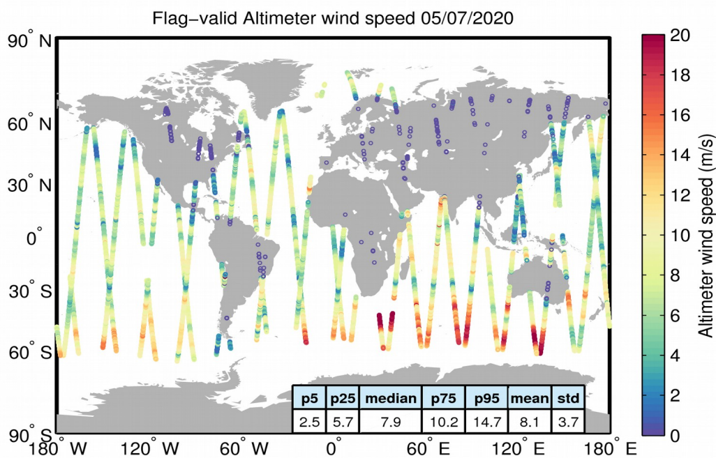
Figure 31. Geographical distribution of flag-valid wind data over oceans and lakes for 05/07/2020. The statistical values shown in the table refer to the wind in m/s and are calculated over all measurements shown in the figure.
