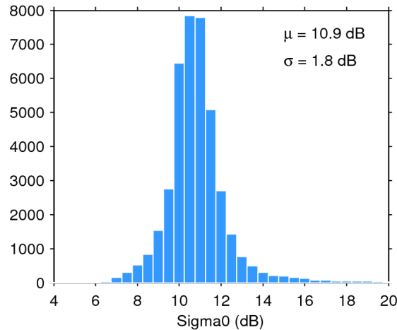
Figure 25. Histogram of flag-valid sigma0 over oceans and lakes for 05/07/2020. The mean ( \mu ) and standard deviation ( \sigma ) are also shown. Note that values outside [4 20] dB are excluded from the histogram for the sake of readability but not from the computation of \mu and \sigma .
