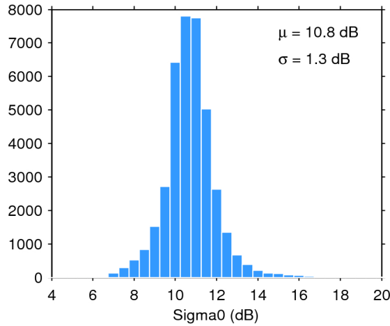
Figure 28. Histogram of science-valid sigma0 over oceans and lakes for 05/07/2020. The mean ( \mu ) and standard deviation ( \sigma ) are also shown. Note that values outside [4 20] dB are excluded from the histogram for the sake of readability but not from the computation of \mu and \sigma .
