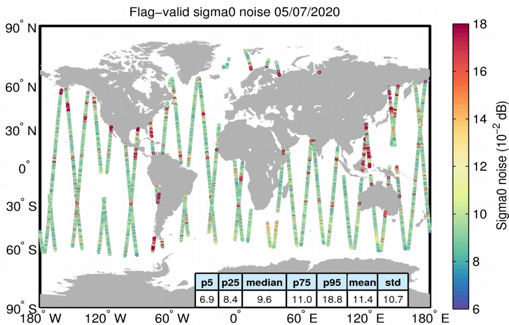
Figure 26. Geographical distribution of flag-valid 20-Hz sigma0 measurement noise over oceans and lakes for 05/07/2020. The statistical values shown in the table refer to the sigma0 noise and are calculated over all measurements shown in the figure.
