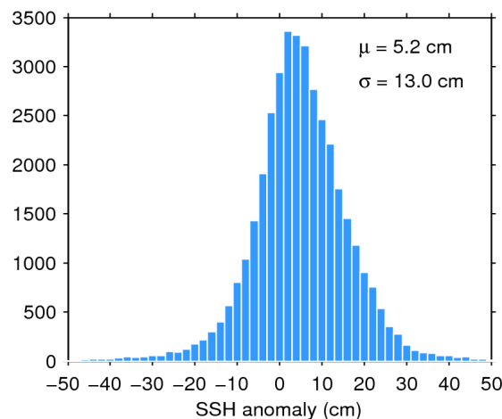
Figure 11. Histogram of science-valid SSH anomaly over oceans and lakes for 05/07/2020. The mean ( \mu ) and standard deviation ( \sigma ) are also shown. Note that values outside [-50 50] cm are excluded from the histogram for the sake of readability but not from the computation of \mu and \sigma .
