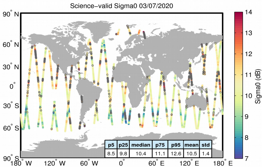
Figure 27. Geographical distribution of science-valid sigma0 data over oceans and lakes for 03/07/2020. The statistical values shown in the table refer to the sigma0 in dB and are calculated over all measurements shown in the figure. Gray circles denote records that have been rejected based on the editing criteria described in Table 4.
