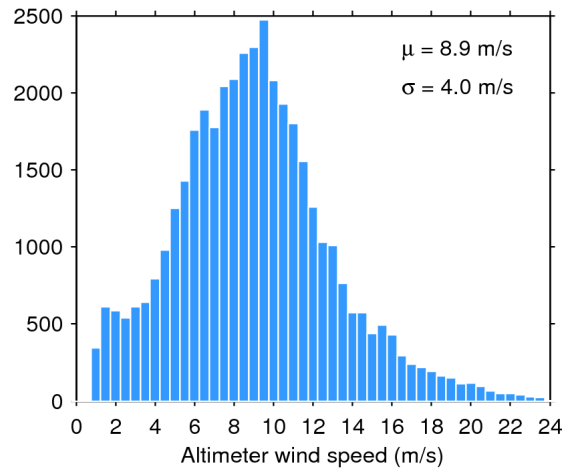
Figure 33. Histogram of flag-valid wind over oceans and lakes for 03/07/2020. The mean ( \mu ) and standard deviation ( \sigma ) are also shown. Note that values larger than 24 m/s are excluded from the histogram for the sake of readability but not from the computation of \mu and \sigma .
