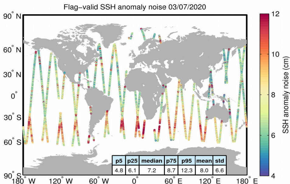
Figure 8. Geographical distribution of flag-valid 20-Hz SSH anomaly measurement noise over oceans and lakes for 03/07/2020. The statistical values shown in the table refer to the SSH anomaly noise and are calculated over all measurements shown in the figure.
