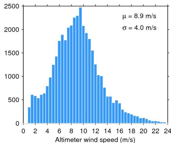
Figure 35. Histogram of science-valid wind over oceans and lakes for 03/07/2020. The mean ( \mu ) and standard deviation ( \sigma ) are also shown. Note that values larger than 24 m/s are excluded from the histogram for the sake of readability but not from the computation of \mu and \sigma .
