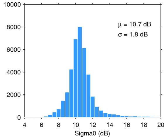
Figure 25. Histogram of flag-valid sigma0 over oceans and lakes for 03/07/2020. The mean ( \mu ) and standard deviation ( \sigma ) are also shown. Note that values outside [4 20] dB are excluded from the histogram for the sake of readability but not from the computation of \mu and \sigma .
