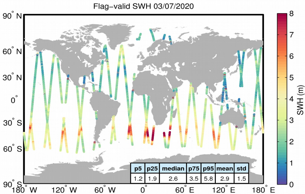
Figure 15. Geographical distribution of flag-valid SWH data over oceans and lakes for 03/07/2020. The statistical values shown in the table refer to the SWH in m and are calculated over all measurements shown in the figure.
