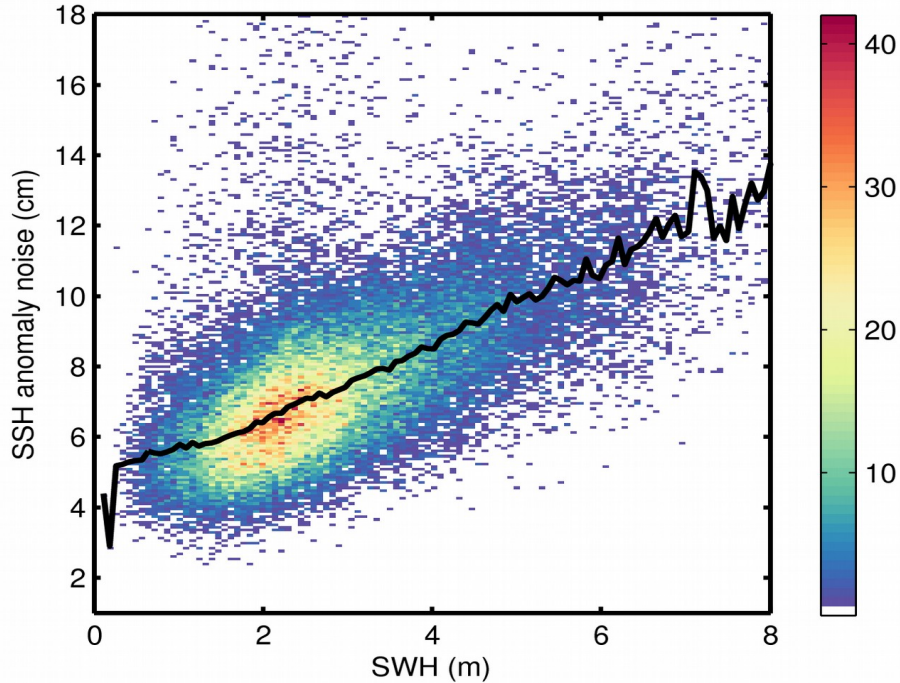
Figure 9. 2D histogram showing flag-valid SSH anomaly noise as a function of SWH for 03/07/2020. The black line denotes the median SSH anomaly noise as a function of SWH.
