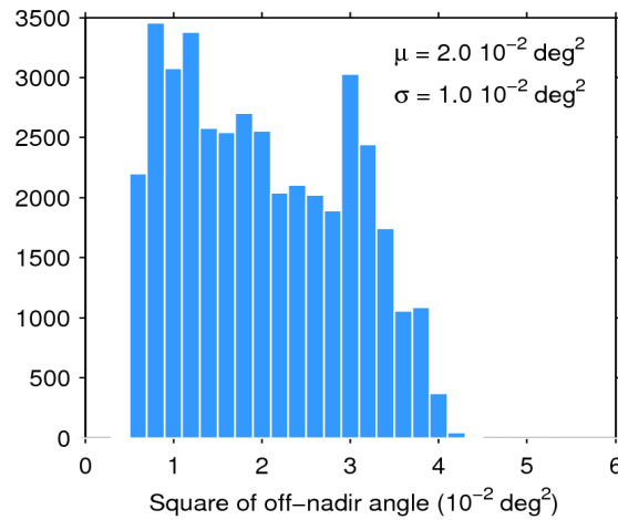
Figure 39. Histogram of flag-valid mispointing over oceans and lakes for 03/07/2020. The mean ( \mu ) and standard deviation ( \sigma ) are also shown. Note that values larger than 6 \cdot 10^{-2} \text{ deg}^2 are excluded from the histogram for the sake of readability but not from the computation of \mu and \sigma .
