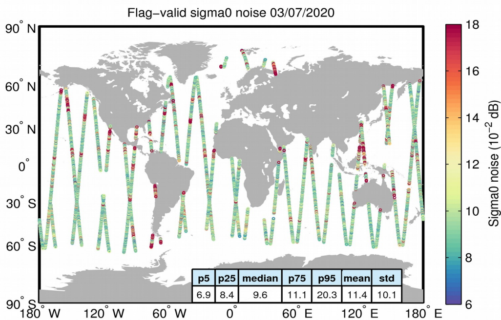
Figure 26. Geographical distribution of flag-valid 20-Hz sigma0 measurement noise over oceans and lakes for 03/07/2020. The statistical values shown in the table refer to the sigma0 noise and are calculated over all measurements shown in the figure.
