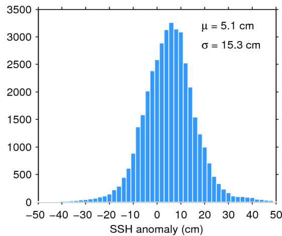
Figure 7. Histogram of flag-valid SSH anomaly over oceans and lakes for 03/07/2020. The mean ( \mu ) and standard deviation ( \sigma ) are also shown. Note that values outside [-50\ 50] cm are excluded from the histogram for the sake of readability but not from the computation of \mu and \sigma .
