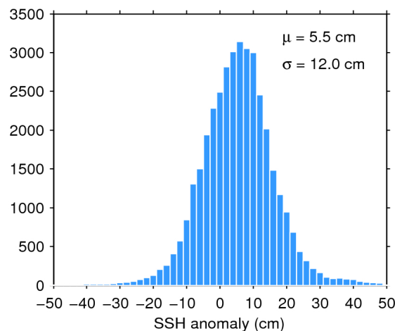
Figure 11. Histogram of science-valid SSH anomaly over oceans and lakes for 03/07/2020. The mean ( \mu ) and standard deviation ( \sigma ) are also shown. Note that values outside [-50 50] cm are excluded from the histogram for the sake of readability but not from the computation of \mu and \sigma .
