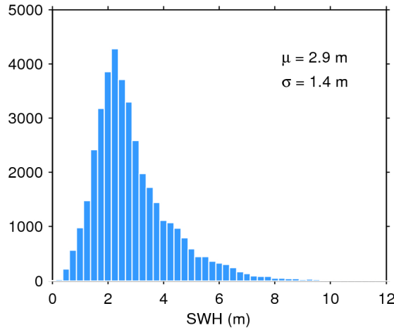
Figure 20. Histogram of science-valid SWH over oceans and lakes for 03/07/2020. The mean ( \mu ) and standard deviation ( \sigma ) are also shown. Note that values larger than 12 m are excluded from the histogram for the sake of readability but not from the computation of \mu and \sigma .
