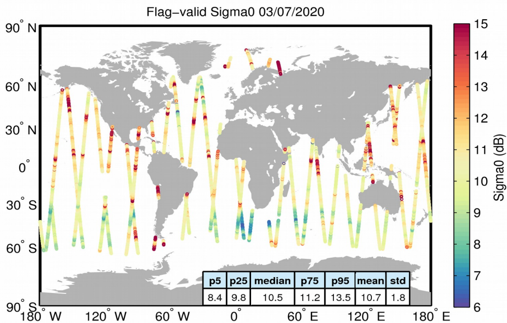
Figure 23. Geographical distribution of flag-valid sigma0 data over oceans and lakes for 03/07/2020. The statistical values shown in the table refer to the sigma0 in dB and are calculated over all measurements shown in the figure.
