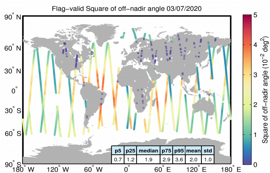
Figure 37. Geographical distribution of flag-valid mispointing data over oceans and lakes for 03/07/2020. The statistical values shown in the table refer to the mispointing in 10^{-2} \text{ deg}^2 and are calculated over all measurements shown in the figure.
