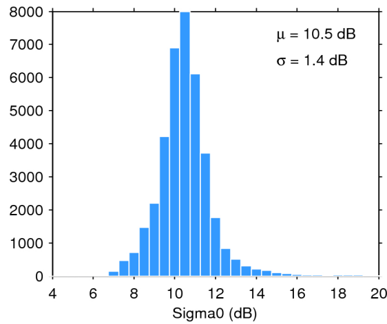
Figure 28. Histogram of science-valid sigma0 over oceans and lakes for 03/07/2020. The mean ( \mu ) and standard deviation ( \sigma ) are also shown. Note that values outside [4 20] dB are excluded from the histogram for the sake of readability but not from the computation of \mu and \sigma .
