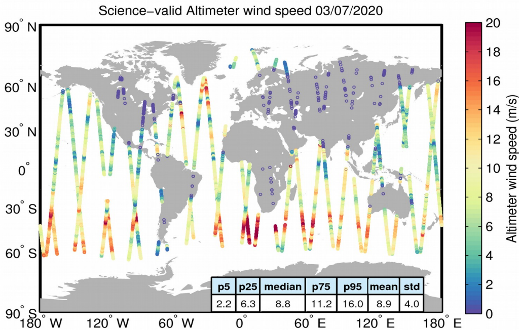
Figure 34. Geographical distribution of science-valid wind data over oceans and lakes for 03/07/2020. The statistical values shown in the table refer to the wind in m/s and are calculated over all measurements shown in the figure. Gray circles denote records that have been rejected based on the editing criteria described in Table 5.
