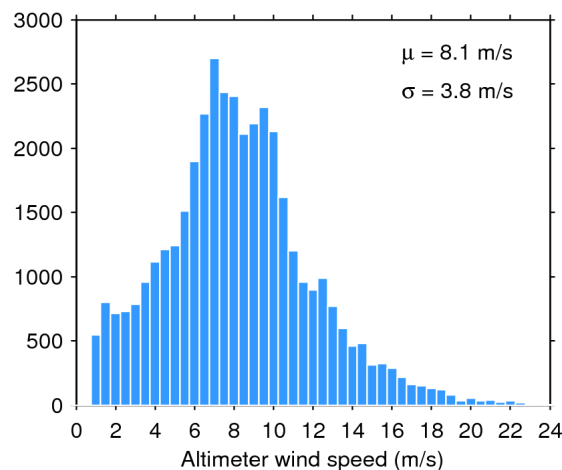
Figure 35. Histogram of science-valid wind over oceans and lakes for 01/07/2020. The mean ( \mu ) and standard deviation ( \sigma ) are also shown. Note that values larger than 24 m/s are excluded from the histogram for the sake of readability but not from the computation of \mu and \sigma .
