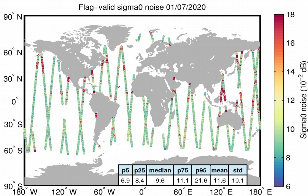
Figure 26. Geographical distribution of flag-valid 20-Hz sigma0 measurement noise over oceans and lakes for 01/07/2020. The statistical values shown in the table refer to the sigma0 noise and are calculated over all measurements shown in the figure.
