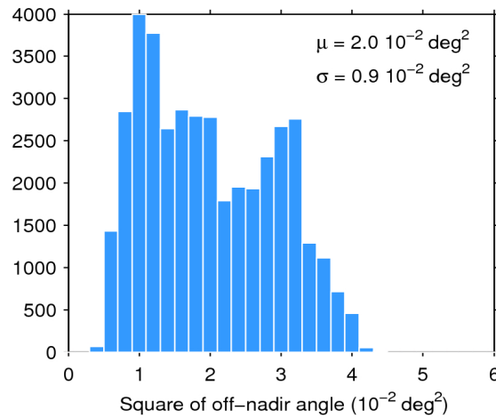
Figure 39. Histogram of flag-valid mispointing over oceans and lakes for 01/07/2020. The mean ( \mu ) and standard deviation ( \sigma ) are also shown. Note that values larger than 6 \cdot 10^{-2} \text{ deg}^2 are excluded from the histogram for the sake of readability but not from the computation of \mu and \sigma .
