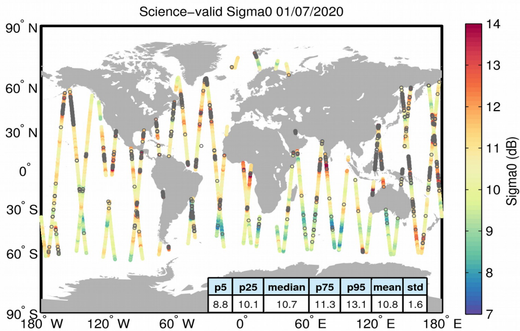
Figure 27. Geographical distribution of science-valid sigma0 data over oceans and lakes for 01/07/2020. The statistical values shown in the table refer to the sigma0 in dB and are calculated over all measurements shown in the figure. Gray circles denote records that have been rejected based on the editing criteria described in Table 4.
