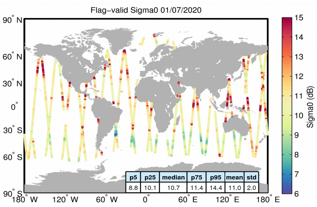
Figure 23. Geographical distribution of flag-valid sigma0 data over oceans and lakes for 01/07/2020. The statistical values shown in the table refer to the sigma0 in dB and are calculated over all measurements shown in the figure.
