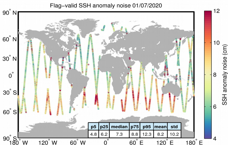
Figure 8. Geographical distribution of flag-valid 20-Hz SSH anomaly measurement noise over oceans and lakes for 01/07/2020. The statistical values shown in the table refer to the SSH anomaly noise and are calculated over all measurements shown in the figure.
