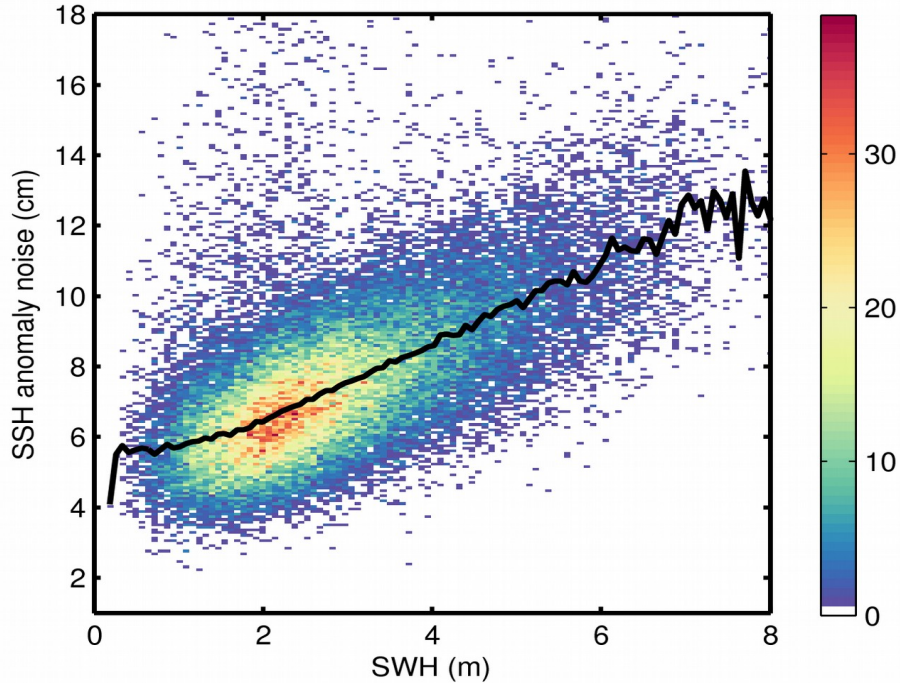
Figure 9. 2D histogram showing flag-valid SSH anomaly noise as a function of SWH for 01/07/2020. The black line denotes the median SSH anomaly noise as a function of SWH.
