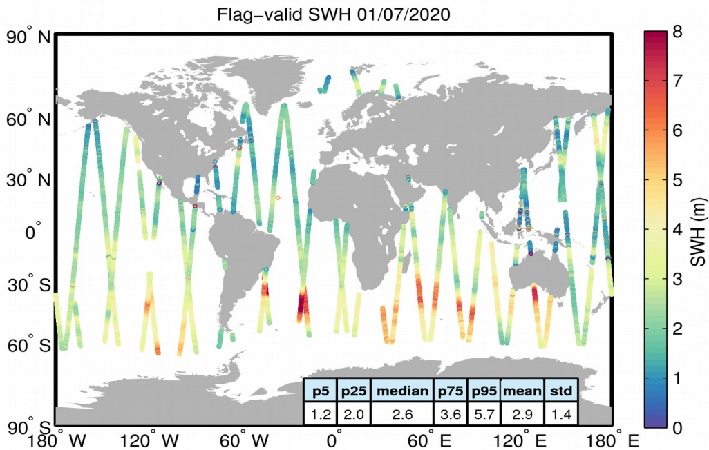
Figure 15. Geographical distribution of flag-valid SWH data over oceans and lakes for 01/07/2020. The statistical values shown in the table refer to the SWH in m and are calculated over all measurements shown in the figure.
