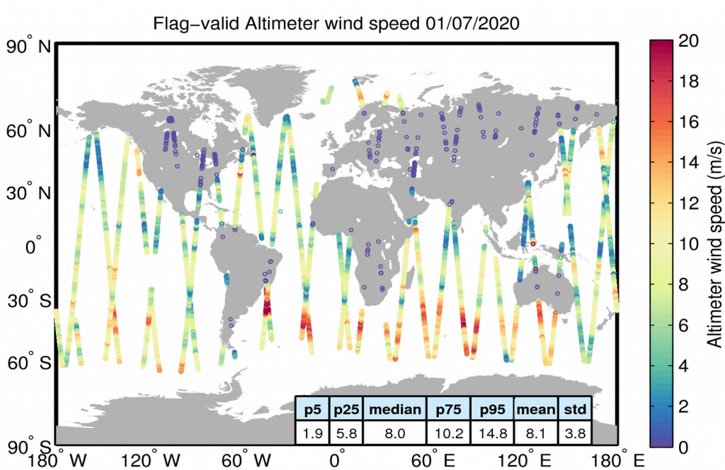
Figure 31. Geographical distribution of flag-valid wind data over oceans and lakes for 01/07/2020. The statistical values shown in the table refer to the wind in m/s and are calculated over all measurements shown in the figure.
