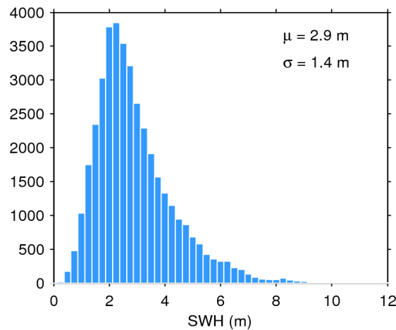
Figure 17. Histogram of flag-valid SWH over oceans and lakes for 01/07/2020. The mean ( \mu ) and standard deviation ( \sigma ) are also shown. Note that values larger than 12 m are excluded from the histogram for the sake of readability but not from the computation of \mu and \sigma .
