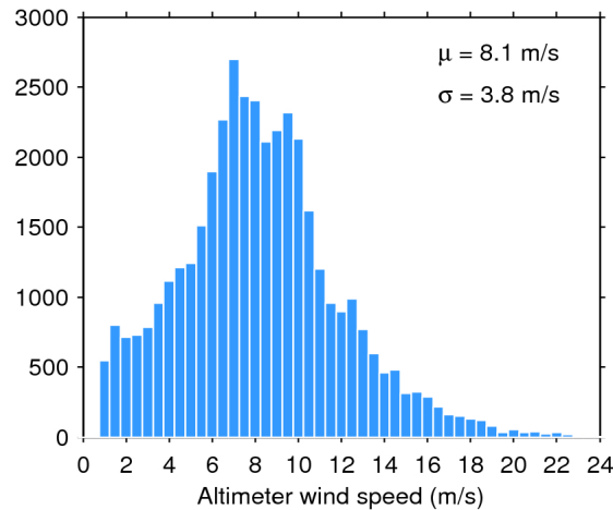
Figure 33. Histogram of flag-valid wind over oceans and lakes for 01/07/2020. The mean ( \mu ) and standard deviation ( \sigma ) are also shown. Note that values larger than 24 m/s are excluded from the histogram for the sake of readability but not from the computation of \mu and \sigma .
