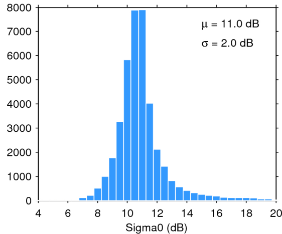
Figure 25. Histogram of flag-valid sigma0 over oceans and lakes for 01/07/2020. The mean ( \mu ) and standard deviation ( \sigma ) are also shown. Note that values outside [4 20] dB are excluded from the histogram for the sake of readability but not from the computation of \mu and \sigma .
