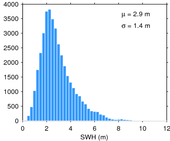
Figure 20. Histogram of science-valid SWH over oceans and lakes for 01/07/2020. The mean ( \mu ) and standard deviation ( \sigma ) are also shown. Note that values larger than 12 m are excluded from the histogram for the sake of readability but not from the computation of \mu and \sigma .
