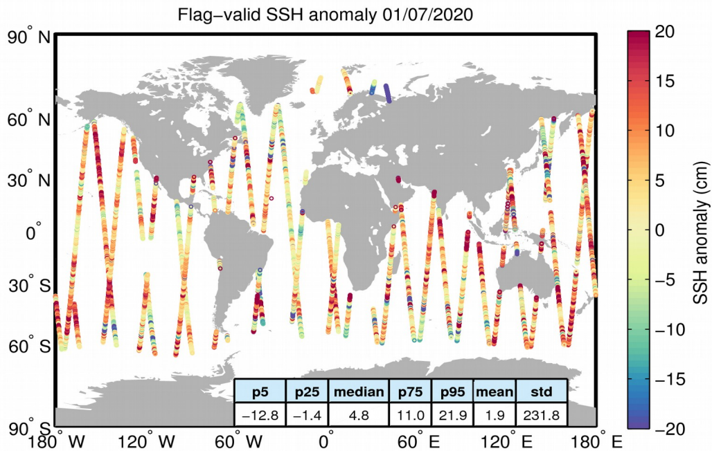
Figure 5. Geographical distribution of flag-valid 1-Hz SSH anomaly data over oceans and lakes for 01/07/2020. The statistical values shown in the table refer to the SSH anomaly in cm and are calculated over all measurements shown in the figure.
