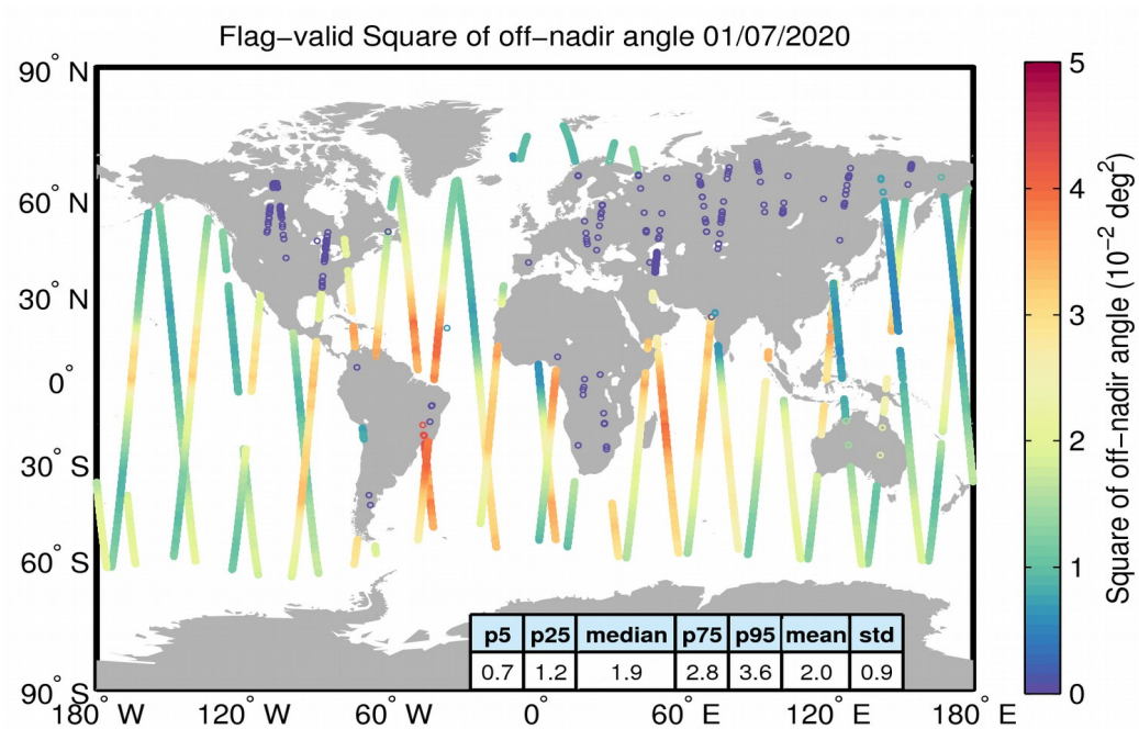
Figure 37. Geographical distribution of flag-valid mispointing data over oceans and lakes for 01/07/2020. The statistical values shown in the table refer to the mispointing in 10^{-2} \text{ deg}^2 and are calculated over all measurements shown in the figure.
