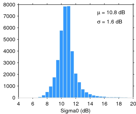
Figure 28. Histogram of science-valid sigma0 over oceans and lakes for 01/07/2020. The mean ( \mu ) and standard deviation ( \sigma ) are also shown. Note that values outside [4 20] dB are excluded from the histogram for the sake of readability but not from the computation of \mu and \sigma .
