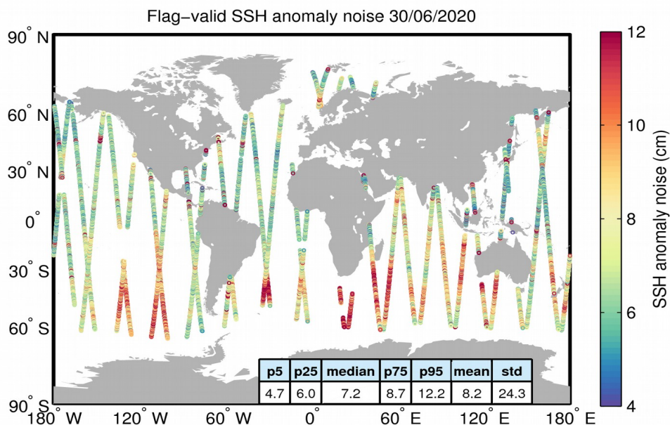
Figure 8. Geographical distribution of flag-valid 20-Hz SSH anomaly measurement noise over oceans and lakes for 30/06/2020. The statistical values shown in the table refer to the SSH anomaly noise and are calculated over all measurements shown in the figure.
