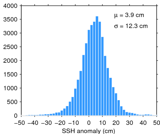
Figure 11. Histogram of science-valid SSH anomaly over oceans and lakes for 30/06/2020. The mean ( \mu ) and standard deviation ( \sigma ) are also shown. Note that values outside [-50 50] cm are excluded from the histogram for the sake of readability but not from the computation of \mu and \sigma .
