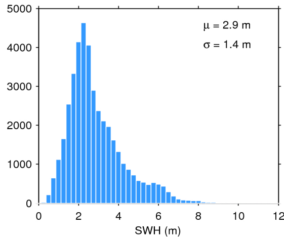
Figure 20. Histogram of science-valid SWH over oceans and lakes for 30/06/2020. The mean ( \mu ) and standard deviation ( \sigma ) are also shown. Note that values larger than 12 m are excluded from the histogram for the sake of readability but not from the computation of \mu and \sigma .
