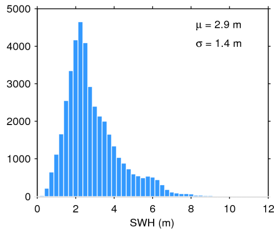
Figure 17. Histogram of flag-valid SWH over oceans and lakes for 30/06/2020. The mean ( \mu ) and standard deviation ( \sigma ) are also shown. Note that values larger than 12 m are excluded from the histogram for the sake of readability but not from the computation of \mu and \sigma .
