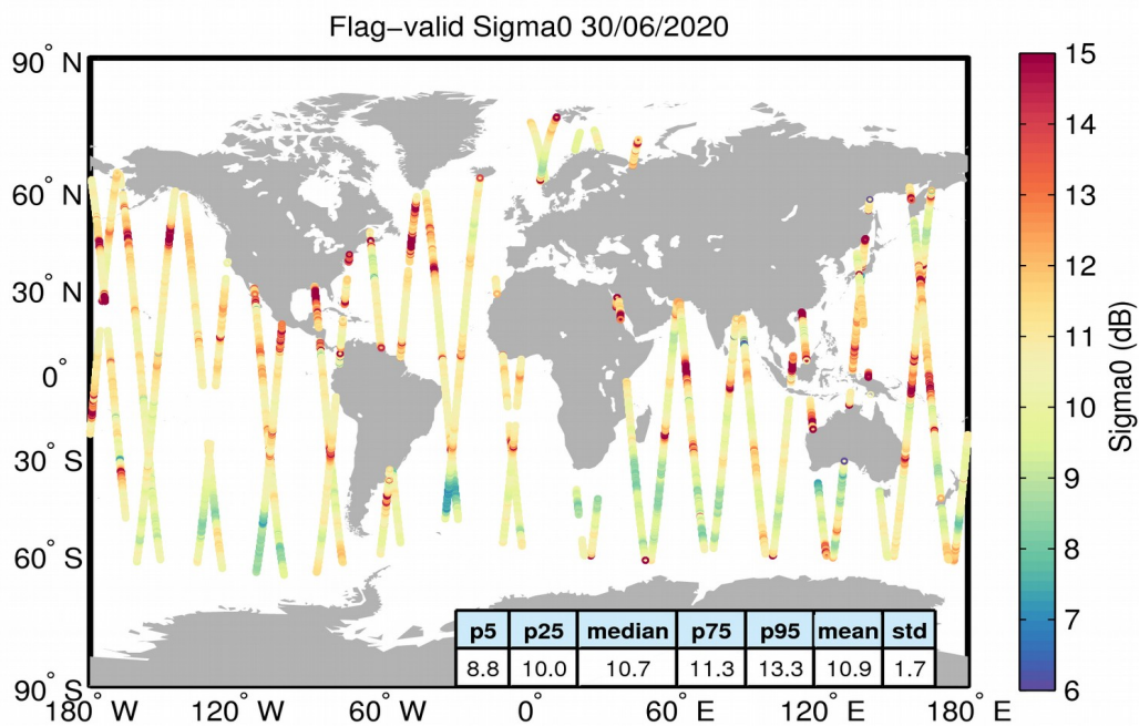
Figure 23. Geographical distribution of flag-valid sigma0 data over oceans and lakes for 30/06/2020. The statistical values shown in the table refer to the sigma0 in dB and are calculated over all measurements shown in the figure.
