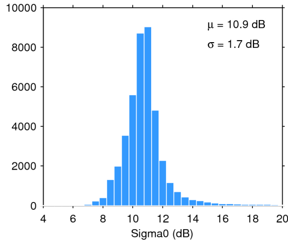
Figure 25. Histogram of flag-valid sigma0 over oceans and lakes for 30/06/2020. The mean ( \mu ) and standard deviation ( \sigma ) are also shown. Note that values outside [4 20] dB are excluded from the histogram for the sake of readability but not from the computation of \mu and \sigma .
