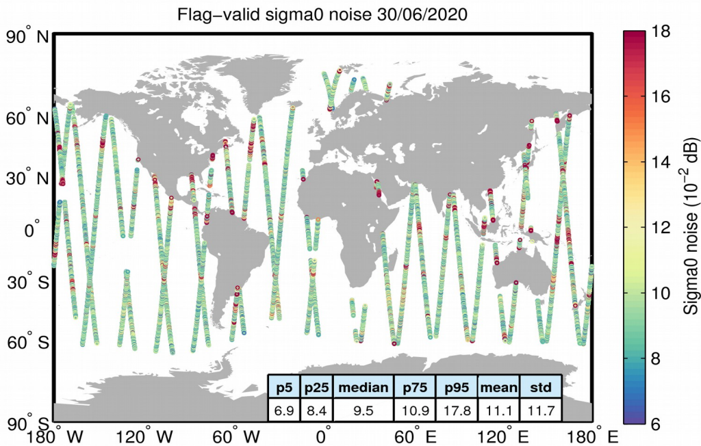
Figure 26. Geographical distribution of flag-valid 20-Hz sigma0 measurement noise over oceans and lakes for 30/06/2020. The statistical values shown in the table refer to the sigma0 noise and are calculated over all measurements shown in the figure.
