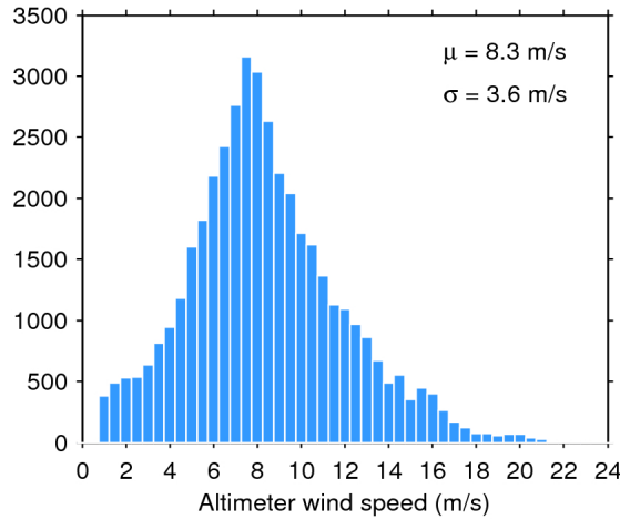
Figure 33. Histogram of flag-valid wind over oceans and lakes for 30/06/2020. The mean ( \mu ) and standard deviation ( \sigma ) are also shown. Note that values larger than 24 m/s are excluded from the histogram for the sake of readability but not from the computation of \mu and \sigma .
