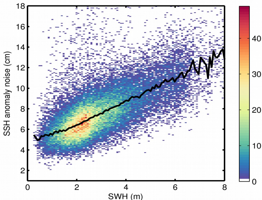
Figure 9. 2D histogram showing flag-valid SSH anomaly noise as a function of SWH for 30/06/2020. The black line denotes the median SSH anomaly noise as a function of SWH.
