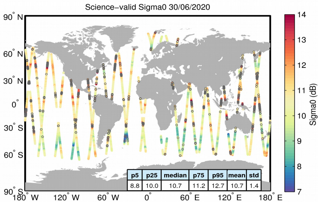
Figure 27. Geographical distribution of science-valid sigma0 data over oceans and lakes for 30/06/2020. The statistical values shown in the table refer to the sigma0 in dB and are calculated over all measurements shown in the figure. Gray circles denote records that have been rejected based on the editing criteria described in Table 4.
