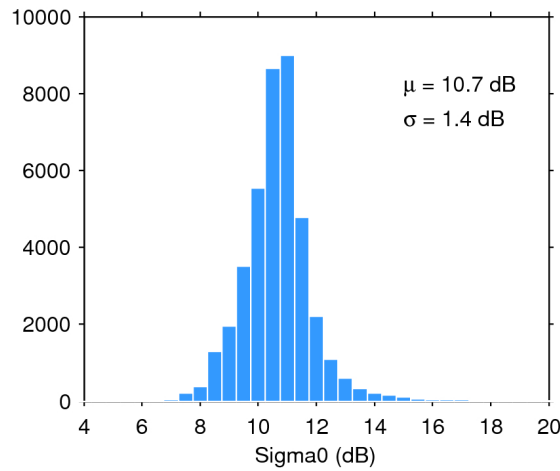
Figure 28. Histogram of science-valid sigma0 over oceans and lakes for 30/06/2020. The mean ( \mu ) and standard deviation ( \sigma ) are also shown. Note that values outside [4 20] dB are excluded from the histogram for the sake of readability but not from the computation of \mu and \sigma .
