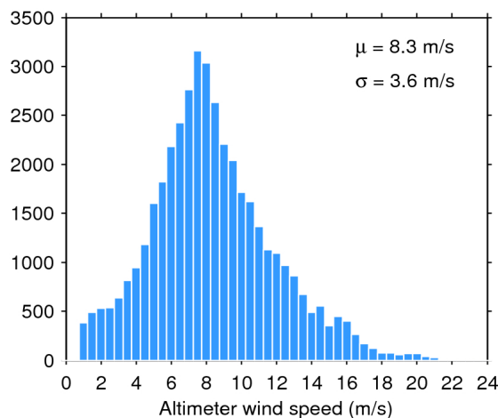
Figure 35. Histogram of science-valid wind over oceans and lakes for 30/06/2020. The mean ( \mu ) and standard deviation ( \sigma ) are also shown. Note that values larger than 24 m/s are excluded from the histogram for the sake of readability but not from the computation of \mu and \sigma .
