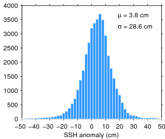
Figure 7. Histogram of flag-valid SSH anomaly over oceans and lakes for 30/06/2020. The mean ( \mu ) and standard deviation ( \sigma ) are also shown. Note that values outside [-50 50] cm are excluded from the histogram for the sake of readability but not from the computation of \mu and \sigma .
