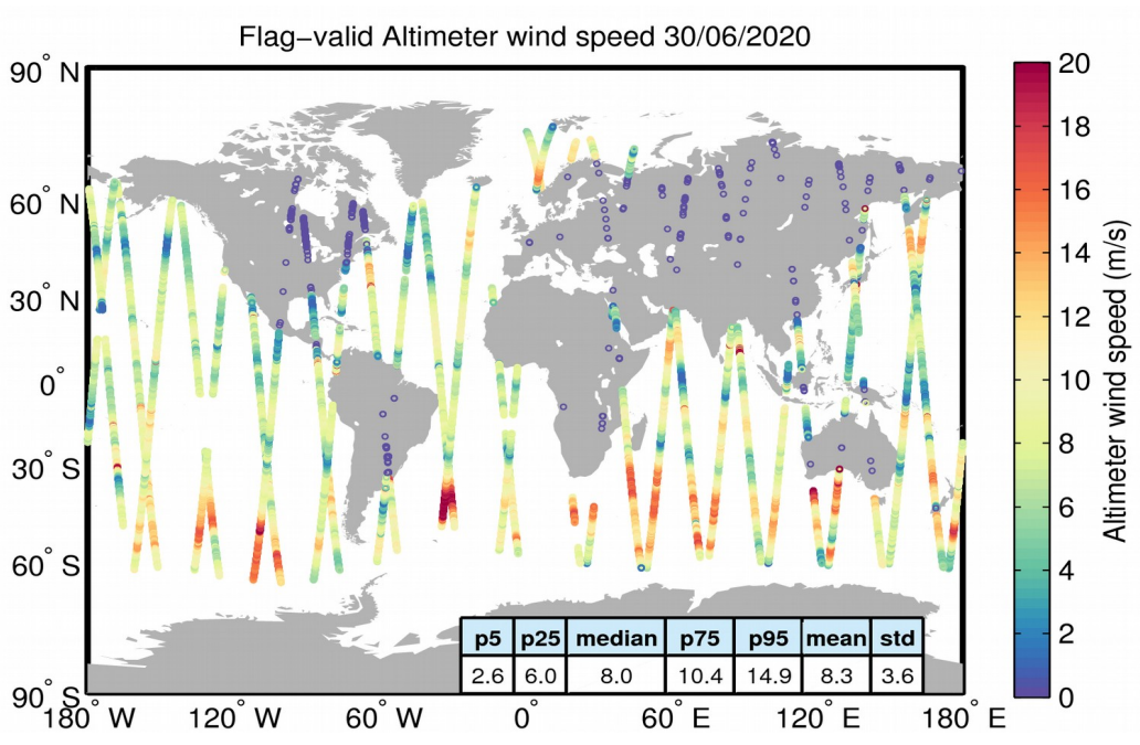
Figure 31. Geographical distribution of flag-valid wind data over oceans and lakes for 30/06/2020. The statistical values shown in the table refer to the wind in m/s and are calculated over all measurements shown in the figure.
