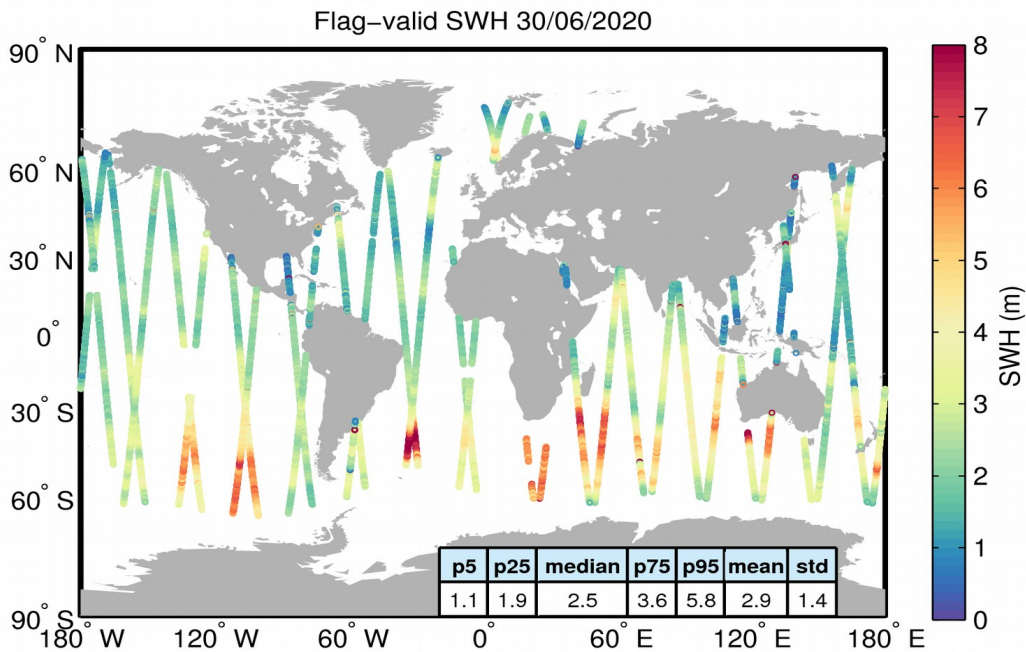
Figure 15. Geographical distribution of flag-valid SWH data over oceans and lakes for 30/06/2020. The statistical values shown in the table refer to the SWH in m and are calculated over all measurements shown in the figure.
