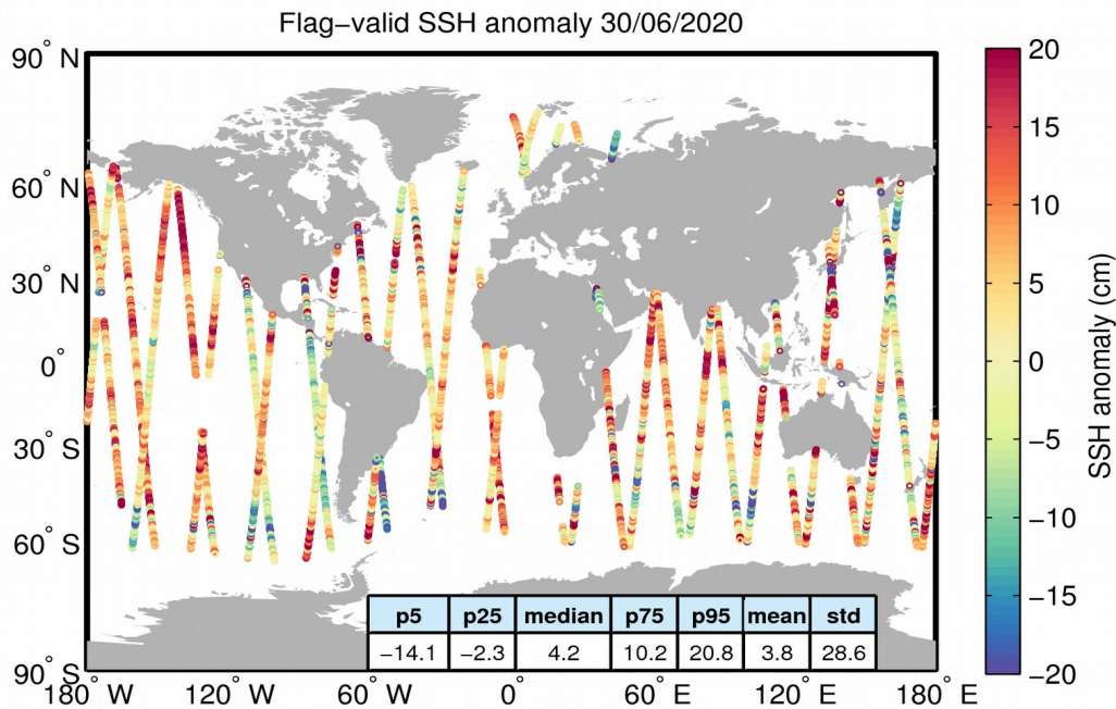
Figure 5. Geographical distribution of flag-valid 1-Hz SSH anomaly data over oceans and lakes for 30/06/2020. The statistical values shown in the table refer to the SSH anomaly in cm and are calculated over all measurements shown in the figure.
