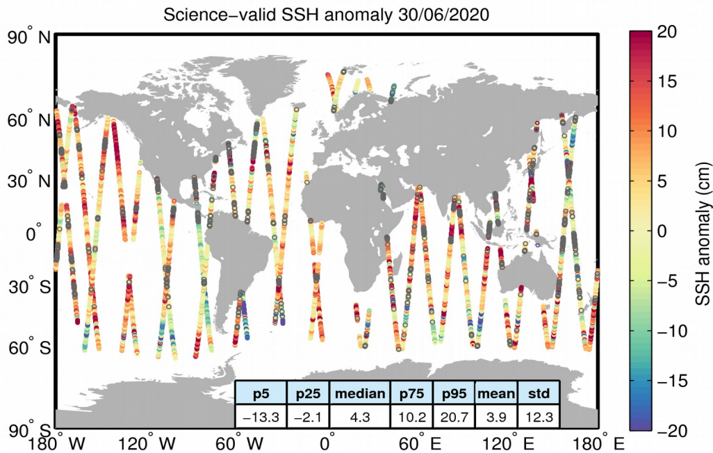
Figure 10. Geographical distribution of science-valid SSH anomaly data over oceans and lakes for 30/06/2020. The statistical values shown in the table refer to the SSH anomaly in cm and are calculated over all measurements shown in the figure. Gray circles denote records that have been rejected based on the editing criteria described in Table 2.
