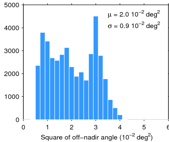
Figure 39. Histogram of flag-valid mispointing over oceans and lakes for 30/06/2020. The mean ( \mu ) and standard deviation ( \sigma ) are also shown. Note that values larger than 6 \cdot 10^{-2} \text{ deg}^2 are excluded from the histogram for the sake of readability but not from the computation of \mu and \sigma .
