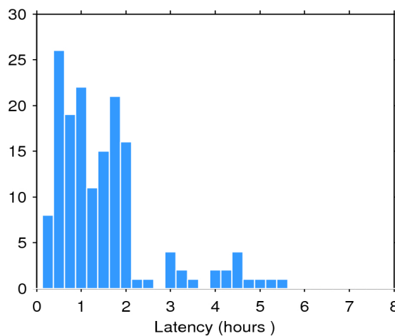
Figure 2. Histogram of the data latency for 30/06/2020. The y-axis denotes the number of files that are made available with a delay of x-hours with respect to the mean time of the records stored in the file.
