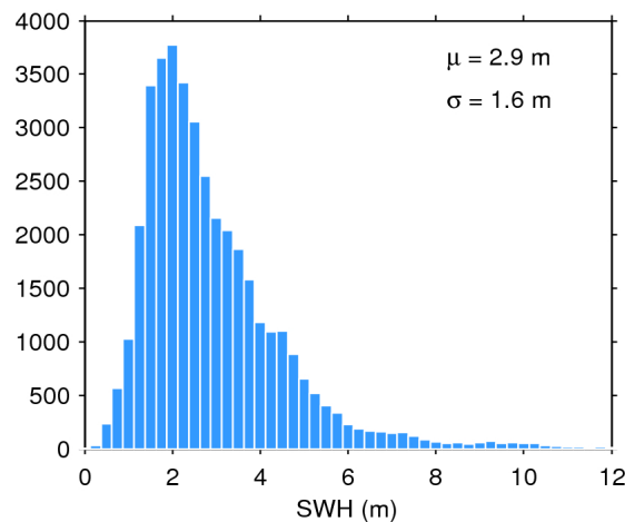
Figure 17. Histogram of flag-valid SWH over oceans and lakes for 27/06/2020. The mean ( \mu ) and standard deviation ( \sigma ) are also shown. Note that values larger than 12 m are excluded from the histogram for the sake of readability but not from the computation of \mu and \sigma .
