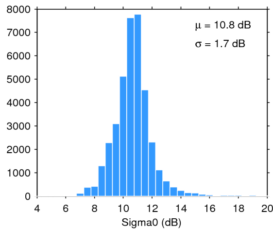
Figure 28. Histogram of science-valid sigma0 over oceans and lakes for 27/06/2020. The mean ( \mu ) and standard deviation ( \sigma ) are also shown. Note that values outside [4 20] dB are excluded from the histogram for the sake of readability but not from the computation of \mu and \sigma .
