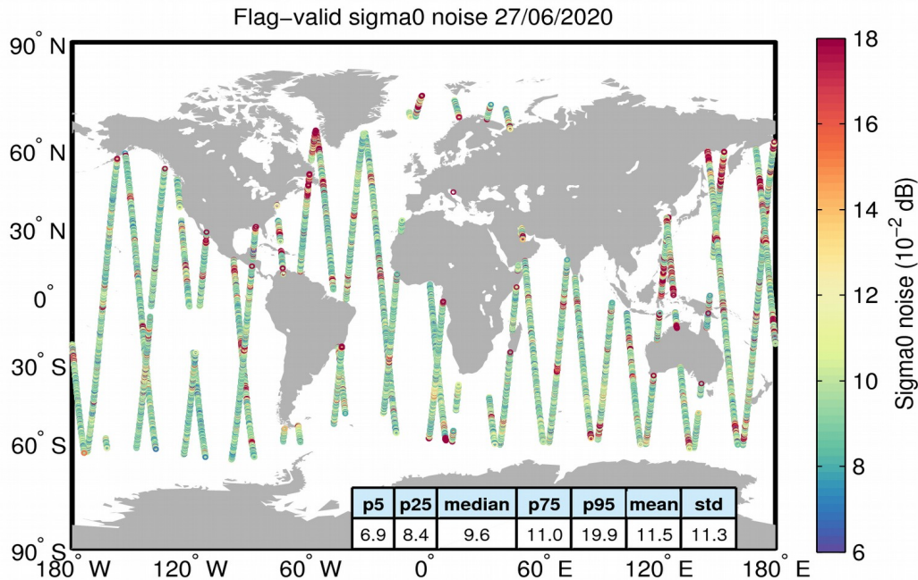
Figure 26. Geographical distribution of flag-valid 20-Hz sigma0 measurement noise over oceans and lakes for 27/06/2020. The statistical values shown in the table refer to the sigma0 noise and are calculated over all measurements shown in the figure.
