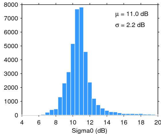
Figure 25. Histogram of flag-valid sigma0 over oceans and lakes for 27/06/2020. The mean ( \mu ) and standard deviation ( \sigma ) are also shown. Note that values outside [4 20] dB are excluded from the histogram for the sake of readability but not from the computation of \mu and \sigma .
