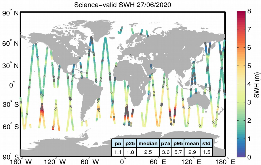
Figure 19. Geographical distribution of science-valid SWH data over oceans and lakes for 27/06/2020. The statistical values shown in the table refer to the SWH in m and are calculated over all measurements shown in the figure. Gray circles denote records that have been rejected based on the editing criteria described in Table 3.
