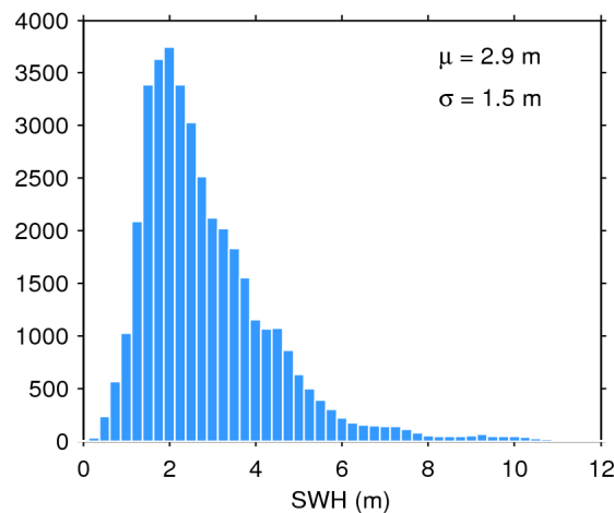
Figure 20. Histogram of science-valid SWH over oceans and lakes for 27/06/2020. The mean ( \mu ) and standard deviation ( \sigma ) are also shown. Note that values larger than 12 m are excluded from the histogram for the sake of readability but not from the computation of \mu and \sigma .
