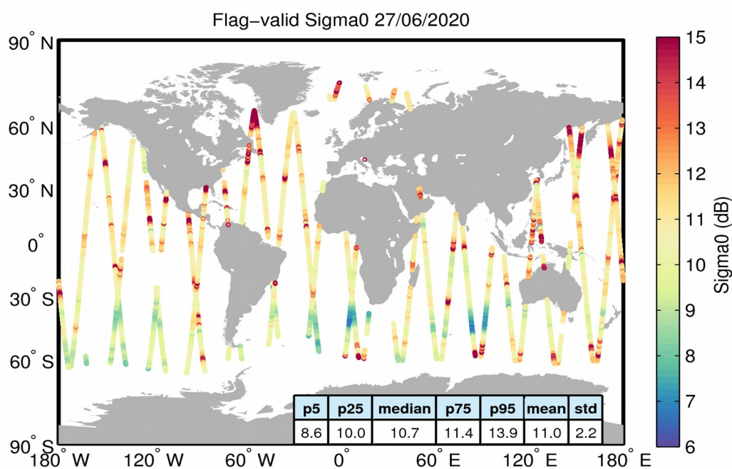
Figure 23. Geographical distribution of flag-valid sigma0 data over oceans and lakes for 27/06/2020. The statistical values shown in the table refer to the sigma0 in dB and are calculated over all measurements shown in the figure.
