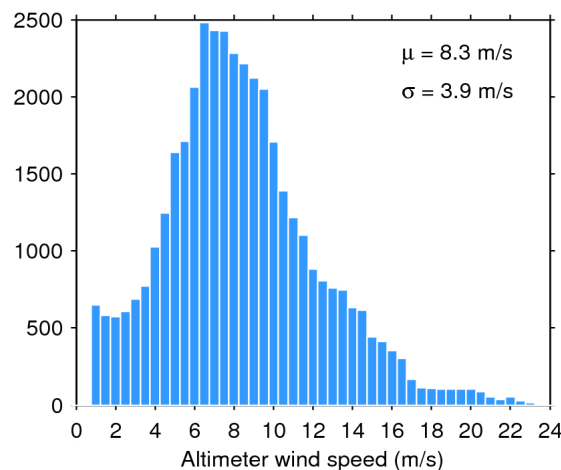
Figure 35. Histogram of science-valid wind over oceans and lakes for 27/06/2020. The mean ( \mu ) and standard deviation ( \sigma ) are also shown. Note that values larger than 24 m/s are excluded from the histogram for the sake of readability but not from the computation of \mu and \sigma .
