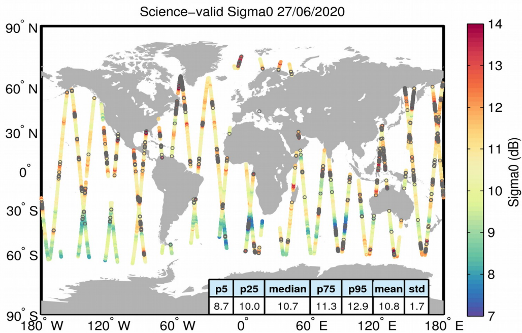
Figure 27. Geographical distribution of science-valid sigma0 data over oceans and lakes for 27/06/2020. The statistical values shown in the table refer to the sigma0 in dB and are calculated over all measurements shown in the figure. Gray circles denote records that have been rejected based on the editing criteria described in Table 4.
