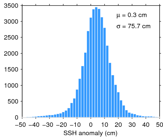
Figure 7. Histogram of flag-valid SSH anomaly over oceans and lakes for 27/06/2020. The mean ( \mu ) and standard deviation ( \sigma ) are also shown. Note that values outside [-50\ 50] cm are excluded from the histogram for the sake of readability but not from the computation of \mu and \sigma .
