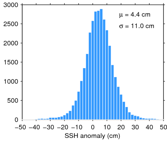
Figure 11. Histogram of science-valid SSH anomaly over oceans and lakes for 27/06/2020. The mean ( \mu ) and standard deviation ( \sigma ) are also shown. Note that values outside [-50 50] cm are excluded from the histogram for the sake of readability but not from the computation of \mu and \sigma .
