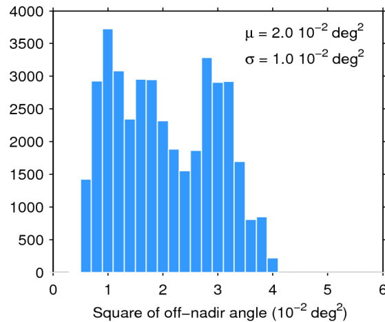
Figure 39. Histogram of flag-valid mispointing over oceans and lakes for 27/06/2020. The mean ( \mu ) and standard deviation ( \sigma ) are also shown. Note that values larger than 6 \cdot 10^{-2} \text{ deg}^2 are excluded from the histogram for the sake of readability but not from the computation of \mu and \sigma .
