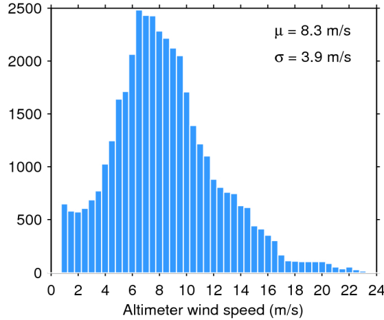
Figure 33. Histogram of flag-valid wind over oceans and lakes for 27/06/2020. The mean ( \mu ) and standard deviation ( \sigma ) are also shown. Note that values larger than 24 m/s are excluded from the histogram for the sake of readability but not from the computation of \mu and \sigma .
