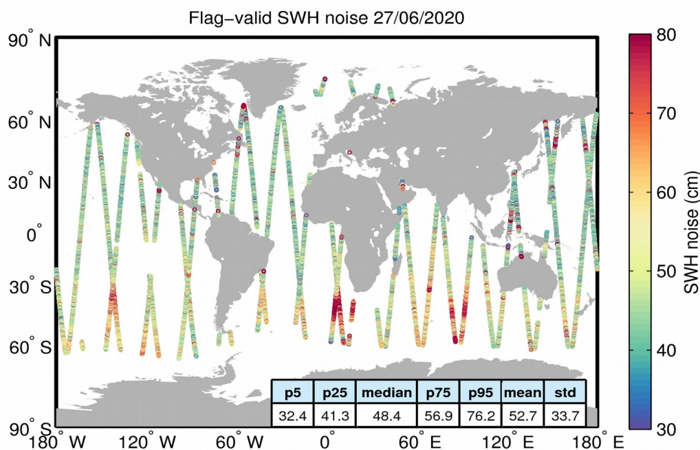
Figure 18. Geographical distribution of flag-valid 20-Hz SWH measurement noise over oceans and lakes for 27/06/2020. The statistical values shown in the table refer to the SWH noise and are calculated over all measurements shown in the figure.
