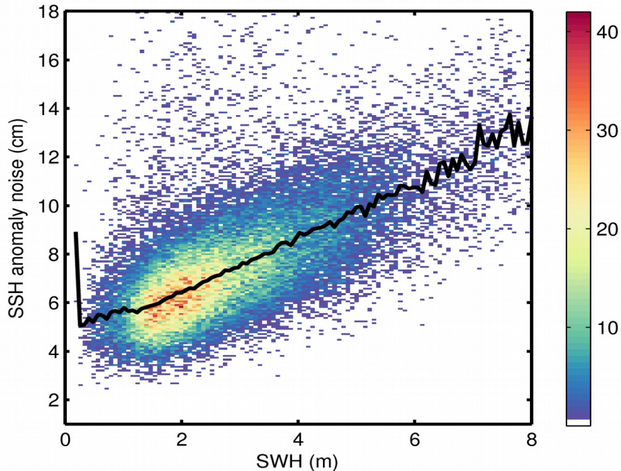
Figure 9. 2D histogram showing flag-valid SSH anomaly noise as a function of SWH for 27/06/2020. The black line denotes the median SSH anomaly noise as a function of SWH.
