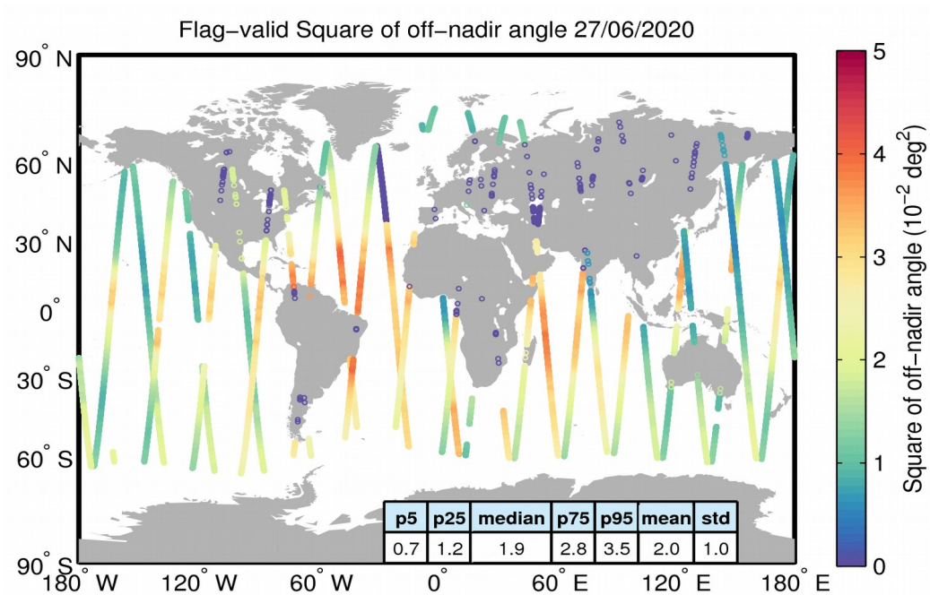
Figure 37. Geographical distribution of flag-valid mispointing data over oceans and lakes for 27/06/2020. The statistical values shown in the table refer to the mispointing in 10^{-2} \text{ deg}^2 and are calculated over all measurements shown in the figure.
