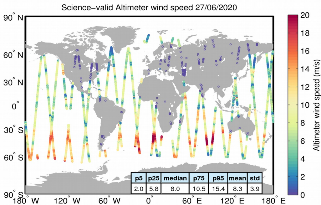
Figure 34. Geographical distribution of science-valid wind data over oceans and lakes for 27/06/2020. The statistical values shown in the table refer to the wind in m/s and are calculated over all measurements shown in the figure. Gray circles denote records that have been rejected based on the editing criteria described in Table 5.
