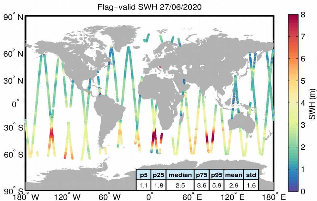
Figure 15. Geographical distribution of flag-valid SWH data over oceans and lakes for 27/06/2020. The statistical values shown in the table refer to the SWH in m and are calculated over all measurements shown in the figure.
