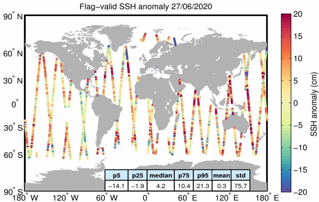
Figure 5. Geographical distribution of flag-valid 1-Hz SSH anomaly data over oceans and lakes for 27/06/2020. The statistical values shown in the table refer to the SSH anomaly in cm and are calculated over all measurements shown in the figure.
