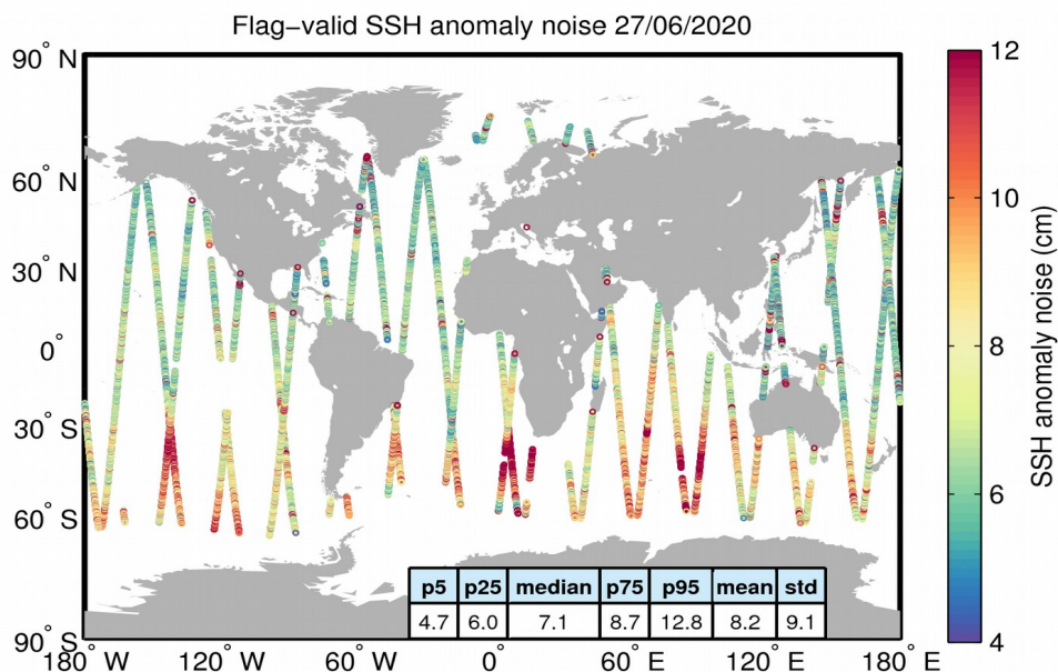
Figure 8. Geographical distribution of flag-valid 20-Hz SSH anomaly measurement noise over oceans and lakes for 27/06/2020. The statistical values shown in the table refer to the SSH anomaly noise and are calculated over all measurements shown in the figure.
