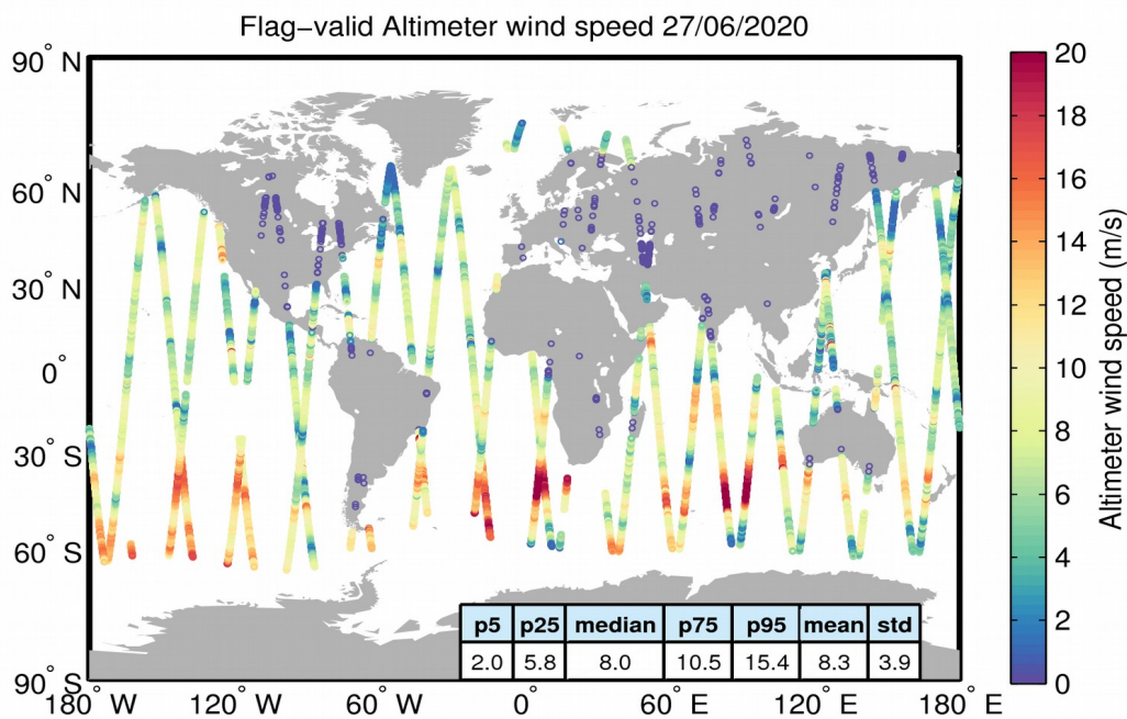
Figure 31. Geographical distribution of flag-valid wind data over oceans and lakes for 27/06/2020. The statistical values shown in the table refer to the wind in m/s and are calculated over all measurements shown in the figure.
