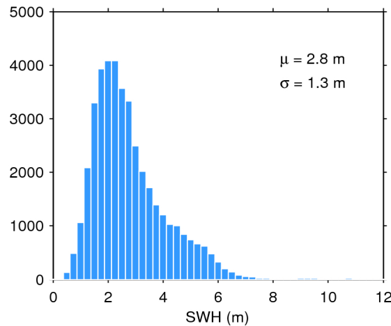
Figure 20. Histogram of science-valid SWH over oceans and lakes for 26/06/2020. The mean ( \mu ) and standard deviation ( \sigma ) are also shown. Note that values larger than 12 m are excluded from the histogram for the sake of readability but not from the computation of \mu and \sigma .
