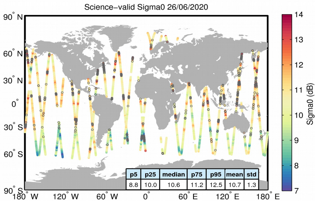
Figure 27. Geographical distribution of science-valid sigma0 data over oceans and lakes for 26/06/2020. The statistical values shown in the table refer to the sigma0 in dB and are calculated over all measurements shown in the figure. Gray circles denote records that have been rejected based on the editing criteria described in Table 4.
