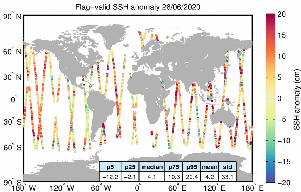
Figure 5. Geographical distribution of flag-valid 1-Hz SSH anomaly data over oceans and lakes for 26/06/2020. The statistical values shown in the table refer to the SSH anomaly in cm and are calculated over all measurements shown in the figure.
