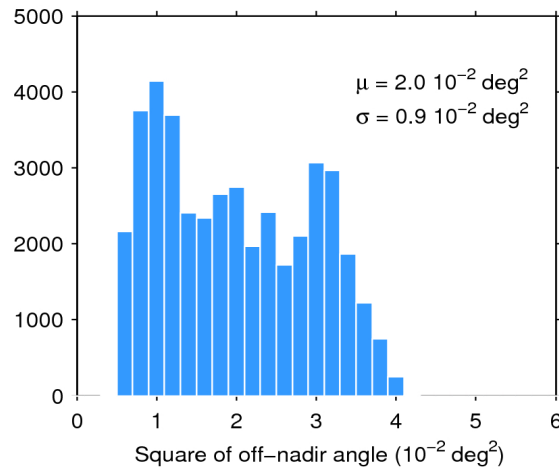
Figure 39. Histogram of flag-valid mispointing over oceans and lakes for 26/06/2020. The mean ( \mu ) and standard deviation ( \sigma ) are also shown. Note that values larger than 6 \cdot 10^{-2} \text{ deg}^2 are excluded from the histogram for the sake of readability but not from the computation of \mu and \sigma .
