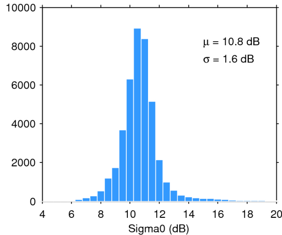
Figure 25. Histogram of flag-valid sigma0 over oceans and lakes for 26/06/2020. The mean ( \mu ) and standard deviation ( \sigma ) are also shown. Note that values outside [4 20] dB are excluded from the histogram for the sake of readability but not from the computation of \mu and \sigma .
