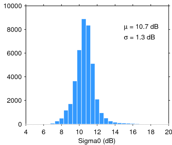
Figure 28. Histogram of science-valid sigma0 over oceans and lakes for 26/06/2020. The mean ( \mu ) and standard deviation ( \sigma ) are also shown. Note that values outside [4 20] dB are excluded from the histogram for the sake of readability but not from the computation of \mu and \sigma .
