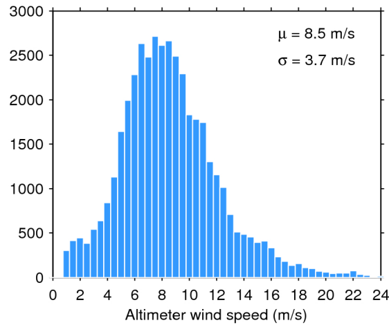
Figure 33. Histogram of flag-valid wind over oceans and lakes for 26/06/2020. The mean ( \mu ) and standard deviation ( \sigma ) are also shown. Note that values larger than 24 m/s are excluded from the histogram for the sake of readability but not from the computation of \mu and \sigma .
