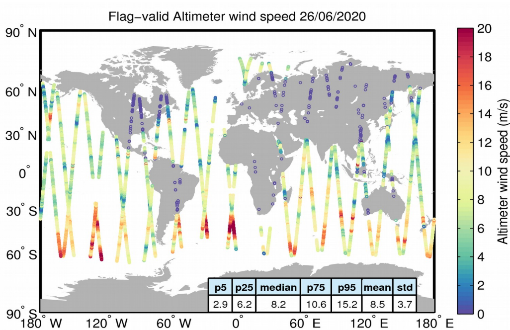
Figure 31. Geographical distribution of flag-valid wind data over oceans and lakes for 26/06/2020. The statistical values shown in the table refer to the wind in m/s and are calculated over all measurements shown in the figure.
