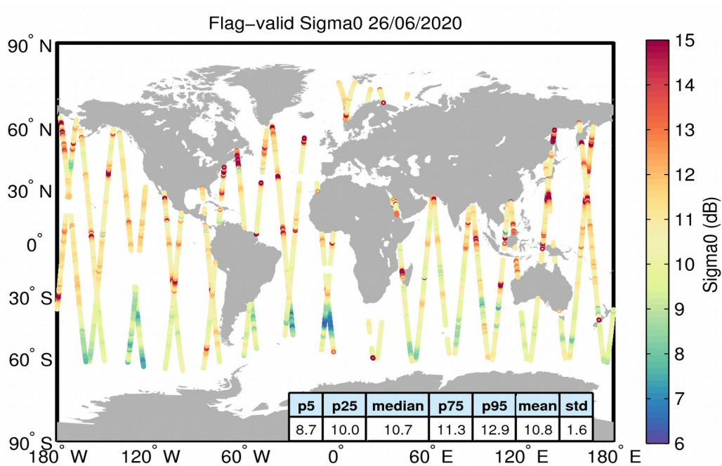
Figure 23. Geographical distribution of flag-valid sigma0 data over oceans and lakes for 26/06/2020. The statistical values shown in the table refer to the sigma0 in dB and are calculated over all measurements shown in the figure.
