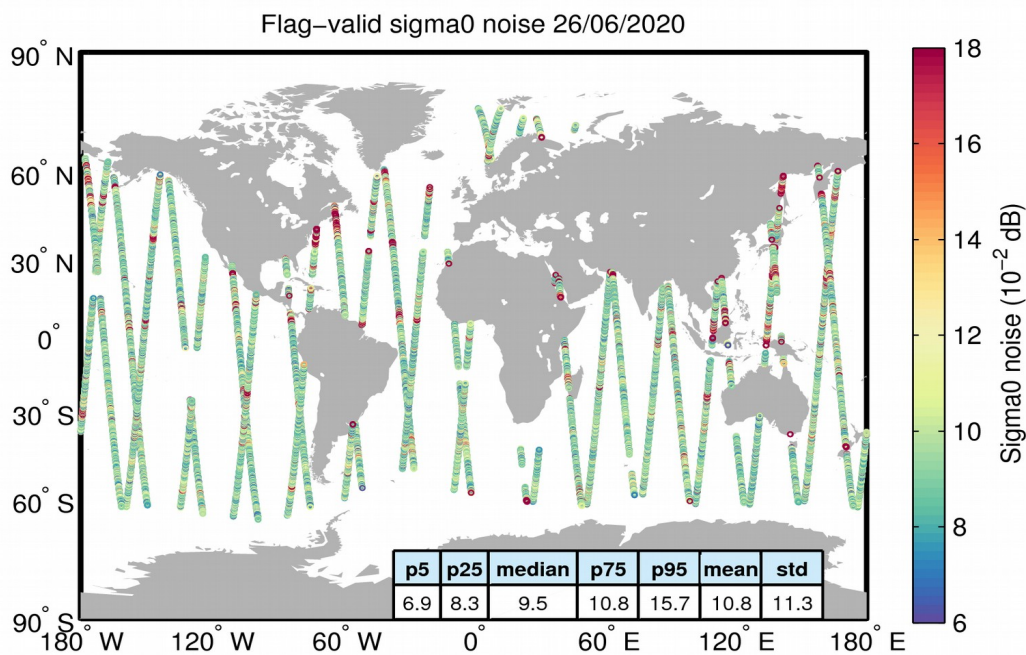
Figure 26. Geographical distribution of flag-valid 20-Hz sigma0 measurement noise over oceans and lakes for 26/06/2020. The statistical values shown in the table refer to the sigma0 noise and are calculated over all measurements shown in the figure.
