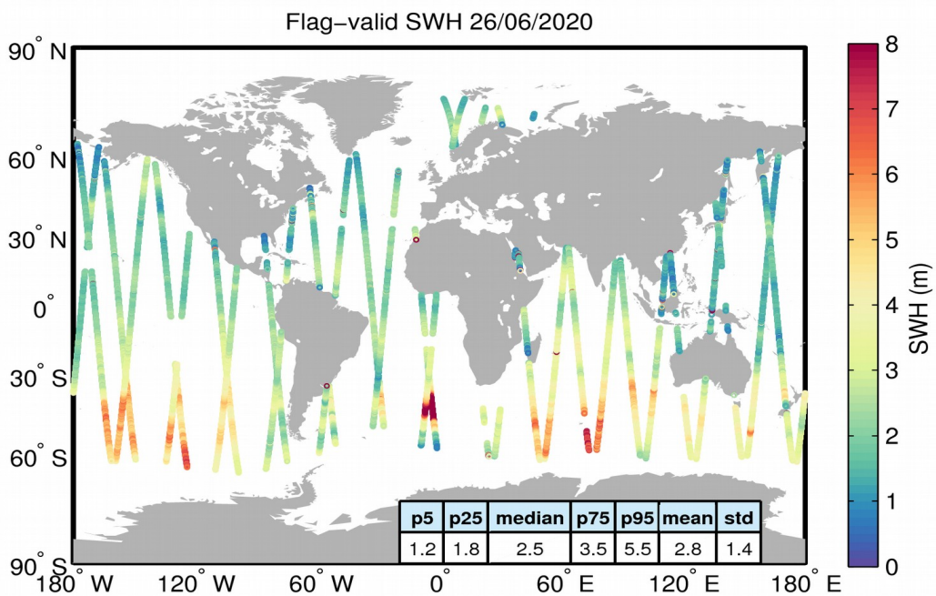
Figure 15. Geographical distribution of flag-valid SWH data over oceans and lakes for 26/06/2020. The statistical values shown in the table refer to the SWH in m and are calculated over all measurements shown in the figure.
