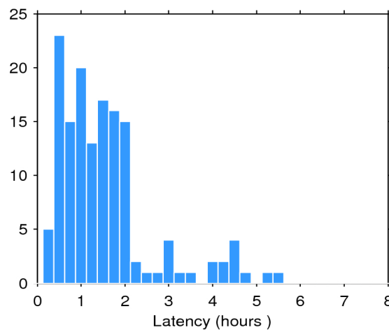
Figure 2. Histogram of the data latency for 26/06/2020. The y-axis denotes the number of files that are made available with a delay of x-hours with respect to the mean time of the records stored in the file.
