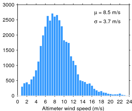
Figure 35. Histogram of science-valid wind over oceans and lakes for 26/06/2020. The mean ( \mu ) and standard deviation ( \sigma ) are also shown. Note that values larger than 24 m/s are excluded from the histogram for the sake of readability but not from the computation of \mu and \sigma .
