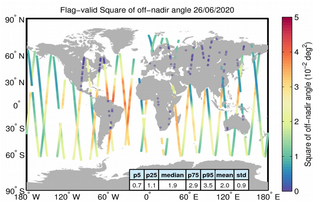
Figure 37. Geographical distribution of flag-valid mispointing data over oceans and lakes for 26/06/2020. The statistical values shown in the table refer to the mispointing in 10^{-2} \text{deg}^2 and are calculated over all measurements shown in the figure.
