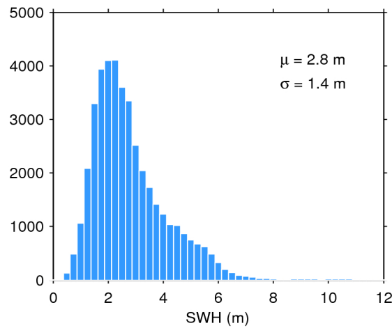
Figure 17. Histogram of flag-valid SWH over oceans and lakes for 26/06/2020. The mean ( \mu ) and standard deviation ( \sigma ) are also shown. Note that values larger than 12 m are excluded from the histogram for the sake of readability but not from the computation of \mu and \sigma .
