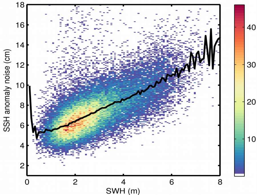
Figure 9. 2D histogram showing flag-valid SSH anomaly noise as a function of SWH for 26/06/2020. The black line denotes the median SSH anomaly noise as a function of SWH.
