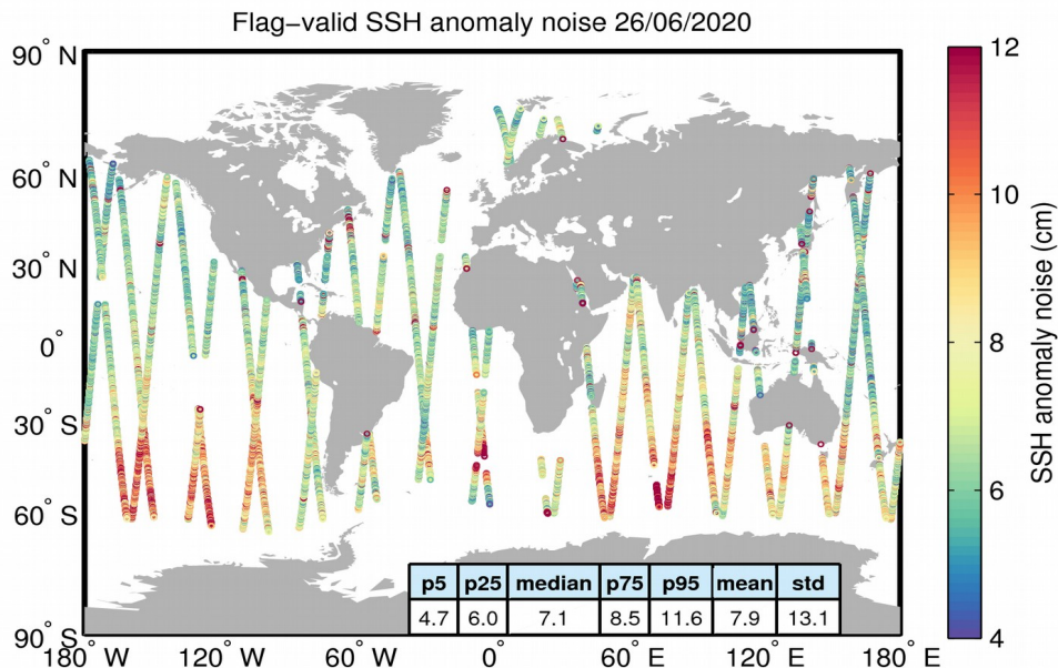
Figure 8. Geographical distribution of flag-valid 20-Hz SSH anomaly measurement noise over oceans and lakes for 26/06/2020. The statistical values shown in the table refer to the SSH anomaly noise and are calculated over all measurements shown in the figure.
