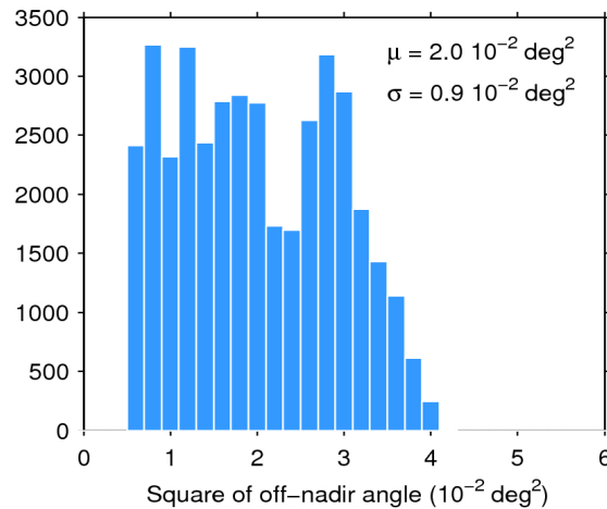
Figure 39. Histogram of flag-valid mispointing over oceans and lakes for 25/06/2020. The mean ( \mu ) and standard deviation ( \sigma ) are also shown. Note that values larger than 6 \cdot 10^{-2} \text{ deg}^2 are excluded from the histogram for the sake of readability but not from the computation of \mu and \sigma .
