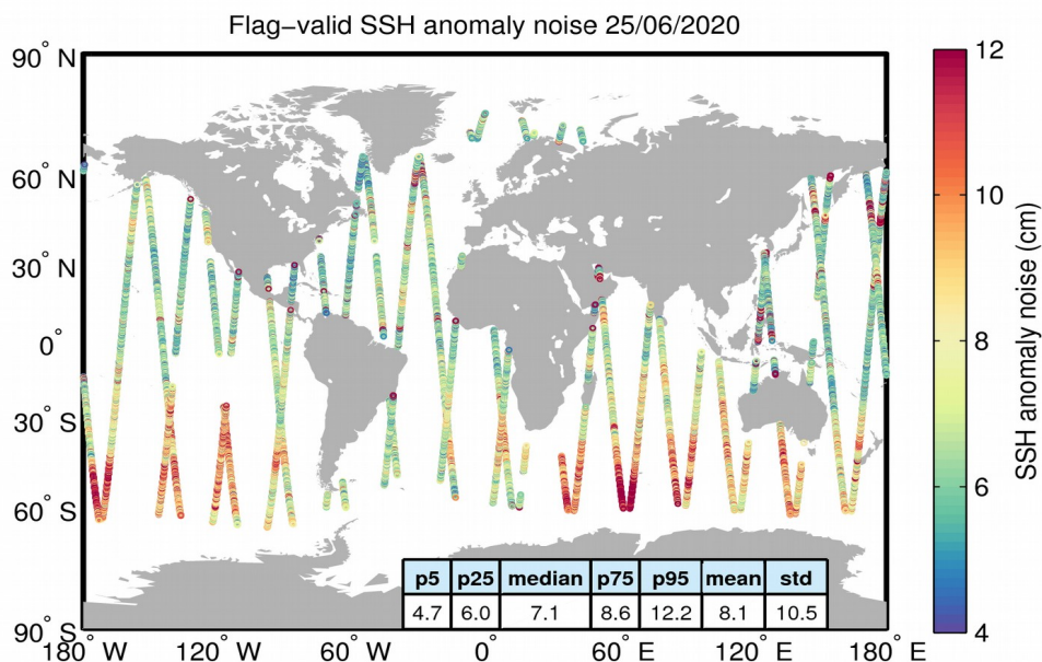
Figure 8. Geographical distribution of flag-valid 20-Hz SSH anomaly measurement noise over oceans and lakes for 25/06/2020. The statistical values shown in the table refer to the SSH anomaly noise and are calculated over all measurements shown in the figure.
