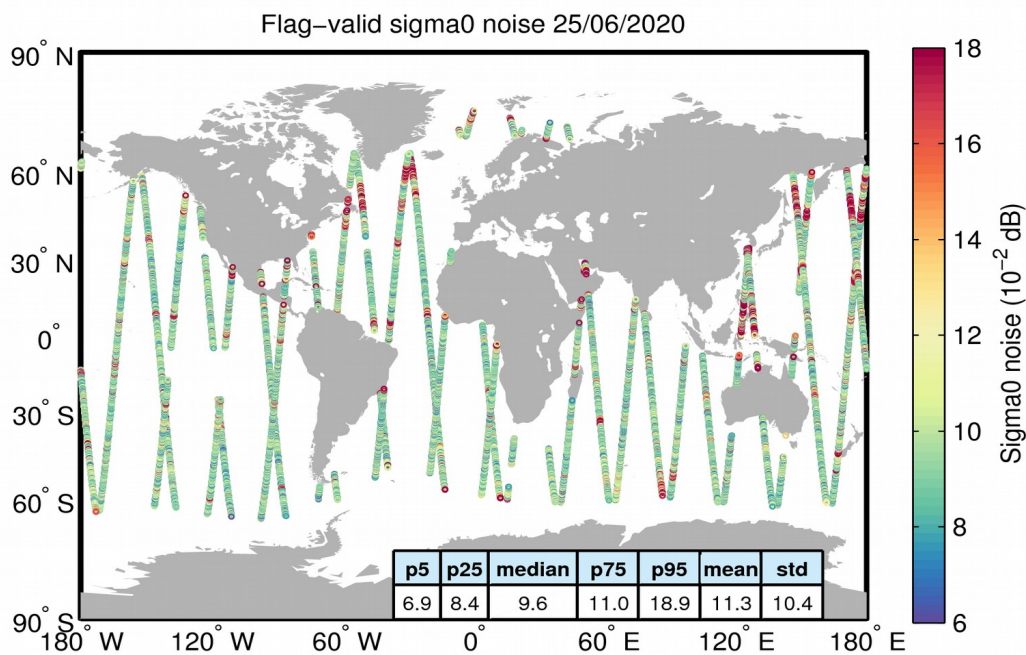
Figure 26. Geographical distribution of flag-valid 20-Hz sigma0 measurement noise over oceans and lakes for 25/06/2020. The statistical values shown in the table refer to the sigma0 noise and are calculated over all measurements shown in the figure.
