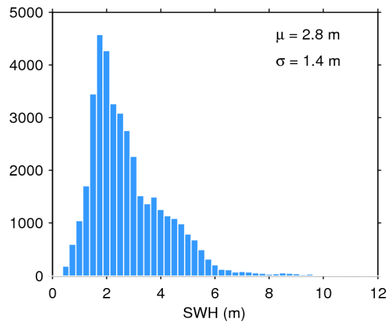
Figure 17. Histogram of flag-valid SWH over oceans and lakes for 25/06/2020. The mean ( \mu ) and standard deviation ( \sigma ) are also shown. Note that values larger than 12 m are excluded from the histogram for the sake of readability but not from the computation of \mu and \sigma .
