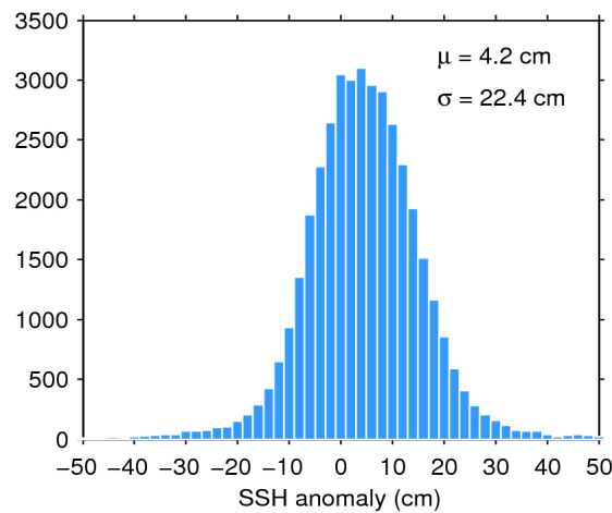
Figure 7. Histogram of flag-valid SSH anomaly over oceans and lakes for 25/06/2020. The mean ( \mu ) and standard deviation ( \sigma ) are also shown. Note that values outside [-50\ 50] cm are excluded from the histogram for the sake of readability but not from the computation of \mu and \sigma .
