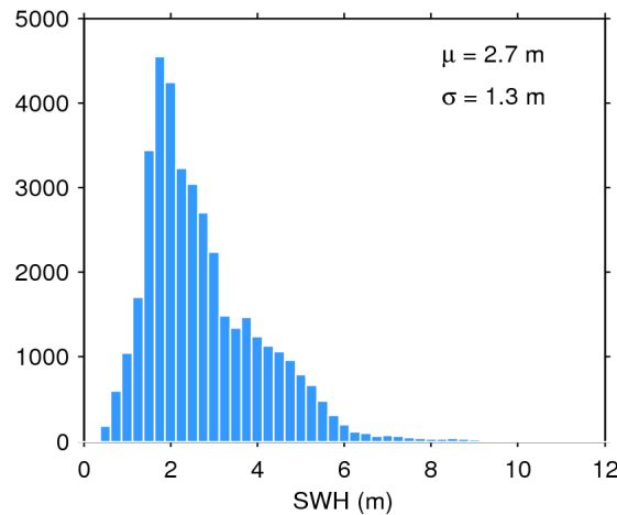
Figure 20. Histogram of science-valid SWH over oceans and lakes for 25/06/2020. The mean ( \mu ) and standard deviation ( \sigma ) are also shown. Note that values larger than 12 m are excluded from the histogram for the sake of readability but not from the computation of \mu and \sigma .
