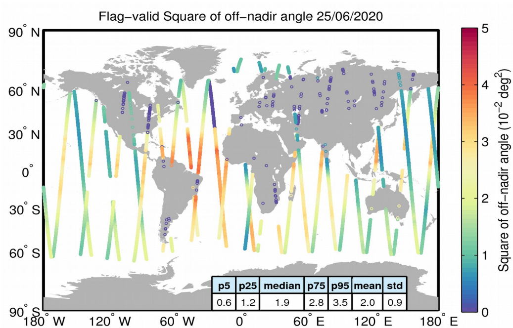
Figure 37. Geographical distribution of flag-valid mispointing data over oceans and lakes for 25/06/2020. The statistical values shown in the table refer to the mispointing in 10^{-2} \text{ deg}^2 and are calculated over all measurements shown in the figure.
