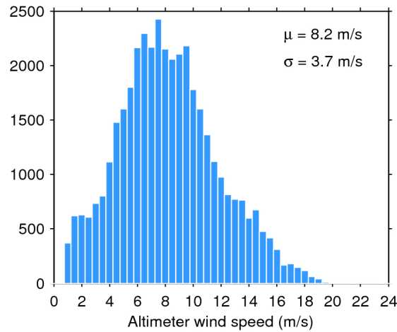
Figure 33. Histogram of flag-valid wind over oceans and lakes for 25/06/2020. The mean ( \mu ) and standard deviation ( \sigma ) are also shown. Note that values larger than 24 m/s are excluded from the histogram for the sake of readability but not from the computation of \mu and \sigma .
