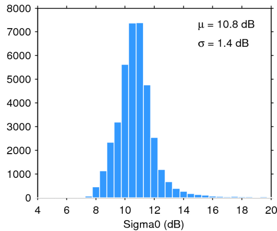
Figure 28. Histogram of science-valid sigma0 over oceans and lakes for 25/06/2020. The mean ( \mu ) and standard deviation ( \sigma ) are also shown. Note that values outside [4 20] dB are excluded from the histogram for the sake of readability but not from the computation of \mu and \sigma .
