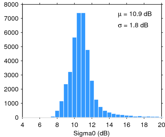
Figure 25. Histogram of flag-valid sigma0 over oceans and lakes for 25/06/2020. The mean ( \mu ) and standard deviation ( \sigma ) are also shown. Note that values outside [4 20] dB are excluded from the histogram for the sake of readability but not from the computation of \mu and \sigma .
