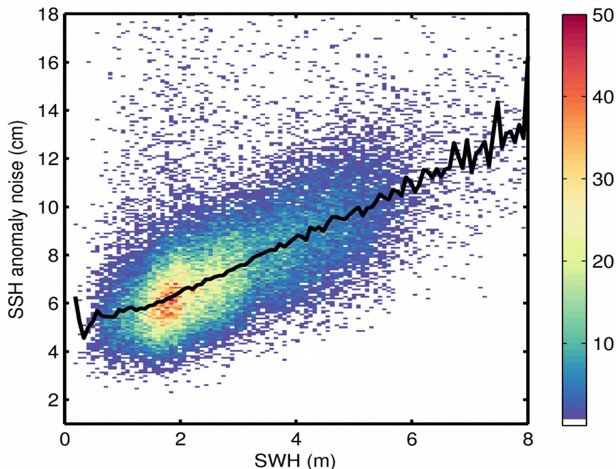
Figure 9. 2D histogram showing flag-valid SSH anomaly noise as a function of SWH for 25/06/2020. The black line denotes the median SSH anomaly noise as a function of SWH.
