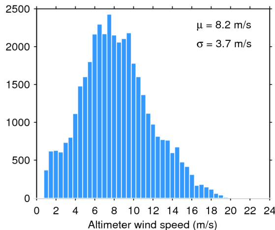
Figure 35. Histogram of science-valid wind over oceans and lakes for 25/06/2020. The mean ( \mu ) and standard deviation ( \sigma ) are also shown. Note that values larger than 24 m/s are excluded from the histogram for the sake of readability but not from the computation of \mu and \sigma .
