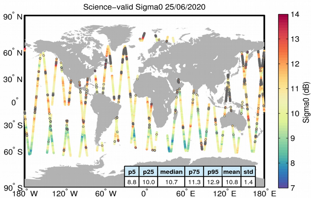
Figure 27. Geographical distribution of science-valid sigma0 data over oceans and lakes for 25/06/2020. The statistical values shown in the table refer to the sigma0 in dB and are calculated over all measurements shown in the figure. Gray circles denote records that have been rejected based on the editing criteria described in Table 4.
