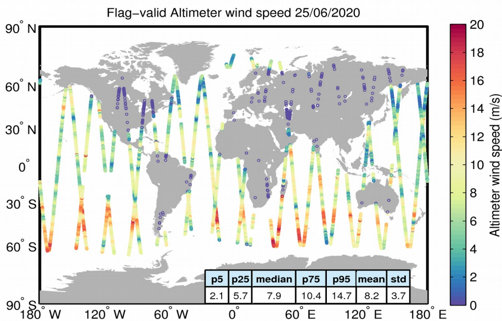
Figure 31. Geographical distribution of flag-valid wind data over oceans and lakes for 25/06/2020. The statistical values shown in the table refer to the wind in m/s and are calculated over all measurements shown in the figure.
