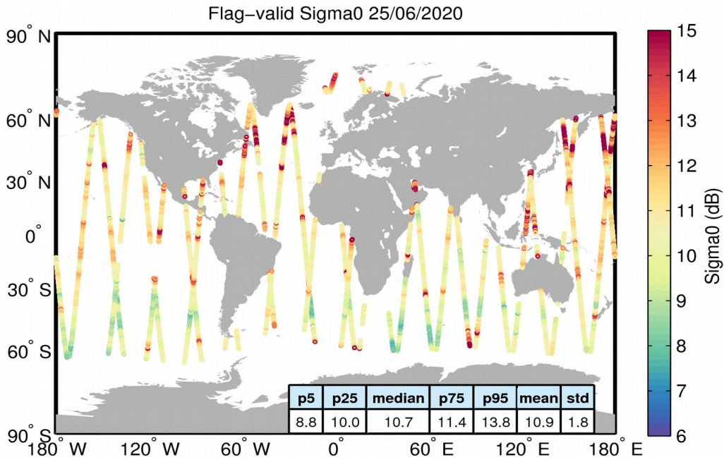
Figure 23. Geographical distribution of flag-valid sigma0 data over oceans and lakes for 25/06/2020. The statistical values shown in the table refer to the sigma0 in dB and are calculated over all measurements shown in the figure.
