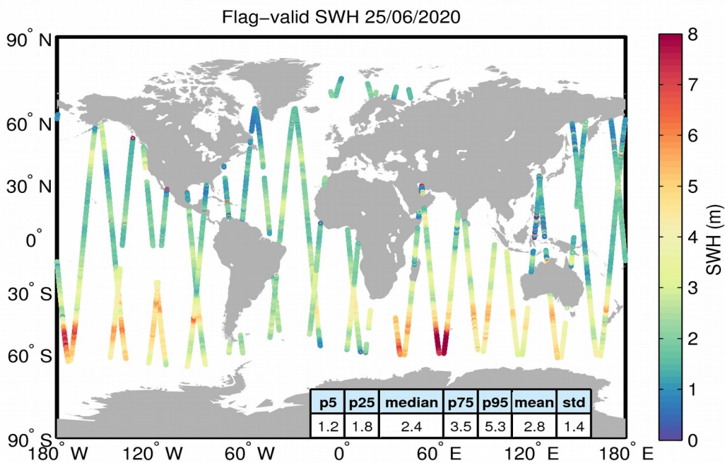
Figure 15. Geographical distribution of flag-valid SWH data over oceans and lakes for 25/06/2020. The statistical values shown in the table refer to the SWH in m and are calculated over all measurements shown in the figure.
