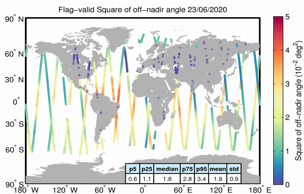
Figure 37. Geographical distribution of flag-valid mispointing data over oceans and lakes for 23/06/2020. The statistical values shown in the table refer to the mispointing in 10^{-2} \text{ deg}^2 and are calculated over all measurements shown in the figure.
