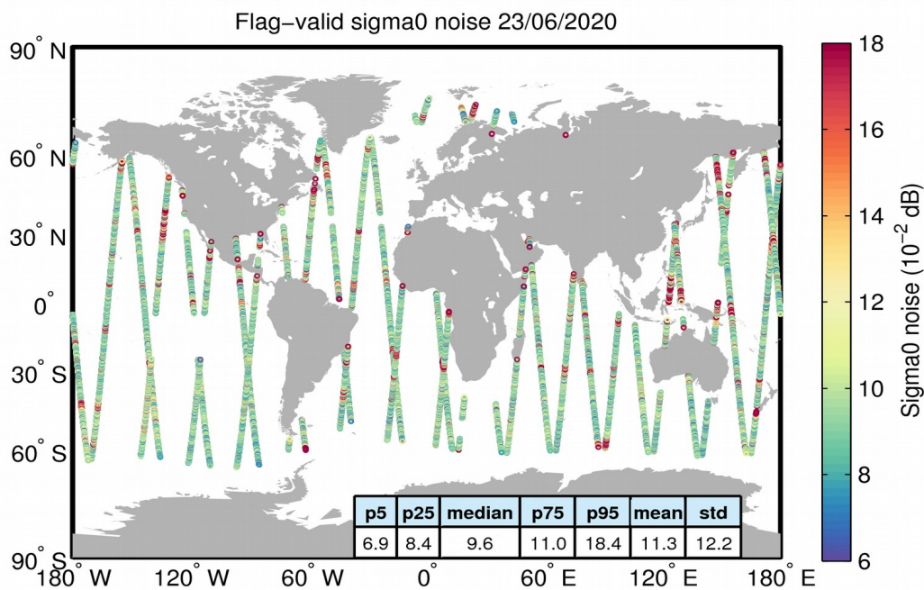
Figure 26. Geographical distribution of flag-valid 20-Hz sigma0 measurement noise over oceans and lakes for 23/06/2020. The statistical values shown in the table refer to the sigma0 noise and are calculated over all measurements shown in the figure.
