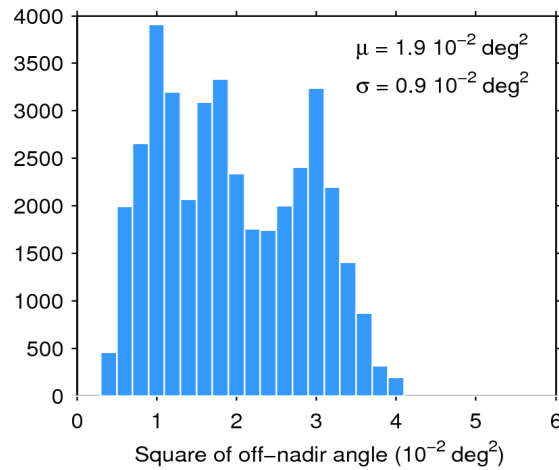
Figure 39. Histogram of flag-valid mispointing over oceans and lakes for 23/06/2020. The mean ( \mu ) and standard deviation ( \sigma ) are also shown. Note that values larger than 6 \cdot 10^{-2} \text{ deg}^2 are excluded from the histogram for the sake of readability but not from the computation of \mu and \sigma .
