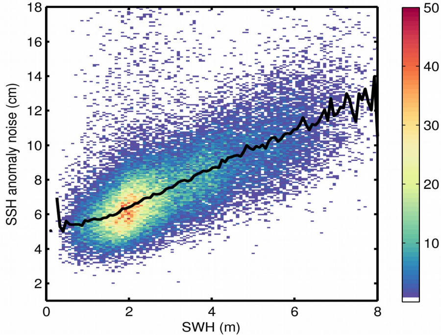
Figure 9. 2D histogram showing flag-valid SSH anomaly noise as a function of SWH for 23/06/2020. The black line denotes the median SSH anomaly noise as a function of SWH.
