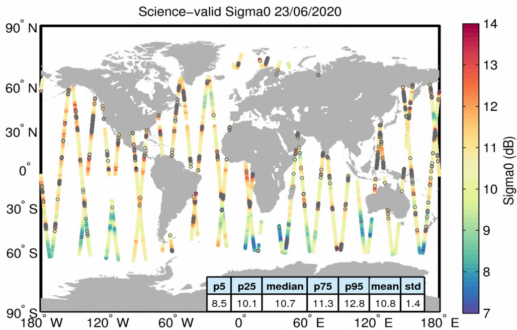
Figure 27. Geographical distribution of science-valid sigma0 data over oceans and lakes for 23/06/2020. The statistical values shown in the table refer to the sigma0 in dB and are calculated over all measurements shown in the figure. Gray circles denote records that have been rejected based on the editing criteria described in Table 4.
