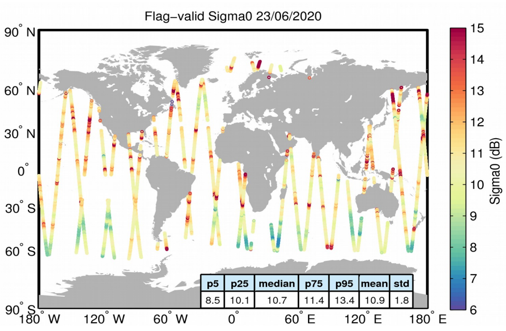
Figure 23. Geographical distribution of flag-valid sigma0 data over oceans and lakes for 23/06/2020. The statistical values shown in the table refer to the sigma0 in dB and are calculated over all measurements shown in the figure.
