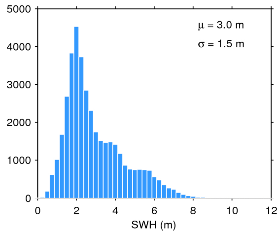
Figure 17. Histogram of flag-valid SWH over oceans and lakes for 23/06/2020. The mean ( \mu ) and standard deviation ( \sigma ) are also shown. Note that values larger than 12 m are excluded from the histogram for the sake of readability but not from the computation of \mu and \sigma .
