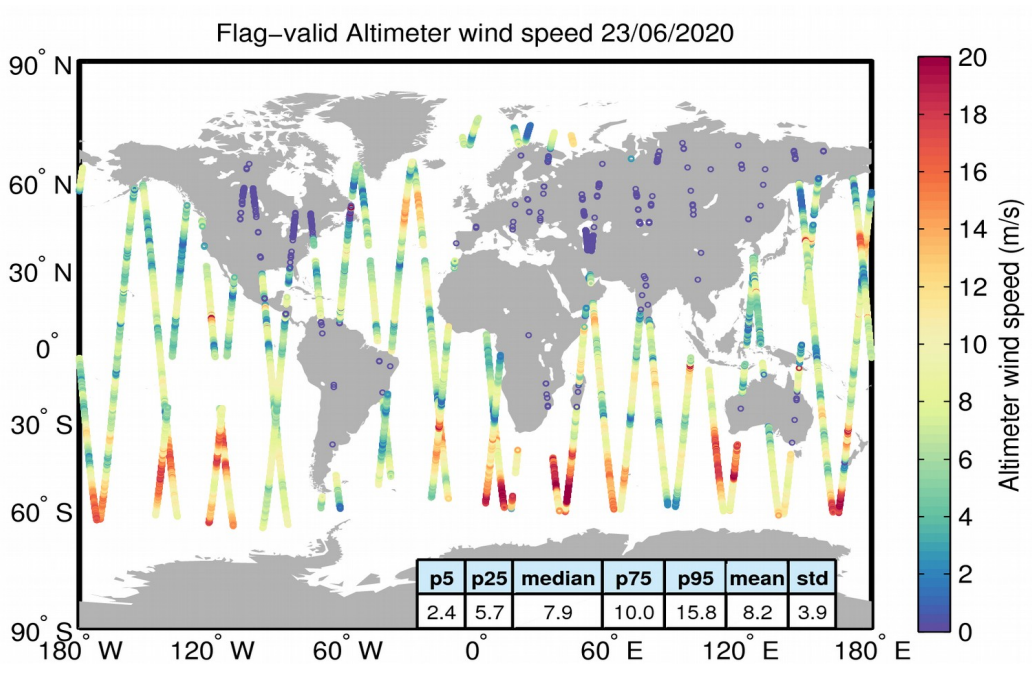
Figure 31. Geographical distribution of flag-valid wind data over oceans and lakes for 23/06/2020. The statistical values shown in the table refer to the wind in m/s and are calculated over all measurements shown in the figure.
