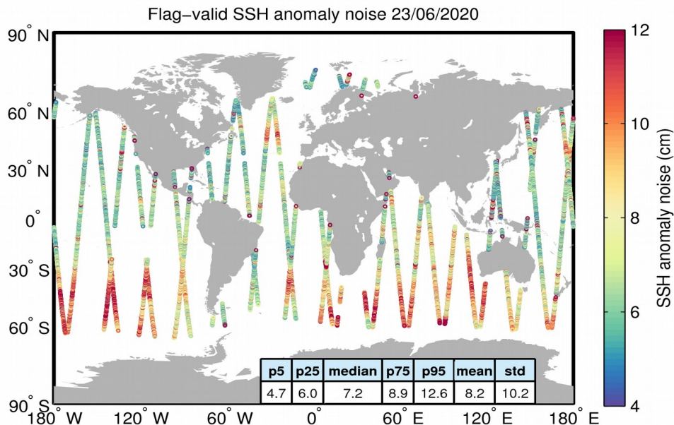
Figure 8. Geographical distribution of flag-valid 20-Hz SSH anomaly measurement noise over oceans and lakes for 23/06/2020. The statistical values shown in the table refer to the SSH anomaly noise and are calculated over all measurements shown in the figure.
