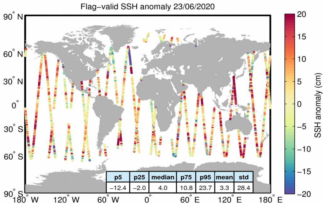
Figure 5. Geographical distribution of flag-valid 1-Hz SSH anomaly data over oceans and lakes for 23/06/2020. The statistical values shown in the table refer to the SSH anomaly in cm and are calculated over all measurements shown in the figure.
