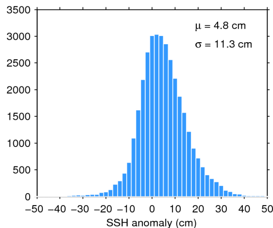
Figure 11. Histogram of science-valid SSH anomaly over oceans and lakes for 23/06/2020. The mean ( \mu ) and standard deviation ( \sigma ) are also shown. Note that values outside [-50 50] cm are excluded from the histogram for the sake of readability but not from the computation of \mu and \sigma .
