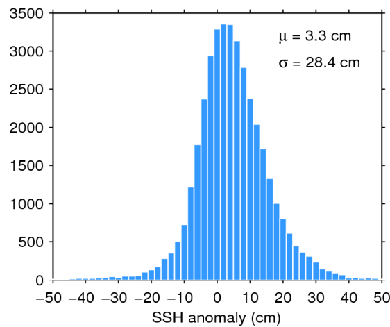
Figure 7. Histogram of flag-valid SSH anomaly over oceans and lakes for 23/06/2020. The mean ( \mu ) and standard deviation ( \sigma ) are also shown. Note that values outside [-50 50] cm are excluded from the histogram for the sake of readability but not from the computation of \mu and \sigma .
