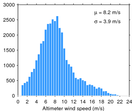
Figure 35. Histogram of science-valid wind over oceans and lakes for 23/06/2020. The mean ( \mu ) and standard deviation ( \sigma ) are also shown. Note that values larger than 24 m/s are excluded from the histogram for the sake of readability but not from the computation of \mu and \sigma .
