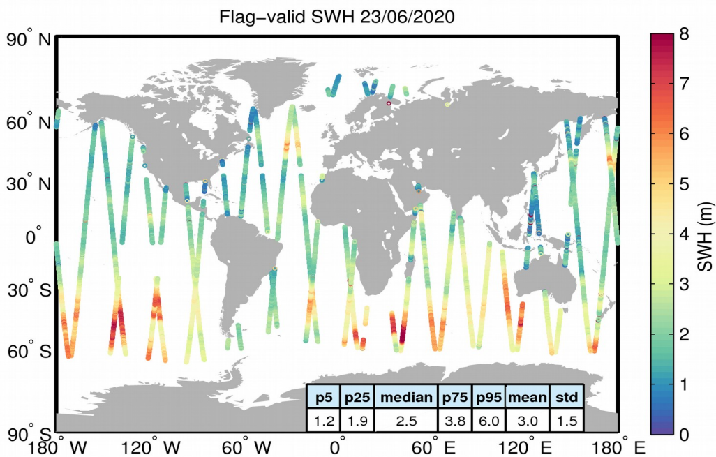
Figure 15. Geographical distribution of flag-valid SWH data over oceans and lakes for 23/06/2020. The statistical values shown in the table refer to the SWH in m and are calculated over all measurements shown in the figure.
