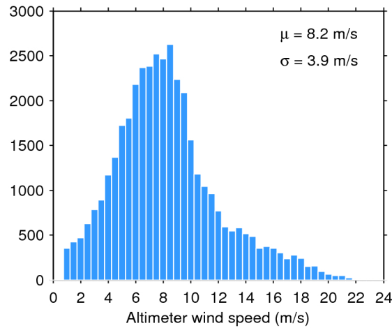
Figure 33. Histogram of flag-valid wind over oceans and lakes for 23/06/2020. The mean ( \mu ) and standard deviation ( \sigma ) are also shown. Note that values larger than 24 m/s are excluded from the histogram for the sake of readability but not from the computation of \mu and \sigma .
