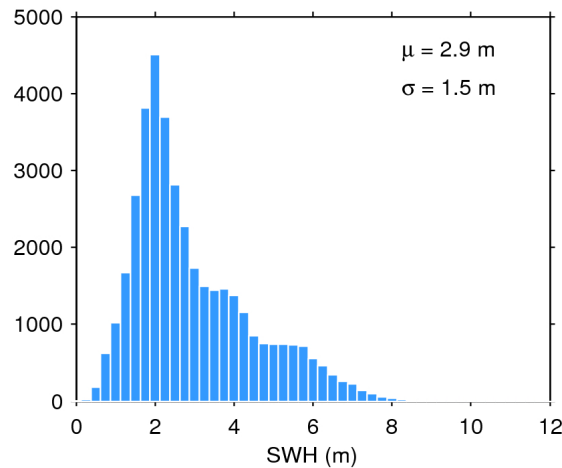
Figure 20. Histogram of science-valid SWH over oceans and lakes for 23/06/2020. The mean ( \mu ) and standard deviation ( \sigma ) are also shown. Note that values larger than 12 m are excluded from the histogram for the sake of readability but not from the computation of \mu and \sigma .
