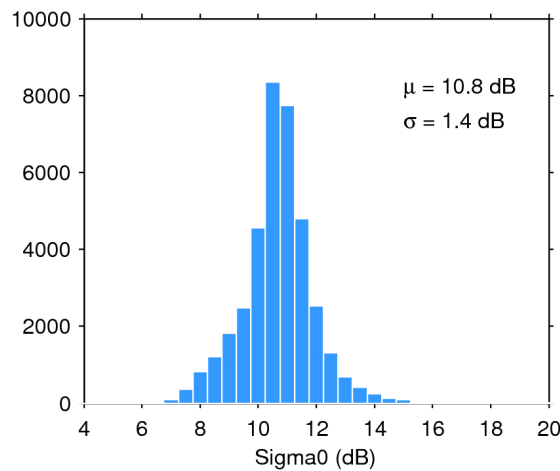
Figure 28. Histogram of science-valid sigma0 over oceans and lakes for 23/06/2020. The mean ( \mu ) and standard deviation ( \sigma ) are also shown. Note that values outside [4 20] dB are excluded from the histogram for the sake of readability but not from the computation of \mu and \sigma .
