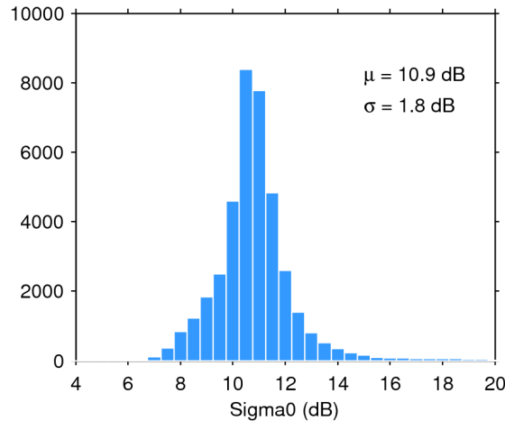
Figure 25. Histogram of flag-valid sigma0 over oceans and lakes for 23/06/2020. The mean ( \mu ) and standard deviation ( \sigma ) are also shown. Note that values outside [4 20] dB are excluded from the histogram for the sake of readability but not from the computation of \mu and \sigma .
