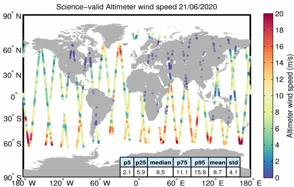
Figure 34. Geographical distribution of science-valid wind data over oceans and lakes for 21/06/2020. The statistical values shown in the table refer to the wind in m/s and are calculated over all measurements shown in the figure. Gray circles denote records that have been rejected based on the editing criteria described in Table 5.
