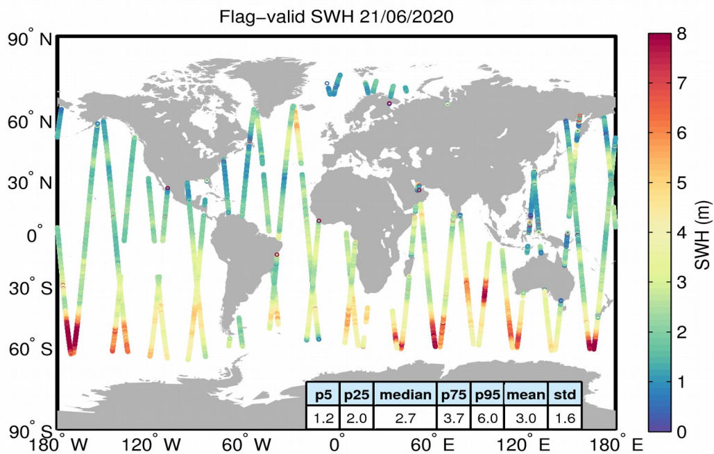
Figure 15. Geographical distribution of flag-valid SWH data over oceans and lakes for 21/06/2020. The statistical values shown in the table refer to the SWH in m and are calculated over all measurements shown in the figure.
