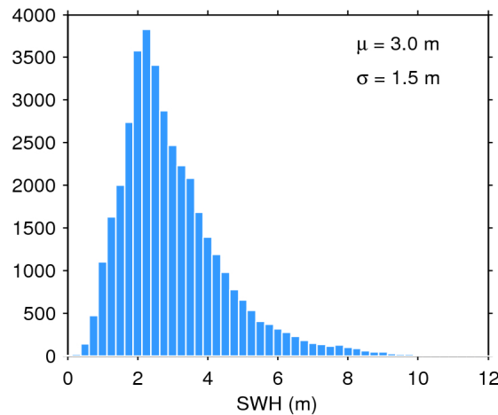
Figure 20. Histogram of science-valid SWH over oceans and lakes for 21/06/2020. The mean ( \mu ) and standard deviation ( \sigma ) are also shown. Note that values larger than 12 m are excluded from the histogram for the sake of readability but not from the computation of \mu and \sigma .
