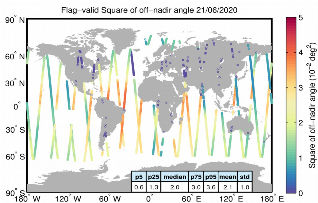
Figure 37. Geographical distribution of flag-valid mispointing data over oceans and lakes for 21/06/2020. The statistical values shown in the table refer to the mispointing in 10^{-2} \text{ deg}^2 and are calculated over all measurements shown in the figure.
