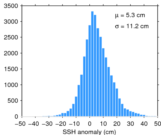
Figure 11. Histogram of science-valid SSH anomaly over oceans and lakes for 21/06/2020. The mean ( \mu ) and standard deviation ( \sigma ) are also shown. Note that values outside [-50 50] cm are excluded from the histogram for the sake of readability but not from the computation of \mu and \sigma .
