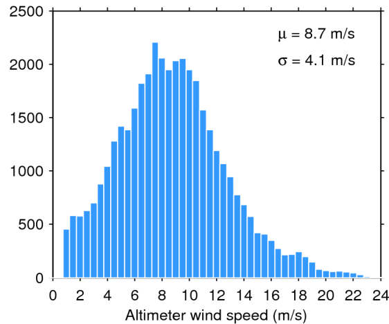
Figure 33. Histogram of flag-valid wind over oceans and lakes for 21/06/2020. The mean ( \mu ) and standard deviation ( \sigma ) are also shown. Note that values larger than 24 m/s are excluded from the histogram for the sake of readability but not from the computation of \mu and \sigma .
