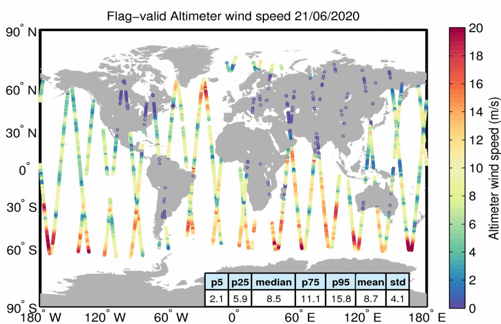
Figure 31. Geographical distribution of flag-valid wind data over oceans and lakes for 21/06/2020. The statistical values shown in the figure refer to the wind in m/s and are calculated over all measurements shown in the figure.
