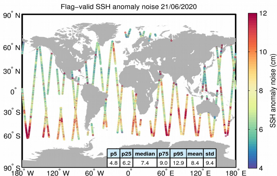
Figure 8. Geographical distribution of flag-valid 20-Hz SSH anomaly measurement noise over oceans and lakes for 21/06/2020. The statistical values shown in the table refer to the SSH anomaly noise and are calculated over all measurements shown in the figure.
