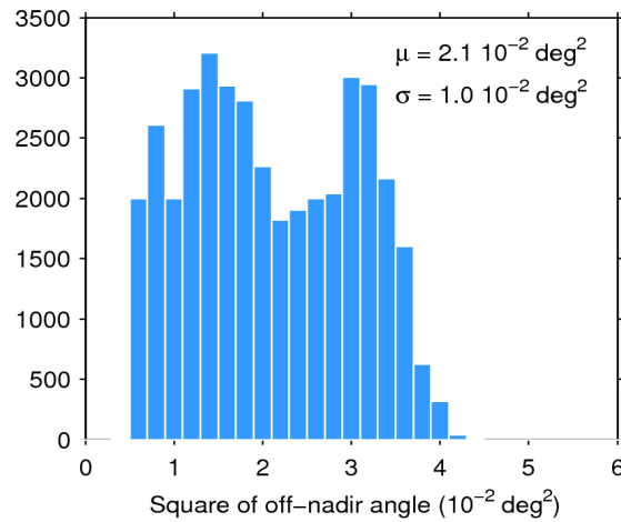
Figure 39. Histogram of flag-valid mispointing over oceans and lakes for 21/06/2020. The mean ( \mu ) and standard deviation ( \sigma ) are also shown. Note that values larger than 6 \cdot 10^{-2} \text{ deg}^2 are excluded from the histogram for the sake of readability but not from the computation of \mu and \sigma .
