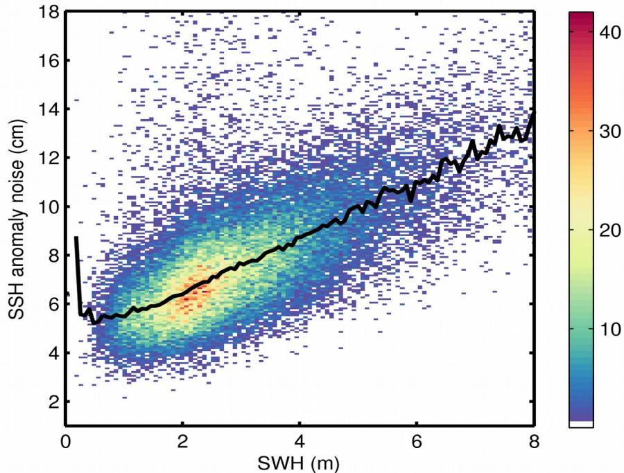
Figure 9. 2D histogram showing flag-valid SSH anomaly noise as a function of SWH for 21/06/2020. The black line denotes the median SSH anomaly noise as a function of SWH.
