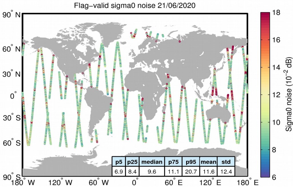
Figure 26. Geographical distribution of flag-valid 20-Hz sigma0 measurement noise over oceans and lakes for 21/06/2020. The statistical values shown in the table refer to the sigma0 noise and are calculated over all measurements shown in the figure.
