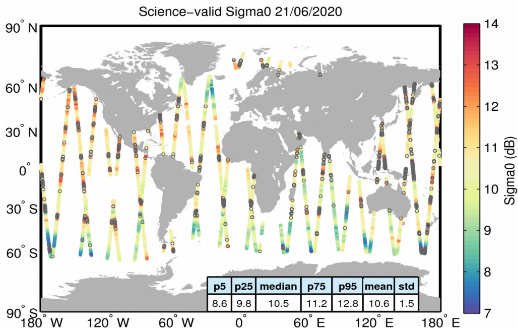
Figure 27. Geographical distribution of science-valid sigma0 data over oceans and lakes for 21/06/2020. The statistical values shown in the table refer to the sigma0 in dB and are calculated over all measurements shown in the figure. Gray circles denote records that have been rejected based on the editing criteria described in Table 4.
