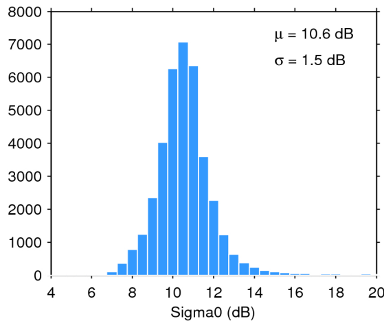
Figure 28. Histogram of science-valid sigma0 over oceans and lakes for 21/06/2020. The mean ( \mu ) and standard deviation ( \sigma ) are also shown. Note that values outside [4 20] dB are excluded from the histogram for the sake of readability but not from the computation of \mu and \sigma .
