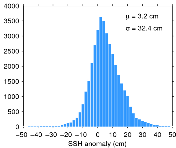
Figure 7. Histogram of flag-valid SSH anomaly over oceans and lakes for 21/06/2020. The mean ( \mu ) and standard deviation ( \sigma ) are also shown. Note that values outside [-50 50] cm are excluded from the histogram for the sake of readability but not from the computation of \mu and \sigma .
