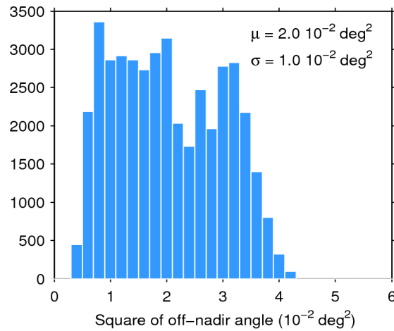
Figure 39. Histogram of flag-valid mispointing over oceans and lakes for 18/06/2020. The mean ( \mu ) and standard deviation ( \sigma ) are also shown. Note that values larger than 6 \cdot 10^{-2} \text{ deg}^2 are excluded from the histogram for the sake of readability but not from the computation of \mu and \sigma .
