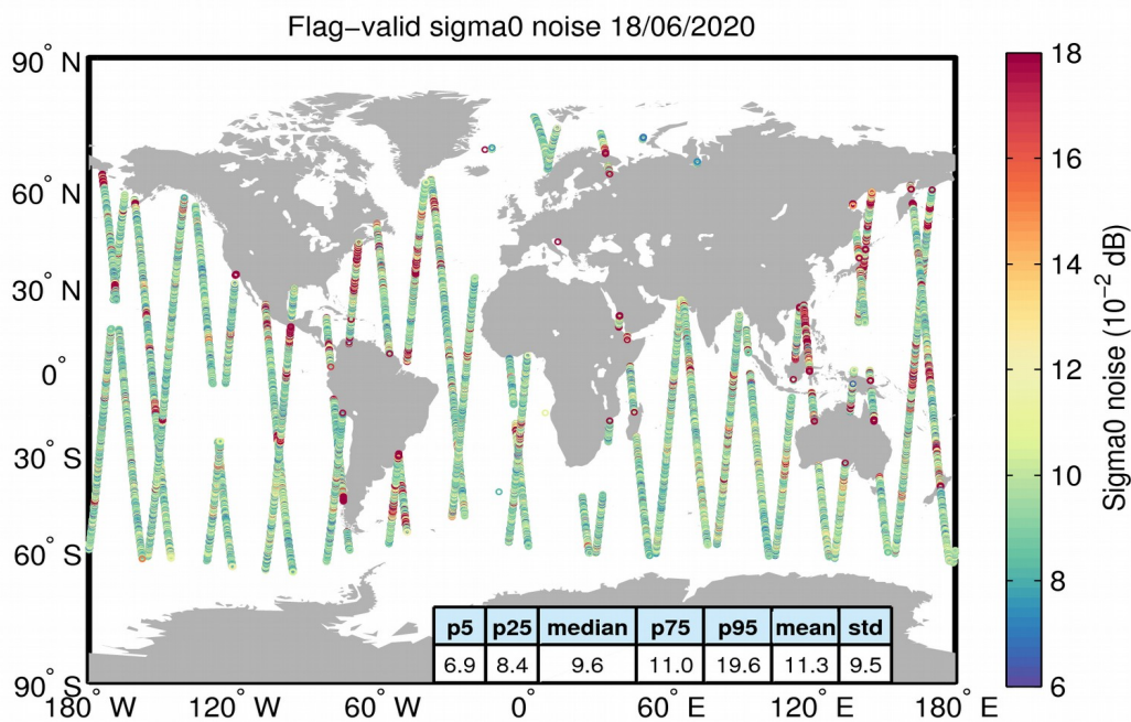
Figure 26. Geographical distribution of flag-valid 20-Hz sigma0 measurement noise over oceans and lakes for 18/06/2020. The statistical values shown in the table refer to the sigma0 noise and are calculated over all measurements shown in the figure.
