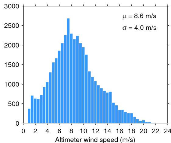
Figure 35. Histogram of science-valid wind over oceans and lakes for 18/06/2020. The mean ( \mu ) and standard deviation ( \sigma ) are also shown. Note that values larger than 24 m/s are excluded from the histogram for the sake of readability but not from the computation of \mu and \sigma .
