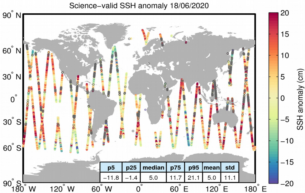
Figure 10. Geographical distribution of science-valid SSH anomaly data over oceans and lakes for 18/06/2020. The statistical values shown in the table refer to the SSH anomaly in cm and are calculated over all measurements shown in the figure. Gray circles denote records that have been rejected based on the editing criteria described in Table 2.
