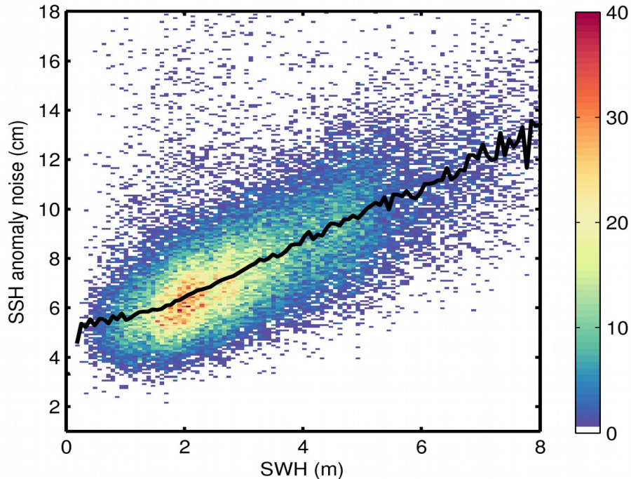
Figure 9. 2D histogram showing flag-valid SSH anomaly noise as a function of SWH for 18/06/2020. The black line denotes the median SSH anomaly noise as a function of SWH.
