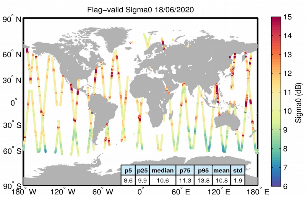
Figure 23. Geographical distribution of flag-valid sigma0 data over oceans and lakes for 18/06/2020. The statistical values shown in the table refer to the sigma0 in dB and are calculated over all measurements shown in the figure.
