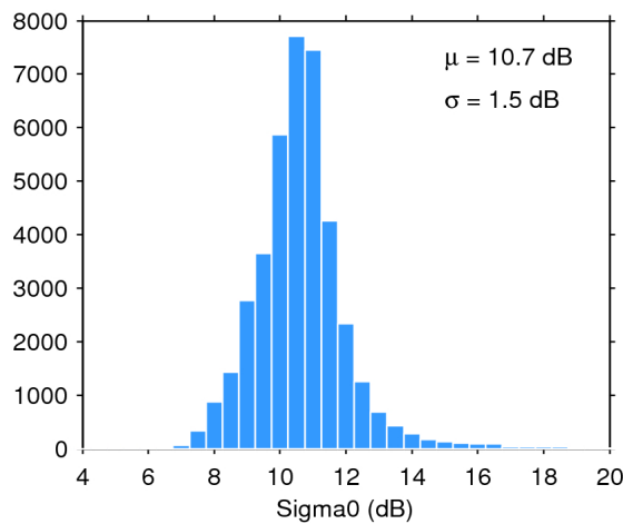
Figure 28. Histogram of science-valid sigma0 over oceans and lakes for 18/06/2020. The mean ( \mu ) and standard deviation ( \sigma ) are also shown. Note that values outside [4 20] dB are excluded from the histogram for the sake of readability but not from the computation of \mu and \sigma .
