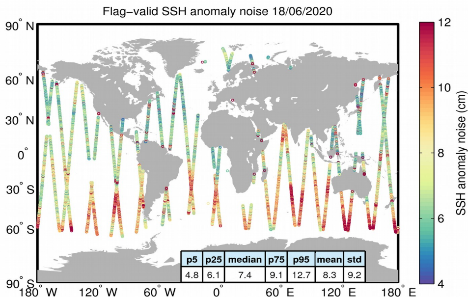
Figure 8. Geographical distribution of flag-valid 20-Hz SSH anomaly measurement noise over oceans and lakes for 18/06/2020. The statistical values shown in the table refer to the SSH anomaly noise and are calculated over all measurements shown in the figure.
