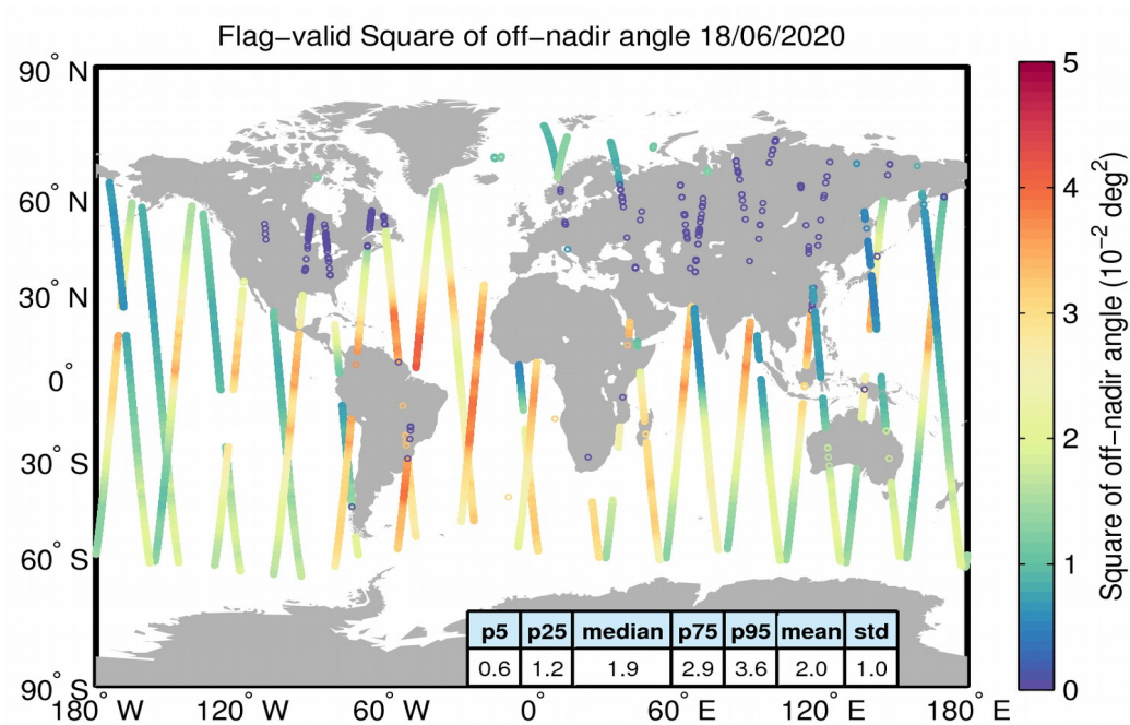
Figure 37. Geographical distribution of flag-valid mispointing data over oceans and lakes for 18/06/2020. The statistical values shown in the table refer to the mispointing in 10^{-2} \text{ deg}^2 and are calculated over all measurements shown in the figure.
