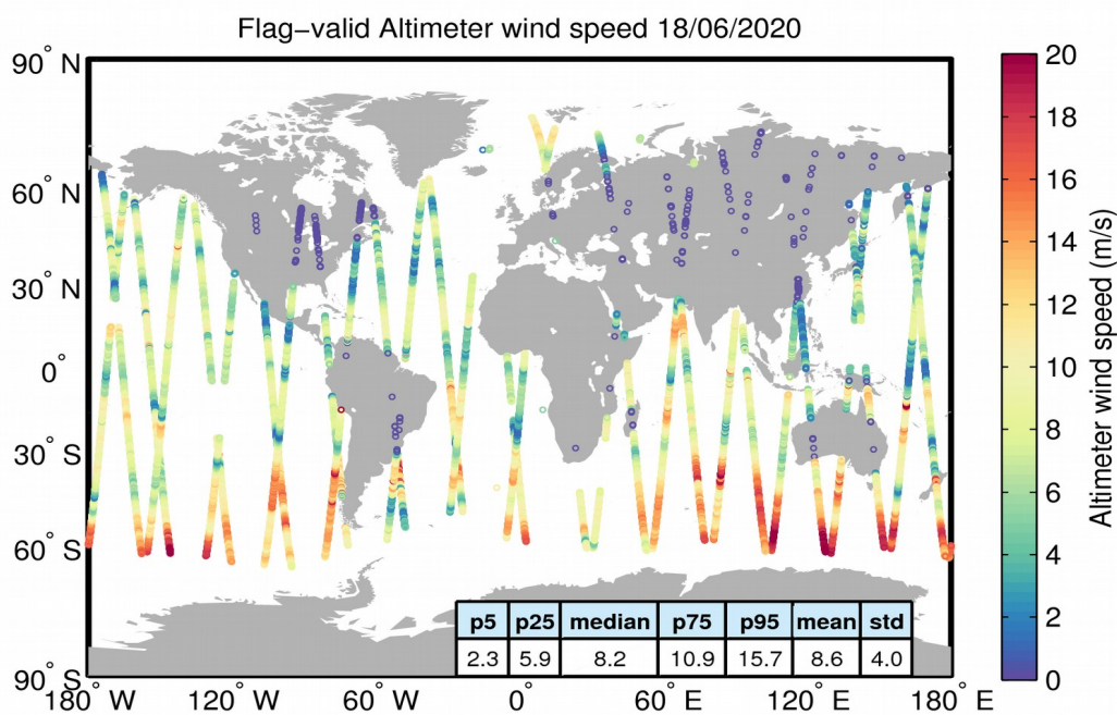
Figure 31. Geographical distribution of flag-valid wind data over oceans and lakes for 18/06/2020. The statistical values shown in the table refer to the wind in m/s and are calculated over all measurements shown in the figure.
