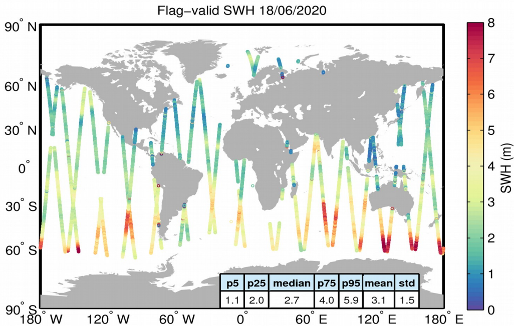
Figure 15. Geographical distribution of flag-valid SWH data over oceans and lakes for 18/06/2020. The statistical values shown in the table refer to the SWH in m and are calculated over all measurements shown in the figure.
