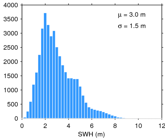
Figure 20. Histogram of science-valid SWH over oceans and lakes for 18/06/2020. The mean ( \mu ) and standard deviation ( \sigma ) are also shown. Note that values larger than 12 m are excluded from the histogram for the sake of readability but not from the computation of \mu and \sigma .
