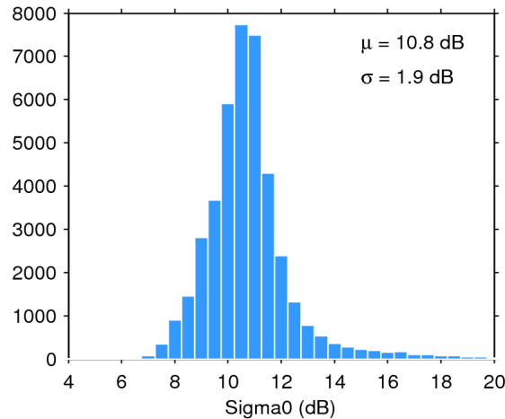
Figure 25. Histogram of flag-valid sigma0 over oceans and lakes for 18/06/2020. The mean ( \mu ) and standard deviation ( \sigma ) are also shown. Note that values outside [4 20] dB are excluded from the histogram for the sake of readability but not from the computation of \mu and \sigma .
