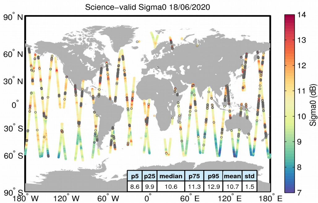
Figure 27. Geographical distribution of science-valid sigma0 data over oceans and lakes for 18/06/2020. The statistical values shown in the table refer to the sigma0 in dB and are calculated over all measurements shown in the figure. Gray circles denote records that have been rejected based on the editing criteria described in Table 4.
