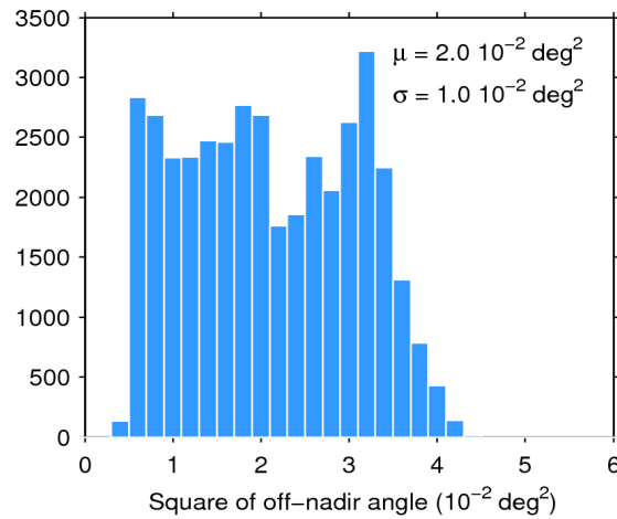
Figure 39. Histogram of flag-valid mispointing over oceans and lakes for 17/06/2020. The mean ( \mu ) and standard deviation ( \sigma ) are also shown. Note that values larger than 6 \cdot 10^{-2} \text{ deg}^2 are excluded from the histogram for the sake of readability but not from the computation of \mu and \sigma .
