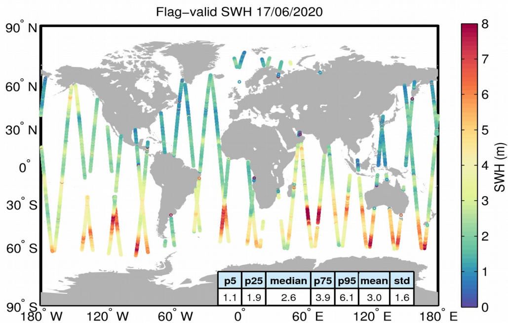
Figure 15. Geographical distribution of flag-valid SWH data over oceans and lakes for 17/06/2020. The statistical values shown in the table refer to the SWH in m and are calculated over all measurements shown in the figure.
