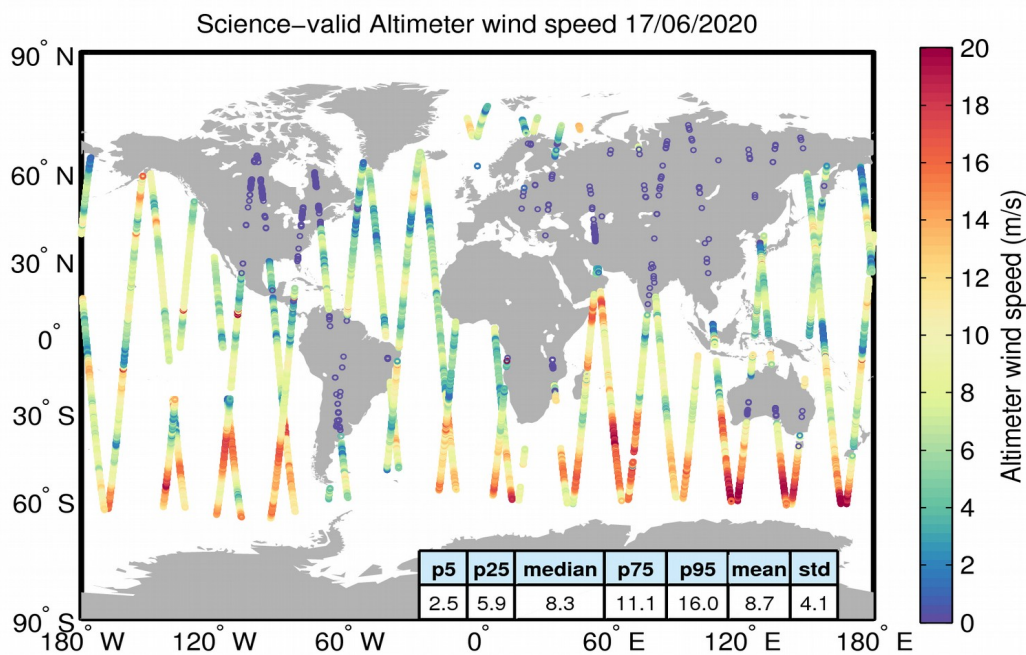
Figure 34. Geographical distribution of science-valid wind data over oceans and lakes for 17/06/2020. The statistical values shown in the table refer to the wind in m/s and are calculated over all measurements shown in the figure. Gray circles denote records that have been rejected based on the editing criteria described in Table 5.
