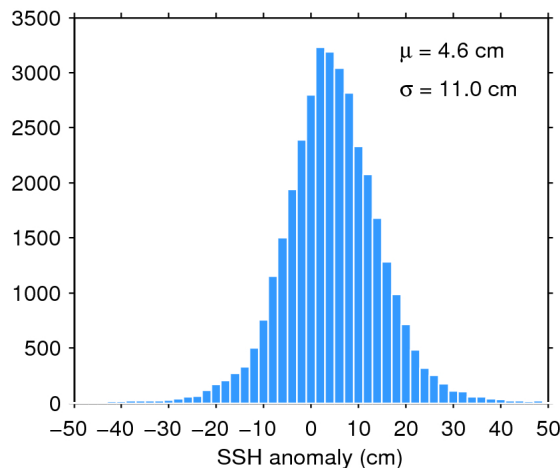
Figure 11. Histogram of science-valid SSH anomaly over oceans and lakes for 17/06/2020. The mean ( \mu ) and standard deviation ( \sigma ) are also shown. Note that values outside [-50 50] cm are excluded from the histogram for the sake of readability but not from the computation of \mu and \sigma .
