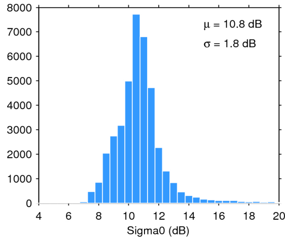
Figure 25. Histogram of flag-valid sigma0 over oceans and lakes for 17/06/2020. The mean ( \mu ) and standard deviation ( \sigma ) are also shown. Note that values outside [4 20] dB are excluded from the histogram for the sake of readability but not from the computation of \mu and \sigma .
