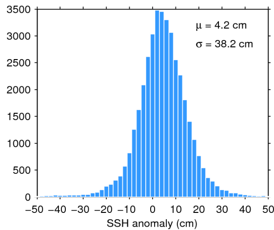
Figure 7. Histogram of flag-valid SSH anomaly over oceans and lakes for 17/06/2020. The mean ( \mu ) and standard deviation ( \sigma ) are also shown. Note that values outside [-50\ 50] cm are excluded from the histogram for the sake of readability but not from the computation of \mu and \sigma .
