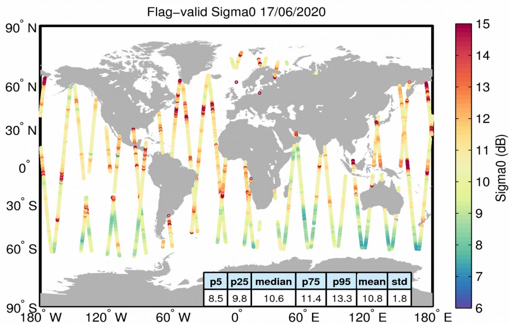
Figure 23. Geographical distribution of flag-valid sigma0 data over oceans and lakes for 17/06/2020. The statistical values shown in the table refer to the sigma0 in dB and are calculated over all measurements shown in the figure.
