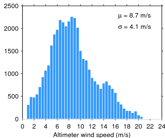
Figure 35. Histogram of science-valid wind over oceans and lakes for 17/06/2020. The mean ( \mu ) and standard deviation ( \sigma ) are also shown. Note that values larger than 24 m/s are excluded from the histogram for the sake of readability but not from the computation of \mu and \sigma .
