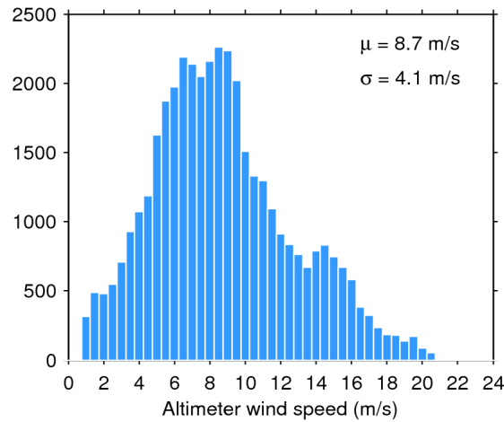
Figure 33. Histogram of flag-valid wind over oceans and lakes for 17/06/2020. The mean ( \mu ) and standard deviation ( \sigma ) are also shown. Note that values larger than 24 m/s are excluded from the histogram for the sake of readability but not from the computation of \mu and \sigma .
