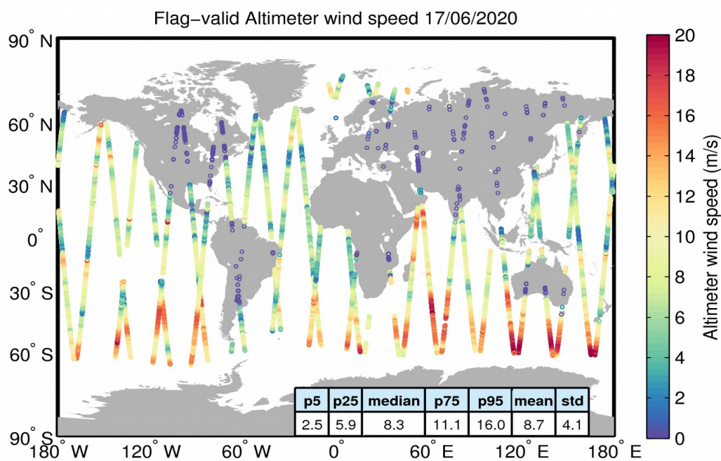
Figure 31. Geographical distribution of flag-valid wind data over oceans and lakes for 17/06/2020. The statistical values shown in the table refer to the wind in m/s and are calculated over all measurements shown in the figure.
