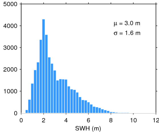
Figure 20. Histogram of science-valid SWH over oceans and lakes for 17/06/2020. The mean ( \mu ) and standard deviation ( \sigma ) are also shown. Note that values larger than 12 m are excluded from the histogram for the sake of readability but not from the computation of \mu and \sigma .
