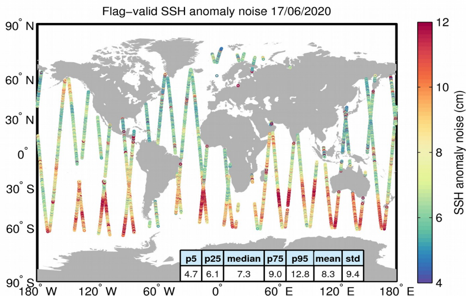
Figure 8. Geographical distribution of flag-valid 20-Hz SSH anomaly measurement noise over oceans and lakes for 17/06/2020. The statistical values shown in the table refer to the SSH anomaly noise and are calculated over all measurements shown in the figure.
