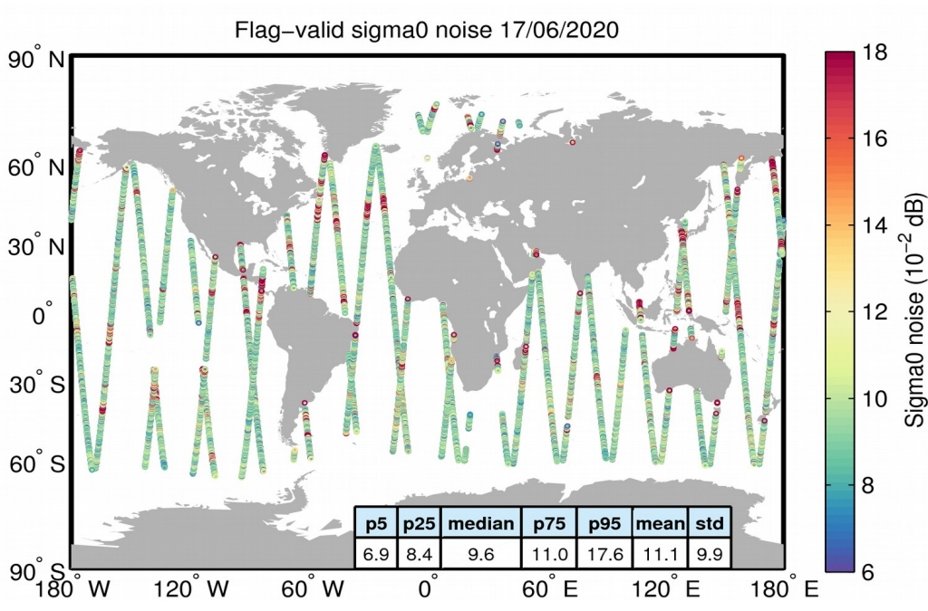
Figure 26. Geographical distribution of flag-valid 20-Hz sigma0 measurement noise over oceans and lakes for 17/06/2020. The statistical values shown in the table refer to the sigma0 noise and are calculated over all measurements shown in the figure.
