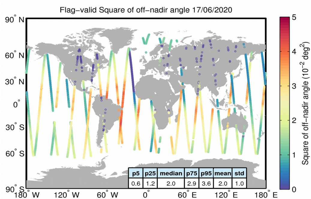
Figure 37. Geographical distribution of flag-valid mispointing data over oceans and lakes for 17/06/2020. The statistical values shown in the table refer to the mispointing in 10^{-2} \text{ deg}^2 and are calculated over all measurements shown in the figure.
