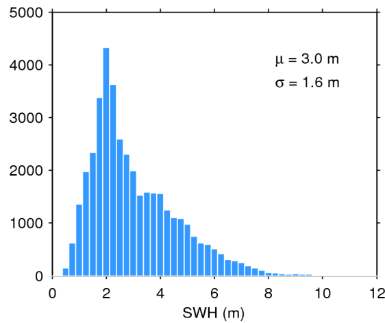
Figure 17. Histogram of flag-valid SWH over oceans and lakes for 17/06/2020. The mean ( \mu ) and standard deviation ( \sigma ) are also shown. Note that values larger than 12 m are excluded from the histogram for the sake of readability but not from the computation of \mu and \sigma .
