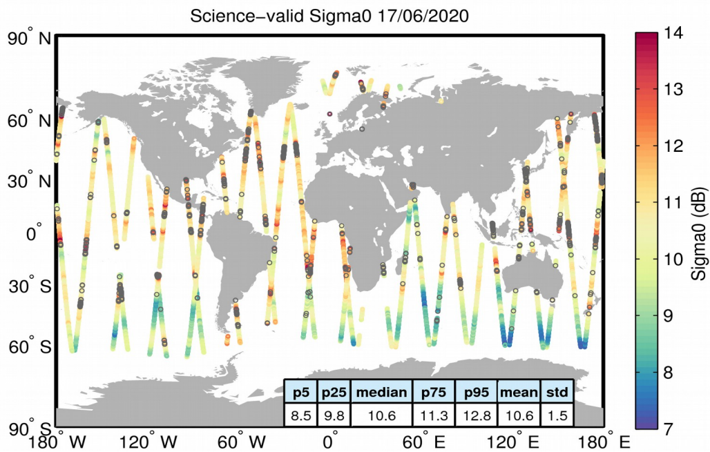
Figure 27. Geographical distribution of science-valid sigma0 data over oceans and lakes for 17/06/2020. The statistical values shown in the table refer to the sigma0 in dB and are calculated over all measurements shown in the figure. Gray circles denote records that have been rejected based on the editing criteria described in Table 4.
