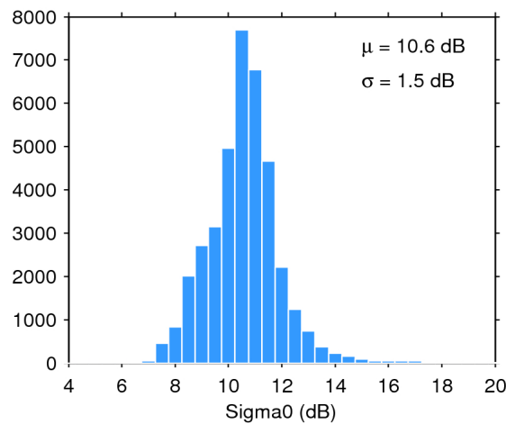
Figure 28. Histogram of science-valid sigma0 over oceans and lakes for 17/06/2020. The mean ( \mu ) and standard deviation ( \sigma ) are also shown. Note that values outside [4 20] dB are excluded from the histogram for the sake of readability but not from the computation of \mu and \sigma .
