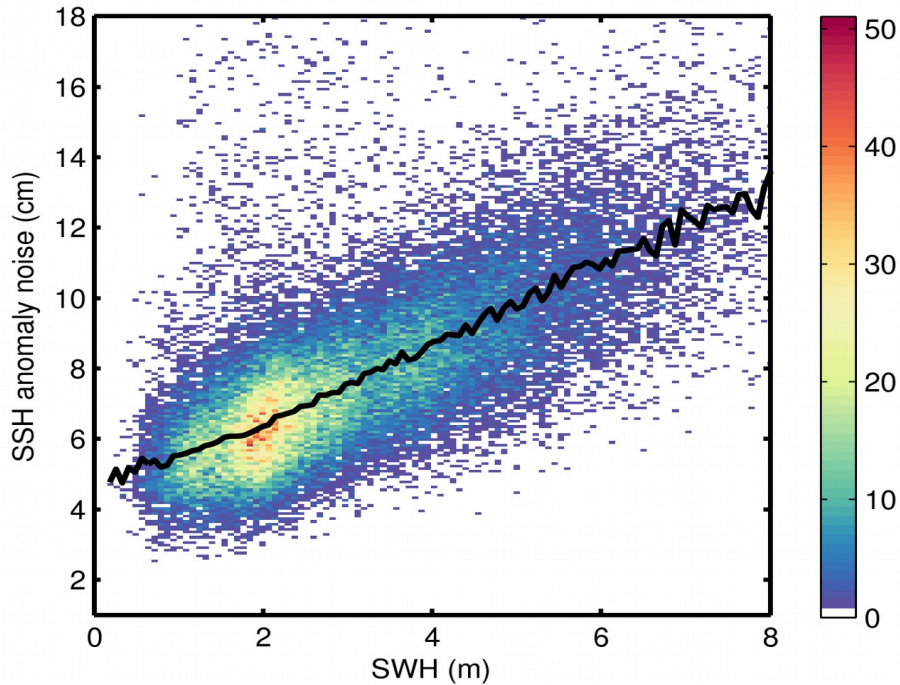
Figure 9. 2D histogram showing flag-valid SSH anomaly noise as a function of SWH for 17/06/2020. The black line denotes the median SSH anomaly noise as a function of SWH.
