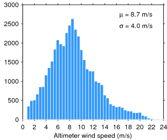
Figure 33. Histogram of flag-valid wind over oceans and lakes for 16/06/2020. The mean ( \mu ) and standard deviation ( \sigma ) are also shown. Note that values larger than 24 m/s are excluded from the histogram for the sake of readability but not from the computation of \mu and \sigma .
