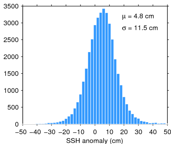
Figure 11. Histogram of science-valid SSH anomaly over oceans and lakes for 16/06/2020. The mean ( \mu ) and standard deviation ( \sigma ) are also shown. Note that values outside [-50 50] cm are excluded from the histogram for the sake of readability but not from the computation of \mu and \sigma .
