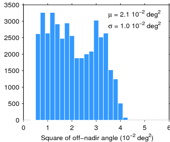
Figure 39. Histogram of flag-valid mispointing over oceans and lakes for 16/06/2020. The mean ( \mu ) and standard deviation ( \sigma ) are also shown. Note that values larger than 6 \cdot 10^{-2} \text{ deg}^2 are excluded from the histogram for the sake of readability but not from the computation of \mu and \sigma .
