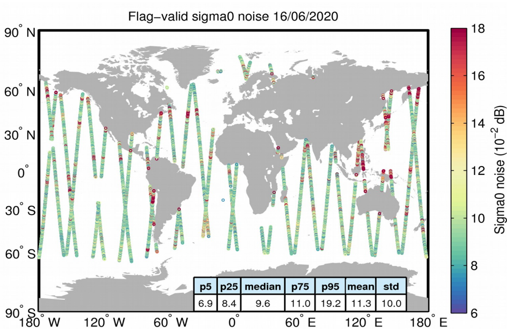
Figure 26. Geographical distribution of flag-valid 20-Hz sigma0 measurement noise over oceans and lakes for 16/06/2020. The statistical values shown in the table refer to the sigma0 noise and are calculated over all measurements shown in the figure.
