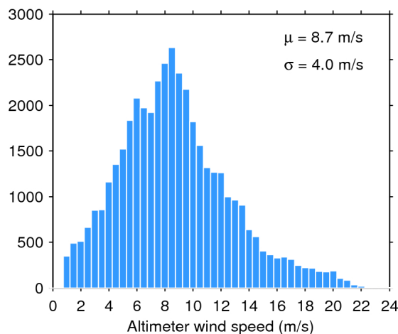
Figure 35. Histogram of science-valid wind over oceans and lakes for 16/06/2020. The mean ( \mu ) and standard deviation ( \sigma ) are also shown. Note that values larger than 24 m/s are excluded from the histogram for the sake of readability but not from the computation of \mu and \sigma .
