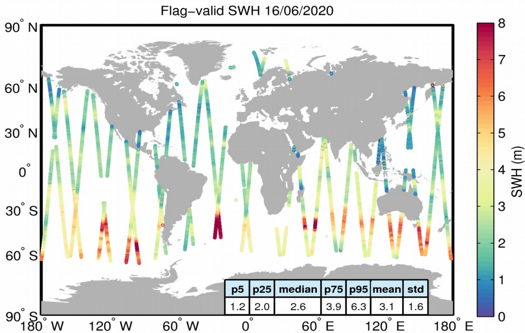
Figure 15. Geographical distribution of flag-valid SWH data over oceans and lakes for 16/06/2020. The statistical values shown in the table refer to the SWH in m and are calculated over all measurements shown in the figure.
