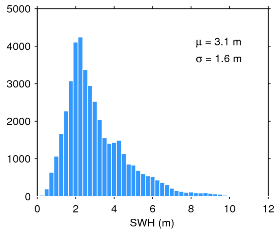
Figure 17. Histogram of flag-valid SWH over oceans and lakes for 16/06/2020. The mean ( \mu ) and standard deviation ( \sigma ) are also shown. Note that values larger than 12 m are excluded from the histogram for the sake of readability but not from the computation of \mu and \sigma .
