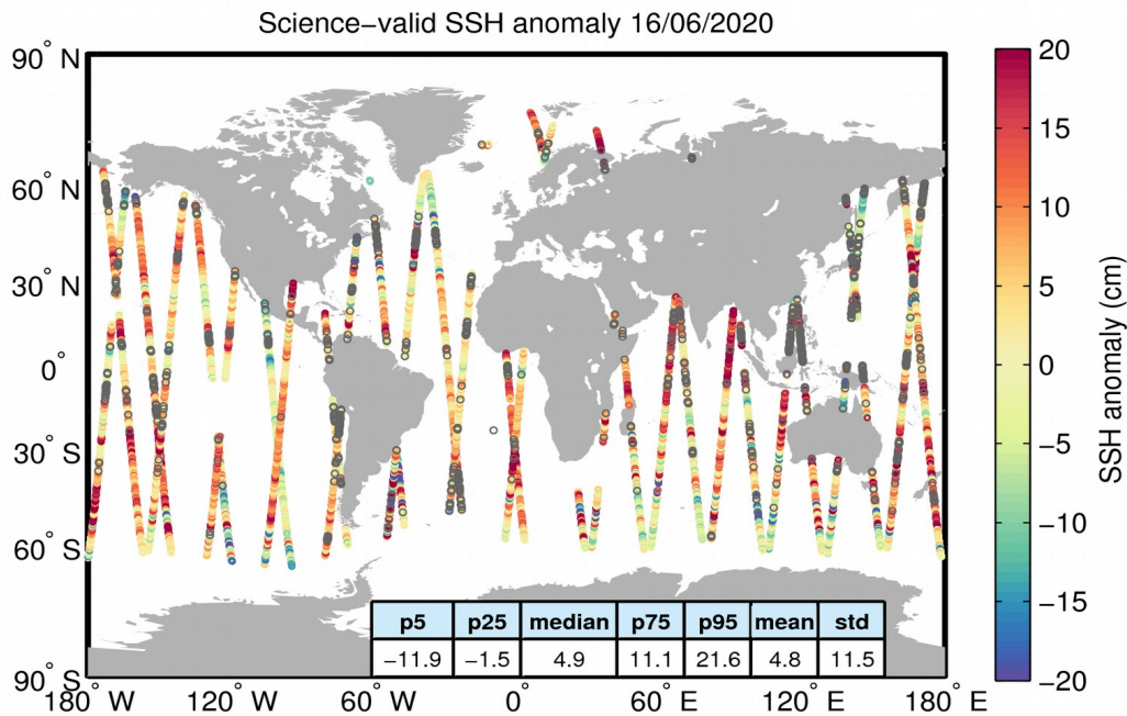
Figure 10. Geographical distribution of science-valid SSH anomaly data over oceans and lakes for 16/06/2020. The statistical values shown in the table refer to the SSH anomaly in cm and are calculated over all measurements shown in the figure. Gray circles denote records that have been rejected based on the editing criteria described in Table 2.
