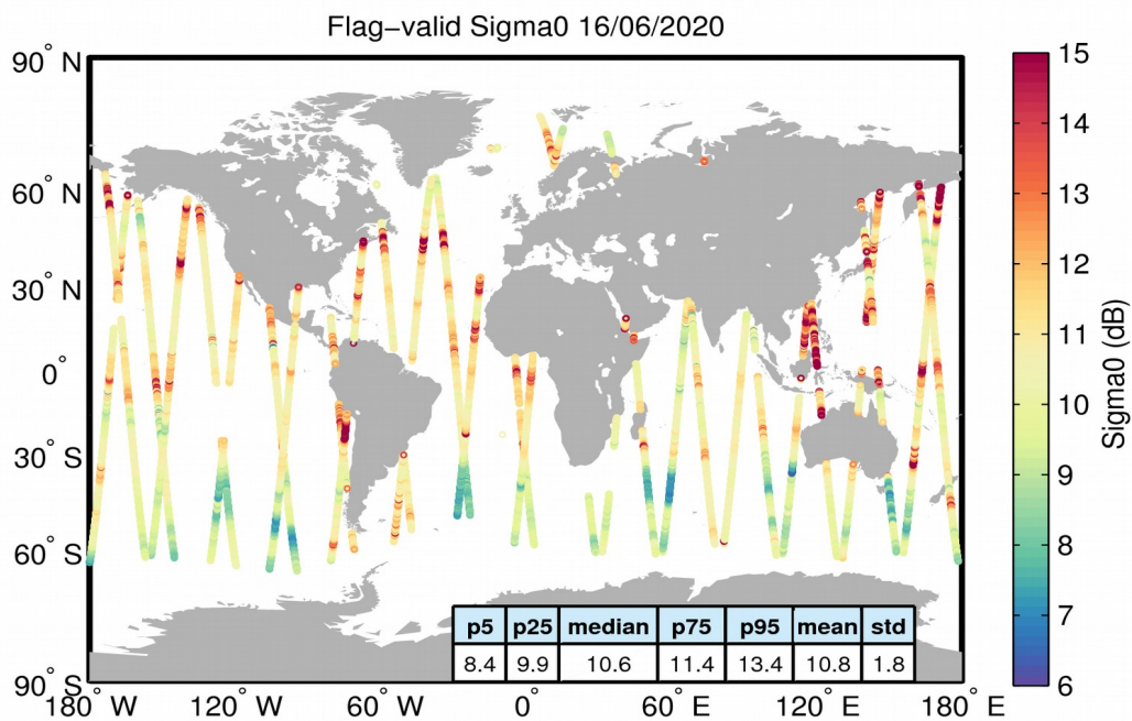
Figure 23. Geographical distribution of flag-valid sigma0 data over oceans and lakes for 16/06/2020. The statistical values shown in the table refer to the sigma0 in dB and are calculated over all measurements shown in the figure.
