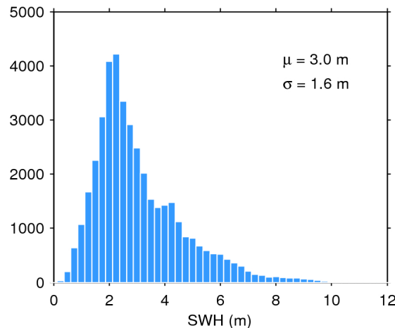
Figure 20. Histogram of science-valid SWH over oceans and lakes for 16/06/2020. The mean ( \mu ) and standard deviation ( \sigma ) are also shown. Note that values larger than 12 m are excluded from the histogram for the sake of readability but not from the computation of \mu and \sigma .
