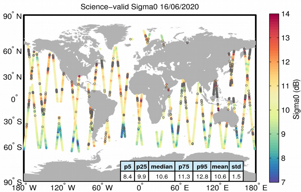
Figure 27. Geographical distribution of science-valid sigma0 data over oceans and lakes for 16/06/2020. The statistical values shown in the table refer to the sigma0 in dB and are calculated over all measurements shown in the figure. Gray circles denote records that have been rejected based on the editing criteria described in Table 4.
