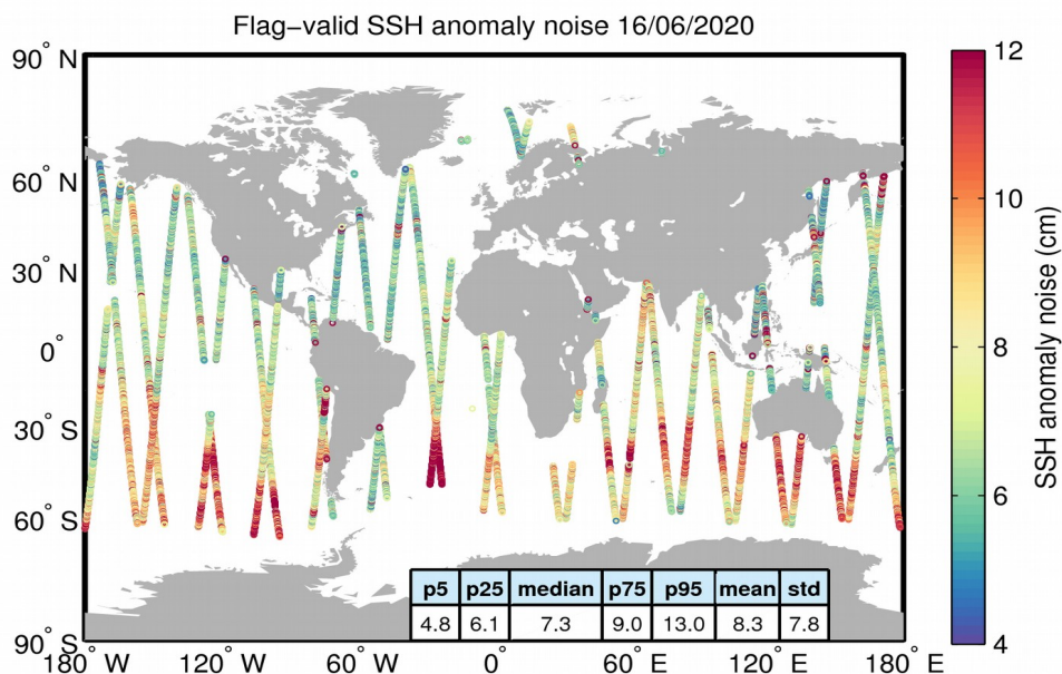
Figure 8. Geographical distribution of flag-valid 20-Hz SSH anomaly measurement noise over oceans and lakes for 16/06/2020. The statistical values shown in the table refer to the SSH anomaly noise and are calculated over all measurements shown in the figure.
