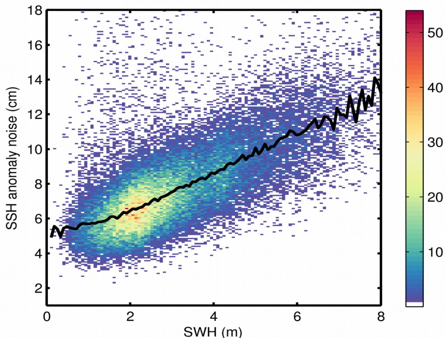
Figure 9. 2D histogram showing flag-valid SSH anomaly noise as a function of SWH for 16/06/2020. The black line denotes the median SSH anomaly noise as a function of SWH.
