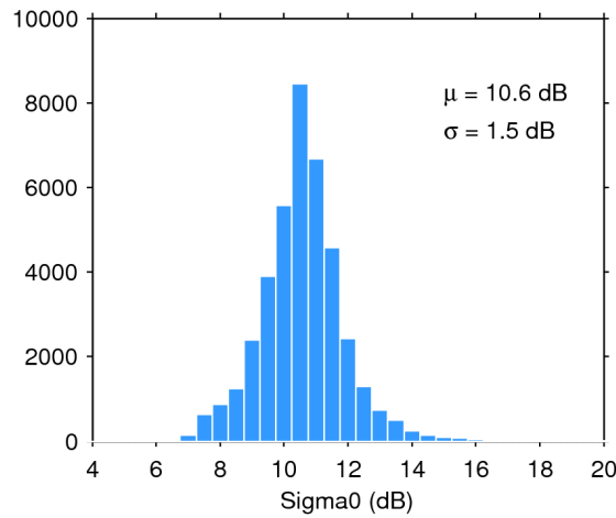
Figure 28. Histogram of science-valid sigma0 over oceans and lakes for 16/06/2020. The mean ( \mu ) and standard deviation ( \sigma ) are also shown. Note that values outside [4 20] dB are excluded from the histogram for the sake of readability but not from the computation of \mu and \sigma .
