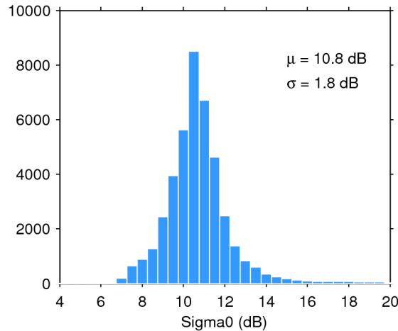
Figure 25. Histogram of flag-valid sigma0 over oceans and lakes for 16/06/2020. The mean ( \mu ) and standard deviation ( \sigma ) are also shown. Note that values outside [4 20] dB are excluded from the histogram for the sake of readability but not from the computation of \mu and \sigma .
